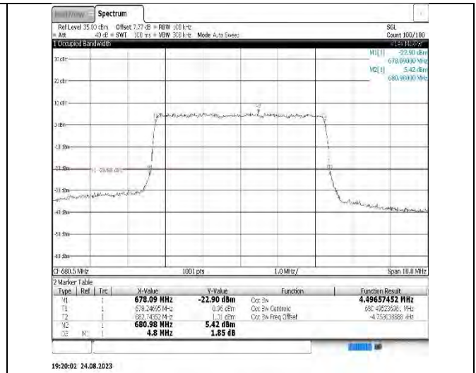
Band71-5MHz-16QAM-133147-25RB#0
