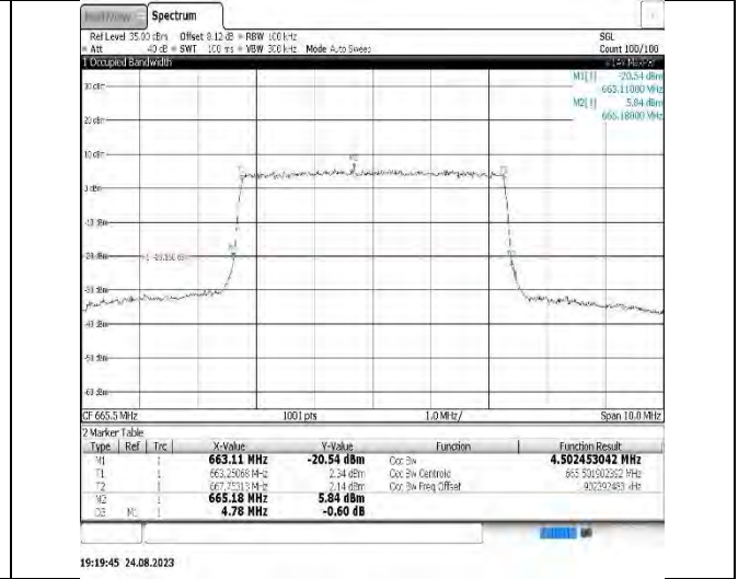
Band71-5MHz-16QAM-133447-25RB#0
