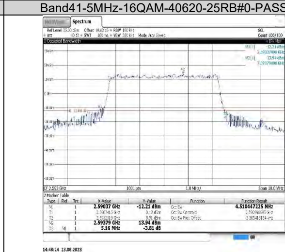
Band41-5MHz-16QAM-40620-25RB#0-PASS
