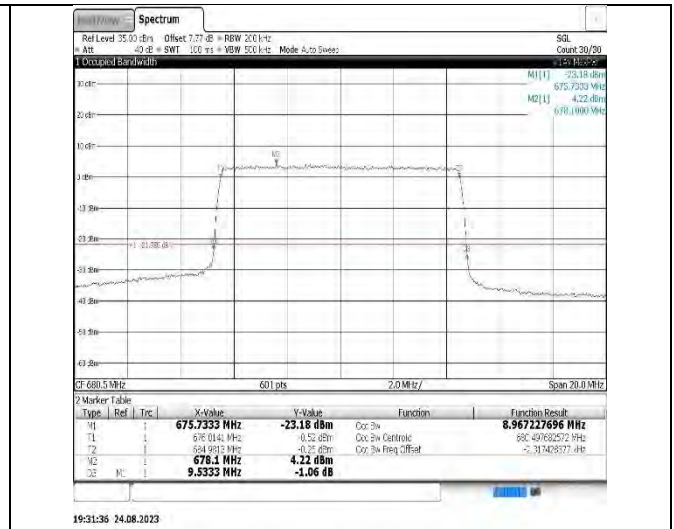
19:31:36 24.08.2023 Band71-10MHz-16QAM-133172-50RB#0
