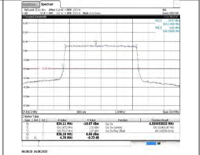
Band5-10MHz-16QAM-20525-50RB#0
