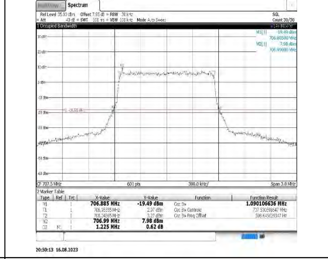
Band12-3MHz-16QAM-23095-15RB#0
