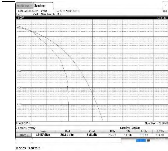
Band71-15MHz-16QAM-133397-1RB#0
