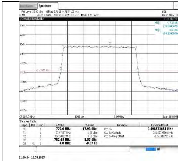
Band13-10MHz-QPSK-23230-50RB#0
