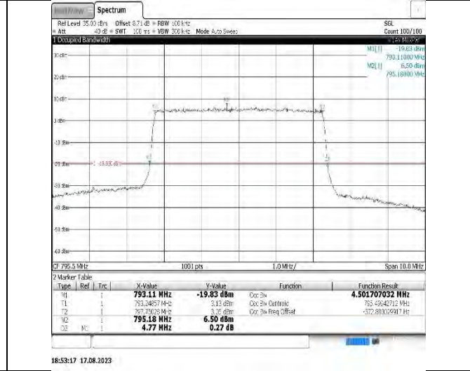
Band14-10MHz-16QAM-23355-50RB#0
