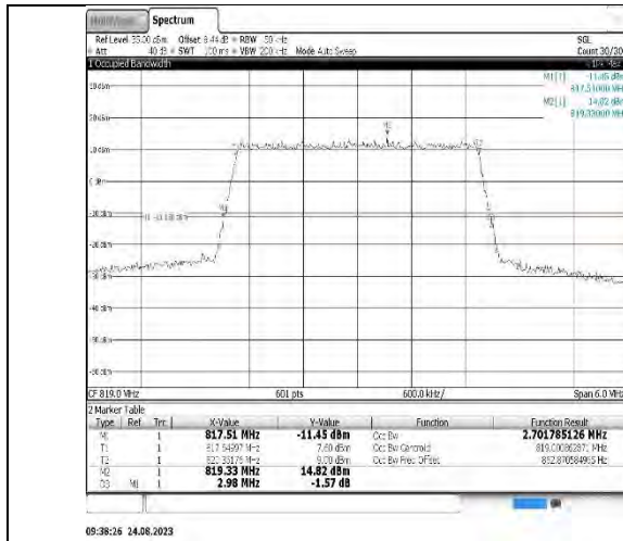
B26(814-824)-5MHz-QPSK-26740-25RB#0-PASS
