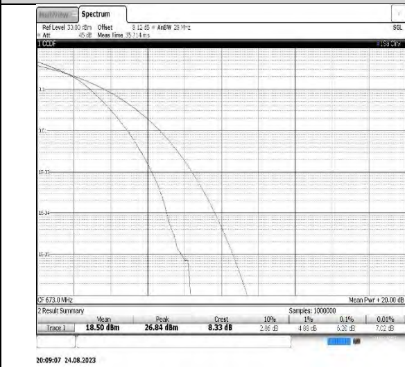
Band71-20MHz-16QAM-133322-100RB#0
