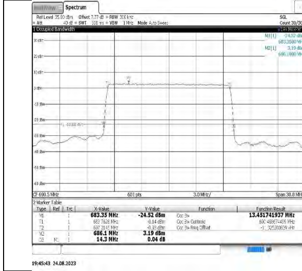
Band71-15MHz-QPSK-133297-75RB#0
