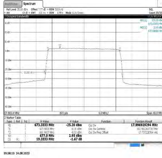
Band71-20MHz-16QAM-133322-100RB#0
