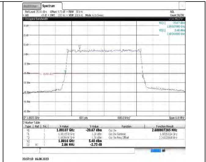
Band25-5MHz-16QAM-26365-25RB#0
