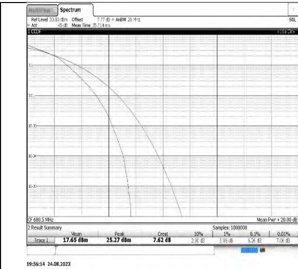
Band71-15MHz-16QAM-133397-75RB#0
