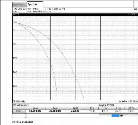
Band71-20MHz-16QAM-133222-100RB#0
