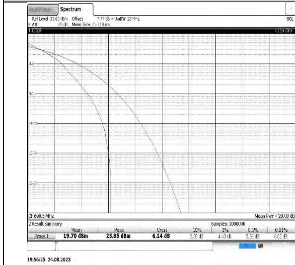
Band71-15MHz-16QAM-133197-1RB#0
