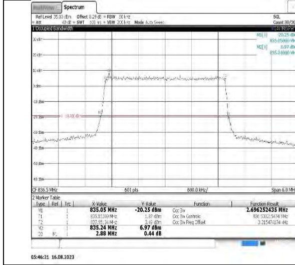
Band5-5MHz-QPSK-20525-25RB#0
