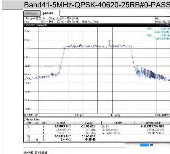
Band41-5MHz-QPSK-40620-25RB#0-PASS
