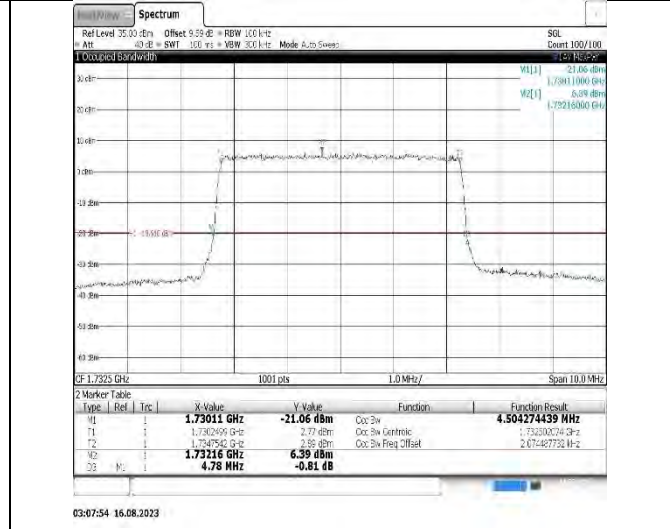
Band4-10MHz-16QAM-20175-50RB#0
