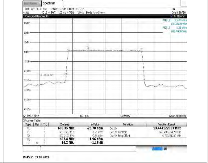
Band71-15MHz-16QAM-133397-75RB#0
