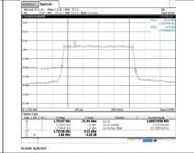
Band4-5MHz-16QAM-20175-25RB#0
