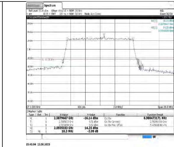
Band41-15MHz-16QAM-40620-75RB#0-PASS
