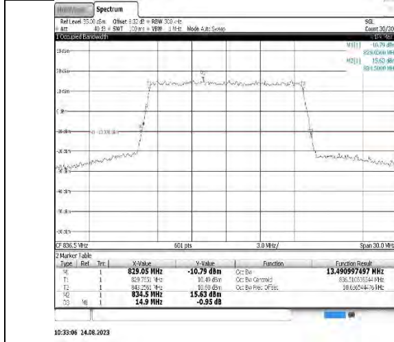
B26(824-849)-15MHz-QPSK-26915-75RB#0-PASS
