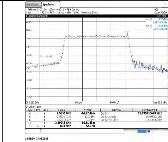
Band41-20MHz-16QAM-40620-100RB#0-PASS
