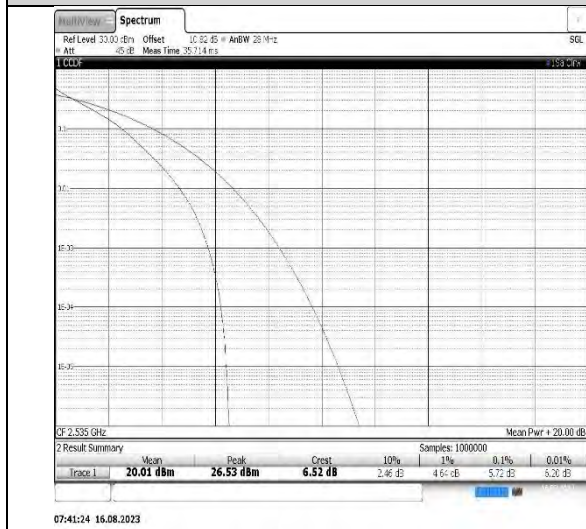
Band7-10MHz-QPSK-21100-50RB#0
