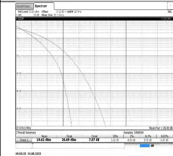
Band71-15MHz-QPSK-133297-75RB#0
