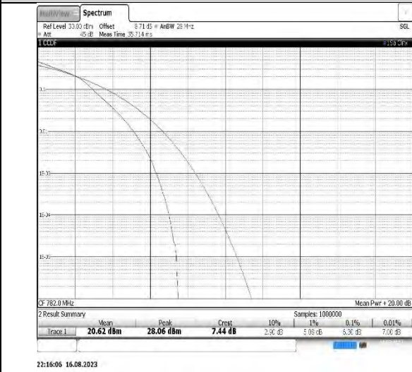
Band 13-10MHz-16QAM-23230-50RB#0
