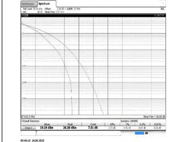
B26(814-824)-3MHz-QPSK-26740-15RB#0-PASS
