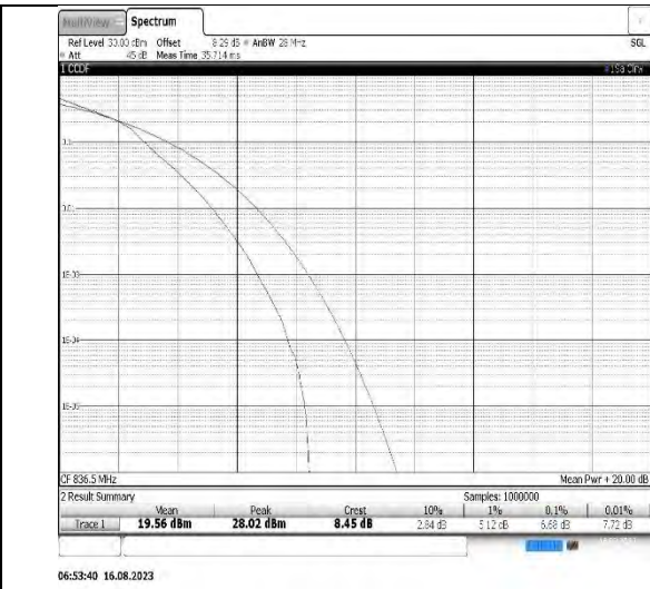
Band5-10MHz-16QAM-20525-50RB#0
