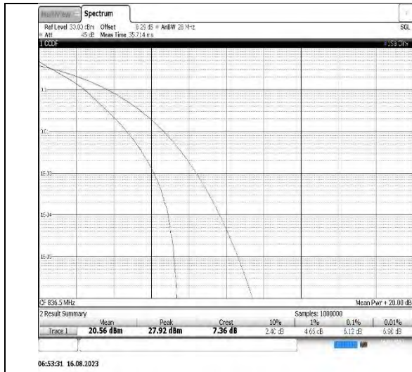
Band5-10MHz-QPSK-20525-50RB#0
