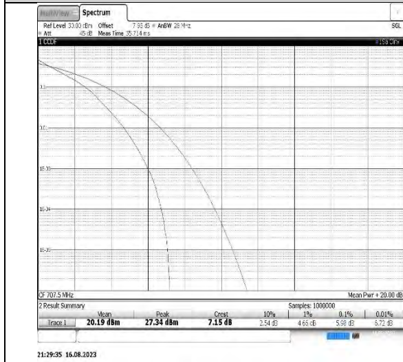
Band12-5MHz-QPSK-23095-25RB#0
