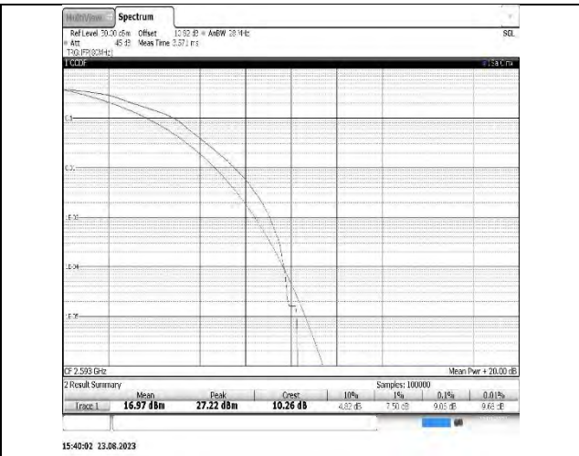
Band41-10MHz-16QAM-40620-50RB#0-PASS
