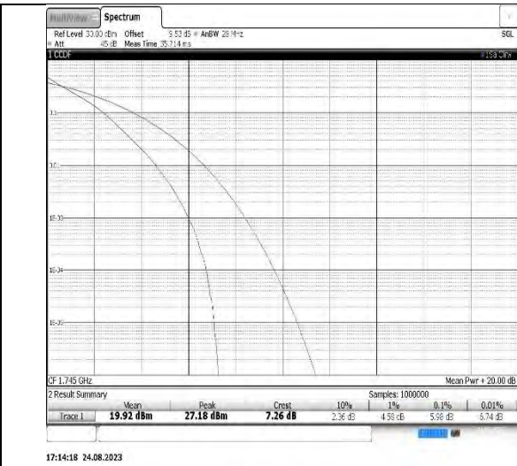
Band66-5MHz-16QAM-132322-25RB#0
