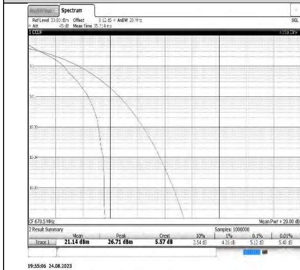
Band71-15MHz-QPSK-133297-1RB#0
