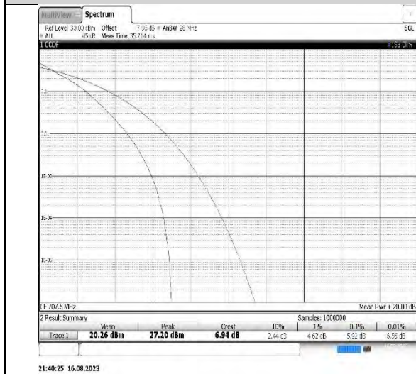
Band12-10MHz-QPSK-23095-50RB#0
