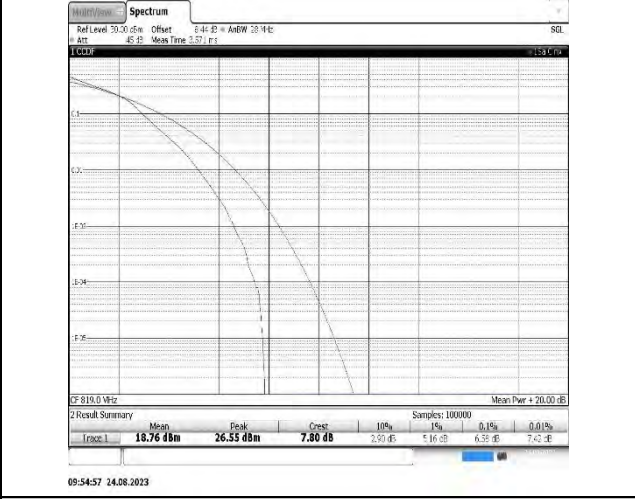
B26(814-824)-10MHz-16QAM-26740-50RB#0-PASS
