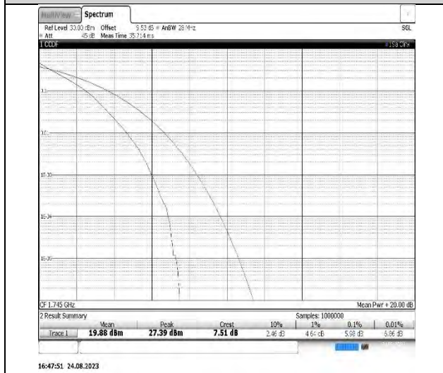
Band66-5MHz-QPSK-132322-1RB#0
