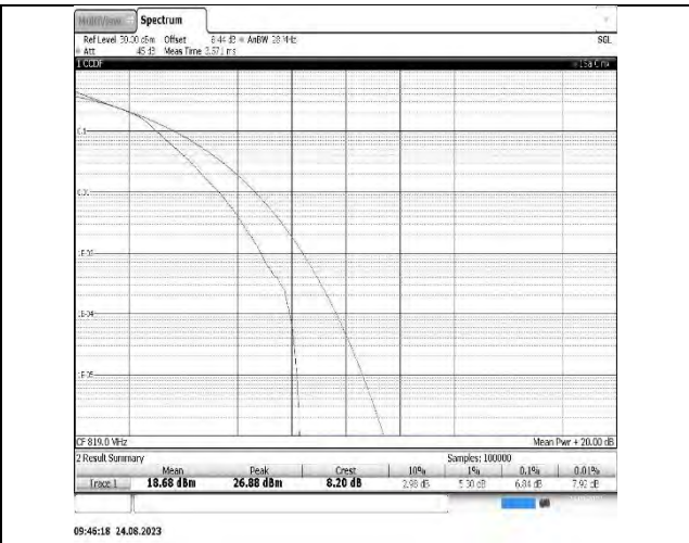
B26(814-824)-3MHz-16QAM-26775-15RB#0-PASS
