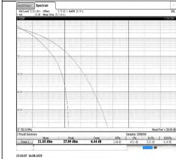
Band 13-10MHz-QPSK-23230-50RB#0
