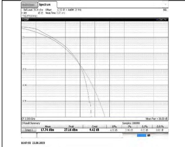
Band41-15MHz-QPSK-40620-75RB#0-PASS
