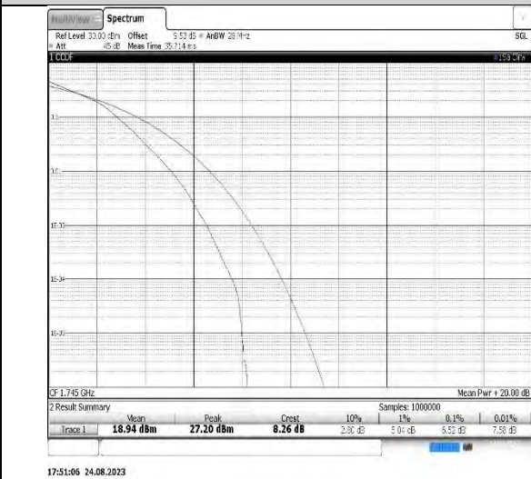
Band66-15MHz-16QAM-132322-75RB#0
