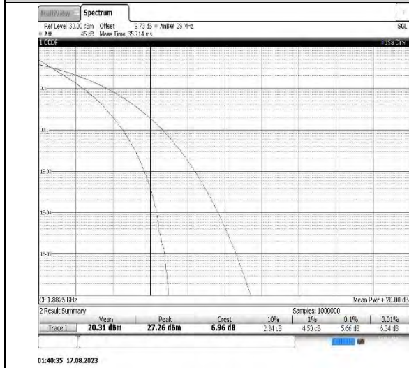
Band25-15MHz-QPSK-26365-75RB#0
