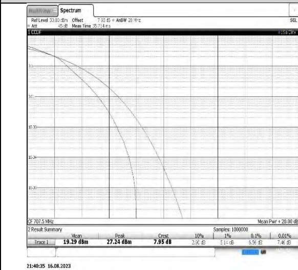
Band12-10MHz-16QAM-23095-50RB#0
