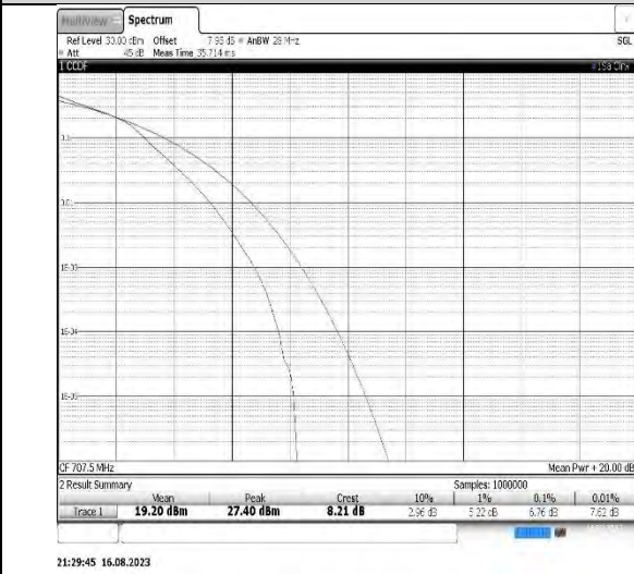
Band12-5MHz-16QAM-23095-25RB#0
