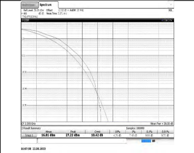
Band41-15MHz-16QAM-40620-75RB#0-PASS
