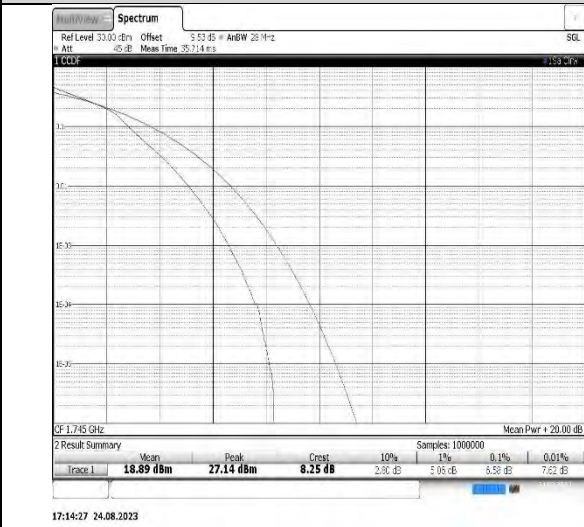
Band66-10MHz-16QAM-132322-50RB#0
