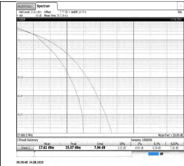
Band71-5MHz-16QAM-133447-25RB#0
