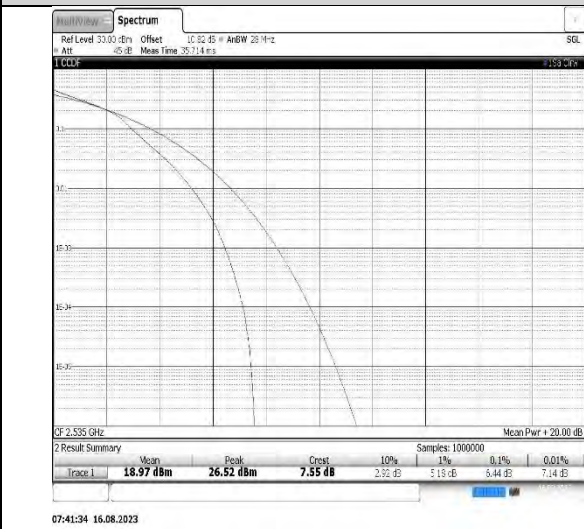
Band7-10MHz-16QAM-21100-50RB#0
