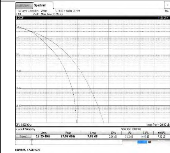
Band25-15MHz-16QAM-26365-75RB#0
