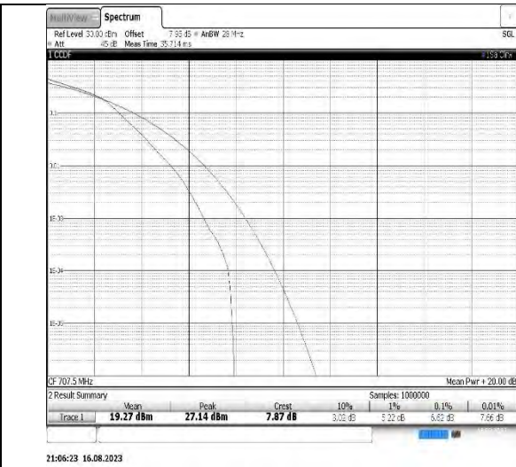
Band12-3MHz-16QAM-23095-15RB#0
