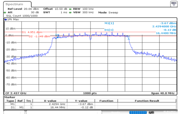
n20_2437MHz_Chain 0
