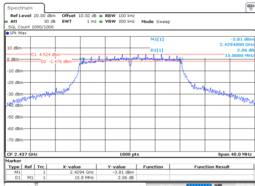
g_2437MHz_Chain 0
