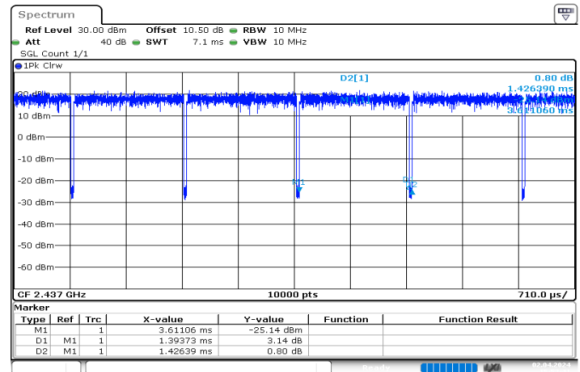
g_2437MHz_Chain 0
