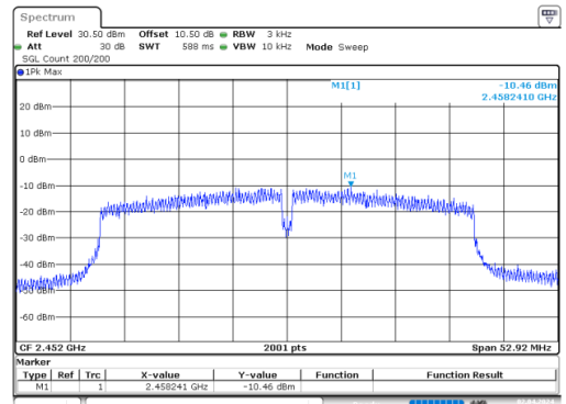
N40_2452MHz_Chain 0
