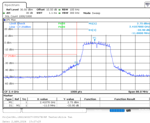
g_2412MHz_Chain 0
