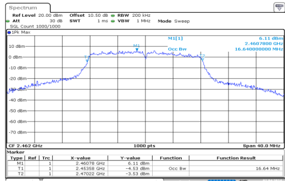
g_2462MHz_Chain 0
