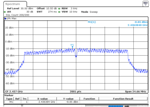
n20_2437MHz_Chain 0
