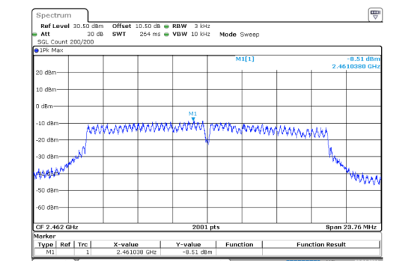
g_2462MHz_Chain 0
