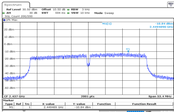
N40_2437MHz_Chain 0
