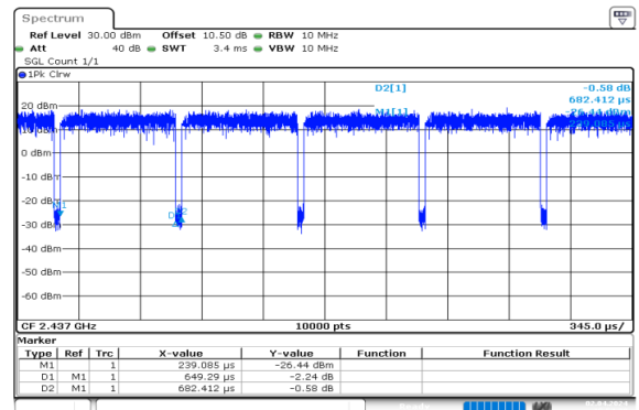
N40_2437MHz_Chain 0
