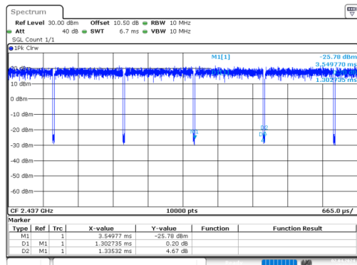
n20_2437MHz_Chain 0
