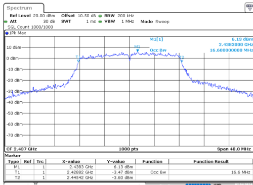
g_2437MHz_Chain 0
