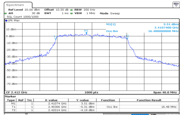
g_2412MHz_Chain 0
