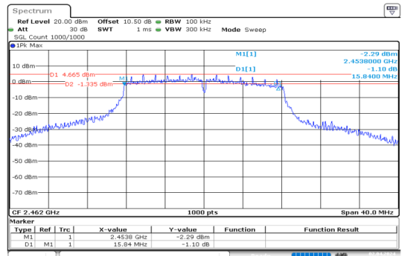
g_2462MHz_Chain 0
