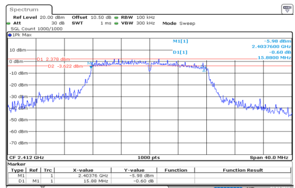
g_2412MHz_Chain 0
