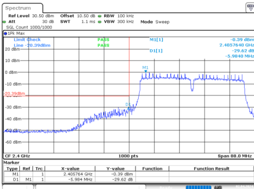
N40_2412MHz_Chain 0
