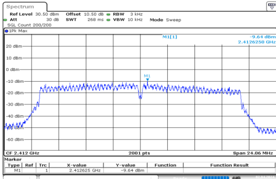
n20_2412MHz_Chain 0
