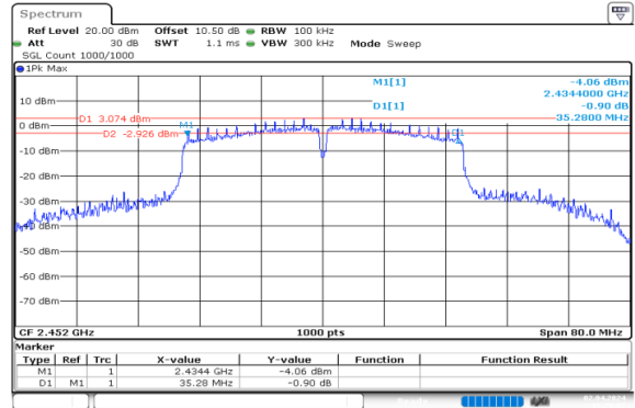
N40_2452MHz_Chain 0
