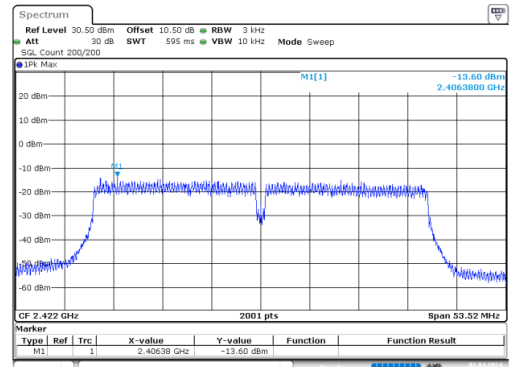
N40_2422MHz_Chain 0
