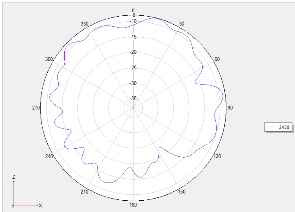
chart 7 Phi 0 2D
