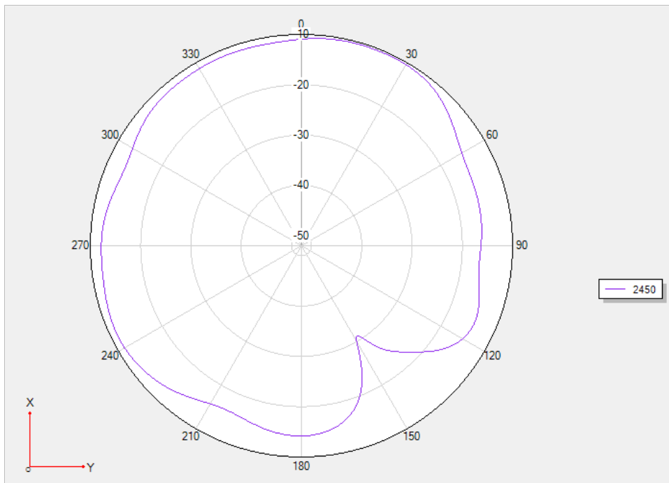
chart 9 Theta 90 2D
