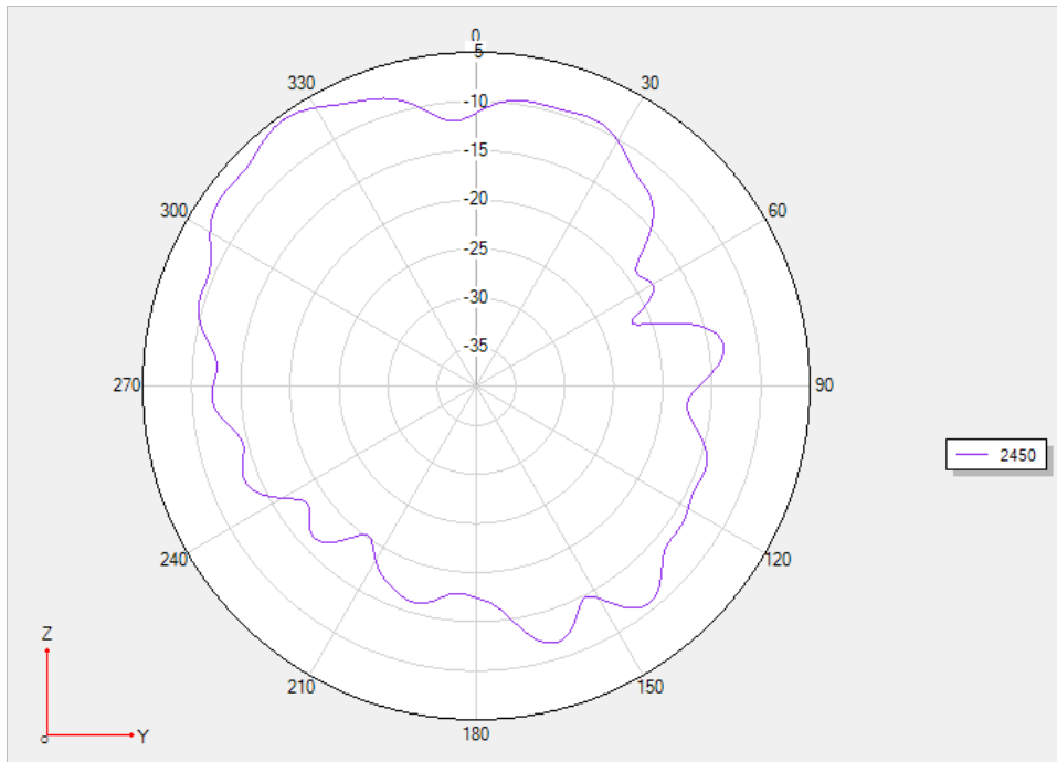
chart 8 Phi 90 2D
