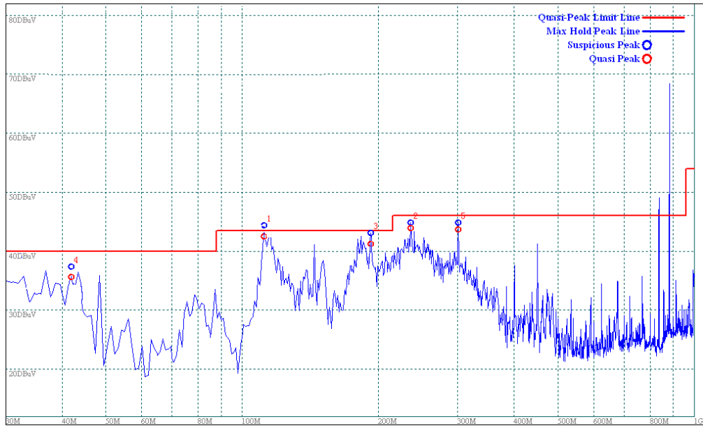
(Plot B: Test Antenna Horizontal)
