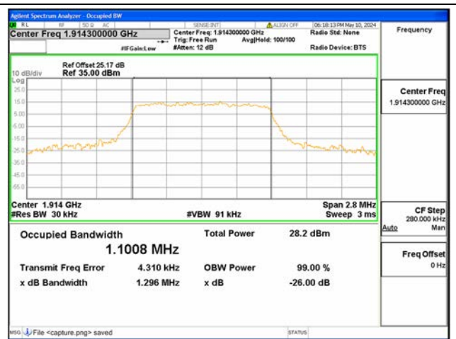
B25 / 1.4MHz / 16QAM/ High CH
