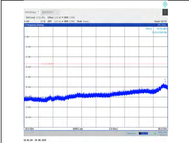
11ax80MIMO-Ant7-7025-10000~40000
