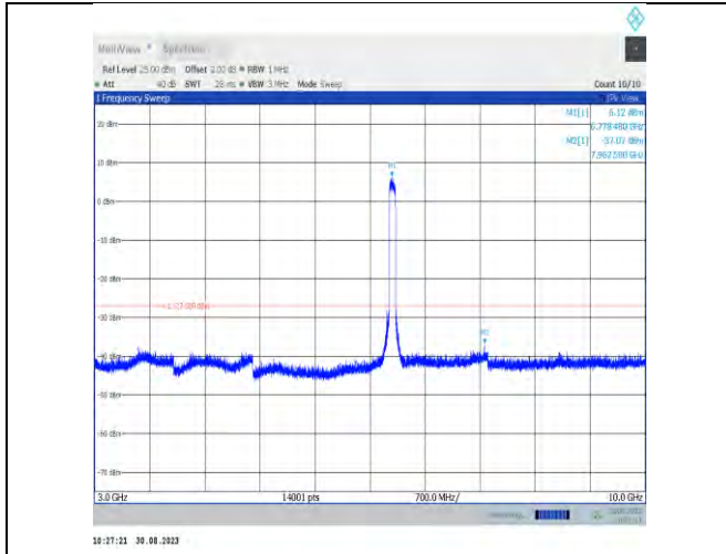
11ax80MIMO-Ant9-6785-3000~10000
