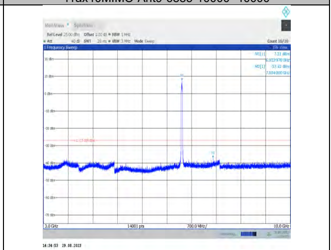
11ax40MIMO-Ant7-6925-3000~10000
