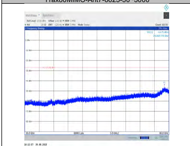
11ax80MIMO-Ant7-6625-10000~40000
