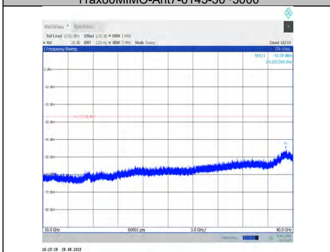
11ax80MIMO-Ant7-6145-10000~40000
