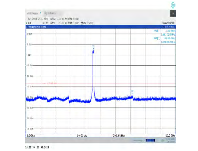
11ax80MIMO-Ant9-6145-3000~10000
