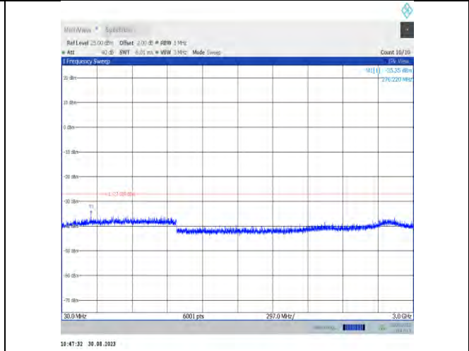
11ax80MIMO-Ant9-7025-30~3000
