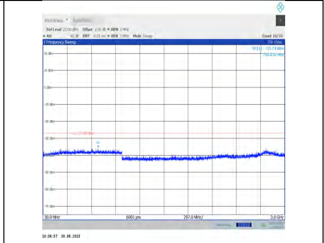
11ax80MIMO-Ant9-6865-30~3000
