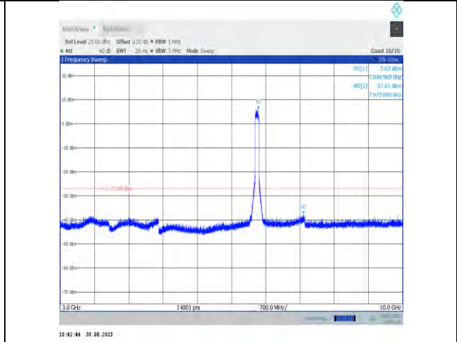
11ax80MIMO-Ant7-7025-3000~10000
