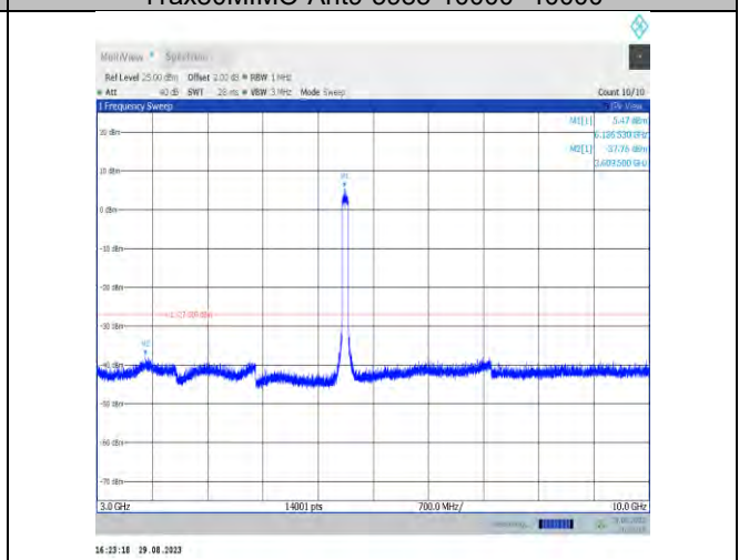
11ax80MIMO-Ant7-6145-3000~10000
