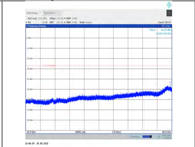
11ax80MIMO-Ant9-6945-10000~40000
