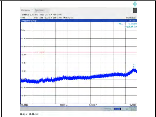
11ax80MIMO-Ant9-5985-10000~40000
