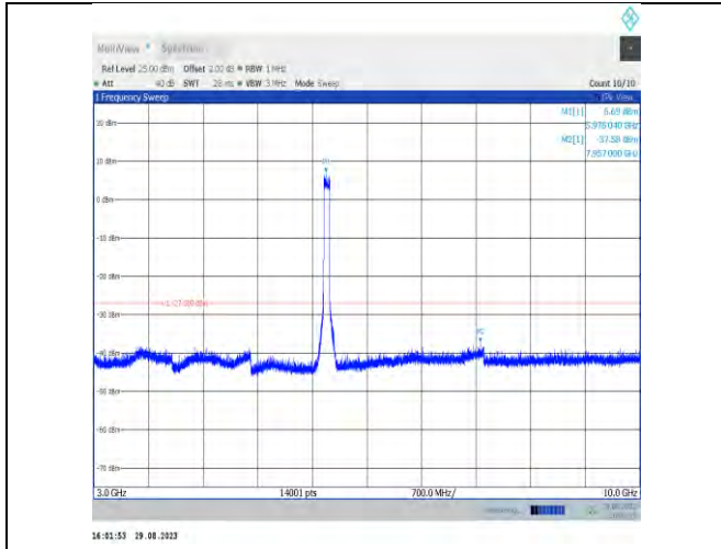
11ax80MIMO-Ant9-5985-3000~10000
