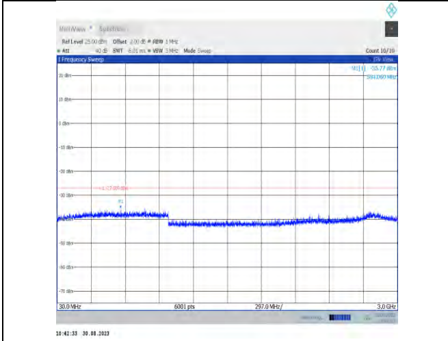
11ax80MIMO-Ant7-7025-30~3000
