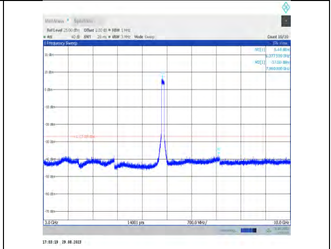
11ax80MIMO-Ant7-6385-3000~10000
