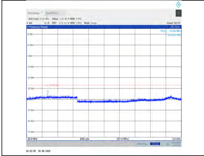
11ax80MIMO-Ant7-6865-30~3000
