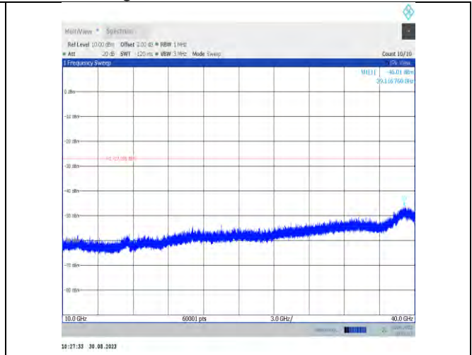
11ax80MIMO-Ant9-6785-10000~40000
