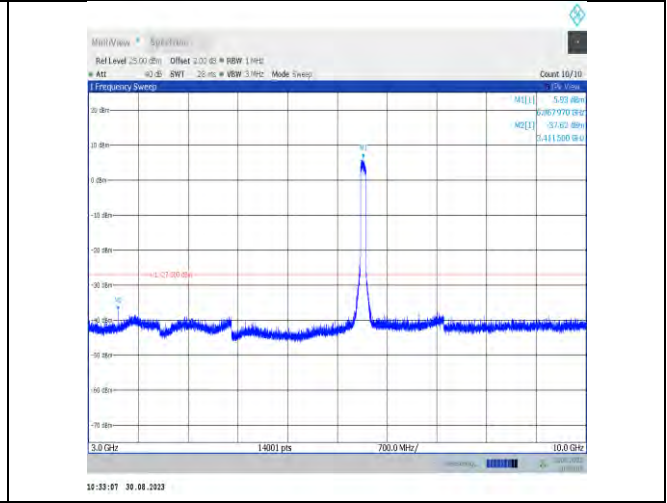
11ax80MIMO-Ant7-6865-3000~10000
