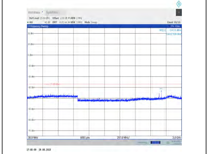
11ax80MIMO-Ant9-6385-30~3000
