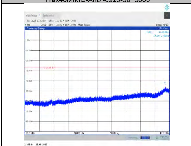
11ax40MIMO-Ant7-6925-10000~40000
