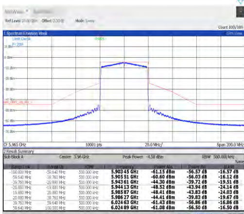
NTNV-11ax40MIMO-Ant7-5965-PASS
