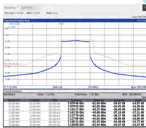
NTNV-11ax20MIMO-Ant9-7115-PASS
