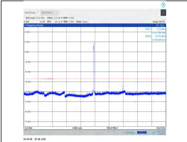
11ax40MIMO-Ant9-6445-3000~10000
