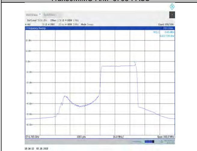
11ax80MIMO-Ant7-6785-PASS
