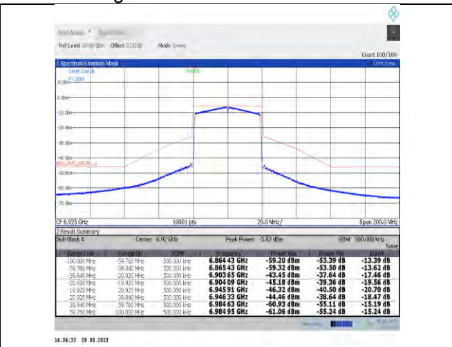
NTNV-11ax40MIMO-Ant9-6925-PASS
