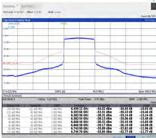
NTVN-11ax80MIMO-Ant7-6625-PASS
