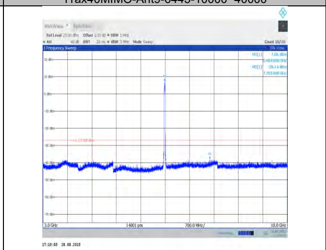
11ax40MIMO-Ant7-6485-3000~10000
