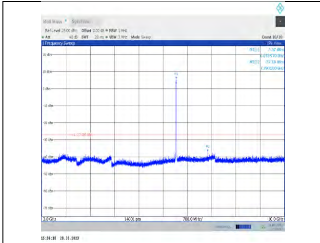
11ax20MIMO-Ant9-6875-3000~10000
