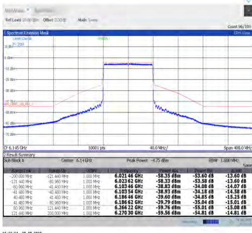
NTVN-11ax80MIMO-Ant7-6145-PASS
