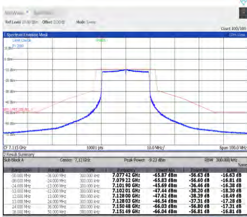
NTNV-11ax20MIMO-Ant7-7115-PASS
