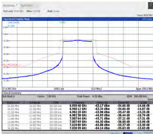
NTNV-11ax20MIMO-Ant7-6995-PASS
