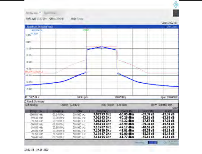
NTNV-11ax40MIMO-Ant9-7085-PASS
