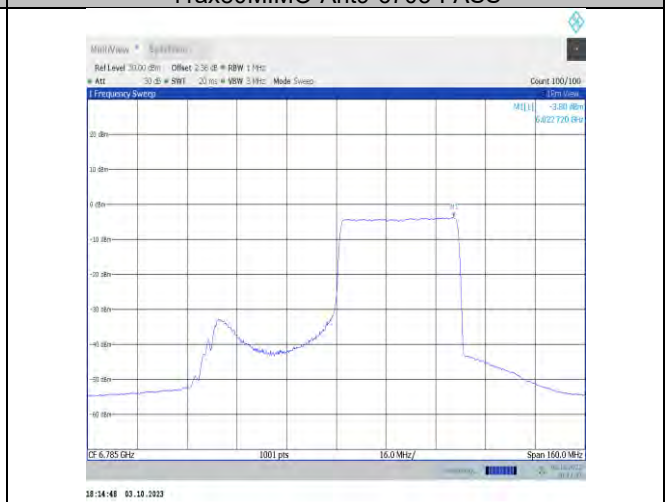
11ax80MIMO-Ant9-6785-PASS
