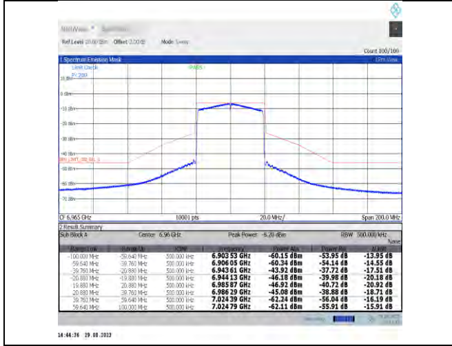
NTNV-11ax40MIMO-Ant7-6965-PASS
