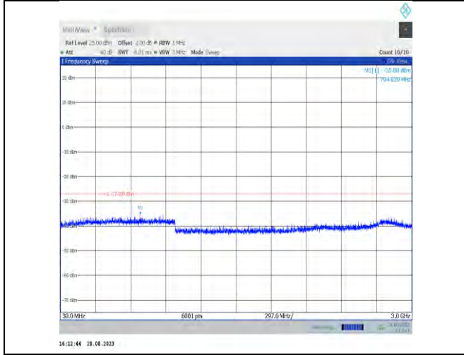
11ax40MIMO-Ant7-5965-30~3000
