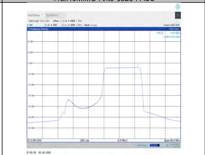
11x40MIMO-Ant9-6965-PASS
