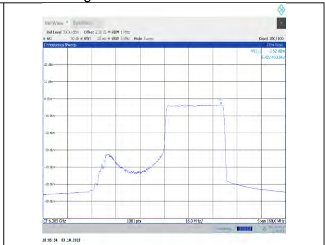
11ax80MIMO-Ant9-6385-PASS
