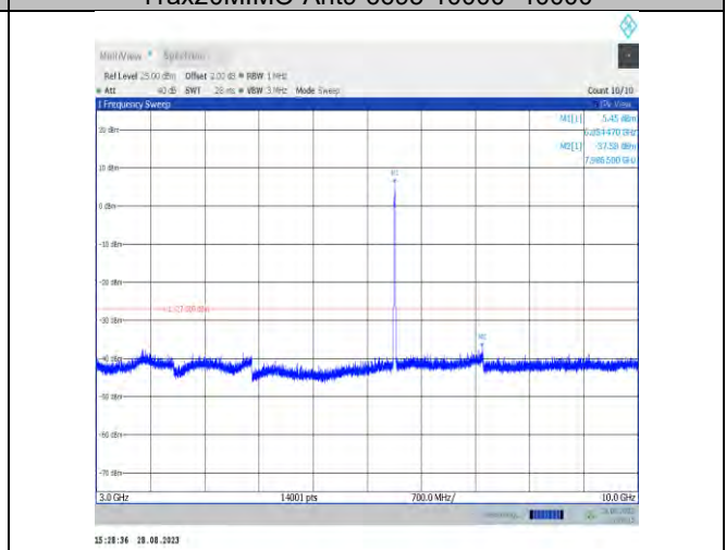
11ax20MIMO-Ant7-6855-3000~10000
