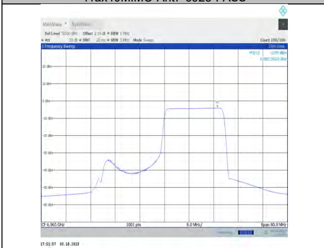
11x40MIMO-Ant7-6965-PASS
