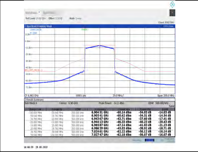
NTNV-11ax40MIMO-Ant9-6965-PASS
