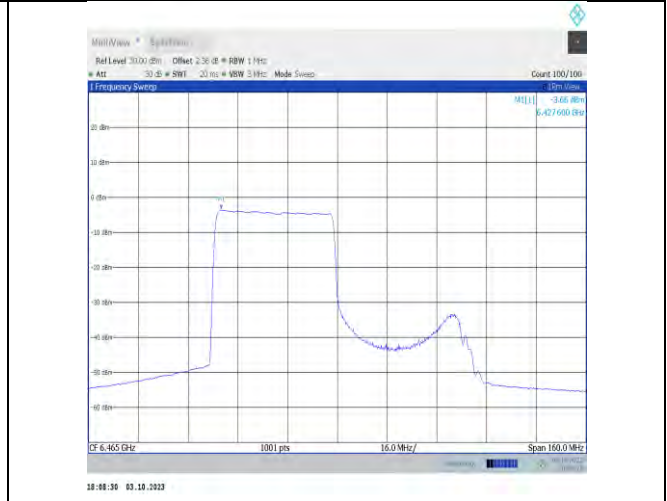
11ax80MIMO-Ant9-6465-PASS
