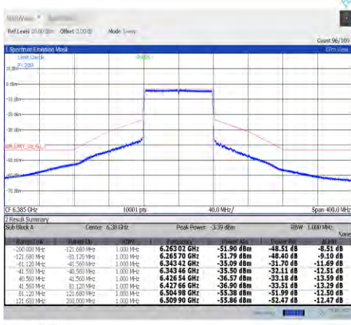
NTVN-11ax80MIMO-Ant7-6385-PASS
