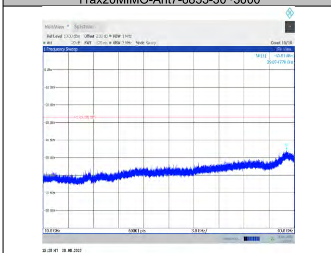
11ax20MIMO-Ant7-6855-10000~40000
