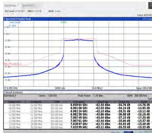
NTNV-11ax20MIMO-Ant9-6995-PASS
