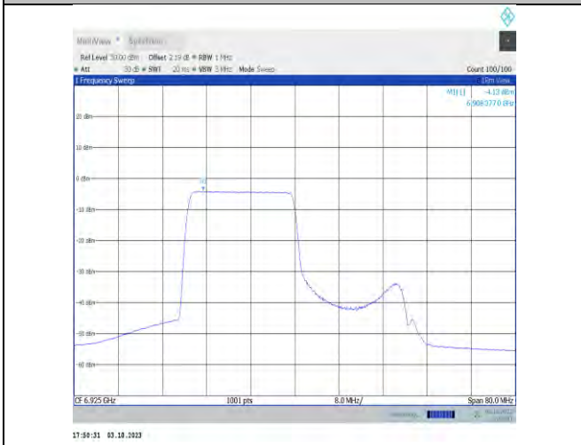
11x40MIMO-Ant7-6925-PASS
