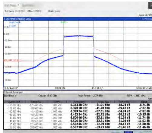
NTVN-11ax80MIMO-Ant9-6465-PASS
