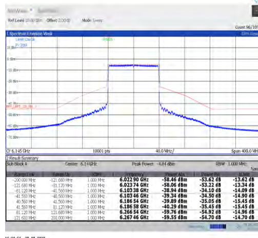
NTVN-11ax80MIMO-Ant9-6145-PASS
