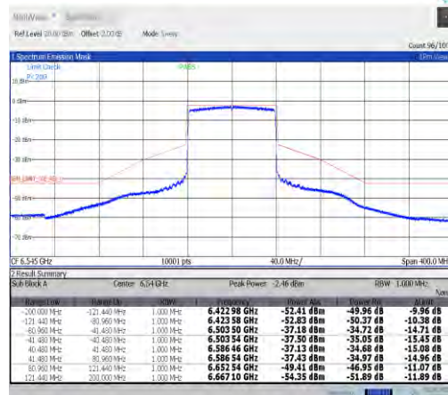
NTVN-11ax80MIMO-Ant9-6545-PASS
