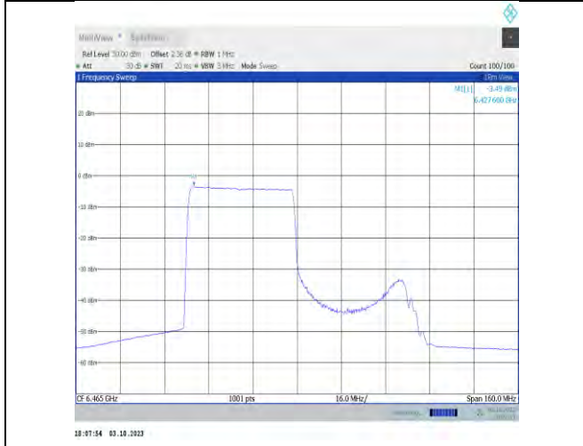
11ax80MIMO-Ant7-6465-PASS
