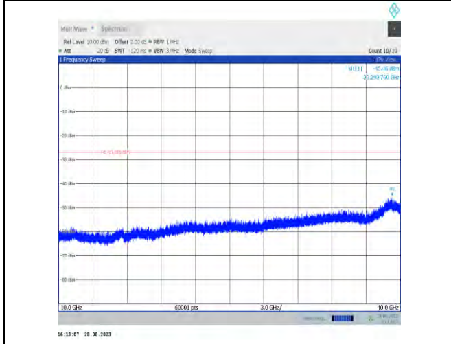
11ax40MIMO-Ant7-5965-10000~40000
