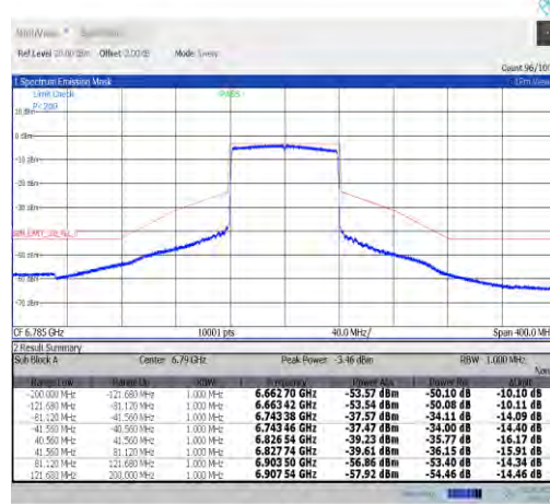
NTVN-11ax80MIMO-Ant9-6785-PASS
