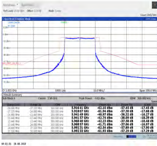
NTVN-11ax20MIMO-Ant7-5955-PASS
