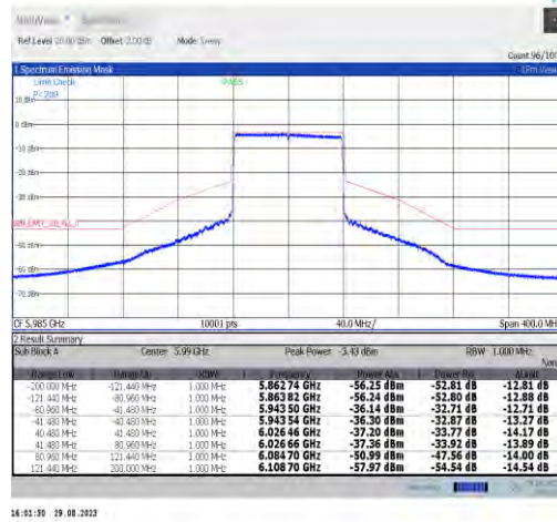
NTVN-11ax80MIMO-Ant9-5985-PASS
