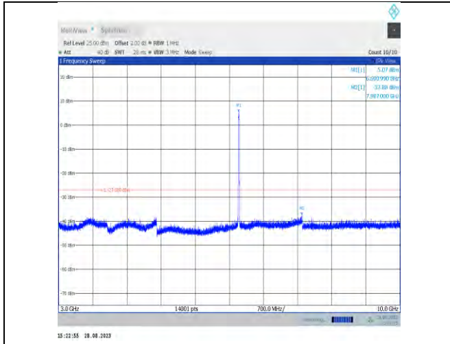
11ax20MIMO-Ant9-6695-3000~10000
