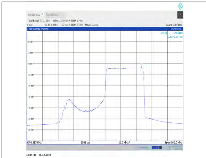
11ax80MIMO-Ant7-6385-PASS
