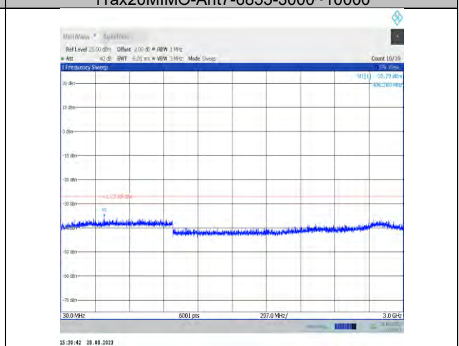
11ax20MIMO-Ant9-6855-30~3000
