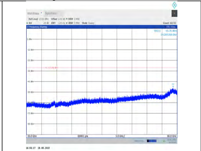
11ax40MIMO-Ant9-6445-10000~40000
