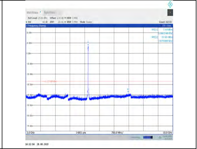
11ax40MIMO-Ant7-5965-3000~10000
