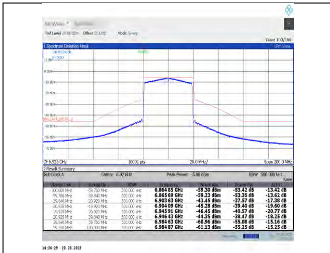
NTNV-11ax40MIMO-Ant7-6925-PASS
