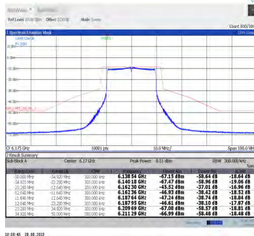
NTVN-11ax20MIMO-Ant9-6175-PASS
