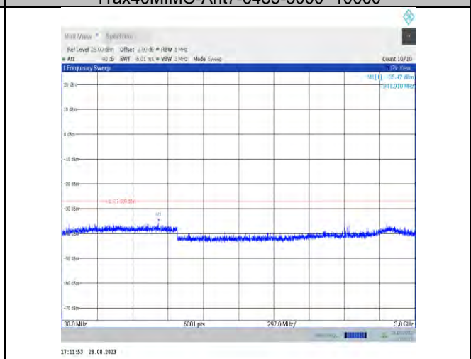
11ax40MIMO-Ant9-6485-30~3000
