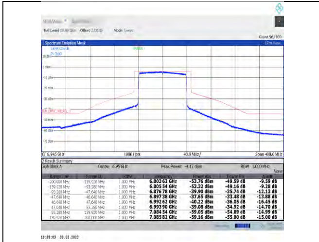
NTVN-11ax80MIMO-Ant7-6945-PASS
