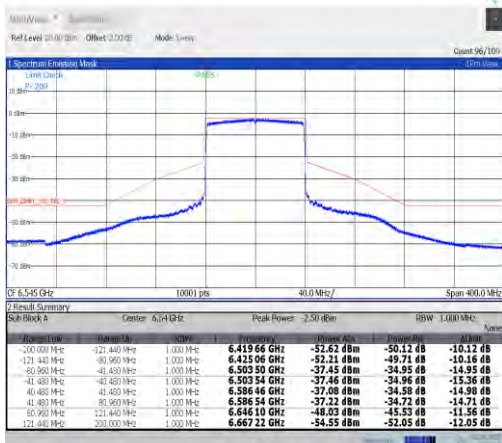
NTVN-11ax80MIMO-Ant7-6545-PASS
