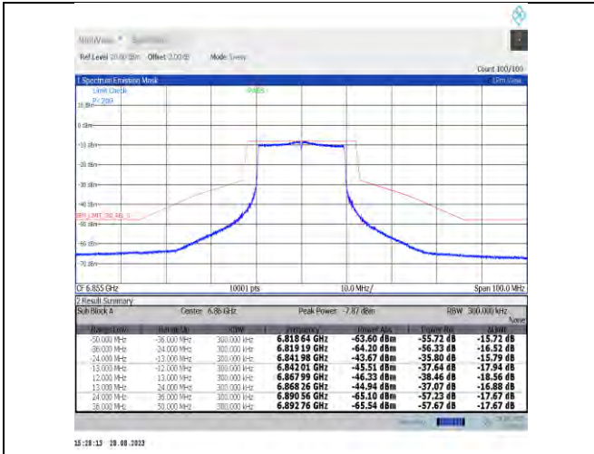
NTNV-11ax20MIMO-Ant7-6855-PASS
