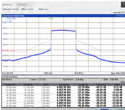
NTVN-11ax80MIMO-Ant7-6705-PASS
