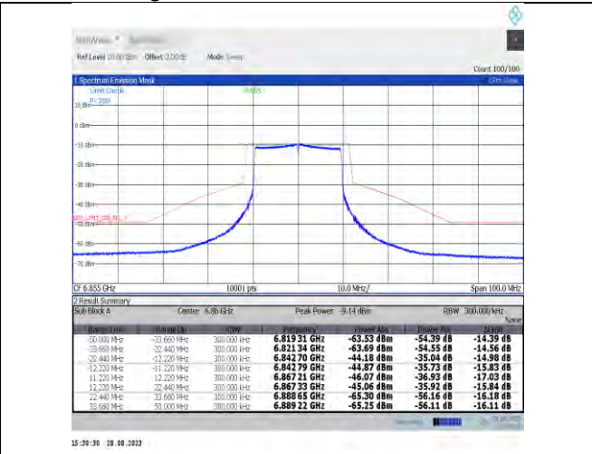
NTNV-11ax20MIMO-Ant9-6855-PASS
