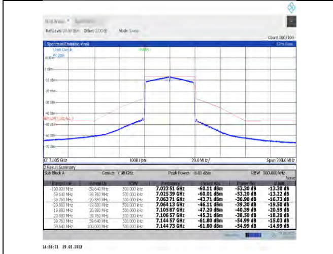
NTNV-11ax40MIMO-Ant7-7085-PASS
