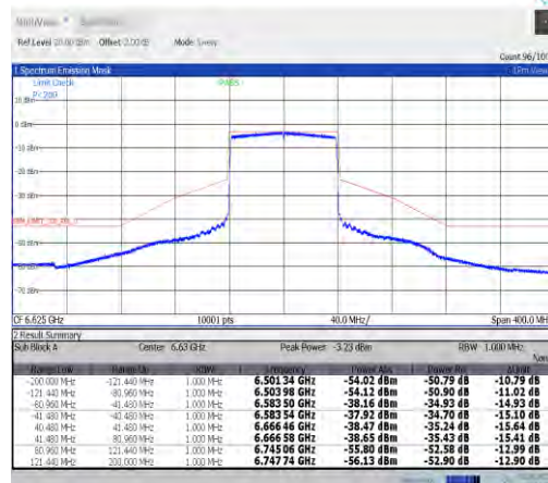
NTVN-11ax80MIMO-Ant9-6625-PASS
