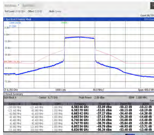
NTVN-11ax80MIMO-Ant9-6705-PASS
