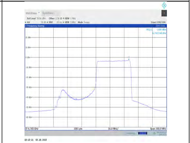
11ax80MIMO-Ant9-6705-PASS
