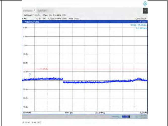
11ax40MIMO-Ant9-5965-30~3000
