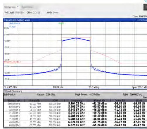
NTNV-11ax40MIMO-Ant9-5965-PASS
