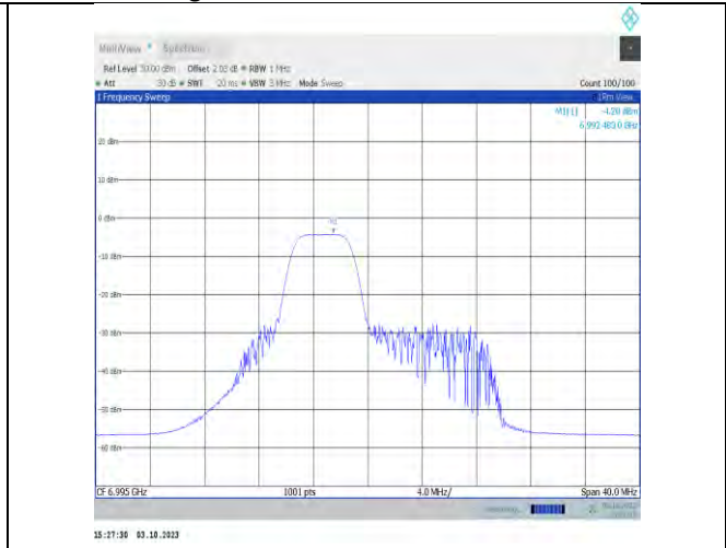
11x20MIMO-Ant7-6995-PASS
