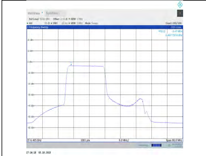
11x40MIMO-Ant7-6485-PASS
