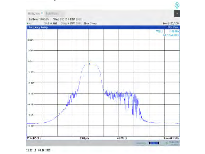
11ax20MIMO-Ant7-6475-PASS
