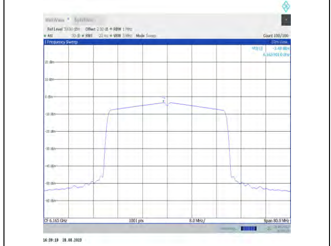
11x40MIMO-Ant9-6165-PASS
