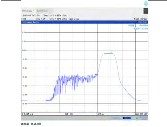
11ax20MIMO-Ant9-6515-PASS
