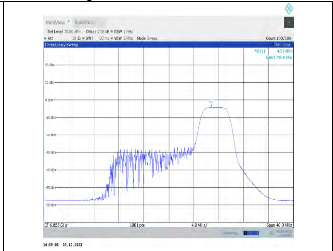
11ax20MIMO-Ant7-6855-PASS
