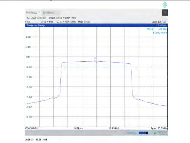
11ax80MIMO-Ant9-6785-PASS
