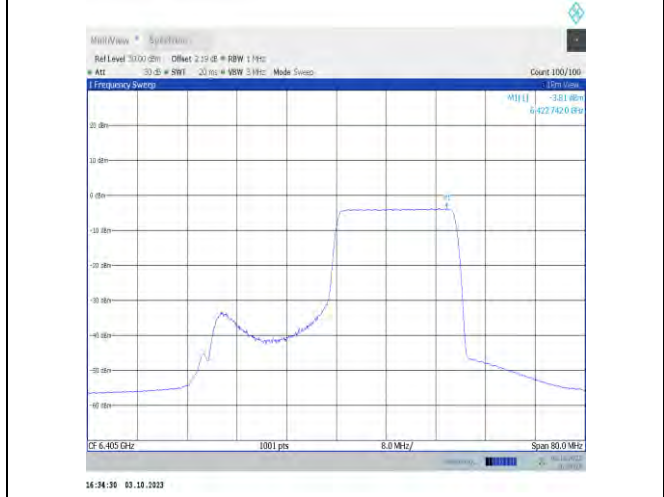
11x40MIMO-Ant9-6405-PASS
