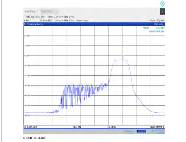
11ax20MIMO-Ant9-6855-PASS
