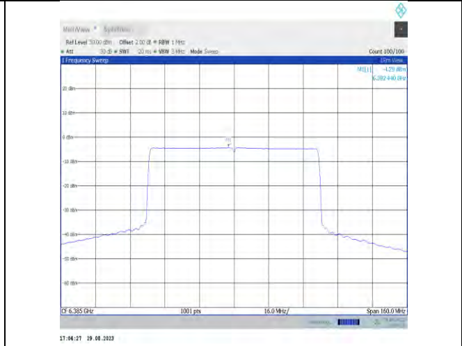
11ax80MIMO-Ant9-6385-PASS
