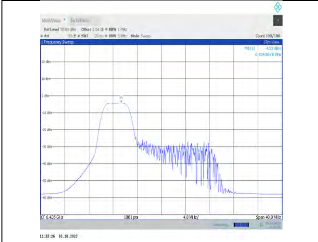
11x20MIMO-Ant9-6435-PASS
