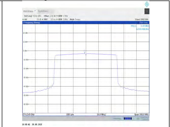
11ax80MIMO-Ant9-6545-PASS
