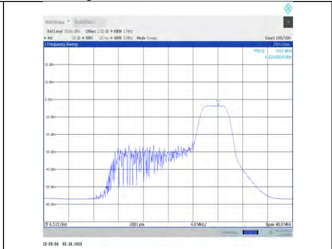
11ax20MIMO-Ant7-6515-PASS
