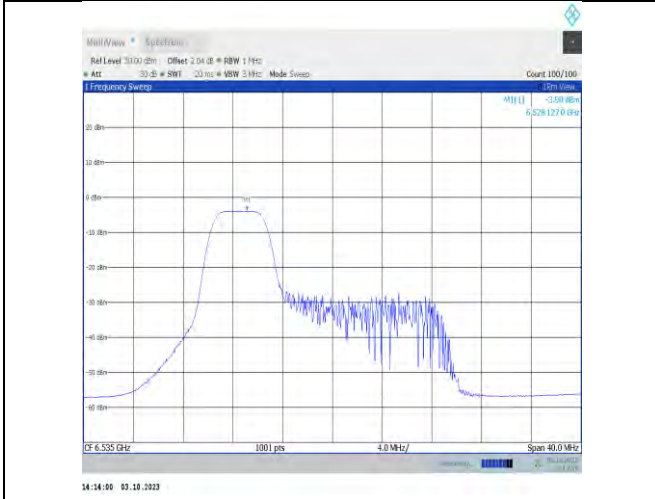
11x20MIMO-Ant9-6535-PASS
