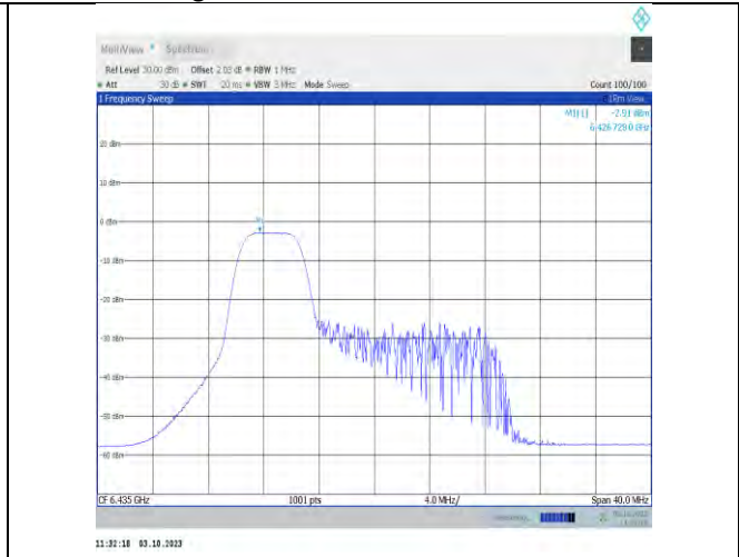
11x20MIMO-Ant7-6435-PASS
