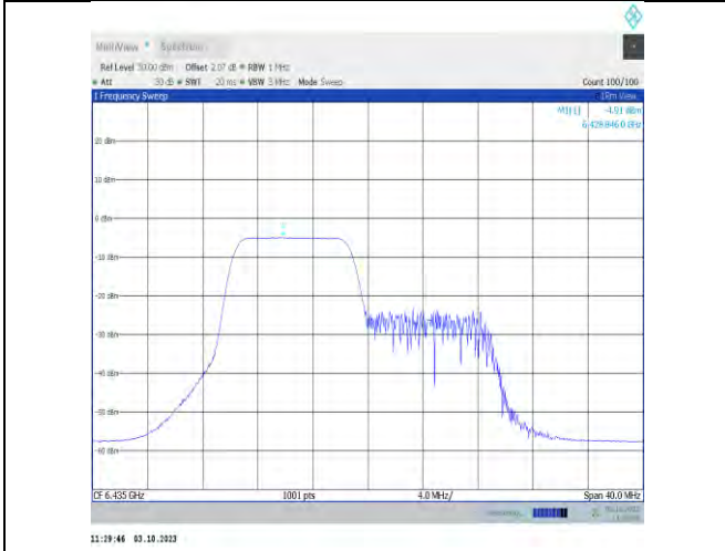
11x20MIMO-Ant7-6435-PASS
