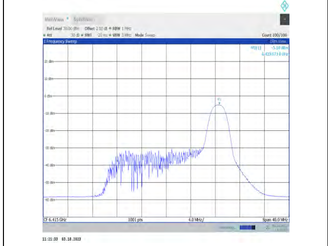
11ax20MIMO-Ant9-6415-PASS
