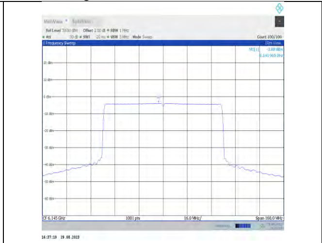
11ax80MIMO-Ant9-6145-PASS
