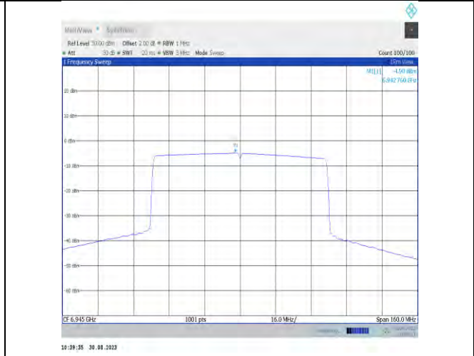
11ax80MIMO-Ant9-6945-PASS
