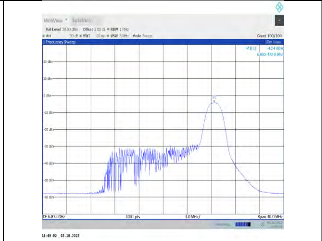
11ax20MIMO-Ant9-6875-PASS
