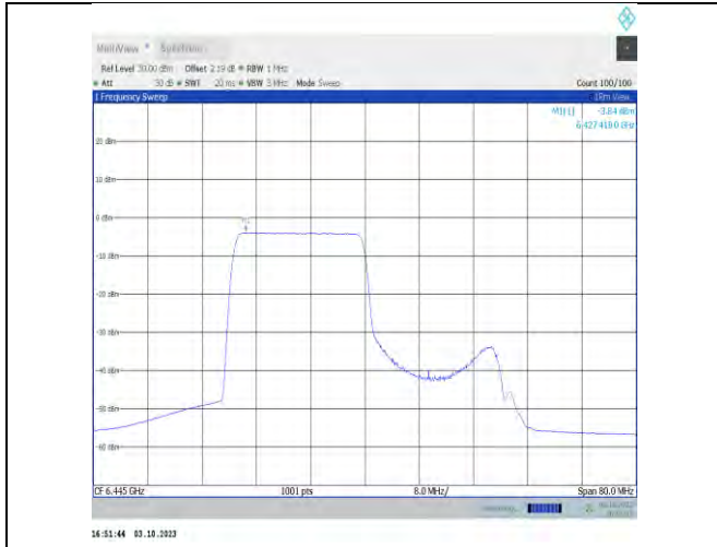
11x40MIMO-Ant7-6445-PASS
