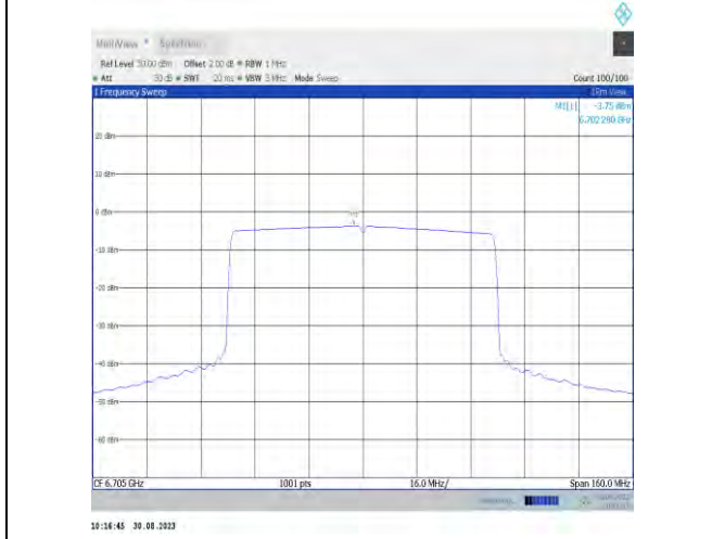
11ax80MIMO-Ant7-6705-PASS
