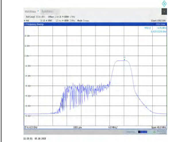
11ax20MIMO-Ant9-6415-PASS
