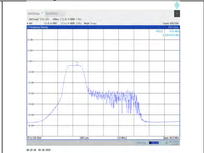
11x20MIMO-Ant7-6535-PASS
