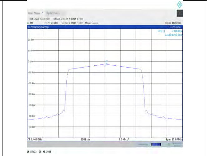
11x40MIMO-Ant9-6445-PASS
