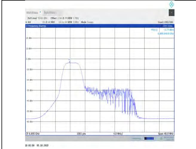
11x20MIMO-Ant9-6895-PASS
