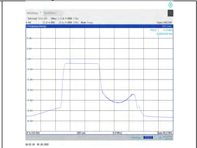
11x40MIMO-Ant9-6445-PASS
