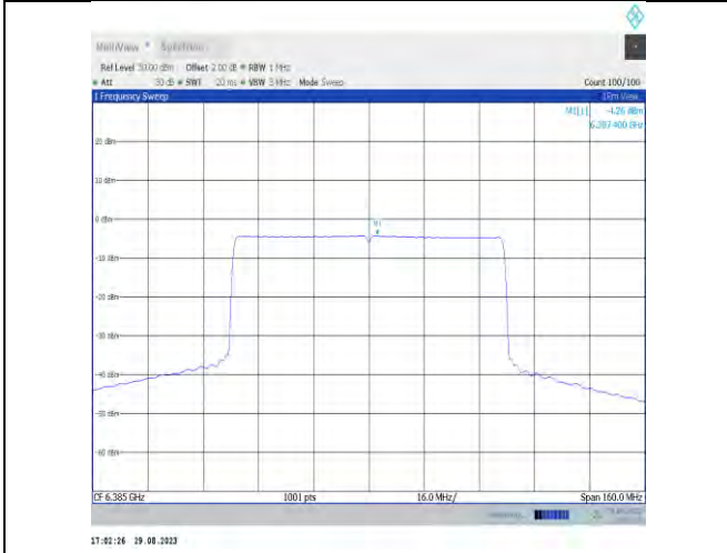
11ax80MIMO-Ant7-6385-PASS
