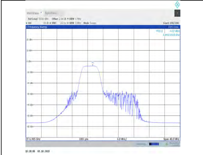
11x20MIMO-Ant9-6995-PASS
