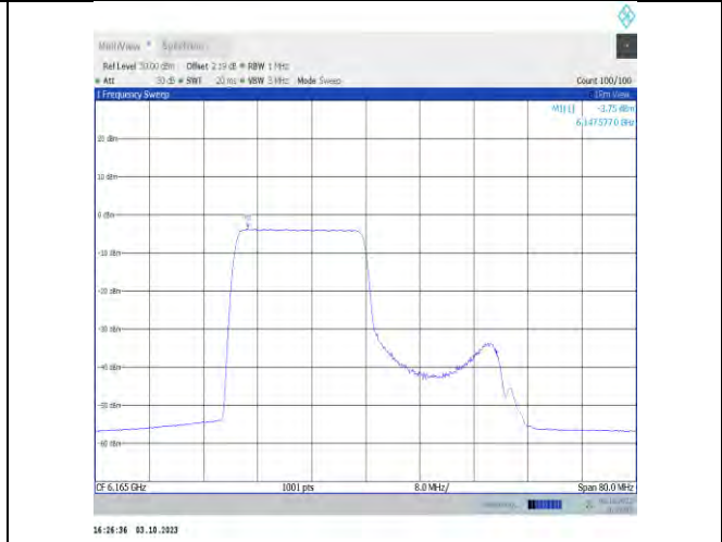
11x40MIMO-Ant9-6165-PASS
