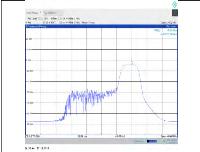
11ax20MIMO-Ant9-6875-PASS
