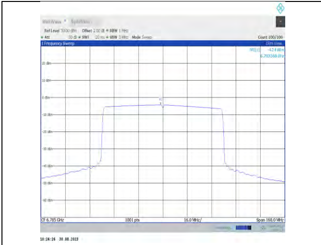
11ax80MIMO-Ant7-6785-PASS
