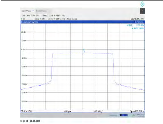
11ax80MIMO-Ant7-6145-PASS
