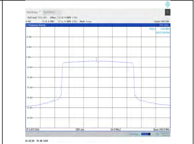
11ax80MIMO-Ant9-6625-PASS
