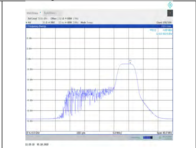
11ax20MIMO-Ant7-6415-PASS
