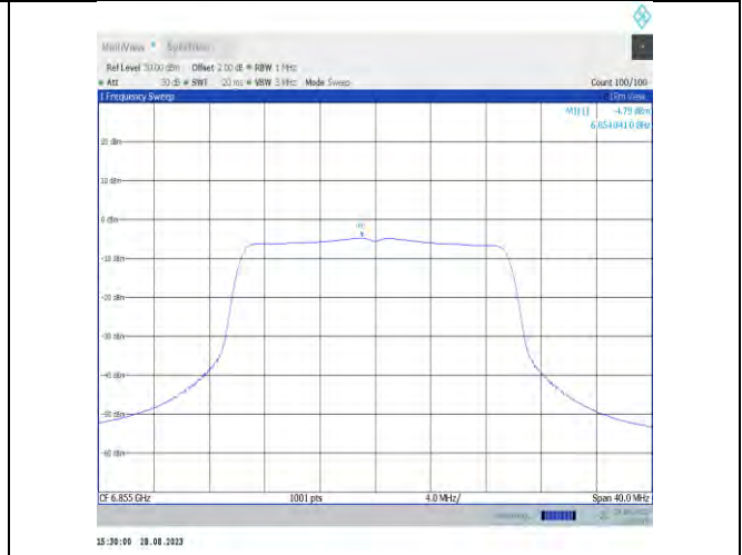
11x20MIMO-Ant9-6855-PASS
