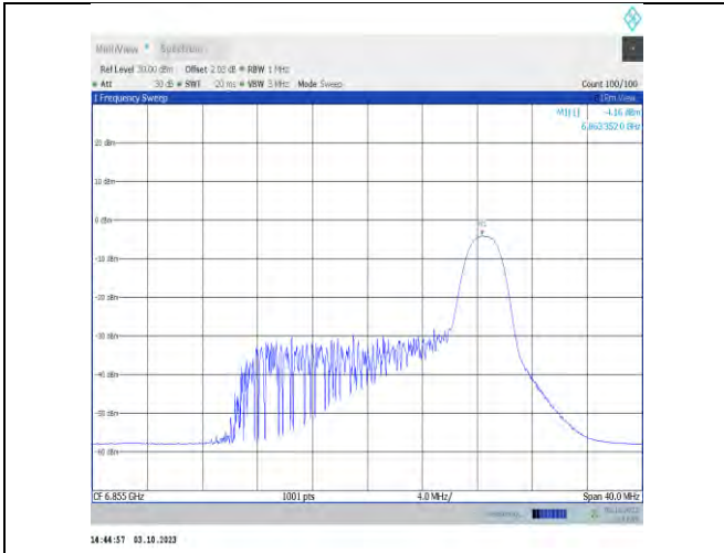
11ax20MIMO-Ant7-6855-PASS
