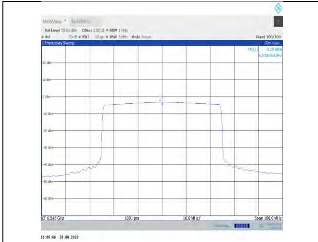
11ax80MIMO-Ant7-6545-PASS
