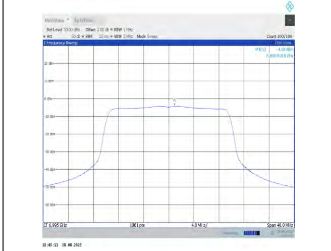
11x20MIMO-Ant7-6995-PASS
