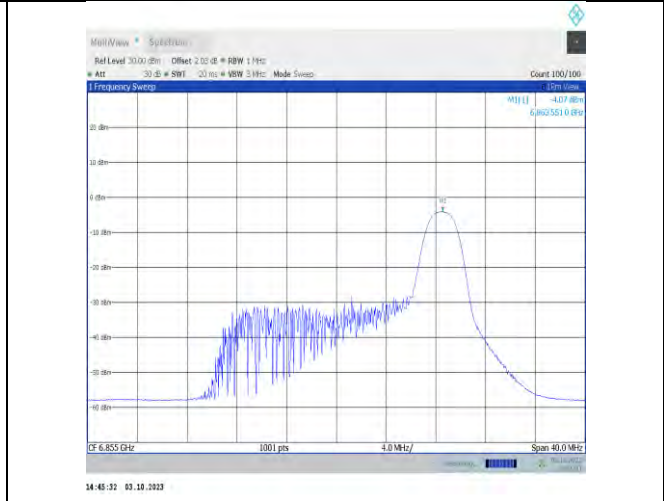
11ax20MIMO-Ant9-6855-PASS
