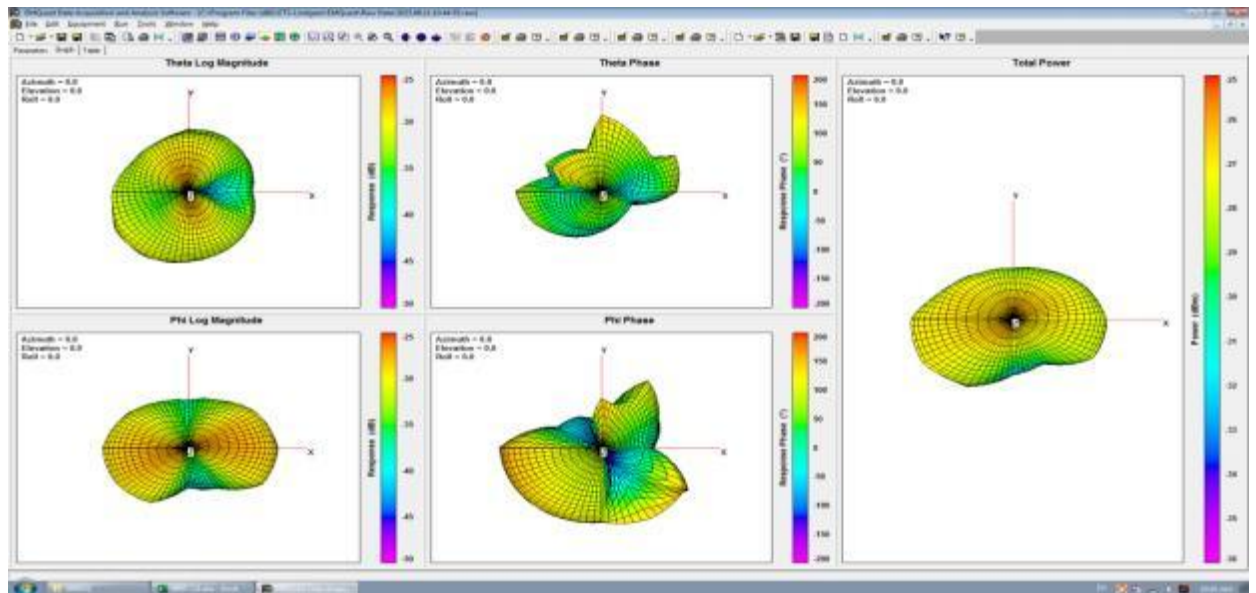
ANT9-WiFi Antenna
