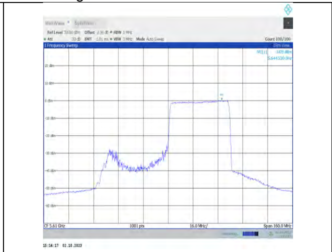
11ax80MIMO-Ant9-5610-PASS
