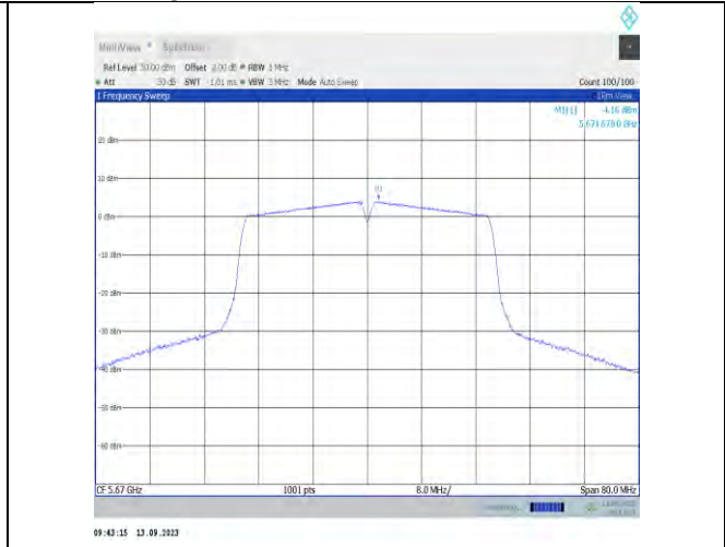
11n40MIMO-Ant9-5670-PASS
