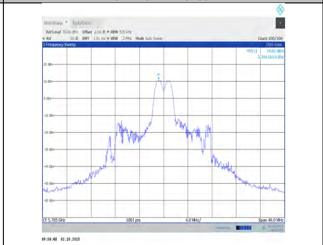
11ax20MIMO-Ant9-5785-PASS
