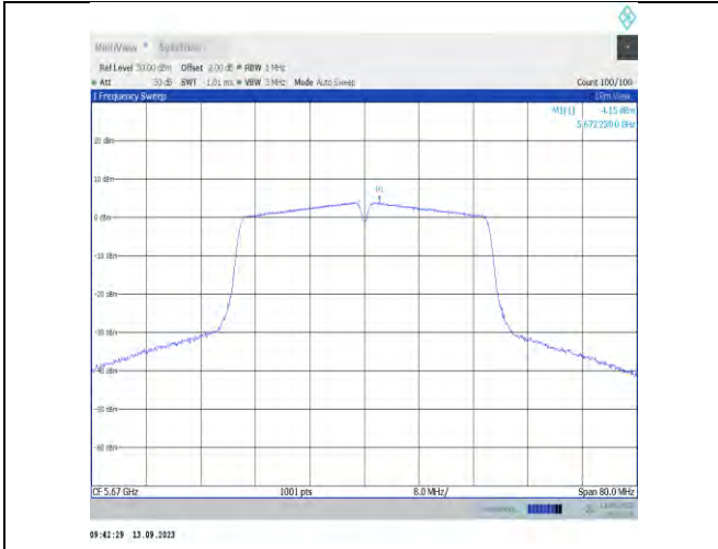
11n40MIMO-Ant7-5670-PASS
