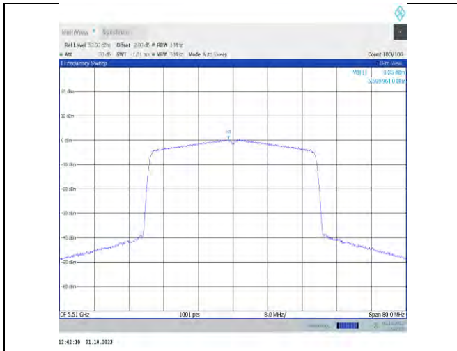
11ax40MIMO-Ant7-5510-PASS
