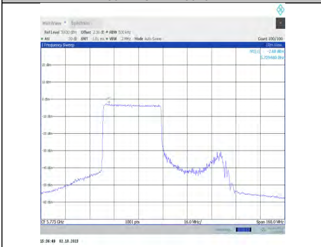
11ax80MIMO-Ant7-5775-PASS
