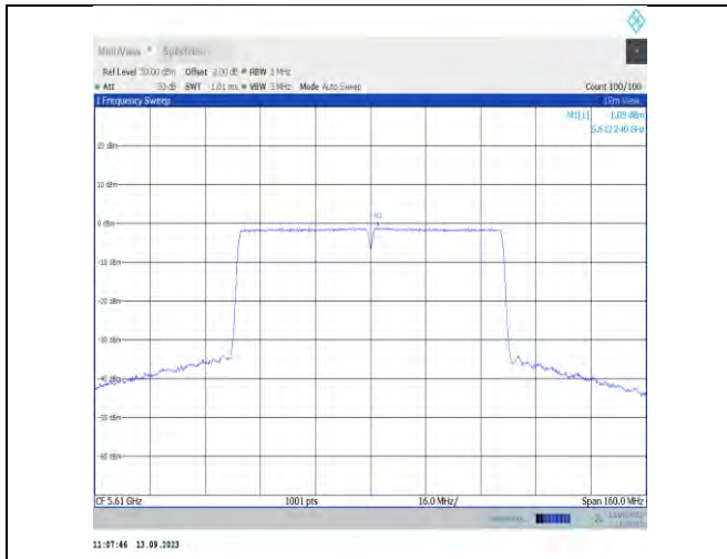
11ac80MIMO-Ant7-5610-PASS
