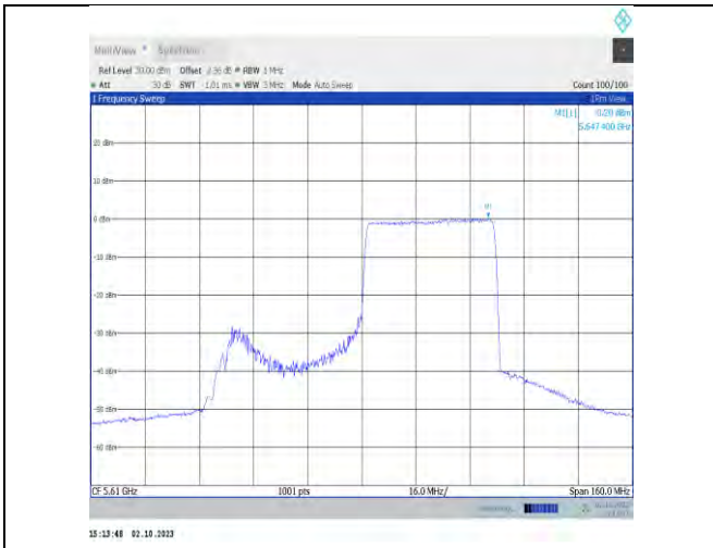
11ax80MIMO-Ant7-5610-PASS
