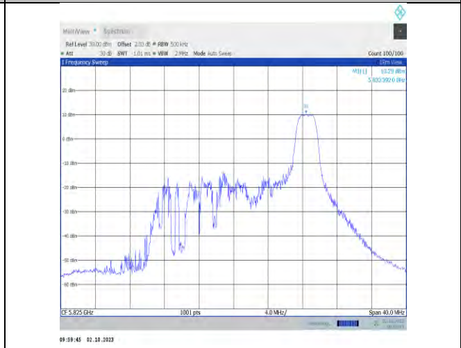
11ax20MIMO-Ant9-5825-PASS
