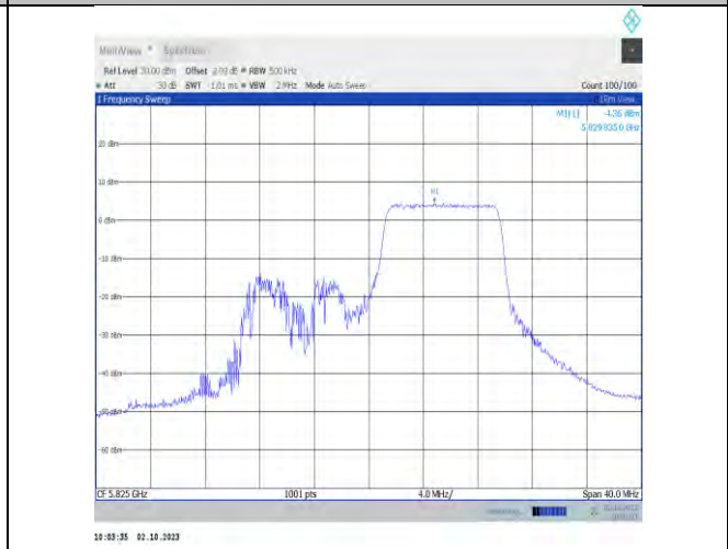
11ax20MIMO-Ant9-5825-PASS
