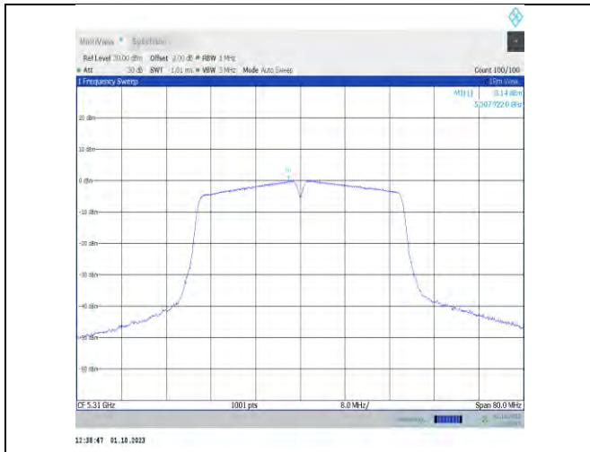
11n40MIMO-Ant7-5310-PASS
