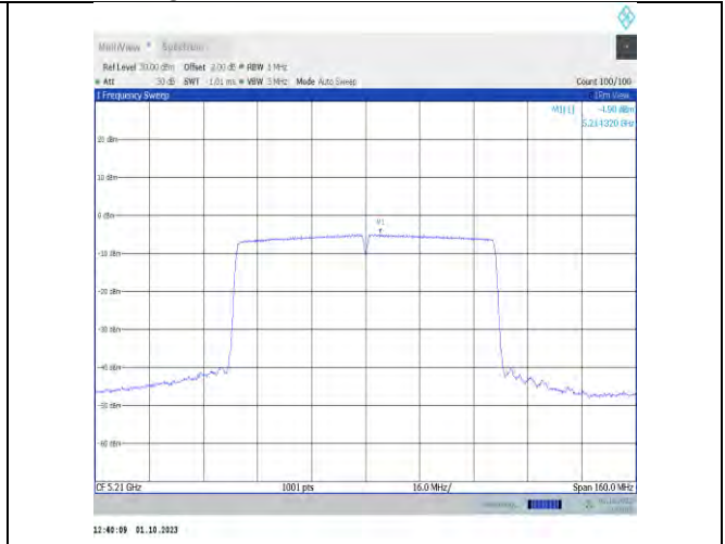
11ac80MIMO-Ant9-5210-PASS
