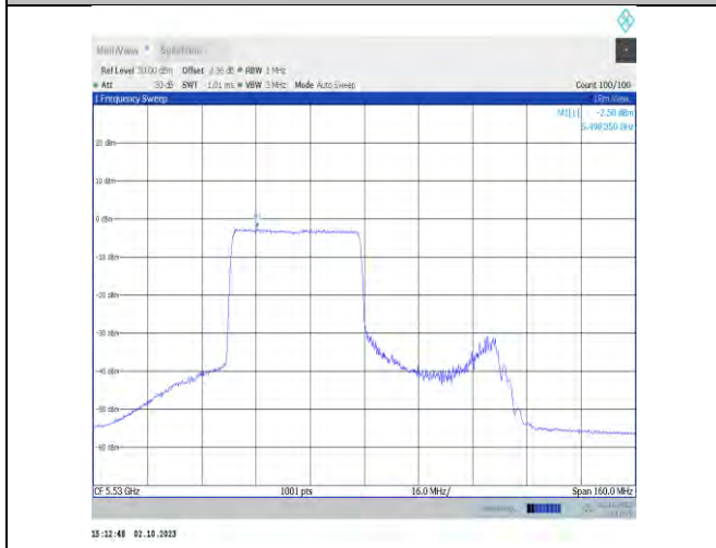
11ax80MIMO-Ant7-5530-PASS
