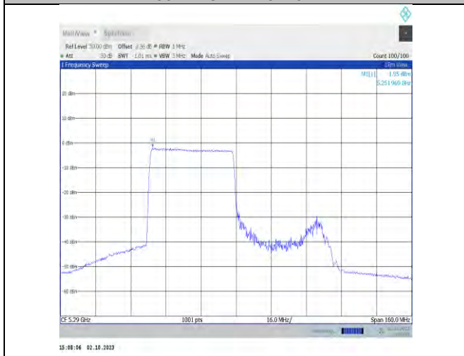
11ax80MIMO-Ant7-5290-PASS
