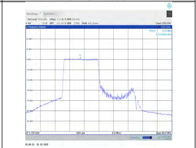
11ax40MIMO-Ant9-5755-PASS
