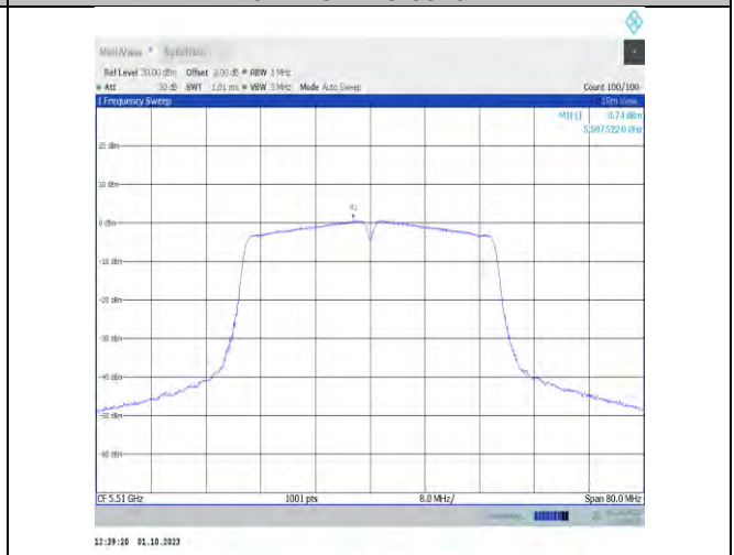
11n40MIMO-Ant9-5510-PASS
