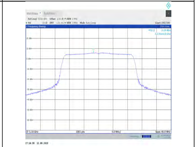
11ax20MIMO-Ant9-5180-PASS
