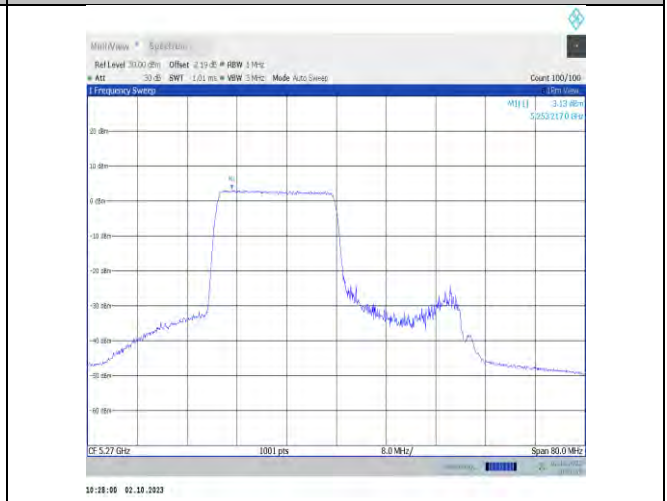
11ax40MIMO-Ant9-5270-PASS
