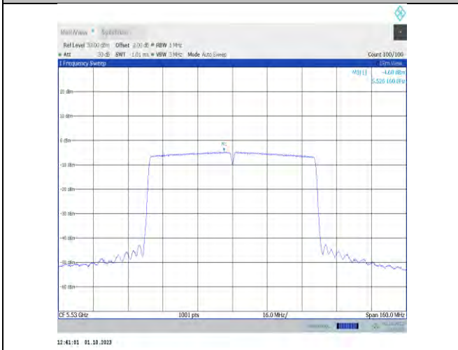
11ac80MIMO-Ant7-5530-PASS
