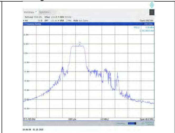
11ax20MIMO-Ant7-5785-PASS
