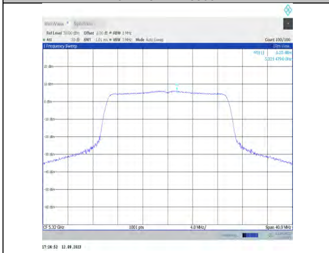
11ax20MIMO-Ant7-5320-PASS
