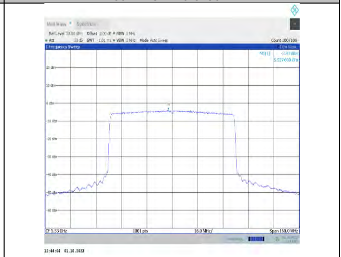
11ax80MIMO-Ant9-5530-PASS
