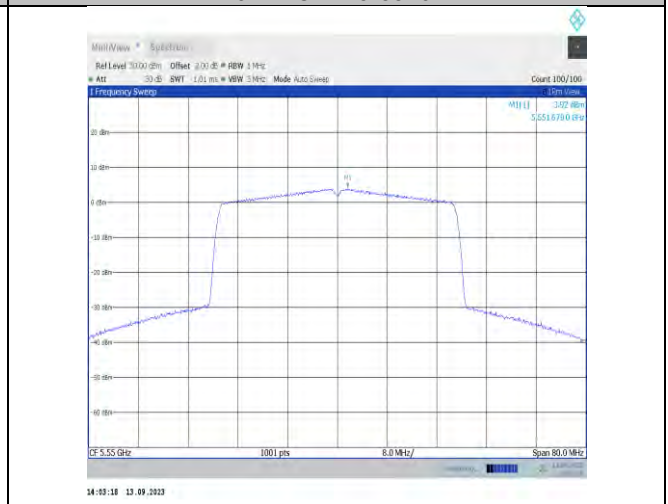
11ax40MIMO-Ant9-5550-PASS
