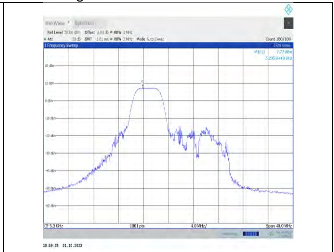
11ax20MIMO-Ant7-5300-PASS
