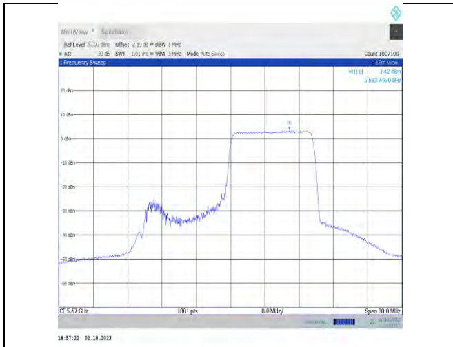
11ax40MIMO-Ant7-5670-PASS
