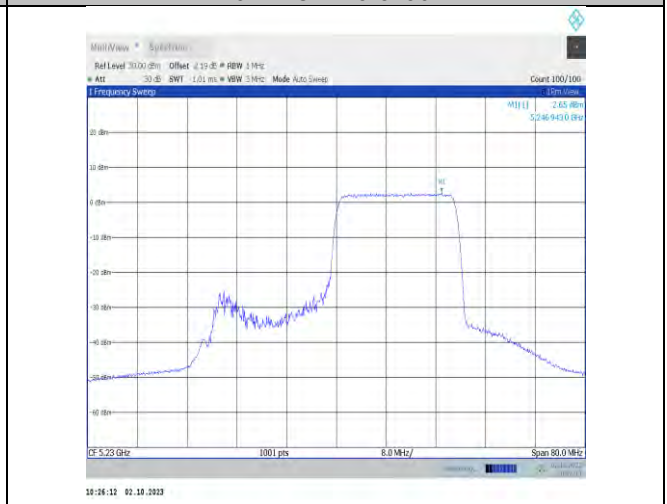
11ax40MIMO-Ant9-5230-PASS
