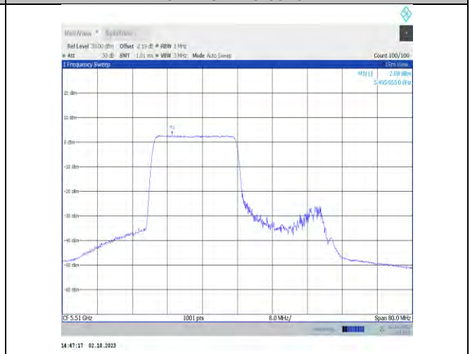
11ax40MIMO-Ant9-5510-PASS
