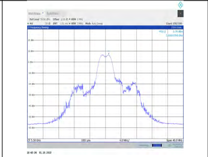
11ax20MIMO-Ant9-5580-PASS
