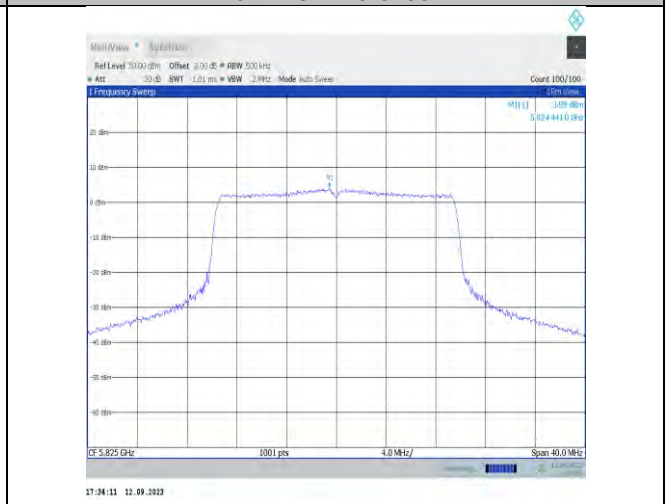
11ax20MIMO-Ant9-5825-PASS
