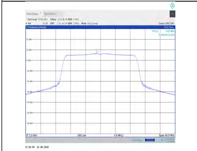
11ax20MIMO-Ant7-5500-PASS
