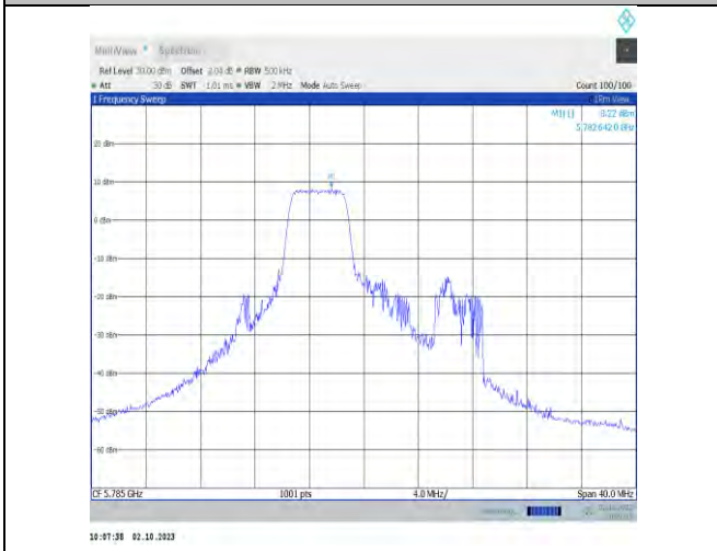
11ax20MIMO-Ant9-5785-PASS
