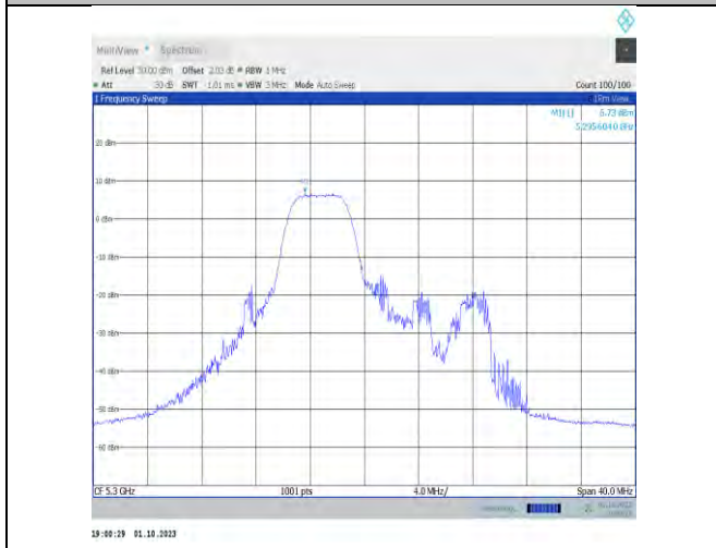
11ax20MIMO-Ant9-5300-PASS
