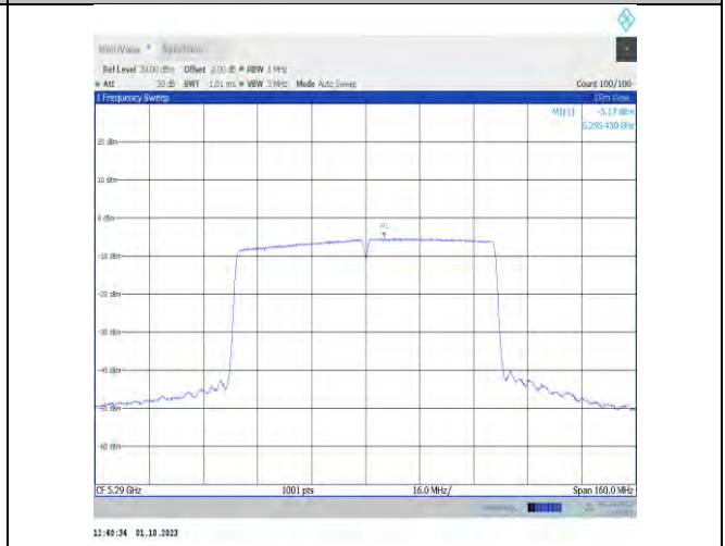
11ac80MIMO-Ant9-5290-PASS
