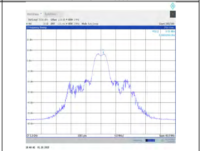
11ax20MIMO-Ant9-5300-PASS
