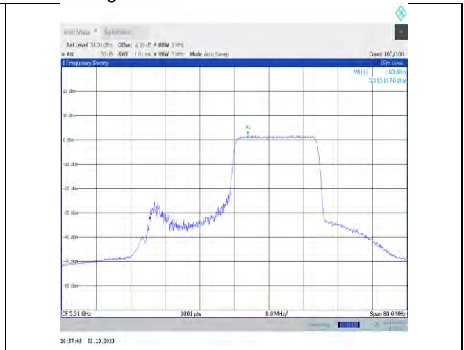
11ax40MIMO-Ant9-5310-PASS
