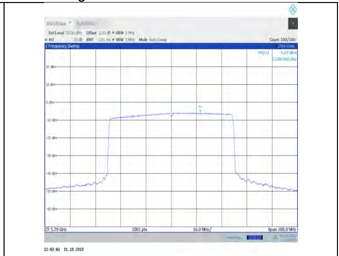
11ax80MIMO-Ant9-5290-PASS
