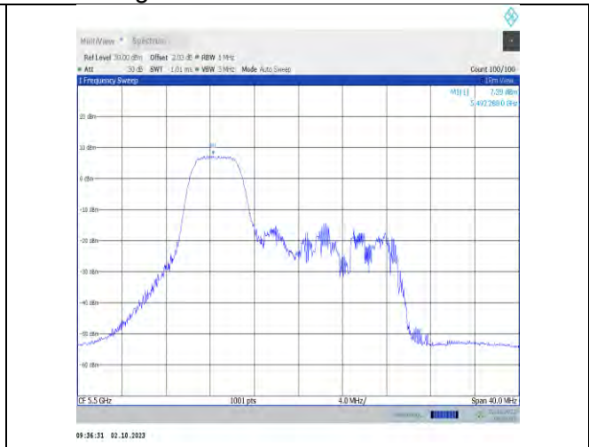
11x20MIMO-Ant7-5500-PASS
