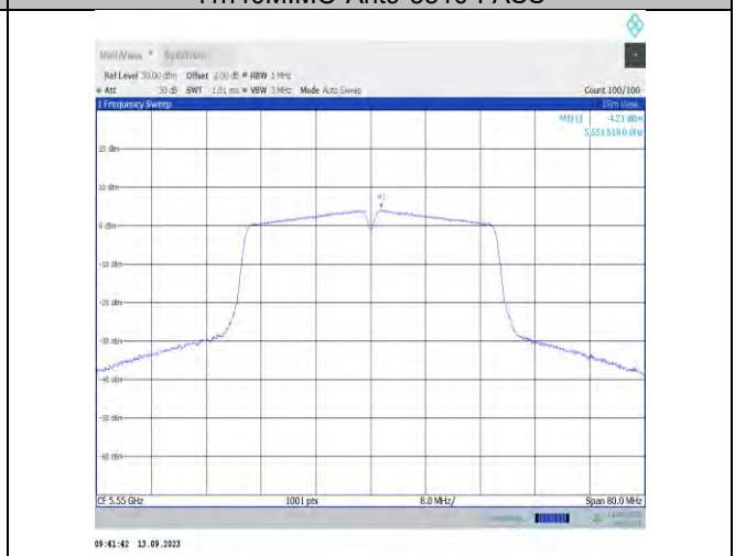
11n40MIMO-Ant9-5550-PASS
