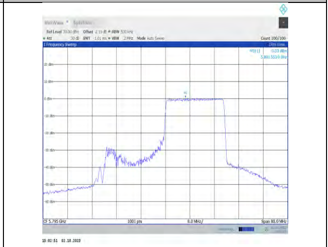
11ax40MIMO-Ant9-5795-PASS
