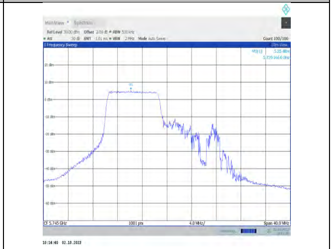
11ax20MIMO-Ant9-5745-PASS
