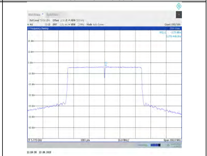
11ac80MIMO-Ant9-5775-PASS
