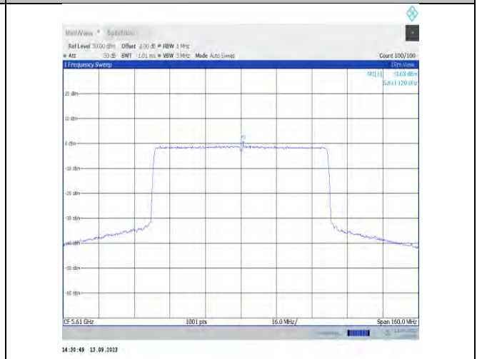
11ax80MIMO-Ant9-5610-PASS
