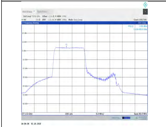
11ax40MIMO-Ant7-5550-PASS
