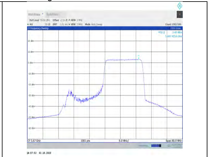
11ax40MIMO-Ant9-5670-PASS
