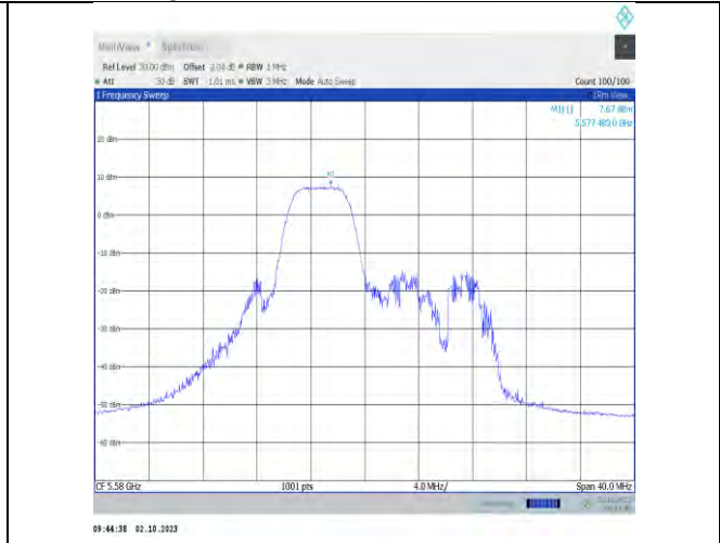
11ax20MIMO-Ant7-5580-PASS
