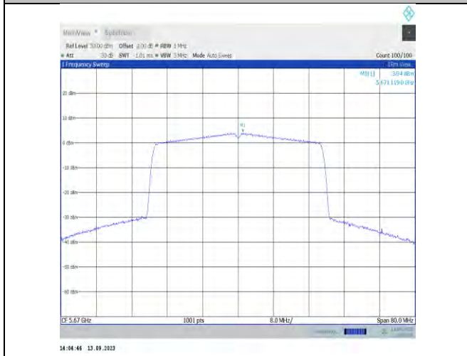
11ax40MIMO-Ant7-5670-PASS
