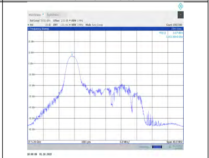
11x20MIMO-Ant9-5260-PASS
