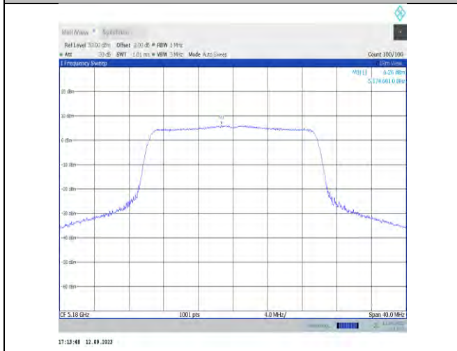
11ax20MIMO-Ant7-5180-PASS
