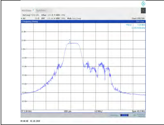
11ax20MIMO-Ant9-5580-PASS
