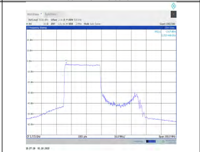
11ax80MIMO-Ant9-5775-PASS
