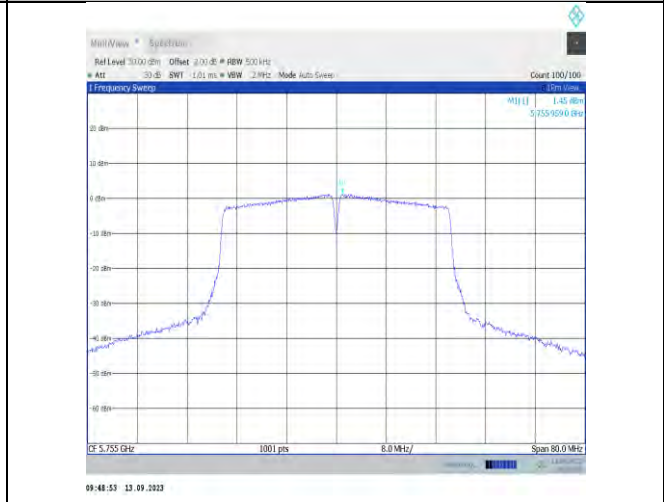
11n40MIMO-Ant9-5755-PASS
