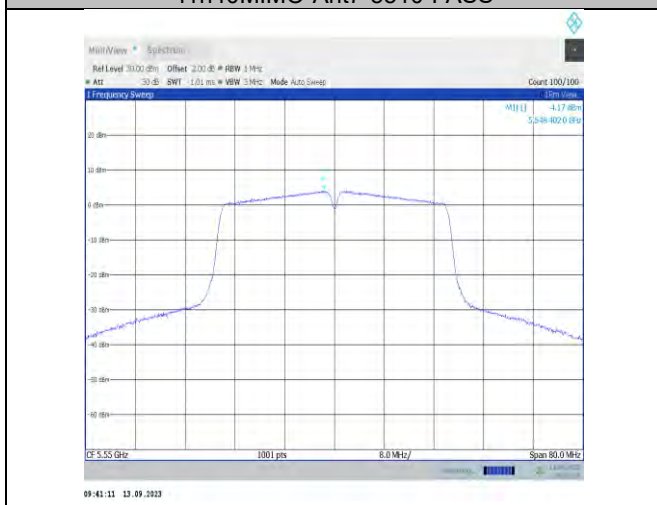
11n40MIMO-Ant7-5550-PASS
