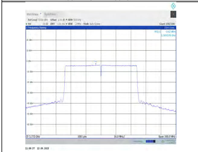
11ac80MIMO-Ant7-5775-PASS
