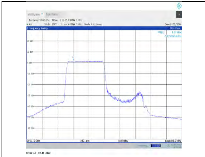
11ax40MIMO-Ant7-5190-PASS
