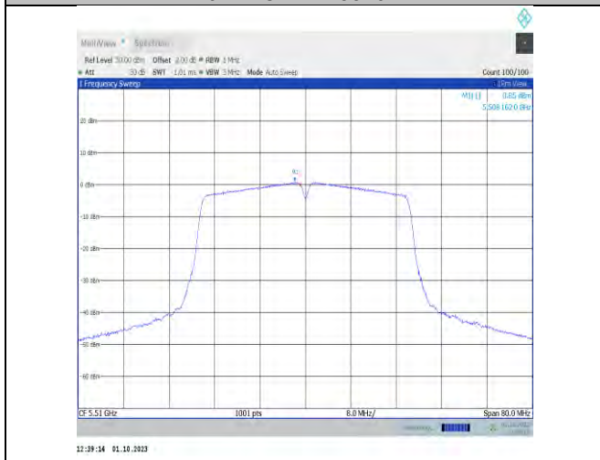
11n40MIMO-Ant7-5510-PASS
