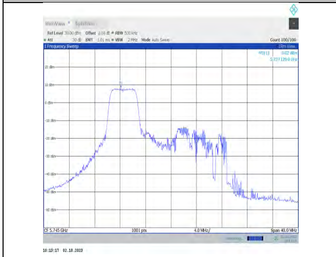
11ax20MIMO-Ant9-5745-PASS
