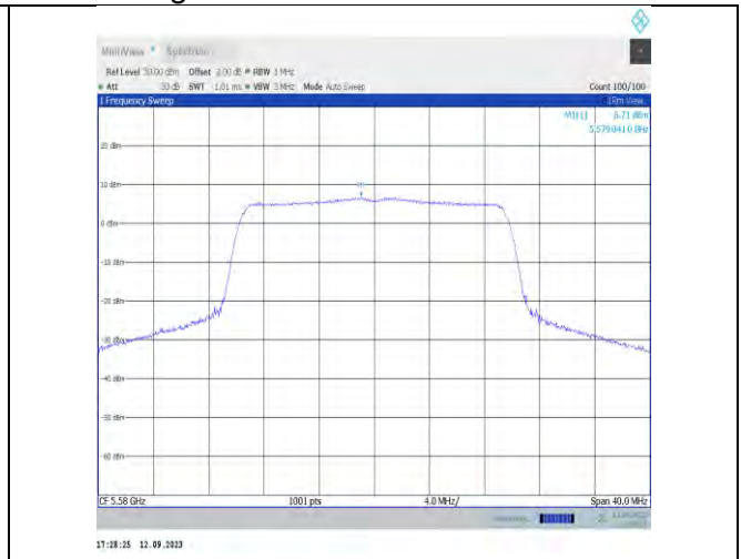
11ax20MIMO-Ant9-5580-PASS
