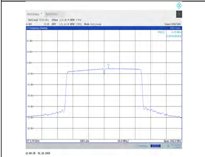
11ac80MIMO-Ant7-5290-PASS
