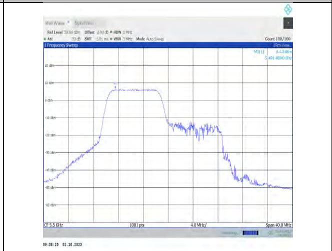
11x20MIMO-Ant9-5500-PASS
