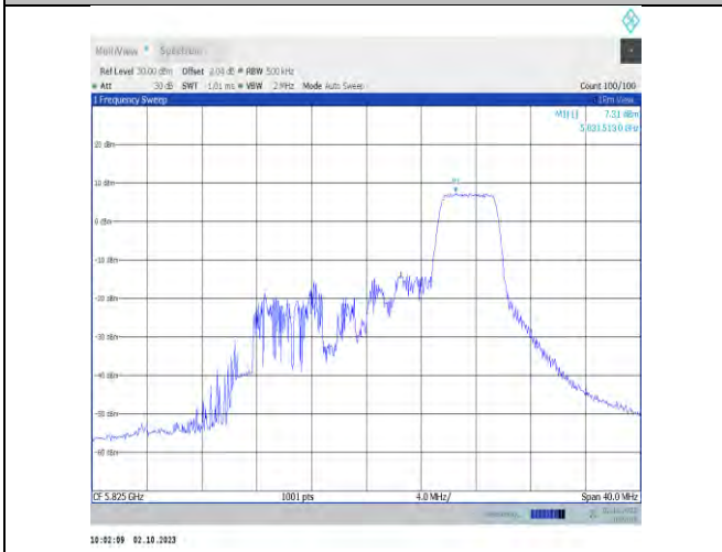
11ax20MIMO-Ant9-5825-PASS
