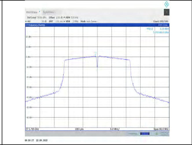
11n40MIMO-Ant9-5795-PASS
