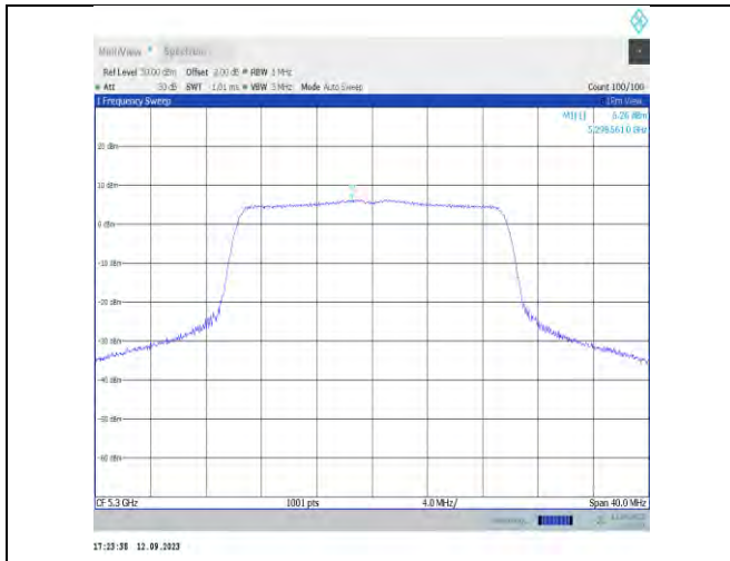
11ax20MIMO-Ant7-5300-PASS
