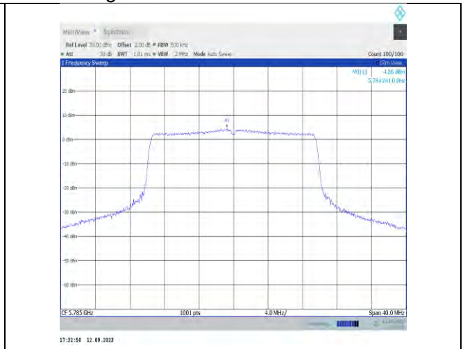
11ax20MIMO-Ant9-5785-PASS
