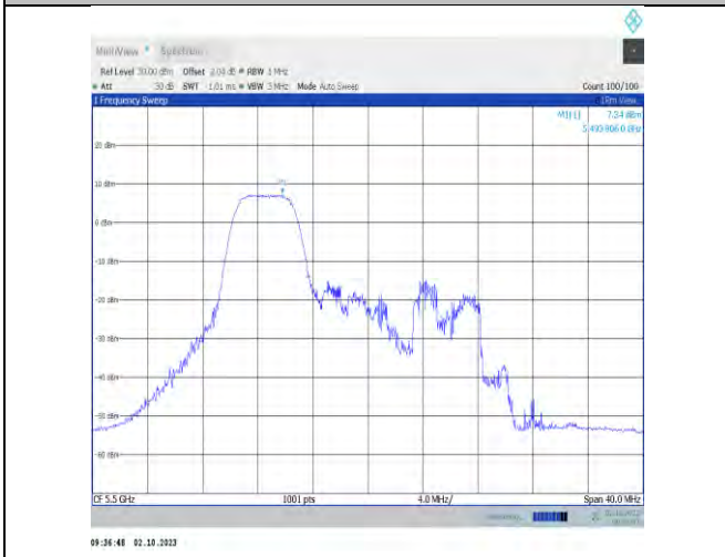
11x20MIMO-Ant9-5500-PASS
