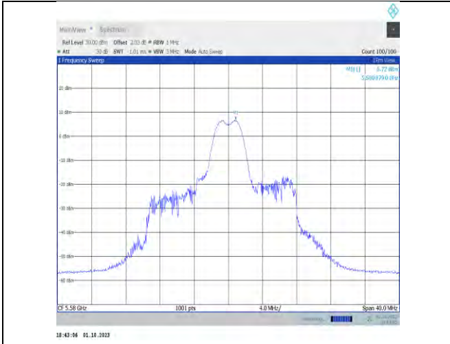
11ax20MIMO-Ant7-5580-PASS
