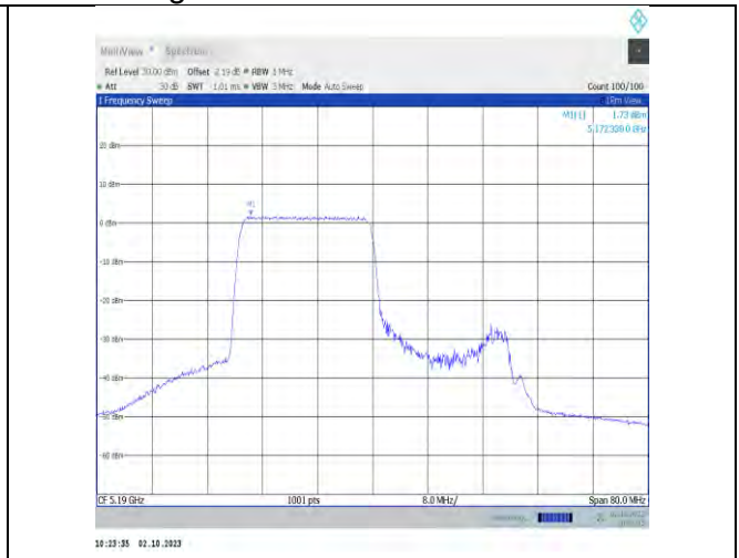
11ax40MIMO-Ant9-5190-PASS
