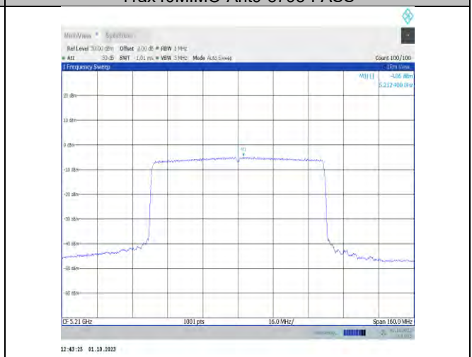
11ax80MIMO-Ant9-5210-PASS
