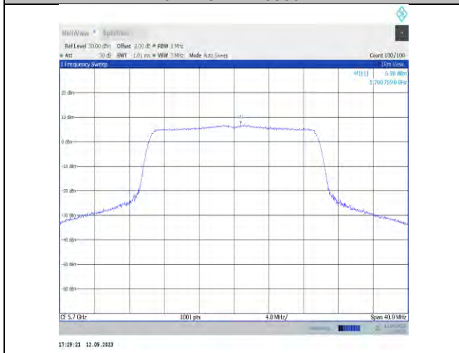
11ax20MIMO-Ant7-5700-PASS
