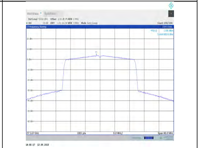
11ax40MIMO-Ant9-5670-PASS
