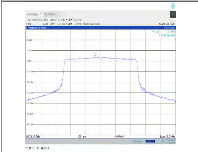
11ax20MIMO-Ant7-5825-PASS
