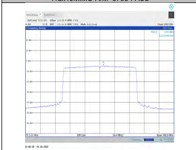
11ax80MIMO-Ant7-5210-PASS
