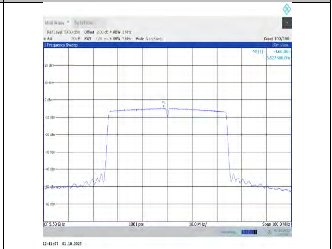
11ac80MIMO-Ant9-5530-PASS
