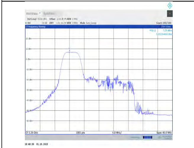
11x20MIMO-Ant9-5260-PASS
