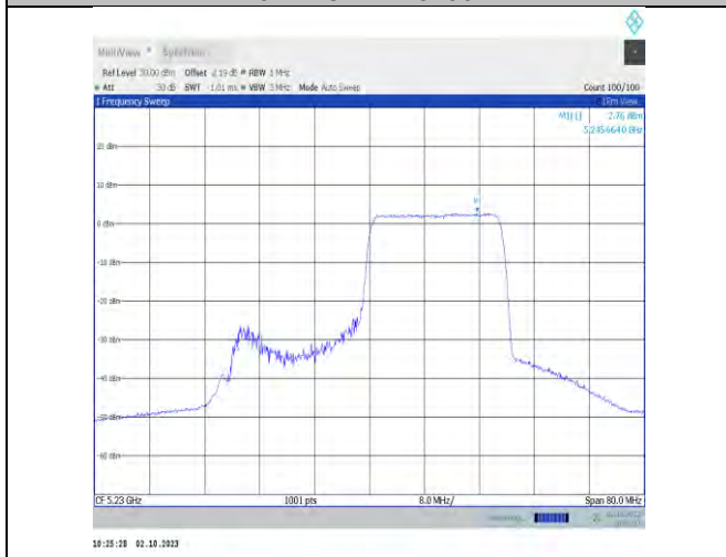
11ax40MIMO-Ant7-5230-PASS
