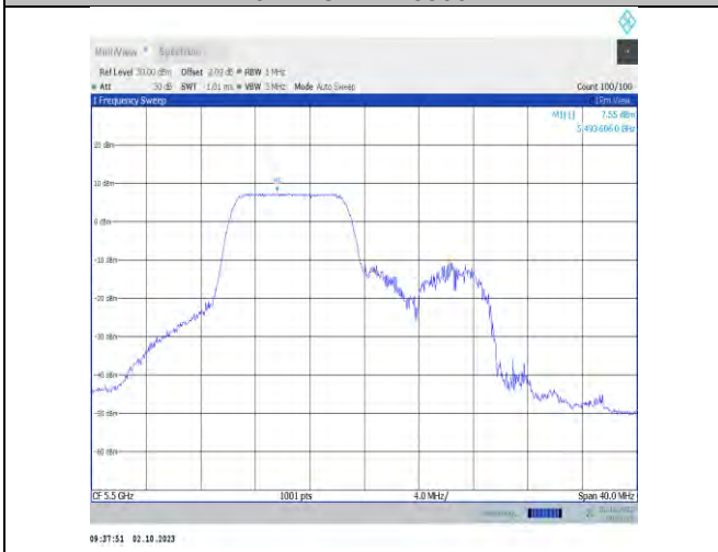
11x20MIMO-Ant7-5500-PASS
