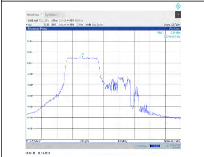
11ax20MIMO-Ant7-5785-PASS
