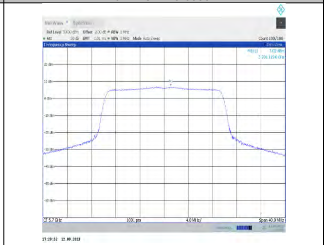
11ax20MIMO-Ant9-5700-PASS
