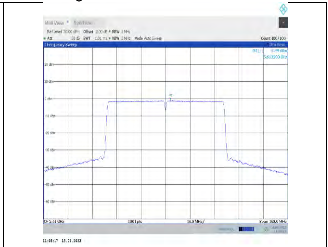
11ac80MIMO-Ant9-5610-PASS
