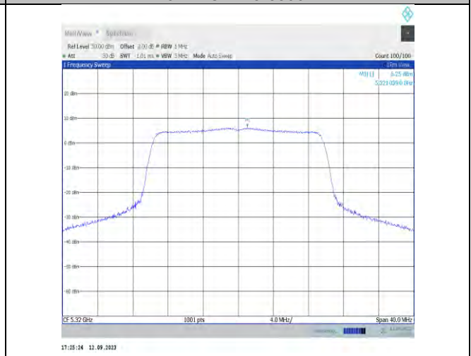
11ax20MIMO-Ant9-5320-PASS
