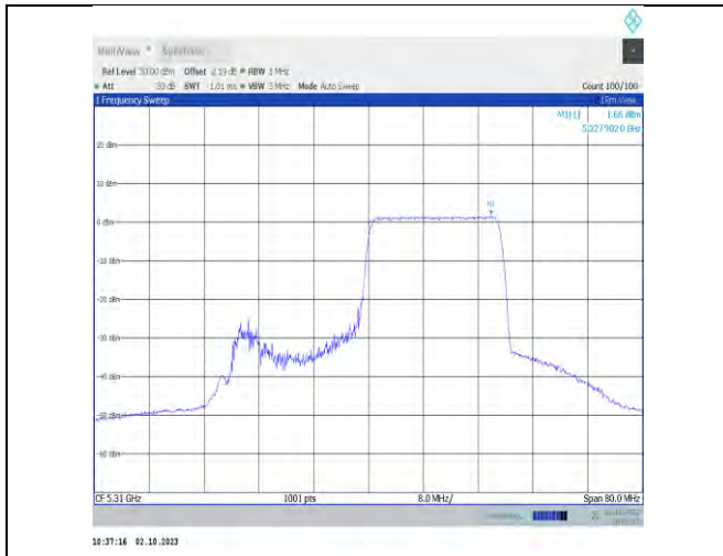
11ax40MIMO-Ant7-5310-PASS
