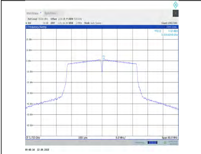
11n40MIMO-Ant7-5755-PASS
