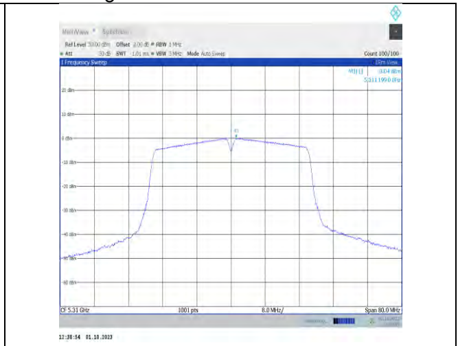
11n40MIMO-Ant9-5310-PASS
