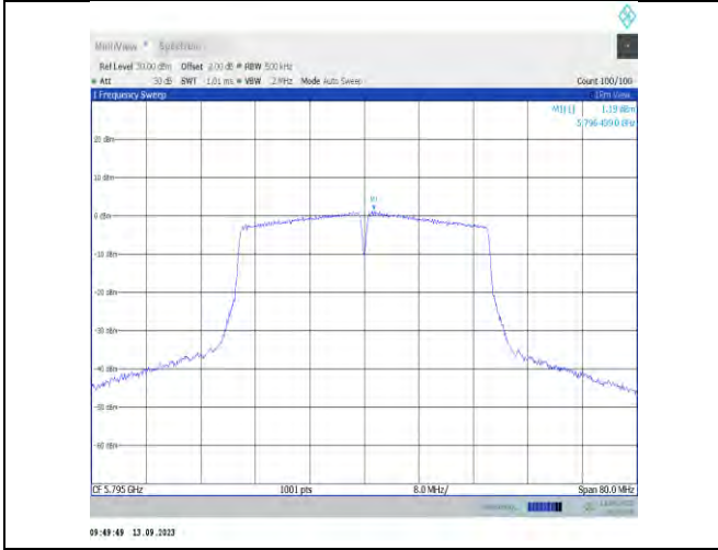
11n40MIMO-Ant7-5795-PASS
