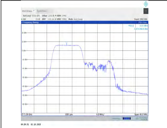
11ax20MIMO-Ant7-5580-PASS
