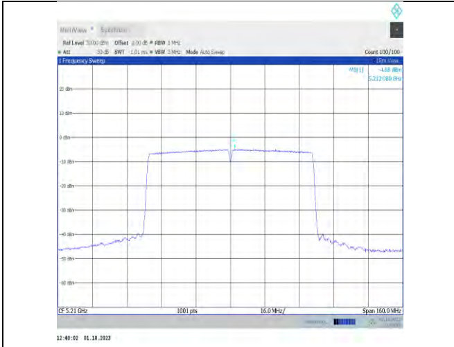
11ac80MIMO-Ant7-5210-PASS
