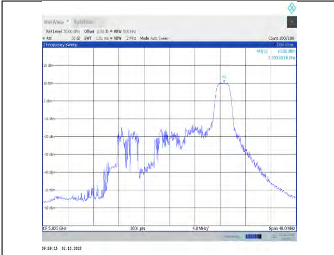
11ax20MIMO-Ant7-5825-PASS
