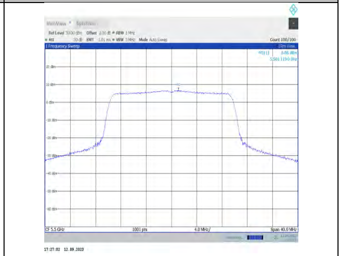
11ax20MIMO-Ant9-5500-PASS
