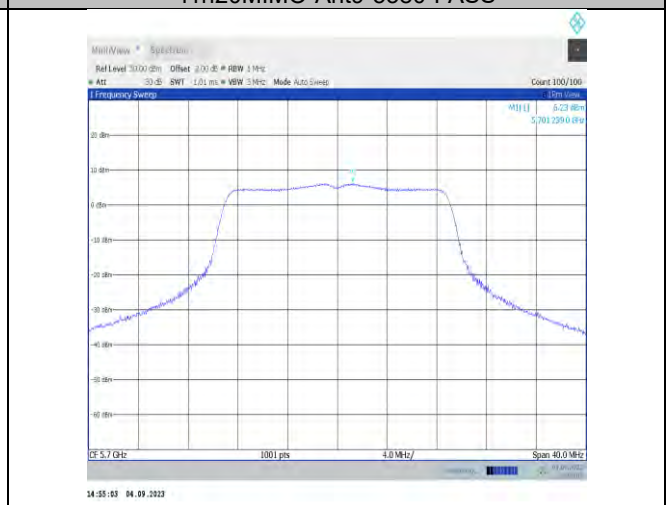
11n20MIMO-Ant9-5700-PASS
