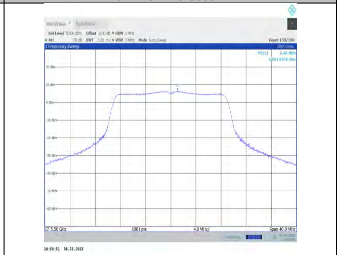
11n20MIMO-Ant9-5580-PASS
