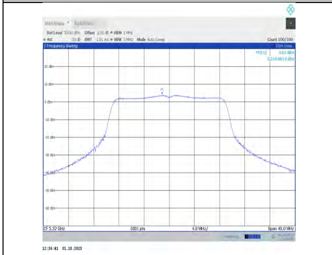
11n20MIMO-Ant7-5320-PASS
