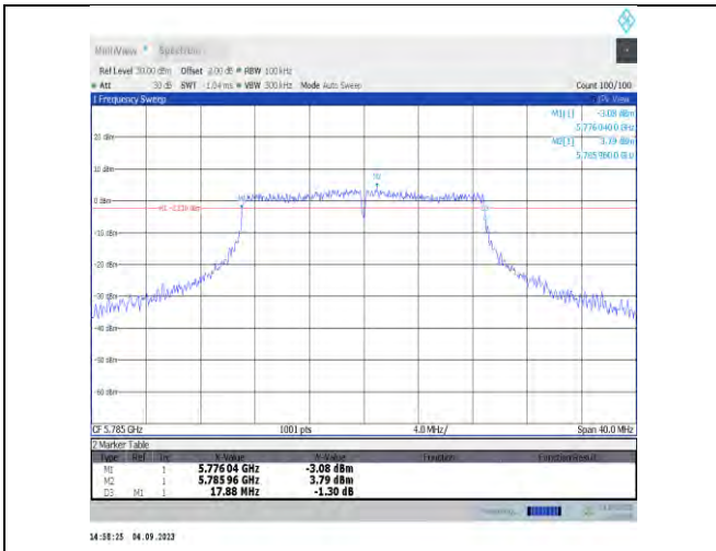
11n20MIMO-Ant9-5785-PASS
