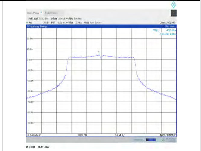
11n20MIMO-Ant9-5785-PASS
