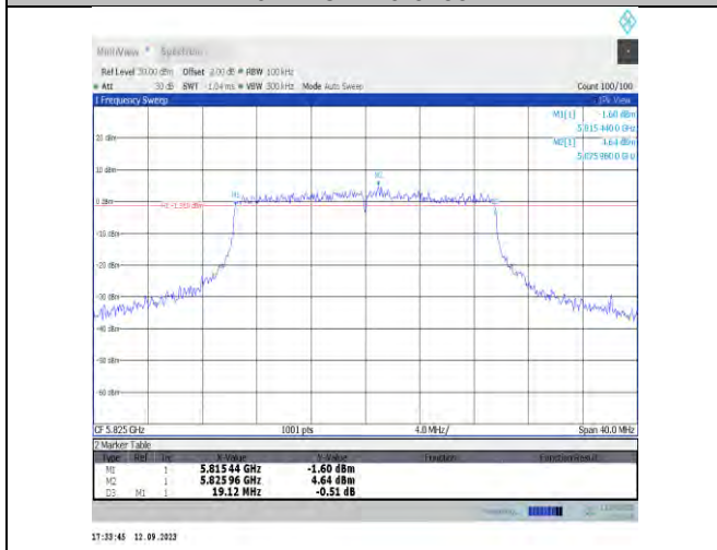
11ax20MIMO-Ant9-5825-PASS
