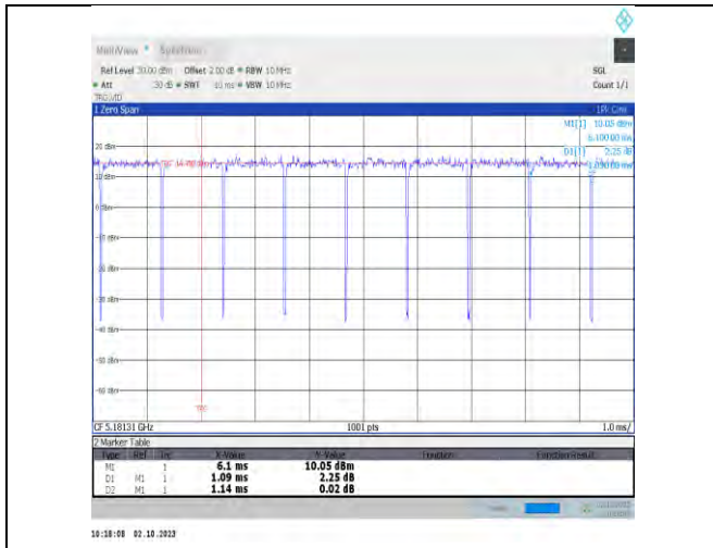
NTNV-11ax40MIMO-Ant7-5190
