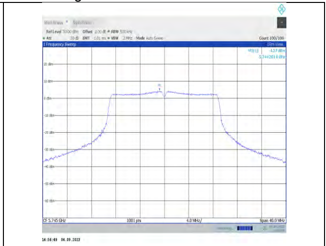
11n20MIMO-Ant9-5745-PASS
