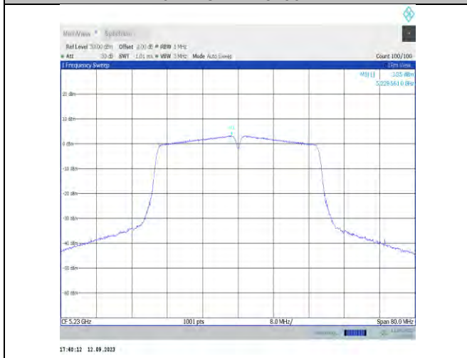
11n40MIMO-Ant7-5230-PASS
