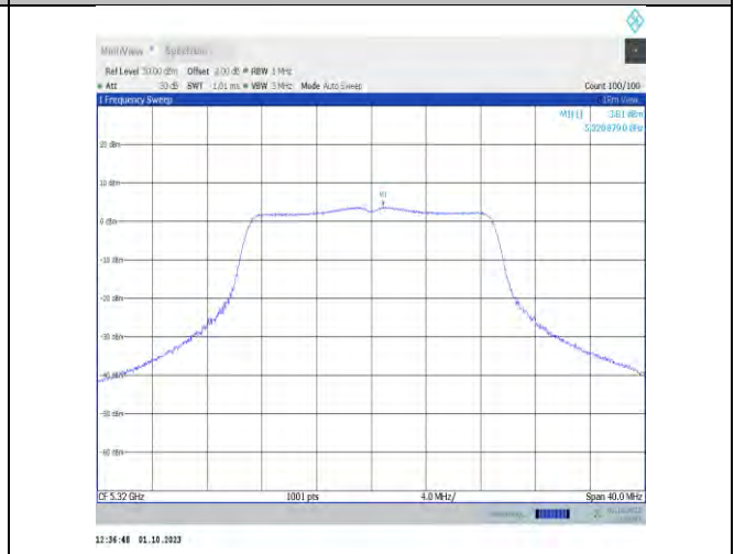
11n20MIMO-Ant9-5320-PASS
