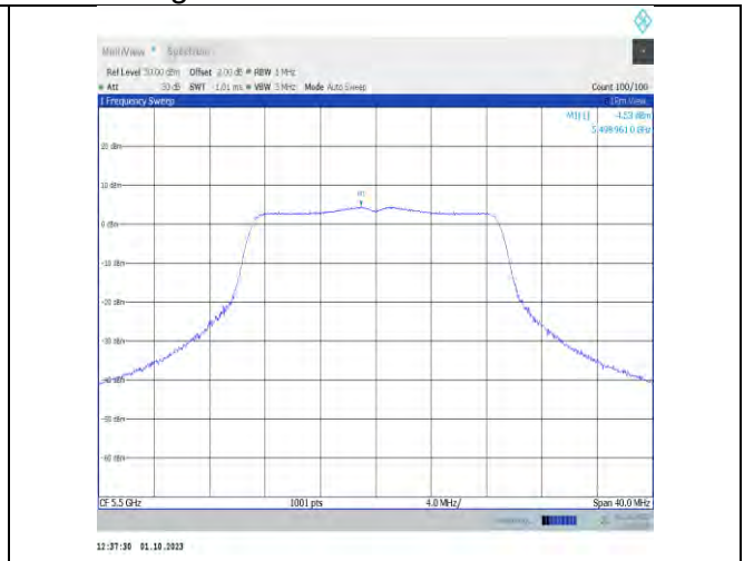
11n20MIMO-Ant9-5500-PASS
