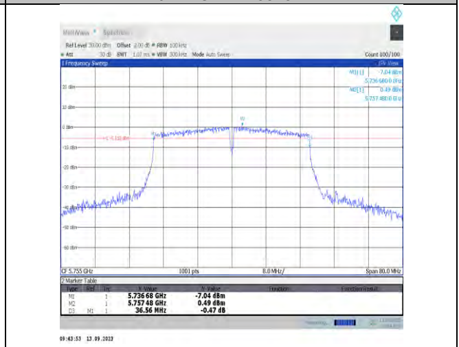
11n40MIMO-Ant7-5755-PASS
