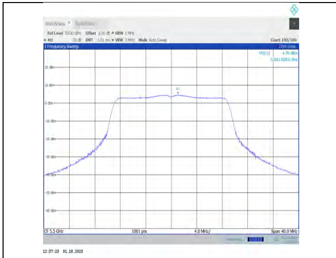
11n20MIMO-Ant7-5500-PASS
