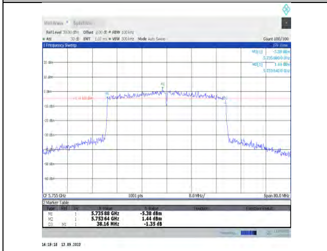
11ax40MIMO-Ant9-5755-PASS
