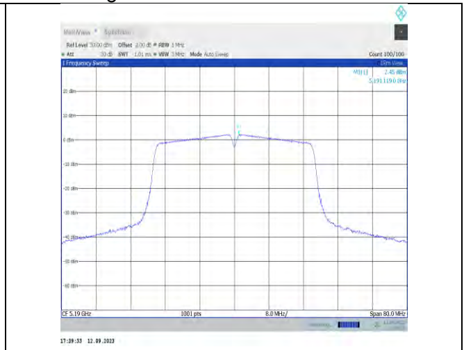
11n40MIMO-Ant9-5190-PASS
