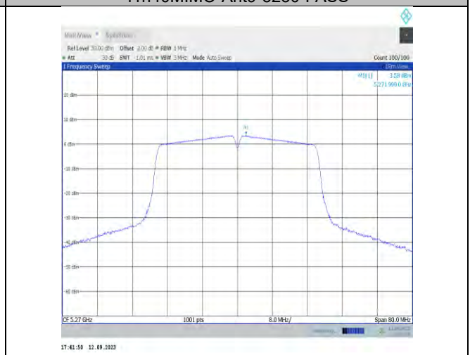
11n40MIMO-Ant9-5270-PASS
