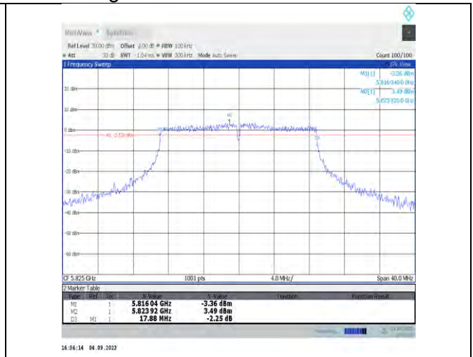
11n20MIMO-Ant7-5825-PASS
