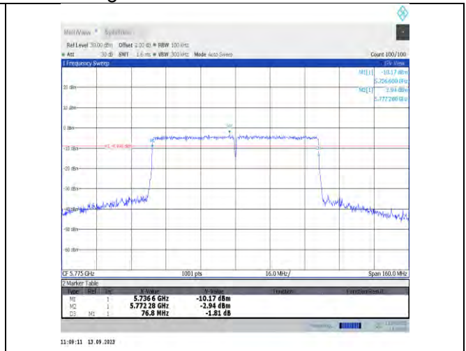
11ac80MIMO-Ant7-5775-PASS
