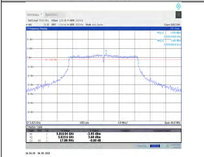
11n20MIMO-Ant9-5825-PASS
