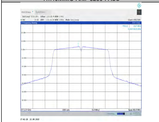
11n40MIMO-Ant7-5270-PASS
