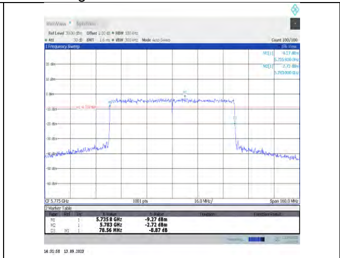
11ax80MIMO-Ant7-5775-PASS
