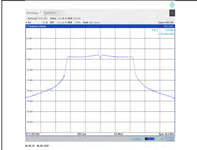
11n20MIMO-Ant7-5785-PASS
