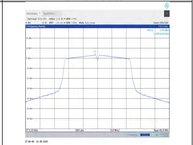
11n40MIMO-Ant9-5230-PASS
