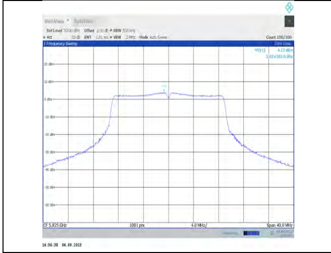
11n20MIMO-Ant7-5825-PASS
