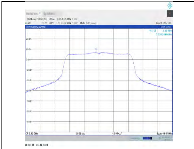
11n20MIMO-Ant7-5260-PASS
