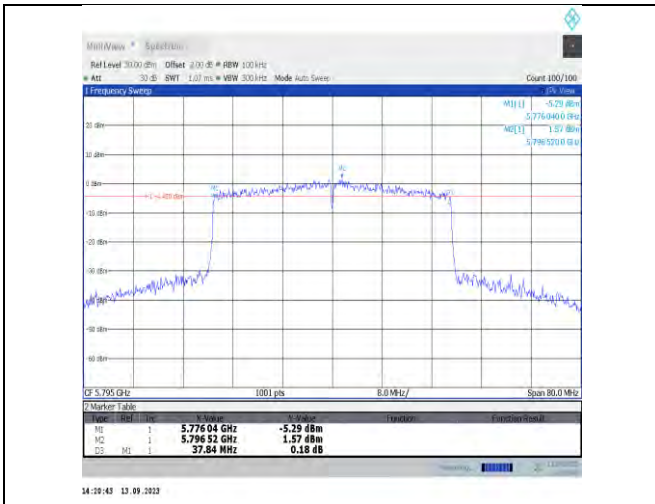
11ax40MIMO-Ant9-5795-PASS
