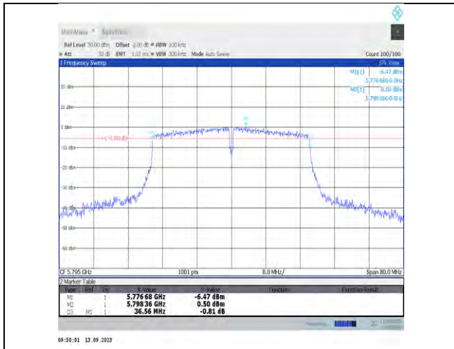
11n40MIMO-Ant9-5795-PASS
