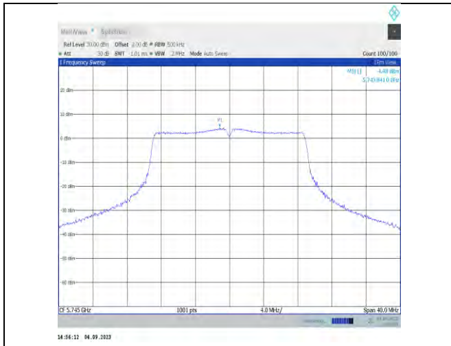
11n20MIMO-Ant7-5745-PASS
