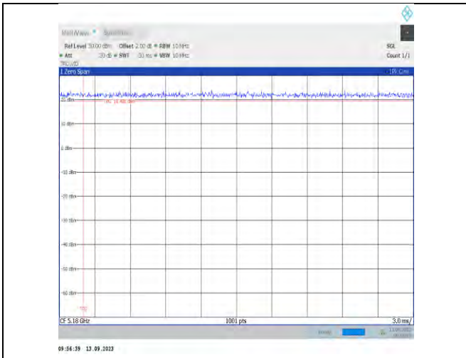
NTNV-11ac20MIMO-Ant7-5180
