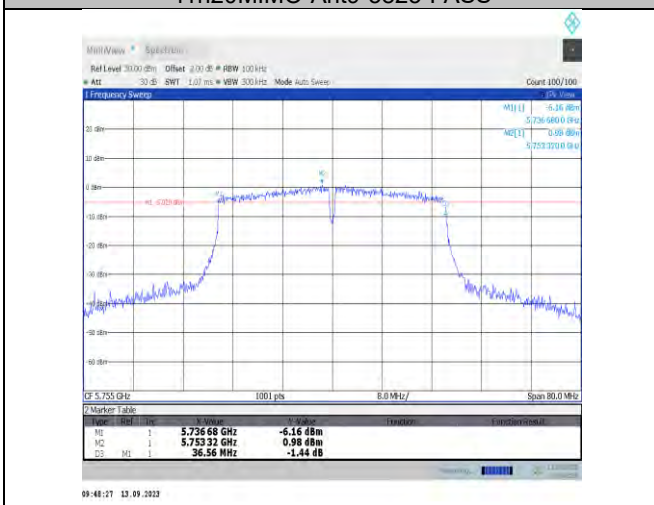
11n40MIMO-Ant9-5755-PASS
