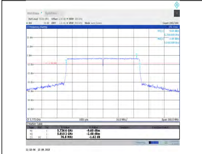
11ac80MIMO-Ant9-5775-PASS
