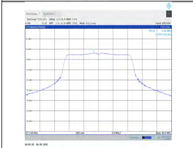
11n20MIMO-Ant7-5580-PASS
