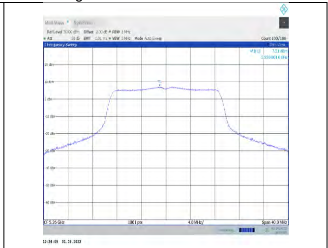
11n20MIMO-Ant9-5260-PASS
