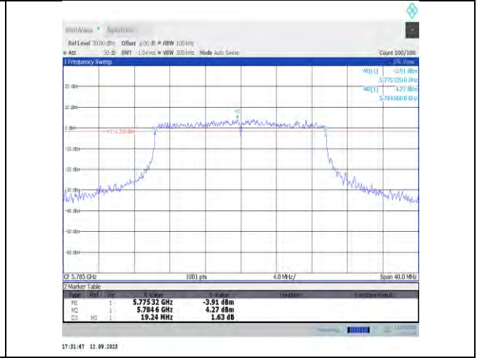
11ax20MIMO-Ant7-5785-PASS
