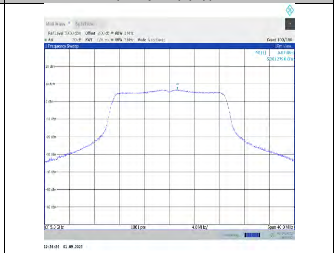
11n20MIMO-Ant9-5300-PASS
