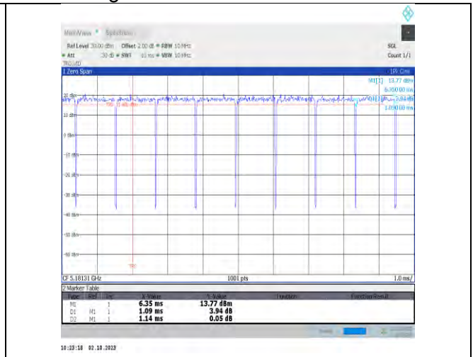
NTNV-11ax40MIMO-Ant9-5190
