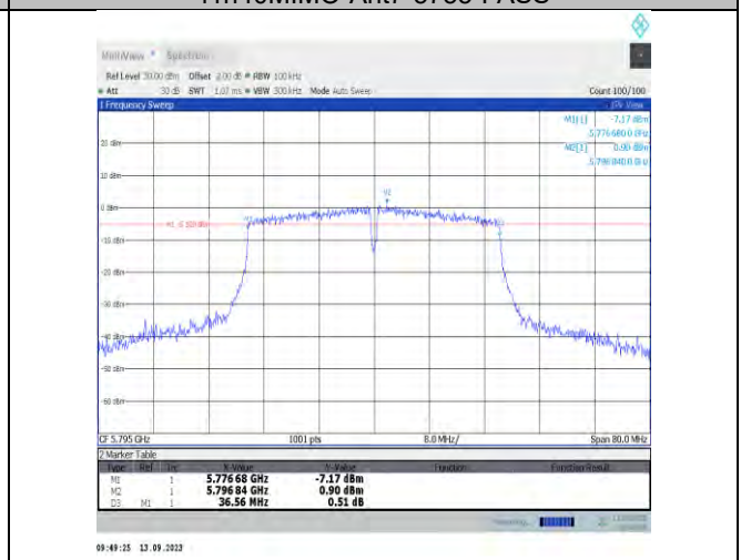
11n40MIMO-Ant7-5795-PASS
