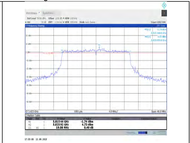
11ax20MIMO-Ant7-5825-PASS
