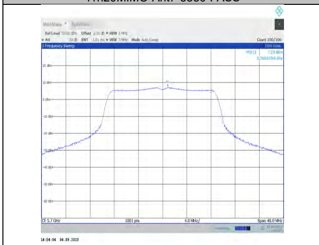
11n20MIMO-Ant7-5700-PASS
