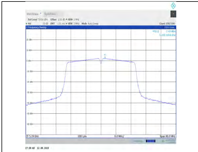
11n40MIMO-Ant7-5190-PASS
