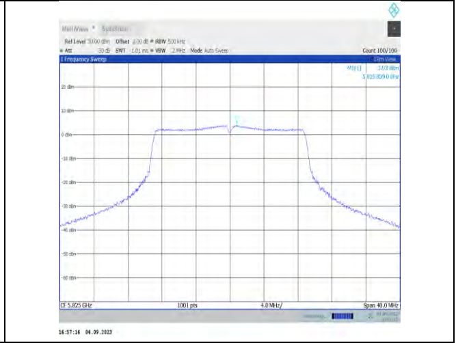
11n20MIMO-Ant9-5825-PASS
