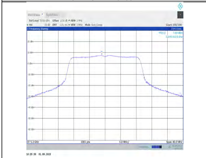
11n20MIMO-Ant7-5300-PASS
