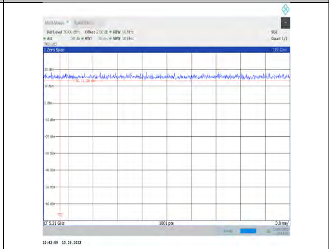
NTNV-11ac80MIMO-Ant9-5210
