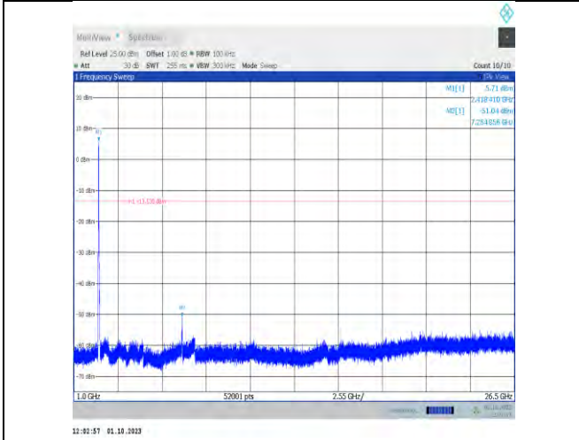
11n20MIMO-Ant9-2417-1000~26500-PASS
