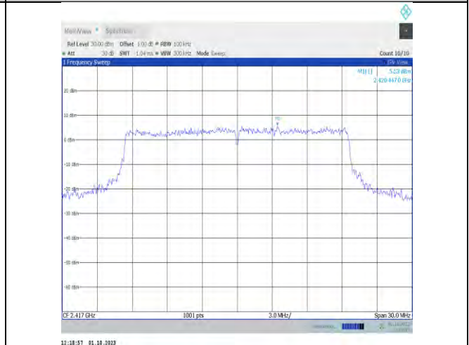
11ax20MIMO-Ant7-2417-0~Reference-PASS
