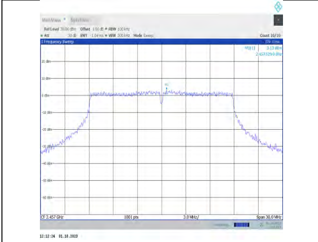
11n20MIMO-Ant9-2457-0~Reference-PASS
