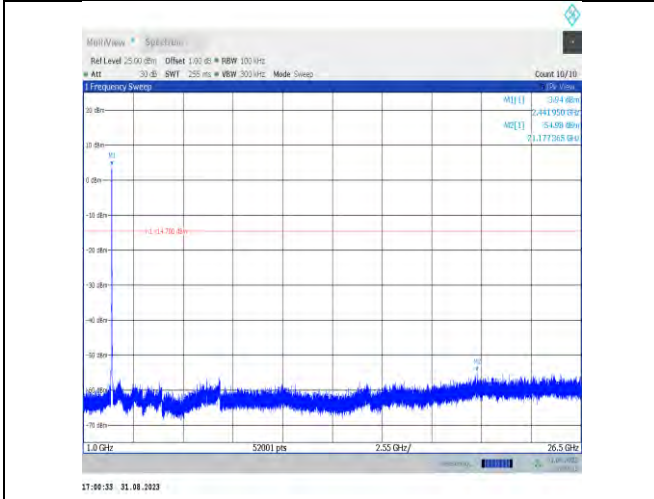
11ax20MIMO-Ant9-2437-1000~26500-PASS
