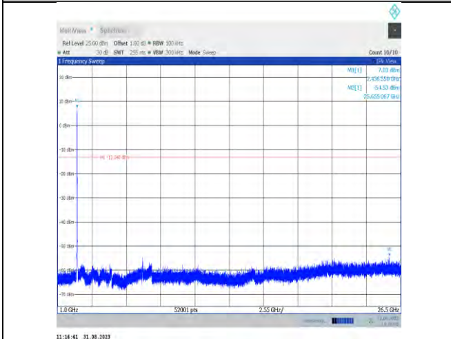
11n20MIMO-Ant9-2437-1000~26500-PASS
