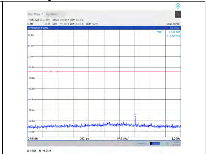
11n20MIMO-Ant7-2412-30~1000-PASS
