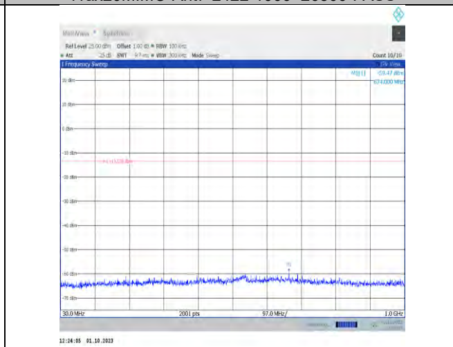
11ax20MIMO-Ant9-2422-30~1000-PASS
