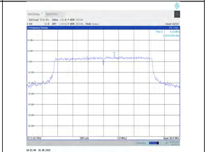
11ax20MIMO-Ant7-2412-0~Reference-PASS
