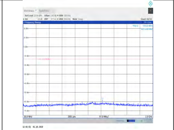
11n20MIMO-Ant9-2417-30~1000-PASS
