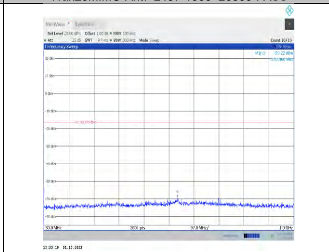
11ax20MIMO-Ant9-2457-30~1000-PASS
