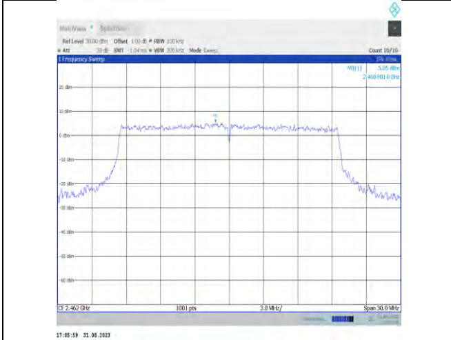
11ax20MIMO-Ant9-2462-0~Reference-PASS
