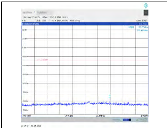
11ax20MIMO-Ant7-2422-30~1000-PASS
