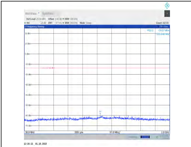
11ax20MIMO-Ant7-2447-30~1000-PASS
