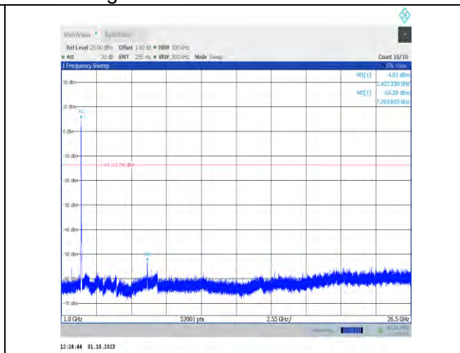
11ax20MIMO-Ant7-2422-1000~26500-PASS
