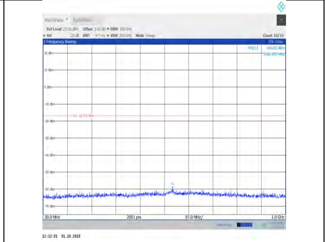
11n20MIMO-Ant9-2457-30~1000-PASS
