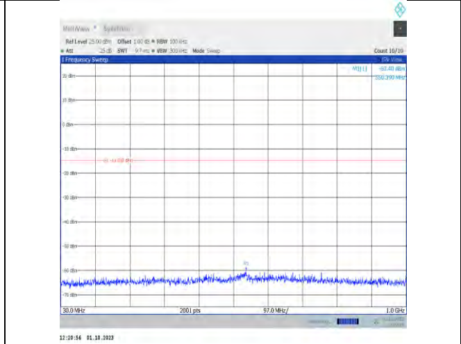
11ax20MIMO-Ant9-2417-30~1000-PASS
