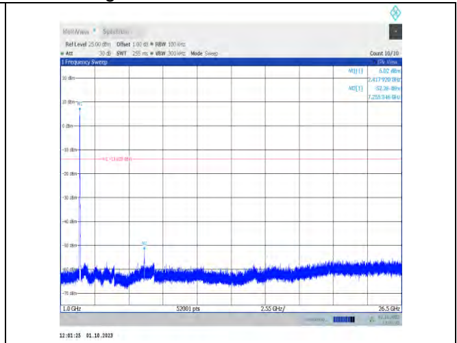
11n20MIMO-Ant7-2417-1000~26500-PASS
