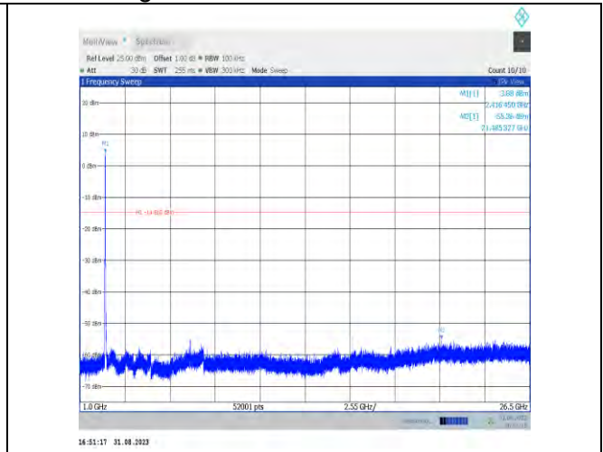
11ax20MIMO-Ant7-2412-1000~26500-PASS
