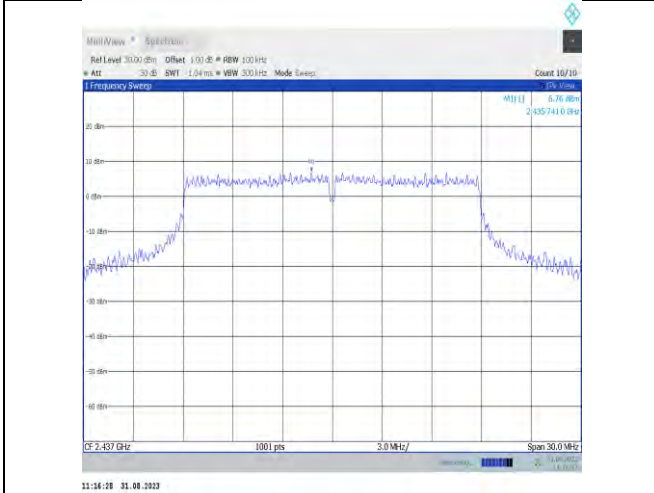
11n20MIMO-Ant9-2437-0~Reference-PASS
