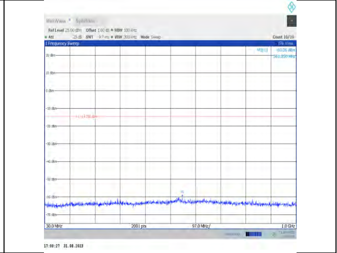
11ax20MIMO-Ant9-2437-30~1000-PASS
