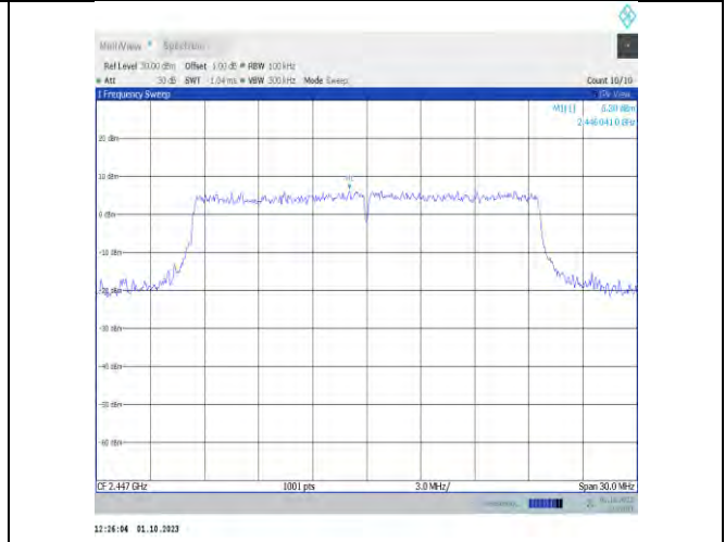
11ax20MIMO-Ant7-2447-0~Reference-PASS
