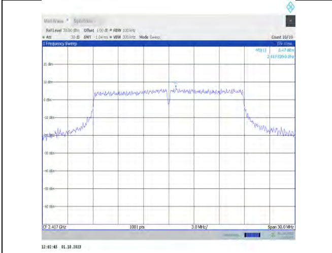
11n20MIMO-Ant9-2417-0~Reference-PASS
