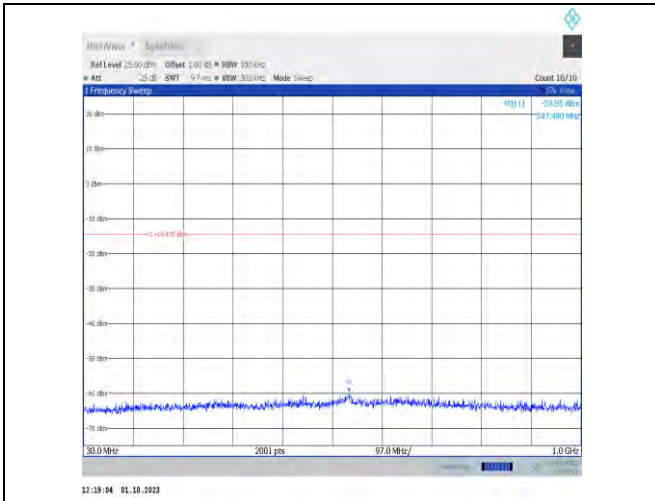
11ax20MIMO-Ant7-2417-30~1000-PASS
