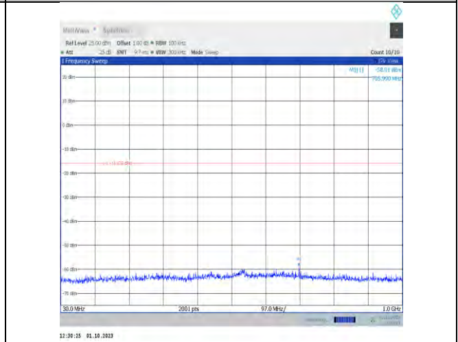
11ax20MIMO-Ant9-2452-30~1000-PASS
