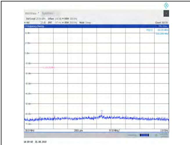
11ax20MIMO-Ant7-2437-30~1000-PASS
