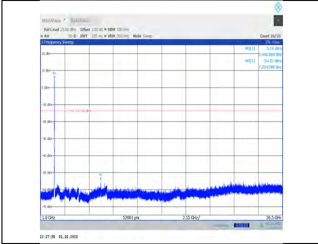
11ax20MIMO-Ant9-2447-1000~26500-PASS
