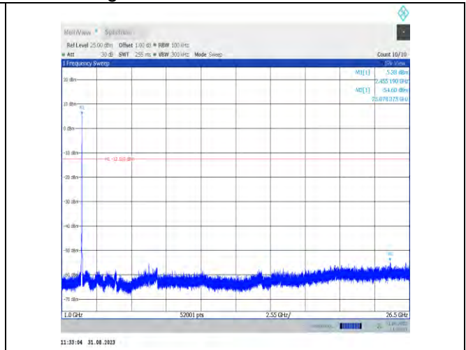
11n20MIMO-Ant7-2462-1000~26500-PASS
