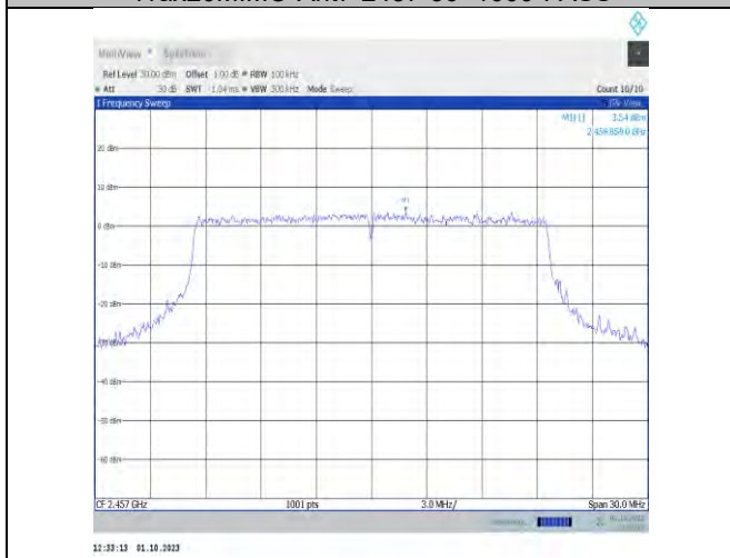
11ax20MIMO-Ant9-2457-0~Reference-PASS
