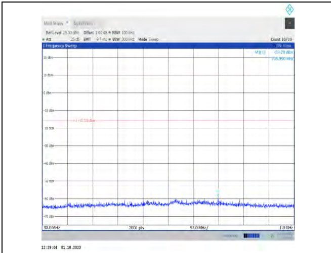
11ax20MIMO-Ant7-2452-30~1000-PASS
