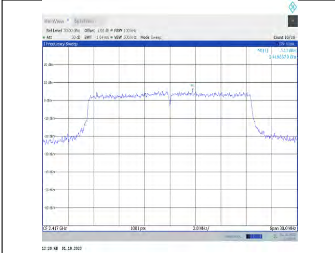
11ax20MIMO-Ant9-2417-0~Reference-PASS
