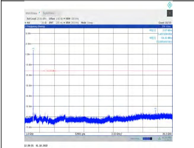
11ax20MIMO-Ant9-2452-1000~26500-PASS
