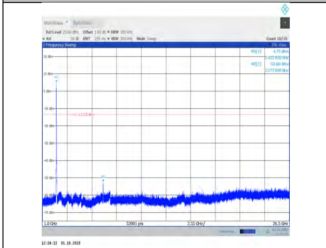
11ax20MIMO-Ant9-2422-1000~26500-PASS
