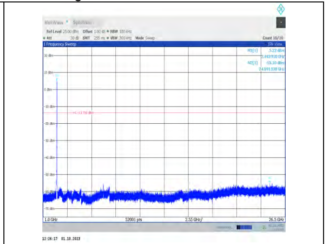
11ax20MIMO-Ant7-2447-1000~26500-PASS
