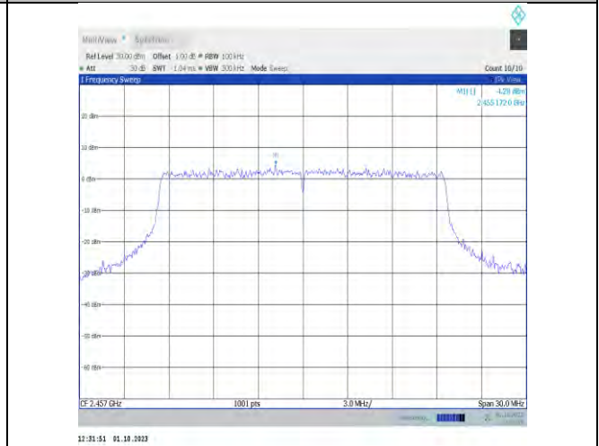
11ax20MIMO-Ant7-2457-0~Reference-PASS
