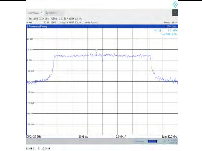
11ax20MIMO-Ant7-2422-0~Reference-PASS
