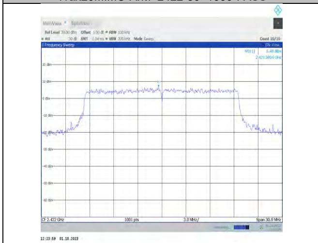
11ax20MIMO-Ant9-2422-0~Reference-PASS
