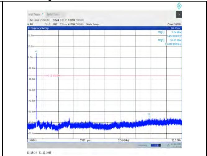
11n20MIMO-Ant7-2457-1000~26500-PASS
