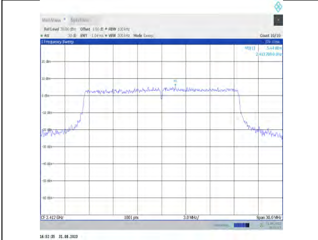
11ax20MIMO-Ant9-2412-0~Reference-PASS
