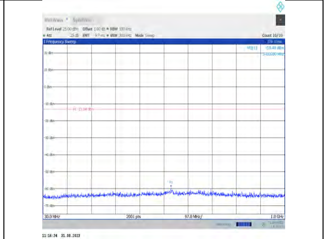
11n20MIMO-Ant9-2437-30~1000-PASS
