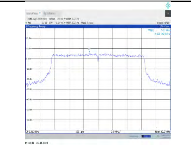
11ax20MIMO-Ant7-2462-0~Reference-PASS
