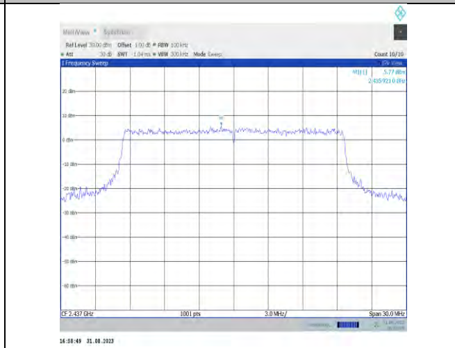
11ax20MIMO-Ant7-2437-0~Reference-PASS
