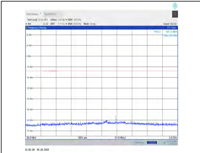
11n20MIMO-Ant7-2417-30~1000-PASS
