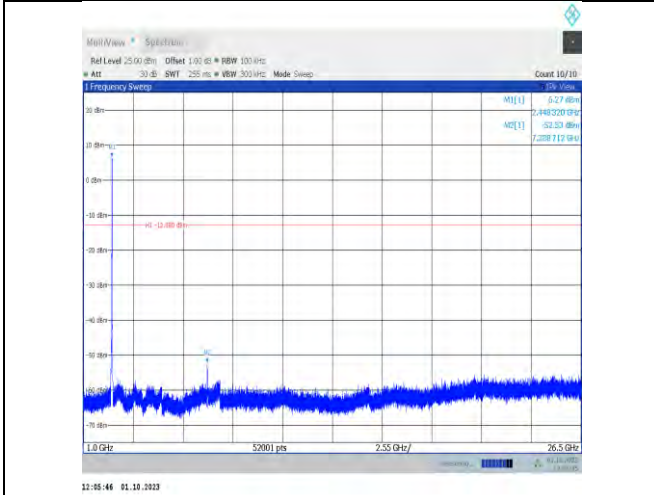
11n20MIMO-Ant9-2447-1000~26500-PASS
