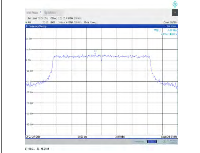
11ax20MIMO-Ant9-2437-0~Reference-PASS
