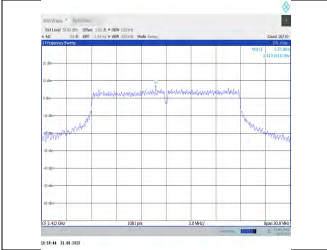
11n20MIMO-Ant9-2412-0~Reference-PASS
