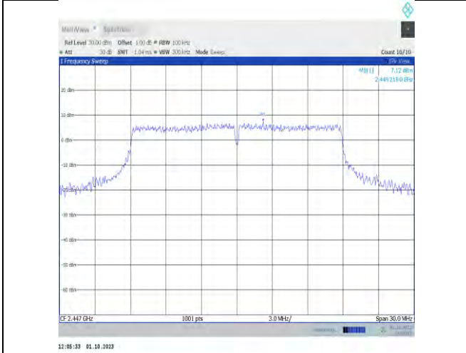
11n20MIMO-Ant9-2447-0~Reference-PASS
