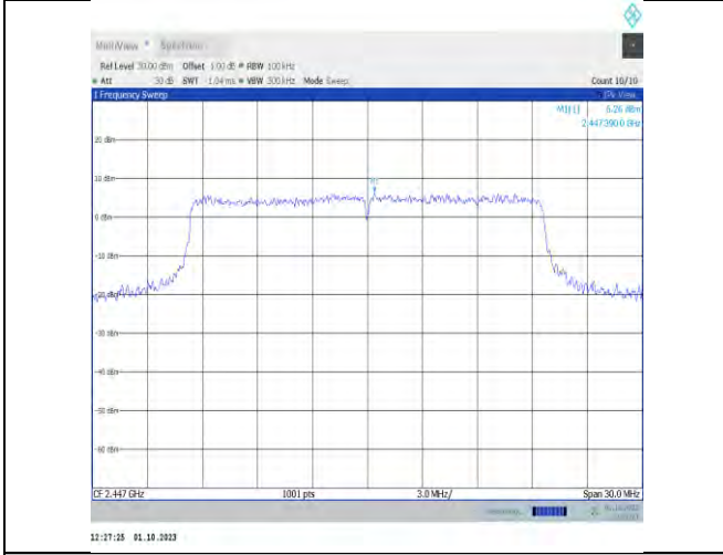
11ax20MIMO-Ant9-2447-0~Reference-PASS
