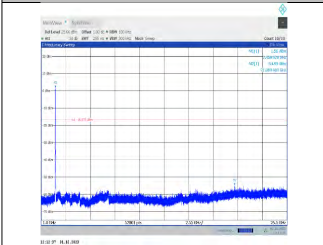
11n20MIMO-Ant9-2457-1000~26500-PASS
