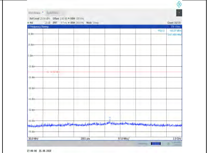
11ax20MIMO-Ant9-2462-30~1000-PASS
