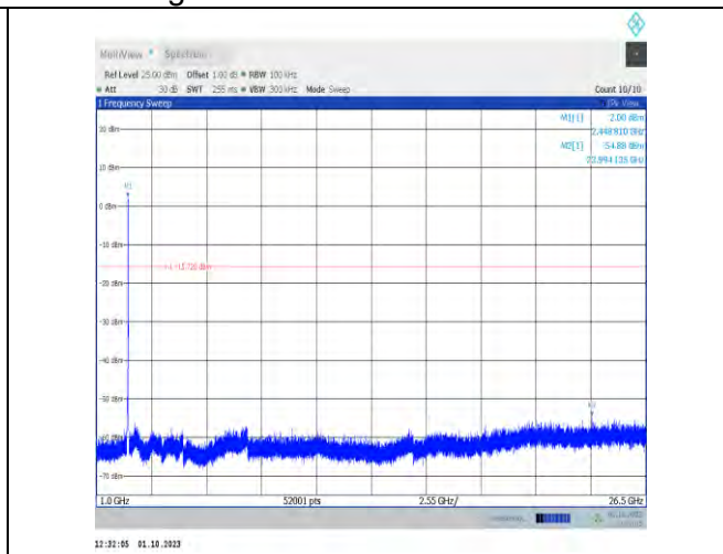
11ax20MIMO-Ant7-2457-1000~26500-PASS
