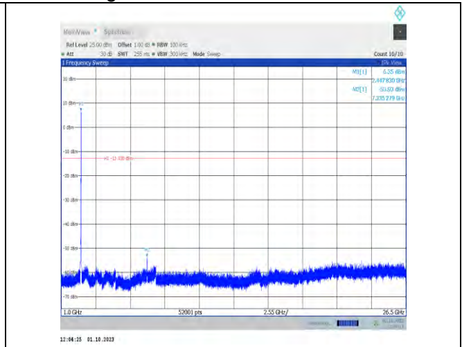
11n20MIMO-Ant7-2447-1000~26500-PASS
