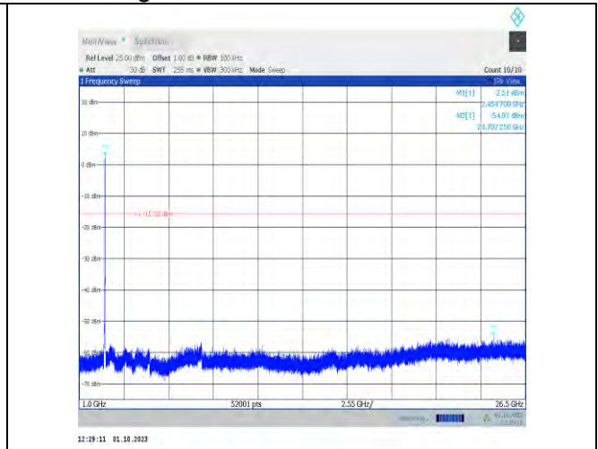
11ax20MIMO-Ant7-2452-1000~26500-PASS
