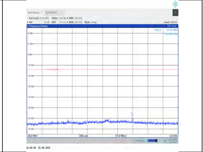
11n20MIMO-Ant9-2412-30~1000-PASS
