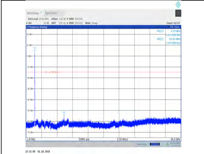
11ax20MIMO-Ant9-2417-1000~26500-PASS
