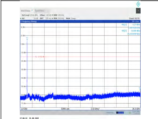
11ax20MIMO-Ant9-2462-1000~26500-PASS
