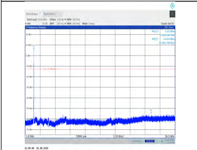
11n20MIMO-Ant9-2462-1000~26500-PASS
