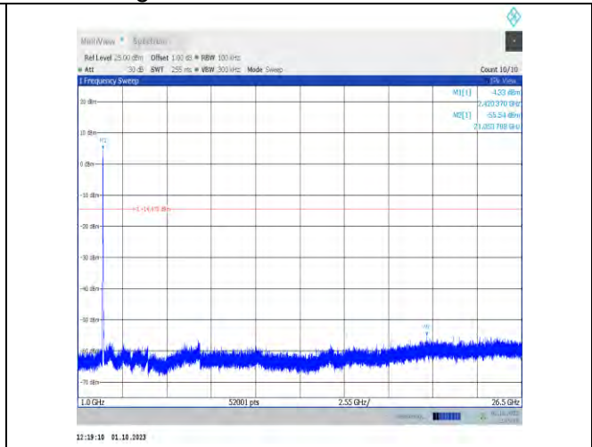
11ax20MIMO-Ant7-2417-1000~26500-PASS
