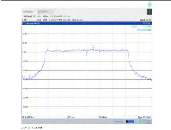
11ax20MIMO-Ant9-2452-0~Reference-PASS
