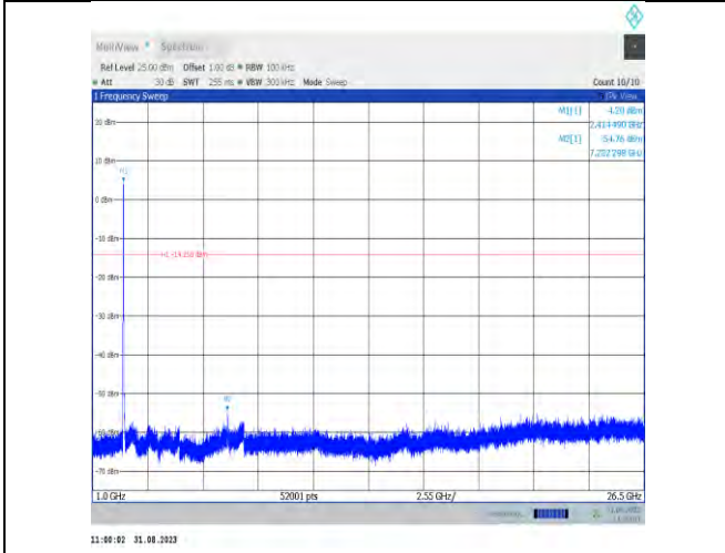
11n20MIMO-Ant9-2412-1000~26500-PASS
