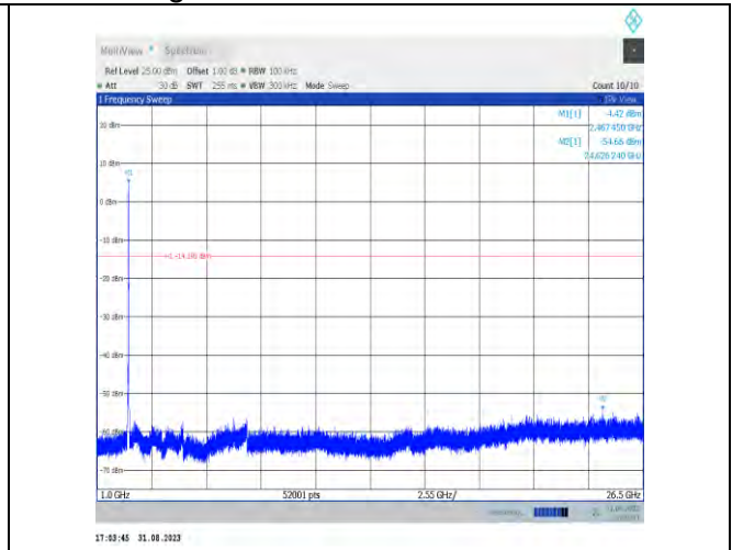
11ax20MIMO-Ant7-2462-1000~26500-PASS
