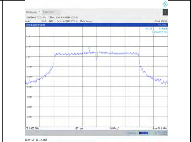
11n20MIMO-Ant7-2452-0~Reference-PASS
