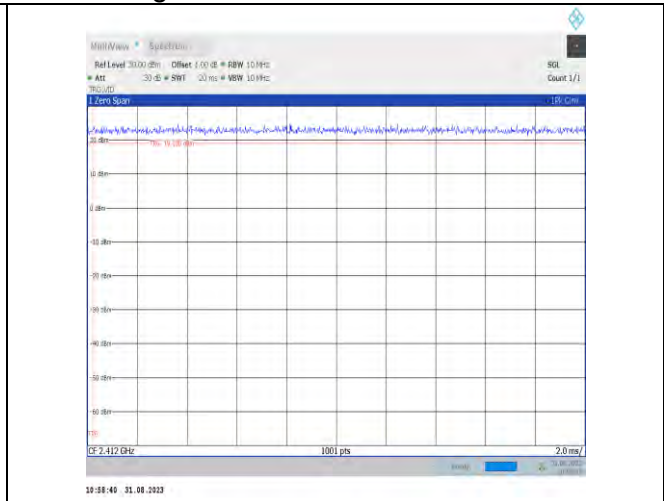
NTVN-11n20MIMO-Ant9-2412
