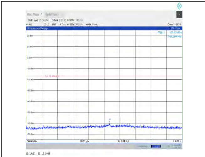
11n20MIMO-Ant7-2457-30~1000-PASS
