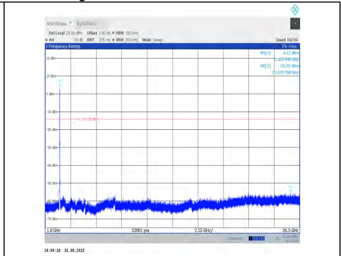
11ax20MIMO-Ant7-2437-1000~26500-PASS
