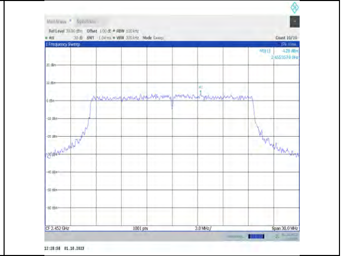
11ax20MIMO-Ant7-2452-0~Reference-PASS
