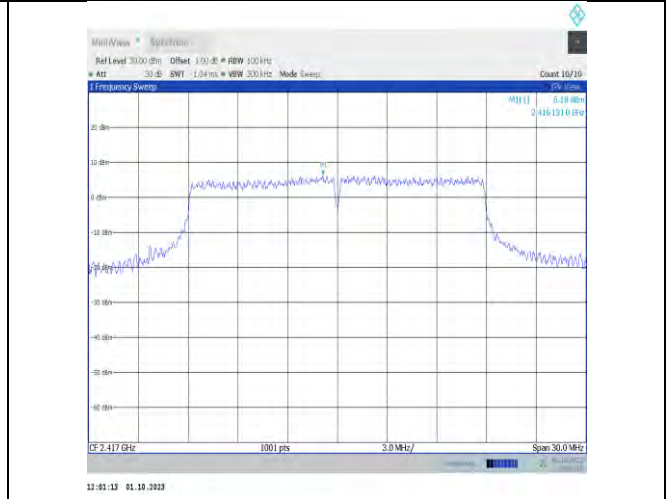
11n20MIMO-Ant7-2417-0~Reference-PASS
