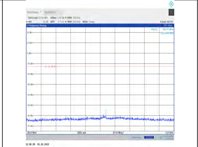
11n20MIMO-Ant9-2447-30~1000-PASS
