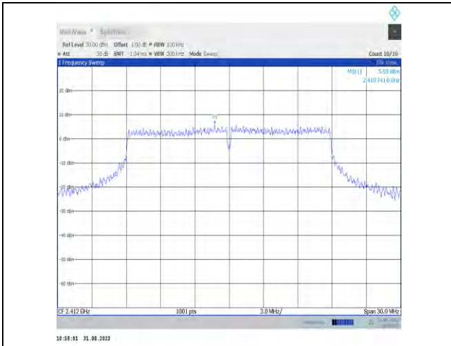
11n20MIMO-Ant7-2412-0~Reference-PASS
