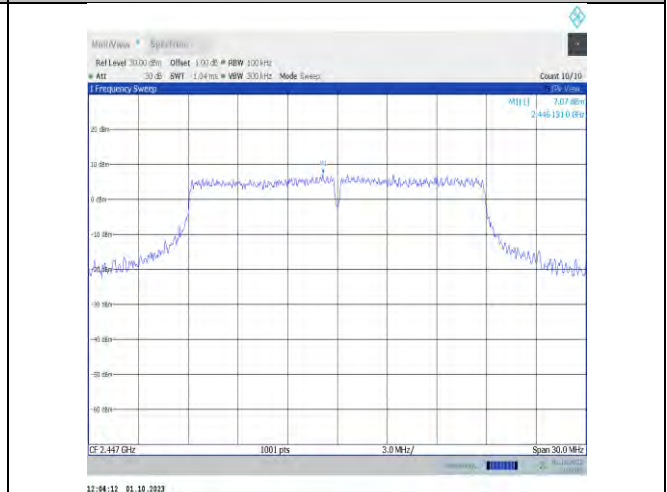
11n20MIMO-Ant7-2447-0~Reference-PASS
