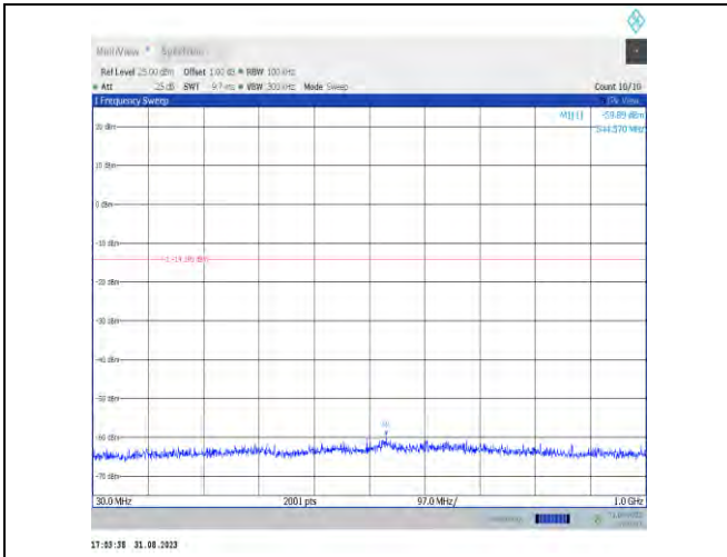
11ax20MIMO-Ant7-2462-30~1000-PASS
