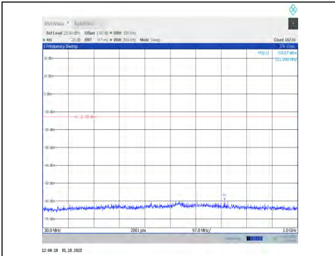
11n20MIMO-Ant7-2447-30~1000-PASS
