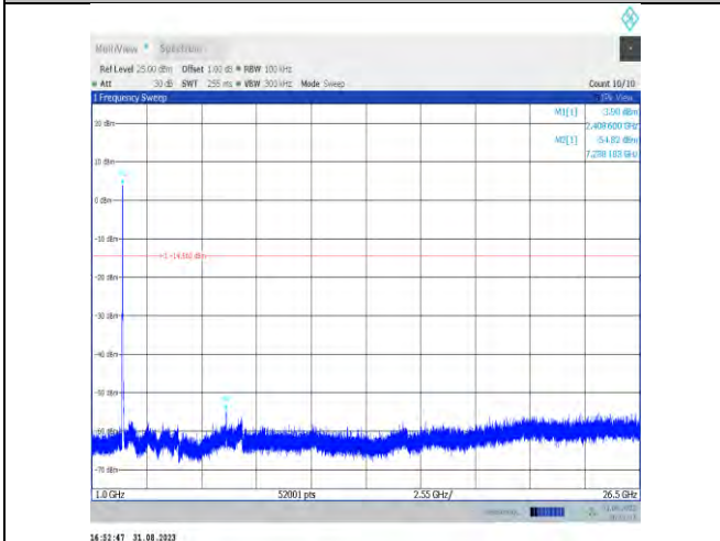
11ax20MIMO-Ant9-2412-1000~26500-PASS
