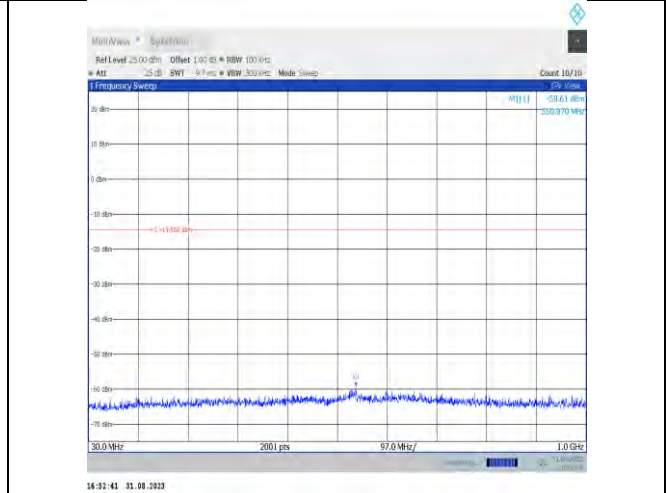
11ax20MIMO-Ant9-2412-30~1000-PASS
