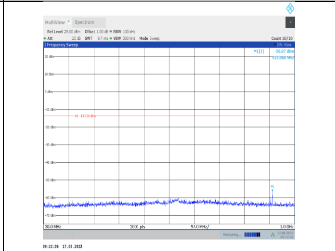
DH5-Ant7-2480-30~1000-PASS
