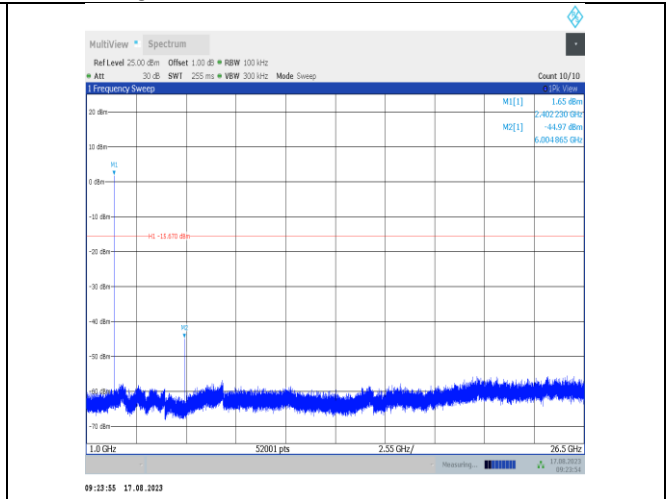
2DH5-Ant7-2402-1000~26500-PASS
