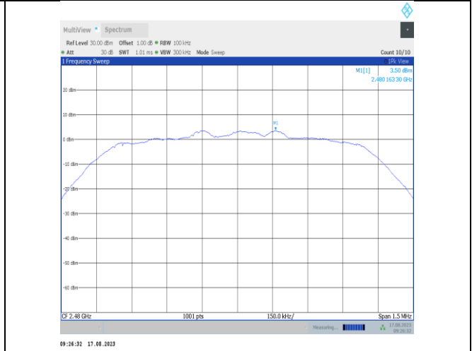
2DH5-Ant7-2480-0~Reference-PASS
