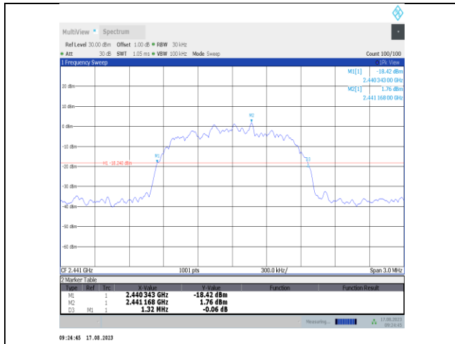
2DH5-Ant7-2441
