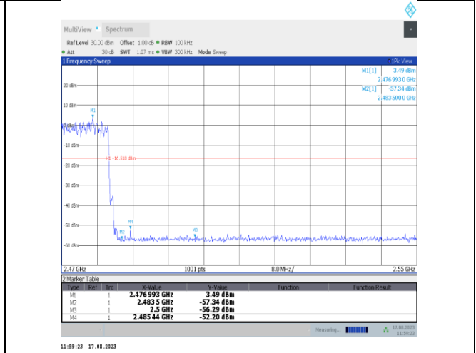
2DH5-Ant7-Hop_2480-PASS
