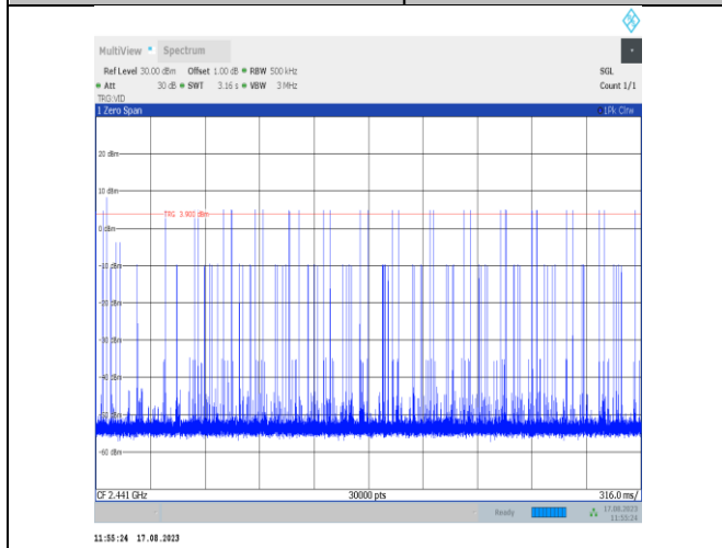
2DH1-Ant7-Hop-PASS
