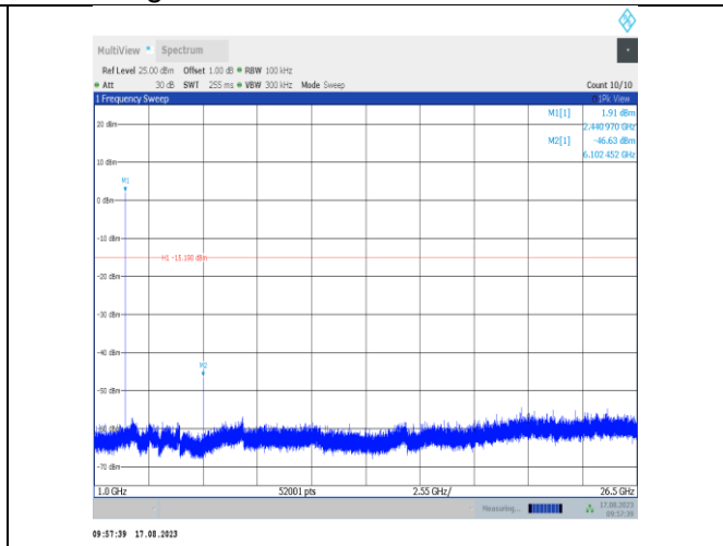
3DH5-Ant7-2441-1000~26500-PASS
