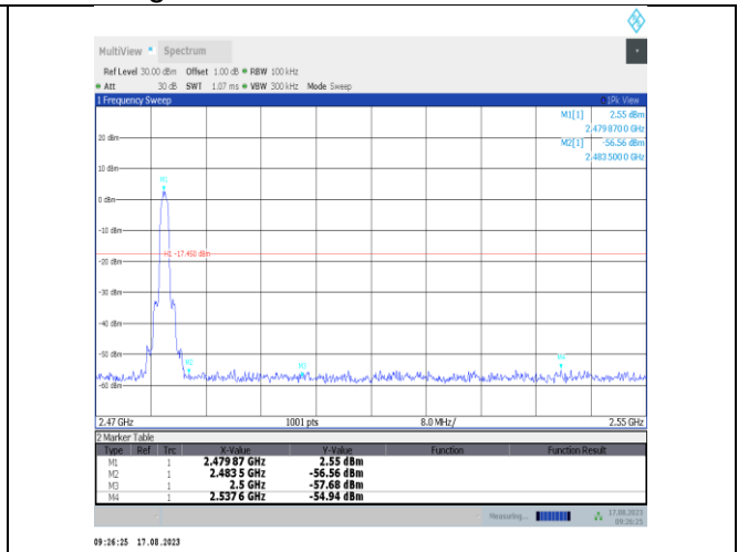
2DH5-Ant7-2480-PASS
