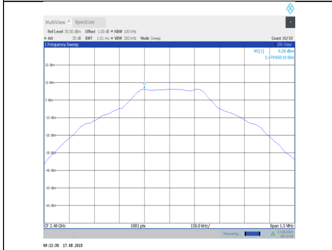
DH5-Ant7-2480-0~Reference-PASS
