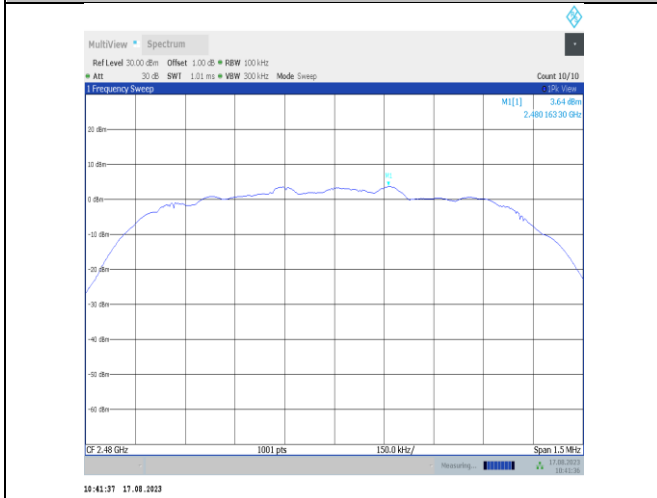
3DH5-Ant7-2480-0~Reference-PASS
