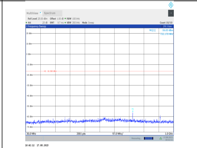
3DH5-Ant7-2480-30~1000-PASS
