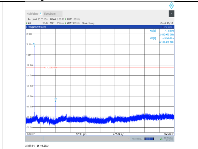
DH5-Ant7-2441-1000~26500-PASS
