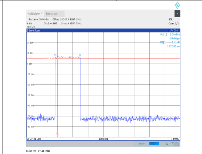
2DH3-Ant7-Hop-PASS
