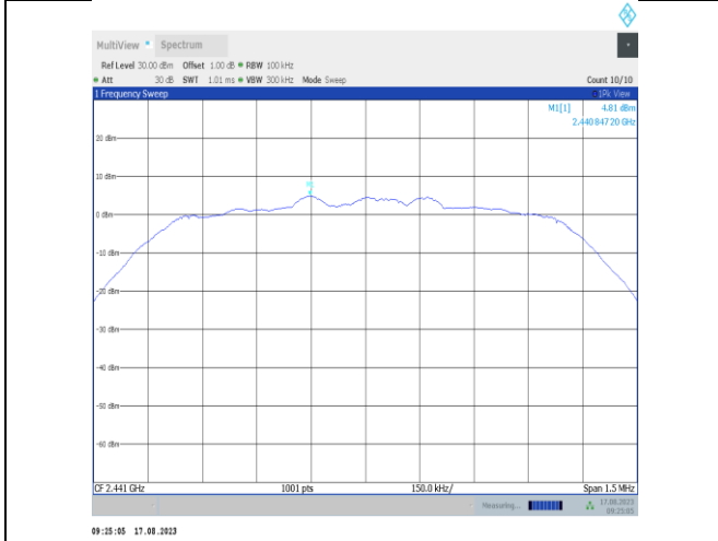
2DH5-Ant7-2441-0~Reference-PASS
