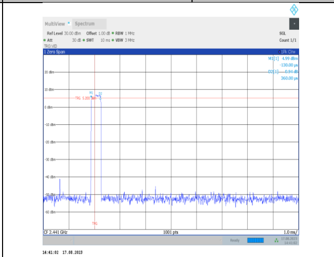
3DH1-Ant7-Hop-PASS
