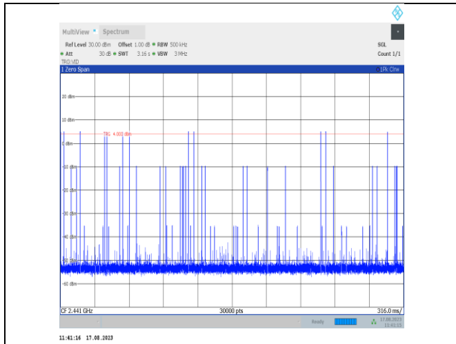
2DH5-Ant7-Hop-PASS
