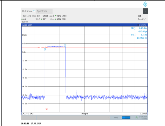
3DH3-Ant7-Hop-PASS
