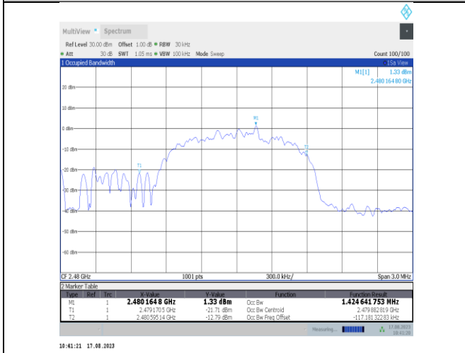
3DH5-Ant7-2480
