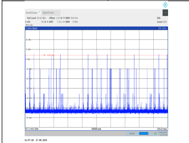
2DH3-Ant7-Hop-PASS
