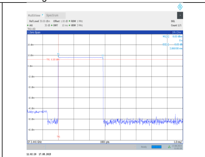
DH5-Ant7-Hop-PASS
