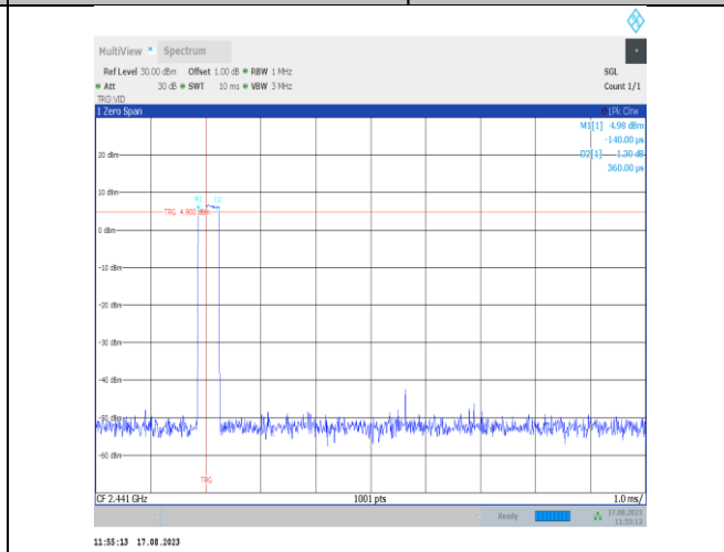
2DH1-Ant7-Hop-PASS
