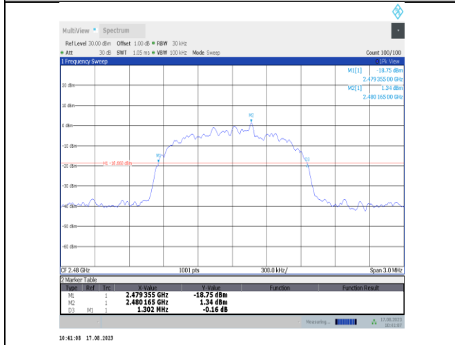
3DH5-Ant7-2480
