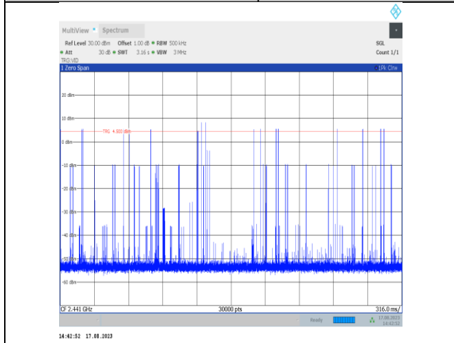
3DH3-Ant7-Hop-PASS
