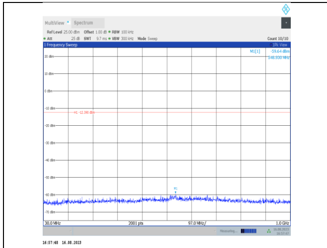
DH5-Ant7-2441-30~1000-PASS
