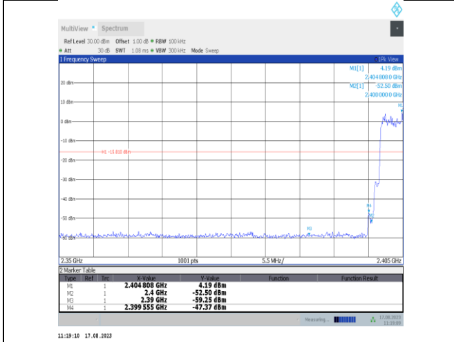
2DH5-Ant7-Hop_2402-PASS
