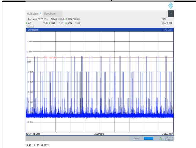
3DH1-Ant7-Hop-PASS
