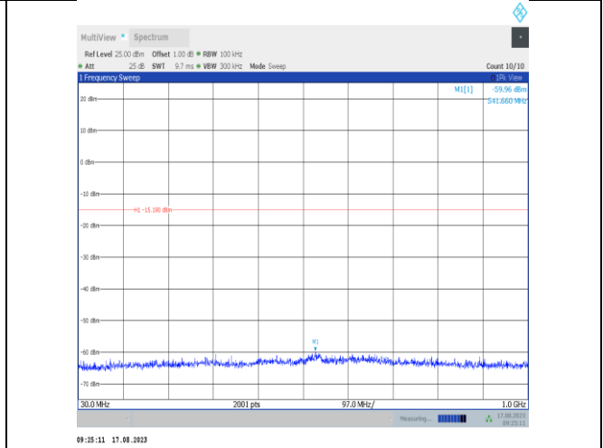
2DH5-Ant7-2441-30~1000-PASS
