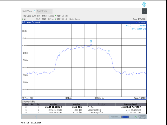
3DH5-Ant7-2441
