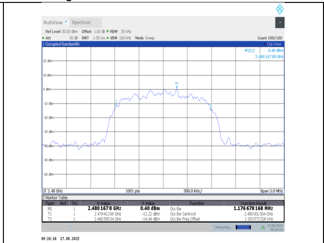
2DH5-Ant7-2480
