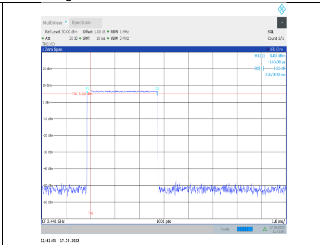
2DH5-Ant7-Hop-PASS
