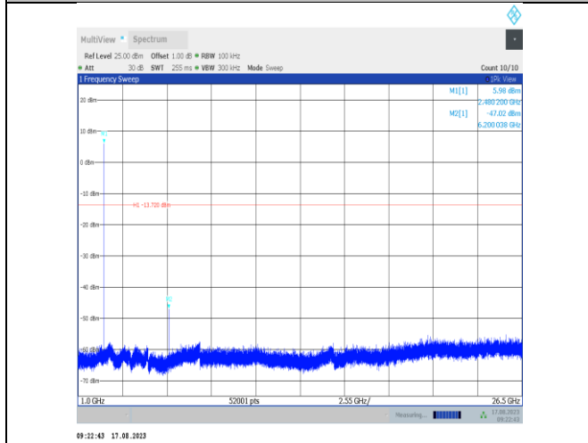
DH5-Ant7-2480-1000~26500-PASS
