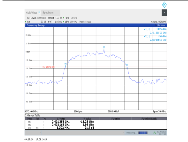
3DH5-Ant7-2402
