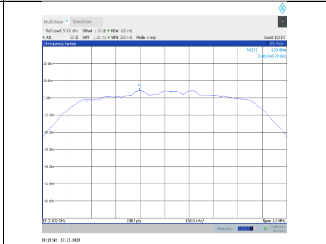
2DH5-Ant7-2402-0~Reference-PASS
