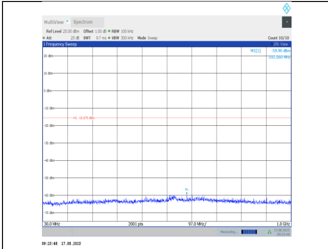
2DH5-Ant7-2402-30~1000-PASS
