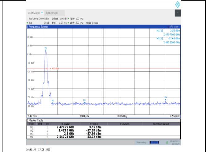
3DH5-Ant7-2480-PASS
