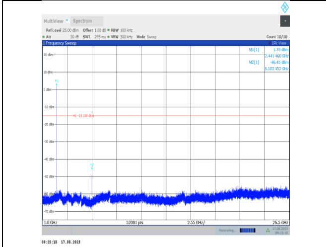
2DH5-Ant7-2441-1000~26500-PASS
