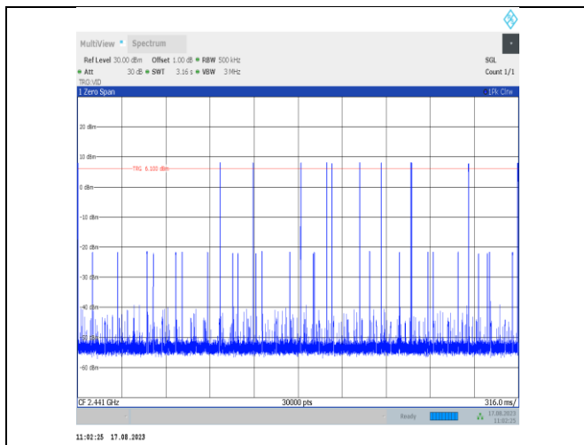
DH5-Ant7-Hop-PASS
