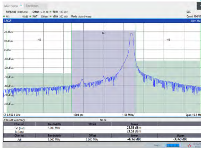
Band48-5MHz-QPSK-55265-1RB#24
