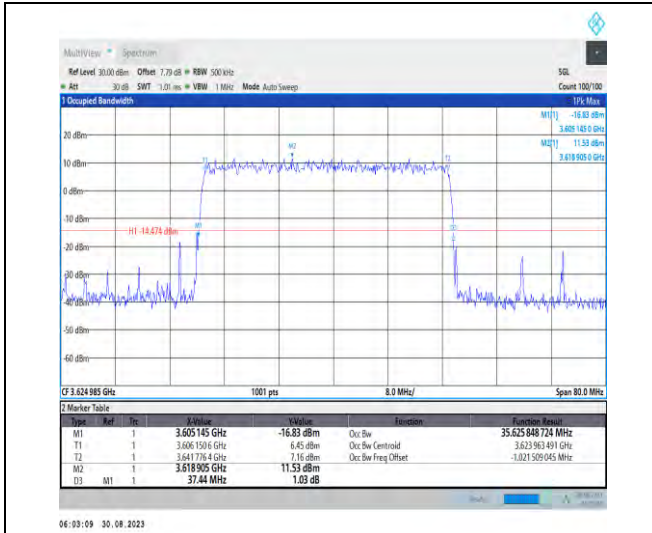
1-N48-PC3-30-40-M-1-DFT-QPSK-Outer_Full-100@ 0-Ant5-35.626-37.440-≤40-PASS
