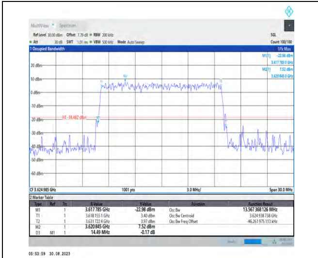
1-N48-PC3-30-15-M-8-CP-64QAM-Outer_Full-38@0 -Ant5-13.567-14.490-≤15-PASS
