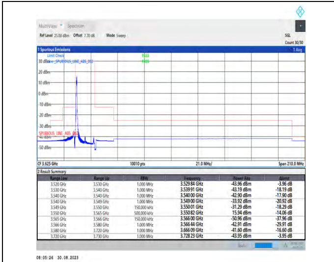
1-N48-PC3-30-15-L-1-DFT-PI2BPSK-Edge_1RB_Left-1@0-Ant5-1--PASS-see graph
