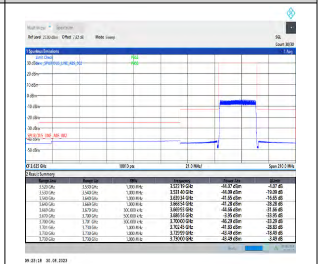
1-N48-PC3-30-30-H-6-CP-QPSK-Outer_Full-78@ 0-Ant5-1--PASS-see graph
