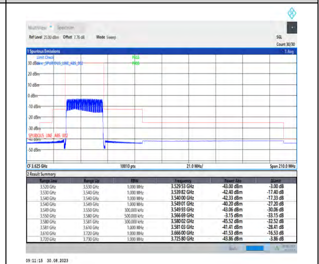
1-N48-PC3-30-30-L-6-CP-QPSK-Outer_Full-78@0-Ant5-1--PASS-see graph
