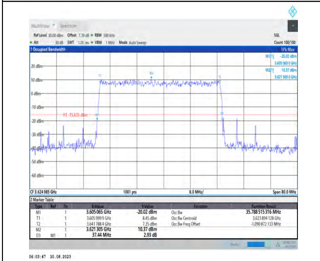
1-N48-PC3-30-40-M-3-DFT-16QAM-Outer_Full-100@0-Ant5-35.789-37.440-≤40-PASS
