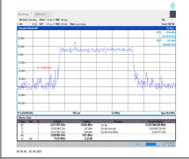
1-N48-PC3-30-15-M-6-CP-QPSK-Outer_Full-38@0- Ant5-13.598-14.250-≤15-PASS
