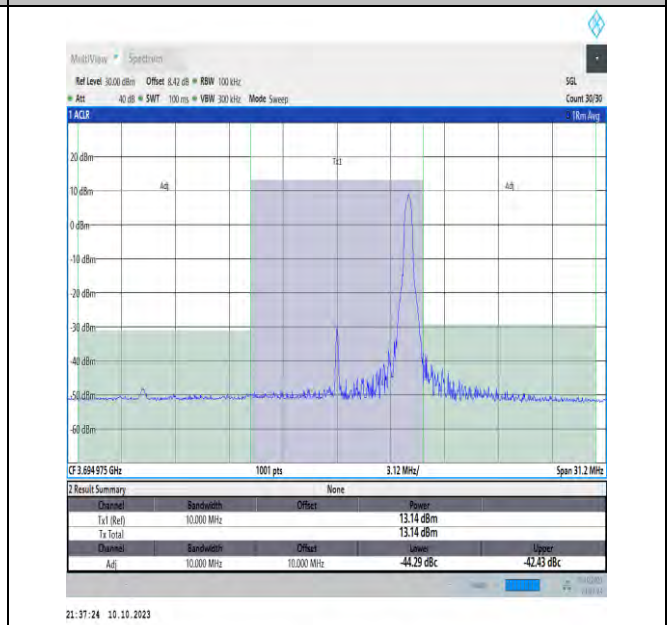
NTVN_N48_PC3_30_10_H_TID18_#1_-10_10
