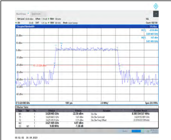
1-N48-PC3-30-10-M-9-CP-256QAM-Outer_Full-24@ 0-Ant5-8.586-9.080-≤10-PASS
