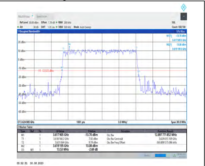
1-N48-PC3-30-15-M-1-DFT-QPSK-Outer_Full-36@ -Ant5-12.898-13.530-≤15-PASS
