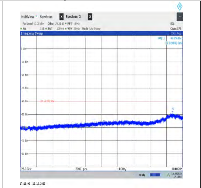
NTVN_N48_PC3_30_40_M_TID1_NS_01_26000_40000_#1
