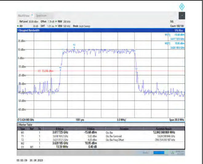
1-N48-PC3-30-15-M-3-DFT-16QAM-Outer_Full-36@ 0-Ant5-12.843-13.590-≤15-PASS
