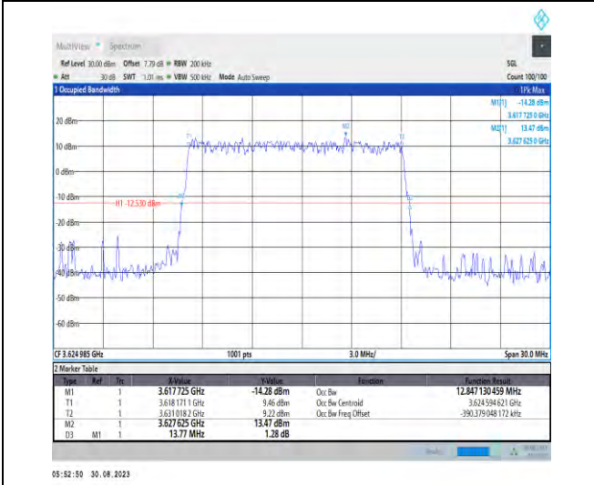
1-N48-PC3-30-15-M-2-DFT-PI2BPSK-Outer_Full-36@ @0-Ant5-12.847-13.770-≤15-PASS
