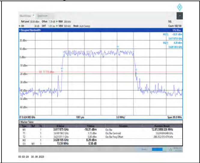
1-N48-PC3-30-15-M-5-DFT-256QAM-Outer_Full-36@ 0-Ant5-12.813-13.590-≤15-PASS
