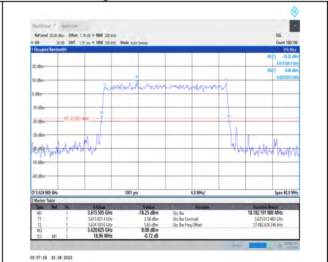
1-N48-PC3-30-20-M-8-CP-64QAM-Outer_Full-51@0 -Ant5-18.182-18.960-<20-PASS
