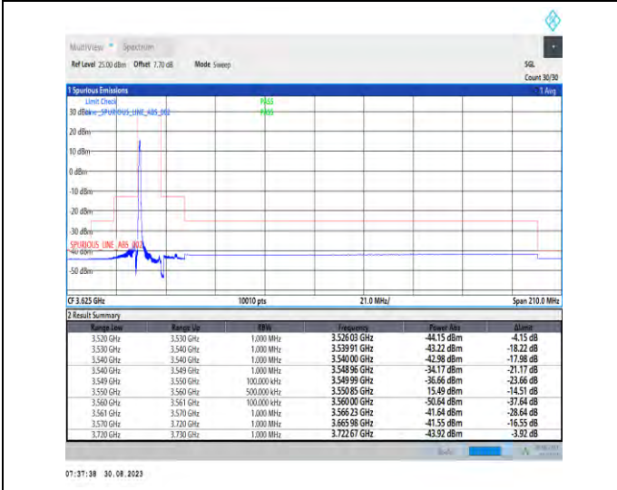
1-N48-PC3-30-10-L-1-DFT-PI2BPSK-Edge_1RB_Left-1@0-Ant5-1--PASS-see graph
