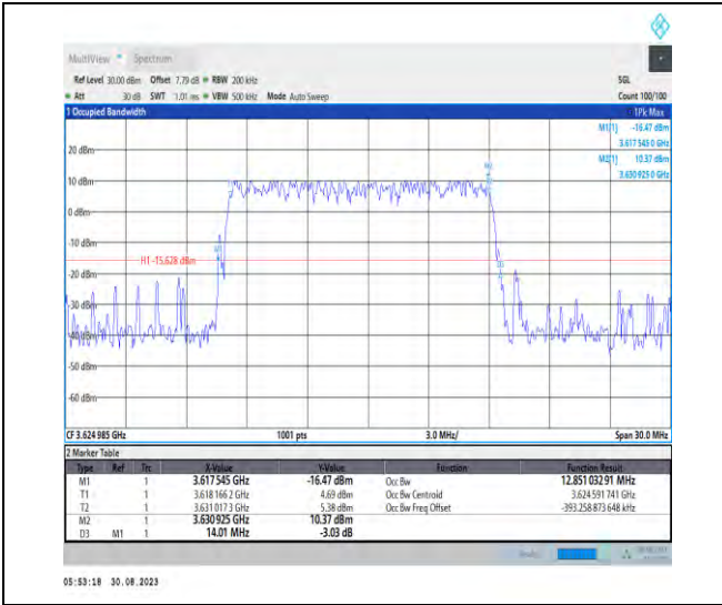
1-N48-PC3-30-15-M-4-DFT-64QAM-Outer_Full-36@ 0-Ant5-12.851-14.010-≤15-PASS
