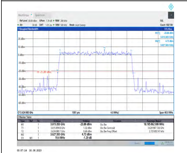
1-N48-PC3-30-20-M-9-CP-256QAM-Outer_Full-51@0 0-Ant5-18.186-19.400-<20-PASS
