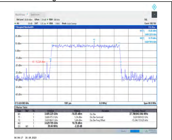
1-N48-PC3-30-40-M-6-CP-QPSK-Outer_Full-106@0 -Ant5-37.789-39.440-≤40-PASS
