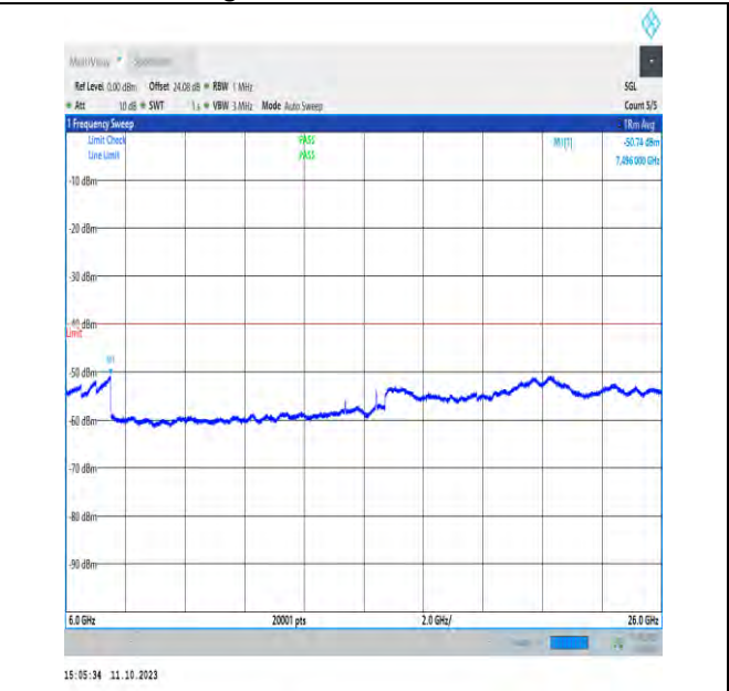
NTNV_N48_PC3_30_40_L_TID1_NS_01_6000_26000_#1
