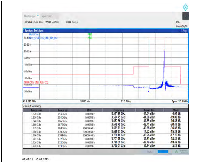
1-N48-PC3-30-20-H-2-DFT-PI2BPSK-Edge_1RB_Right-t-1@50-Ant5-1--PASS-see graph
