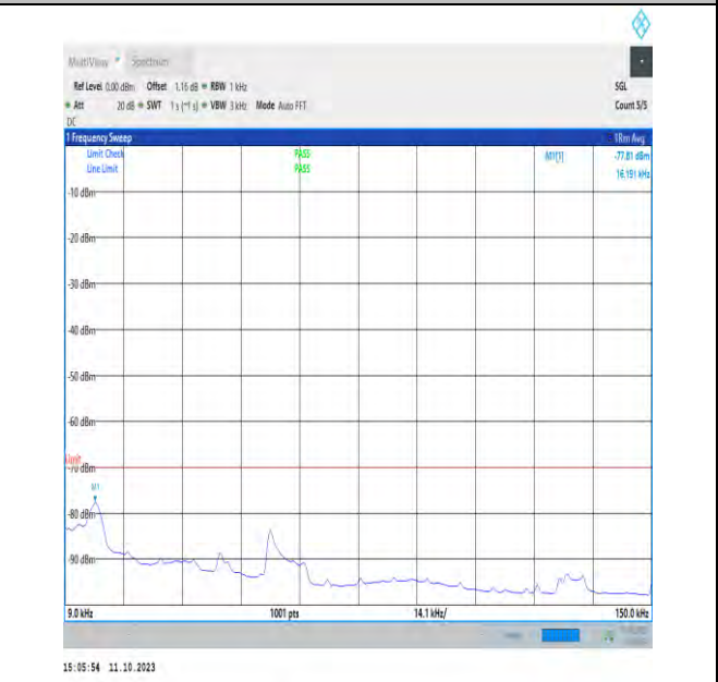
NTNV_N48_PC3_30_40_M_TID1_NS_01_0.009_0.15_#1
