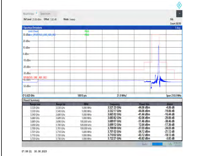
1-N48-PC3-30-10-H-5-CP-QPSK-Edge_1RB_Right-1 @23-Ant5-1--PASS-see graph
