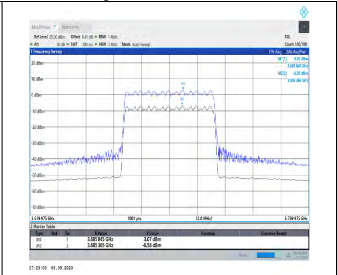
1-N48-PC3-30-40-H-2-CP-256QAM-Outer_Full-106 @0-Ant5-9.65-100%-0.00-9.65-PASS-≤13
