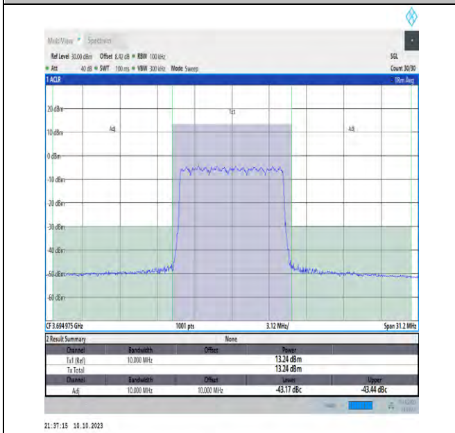
NTVN_N48_PC3_30_10_H_TID16_#1_-10_10
