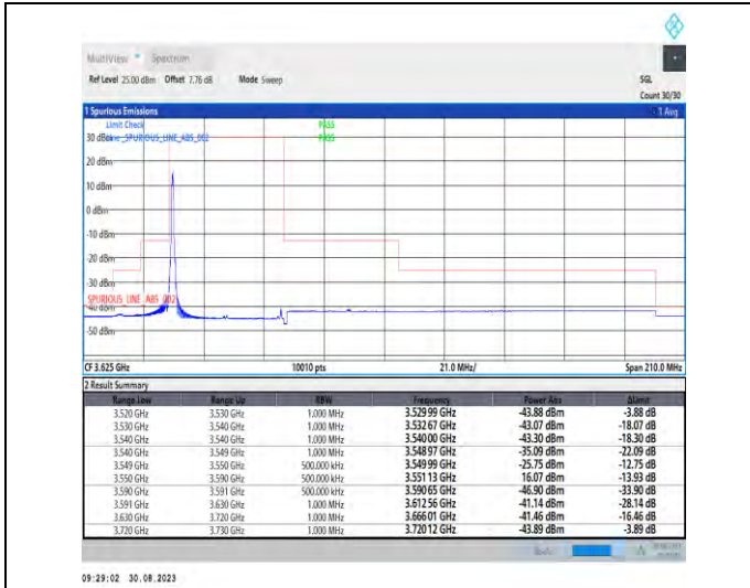
1-N48-PC3-30-40-L-1-DFT-PI2BPSK-Edge_1RB_Left-1@0-Ant5-1--PASS-see graph
