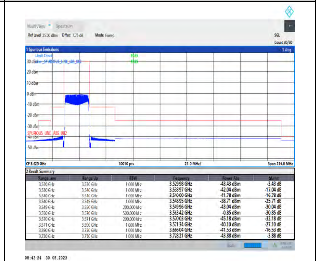
1-N48-PC3-30-20-L-6-CP-QPSK-Outer_Full-51@0-Ant5-1--PASS-see graph
