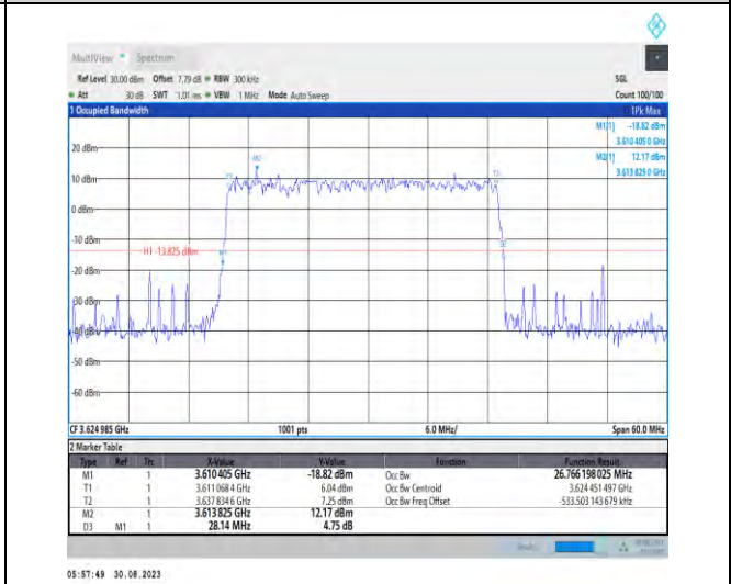
1-N48-PC3-30-30-M-1-DFT-QPSK-Outer_Full-75@0 -Ant5-26.766-28.140-<30-PASS
