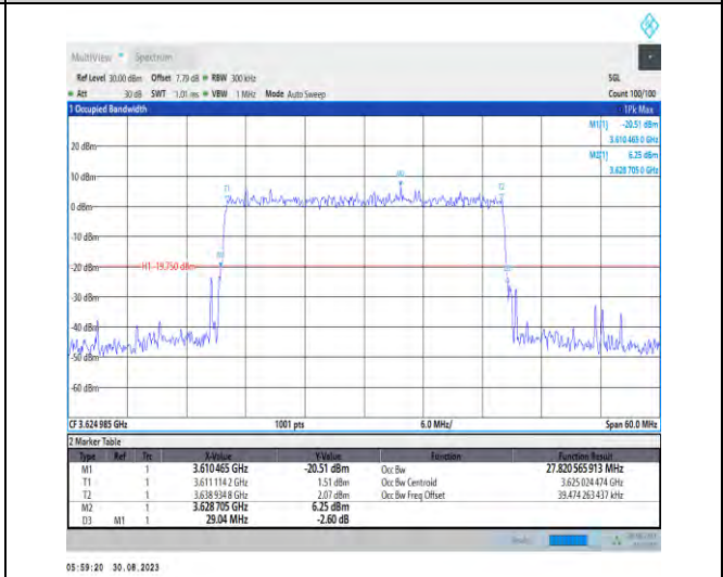
1-N48-PC3-30-30-M-9-CP-256QAM-Outer_Full-78@0-Ant5-27.821-29.040-≤30-PASS
