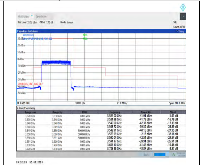
1-N48-PC3-30-40-L-3-DFT-PI2BPSK-Outer_Full-100@0-Ant5-1--PASS-see graph
