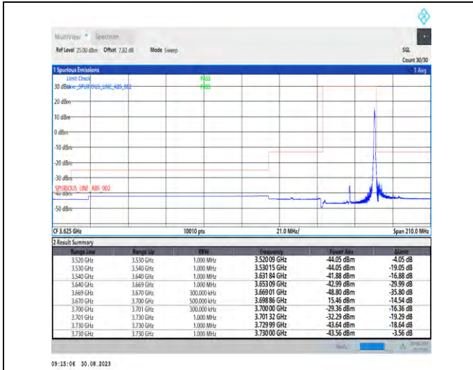
1-N48-PC3-30-30-H-2-DFT-PI2BPSK-Edge_1RB_Righ t-1@77-Ant5-1--PASS-see graph
