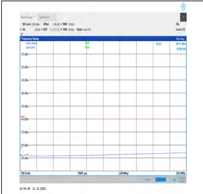
NTNV_N48_PC3_30_40_M_TID1_NS_01_0.15_30_#1
