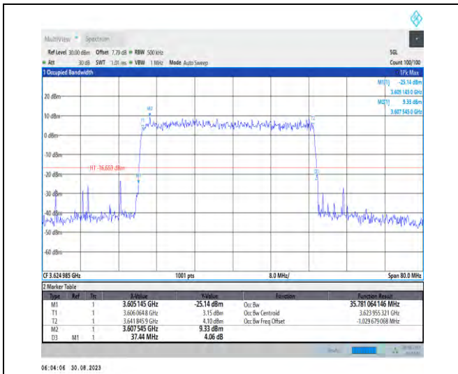
1-N48-PC3-30-40-M-5-DFT-256QAM-Outer_Full-100 @0-Ant5-35.781-37.440-≤40-PASS
