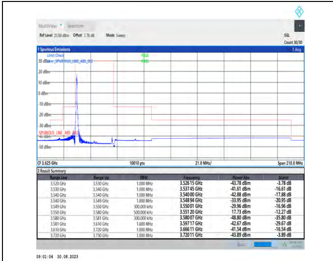
1-N48-PC3-30-30-L-1-DFT-PI2BPSK-Edge_1RB_Left-1@0-Ant5-1--PASS-see graph
