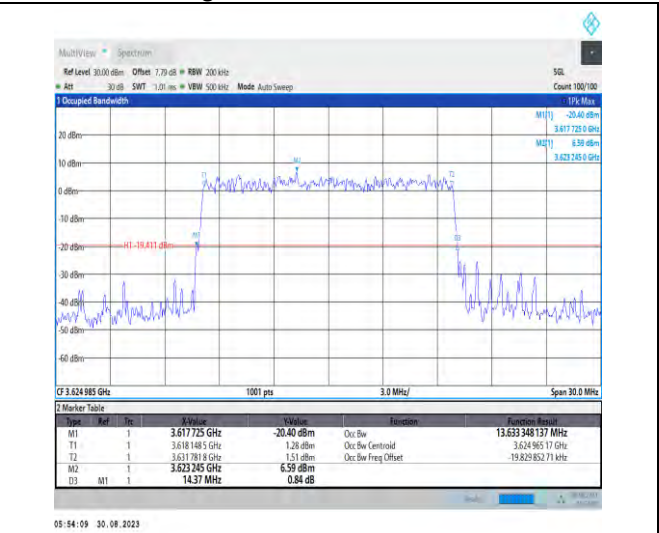
1-N48-PC3-30-15-M-9-CP-256QAM-Outer_Full-38@0-Ant5-13.633-14.370-≤15-PASS
