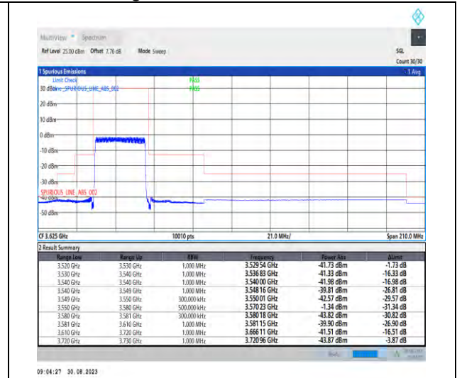
1-N48-PC3-30-30-L-3-DFT-PI2BPSK-Outer_Full-75@0-Ant5-1--PASS-see graph
