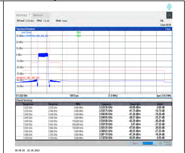
1-N48-PC3-30-15-L-3-DFT-PI2BPSK-Outer_Full-36@0-Ant5-1--PASS-see graph
