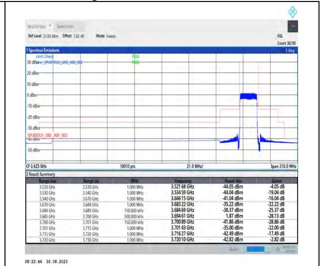
1-N48-PC3-30-15-H-3-DFT-PI2BPSK-Outer_Full-3 6@0-Ant5-1--PASS-see graph
