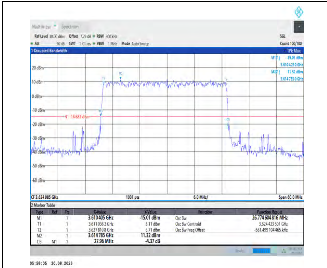
1-N48-PC3-30-30-M-2-DFT-PI2BPSK-Outer_Full-75 @0-Ant5-26.775-27.960-≤30-PASS
