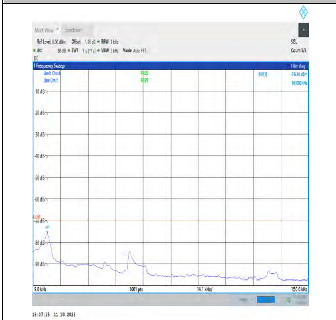
NTVN_N48_PC3_30_40_H_TID1_NS_01_0.009_0.15_#1
