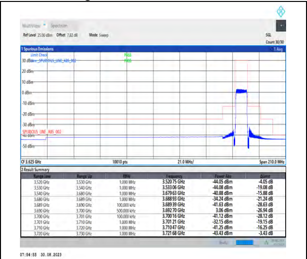
1-N48-PC3-30-10-H-3-DFT-PI2BPSK-Outer_Full-2 4@0-Ant5-1--PASS-see graph
