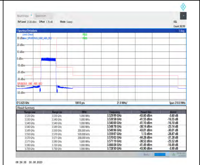
1-N48-PC3-30-20-L-3-DFT-PI2BPSK-Outer_Full-50@0-Ant5-1--PASS-see graph
