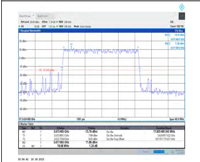
1-N48-PC3-30-20-M-1-DFT-QPSK-Outer_Full-50@0 -Ant5-17.835-18.680-≤20-PASS
