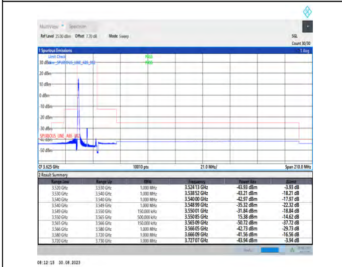
1-N48-PC3-30-15-L-4-CP-QPSK-Edge_1RB_Left-1@0-Ant5-1--PASS-see graph
