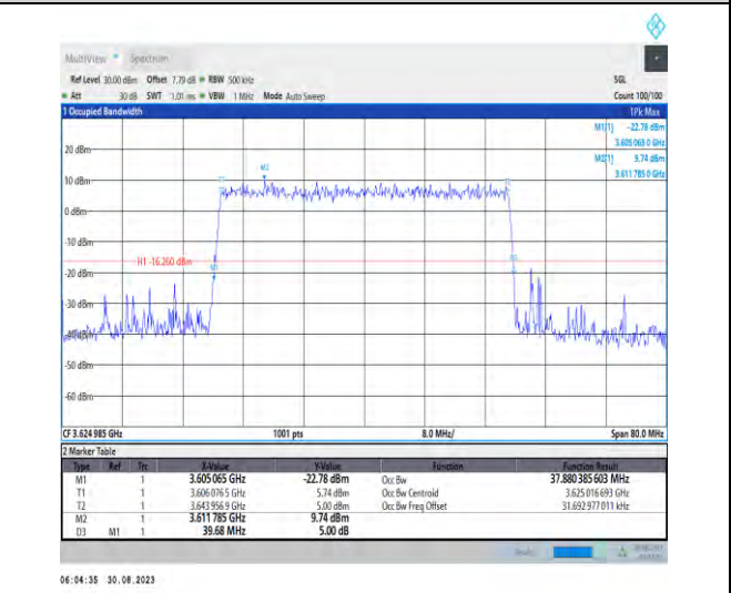
1-N48-PC3-30-40-M-8-CP-64QAM-Outer_Full-106@0-Ant5-37.88-39.680-≤40-PASS
