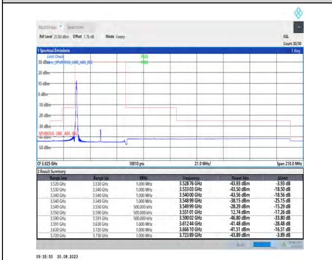
1-N48-PC3-30-40-L-4-CP-QPSK-Edge_1RB_Left-1@0-Ant5-1--PASS-see graph
