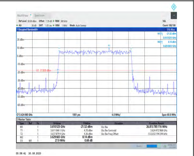
1-N48-PC3-30-30-M-5-DFT-256QAM-Outer_Full-75 @0-Ant5-26.814-27.900-≤30-PASS
