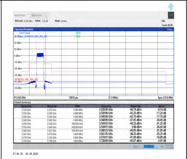
1-N48-PC3-30-10-L-3-DFT-PI2BPSK-Outer_Full-24@0-Ant5-1--PASS-see graph
