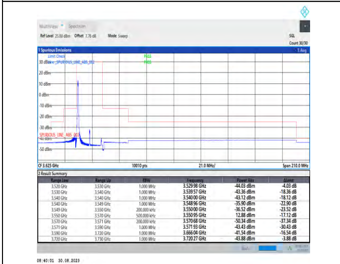
1-N48-PC3-30-20-L-4-CP-QPSK-Edge_1RB_Left-1@0-Ant5-1--PASS-see graph
