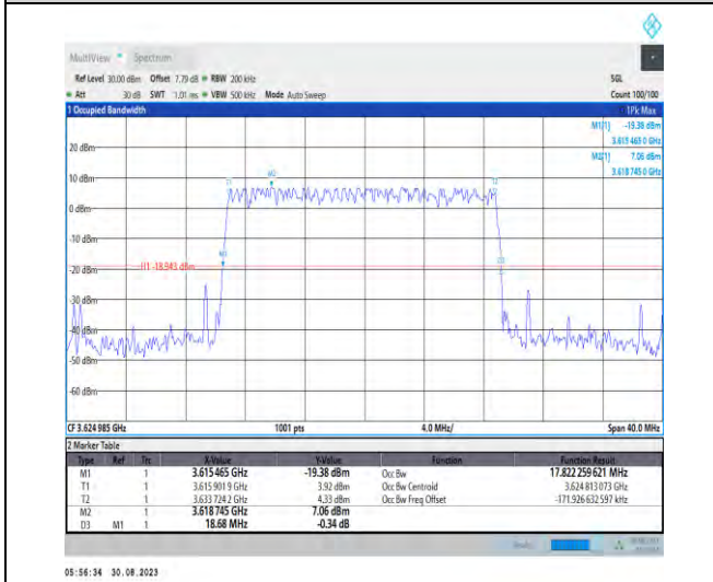
1-N48-PC3-30-20-M-5-DFT-256QAM-Outer_Full-50@ 0-Ant5-17.822-18.680-≤20-PASS
