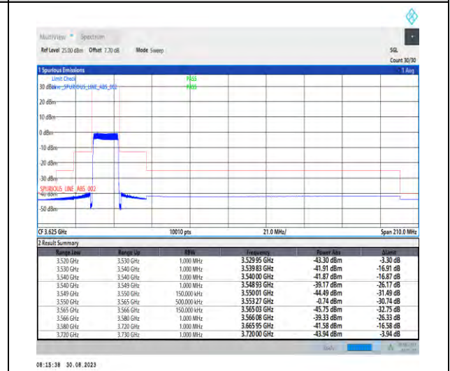
1-N48-PC3-30-15-L-6-CP-QPSK-Outer_Full-38@0-Ant5-1--PASS-see graph
