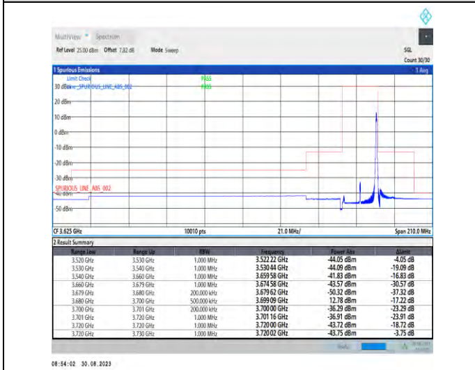
1-N48-PC3-30-20-H-5-CP-QPSK-Edge_1RB_Right-1@50-Ant5-1--PASS-see graph
