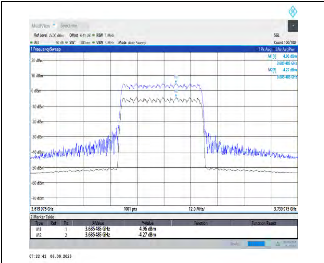
1-N48-PC3-30-40-H-1-DFT-256QAM-Outer_Full-100 @0-Ant5-9.23-100%-0.00-9.23-PASS-≤13
