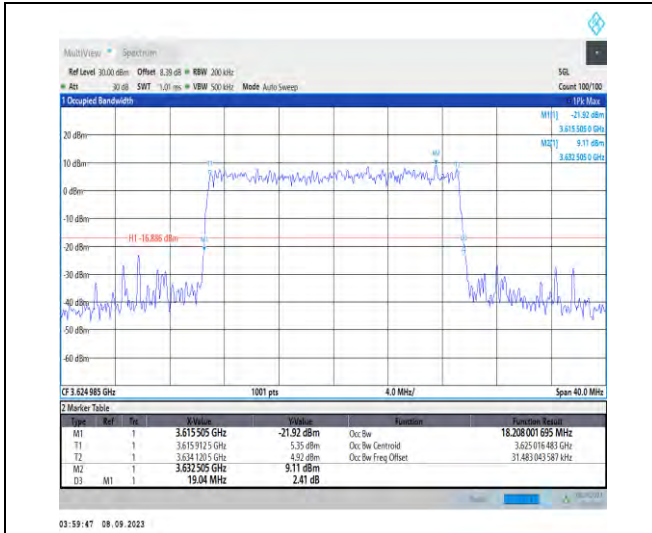
1-N48-PC3-30-20-M-7-CP-16QAM-Outer_Full-51@0 -Ant5-18.208-19.04-<20-PASS
