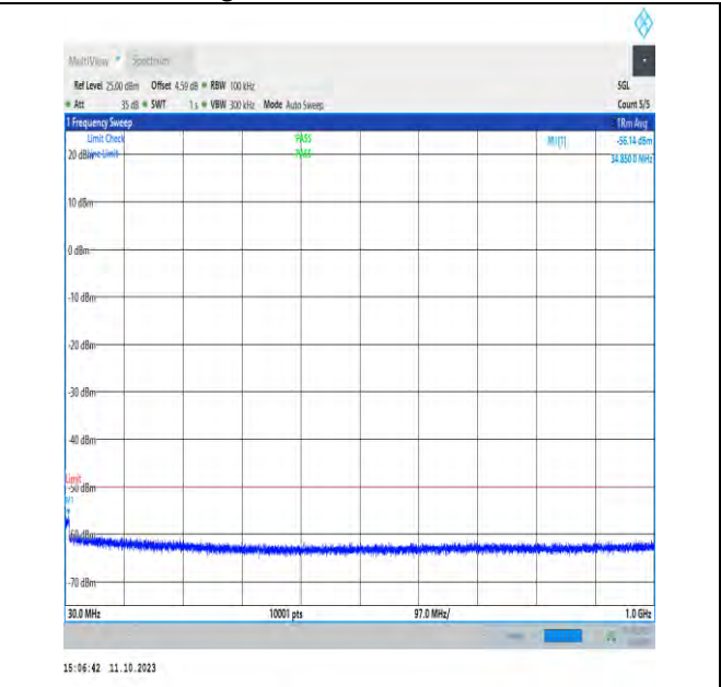
NTNV_N48_PC3_30_40_M_TID1_NS_01_30_1000_#1
