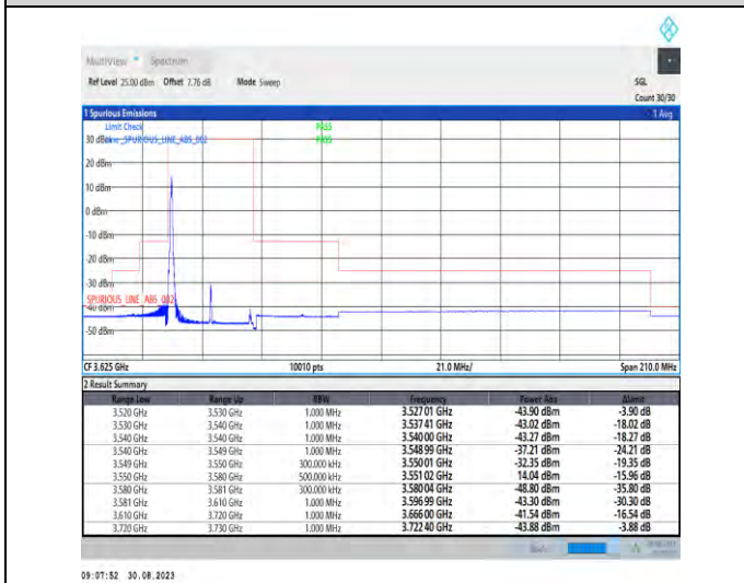
1-N48-PC3-30-30-L-4-CP-QPSK-Edge_1RB_Left-1@0-Ant5-1--PASS-see graph
