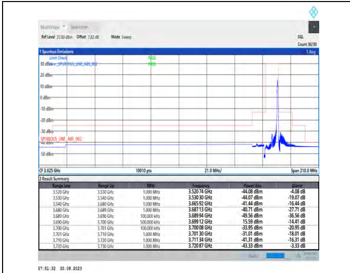
1-N48-PC3-30-10-H-2-DFT-PI2BPSK-Edge_1RB_Righ t-1@23-Ant5-1--PASS-see graph
