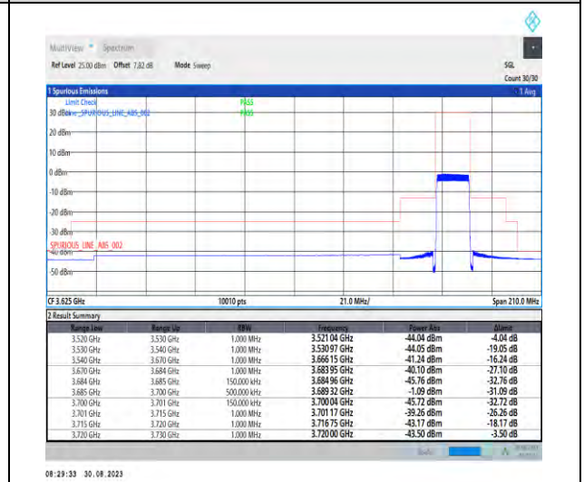
1-N48-PC3-30-15-H-6-CP-QPSK-Outer_Full-38@ 0-Ant5-1--PASS-see graph
