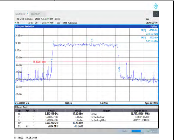
1-N48-PC3-30-30-M-3-DFT-16QAM-Outer_Full-75 @0-Ant5-26.797-28.140-≤30-PASS
