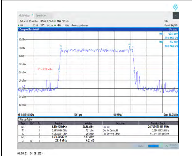
1-N48-PC3-30-30-M-4-DFT-64QAM-Outer_Full-75 @0-Ant5-26.789-28.140-≤30-PASS
