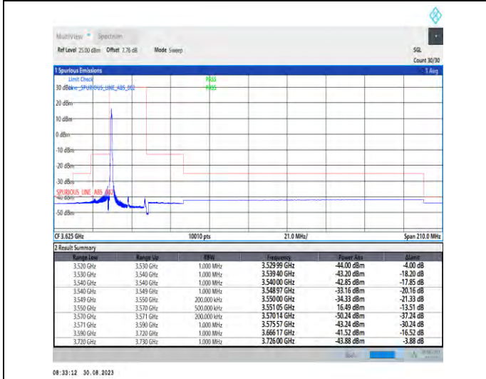
1-N48-PC3-30-20-L-1-DFT-PI2BPSK-Edge_1RB_Left-1@0-Ant5-1--PASS-see graph
