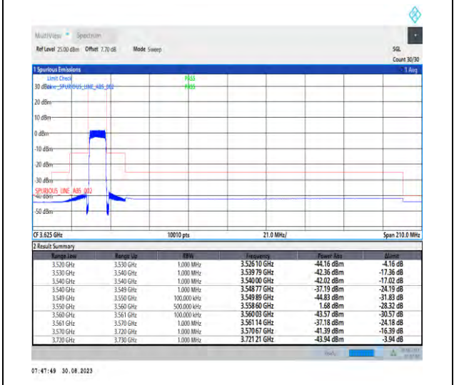
1-N48-PC3-30-10-L-6-CP-QPSK-Outer_Full-24@0-Ant5-1--PASS-see graph
