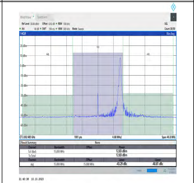
NTVN_N48_PC3_30_15_H_TID18_#1_-15_15
