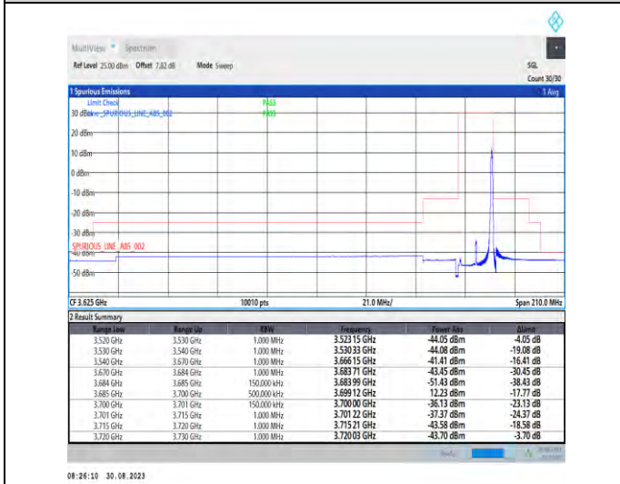
1-N48-PC3-30-15-H-5-CP-QPSK-Edge_1RB_Right-1 @37-Ant5-1--PASS-see graph
