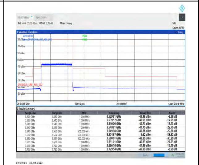
1-N48-PC3-30-40-L-6-CP-QPSK-Outer_Full-106@0-Ant5-1--PASS-see graph
