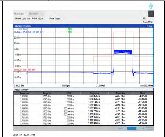
1-N48-PC3-30-30-H-3-DFT-PI2BPSK-Outer_Full-7 5@0-Ant5-1--PASS-see graph
