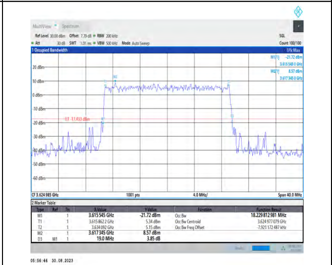
1-N48-PC3-30-20-M-6-CP-QPSK-Outer_Full-51@0- Ant5-18.23-19.000-≤20-PASS
