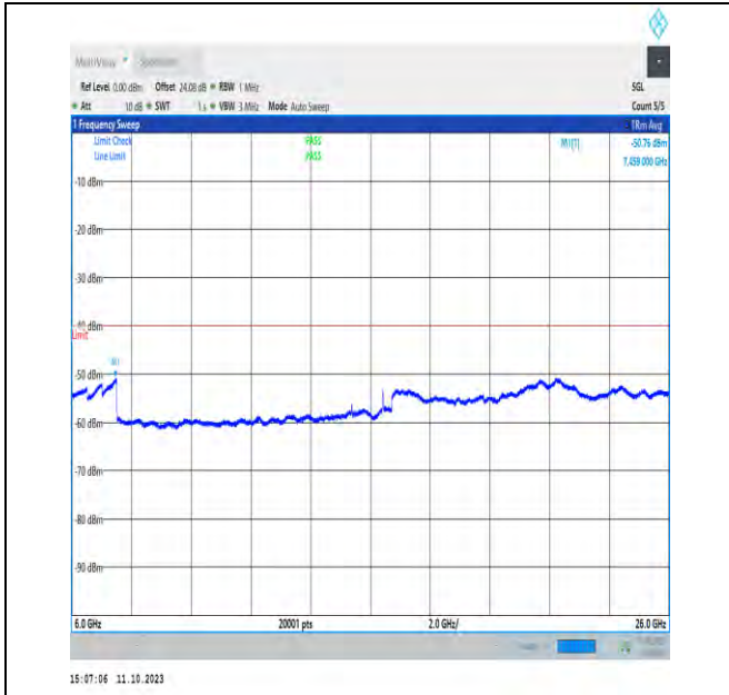
NTVN_N48_PC3_30_40_M_TID1_NS_01_6000_26000_#1
