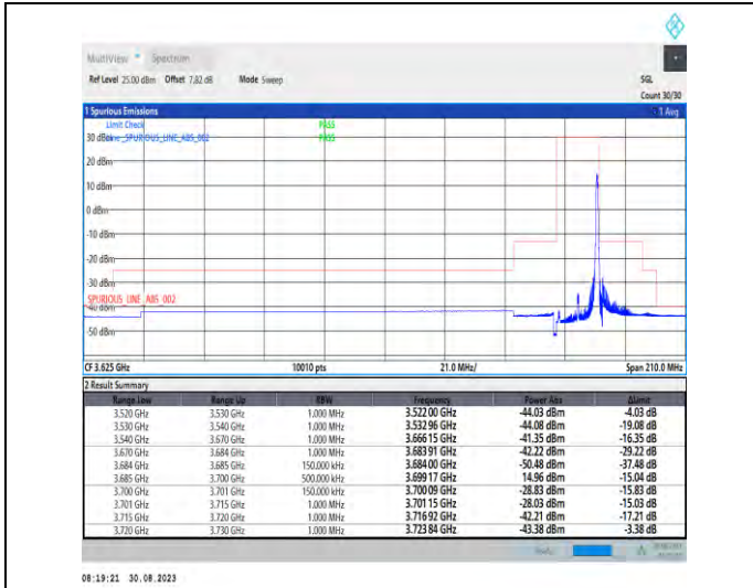
1-N48-PC3-30-15-H-2-DFT-PI2BPSK-Edge_1RB_Righ t-1@37-Ant5-1--PASS-see graph
