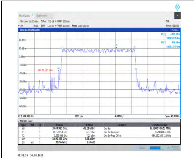
1-N48-PC3-30-20-M-3-DFT-16QAM-Outer_Full-50@ 0-Ant5-17.791-19.160-≤20-PASS
