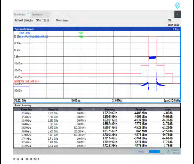
1-N48-PC3-30-10-H-6-CP-QPSK-Outer_Full-24@ 0-Ant5-1--PASS-see graph
