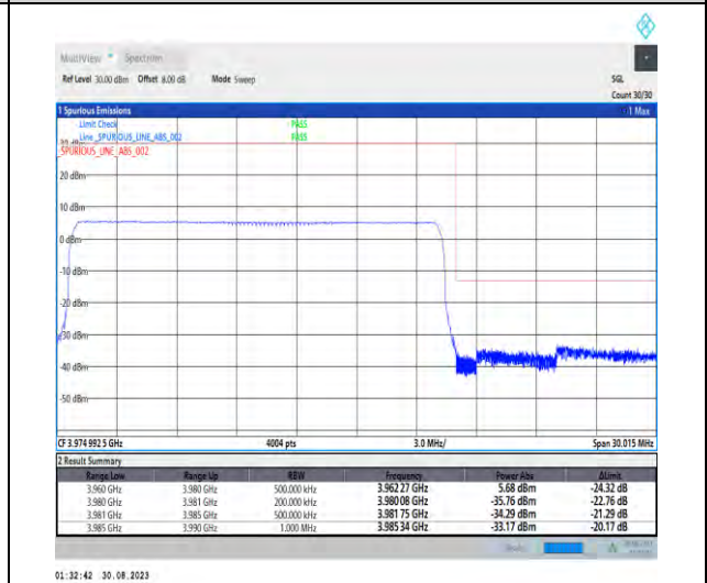
1-N77-3700-3980-PC2-30-20-H-6-CP-QPSK-Outer_Full-51@0-Ant5-1--PASS-see graph
