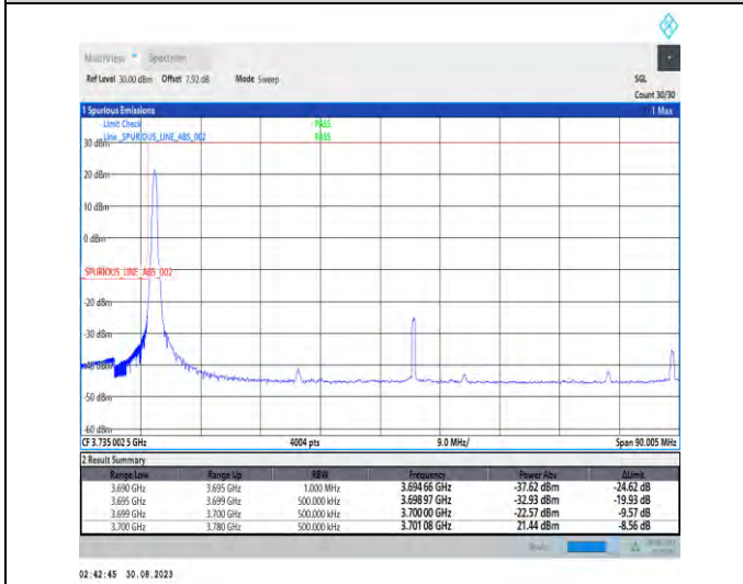
1-N77-3700-3980-PC2-30-80-L-4-CP-QPSK-Edge_1RB_Left-1@0-Ant5-1--PASS-see graph
