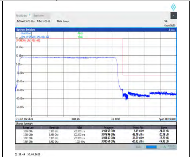
1-N77-3700-3980-PC2-30-20-H-3-DFT-PI2BPSK-Outer_Full-50@0-Ant5-1--PASS-see graph
