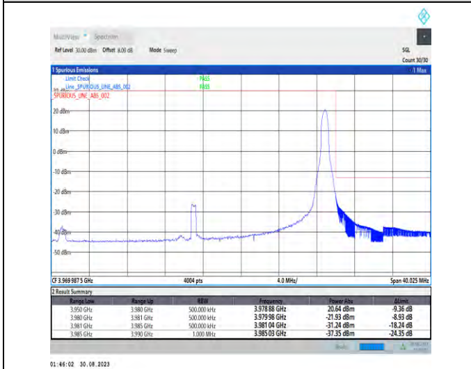
1-N77-3700-3980-PC2-30-30-H-5-CP-QPSK-Edge_1RB_Right-1@77-Ant5-1--PASS-see graph
