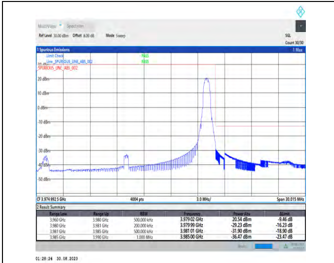
1-N77-3700-3980-PC2-30-20-H-2-DFT-PI2BPSK-Edge_1RB_Right-1@50-Ant5-1--PASS-see graph
