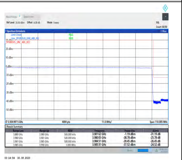
1-N77-3700-3980-PC2-30-100-H-6-CP-QPSK-Outer_Full-273@0-Ant5-1--PASS-see graph
