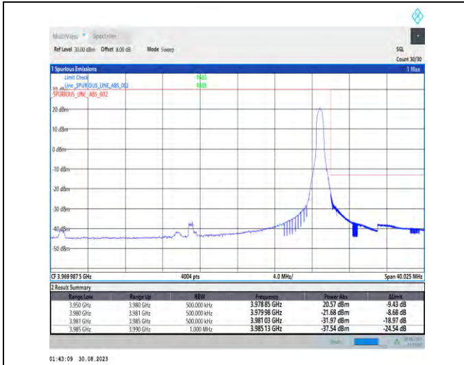
1-N77-3700-3980-PC2-30-30-H-2-DFT-PI2BPSK-Edge_1RB_Right-1@77-Ant5-1--PASS-see graph
