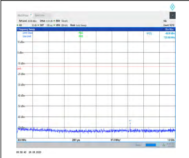
1-N77-3700-3980-PC2-30-100-H-1-DFT-PI2BPSK-I nner_1RB_Left-1@1-30-1000-Ant5-723.55--66.99--1 3-PASS
