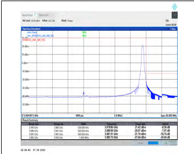
1-N77-3700-3980-PC2-30-40-H-2-DFT-PI2BPSK-Edge_1RB_Right-1@105-Ant5-1--PASS-see graph
