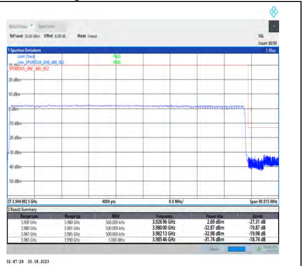
1-N77-3700-3980-PC2-30-80-H-3-DFT-PI2BPSK-Outer_Full-216@0-Ant5-1--PASS-see graph
