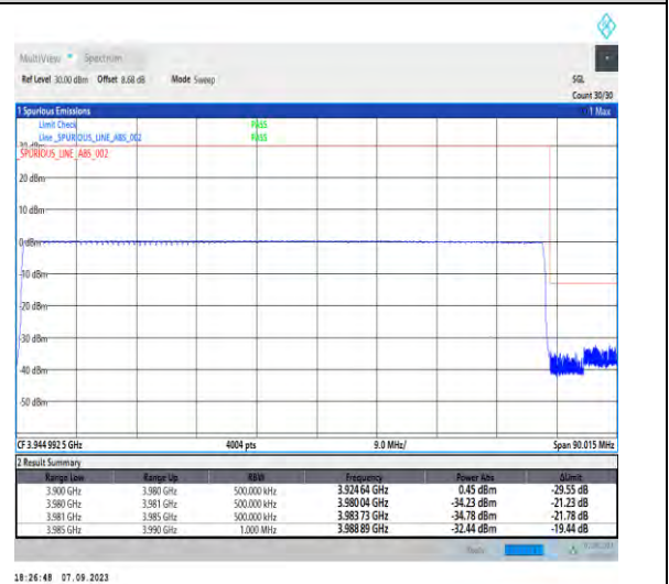
1-N77-3700-3980-PC2-30-80-H-6-CP-QPSK-Outer_Full-217@0-Ant5-1--PASS-see graph
