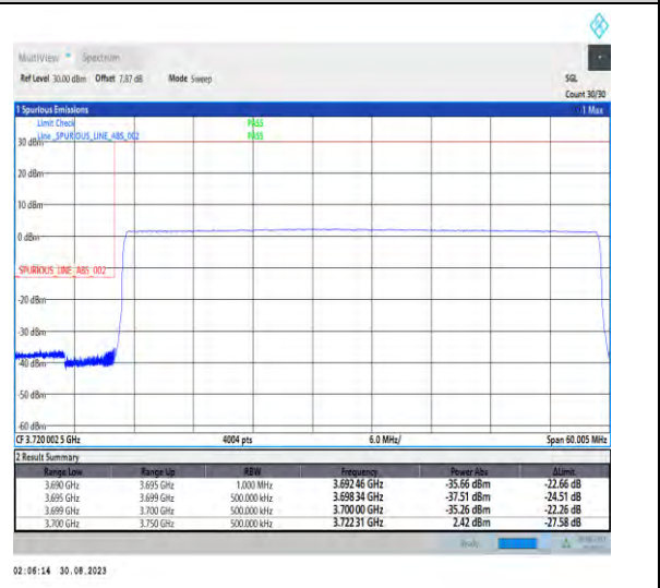
1-N77-3700-3980-PC2-30-50-L-6-CP-QPSK-Outer_Full-133@0-Ant5-1--PASS-see graph
