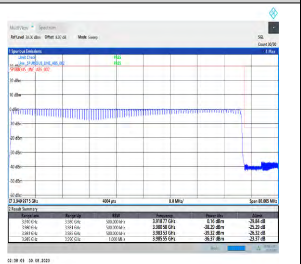
1-N77-3700-3980-PC2-30-70-H-6-CP-QPSK-Outer_Full-189@0-Ant5-1--PASS-see graph
