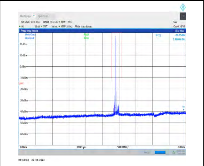
1-N77-3700-3980-PC2-30-100-H-1-DFT-PI2BPSK-In ner_1RB_Left-1@1-1000-6000-Ant5-5931.00--39.37-- 13-PASS
