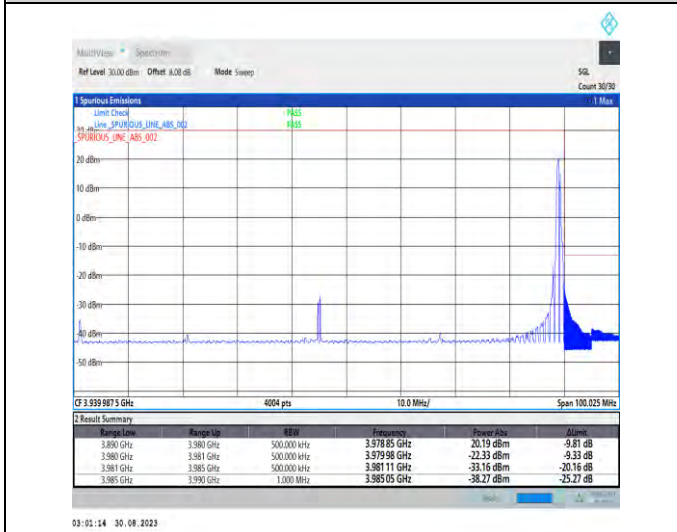
1-N77-3700-3980-PC2-30-90-H-5-CP-QPSK-Edge_1RB_Right-1@244-Ant5-1--PASS-see graph
