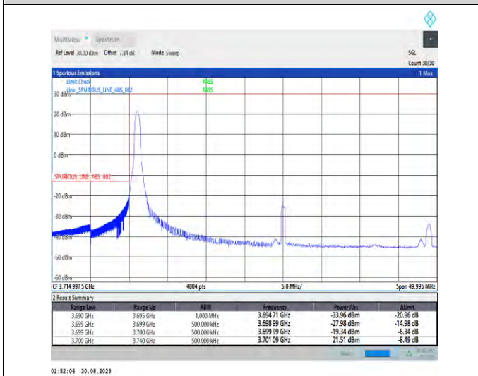
1-N77-3700-3980-PC2-30-40-L-4-CP-QPSK-Edge_1RB_Left-1@0-Ant5-1--PASS-see graph
