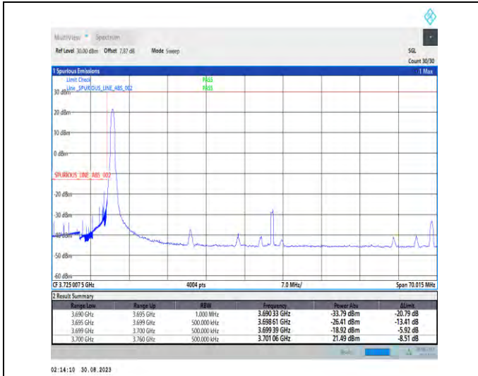
1-N77-3700-3980-PC2-30-60-L-1-DFT-PI2BPSK-Edge_1RB_Left-1@0-Ant5-1--PASS-see graph
