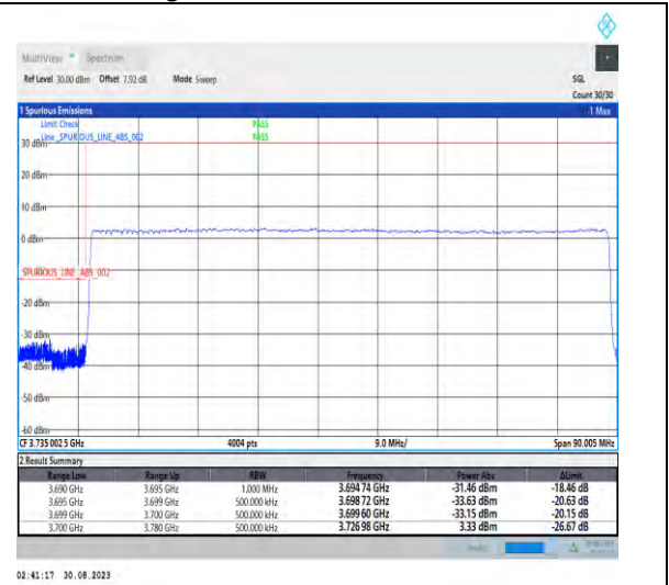
1-N77-3700-3980-PC2-30-80-L-3-DFT-PI2BPSK-Outer_Full-216@0-Ant5-1--PASS-see graph
