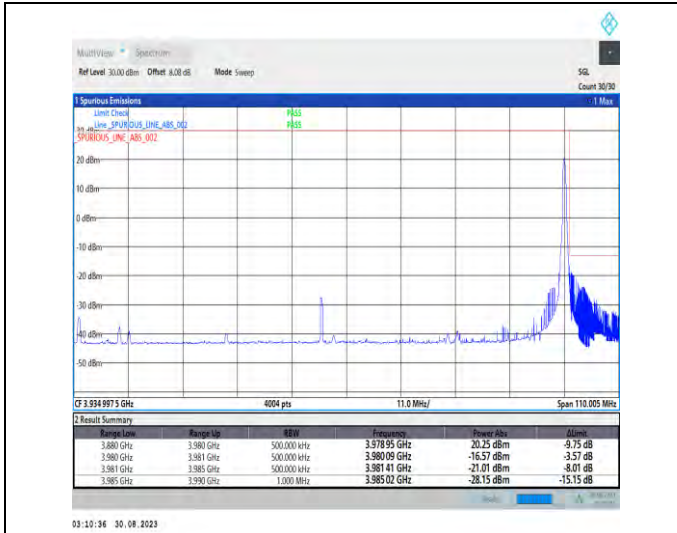
1-N77-3700-3980-PC2-30-100-H-2-DFT-PI2BPSK-Edge_1_RB_Right-1@272-Ant5-1--PASS-see graph
