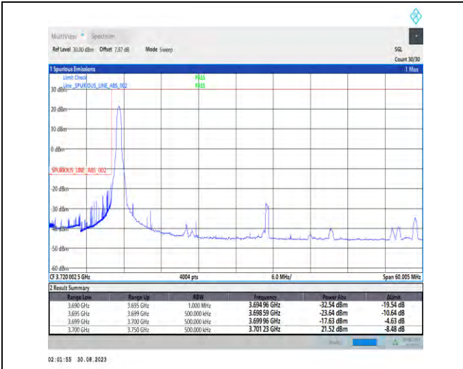
1-N77-3700-3980-PC2-30-50-L-1-DFT-PI2BPSK-Edge_1RB_Left-1@0-Ant5-1--PASS-see graph
