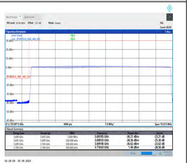
1-N77-3700-3980-PC2-30-60-L-6-CP-QPSK-Outer_Full-162@0-Ant5-1--PASS-see graph
