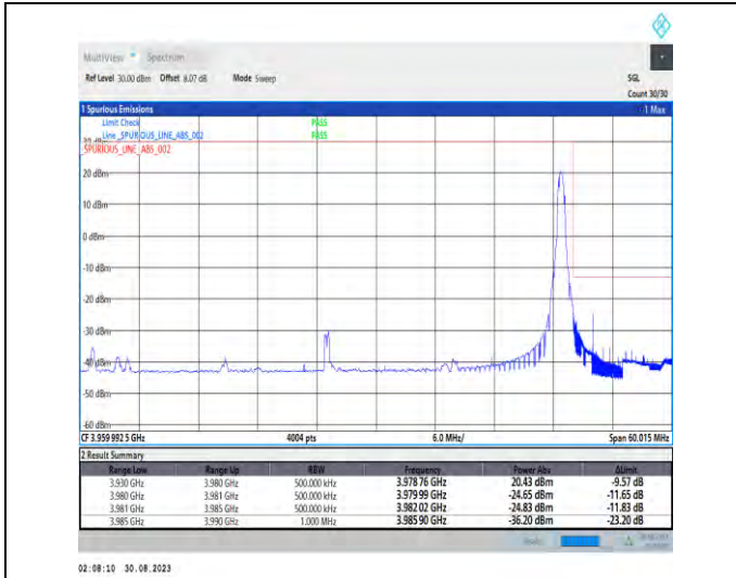
1-N77-3700-3980-PC2-30-50-H-2-DFT-PI2BPSK-Edge_1RB_Right-1@132-Ant5-1--PASS-see graph
