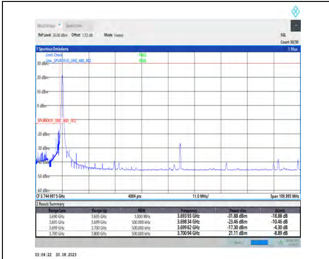
1-N77-3700-3980-PC2-30-100-L-1-DFT-PI2BPSK-Edge_e_1RB_Left-1@0-Ant5-1--PASS-see graph
