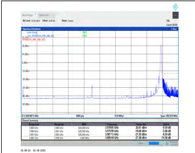
1-N77-3700-3980-PC2-30-90-H-2-DFT-PI2BPSK-Edge_1RB_Right-1@244-Ant5-1--PASS-see graph
