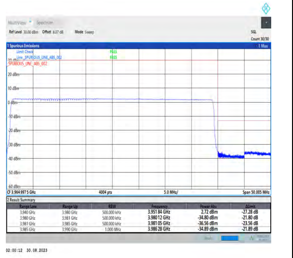
1-N77-3700-3980-PC2-30-40-H-6-CP-QPSK-Outer_Full-106@0-Ant5-1--PASS-see graph
