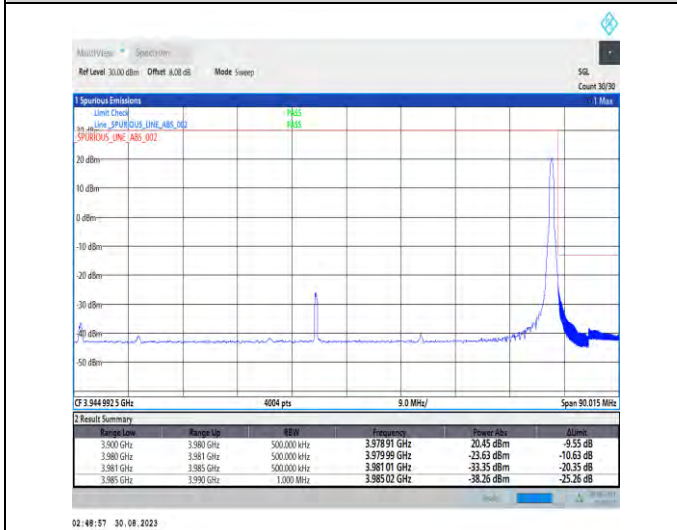
1-N77-3700-3980-PC2-30-80-H-5-CP-QPSK-Edge_1RB_Right-1@216-Ant5-1--PASS-see graph
