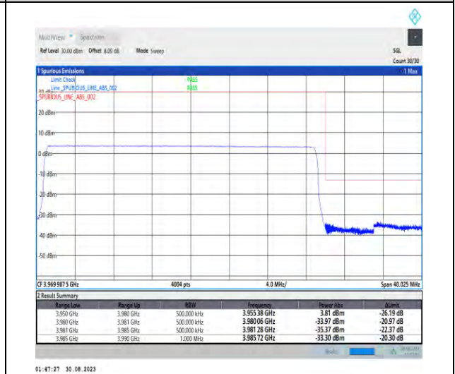
1-N77-3700-3980-PC2-30-30-H-6-CP-QPSK-Outer_Full-78@0-Ant5-1--PASS-see graph
