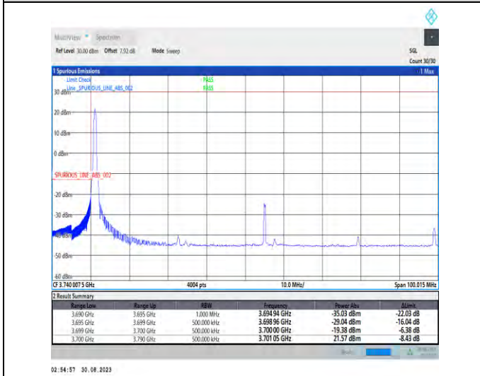
1-N77-3700-3980-PC2-30-90-L-4-CP-QPSK-Edge_1RB_Left-1@0-Ant5-1--PASS-see graph
