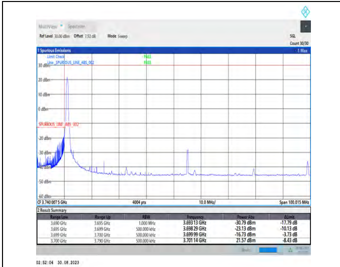
1-N77-3700-3980-PC2-30-90-L-1-DFT-PI2BPSK-Edge_1RB_Left-1@0-Ant5-1--PASS-see graph
