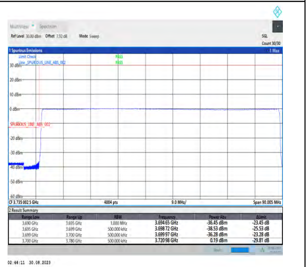
1-N77-3700-3980-PC2-30-80-L-6-CP-QPSK-Outer_Full-217@0-Ant5-1--PASS-see graph
