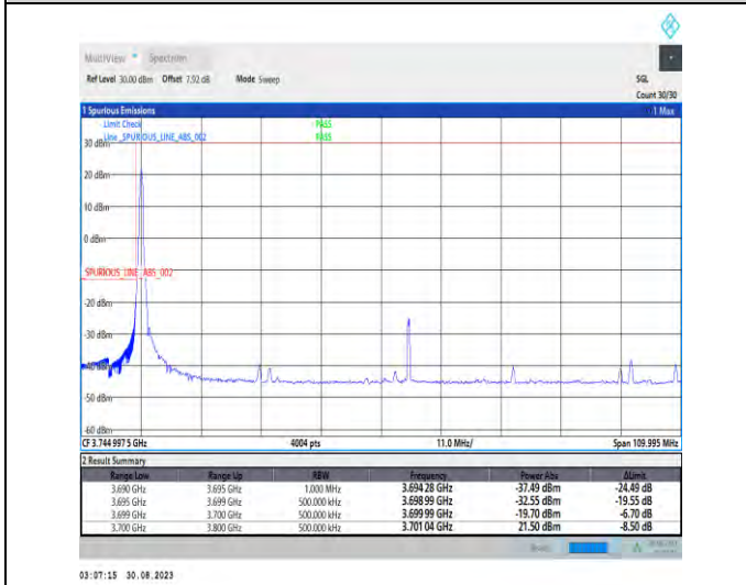
1-N77-3700-3980-PC2-30-100-L-4-CP-QPSK-Edge_1RB_Left-1@0-Ant5-1--PASS-see graph
