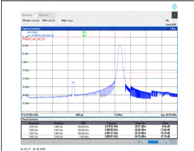
1-N77-3700-3980-PC2-30-20-H-5-CP-QPSK-Edge_1RB_Right-1@50-Ant5-1--PASS-see graph
