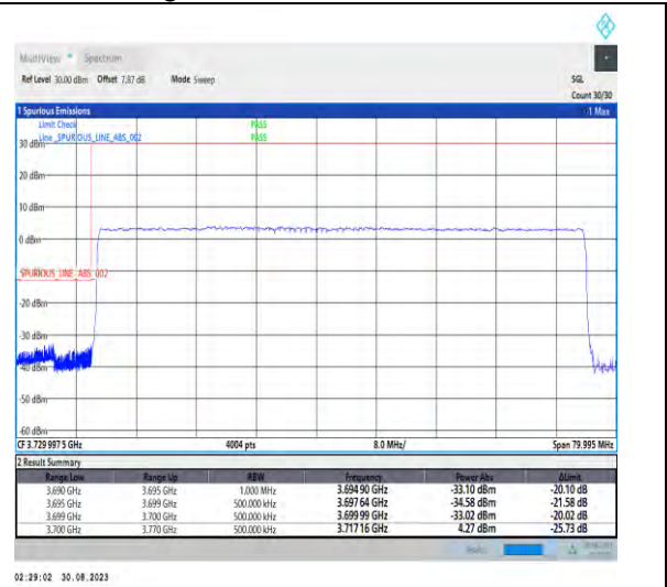
1-N77-3700-3980-PC2-30-70-L-3-DFT-PI2BPSK-Outer_Full-180@0-Ant5-1--PASS-see graph
