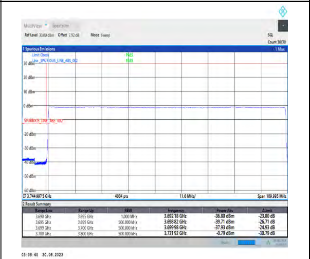
1-N77-3700-3980-PC2-30-100-L-6-CP-QPSK-Outer_Full-273@0-Ant5-1--PASS-see graph
