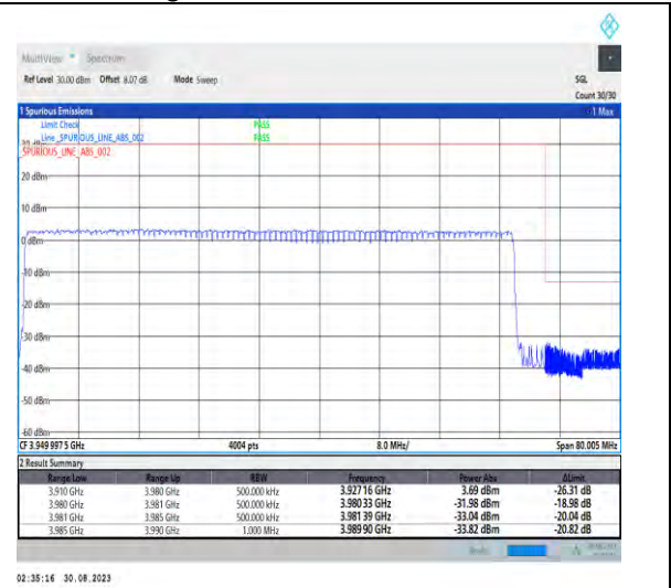
1-N77-3700-3980-PC2-30-70-H-3-DFT-PI2BPSK-Outer_Full-180@0-Ant5-1--PASS-see graph
