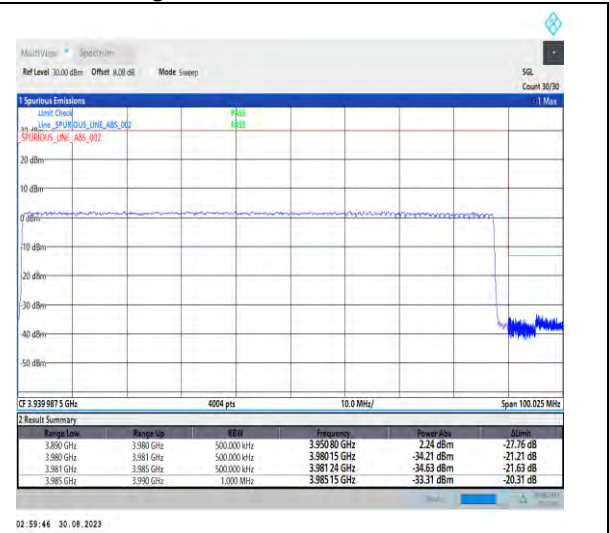
1-N77-3700-3980-PC2-30-90-H-3-DFT-PI2BPSK-Outer_Full-240@0-Ant5-1--PASS-see graph
