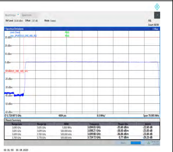
1-N77-3700-3980-PC2-30-70-L-6-CP-QPSK-Outer_Full-189@0-Ant5-1--PASS-see graph
