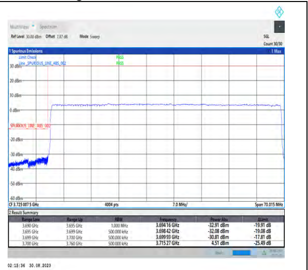
1-N77-3700-3980-PC2-30-60-L-3-DFT-PI2BPSK-Outer_Full-162@0-Ant5-1--PASS-see graph
