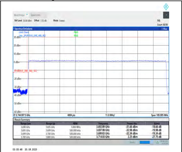
1-N77-3700-3980-PC2-30-100-L-3-DFT-PI2BPSK-Outer_Full-270@0-Ant5-1--PASS-see graph
