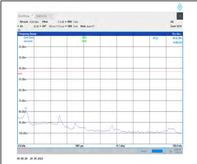
1-N77-3700-3980-PC2-30-100-H-1-DFT-PI2BPSK- Inner_1RB_Left-1@1-0.009-0.15-Ant5-0.02--80.42--4 3-PASS
