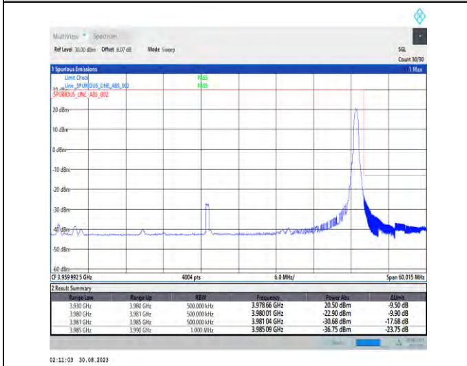
1-N77-3700-3980-PC2-30-50-H-5-CP-QPSK-Edge_1RB_Right-1@132-Ant5-1--PASS-see graph
