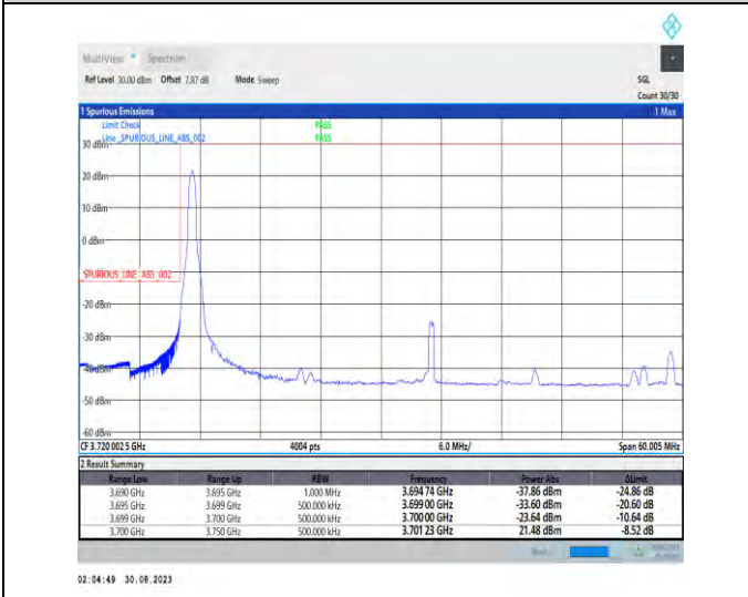
1-N77-3700-3980-PC2-30-50-L-4-CP-QPSK-Edge_1RB_Left-1@0-Ant5-1--PASS-see graph
