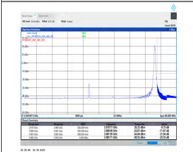
1-N77-3700-3980-PC2-30-70-H-5-CP-QPSK-Edge_1RB_Right-1@188-Ant5-1--PASS-see graph
