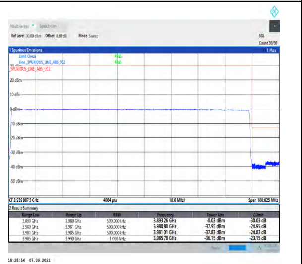
1-N77-3700-3980-PC2-30-90-H-6-CP-QPSK-Outer_Full-245@0-Ant5-1--PASS-see graph
