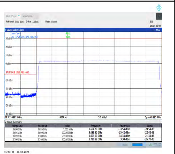
1-N77-3700-3980-PC2-30-40-L-6-CP-QPSK-Outer_Full-106@0-Ant5-1--PASS-see graph
