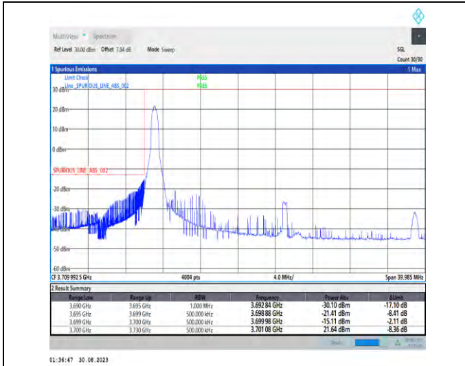
1-N77-3700-3980-PC2-30-30-L-1-DFT-PI2BPSK-Edge_1RB_Left-1@0-Ant5-1--PASS-see graph
