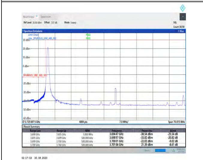
1-N77-3700-3980-PC2-30-60-L-4-CP-QPSK-Edge_1RB_Left-1@0-Ant5-1--PASS-see graph
