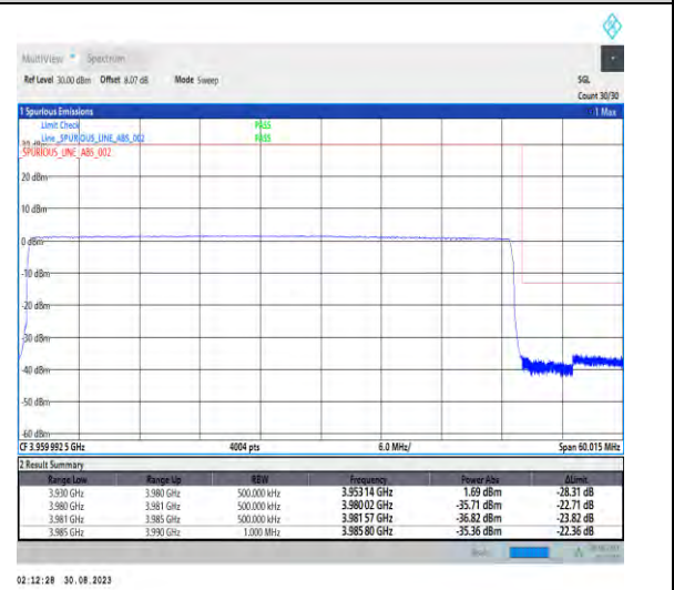
1-N77-3700-3980-PC2-30-50-H-6-CP-QPSK-Outer_Full-133@0-Ant5-1--PASS-see graph
