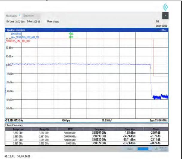
1-N77-3700-3980-PC2-30-100-H-3-DFT-PI2BPSK-Outer_Full-270@0-Ant5-1--PASS-see graph
