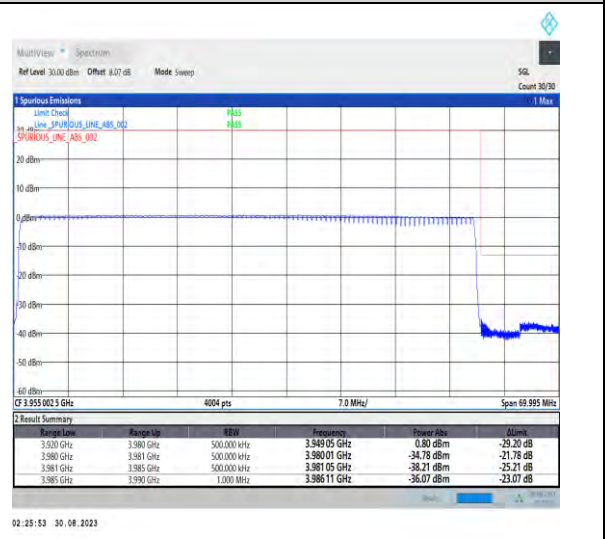
1-N77-3700-3980-PC2-30-60-H-6-CP-QPSK-Outer_Full-162@0-Ant5-1--PASS-see graph
