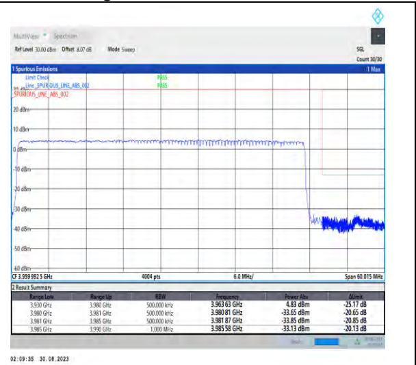
1-N77-3700-3980-PC2-30-50-H-3-DFT-PI2BPSK-Outer_Full-128@0-Ant5-1--PASS-see graph
