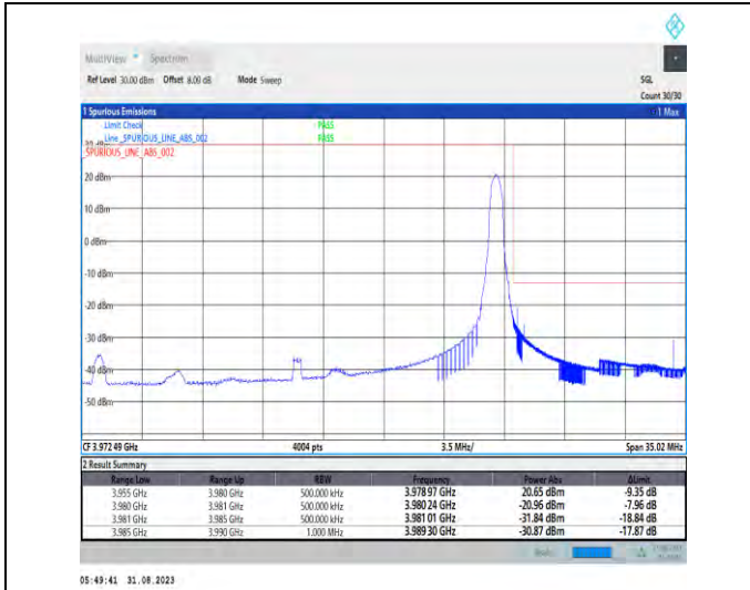
1-N77-3700-3980-PC2-30-25-H-2-DFT-PI2BPSK-Edge_1RB_Right-1@64-Ant5-1--PASS-see graph
