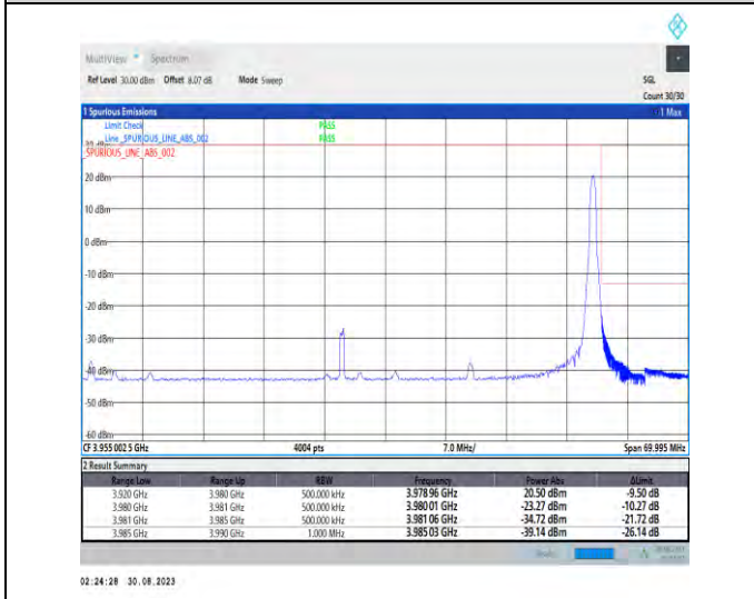
1-N77-3700-3980-PC2-30-60-H-5-CP-QPSK-Edge_1RB_Right-1@161-Ant5-1--PASS-see graph
