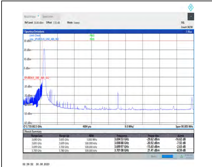
1-N77-3700-3980-PC2-30-80-L-1-DFT-PI2BPSK-Edge_1RB_Left-1@0-Ant5-1--PASS-see graph
