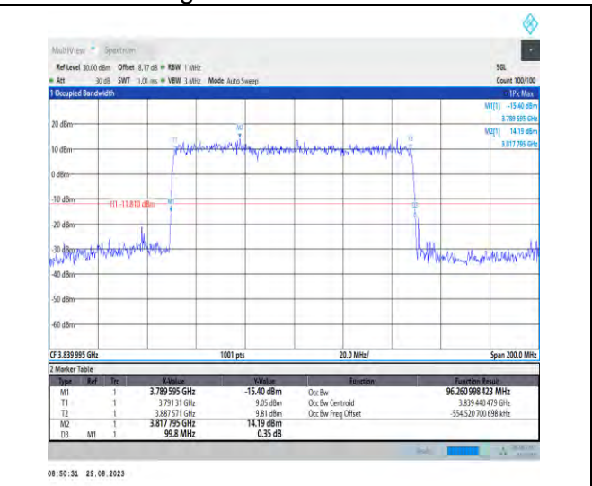
1-N77-3700-3980-PC2-30-100-M-3-DFT-16QAM-Out_Full-270@0-Ant5-96.261-99.800-≤100-PASS
