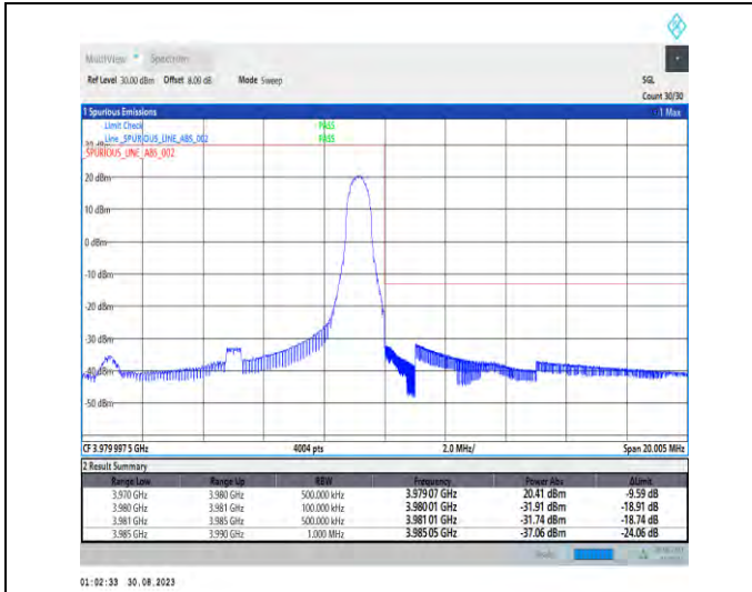
1-N77-3700-3980-PC2-30-10-H-2-DFT-PI2BPSK-Edge_1RB_Right-1@23-Ant5-1--PASS-see graph
