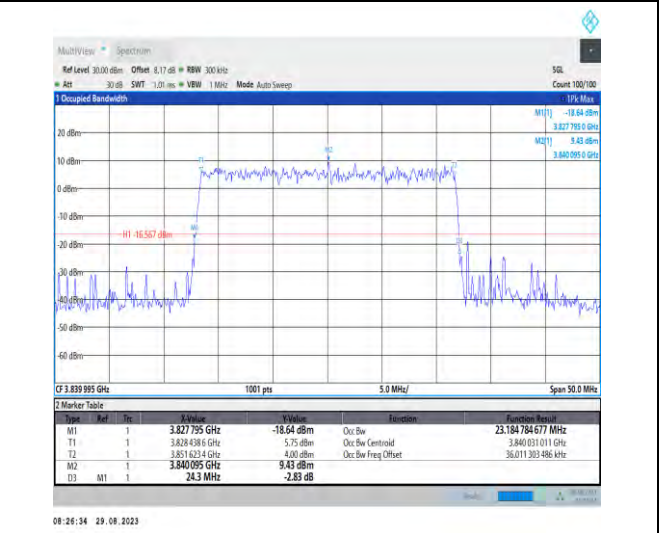
1-N77-3700-3980-PC2-30-25-M-9-CP-256QAM-Outer_Full-65@0-Ant5-23.185-24.300-≤25-PASS
