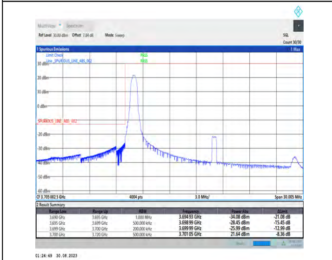
1-N77-3700-3980-PC2-30-20-L-4-CP-QPSK-Edge_1RB_Left-1@0-Ant5-1--PASS-see graph
