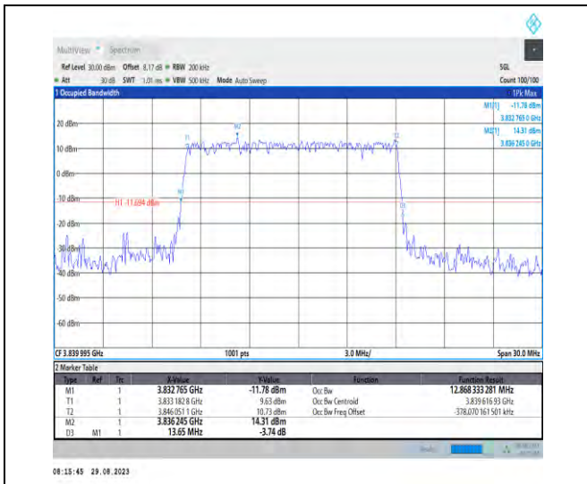
1-N77-3700-3980-PC2-30-15-M-4-DFT-64QAM-Out er_Full-36@0-Ant5-12.868-13.650-≤15-PASS
