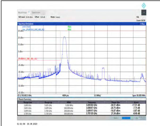
1-N77-3700-3980-PC2-30-20-L-1-DFT-PI2BPSK-Edge_1RB_Left-1@0-Ant5-1--PASS-see graph
