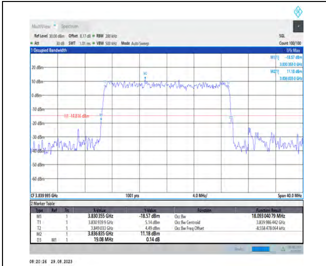
1-N77-3700-3980-PC2-30-20-M-7-CP-16QAM-Outer_Full-51@0-Ant5-18.093-19.080-≤20-PASS
