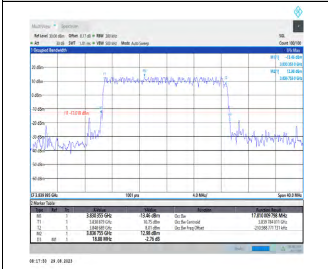
1-N77-3700-3980-PC2-30-20-M-1-DFT-QPSK-Outer_Full-50@0-Ant5-17.81-18.880-≤20-PASS
