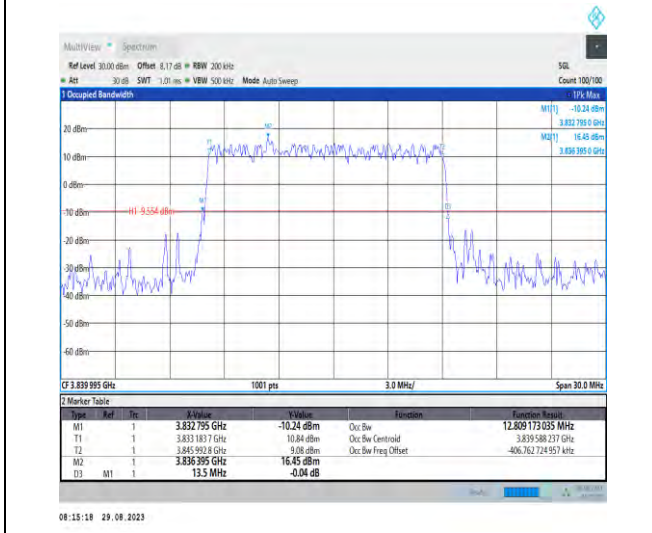
1-N77-3700-3980-PC2-30-15-M-2-DFT-PI2BPSK-Outer_Full-36@0-Ant5-12.809-13.500-≤15-PASS
