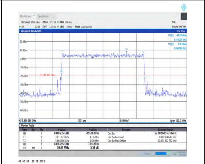
1-N77-3700-3980-PC2-30-60-M-9-CP-256QAM-Outer_Full-162@0-Ant5-57.883-59.640-≤60-PASS
