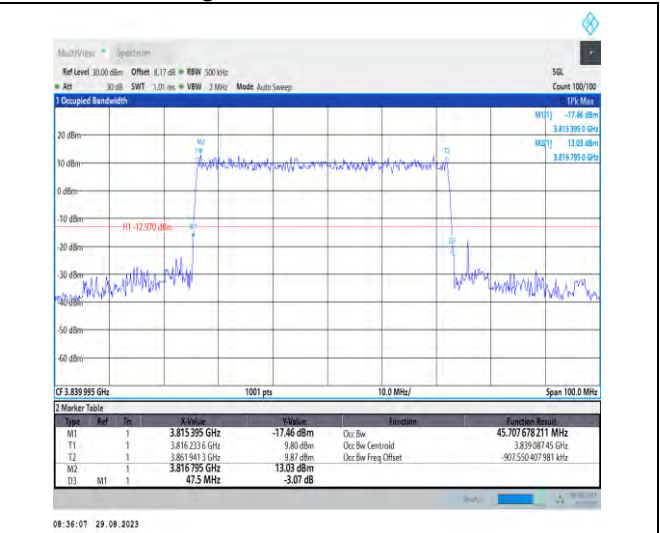
1-N77-3700-3980-PC2-30-50-M-4-DFT-64QAM-Outer_Full-128@0-Ant5-45.708-47.500-≤50-PASS
