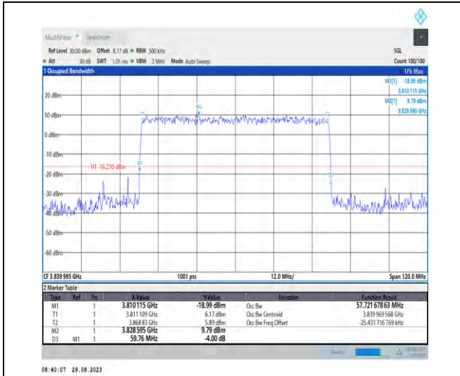
1-N77-3700-3980-PC2-30-60-M-6-CP-QPSK-Outer_Full-162@0-Ant5-57.722-59.760-≤60-PASS
