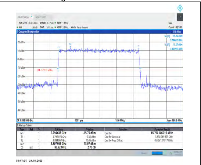
1-N77-3700-3980-PC2-30-90-M-4-DFT-64QAM-Outer_Full-240@0-Ant5-85.794-88.920-≤90-PASS
