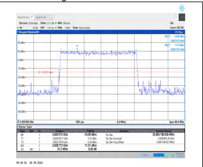
1-N77-3700-3980-PC2-30-40-M-5-DFT-256QAM-Out er_Full-100@0-Ant5-35.805-37.200-≤40-PASS
