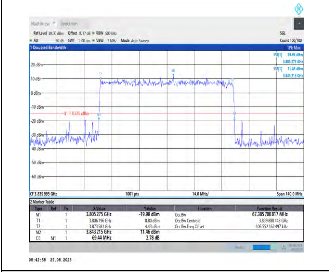
1-N77-3700-3980-PC2-30-70-M-7-CP-16QAM-Outer_Full-189@0-Ant5-67.386-69.440-≤70-PASS
