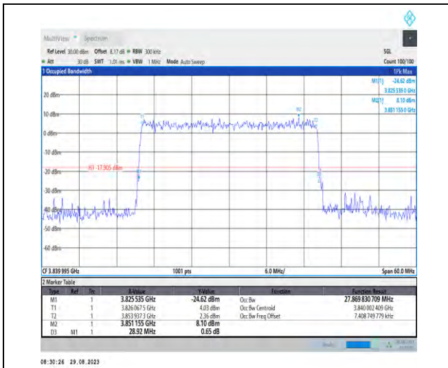
1-N77-3700-3980-PC2-30-30-M-9-CP-256QAM-Out er_Full-78@0-Ant5-27.87-28.920-<30-PASS
