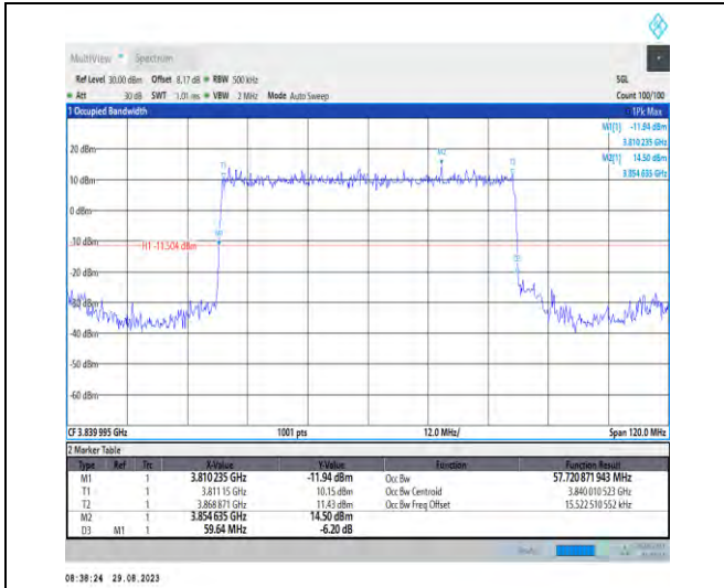
1-N77-3700-3980-PC2-30-60-M-2-DFT-PI2BPSK-Outer_Full-162@0-Ant5-57.721-59.640-≤60-PASS
