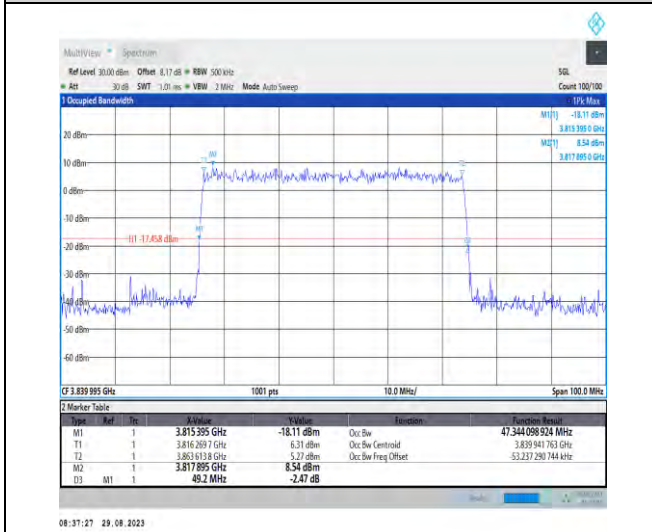
1-N77-3700-3980-PC2-30-50-M-9-CP-256QAM-Outer_Full-133@0-Ant5-47.344-49.200-≤50-PASS
