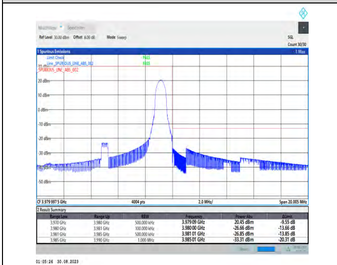
1-N77-3700-3980-PC2-30-10-H-5-CP-QPSK-Edge_1RB_Right-1@23-Ant5-1--PASS-see graph
