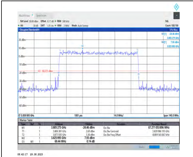
1-N77-3700-3980-PC2-30-70-M-9-CP-256QAM-Out er_Full-189@0-Ant5-67.211-69.440-≤70-PASS
