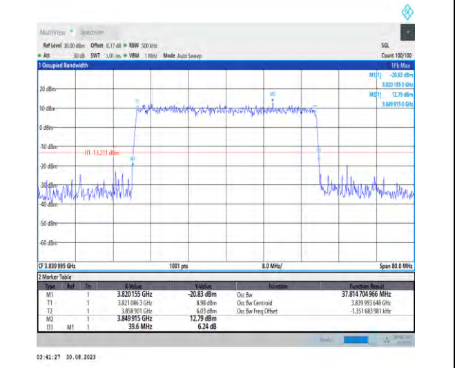
1-N77-3700-3980-PC2-30-40-M-7-CP-16QAM-Outer_Full-106@0-Ant5-37.815-39.600-≤40-PASS
