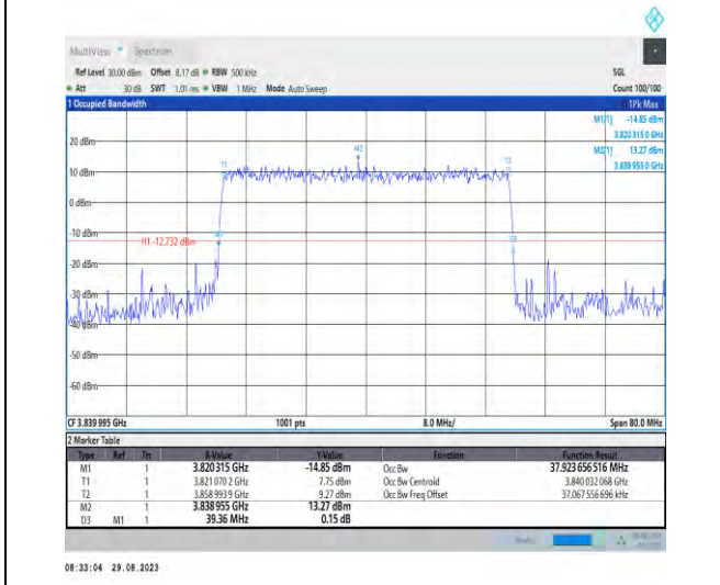
1-N77-3700-3980-PC2-30-40-M-6-CP-QPSK-Outer_Full-106@0-Ant5-37.924-39.360-≤40-PASS
