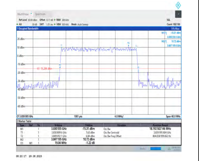
1-N77-3700-3980-PC2-30-20-M-6-CP-QPSK-Outer_Full-51@0-Ant5-18.193-19.040-≤20-PASS
