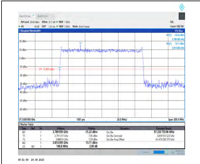
1-N77-3700-3980-PC2-30-100-M-6-CP-QPSK-Outer_Full-273@0-Ant5-97.234-100.800-≤100-PASS
