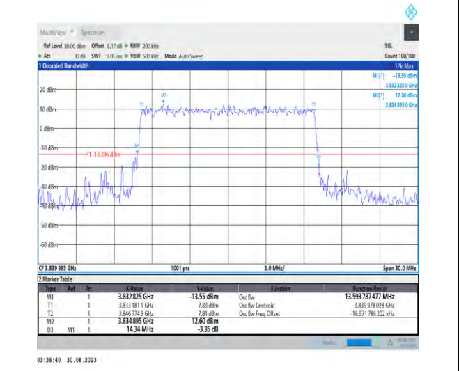
1-N77-3700-3980-PC2-30-15-M-7-CP-16QAM-Outer_Full-38@0-Ant5-13.594-14.340-≤15-PASS
