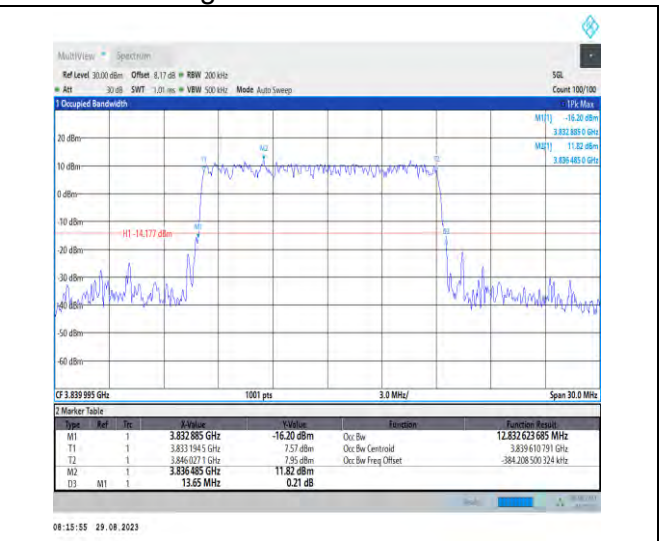
1-N77-3700-3980-PC2-30-15-M-5-DFT-256QAM-Out er_Full-36@0-Ant5-12.833-13.650-≤15-PASS
