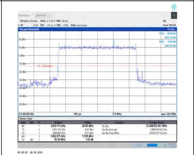
1-N77-3700-3980-PC2-30-60-M-1-DFT-QPSK-Outer_Full-162@0-Ant5-57.649-59.760-≤60-PASS
