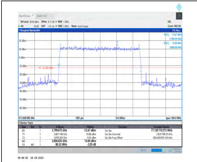
1-N77-3700-3980-PC2-30-80-M-4-DFT-64QAM-Out er_Full-216@0-Ant5-77.121-80.320-≤80-PASS
