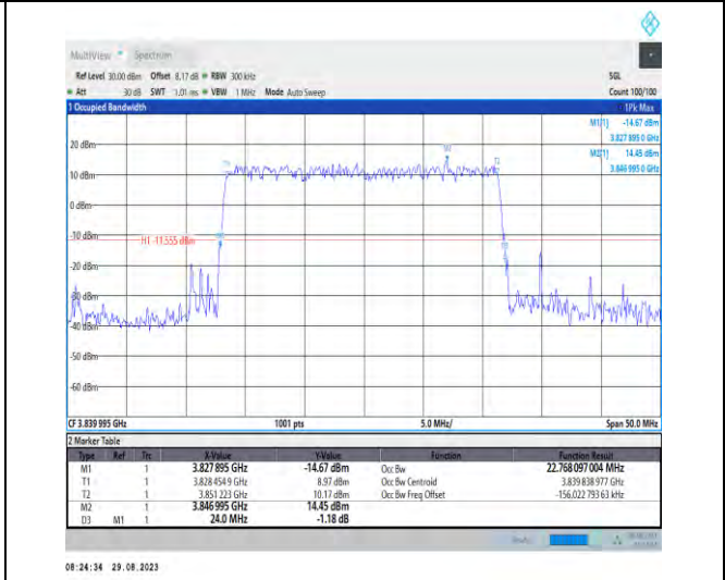
1-N77-3700-3980-PC2-30-25-M-1-DFT-QPSK-Outer_Full-64@0-Ant5-22.768-24.000-≤25-PASS
