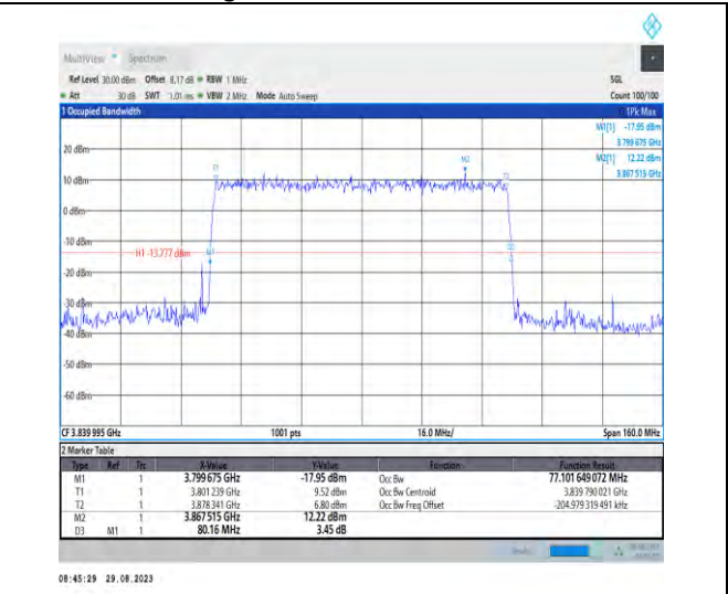
1-N77-3700-3980-PC2-30-80-M-5-DFT-256QAM-Out er_Full-216@0-Ant5-77.102-80.160-≤80-PASS
