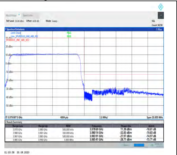
1-N77-3700-3980-PC2-30-10-H-3-DFT-PI2BPSK-Outer_Full-24@0-Ant5-1--PASS-see graph
