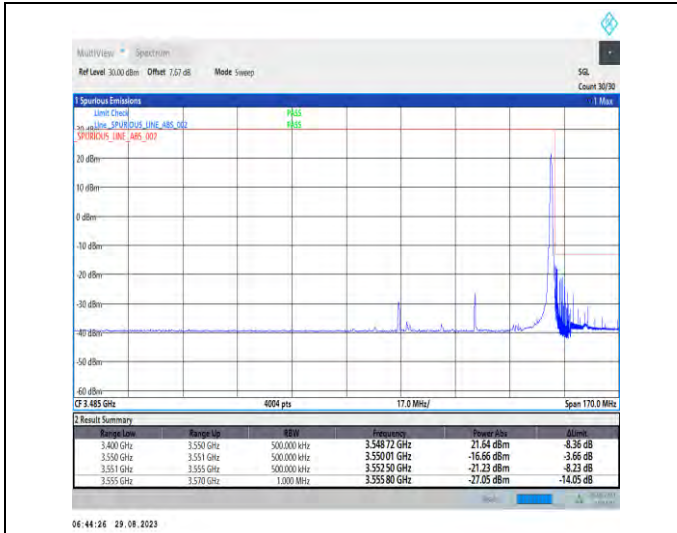
1-N77-3450-3550-PC2-30-50-H-2-DFT-PI2BPSK-Edge_1RB_Right-1@132-Ant5-1--PASS-see graph
