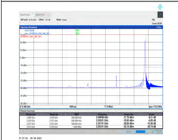
1-N77-3450-3550-PC2-30-70-H-5-CP-QPSK-Edge_1RB_Right-1@188-Ant5-1--PASS-see graph
