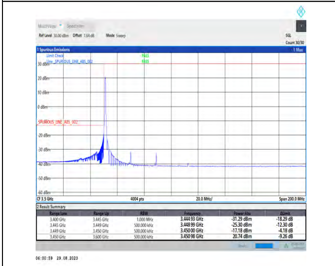
1-N77-3450-3550-PC2-30-40-L-4-CP-QPSK-Edge_1RB_Left-1@0-Ant5-1--PASS-see graph
