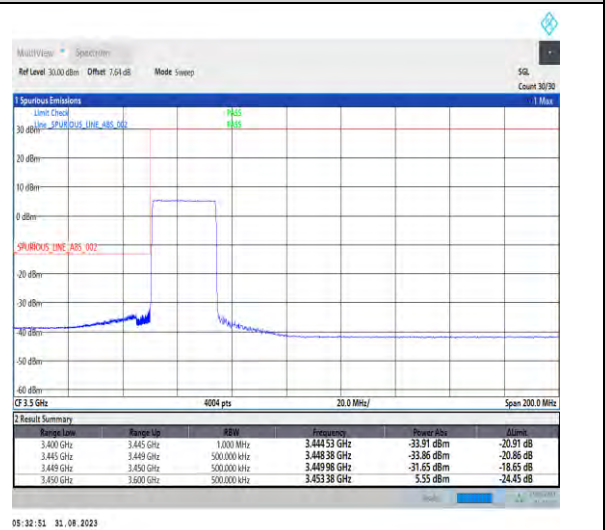
1-N77-3450-3550-PC2-30-25-L-6-CP-QPSK-Outer_Full-65@0-Ant5-1--PASS-see graph
