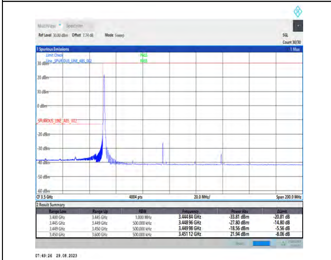
1-N77-3450-3550-PC2-30-90-L-4-CP-QPSK-Edge_1RB_Left-1@0-Ant5-1--PASS-see graph
