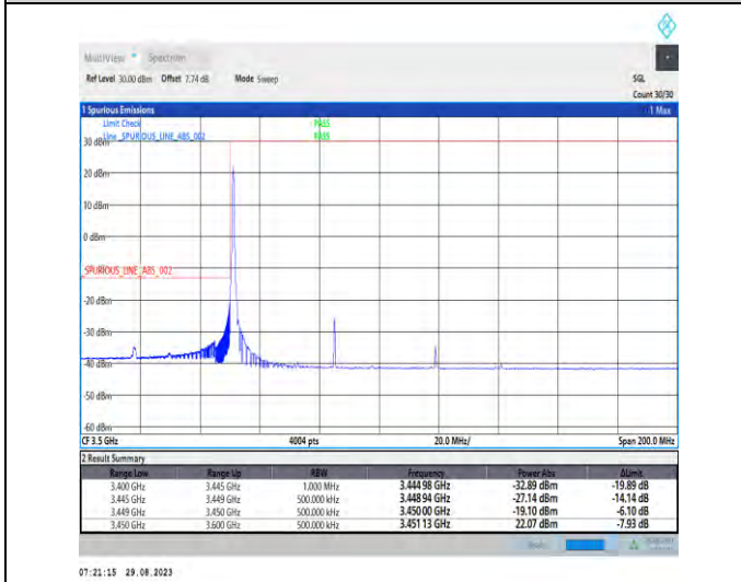
1-N77-3450-3550-PC2-30-70-L-4-CP-QPSK-Edge_1RB_Left-1@0-Ant5-1--PASS-see graph
