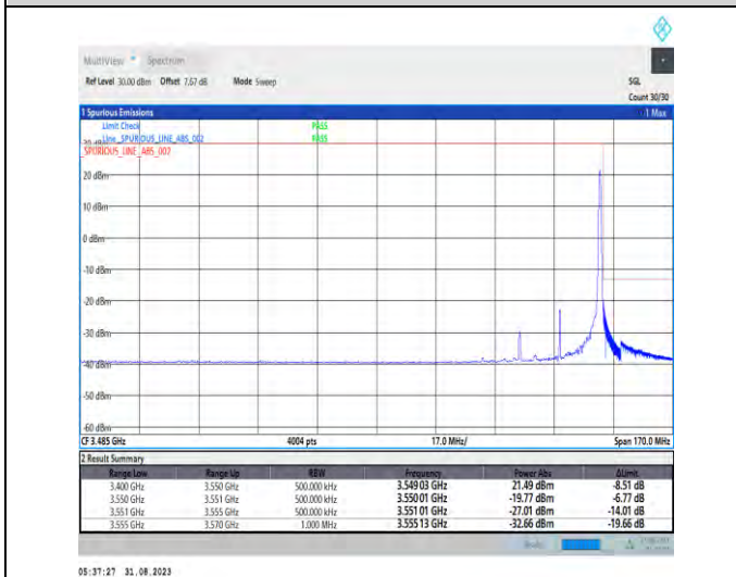
1-N77-3450-3550-PC2-30-25-H-5-CP-QPSK-Edge_1RB_Right-1@64-Ant5-1--PASS-see graph
