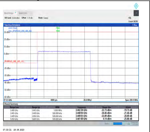
1-N77-3450-3550-PC2-30-80-L-3-DFT-PI2BPSK-Outer_Full-216@0-Ant5-1--PASS-see graph
