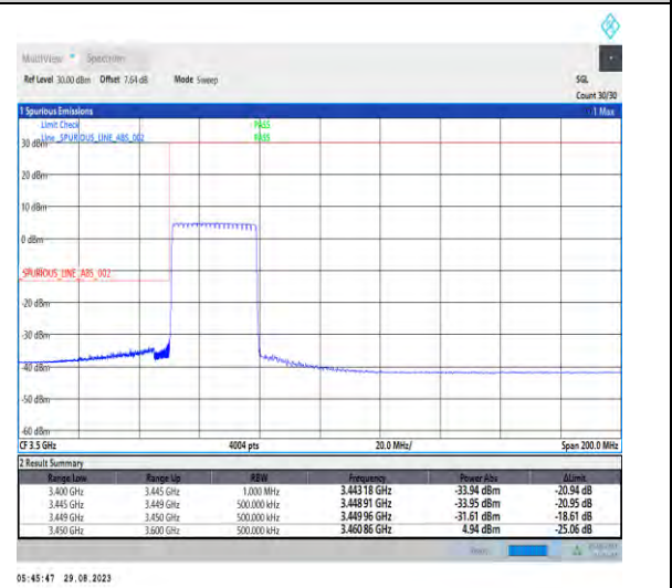
1-N77-3450-3550-PC2-30-30-L-6-CP-QPSK-Outer_Full-78@0-Ant5-1--PASS-see graph
