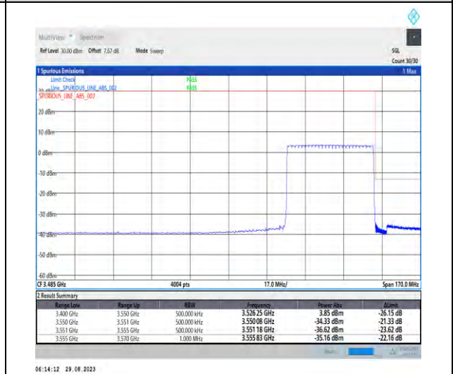
1-N77-3450-3550-PC2-30-40-H-6-CP-QPSK-Outer_Full-106@0-Ant5-1--PASS-see graph
