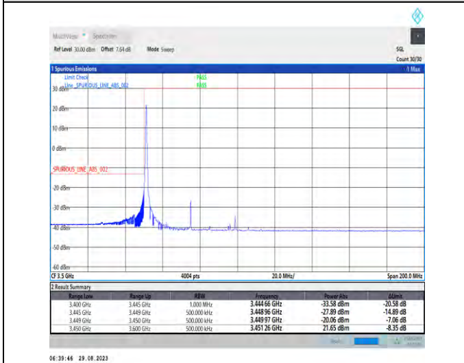
1-N77-3450-3550-PC2-30-50-L-4-CP-QPSK-Edge_1RB_Left-1@0-Ant5-1--PASS-see graph
