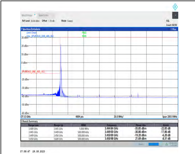
1-N77-3450-3550-PC2-30-100-L-1-DFT-PI2BPSK-Edge_1_RB_Left-1@0-Ant5-1--PASS-see graph
