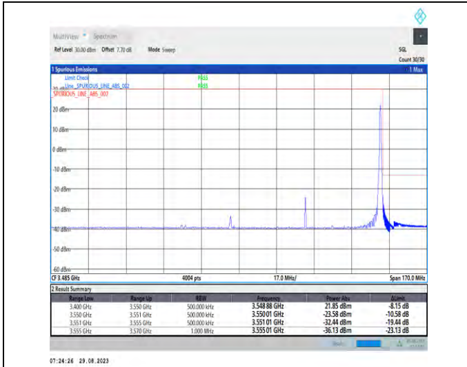
1-N77-3450-3550-PC2-30-70-H-2-DFT-PI2BPSK-Edge_1RB_Right-1@188-Ant5-1--PASS-see graph
