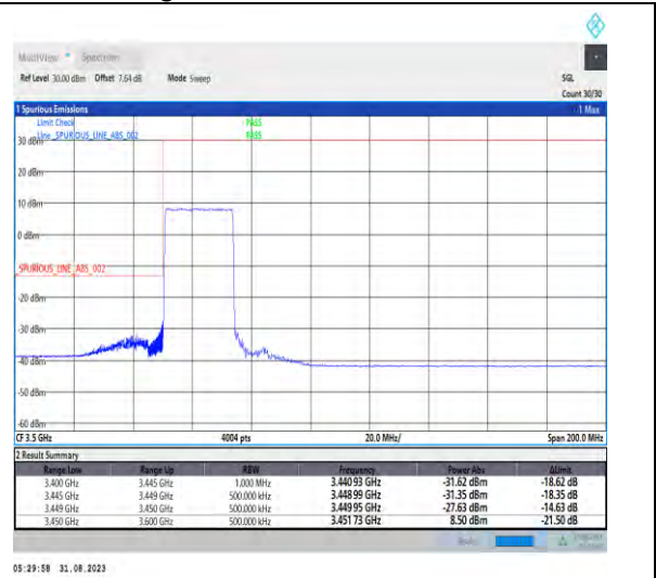
1-N77-3450-3550-PC2-30-25-L-3-DFT-PI2BPSK-Outer_Full-64@0-Ant5-1--PASS-see graph
