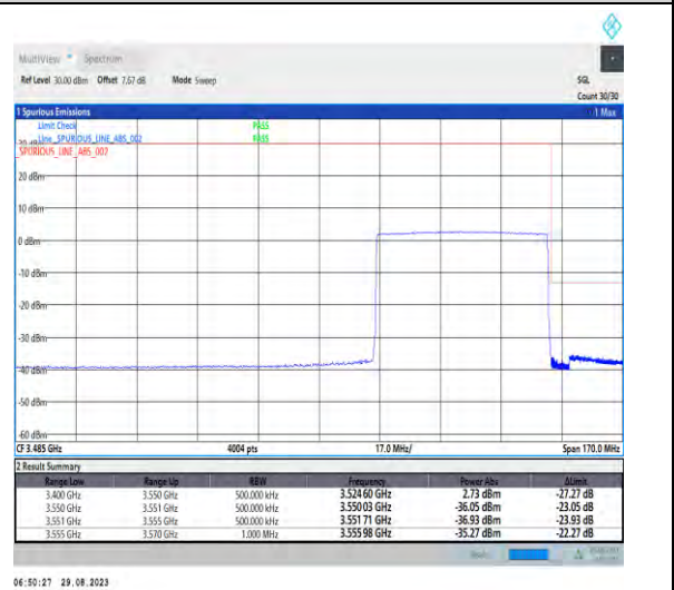
1-N77-3450-3550-PC2-30-50-H-6-CP-QPSK-Outer_Full-133@0-Ant5-1--PASS-see graph
