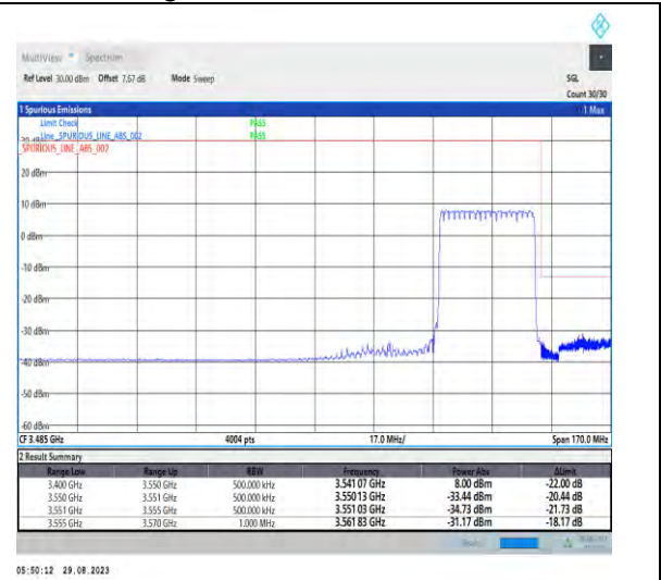
1-N77-3450-3550-PC2-30-30-H-3-DFT-PI2BPSK-Outer_Full-75@0-Ant5-1--PASS-see graph
