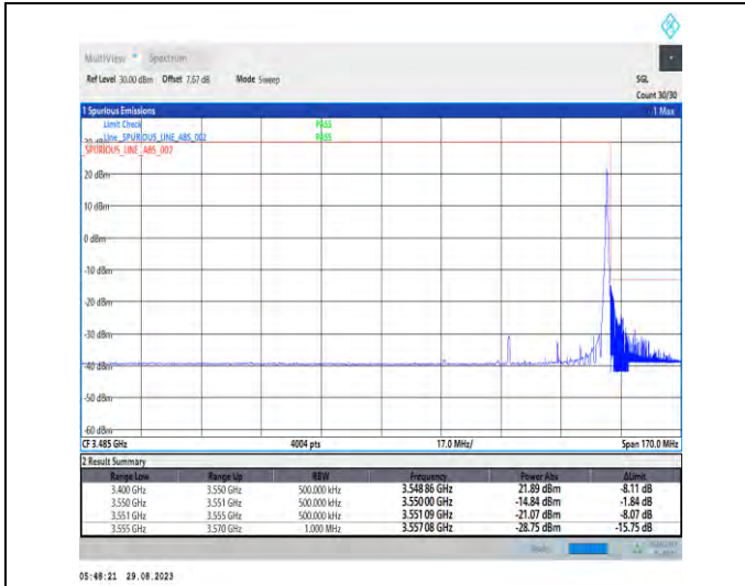
1-N77-3450-3550-PC2-30-30-H-2-DFT-PI2BPSK-Edge_1RB_Right-1@77-Ant5-1--PASS-see graph
