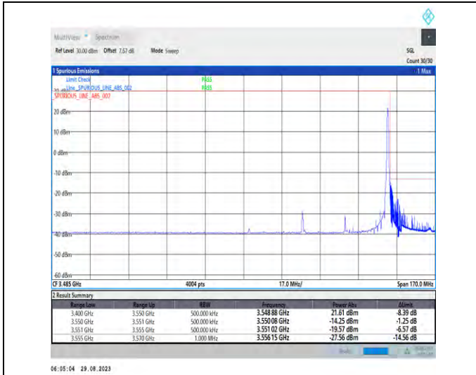
1-N77-3450-3550-PC2-30-40-H-2-DFT-PI2BPSK-Edge_1RB_Right-1@105-Ant5-1--PASS-see graph
