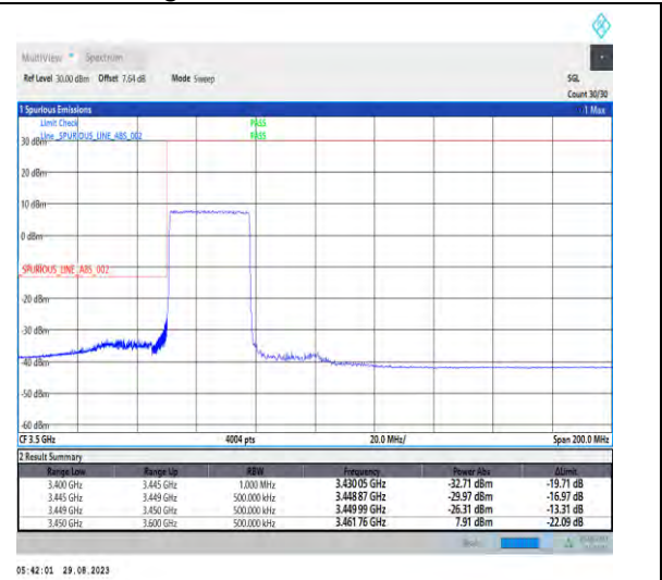
1-N77-3450-3550-PC2-30-30-L-3-DFT-PI2BPSK-Outer_Full-75@0-Ant5-1--PASS-see graph
