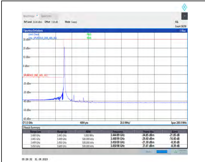
1-N77-3450-3550-PC2-30-25-L-1-DFT-PI2BPSK-Edge_1RB_Left-1@0-Ant5-1--PASS-see graph
