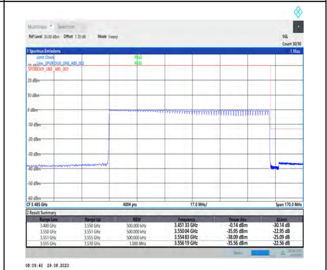
1-N77-3450-3550-PC2-30-100-H-6-CP-QPSK-Outer_Full-273@0-Ant5-1--PASS-see graph
