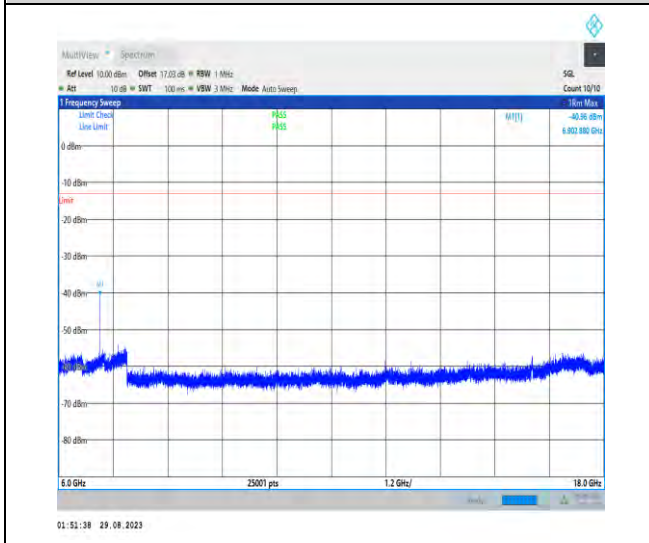
1-N77-3450-3550-PC2-30-100-M-1-DFT-PI2BPSK- Inner_1RB_Left-1@1-6000-18000-Ant5-6902.88--40. 96--13-PASS
