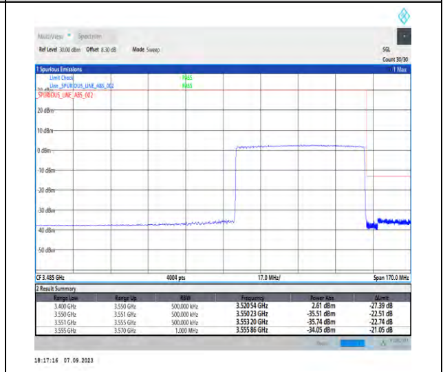
1-N77-3450-3550-PC2-30-60-H-6-CP-QPSK-Outer_Full-162@0-Ant5-1--PASS-see graph
