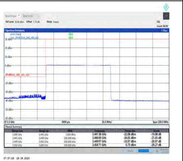
1-N77-3450-3550-PC2-30-80-L-6-CP-QPSK-Outer_Full-217@0-Ant5-1--PASS-see graph
