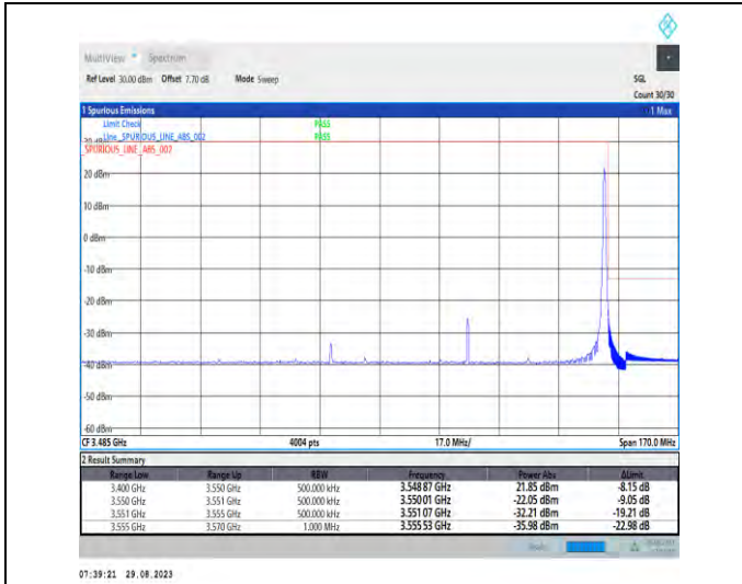
1-N77-3450-3550-PC2-30-80-H-2-DFT-PI2BPSK-Edge_1RB_Right-1@216-Ant5-1--PASS-see graph
