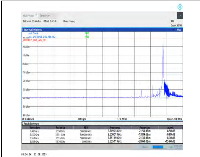
1-N77-3450-3550-PC2-30-25-H-2-DFT-PI2BPSK-Edge_1RB_Right-1@64-Ant5-1--PASS-see graph
