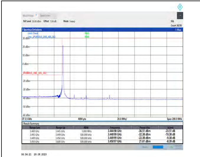
1-N77-3450-3550-PC2-30-60-L-1-DFT-PI2BPSK-Edge_1RB_Left-1@0-Ant5-1--PASS-see graph
