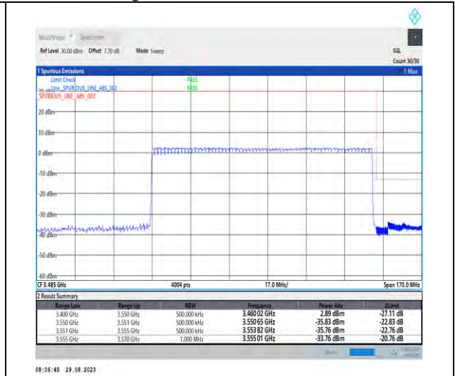
1-N77-3450-3550-PC2-30-100-H-3-DFT-PI2BPSK-Outer_Full-270@0-Ant5-1--PASS-see graph
