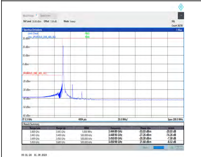
1-N77-3450-3550-PC2-30-25-L-4-CP-QPSK-Edge_1RB_Left-1@0-Ant5-1--PASS-see graph
