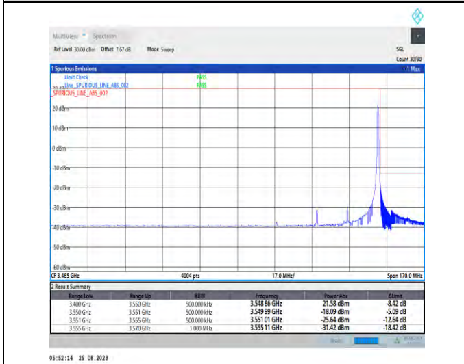
1-N77-3450-3550-PC2-30-30-H-5-CP-QPSK-Edge_1RB_Right-1@77-Ant5-1--PASS-see graph
