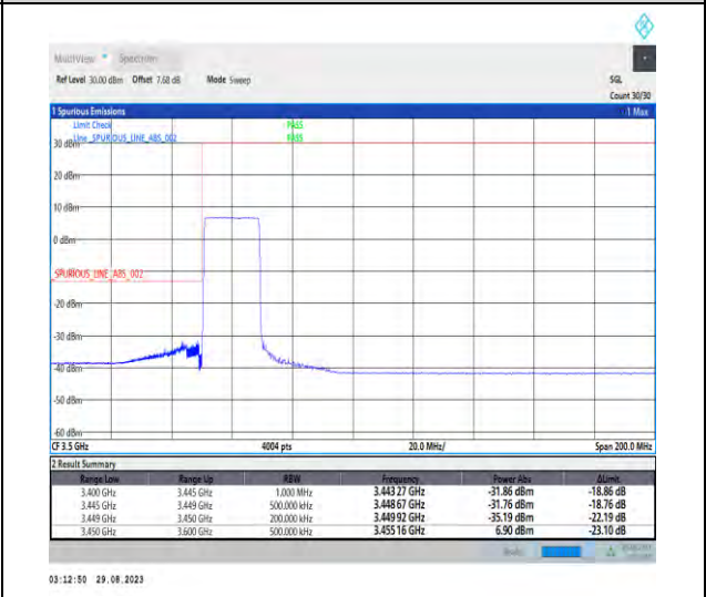
1-N77-3450-3550-PC2-30-20-L-6-CP-QPSK-Outer_Full-51@0-Ant5-1--PASS-see graph
