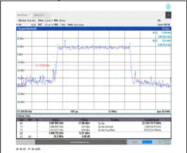
1-N77-3450-3550-PC2-30-25-M-7-CP-16QAM-Outer_Full-65@0-Ant5-23.156-24.30-≤25-PASS
