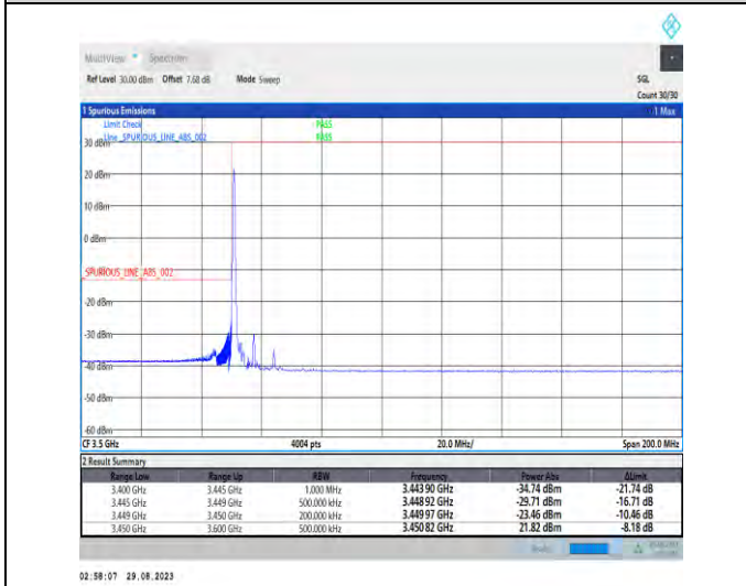
1-N77-3450-3550-PC2-30-15-L-4-CP-QPSK-Edge_1RB_Left-1@0-Ant5-1--PASS-see graph
