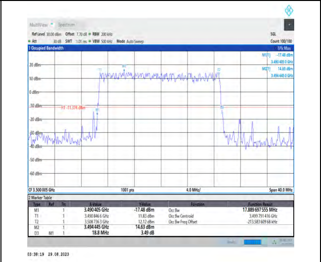
1-N77-3450-3550-PC2-30-20-M-2-DFT-PI2BPSK-Outer_Full-50@0-Ant5-17.89-18.800-≤20-PASS
