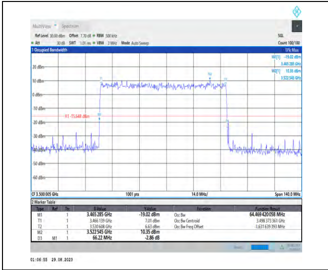
1-N77-3450-3550-PC2-30-70-M-5-DFT-256QAM-Out_er_Full-180@0-Ant5-64.469-66.220-≤70-PASS
