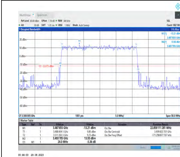
1-N77-3450-3550-PC2-30-25-M-4-DFT-64QAM-Outer_Full-64@0-Ant5-22.859-24.000-≤25-PASS
