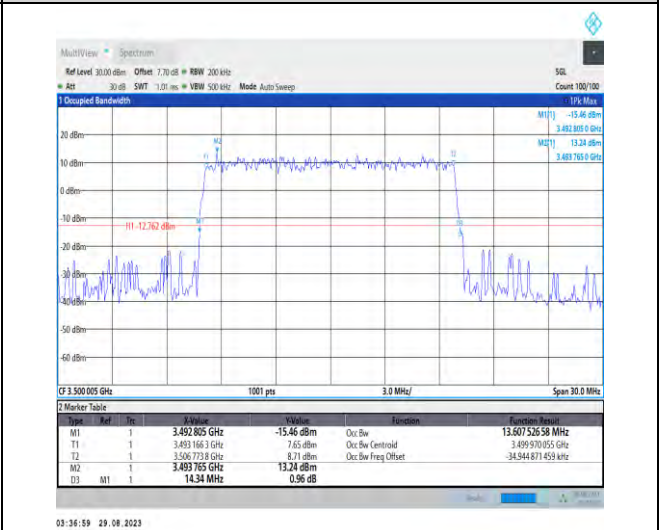
1-N77-3450-3550-PC2-30-15-M-7-CP-16QAM-Outer_Full-38@0-Ant5-13.608-14.340-≤15-PASS
