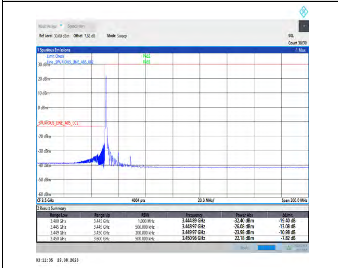
1-N77-3450-3550-PC2-30-20-L-4-CP-QPSK-Edge_1RB_Left-1@0-Ant5-1--PASS-see graph
