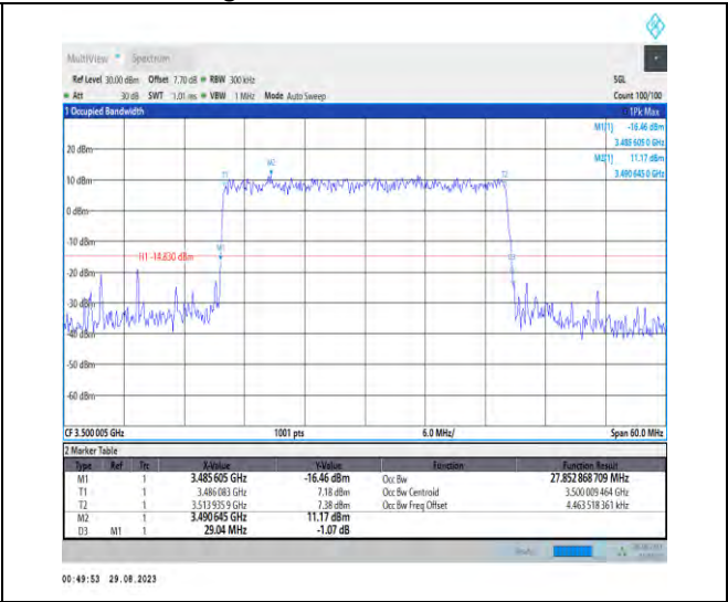
1-N77-3450-3550-PC2-30-30-M-6-CP-QPSK-Outer _Full-78@0-Ant5-27.853-29.040-≤30-PASS
