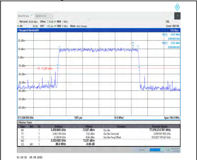
1-N77-3450-3550-PC2-30-80-M-5-DFT-256QAM-Outer_Full-216@0-Ant5-77.076-80.000-≤80-PASS
