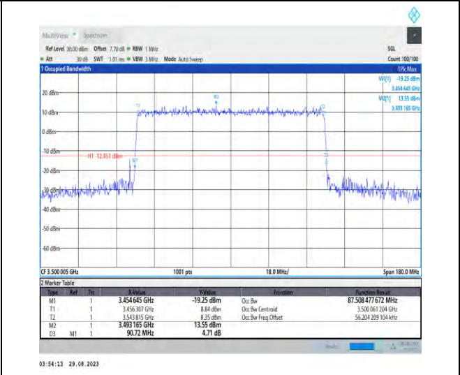
1-N77-3450-3550-PC2-30-90-M-6-CP-QPSK-Outer_Full-245@0-Ant5-87.508-90.720-≤90-PASS
