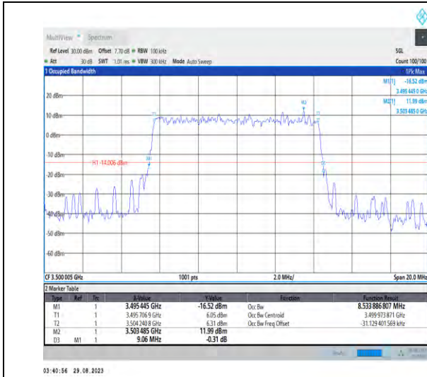
1-N77-3450-3550-PC2-30-10-M-5-DFT-256QAM-Out _Full-24@0-Ant5-8.534-9.060-≤10-PASS
