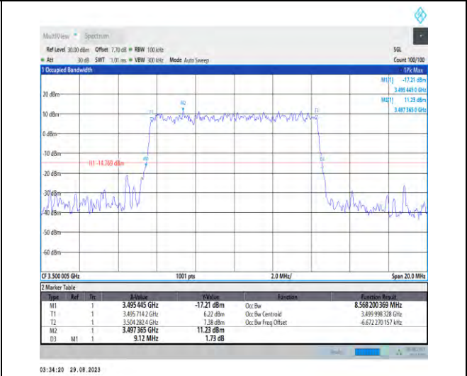
1-N77-3450-3550-PC2-30-10-M-8-CP-64QAM-Outer _Full-24@0-Ant5-8.568-9.120-≤10-PASS
