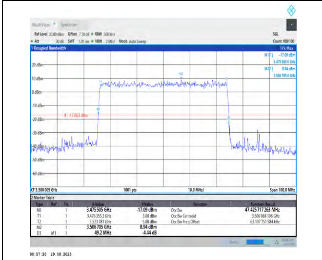
1-N77-3450-3550-PC2-30-50-M-9-CP-256QAM-Outer _Full-133@0-Ant5-47.426-49.200-≤50-PASS
