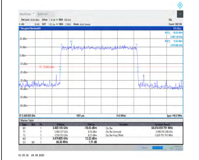
1-N77-3450-3550-PC2-30-70-M-3-DFT-16QAM-Outer_Full-180@0-Ant5-64.016-66.360-≤70-PASS
