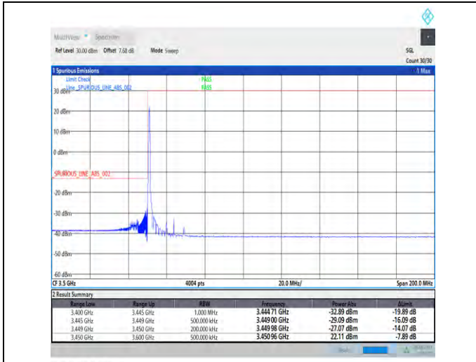
1-N77-3450-3550-PC2-30-20-L-1-DFT-PI2BPSK-Edge_1RB_Left-1@0-Ant5-1--PASS-see graph
