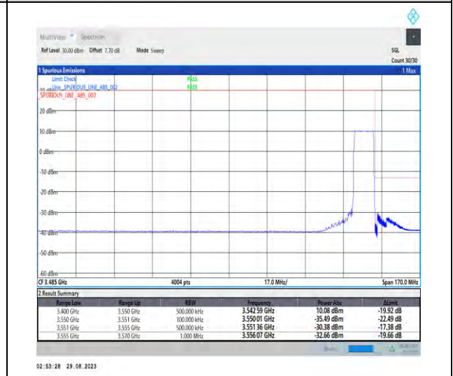
1-N77-3450-3550-PC2-30-10-H-6-CP-QPSK-Outer_Full-24@0-Ant5-1--PASS-see graph
