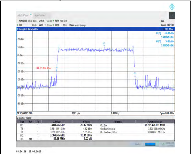
1-N77-3450-3550-PC2-30-40-M-9-CP-256QAM-Outer_Full-106@0-Ant5-37.785-39.680-≤40-PASS
