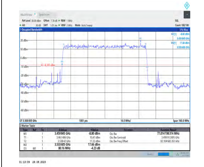
1-N77-3450-3550-PC2-30-80-M-2-DFT-PI2BPSK-Outer_Full-216@0-Ant5-77.014-80.160-≤80-PASS
