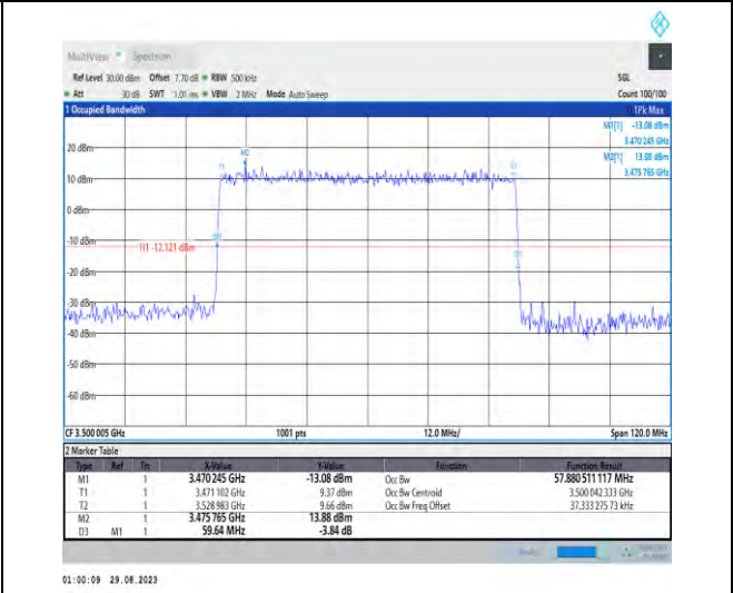
1-N77-3450-3550-PC2-30-60-M-1-DFT-QPSK-Outer _Full-162@0-Ant5-57.881-59.640-≤60-PASS
