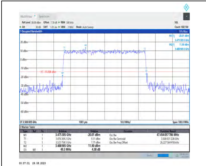
1-N77-3450-3550-PC2-30-50-M-7-CP-16QAM-Outer _Full-133@0-Ant5-47.454-49.300-≤50-PASS
