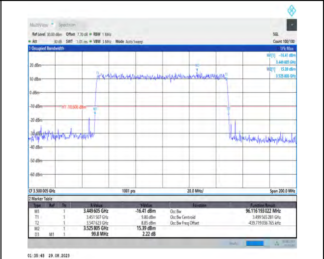
1-N77-3450-3550-PC2-30-100-M-1-DFT-QPSK-Outer_Full-270@0-Ant5-96.116-99.800-≤100-PASS
