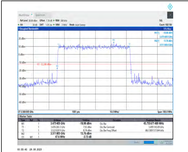
1-N77-3450-3550-PC2-30-50-M-3-DFT-16QAM-Outer_Full-128@0-Ant5-45.756-47.600-≤50-PASS
