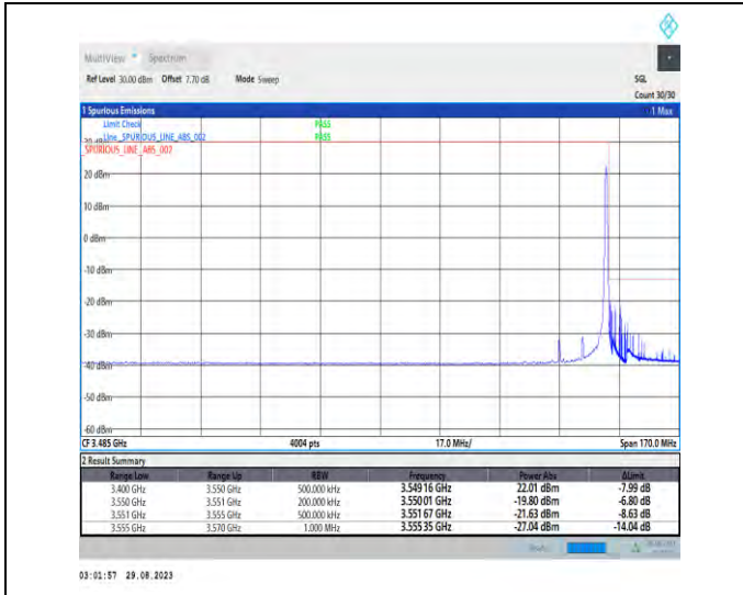
1-N77-3450-3550-PC2-30-15-H-2-DFT-PI2BPSK-Edge_1RB_Right-1@37-Ant5-1--PASS-see graph
