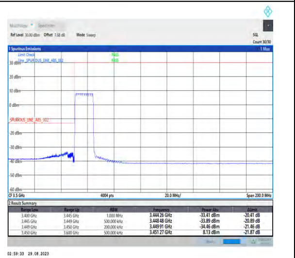
1-N77-3450-3550-PC2-30-15-L-6-CP-QPSK-Outer_Full-38@0-Ant5-1--PASS-see graph
