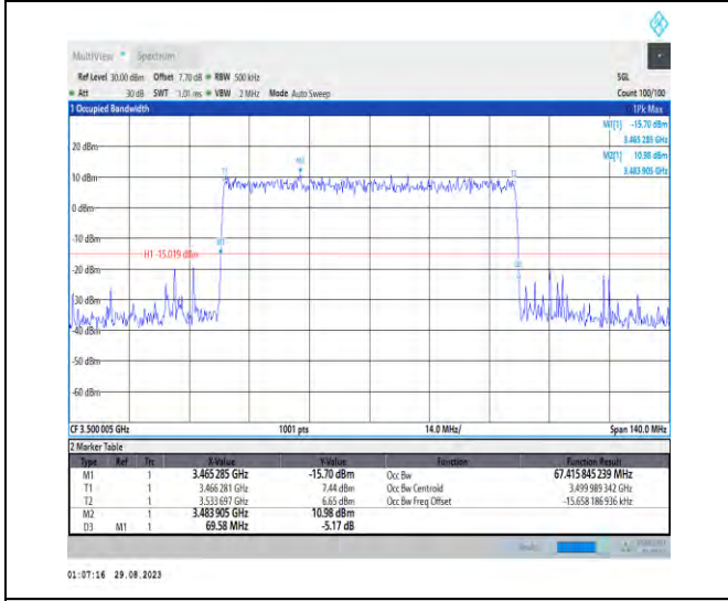
1-N77-3450-3550-PC2-30-70-M-7-CP-16QAM-Outer_Full-189@0-Ant5-67.416-69.580-≤70-PASS
