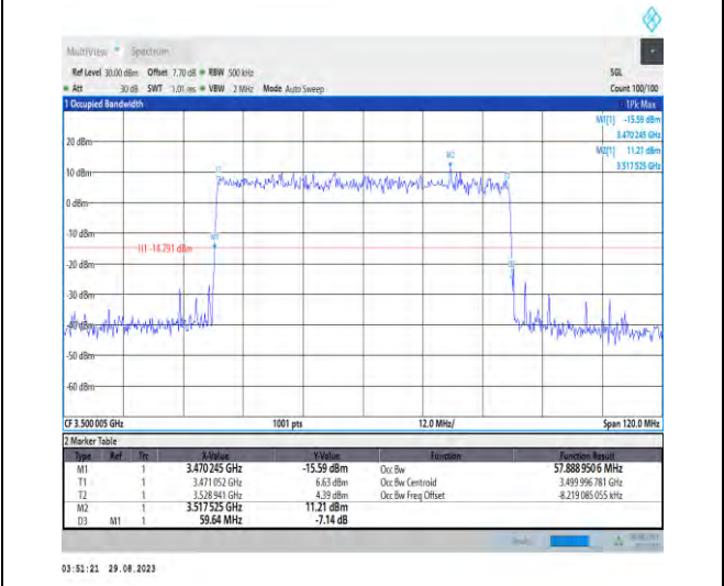
1-N77-3450-3550-PC2-30-60-M-5-DFT-256QAM-Outer_Full-162@0-Ant5-57.889-59.640-≤60-PASS
