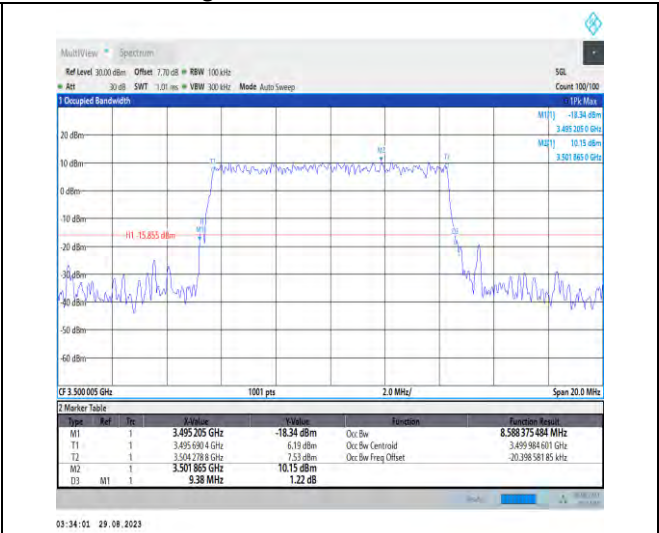
1-N77-3450-3550-PC2-30-10-M-6-CP-QPSK-Outer _Full-24@0-Ant5-8.588-9.380-≤10-PASS
