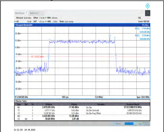
1-N77-3450-3550-PC2-30-60-M-7-CP-16QAM-Outer_Full-162@0-Ant5-57.612-59.640-≤60-PASS
