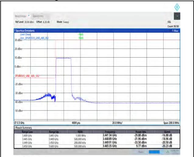
1-N77-3450-3550-PC2-30-20-L-3-DFT-PI2BPSK-Outer_Full-50@0-Ant5-1--PASS-see graph
