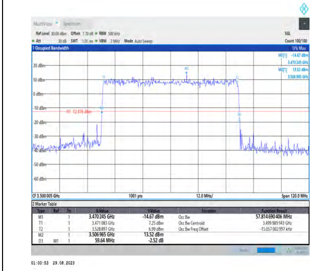
1-N77-3450-3550-PC2-30-60-M-4-DFT-64QAM-Outer_Full-162@0-Ant5-57.815-59.640-≤60-PASS
