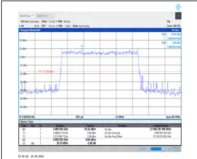
1-N77-3450-3550-PC2-30-30-M-9-CP-256QAM-Outer_Full-78@0-Ant5-27.947-29.160-≤30-PASS
