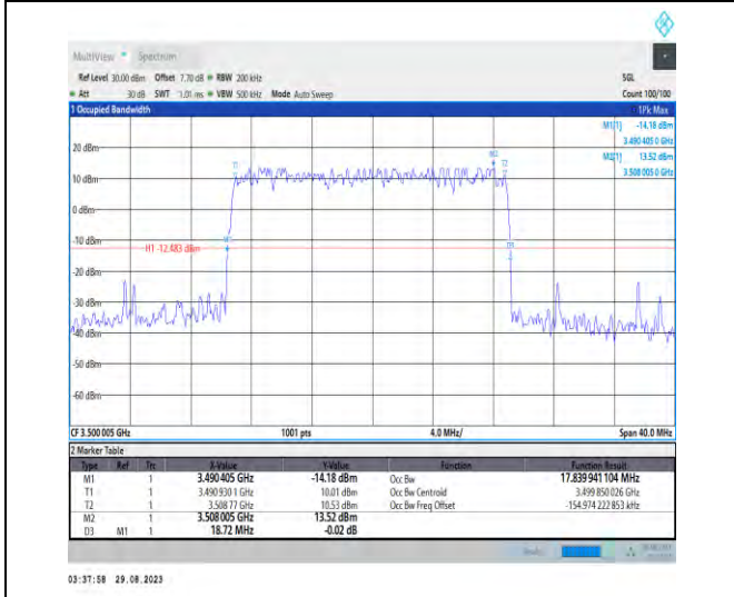
1-N77-3450-3550-PC2-30-20-M-1-DFT-QPSK-Outer_Full-50@0-Ant5-17.84-18.720-≤20-PASS
