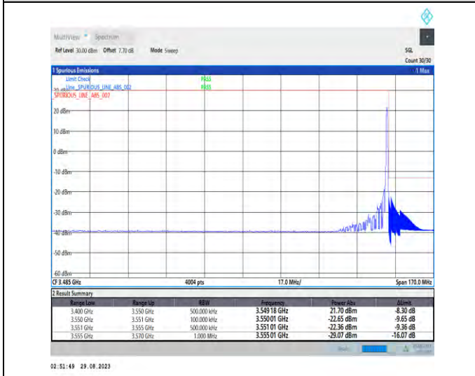
1-N77-3450-3550-PC2-30-10-H-5-CP-QPSK-Edge_1RB_Right-1@23-Ant5-1--PASS-see graph
