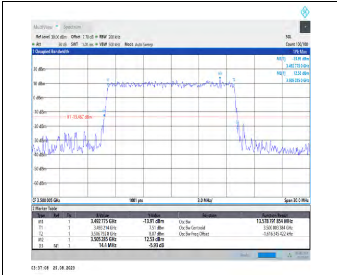
1-N77-3450-3550-PC2-30-15-M-8-CP-64QAM-Outer_Full-38@0-Ant5-13.579-14.400-≤15-PASS
