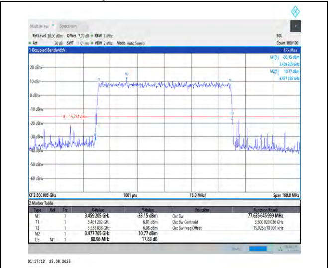
1-N77-3450-3550-PC2-30-80-M-9-CP-256QAM-Out_er_Full-217@0-Ant5-77.636-80.960-≤80-PASS
