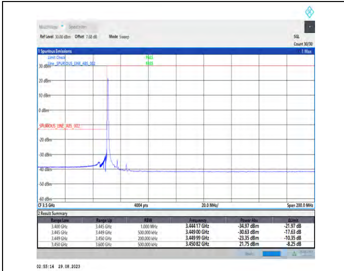
1-N77-3450-3550-PC2-30-15-L-1-DFT-PI2BPSK-Edge_1RB_Left-1@0-Ant5-1--PASS-see graph
