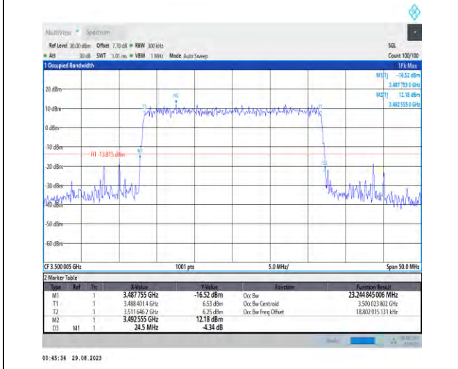
1-N77-3450-3550-PC2-30-25-M-8-CP-64QAM-Outer_Full-65@0-Ant5-23.245-24.500-≤25-PASS
