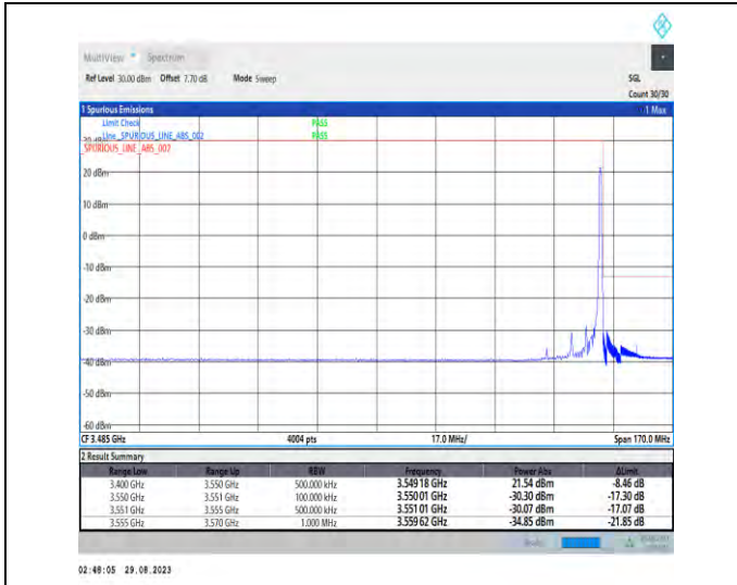
1-N77-3450-3550-PC2-30-10-H-2-DFT-PI2BPSK-Edge_1RB_Right-1@23-Ant5-1--PASS-see graph
