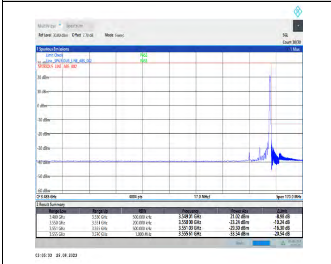
1-N77-3450-3550-PC2-30-15-H-5-CP-QPSK-Edge_1RB_Right-1@37-Ant5-1--PASS-see graph
