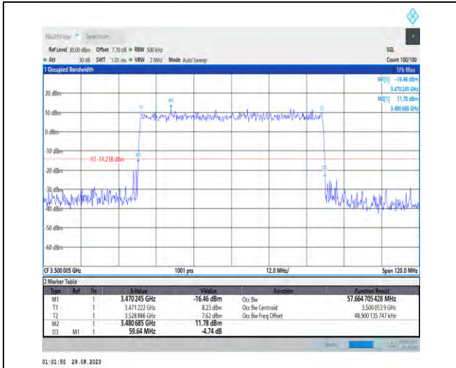
1-N77-3450-3550-PC2-30-60-M-6-CP-QPSK-Outer_Full-162@0-Ant5-57.665-59.640-≤60-PASS
