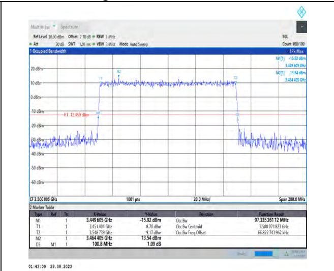
1-N77-3450-3550-PC2-30-100-M-7-CP-16QAM-Outer_Full-273@0-Ant5-97.335-100.800-≤100-PASS
