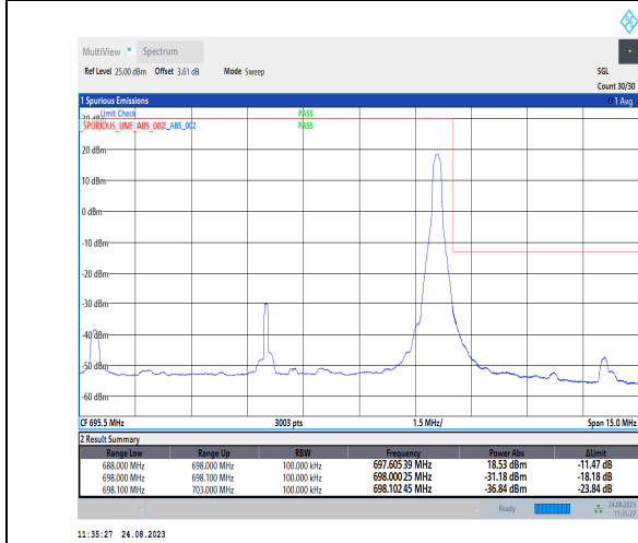
1-N71-PC3-15-10-H-5-CP-QPSK-Edge_1RB_Right-1@51-Ant1-1--PASS-see graph
