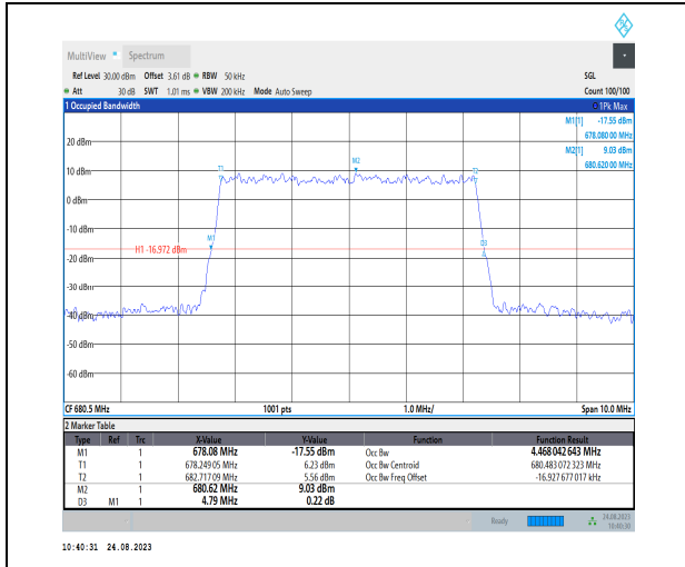
1-N71-PC3-15-5-M-5-DFT-256QAM-Outer_Full-25@ 0-Ant1-4.468-4.790-≤5-PASS
