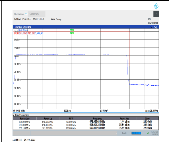
1-N71-PC3-15-20-H-6-CP-QPSK-Outer_Full-106 @0-Ant1-1--PASS-see graph
