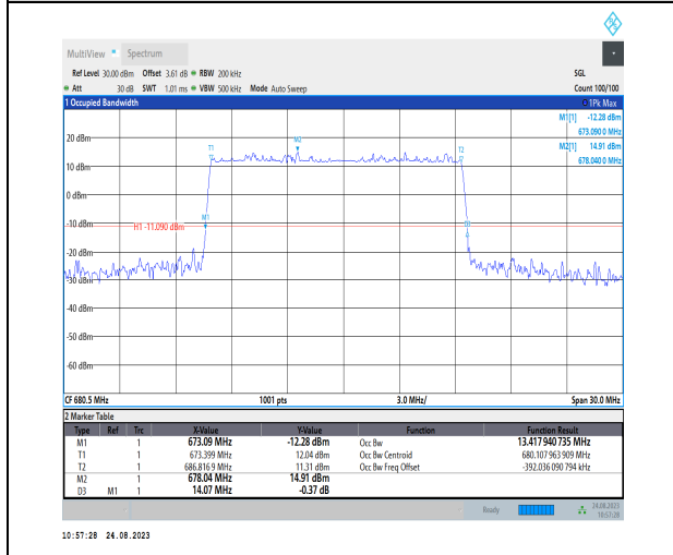
1-N71-PC3-15-15-M-1-DFT-QPSK-Outer_Full-75@0 -Ant1-13.418-14.070-≤15-PASS
