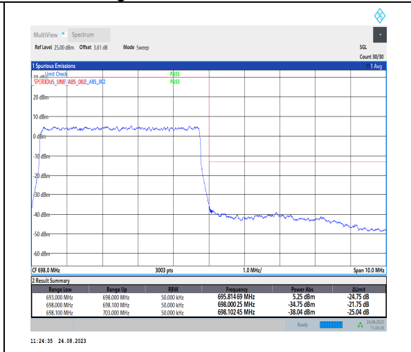
1-N71-PC3-15-5-H-3-DFT-PI2BPSK-Outer_Full-25@0-Ant1-1--PASS-see graph
