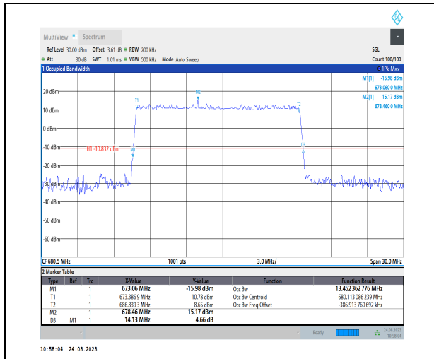
1-N71-PC3-15-15-M-3-DFT-16QAM-Outer_Full-75@ 0-Ant1-13.452-14.130-≤15-PASS
