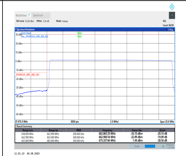
1-N71-PC3-15-20-L-6-CP-QPSK-Outer_Full-106@0-Ant1-1--PASS-see graph
