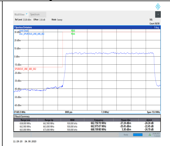
1-N71-PC3-15-10-L-3-DFT-PI2BPSK-Outer_Full-5@0-Ant1-1--PASS-see graph
