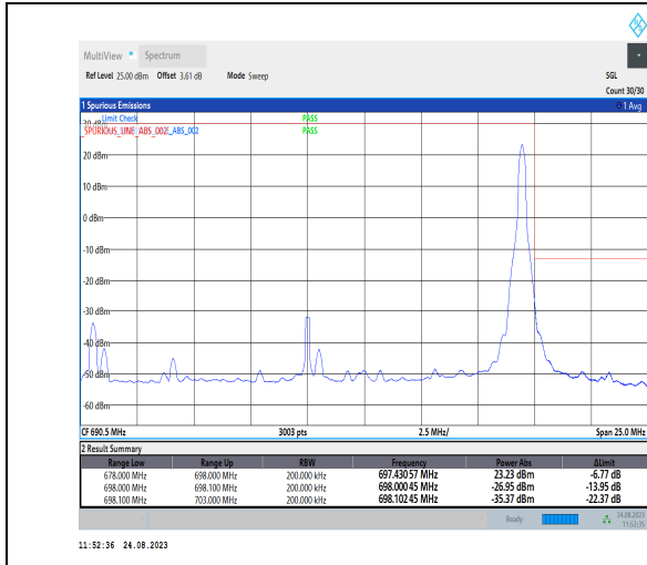
1-N71-PC3-15-20-H-2-DFT-PI2BPSK-Edge_1RB_Righ t-1@105-Ant1-1--PASS-see graph
