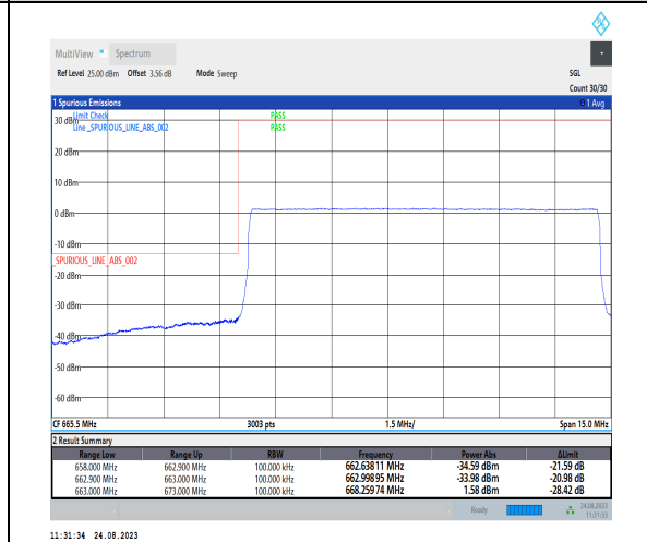
1-N71-PC3-15-10-L-6-CP-QPSK-Outer_Full-52@0-Ant1-1--PASS-see graph
