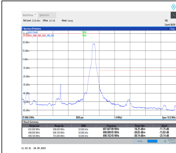
1-N71-PC3-15-5-H-2-DFT-PI2BPSK-Edge_1RB_Right-1@24-Ant1-1--PASS-see graph
