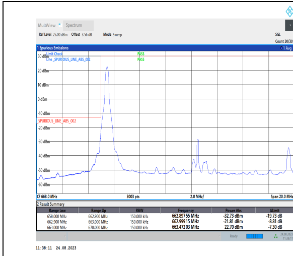
1-N71-PC3-15-15-L-1-DFT-PI2BPSK-Edge_1RB_Left-1@0-Ant1-1--PASS-see graph
