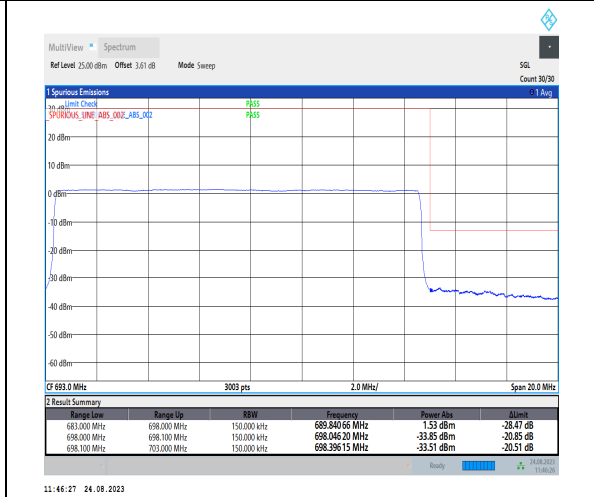
1-N71-PC3-15-15-H-6-CP-QPSK-Outer_Full-79@0-Ant1-1--PASS-see graph
