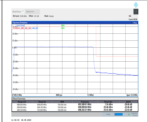
1-N71-PC3-15-10-H-6-CP-QPSK-Outer_Full-52@0-Ant1-1--PASS-see graph
