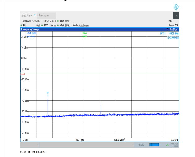
1-N71-PC3-15-20-M-1-DFT-PI2BPSK-Inner_1RB_Lef t-1@1-1000-3000-Ant1-1342.00--36.06--13-PASS
