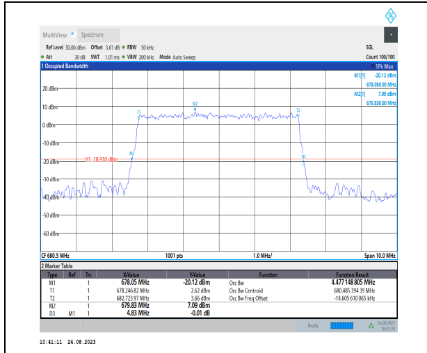
1-N71-PC3-15-5-M-9-CP-256QAM-Outer_Full-25@0 -Ant1-4.477-4.830-≤5-PASS
