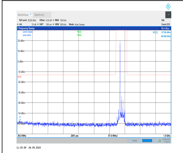
1-N71-PC3-15-20-H-1-DFT-PI2BPSK-Inner_1RB_L eft-1@1-30-1000-Ant1-49.40--57.06--13-PASS
