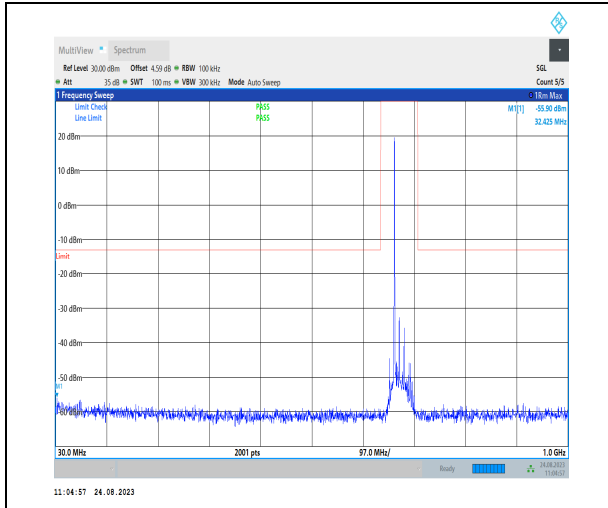
1-N71-PC3-15-20-M-1-DFT-PI2BPSK-Inner_1RB_L eft-1@1-30-1000-Ant1-32.43--55.90--13-PASS
