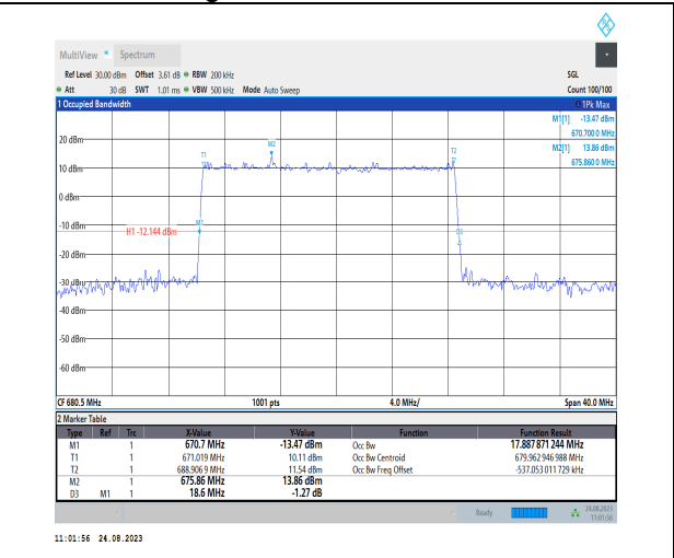
1-N71-PC3-15-20-M-3-DFT-16QAM-Outer_Full-100 @0-Ant1-17.888-18.600-≤20-PASS
