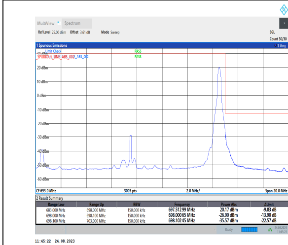
1-N71-PC3-15-15-H-5-CP-QPSK-Edge_1RB_Right-1@78-Ant1-1--PASS-see graph
