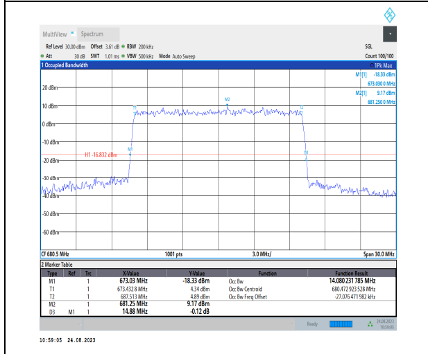
1-N71-PC3-15-15-M-9-CP-256QAM-Outer_Full-79@0 -Ant1-14.08-14.880-≤15-PASS
