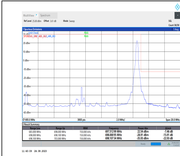
1-N71-PC3-15-15-H-2-DFT-PI2BPSK-Edge_1RB_Right-t1@78-Ant1-1--PASS-see graph
