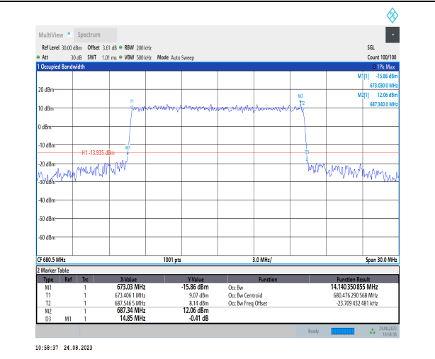
1-N71-PC3-15-15-M-6-CP-QPSK-Outer_Full-79@0- Ant1-14.14-14.850-≤15-PASS
