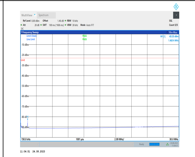
1-N71-PC3-15-20-M-1-DFT-PI2BPSK-Inner_1RB_Lef t-1@1-0.15-30-Ant1-1.46--83.33--23-PASS
