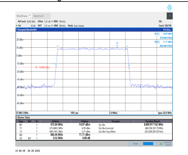
1-N71-PC3-15-10-M-5-DFT-256QAM-Outer_Full-50 @0-Ant1-8.896-9.320-≤10-PASS
