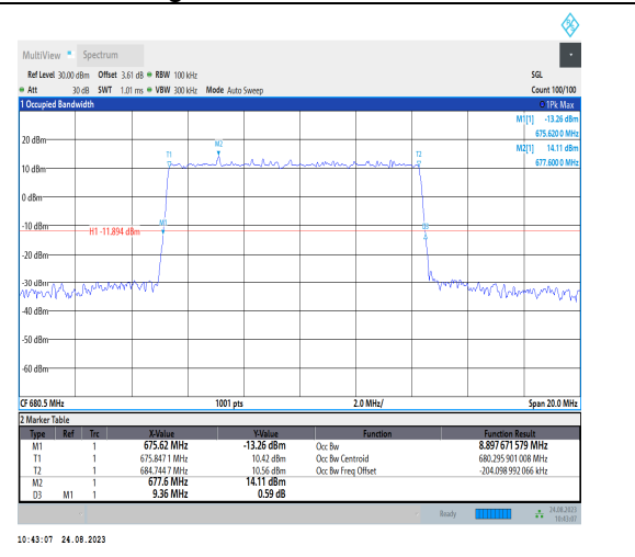
1-N71-PC3-15-10-M-1-DFT-QPSK-Outer_Full-50@0- Ant1-8.898-9.360-≤10-PASS
