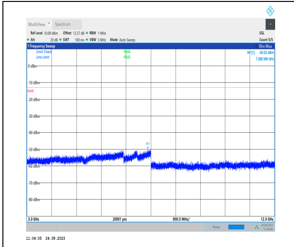
1-N71-PC3-15-20-L-1-DFT-PI2BPSK-Inner_1RB_Lef ft-1@1-3000-12000-Ant1-7389.30--50.02--13-PASS
