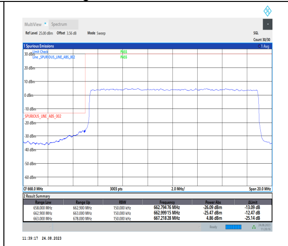
1-N71-PC3-15-15-L-3-DFT-PI2BPSK-Outer_Full-75@0-Ant1-1--PASS-see graph
