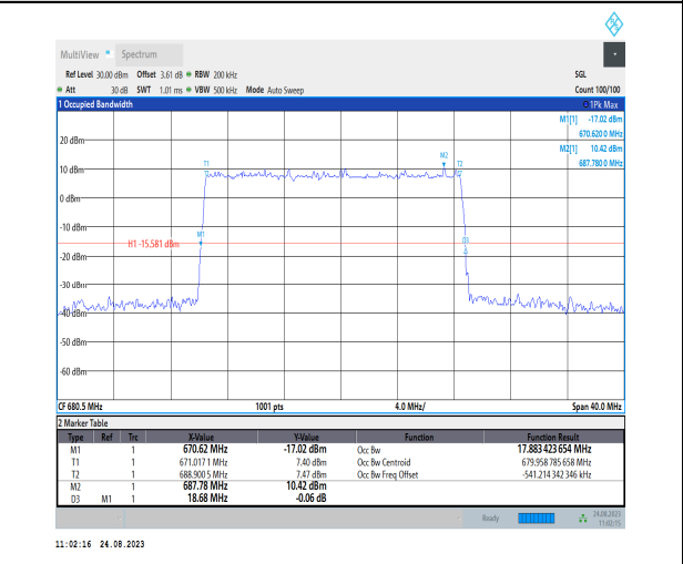
1-N71-PC3-15-20-M-5-DFT-256QAM-Outer_Full-100 @0-Ant1-17.883-18.680-≤20-PASS
