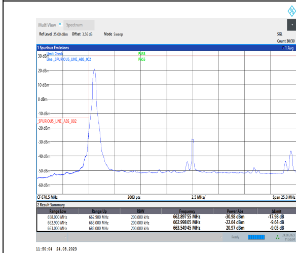
1-N71-PC3-15-20-L-4-CP-QPSK-Edge_1RB_Left-1@0-Ant1-1--PASS-see graph
