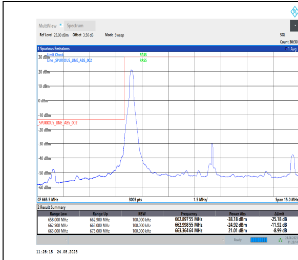
1-N71-PC3-15-10-L-1-DFT-PI2BPSK-Edge_1RB_Left-1@0-Ant1-1--PASS-see graph
