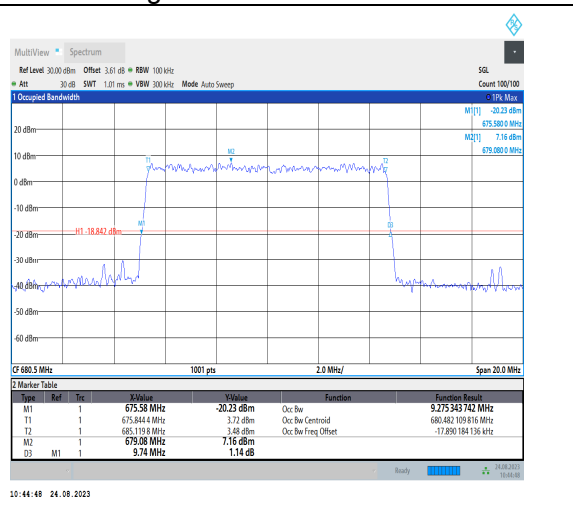
1-N71-PC3-15-10-M-9-CP-256QAM-Outer_Full-52@0 -Ant1-9.275-9.740-≤10-PASS
