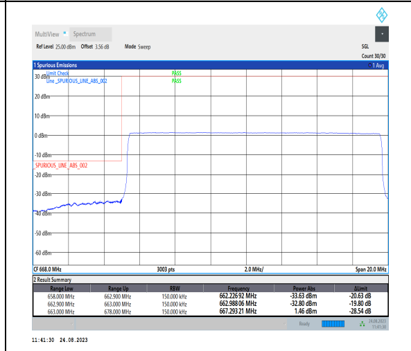
1-N71-PC3-15-15-L-6-CP-QPSK-Outer_Full-79@0-Ant1-1--PASS-see graph
