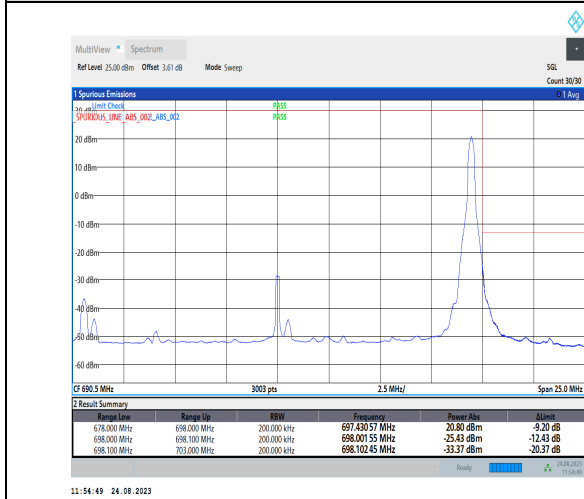
1-N71-PC3-15-20-H-5-CP-QPSK-Edge_1RB_Right-1 @105-Ant1-1--PASS-see graph
