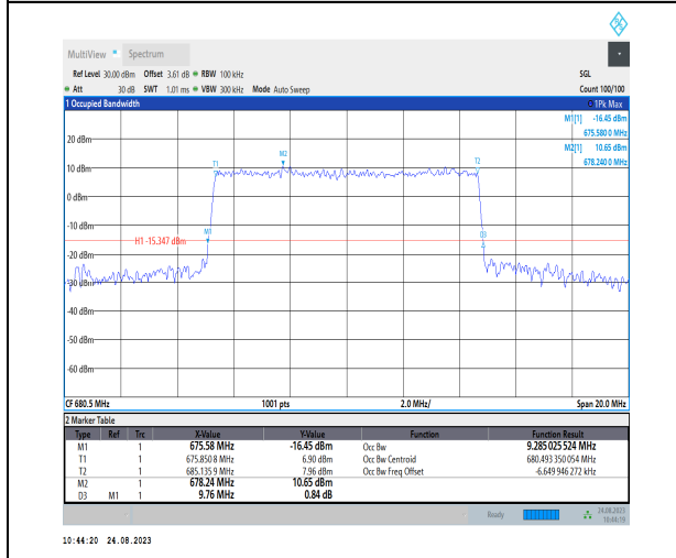
1-N71-PC3-15-10-M-6-CP-QPSK-Outer_Full-52@0- Ant1-9.285-9.760-≤10-PASS
