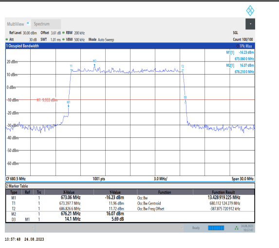
1-N71-PC3-15-15-M-2-DFT-PI2BPSK-Outer_Full-75@0 -Ant1-13.429-14.100-≤15-PASS
