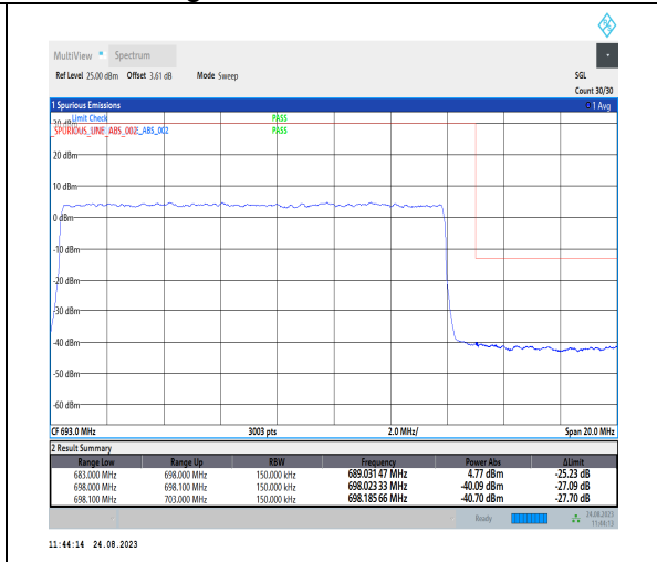
1-N71-PC3-15-15-H-3-DFT-PI2BPSK-Outer_Full-75@0-Ant1-1--PASS-see graph
