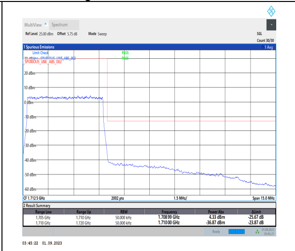
1-N70-PC3-15-5-H-3-DFT-PI2BPSK-Outer_Full-25 @0-Ant3-1-seegraph-PASS-see graph
