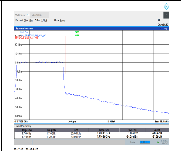
1-N70-PC3-15-5-H-6-CP-QPSK-Outer_Full-25@0-Ant3-1-seegraph-PASS-see graph
