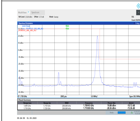
1-N70-PC3-15-20-H-5-CP-QPSK-Edge_1RB_Right-1@105-Ant3-1-seegraph-PASS-see graph
