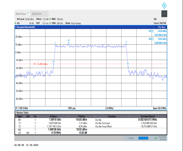
1-N70-PC3-15-10-M-7-CP-16QAM-Outer_Full-52@0 -Ant3-9.302-9.780-≤10-PASS
