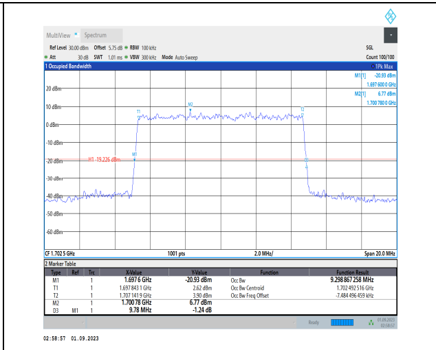
1-N70-PC3-15-10-M-9-CP-256QAM-Outer_Full-52@ 0-Ant3-9.299-9.780-≤10-PASS
