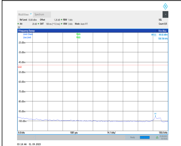
1-N70-PC3-15-15-H-1-DFT-PI2BPSK-Inner_1RB_Le ft-1@1-0.009-0.15-Ant3-0.14--95.92--43-PASS
