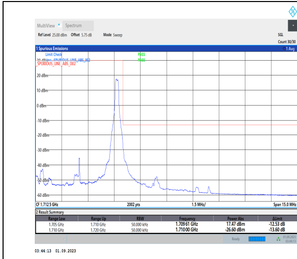
1-N70-PC3-15-5-H-2-DFT-PI2BPSK-Edge_1RB_Right -1@24-Ant3-1-seegraph-PASS-see graph
