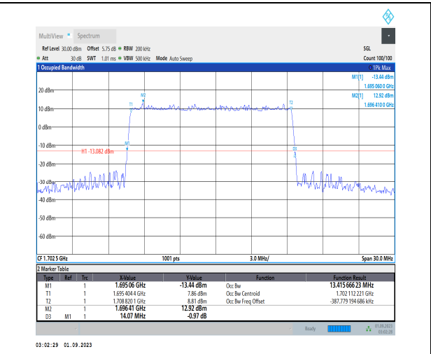
1-N70-PC3-15-15-M-4-DFT-64QAM-Outer_Full-75@ 0-Ant3-13.416-14.070-≤15-PASS
