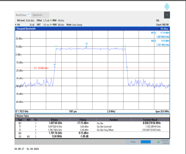
1-N70-PC3-15-10-M-5-DFT-256QAM-Outer_Full-50 @0-Ant3-8.938-9.340-≤10-PASS
