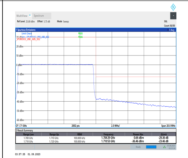
1-N70-PC3-15-10-H-6-CP-QPSK-Outer_Full-52@0-Ant3-1-seegraph-PASS-see graph
