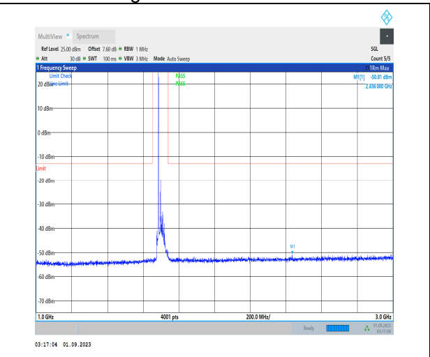
1-N70-PC3-15-15-H-1-DFT-PI2BPSK-Inner_1RB_Le ft-1@1-1000-3000-Ant3-2436.00--50.81--13-PASS
