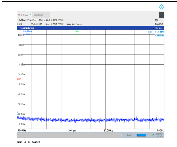
1-N70-PC3-15-15-H-1-DFT-PI2BPSK-Inner_1RB_Le ft-1@1-30-1000-Ant3-34.37--61.81--23-PASS
