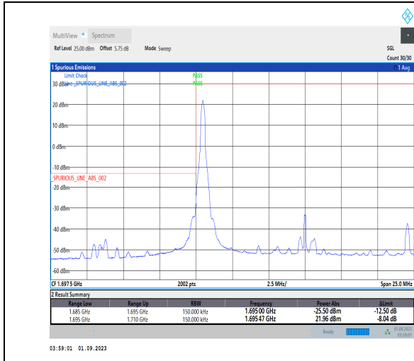
1-N70-PC3-15-15-L-1-DFT-PI2BPSK-Edge_1RB_Left-1@0-Ant3-1-seegraph-PASS-see graph
