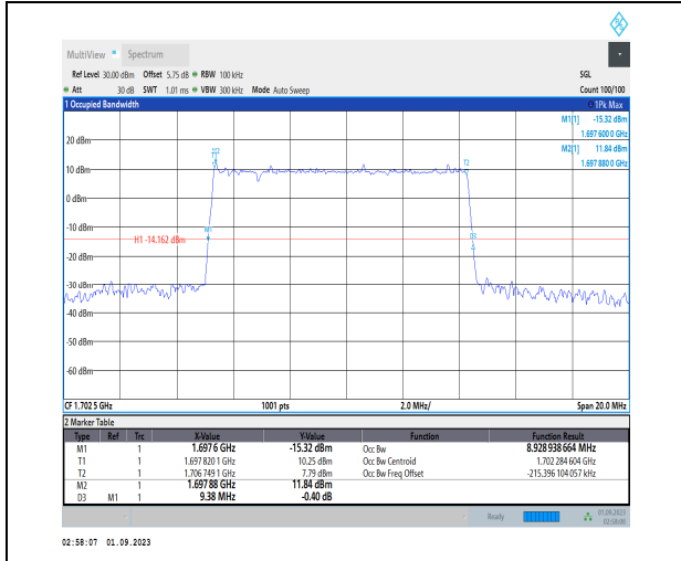
1-N70-PC3-15-10-M-4-DFT-64QAM-Outer_Full-50@ 0-Ant3-8.929-9.380-≤10-PASS
