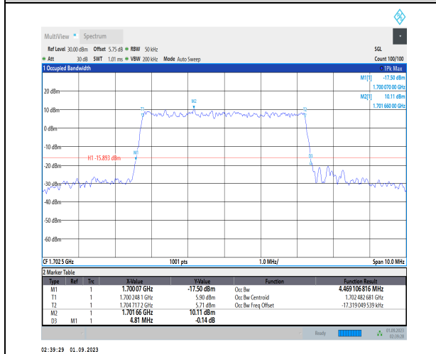
1-N70-PC3-15-5-M-7-CP-16QAM-Outer_Full-25@0- Ant3-4.469-4.810- \leq 5-PASS
