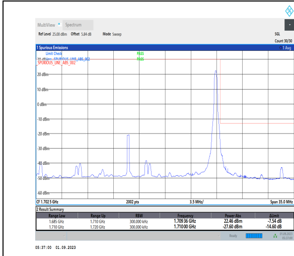
1-N70-PC3-15-25-H-2-DFT-PI2BPSK-Edge_1RB_Righ t-1@132-Ant3-1-seegraph-PASS-see graph
