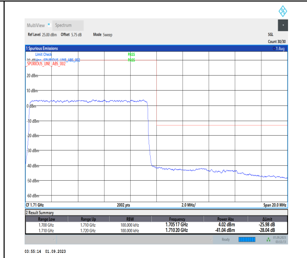
1-N70-PC3-15-10-H-3-DFT-PI2BPSK-Outer_Full-50@0-Ant3-1-seegraph-PASS-see graph
