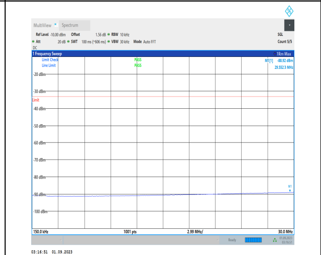
1-N70-PC3-15-15-H-1-DFT-PI2BPSK-Inner_1RB_Le ft-1@1-0.15-30-Ant3-29.55--88.92--33-PASS
