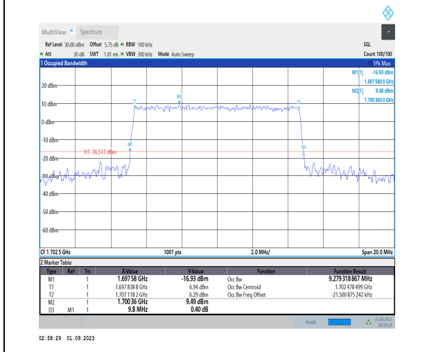
1-N70-PC3-15-10-M-6-CP-QPSK-Outer_Full-52@0- Ant3-9.279-9.800-≤10-PASS
