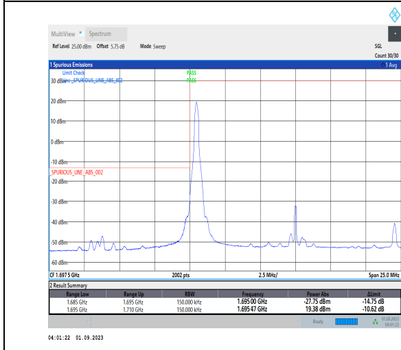
1-N70-PC3-15-15-L-4-CP-QPSK-Edge_1RB_Left-1@0-Ant3-1-seegraph-PASS-see graph
