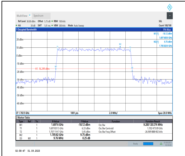
1-N70-PC3-15-10-M-8-CP-64QAM-Outer_Full-52@ 0-Ant3-9.283-9.760-≤10-PASS
