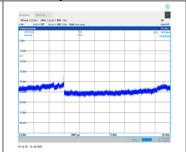
1-N70-PC3-15-15-M-1-DFT-PI2BPSK-Inner_1RB_Le ft-1@1-3000-18000-Ant3-7454.50--39.38--13-PASS
