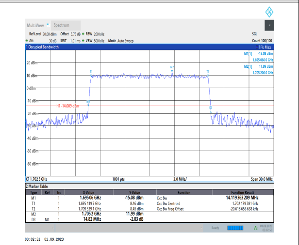
1-N70-PC3-15-15-M-6-CP-QPSK-Outer_Full-79@0- Ant3-14.119-14.820-≤15-PASS
