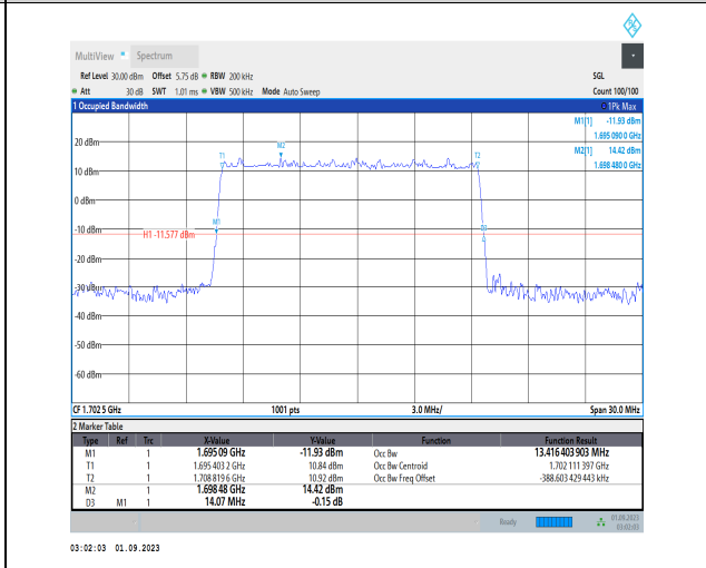
1-N70-PC3-15-15-M-2-DFT-PI2BPSK-Outer_Full-75@ 0-Ant3-13.416-14.070-≤15-PASS
