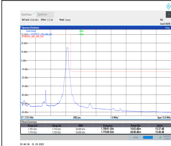
1-N70-PC3-15-5-H-5-CP-QPSK-Edge_1RB_Right-1@ 24-Ant3-1-seegraph-PASS-see graph
