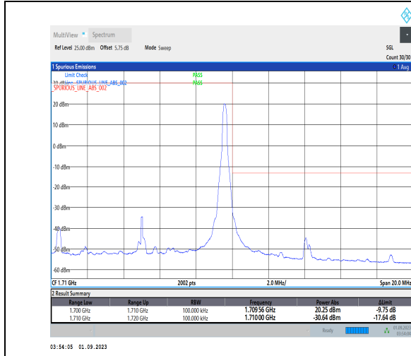
1-N70-PC3-15-10-H-2-DFT-PI2BPSK-Edge_1RB_Right-t-1@51-Ant3-1-seegraph-PASS-see graph
