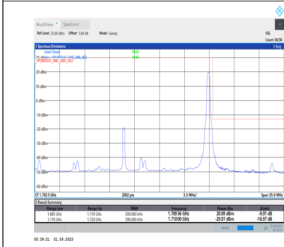
1-N70-PC3-15-25-H-5-CP-QPSK-Edge_1RB_Right-1 @132-Ant3-1-seegraph-PASS-see graph
