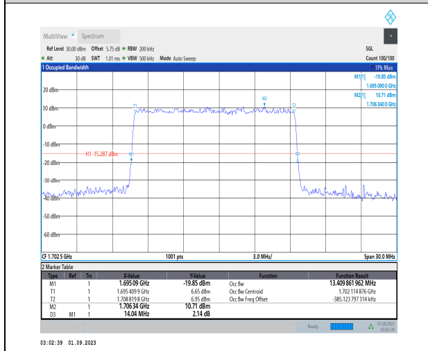
1-N70-PC3-15-15-M-5-DFT-256QAM-Outer_Full-75 @0-Ant3-13.41-14.040-≤15-PASS
