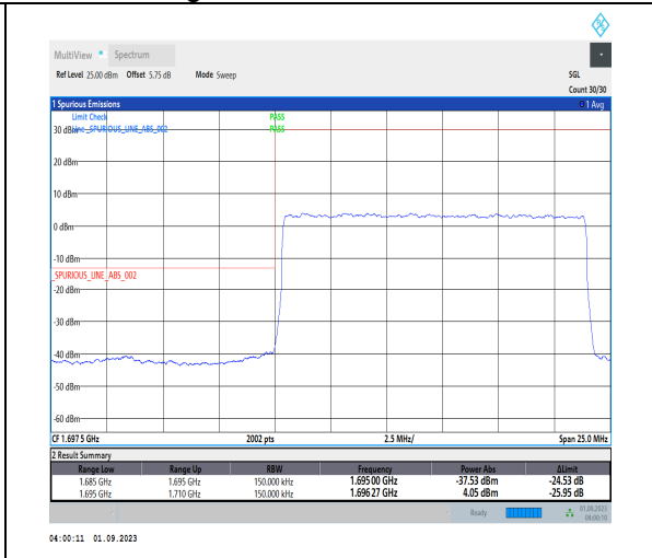
1-N70-PC3-15-15-L-3-DFT-PI2BPSK-Outer_Full-75@0-Ant3-1-seegraph-PASS-see graph
