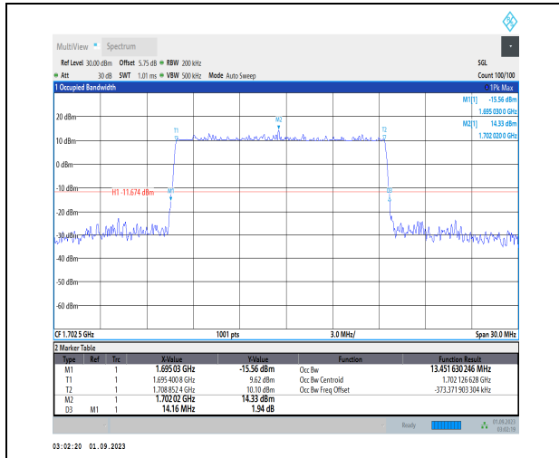
1-N70-PC3-15-15-M-3-DFT-16QAM-Outer_Full-75@ 0-Ant3-13.452-14.160-≤15-PASS
