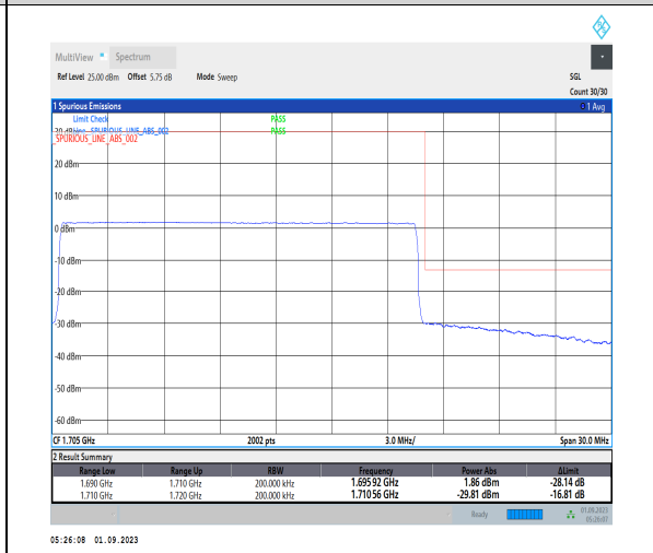
1-N70-PC3-15-20-H-6-CP-QPSK-Outer_Full-106@0-Ant3-1-seegraph-PASS-see graph
