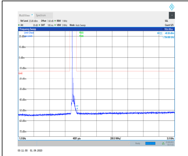
1-N70-PC3-15-15-M-1-DFT-PI2BPSK-Inner_1RB_Le ft-1@1-1000-3000-Ant3-1756.00--49.38--13-PASS
