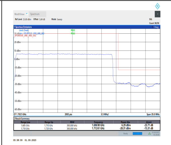
1-N70-PC3-15-25-H-3-DFT-PI2BPSK-Outer_Full-1 28@0-Ant3-1-seegraph-PASS-see graph
