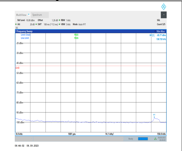
1-N70-PC3-15-15-M-1-DFT-PI2BPSK-Inner_1RB_Le ft-1@1-0.009-0.15-Ant3-0.14--95.77--43-PASS
