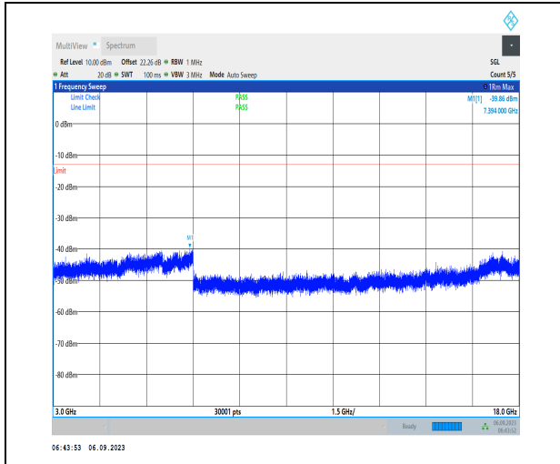
1-N70-PC3-15-15-L-1-DFT-PI2BPSK-Inner_1RB_Lef t-1@1-3000-18000-Ant3-7394.00--39.86--13-PASS
