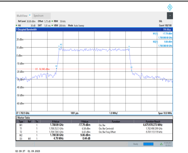
1-N70-PC3-15-5-M-8-CP-64QAM-Outer_Full-25@0- Ant3-4.476-4.790- \leq 5-PASS
