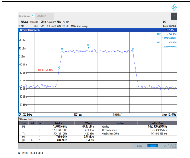
1-N70-PC3-15-5-M-5-DFT-256QAM-Outer_Full-25@ 0-Ant3-4.482-4.840- \leq 5-PASS
