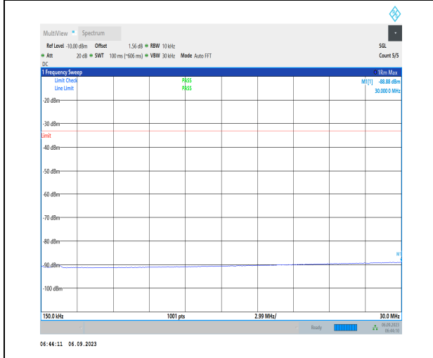
1-N70-PC3-15-15-M-1-DFT-PI2BPSK-Inner_1RB_Le ft-1@1-0.15-30-Ant3-30.00--88.88--33-PASS
