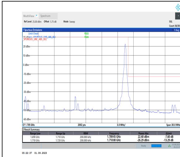
1-N70-PC3-15-20-H-2-DFT-PI2BPSK-Edge_1RB_Right-t-1@105-Ant3-1-seegraph-PASS-see graph
