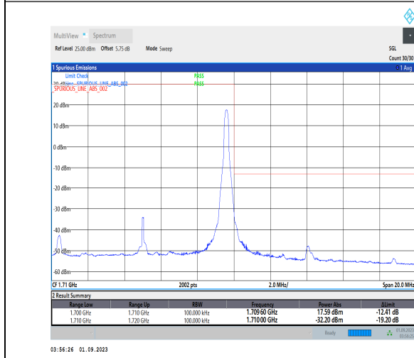
1-N70-PC3-15-10-H-5-CP-QPSK-Edge_1RB_Right-1@51-Ant3-1-seegraph-PASS-see graph
