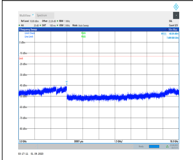
1-N70-PC3-15-15-H-1-DFT-PI2BPSK-Inner_1RB_Le ft-1@1-3000-18000-Ant3-7499.00--40.04--13-PASS
