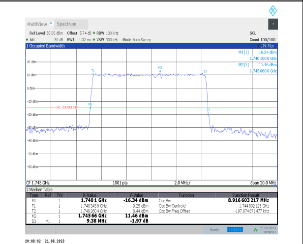
1-N66-PC3-15-10-M-3-DFT-16QAM-Outer_Full-50@0-Ant3-8.917-9.380-<=10-PASS
