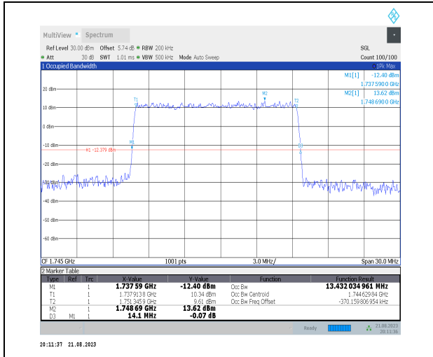
1-N66-PC3-15-15-M-3-DFT-16QAM-Outer_Full-75@ 0-Ant3-13.432-14.100≤15-PASS
