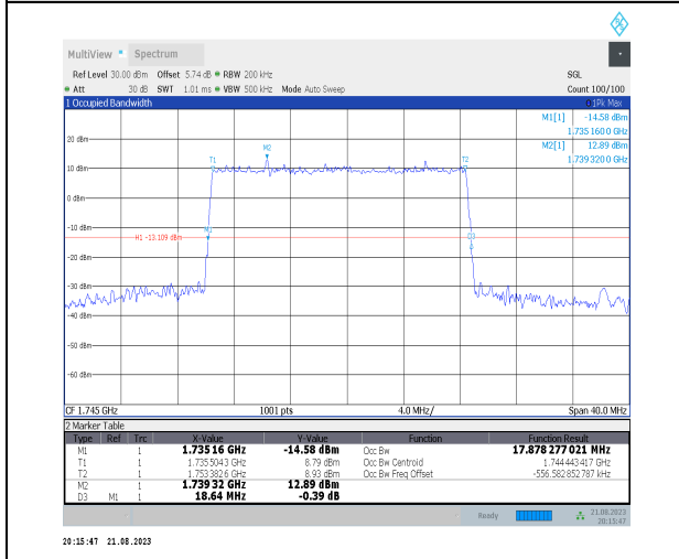
1-N66-PC3-15-20-M-4-DFT-64QAM-Outer_Full-100 @0-Ant3-17.878-18.640-≤20-PASS
