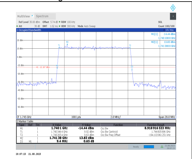
1-N66-PC3-15-10-M-1-DFT-QPSK-Outer_Full-50@0 -Ant3-8.919-9.400-<=10-PASS
