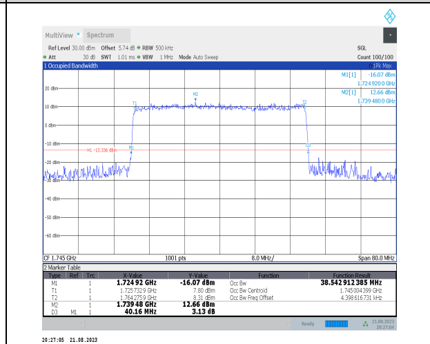
1-N66-PC3-15-40-M-6-CP-QPSK-Outer_Full-216@0 -Ant3-38.526-40.160-≤40-PASS
