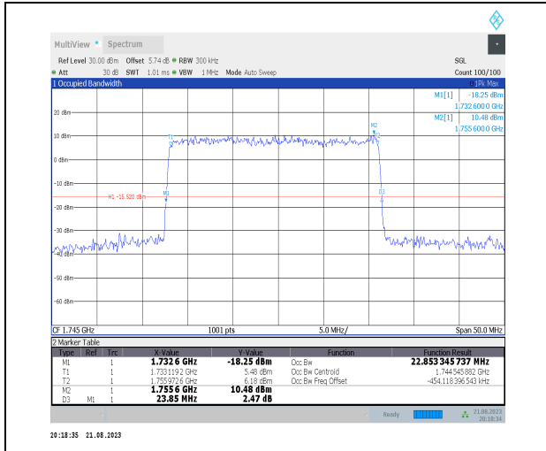
1-N66-PC3-15-25-M-5-DFT-256QAM-Outer_Full-128 @0-Ant3-22.853-23.850-≤25-PASS
