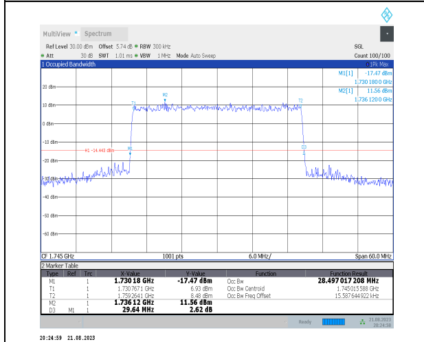
1-N66-PC3-15-30-M-6-CP-QPSK-Outer_Full-160@0 -Ant3-28.5-29.640-≤30-PASS
