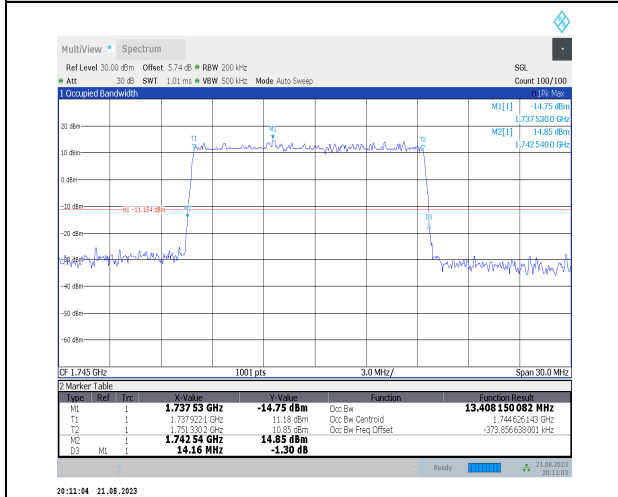
1-N66-PC3-15-15-M-1-DFT-QPSK-Outer_Full-75@0 -Ant3-13.408-14.160-≤15-PASS
