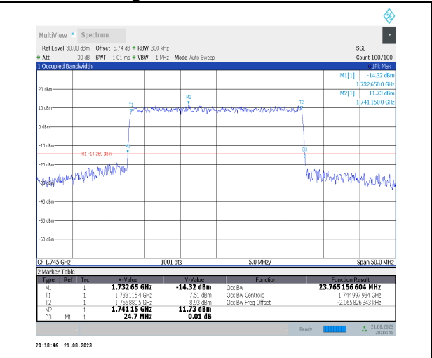
1-N66-PC3-15-25-M-6-CP-QPSK-Outer_Full-133@0 -Ant3-23.765-24.700-≤25-PASS
