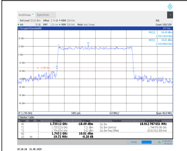
1-N66-PC3-15-20-M-8-CP-64QAM-Outer_Full-106@0 0-Ant3-18.913-19.720-<=20-PASS
