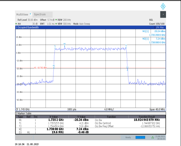
1-N66-PC3-15-20-M-9-CP-256QAM-Outer_Full-106@0 @0-Ant3-18.925-19.600-<=20-PASS
