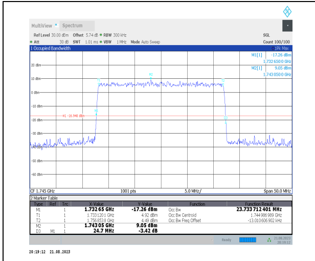
1-N66-PC3-15-25-M-9-CP-25QAM-Outer_Full-133 @0-Ant3-23.734-24.700-≤25-PASS
