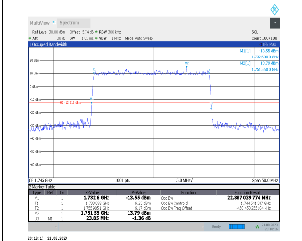
1-N66-PC3-15-25-M-3-DFT-16QAM-Outer_Full-128@ 0-Ant3-22.887-23.850-≤25-PASS
