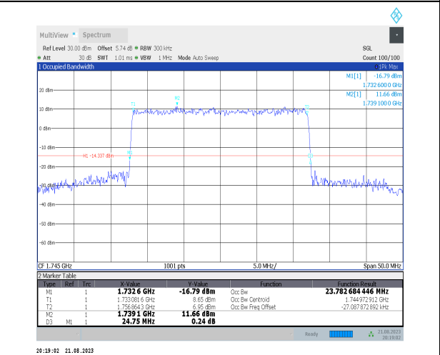
1-N66-PC3-15-25-M-8-CP-64QAM-Outer_Full-133@0-Ant3-23.783-24.750-≤25-PASS
