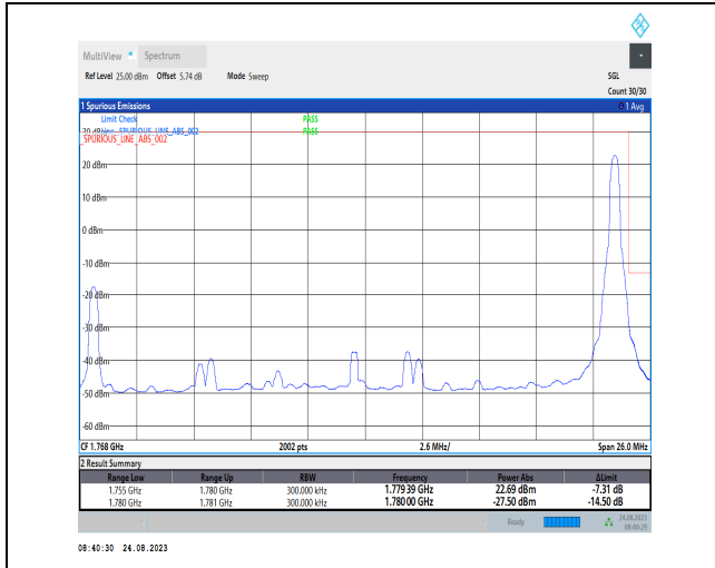
1-N66-PC3-15-25-H-2-DFT-PI2BPSK-Edge_1RB_Right-t-1@132-Ant3-1-seegraph-PASS-see graph
