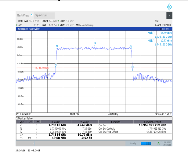
1-N66-PC3-15-20-M-7-CP-16QAM-Outer_Full-106@0 0-Ant3-18.96-19.680-<=20-PASS
