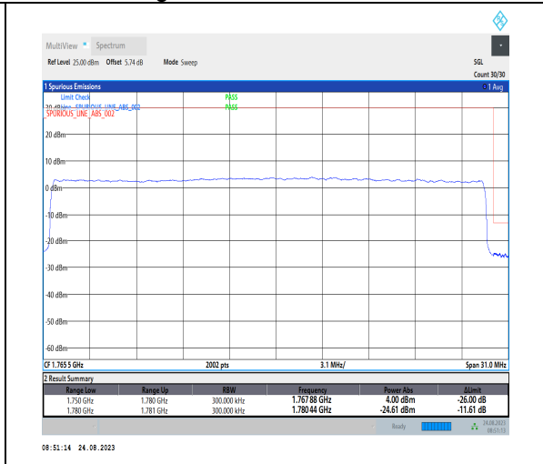
1-N66-PC3-15-30-H-3-DFT-PI2BPSK-Outer_Full-160@0-Ant3-1-seegraph-PASS-see graph
