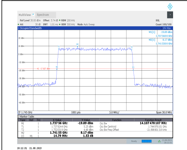
1-N66-PC3-15-15-M-9-CP-256QAM-Outer_Full-79@0 -Ant3-14.107-14.790-≤15-PASS
