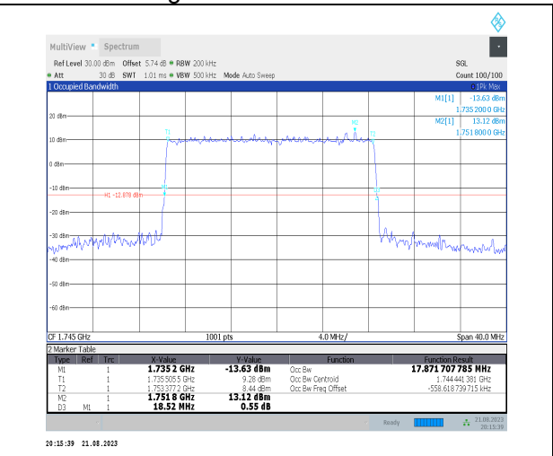
1-N66-PC3-15-20-M-3-DFT-16QAM-Outer_Full-100 @0-Ant3-17.872-18.520-≤20-PASS
