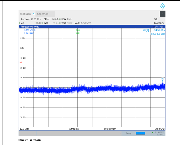
1-N66-PC3-15-40-M-1-DFT-PI2BPSK-Inner_1RB_Lef t-1@1-12000-20000-Ant3-19858.00--34.31--13-PASS
