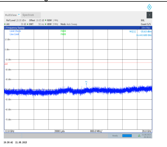
1-N66-PC3-15-40-H-1-DFT-PI2BPSK-Inner_1RB_Lef t-1@1-12000-20000-Ant3-16441.60--35.63--13-PASS
