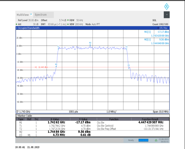
1-N66-PC3-15-5-M-8-CP-64QAM-Outer_Full-25@0-Ant3-4.447-4.730-≤5-PASS
