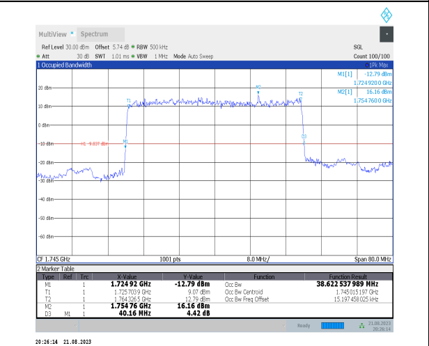
1-N66-PC3-15-40-M-2-DFT-PI2BPSK-Outer_Full-216@ 6@0-Ant3-38.634-40.160-≤40-PASS
