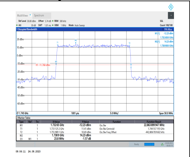
1-N66-PC3-15-25-M-2-DFT-PI2BPSK-Outer_Full-128@ 0-Ant3-22.864-23.800-≤25-PASS
