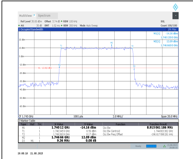
1-N66-PC3-15-10-M-4-DFT-64QAM-Outer_Full-50@ 0-Ant3-8.915-9.360-≤10-PASS
