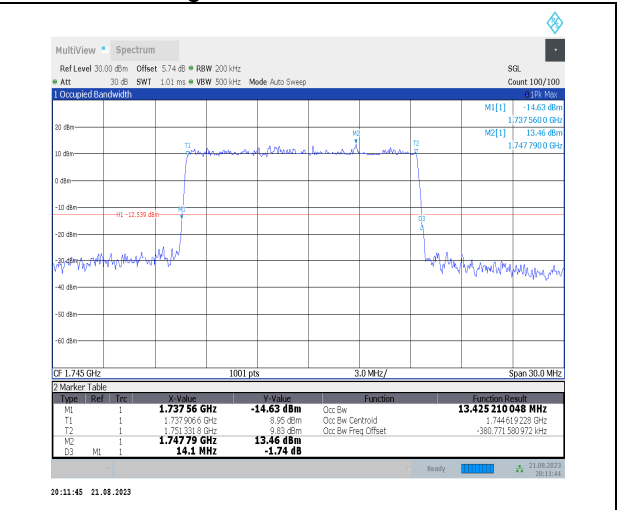
1-N66-PC3-15-15-M-4-DFT-64QAM-Outer_Full-75@ 0-Ant3-13.425-14.100≤15-PASS
