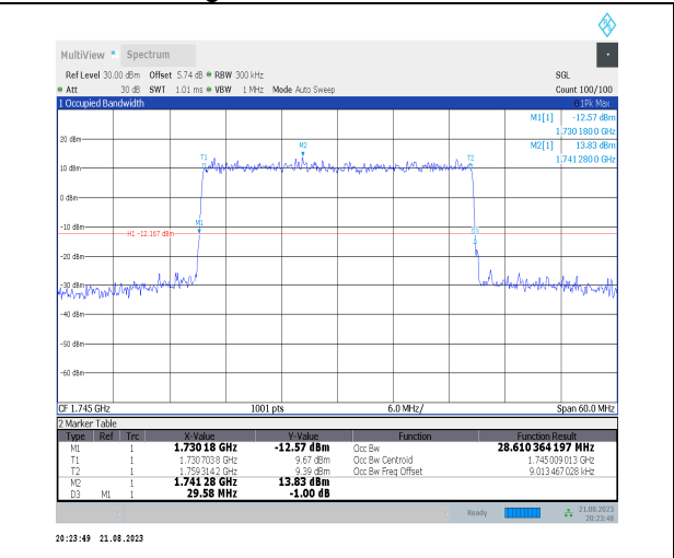
1-N66-PC3-15-30-M-1-DFT-QPSK-Outer_Full-160 @0-Ant3-28.611-29.580-≤30-PASS
