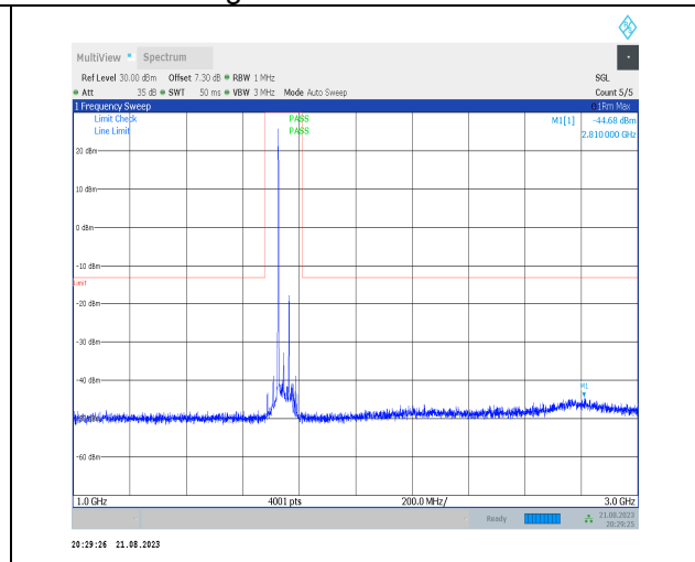
1-N66-PC3-15-40-M-1-DFT-PI2BPSK-Inner_1RB_Lef t-1@1-1000-3000-Ant3-2810.00--44.68--13-PASS
