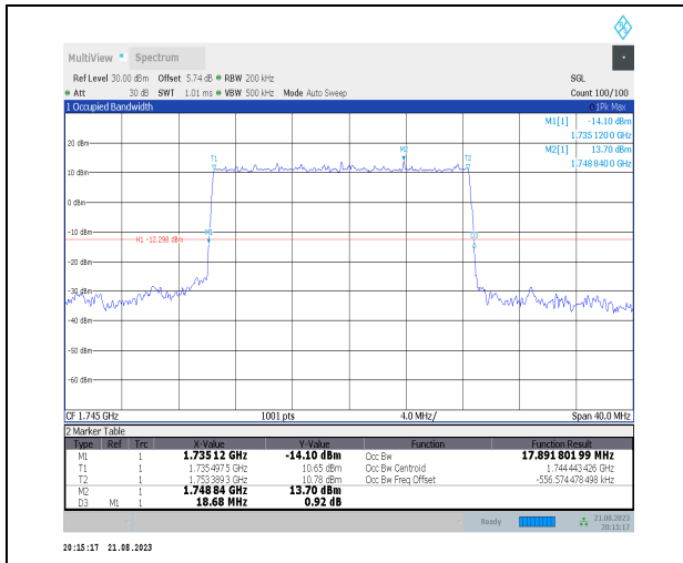
1-N66-PC3-15-20-M-2-DFT-PI2BPSK-Outer_Full-100 @0-Ant3-17.892-18.680-≤20-PASS
