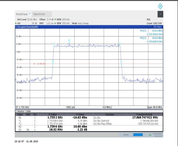
1-N66-PC3-15-20-M-5-DFT-256QAM-Outer_Full-100 @0-Ant3-17.867-18.520-≤20-PASS
