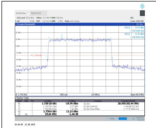
1-N66-PC3-15-30-M-4-DFT-64QAM-Outer_Full-160 @0-Ant3-28.541-29.640-≤30-PASS
