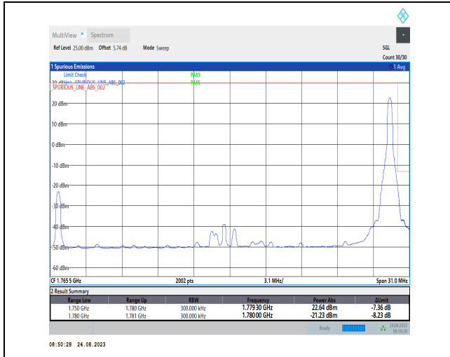
1-N66-PC3-15-30-H-2-DFT-PI2BPSK-Edge_1RB_Right-t-1@159-Ant3-1-seegraph-PASS-see graph
