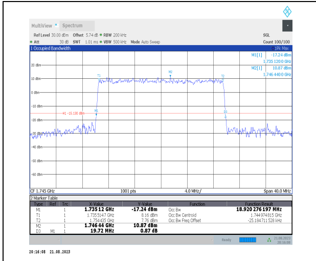
1-N66-PC3-15-20-M-6-CP-QPSK-Outer_Full-106@0 -Ant3-18.92-19.720-<=20-PASS
