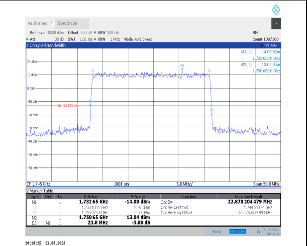
1-N66-PC3-15-25-M-4-DFT-64QAM-Outer_Full-128@ 0-Ant3-22.87-23.800-≤25-PASS
