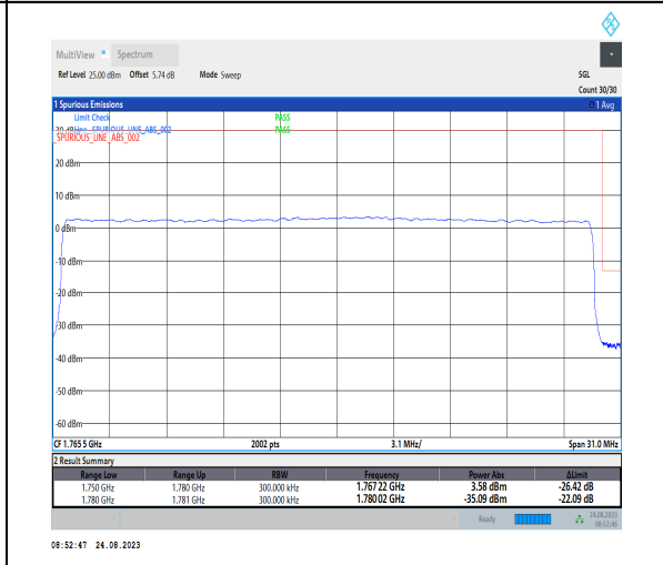
1-N66-PC3-15-30-H-6-CP-QPSK-Outer_Full-160@0-Ant3-1-seegraph-PASS-see graph
