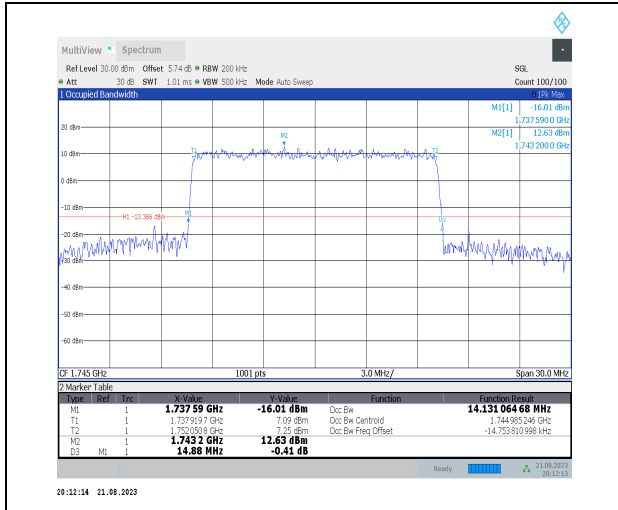
1-N66-PC3-15-15-M-7-CP-16QAM-Outer_Full-79@0 -Ant3-14.131-14.880-≤15-PASS
