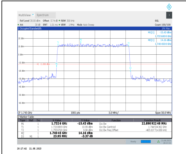
1-N66-PC3-15-25-M-1-DFT-QPSK-Outer_Full-128@ 0-Ant3-22.891-23.950-≤25-PASS
