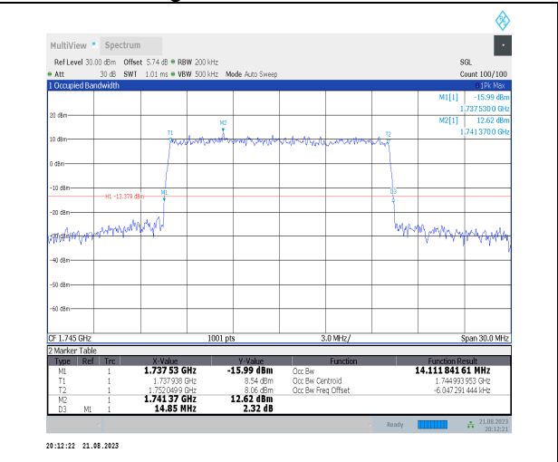
1-N66-PC3-15-15-M-8-CP-64QAM-Outer_Full-79@0 -Ant3-14.112-14.850-≤15-PASS
