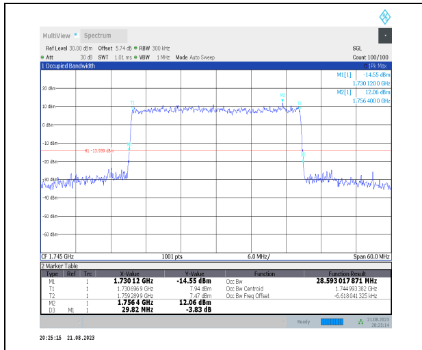
1-N66-PC3-15-30-M-8-CP-64QAM-Outer_Full-160@ 0-Ant3-28.595-29.820-≤30-PASS
