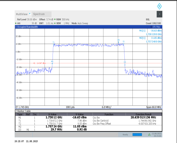
1-N66-PC3-15-30-M-7-CP-16QAM-Outer_Full-160@0 0-Ant3-28.641-29.700-≤30-PASS
