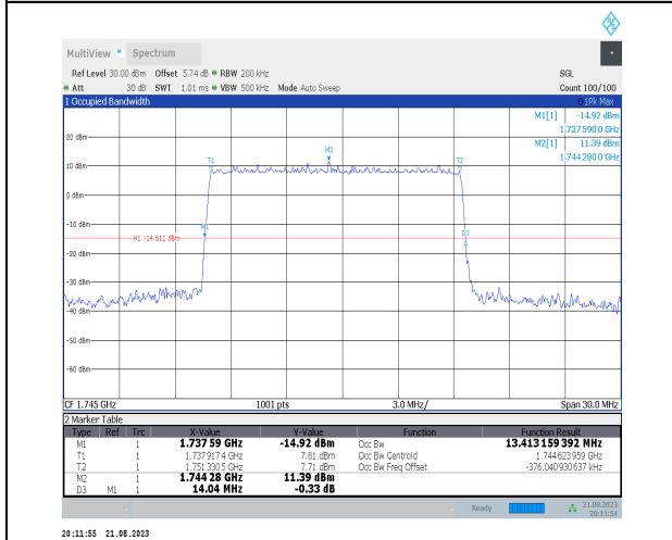
1-N66-PC3-15-15-M-5-DFT-256QAM-Outer_Full-75@ 0-Ant3-13.413-14.040≤15-PASS
