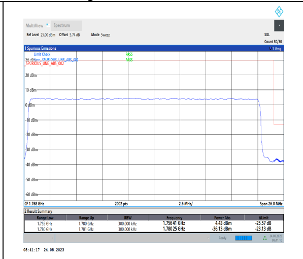
1-N66-PC3-15-25-H-3-DFT-PI2BPSK-Outer_Full-128@0-Ant3-1-seegraph-PASS-see graph
