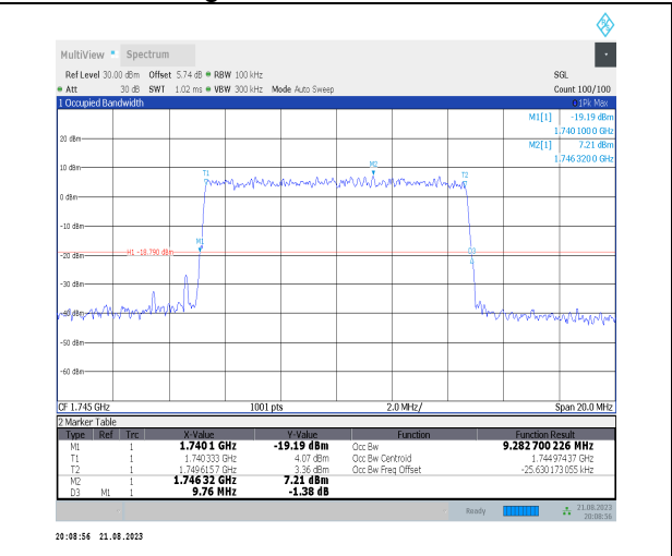
1-N66-PC3-15-10-M-9-CP-256QAM-Outer_Full-52@0-Ant3-9.283-9.760-≤10-PASS
