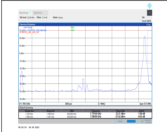
1-N66-PC3-15-30-H-5-CP-QPSK-Edge_1RB_Right-1@159-Ant3-1-seegraph-PASS-see graph
