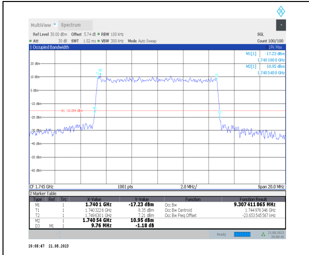
1-N66-PC3-15-10-M-8-CP-64QAM-Outer_Full-52@0 -Ant3-9.307-9.760-≤10-PASS
