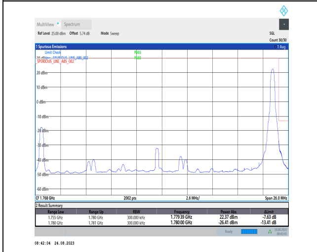
1-N66-PC3-15-25-H-5-CP-QPSK-Edge_1RB_Right-1@132-Ant3-1-seegraph-PASS-see graph
