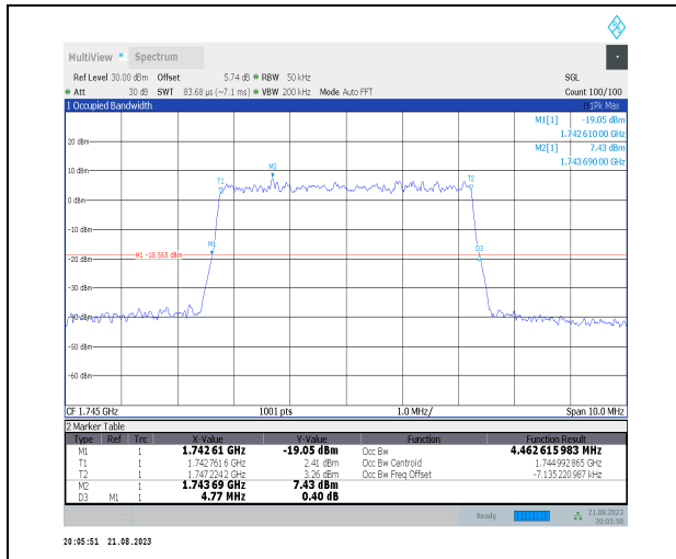
1-N66-PC3-15-5-M-9-CP-256QAM-Outer_Full-25@0 -Ant3-4.463-4.770-<=5-PASS
