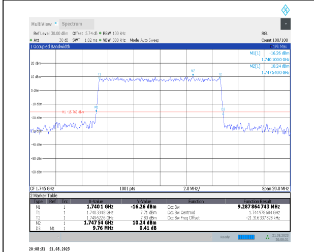
1-N66-PC3-15-10-M-6-CP-QPSK-Outer_Full-52@0- Ant3-9.288-9.760-≤10-PASS
