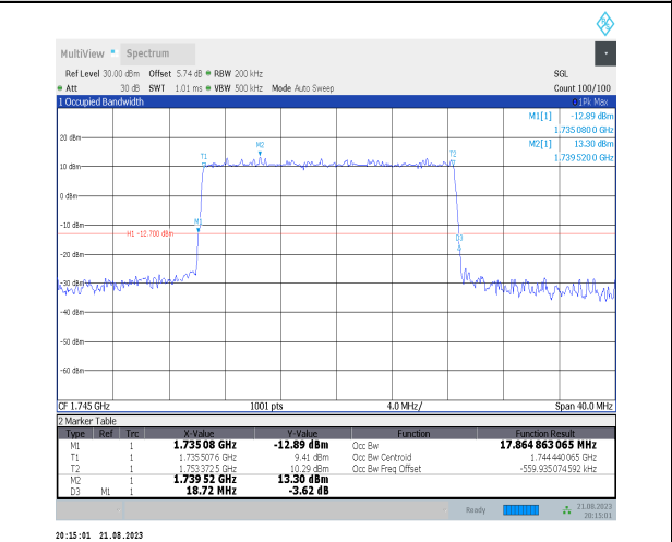
1-N66-PC3-15-20-M-1-DFT-QPSK-Outer_Full-100@0 -Ant3-17.865-18.720-≤20-PASS
