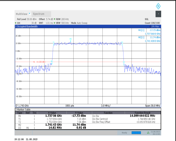
1-N66-PC3-15-15-M-6-CP-QPSK-Outer_Full-79@0- Ant3-14.099-14.820≤15-PASS
