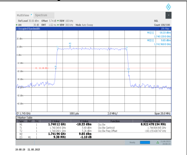
1-N66-PC3-15-10-M-5-DFT-256QAM-Outer_Full-50 @0-Ant3-8.922-9.380-≤10-PASS
