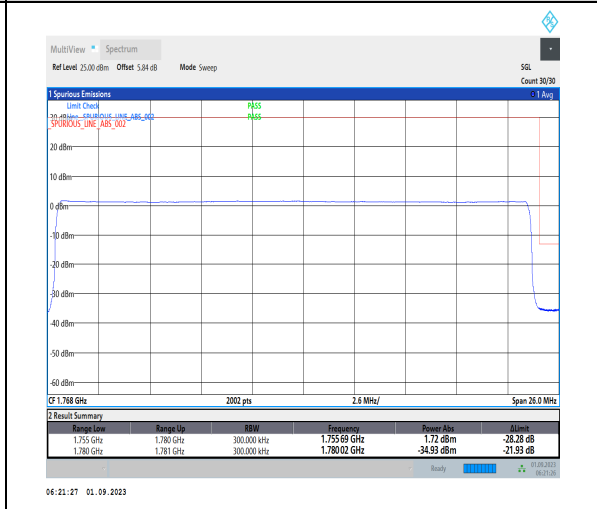
1-N66-PC3-15-25-H-6-CP-QPSK-Outer_Full-133@0-Ant3-1-seegraph-PASS-see graph
