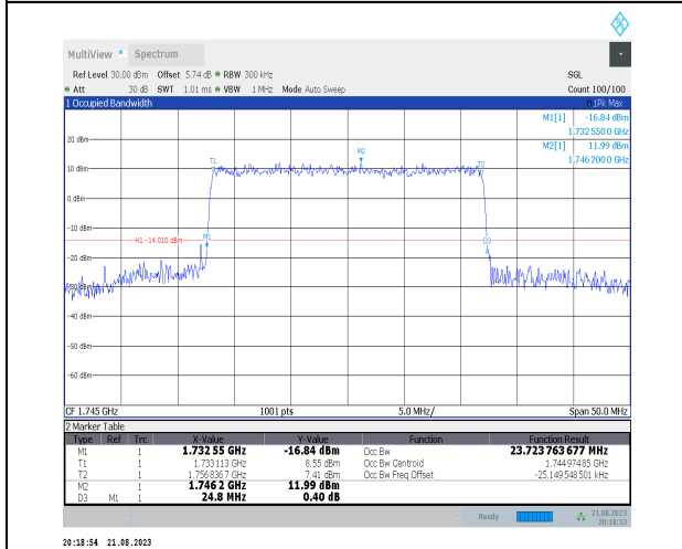
1-N66-PC3-15-25-M-7-CP-16QAM-Outer_Full-133@0-Ant3-23.724-24.800-≤25-PASS
