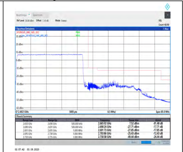
1-N41-PC2-30-40-H-3-DFT-PI2BPSK-Outer_Full-1 00@0-Ant3-1--PASS-see graph
