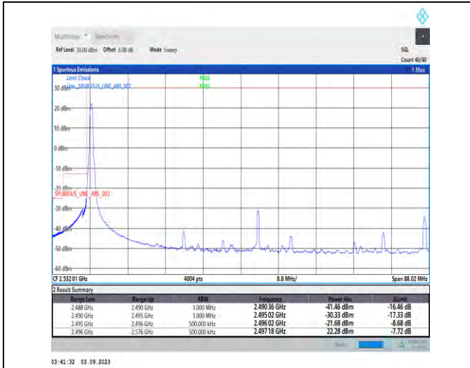
1-N41-PC2-30-80-L-1-DFT-PI2BPSK-Edge_1RB_Left-1@0-Ant3-1--PASS-see graph
