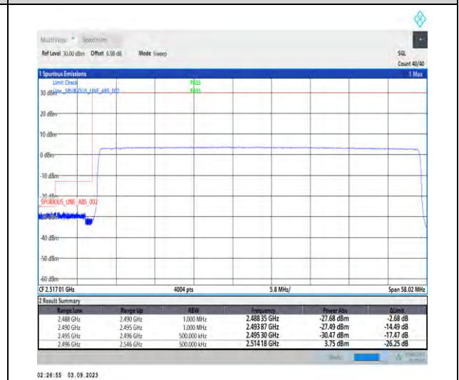
1-N41-PC2-30-50-L-6-CP-QPSK-Outer_Full-133@0-Ant3-1--PASS-see graph
