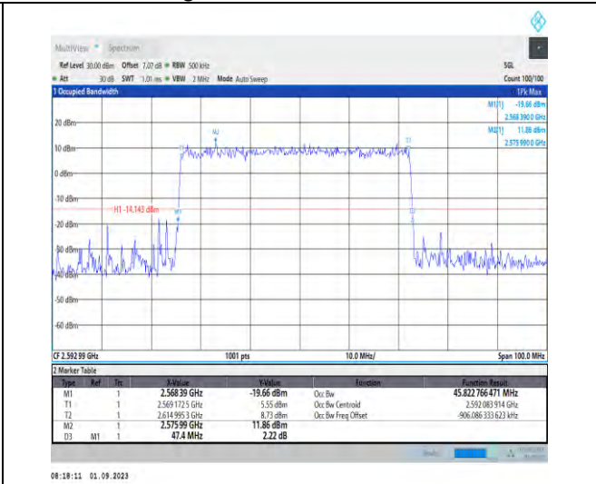
1-N41-PC2-30-50-M-5-DFT-256QAM-Outer_Full-128 @0-Ant3-45.823-47.400-≤50-PASS
