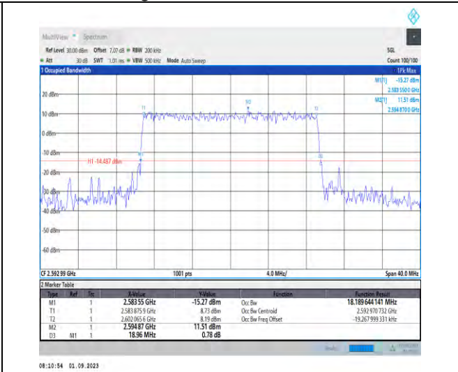
1-N41-PC2-30-20-M-8-CP-64QAM-Outer_Full-51@0 -Ant3-18.19-18.960-≤20-PASS
