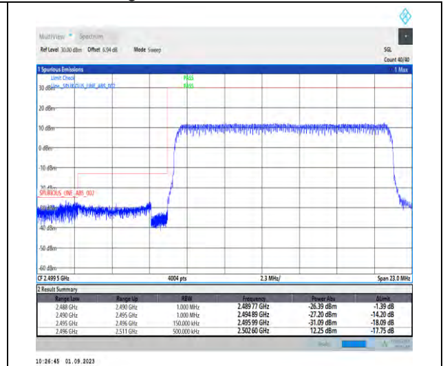
1-N41-PC2-30-15-L-3-DFT-PI2BPSK-Outer_Full-36@0-Ant3-1--PASS-see graph
