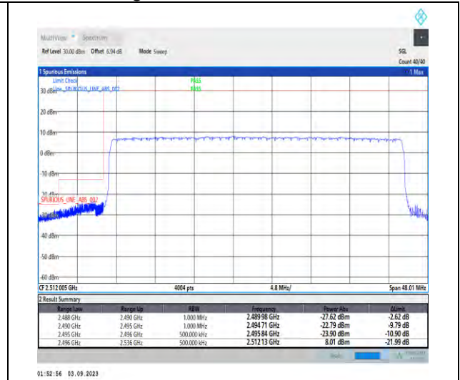
1-N41-PC2-30-40-L-3-DFT-PI2BPSK-Outer_Full-100@0-Ant3-1--PASS-see graph
