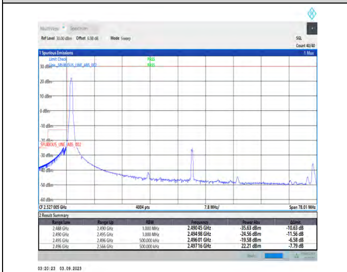
1-N41-PC2-30-70-L-4-CP-QPSK-Edge_1RB_Left-1@0-Ant3-1--PASS-see graph
