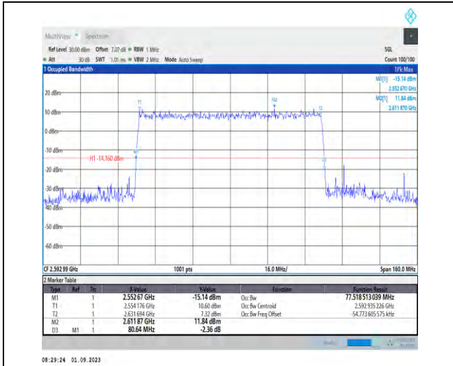
1-N41-PC2-30-80-M-9-CP-256QAM-Outer_Full-217 @0-Ant3-77.519-80.640-≤80-PASS
