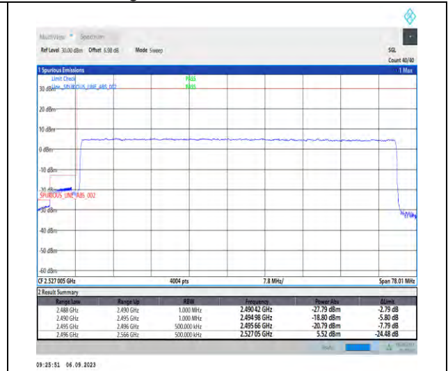
1-N41-PC2-30-70-L-3-DFT-PI2BPSK-Outer_Full-180@0-Ant3-1--PASS-see graph
