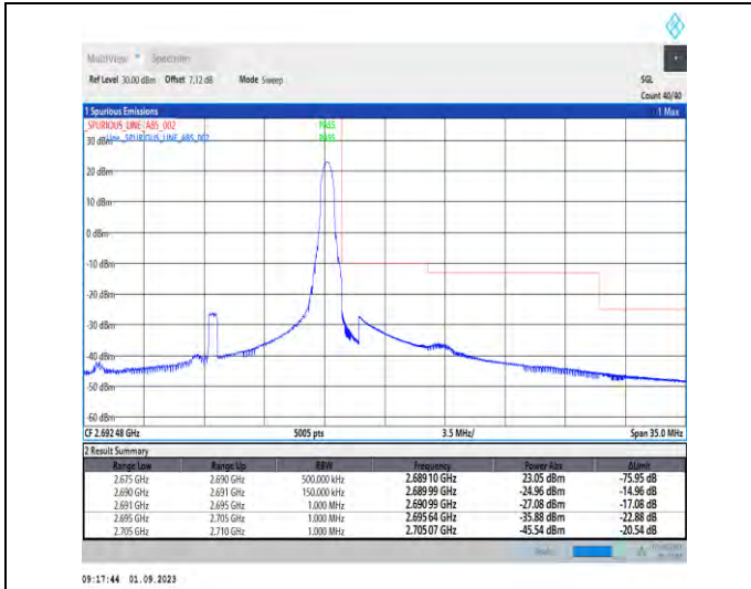
1-N41-PC2-30-15-H-2-DFT-PI2BPSK-Edge_1RB_Righ t-1@37-Ant3-1--PASS-see graph
