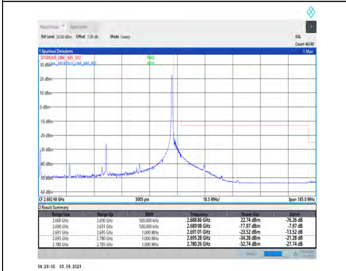
1-N41-PC2-30-90-H-5-CP-QPSK-Edge_1RB_Right-1 @244-Ant3-1--PASS-see graph
