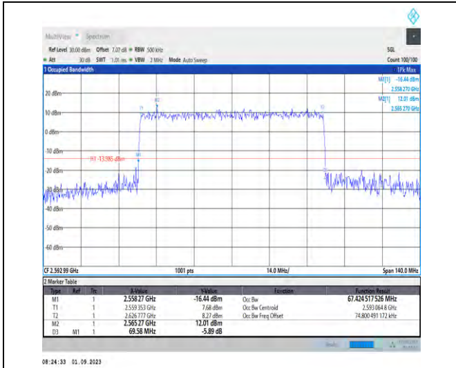
1-N41-PC2-30-70-M-6-CP-QPSK-Outer_Full-189@0 -Ant3-67.425-69.580-≤70-PASS
