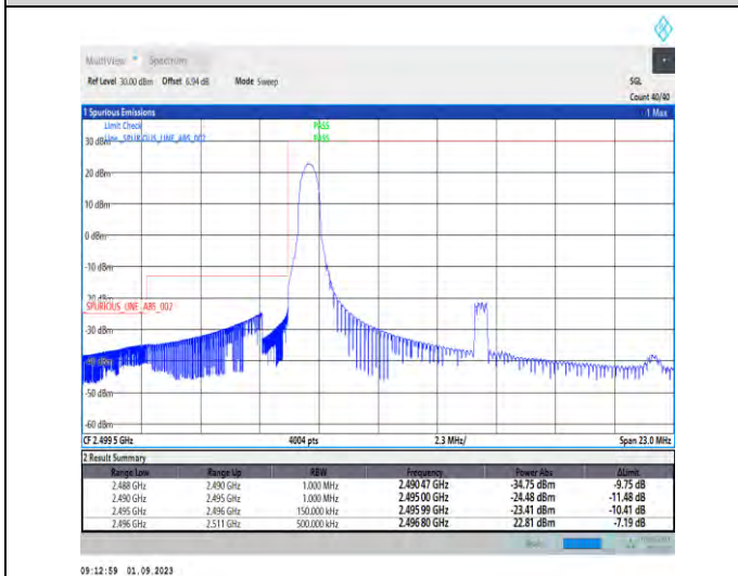
1-N41-PC2-30-15-L-4-CP-QPSK-Edge_1RB_Left-1@0-Ant3-1--PASS-see graph
