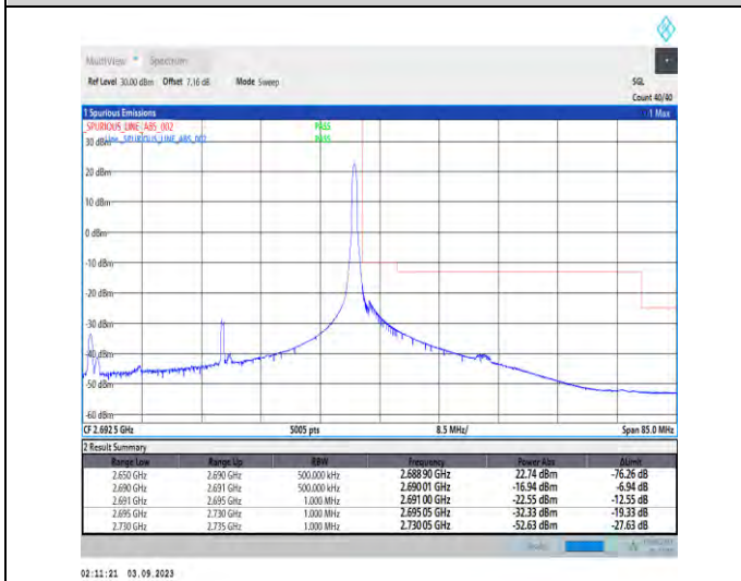
1-N41-PC2-30-40-H-5-CP-QPSK-Edge_1RB_Right-1 @105-Ant3-1--PASS-see graph
