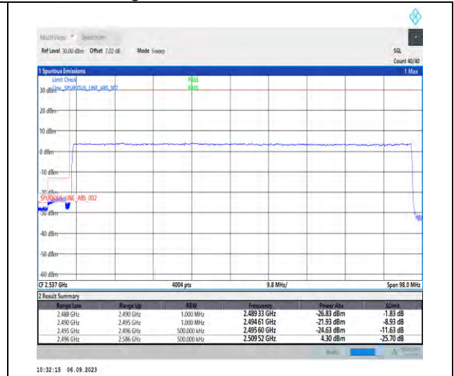
1-N41-PC2-30-90-L-3-DFT-PI2BPSK-Outer_Full-240@0-Ant3-1--PASS-see graph
