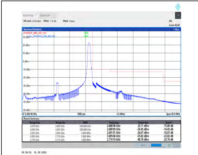
1-N41-PC2-30-20-H-2-DFT-PI2BPSK-Edge_1RB_Righ t-1@50-Ant3-1--PASS-see graph
