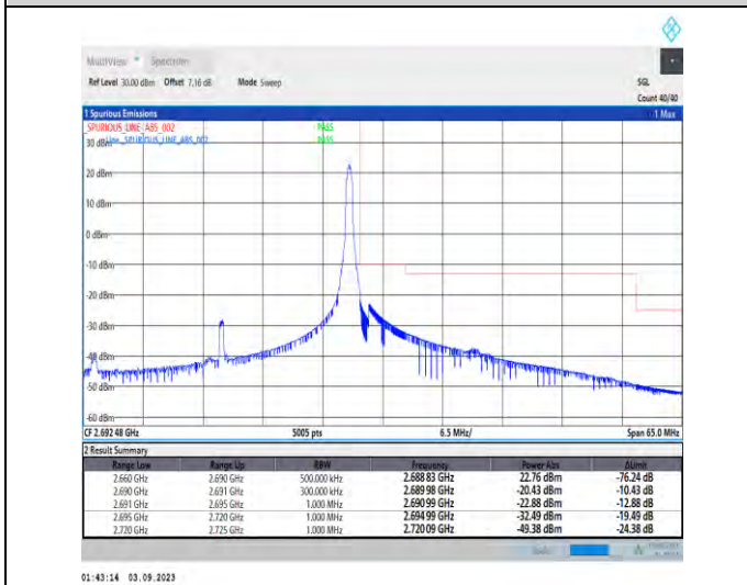
1-N41-PC2-30-30-H-5-CP-QPSK-Edge_1RB_Right-1 @77-Ant3-1--PASS-see graph
