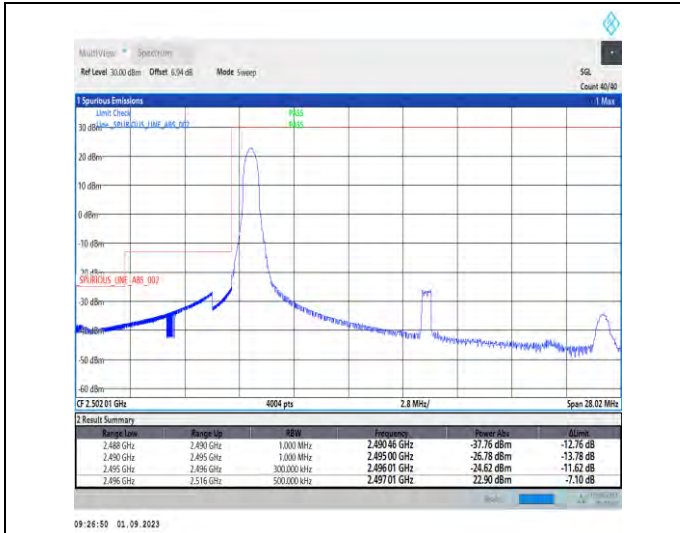
1-N41-PC2-30-20-L-1-DFT-PI2BPSK-Edge_1RB_Left-1@0-Ant3-1--PASS-see graph
