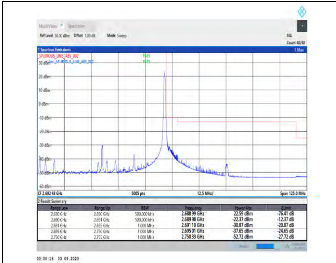
1-N41-PC2-30-60-H-2-DFT-PI2BPSK-Edge_1RB_Righ t-1@161-Ant3-1--PASS-see graph
