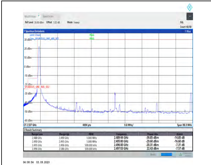
1-N41-PC2-30-90-L-1-DFT-PI2BPSK-Edge_1RB_Left-1@0-Ant3-1--PASS-see graph
