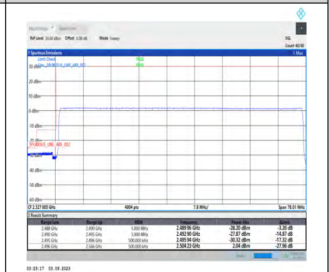
1-N41-PC2-30-70-L-6-CP-QPSK-Outer_Full-189@0-Ant3-1--PASS-see graph
