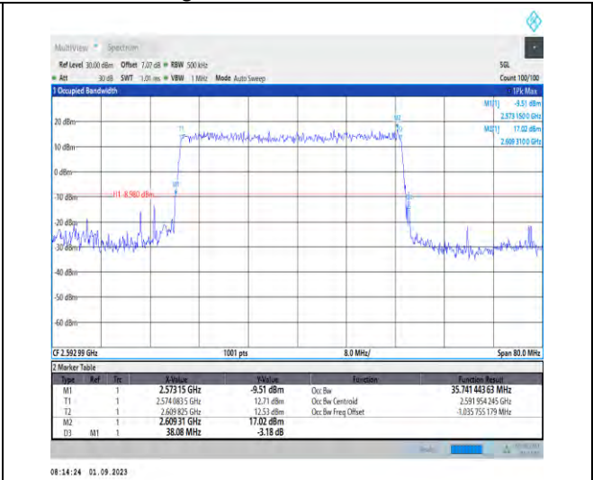
1-N41-PC2-30-40-M-2-DFT-PI2BPSK-Outer_Full-100@ 0-Ant3-35.741-38.080-≤40-PASS
