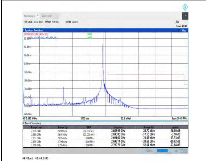
1-N41-PC2-30-100-H-5-CP-QPSK-Edge_1RB_Right-1 @272-Ant3-1--PASS-see graph
