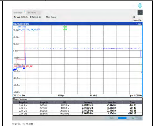
1-N41-PC2-30-80-L-3-DFT-PI2BPSK-Outer_Full-216@0-Ant3-1--PASS-see graph
