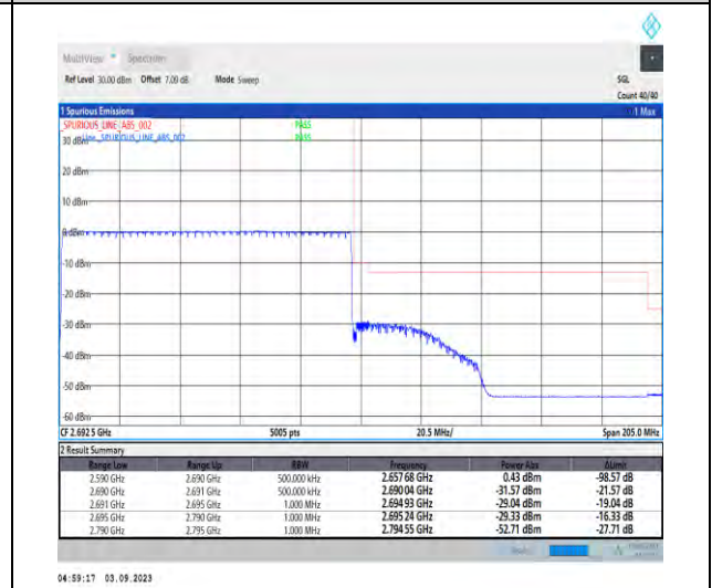
1-N41-PC2-30-100-H-6-CP-QPSK-Outer_Full-273 @0-Ant3-1--PASS-see graph
