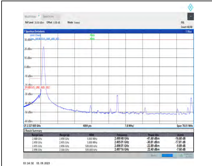
1-N41-PC2-30-70-L-1-DFT-PI2BPSK-Edge_1RB_Left-1@0-Ant3-1--PASS-see graph
