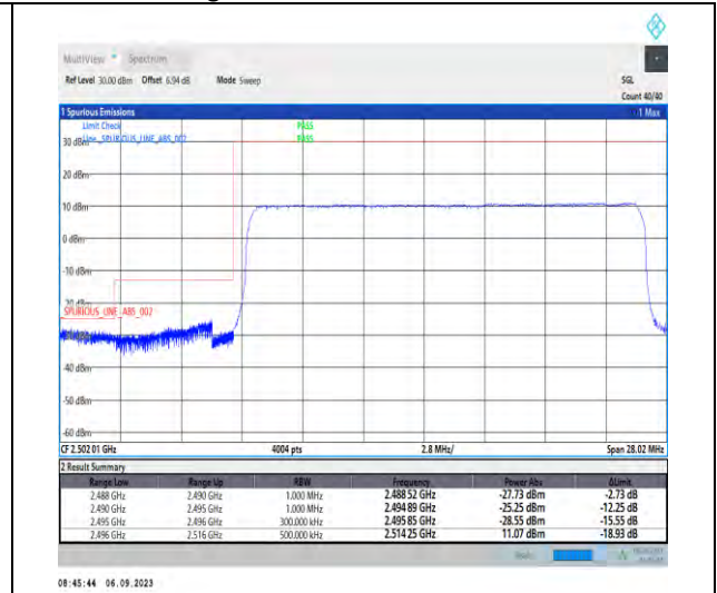
1-N41-PC2-30-20-L-3-DFT-PI2BPSK-Outer_Full-50@0-Ant3-1--PASS-see graph
