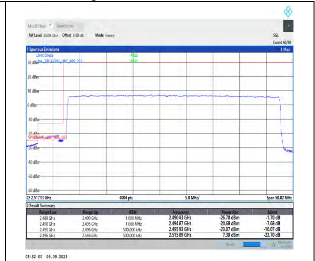
1-N41-PC2-30-50-L-3-DFT-PI2BPSK-Outer_Full-128@0-Ant3-1--PASS-see graph
