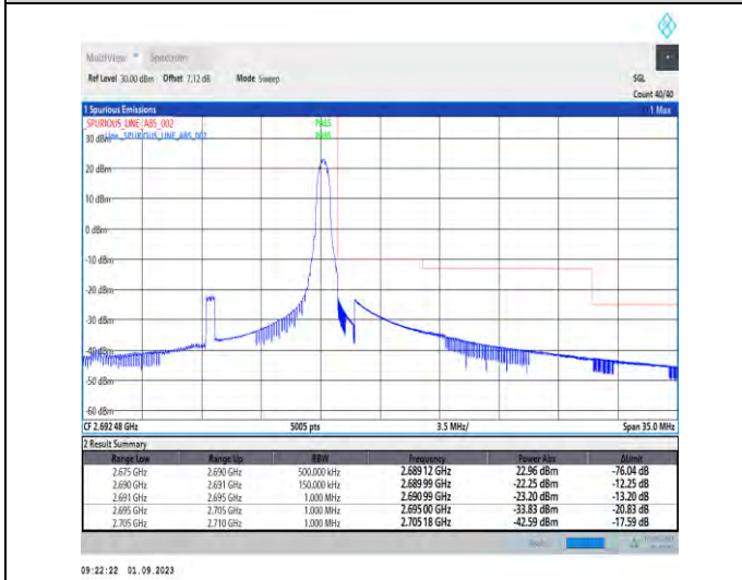
1-N41-PC2-30-15-H-5-CP-QPSK-Edge_1RB_Right-1 @37-Ant3-1--PASS-see graph
