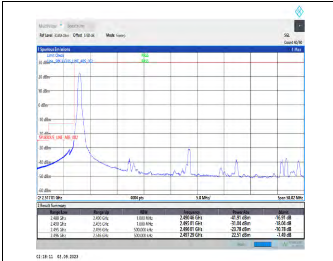
1-N41-PC2-30-50-L-1-DFT-PI2BPSK-Edge_1RB_Left-1@0-Ant3-1--PASS-see graph
