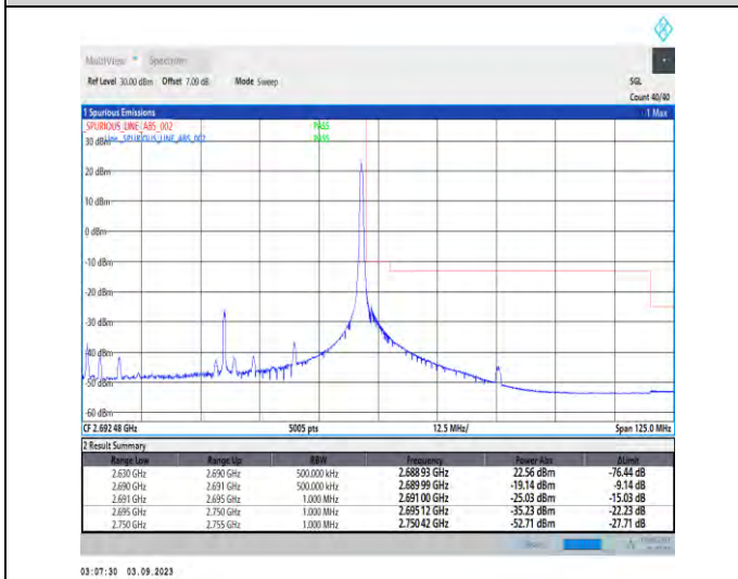
1-N41-PC2-30-60-H-5-CP-QPSK-Edge_1RB_Right-1 @161-Ant3-1--PASS-see graph
