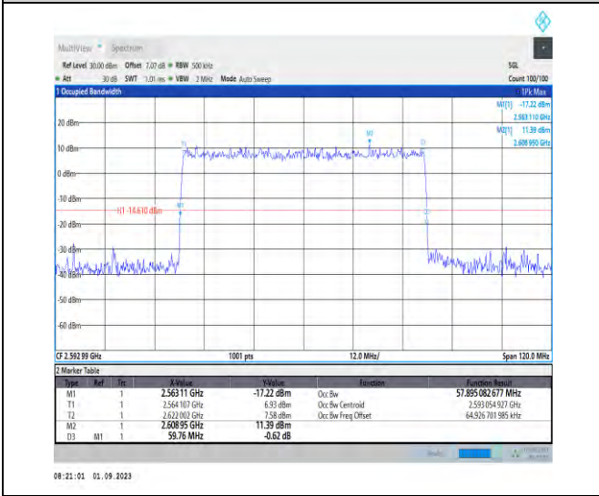
1-N41-PC2-30-60-M-5-DFT-256QAM-Outer_Full-162 @0-Ant3-57.895-59.760-≤60-PASS
