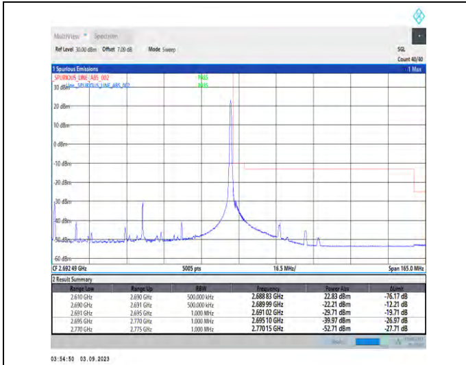
1-N41-PC2-30-80-H-2-DFT-PI2BPSK-Edge_1RB_Righ t-1@216-Ant3-1--PASS-see graph
