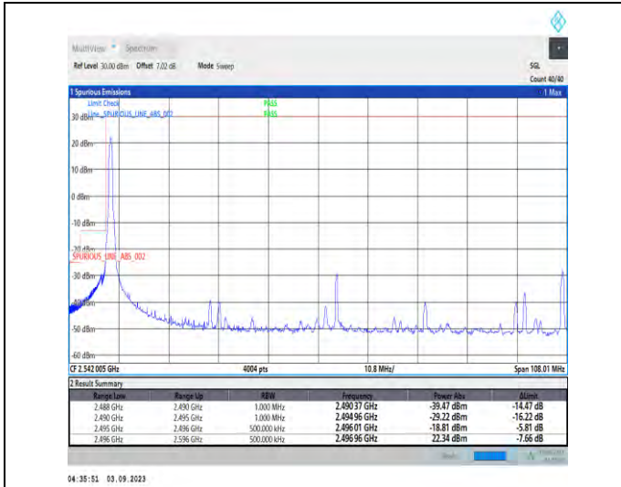
1-N41-PC2-30-100-L-1-DFT-PI2BPSK-Edge_1RB_Left-1@0-Ant3-1--PASS-see graph
