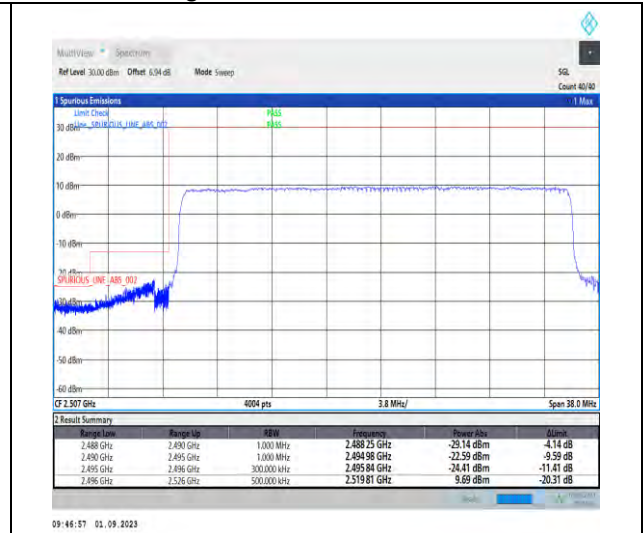
1-N41-PC2-30-30-L-3-DFT-PI2BPSK-Outer_Full-75@0-Ant3-1--PASS-see graph
