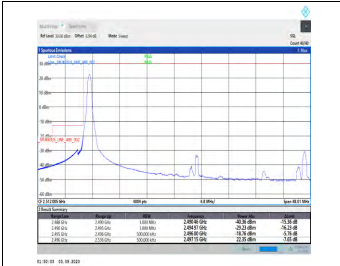
1-N41-PC2-30-40-L-1-DFT-PI2BPSK-Edge_1RB_Left-1@0-Ant3-1--PASS-see graph
