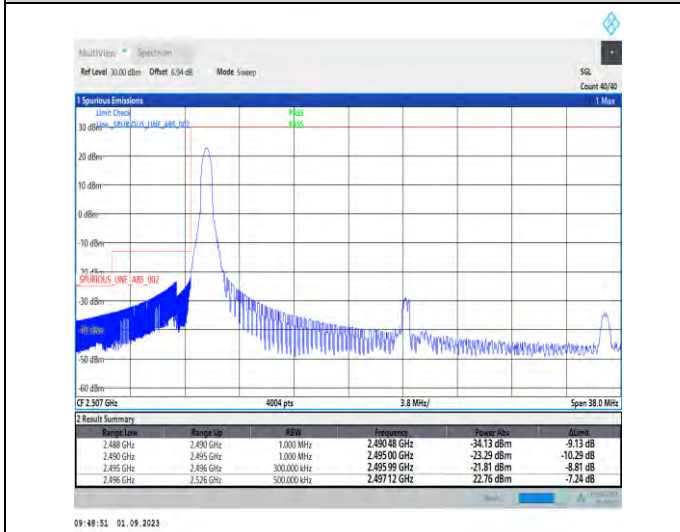
1-N41-PC2-30-30-L-4-CP-QPSK-Edge_1RB_Left-1@0-Ant3-1--PASS-see graph
