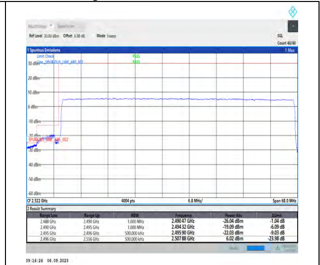
1-N41-PC2-30-60-L-3-DFT-PI2BPSK-Outer_Full-162@0-Ant3-1--PASS-see graph
