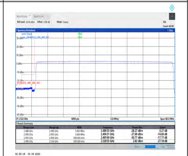
1-N41-PC2-30-60-L-6-CP-QPSK-Outer_Full-162@0-Ant3-1--PASS-see graph
