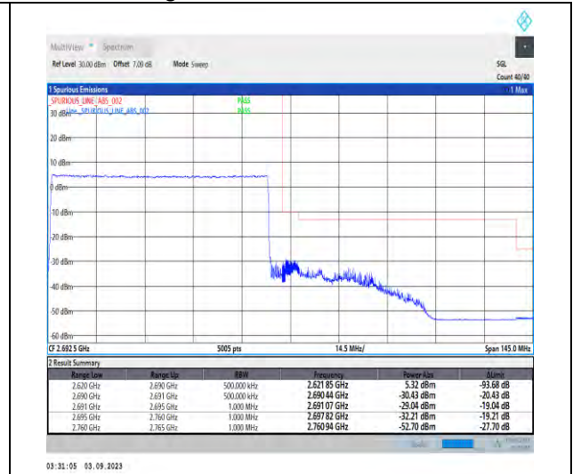
1-N41-PC2-30-70-H-3-DFT-PI2BPSK-Outer_Full-1 80@0-Ant3-1--PASS-see graph
