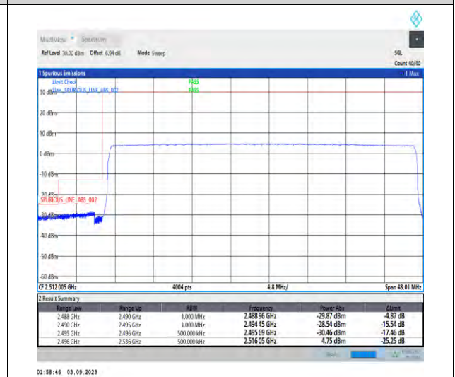
1-N41-PC2-30-40-L-6-CP-QPSK-Outer_Full-106@0-Ant3-1--PASS-see graph
