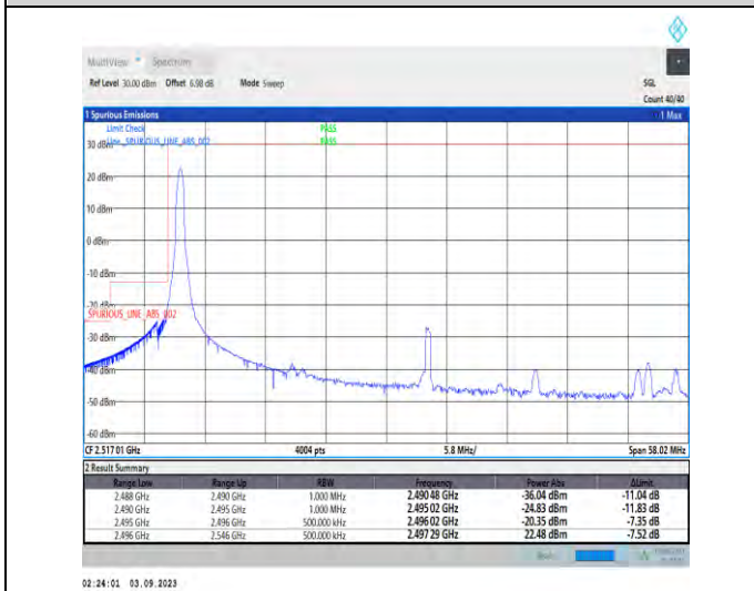
1-N41-PC2-30-50-L-4-CP-QPSK-Edge_1RB_Left-1@0-Ant3-1--PASS-see graph
