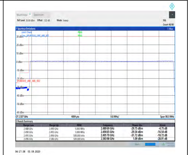
1-N41-PC2-30-90-L-6-CP-QPSK-Outer_Full-245@0-Ant3-1--PASS-see graph
