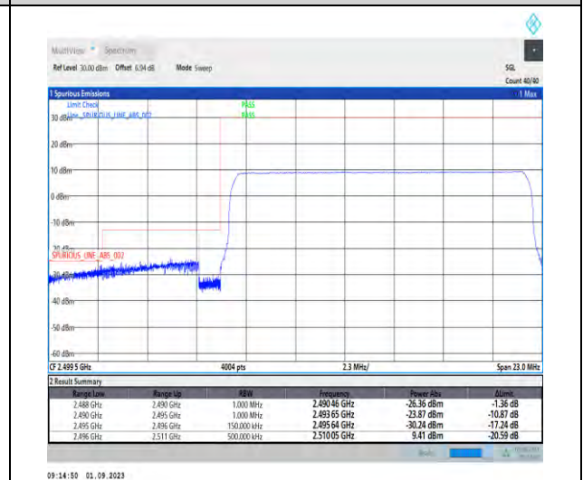
1-N41-PC2-30-15-L-6-CP-QPSK-Outer_Full-38@0-Ant3-1--PASS-see graph
