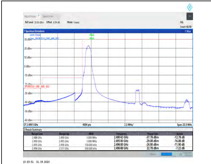
1-N41-PC2-30-15-L-1-DFT-PI2BPSK-Edge_1RB_Left-1@0-Ant3-1--PASS-see graph
