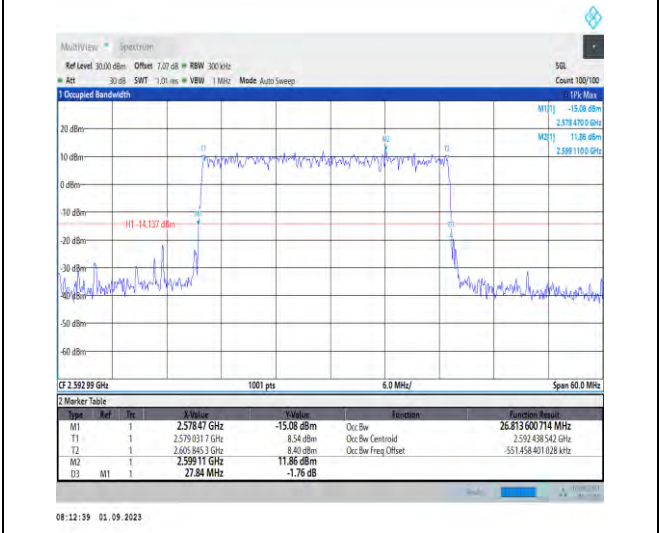
1-N41-PC2-30-30-M-5-DFT-256QAM-Outer_Full-75 @0-Ant3-26.814-27.840-≤30-PASS
