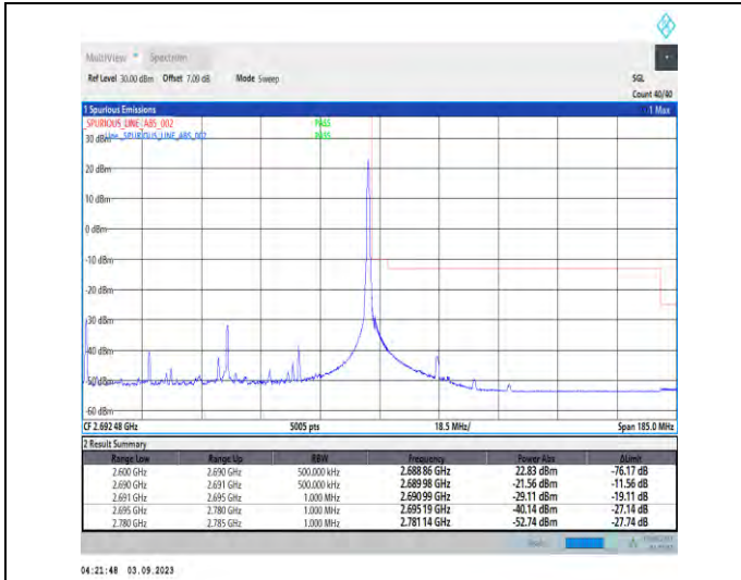
1-N41-PC2-30-90-H-2-DFT-PI2BPSK-Edge_1RB_Righ t-1@244-Ant3-1--PASS-see graph
