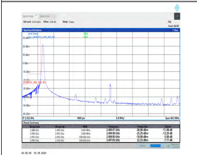
1-N41-PC2-30-60-L-4-CP-QPSK-Edge_1RB_Left-1@0-Ant3-1--PASS-see graph
