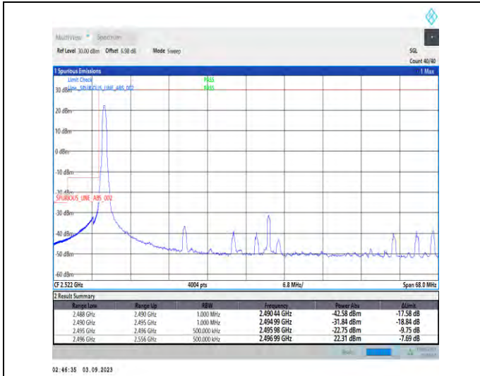
1-N41-PC2-30-60-L-1-DFT-PI2BPSK-Edge_1RB_Left-1@0-Ant3-1--PASS-see graph
