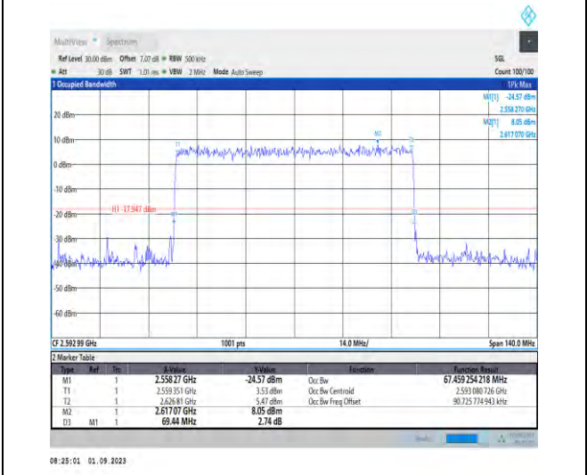
1-N41-PC2-30-70-M-9-CP-256QAM-Outer_Full-189@0 -Ant3-67.459-69.440-≤70-PASS
