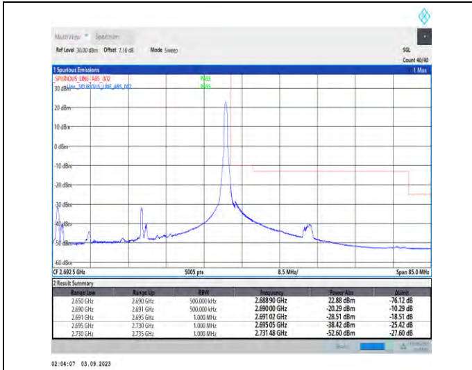
1-N41-PC2-30-40-H-2-DFT-PI2BPSK-Edge_1RB_Righ t-1@105-Ant3-1--PASS-see graph
