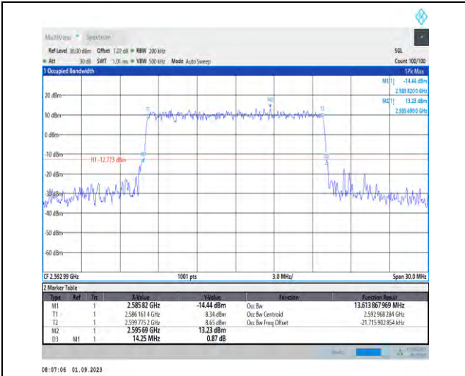
1-N41-PC2-30-15-M-8-CP-64QAM-Outer_Full-38@0 -Ant3-13.614-14.250-<=15-PASS
