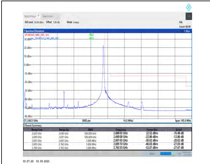
1-N41-PC2-30-70-H-2-DFT-PI2BPSK-Edge_1RB_Righ t-1@188-Ant3-1--PASS-see graph
