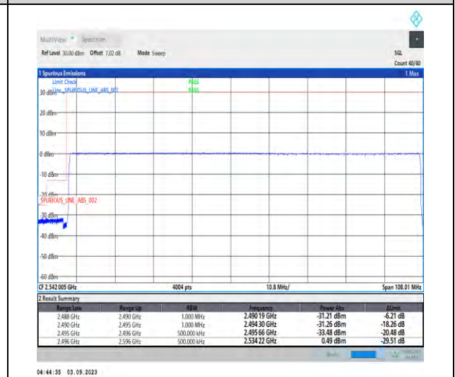
1-N41-PC2-30-100-L-6-CP-QPSK-Outer_Full-273@0-Ant3-1--PASS-see graph
