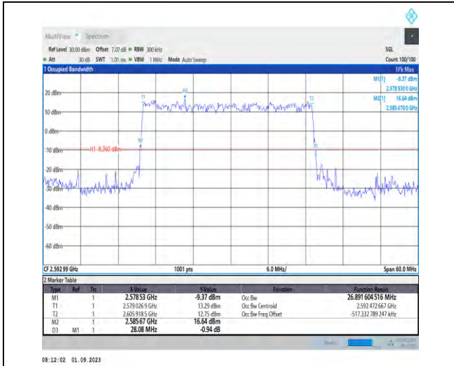
1-N41-PC2-30-30-M-2-DFT-PI2BPSK-Outer_Full-75 @0-Ant3-26.892-28.080-≤30-PASS
