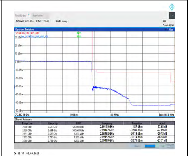
1-N41-PC2-30-90-H-6-CP-QPSK-Outer_Full-245 @0-Ant3-1--PASS-see graph
