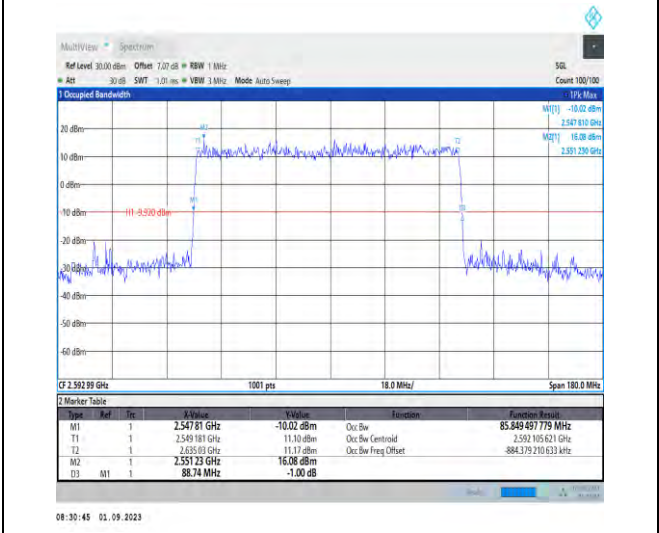
1-N41-PC2-30-90-M-3-DFT-16QAM-Outer_Full-240 @0-Ant3-85.849-88.740-≤90-PASS
