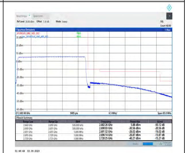
1-N41-PC2-30-30-H-6-CP-QPSK-Outer_Full-78@ 0-Ant3-1--PASS-see graph
