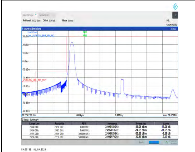
1-N41-PC2-30-20-L-4-CP-QPSK-Edge_1RB_Left-1@0-Ant3-1--PASS-see graph
