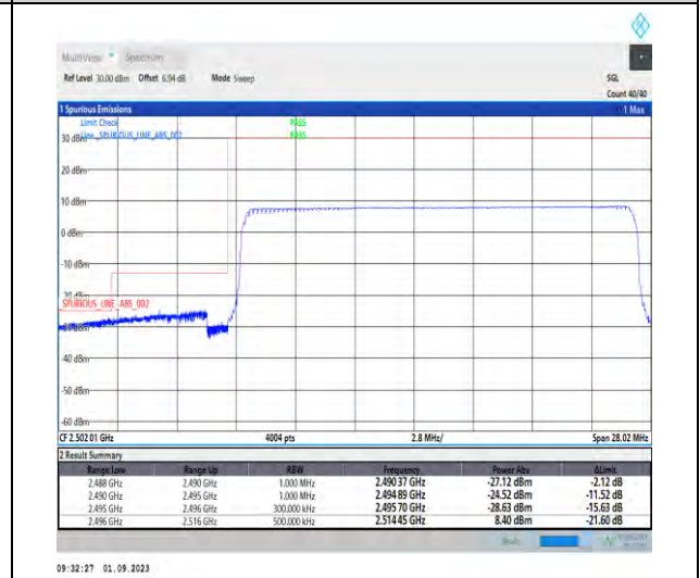
1-N41-PC2-30-20-L-6-CP-QPSK-Outer_Full-51@0-Ant3-1--PASS-see graph
