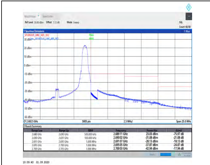
1-N41-PC2-30-10-H-2-DFT-PI2BPSK-Edge_1RB_Righ t-1@23-Ant3-1--PASS-see graph
