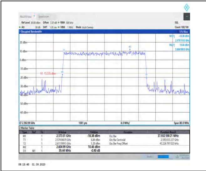
1-N41-PC2-30-40-M-9-CP-256QAM-Outer_Full-106 @0-Ant3-37.933-39.440-≤40-PASS
