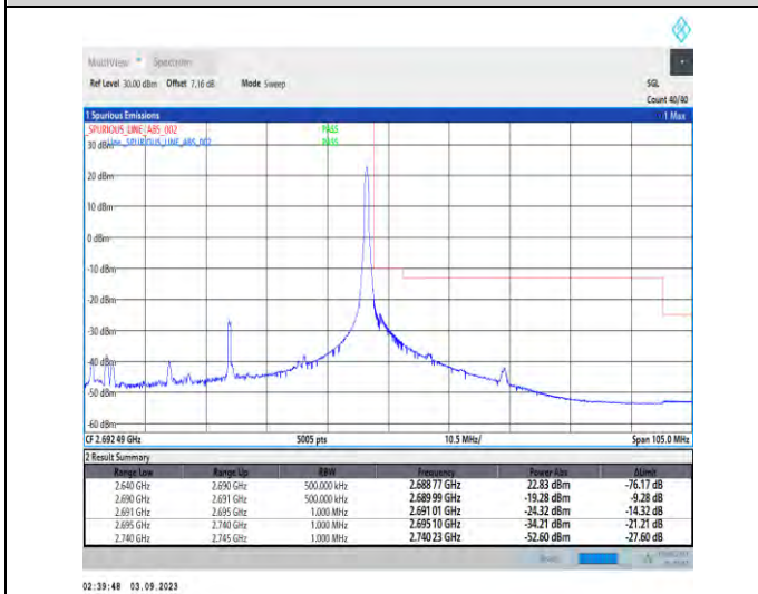
1-N41-PC2-30-50-H-5-CP-QPSK-Edge_1RB_Right-1 @132-Ant3-1--PASS-see graph
