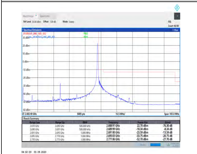
1-N41-PC2-30-80-H-5-CP-QPSK-Edge_1RB_Right-1 @216-Ant3-1--PASS-see graph
