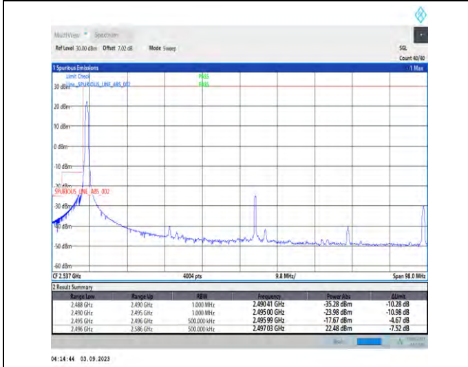
1-N41-PC2-30-90-L-4-CP-QPSK-Edge_1RB_Left-1@0-Ant3-1--PASS-see graph
