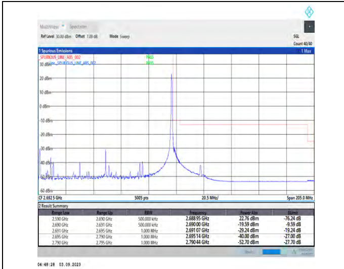
1-N41-PC2-30-100-H-2-DFT-PI2BPSK-Edge_1RB_Rig ht-1@272-Ant3-1--PASS-see graph
