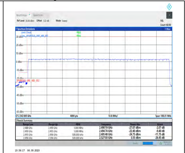
1-N41-PC2-30-100-L-3-DFT-PI2BPSK-Outer_Full-270@0-Ant3-1--PASS-see graph
