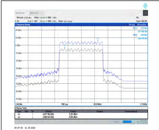
1-N41-PC2-30-100-H-1-DFT-256QAM-Outer_Full-27 0@0-Ant3-9.19-100%-0.00-9.19-PASS-≤13
