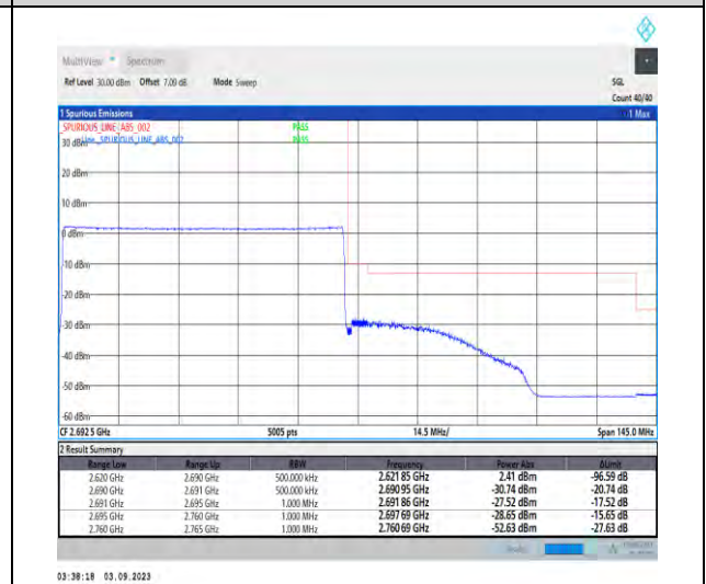
1-N41-PC2-30-70-H-6-CP-QPSK-Outer_Full-189 @0-Ant3-1--PASS-see graph
