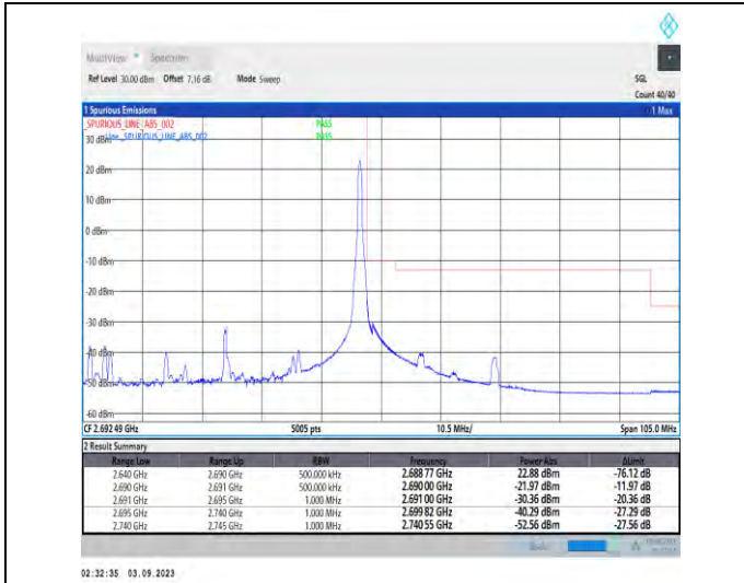
1-N41-PC2-30-50-H-2-DFT-PI2BPSK-Edge_1RB_Righ t-1@132-Ant3-1--PASS-see graph
