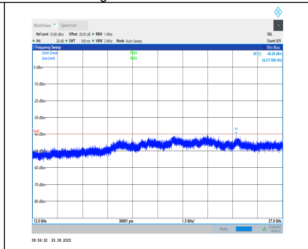
1-N30-PC3-15-10-L-1-DFT-PI2BPSK-Inner_1RB_Left -1@1-12000-27000-Ant3-20492.50--40.28--40-PASS
