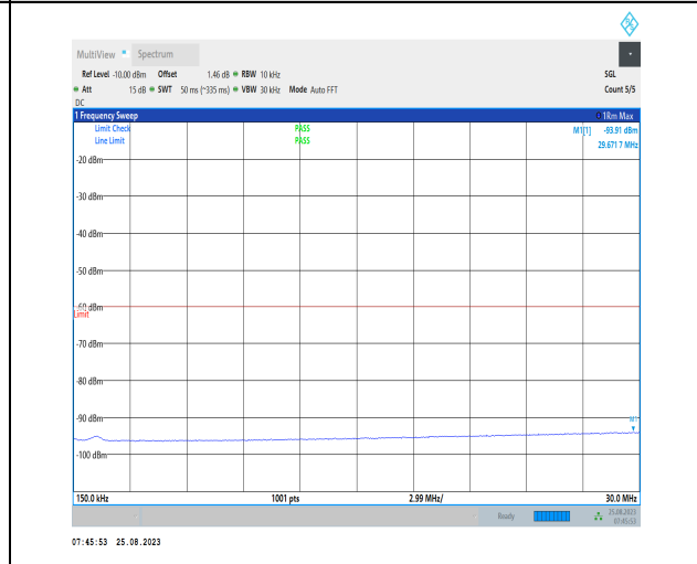
1-N30-PC3-15-10-M-1-DFT-PI2BPSK-Inner_1RB_Lef t-1@1-0.15-30-Ant3-29.67--93.91--60-PASS
