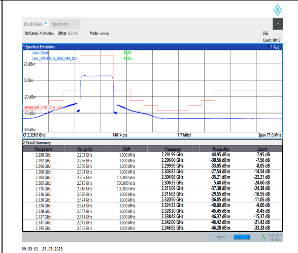
1-N30-PC3-15-10-L-6-CP-QPSK-Outer_Full-52@0-Ant3-1--PASS-see graph
