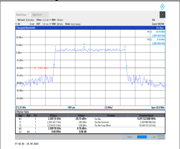
1-N30-PC3-15-10-M-9-CP-256QAM-Outer_Full-52@0-Ant3-9.292-9.680-≤10-PASS
