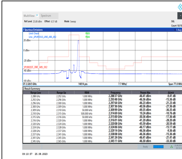
1-N30-PC3-15-5-H-2-DFT-P12BPSK-Edge_1RB_Right-1@24-Ant3-1--PASS-see graph
