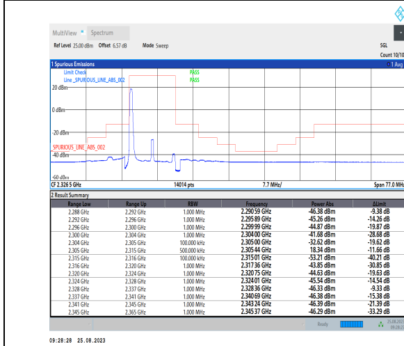
1-N30-PC3-15-10-L-4-CP-QPSK-Edge_1RB_Left-1@0-Ant3-1--PASS-see graph
