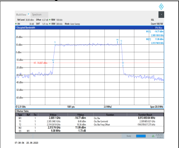
1-N30-PC3-15-10-M-1-DFT-QPSK-Outer_Full-50@0 -Ant3-8.913-9.380-<=10-PASS
