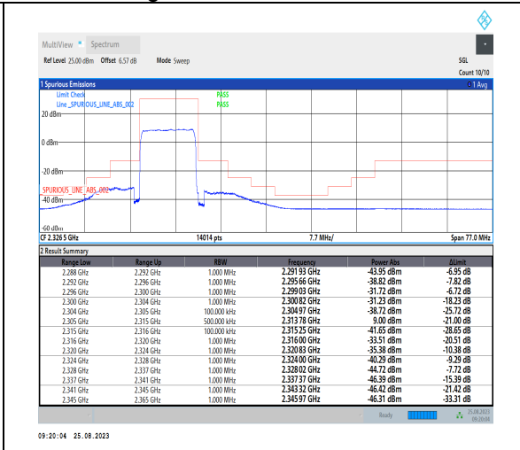
1-N30-PC3-15-10-L-3-DFT-PI2BPSK-Outer_Full-50@0-Ant3-1--PASS-see graph
