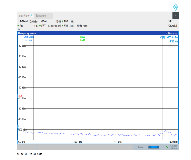
1-N30-PC3-15-10-H-1-DFT-PI2BPSK-Inner_1RB_L eft-1@1-0.009-0.15-Ant3-0.14--100.50--70-PASS
