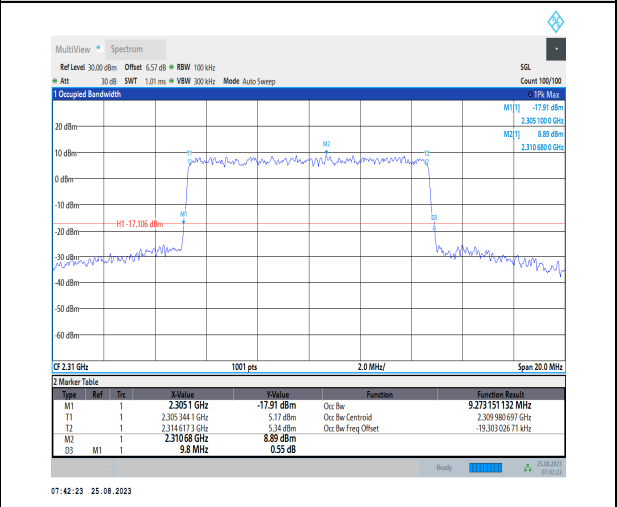
1-N30-PC3-15-10-M-7-CP-16QAM-Outer_Full-52@0 -Ant3-9.273-9.800-≤10-PASS
