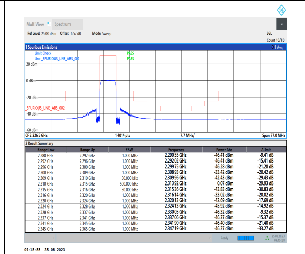
1-N30-PC3-15-5-H-6-CP-QPSK-Outer_Full-25@0-Ant3-1--PASS-see graph
