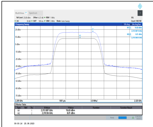
1-N30-PC3-15-10-H-1-DFT-256QAM-Outer_Full-50 @0-Ant3-8.62-100%-0.00-8.62-PASS-≤13
