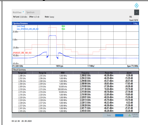
1-N30-PC3-15-5-H-3-DFT-P12BPSK-Outer_Full-25@0-Ant3-1--PASS-see graph
