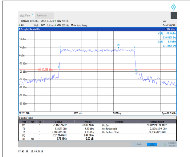
1-N30-PC3-15-10-M-8-CP-64QAM-Outer_Full-52@0 -Ant3-9.308-9.760-≤10-PASS
