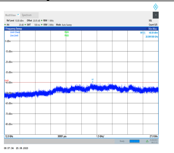
1-N30-PC3-15-10-H-1-DFT-PI2BPSK-Inner_1RB_Lef t-t1@1-12000-27000-Ant3-20462.00--40.59--40-PASS
