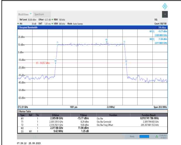
1-N30-PC3-15-10-M-2-DFT-PI2BPSK-Outer_Full-50 @0-Ant3-8.911-9.420-<=10-PASS
