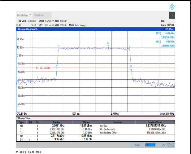
1-N30-PC3-15-10-M-3-DFT-16QAM-Outer_Full-50@0 0-Ant3-8.928-9.360-<=10-PASS
