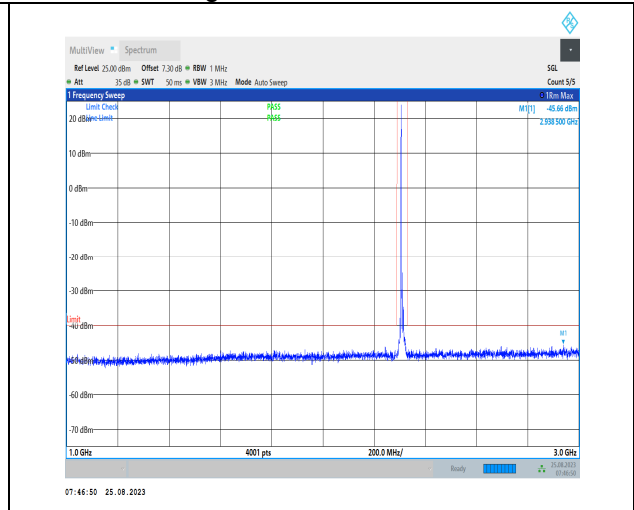
1-N30-PC3-15-10-M-1-DFT-PI2BPSK-Inner_1RB_Lef t-1@1-1000-3000-Ant3-2938.50--45.66--40-PASS
