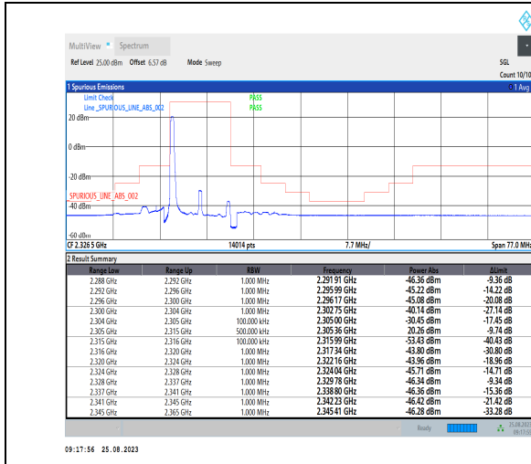
1-N30-PC3-15-10-L-1-DFT-PI2BPSK-Edge_1RB_Left-1@0-Ant3-1--PASS-see graph
