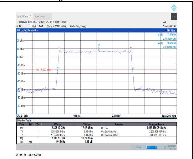
1-N30-PC3-15-10-M-5-DFT-256QAM-Outer_Full-50 @0-Ant3-8.944-9.400-≤10-PASS
