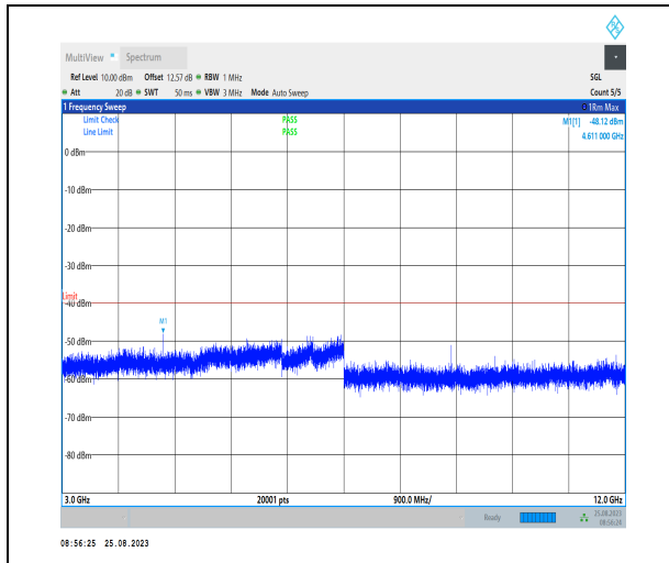
1-N30-PC3-15-10-L-1-DFT-PI2BPSK-Inner_1RB_Lef ft-1@1-3000-12000-Ant3-4611.00--48.12--40-PASS
