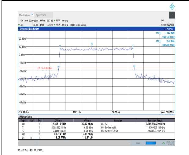
1-N30-PC3-15-10-M-6-CP-QPSK-Outer_Full-52@0- Ant3-9.286-9.680-≤10-PASS
