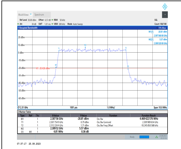
1-N30-PC3-15-5-M-9-CP-256QAM-Outer_Full-25@0 -Ant3-4.469-4.810-<=5-PASS
