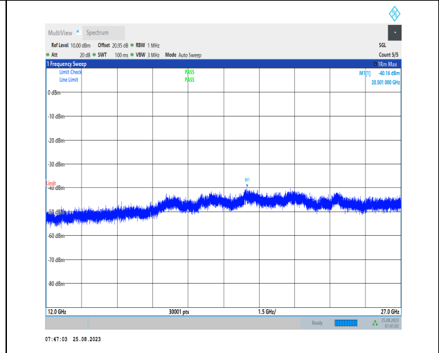
1-N30-PC3-15-10-M-1-DFT-PI2BPSK-Inner_1RB_Lef t-1@1-12000-27000-Ant3-20501.00--40.16--40-PASS
