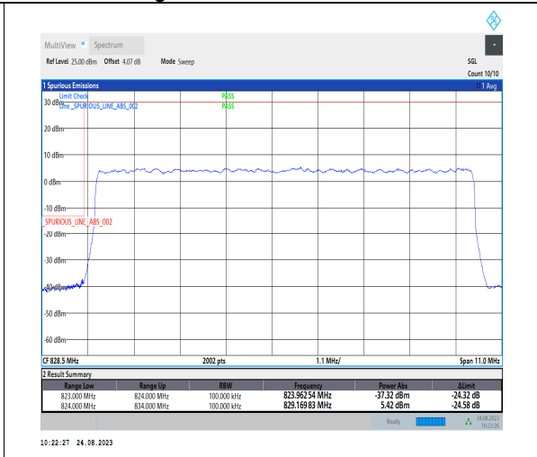
1-N26-824-849-PC3-15-10-L-3-DFT-PI2BPSK-Out er_Full-50@0-Ant1-1-seegraph-PASS-see graph
