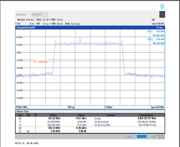
1-N26-824-849-PC3-15-10-M-1-DFT-QPSK-Outer_F ull-50@0-Ant1-8.904-9.340-<10-PASS
