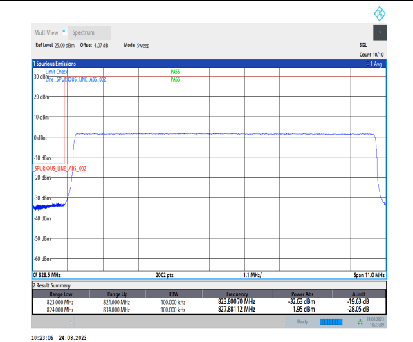
1-N26-824-849-PC3-15-10-L-6-CP-QPSK-Outer_F ull-52@0-Ant1-1-seegraph-PASS-see graph
