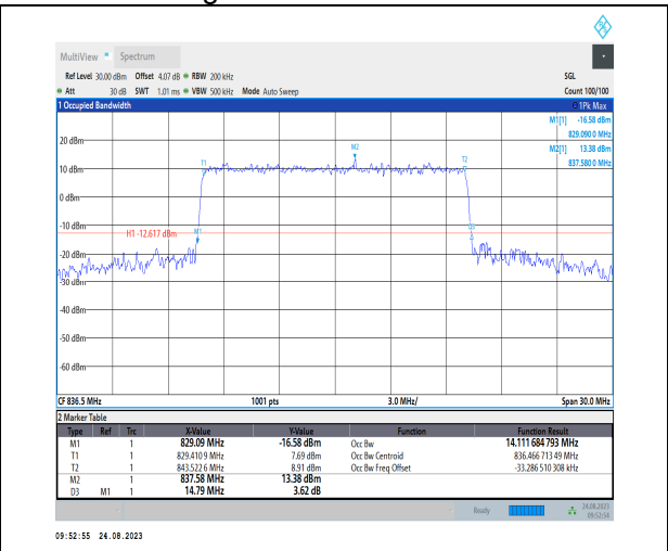
1-N26-824-849-PC3-15-15-M-8-CP-64QAM-Outer_Full-79@0-Ant1-14.112-14.790-≤15-PASS
