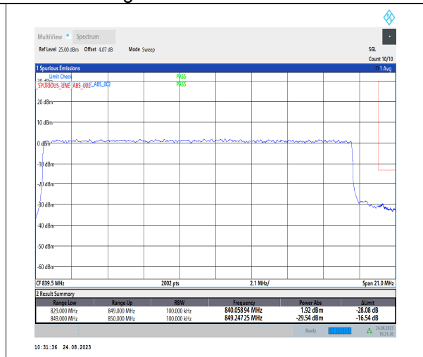
1-N26-824-849-PC3-15-20-H-3-DFT-PI2BPSK-Outer_Full-100@0-Ant1-1-seegraph-PASS-see graph
