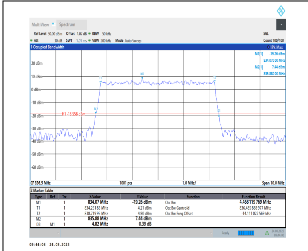
1-N26-824-849-PC3-15-5-M-9-CP-256QAM-Outer_F ull-25@0-Ant1-4.468-4.820-<5-PASS
