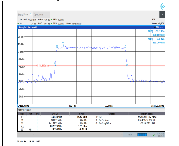
1-N26-824-849-PC3-15-10-M-9-CP-256QAM-Outer_Full-52@0-Ant1-9.253-9.760-≤10-PASS
