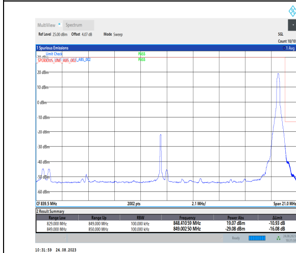
1-N26-824-849-PC3-15-20-H-5-CP-QPSK-Edge_1RB_Right-1@105-Ant1-1-seegraph-PASS-see graph
