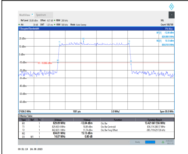
1-N26-824-849-PC3-15-15-M-1-DFT-QPSK-Outer_Full-75@0-Ant1-13.422-14.070-≤15-PASS
