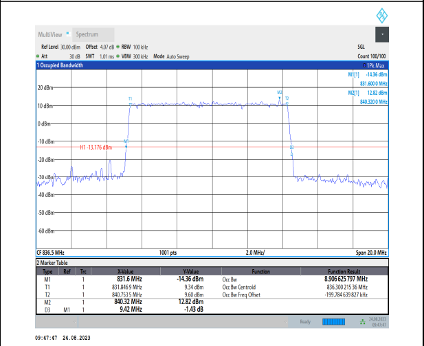
1-N26-824-849-PC3-15-10-M-3-DFT-16QAM-Outer_F ull-50@0-Ant1-8.907-9.420-<10-PASS
