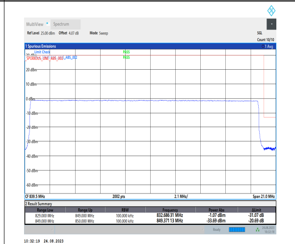
1-N26-824-849-PC3-15-20-H-6-CP-QPSK-Outer_Full-106@0-Ant1-1-seegraph-PASS-see graph
