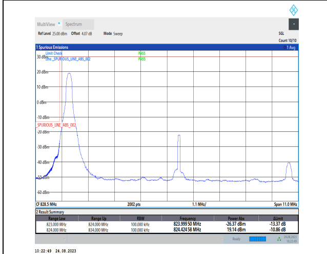
1-N26-824-849-PC3-15-10-L-4-CP-QPSK-Edge_1RB_Left-1@0-Ant1-1-seegraph-PASS-see graph
