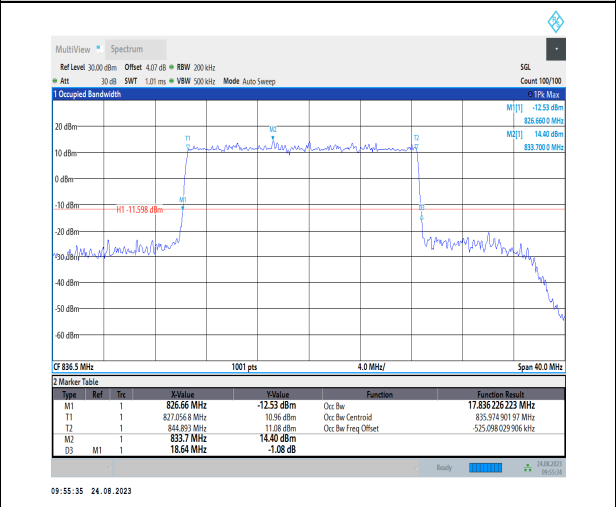
1-N26-824-849-PC3-15-20-M-1-DFT-QPSK-Outer_Full-100@0-Ant1-17.836-18.640-≤20-PASS
