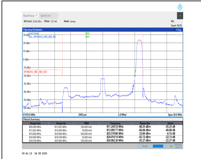
1-N26-814-824-PC3-15-10-H-2-DFT-PI2BPSK-Edge_1 RB_Right-1@51-Ant1-1--PASS-see graph
