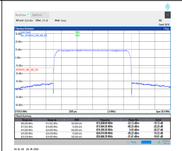
1-N26-814-824-PC3-15-10-H-6-CP-QPSK-Outer_Full-52@0-Ant1-1--PASS-see graph
