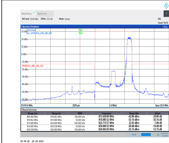
1-N26-814-824-PC3-15-5-H-5-CP-QPSK-Edge_1RB_Right-1@24-Ant1-1--PASS-see graph
