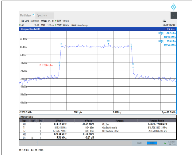
1-N26-814-824-PC3-15-10-M-4-DFT-64QAM-Outer_Full-50@0-Ant1-8.903-9.360-≤10-PASS
