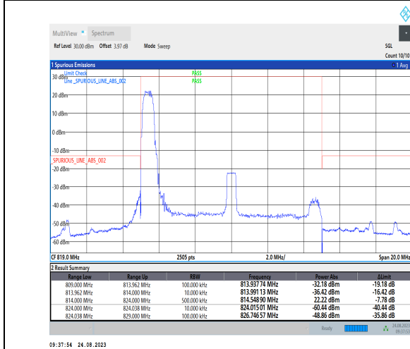
1-N26-814-824-PC3-15-10-L-4-CP-QPSK-Edge_1RB_Left-1@0-Ant1-1--PASS-see graph
