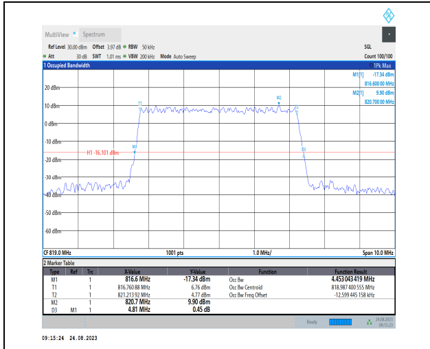
1-N26-814-824-PC3-15-5-M-9-CP-256QAM-Outer_F ull-25@0-Ant1-4.453-4.810-≤5-PASS
