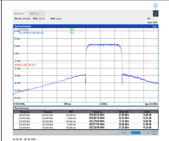
1-N26-814-824-PC3-15-5-H-6-CP-QPSK-Outer_Full-25@0-Ant1-1--PASS-see graph
