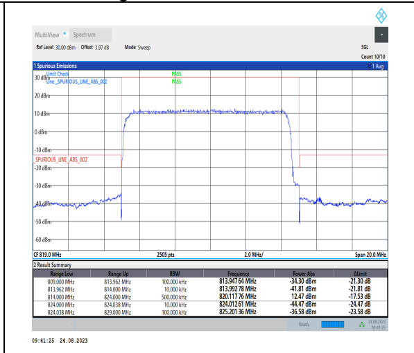
1-N26-814-824-PC3-15-10-H-3-DFT-PI2BPSK-Out_er_Full-50@0-Ant1-1--PASS-see graph
