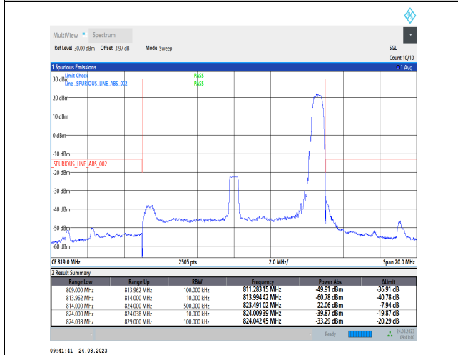
1-N26-814-824-PC3-15-10-H-5-CP-QPSK-Edge_1RB_Right-1@51-Ant1-1--PASS-see graph
