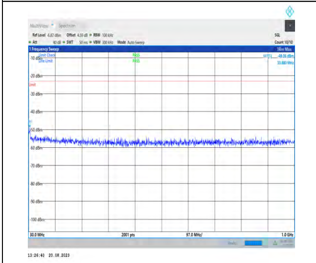
1-N25-PC3-15-40-H-1-DFT-PI2BPSK-Inner_1RB_L eft-1@1-30-1000-Ant3-33.88--49.06--23-PASS
