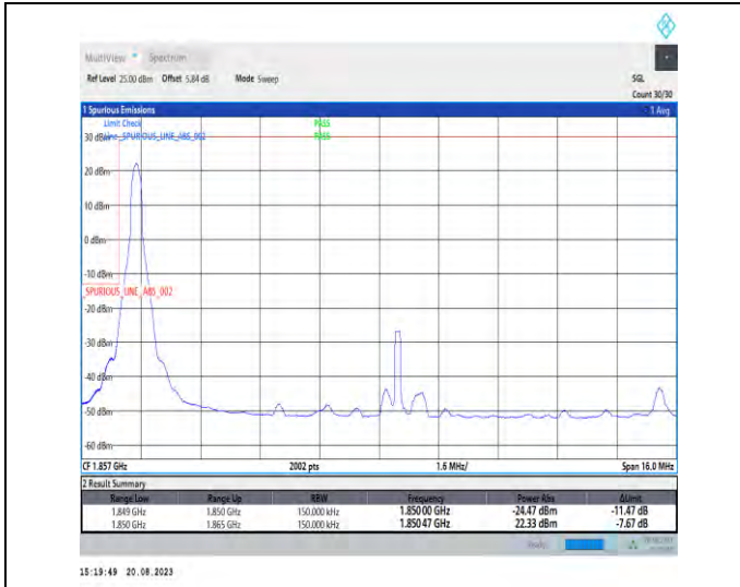
1-N25-PC3-15-15-L-1-DFT-PI2BPSK-Edge_1RB_Left-1@0-Ant3-1-seegraph-PASS-see graph
