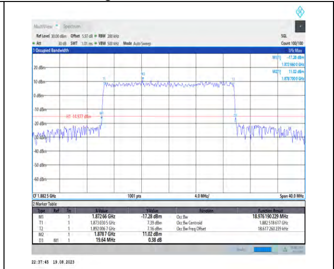
1-N25-PC3-15-20-M-7-CP-16QAM-Outer_Full-106@0 -Ant3-18.976-19.640-≤20-PASS
