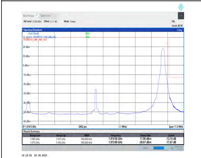
1-N25-PC3-15-10-H-5-CP-QPSK-Edge_1RB_Right-1@51-Ant3-1-seegraph-PASS-see graph
