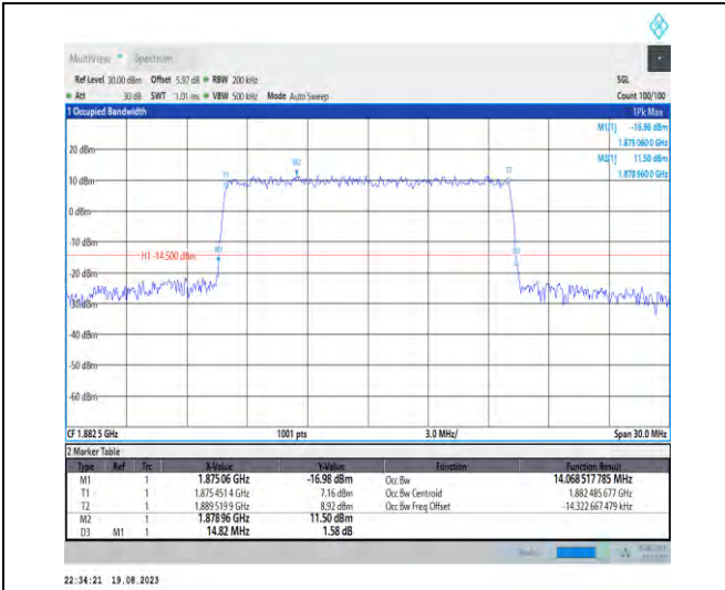
1-N25-PC3-15-15-M-7-CP-16QAM-Outer_Full-79@0 -Ant3-14.069-14.820-≤15-PASS
