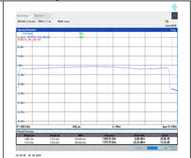
1-N25-PC3-15-30-H-3-DFT-PI2BPSK-Outer_Full-160@0-Ant3-1-seegraph-PASS-see graph
