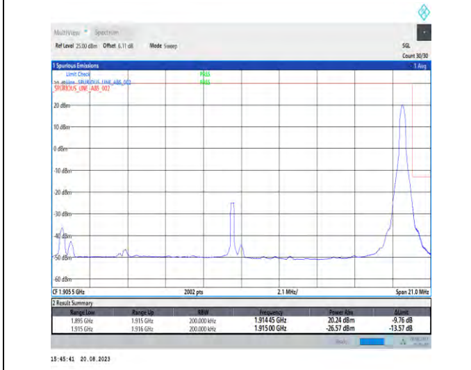
1-N25-PC3-15-20-H-5-CP-QPSK-Edge_1RB_Right-1@105-Ant3-1-seegraph-PASS-see graph
