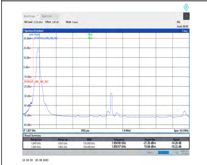
1-N25-PC3-15-15-L-4-CP-QPSK-Edge_1RB_Left-1@0-Ant3-1-seegraph-PASS-see graph
