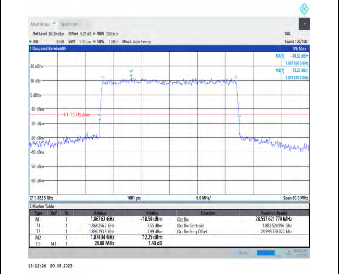
1-N25-PC3-15-30-M-3-DFT-16QAM-Outer_Full-160 @0-Ant3-28.538-29.880-≤30-PASS
