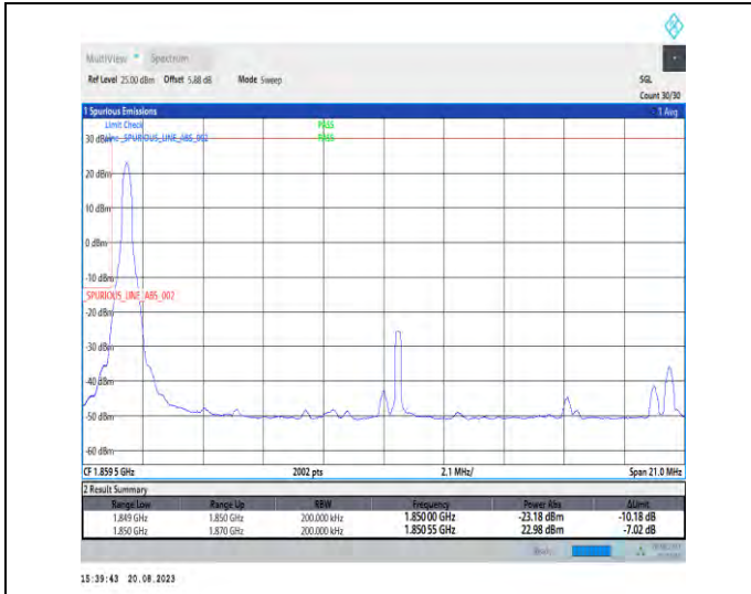
1-N25-PC3-15-20-L-1-DFT-PI2BPSK-Edge_1RB_Left-1@0-Ant3-1-seegrph-PASS-see graph
