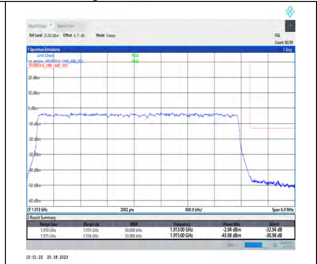
1-N25-PC3-15-5-H-3-DFT-PI2BPSK-Outer_Full-25@0-Ant3-1-seegraph-PASS-see graph
