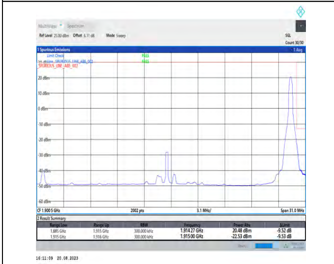
1-N25-PC3-15-30-H-5-CP-QPSK-Edge_1RB_Right-1@159-Ant3-1-seegraph-PASS-see graph
