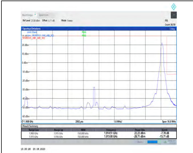
1-N25-PC3-15-15-H-2-DFT-PI2BPSK-Edge_1RB_Right-t1@78-Ant3-1-seegraph-PASS-see graph
