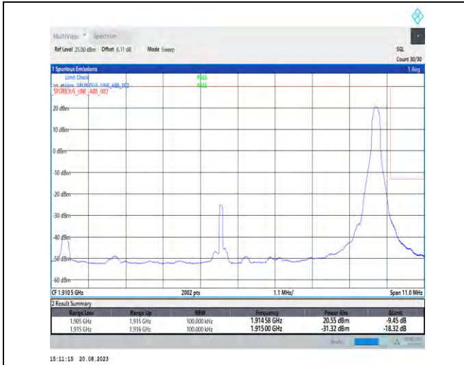
1-N25-PC3-15-10-H-2-DFT-PI2BPSK-Edge_1RB_Right-t@51-Ant3-1-seegraph-PASS-see graph
