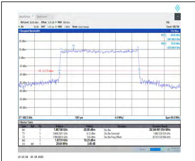
1-N25-PC3-15-30-M-8-CP-64QAM-Outer_Full-160@0-Ant3-28.544-29.640-≤30-PASS
