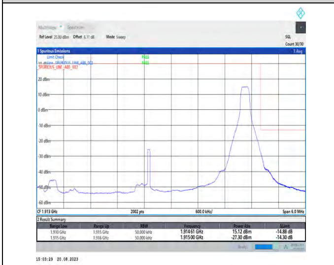
1-N25-PC3-15-5-H-5-CP-QPSK-Edge_1RB_Right-1@24-Ant3-1-seegraph-PASS-see graph
