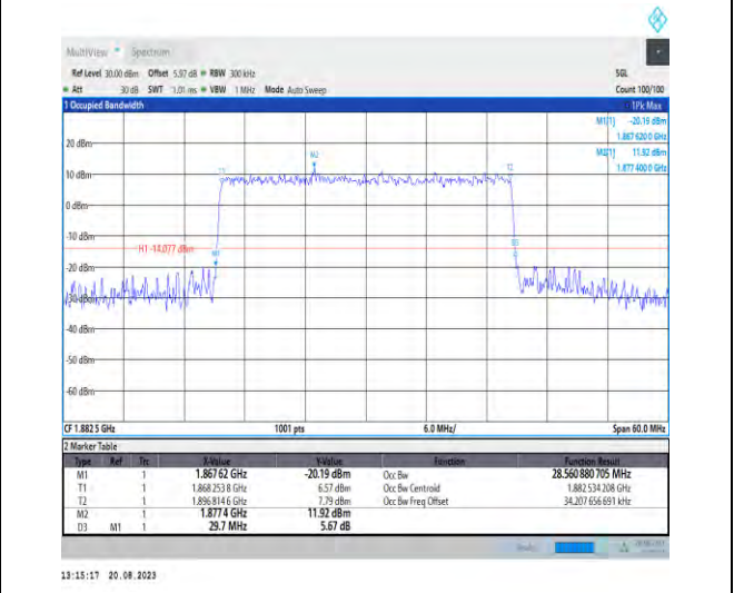
1-N25-PC3-15-30-M-7-CP-16QAM-Outer_Full-160@0 -Ant3-28.561-29.700-≤30-PASS
