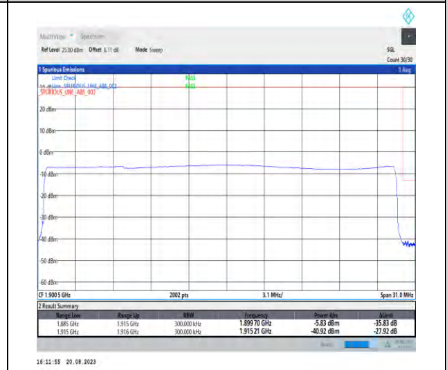
1-N25-PC3-15-30-H-6-CP-QPSK-Outer_Full-160@0-Ant3-1-seegraph-PASS-see graph
