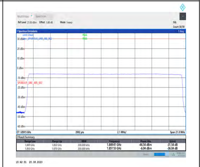
1-N25-PC3-15-20-L-6-CP-QPSK-Outer_Full-106@0-Ant3-1-seegrph-PASS-see graph
