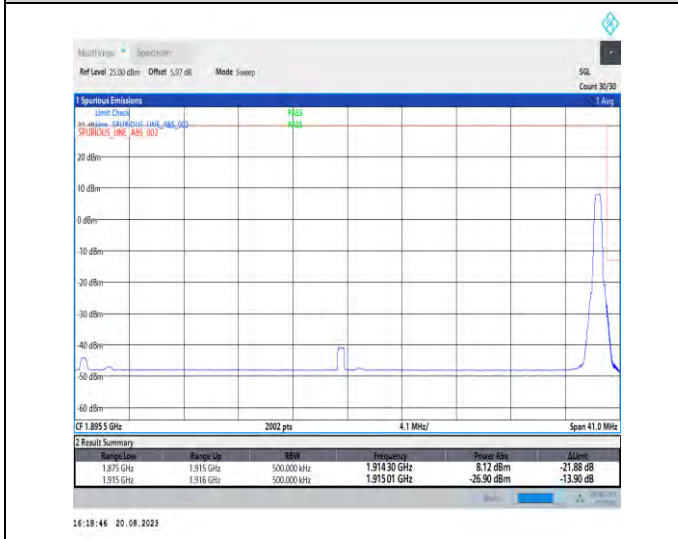
1-N25-PC3-15-40-H-5-CP-QPSK-Edge_1RB_Right-1@215-Ant3-1-seegraph-PASS-see graph
