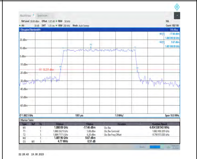
1-N25-PC3-15-5-M-8-CP-64QAM-Outer_Full-25@0-Ant3-4.455-4.770-≤5-PASS
