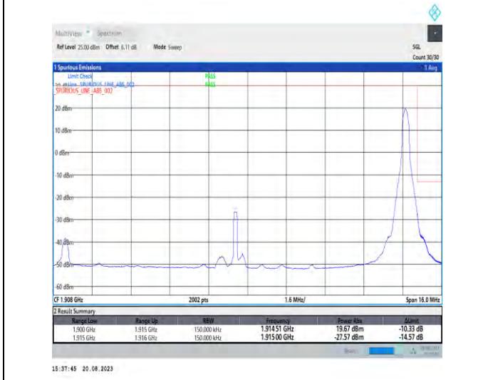
1-N25-PC3-15-15-H-5-CP-QPSK-Edge_1RB_Right-1@78-Ant3-1-seegraph-PASS-see graph
