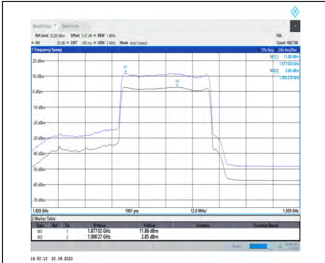
1-N25-PC3-15-40-H-1-DFT-256QAM-Outer_Full-216 @0-Ant3-9.03-100%-0.00-9.03-PASS-≤13
