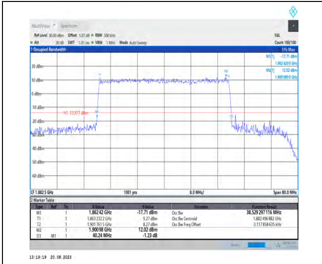
1-N25-PC3-15-40-M-7-CP-16QAM-Outer_Full-216@0-Ant3-38.529-40.240-≤40-PASS
