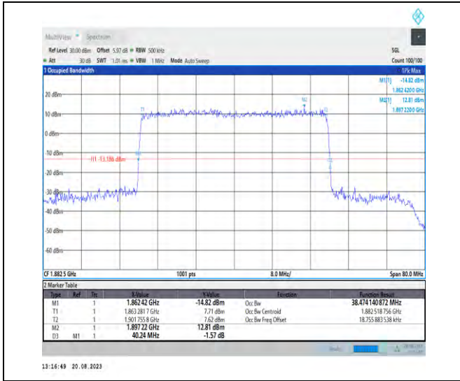
1-N25-PC3-15-40-M-3-DFT-16QAM-Outer_Full-216 @0-Ant3-38.474-40.240-≤40-PASS
