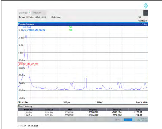
1-N25-PC3-15-25-L-1-DFT-PI2BPSK-Edge_1RB_Left-1@0-Ant3-1-seegraph-PASS-see graph
