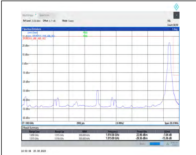
1-N25-PC3-15-25-H-2-DFT-PI2BPSK-Edge_1RB_Right-t-1@132-Ant3-1-seegraph-PASS-see graph
