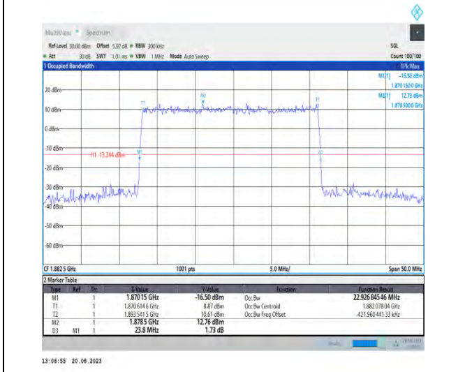
1-N25-PC3-15-25-M-3-DFT-16QAM-Outer_Full-128@0-Ant3-22.927-23.800-≤25-PASS
