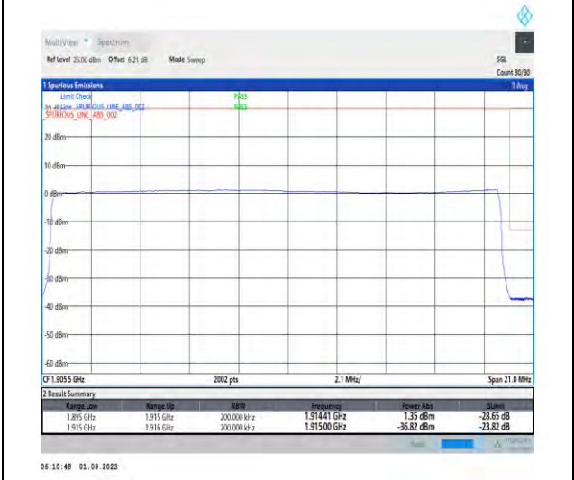
1-N25-PC3-15-20-H-6-CP-QPSK-Outer_Full-106@0-Ant3-1-seegraph-PASS-see graph
