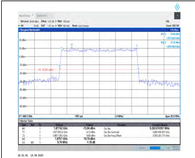
1-N25-PC3-15-10-M-8-CP-64QAM-Outer_Full-52@0 -Ant3-9.283-9.740-≤10-PASS
