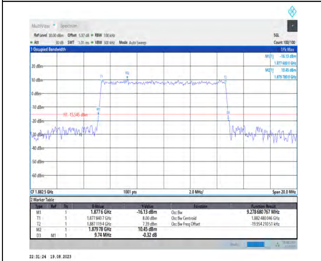
1-N25-PC3-15-10-M-6-CP-QPSK-Outer_Full-52@0- Ant3-9.279-9.740-≤10-PASS
