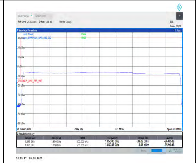
1-N25-PC3-15-40-L-6-CP-QPSK-Outer_Full-216@0-Ant3-1-seegraph-PASS-see graph
