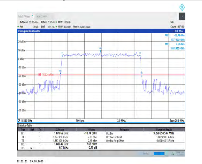
1-N25-PC3-15-10-M-9-CP-256QAM-Outer_Full-52@0 -Ant3-9.279-9.700-≤10-PASS
