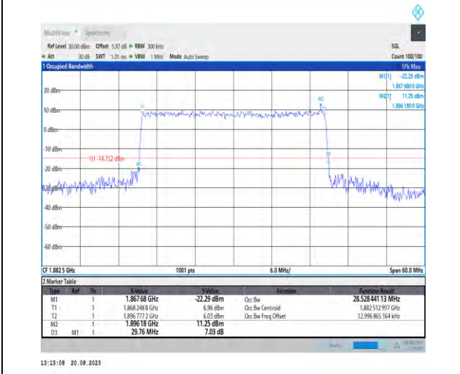
1-N25-PC3-15-30-M-6-CP-QPSK-Outer_Full-160@0 -Ant3-28.528-29.760-≤30-PASS
