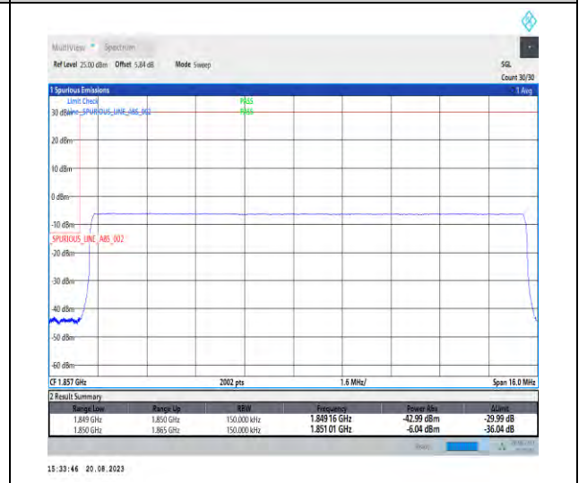
1-N25-PC3-15-15-L-6-CP-QPSK-Outer_Full-79@0-Ant3-1-seegraph-PASS-see graph
