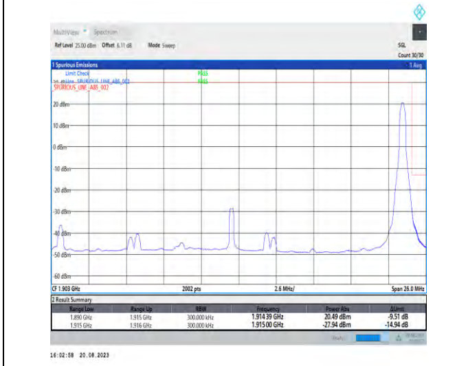
1-N25-PC3-15-25-H-5-CP-QPSK-Edge_1RB_Right-1@132-Ant3-1-seegraph-PASS-see graph
