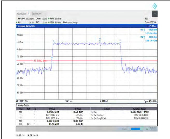
1-N25-PC3-15-20-M-6-CP-QPSK-Outer_Full-106@0 -Ant3-18.964-19.760-≤20-PASS
