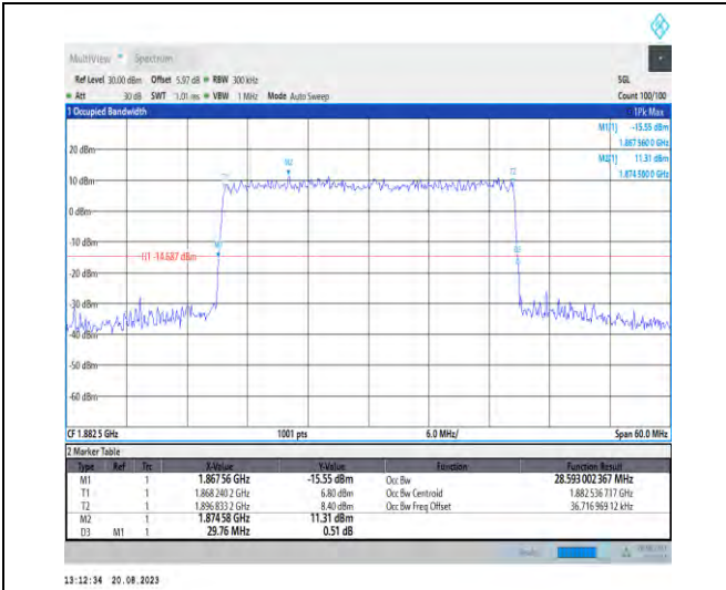
1-N25-PC3-15-30-M-4-DFT-64QAM-Outer_Full-160 @0-Ant3-28.593-29.760-≤30-PASS
