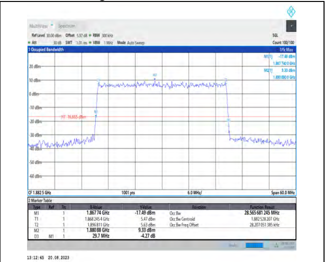
1-N25-PC3-15-30-M-5-DFT-256QAM-Outer_Full-160 @0-Ant3-28.566-29.700-≤30-PASS
