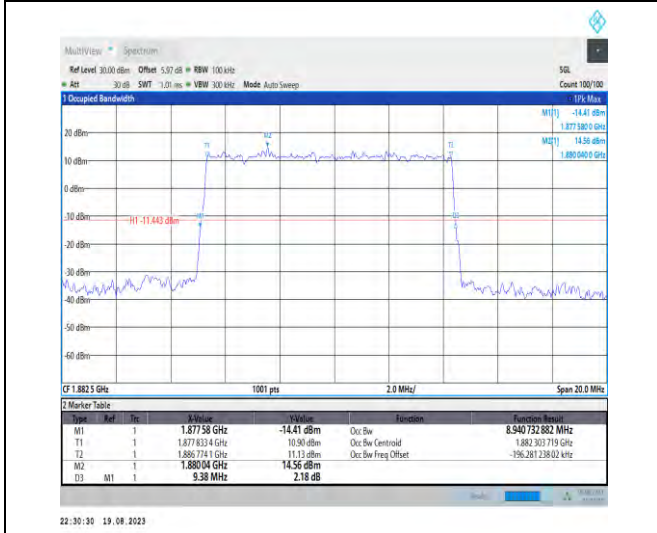
1-N25-PC3-15-10-M-2-DFT-PI2BPSK-Outer_Full-50@0-Ant3-8.941-9.380-≤10-PASS
