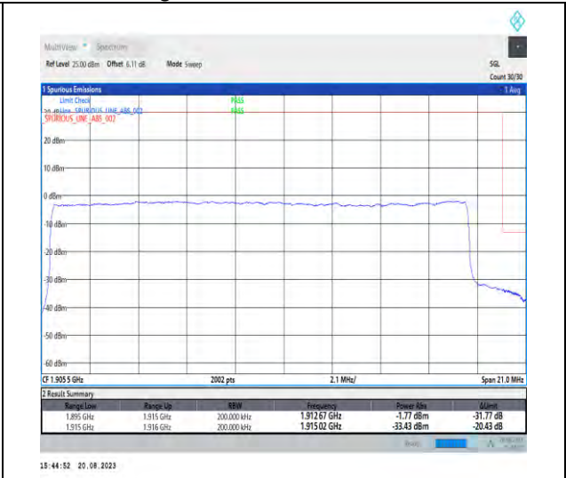
1-N25-PC3-15-20-H-3-DFT-PI2BPSK-Outer_Full-100@0-Ant3-1-seegraph-PASS-see graph
