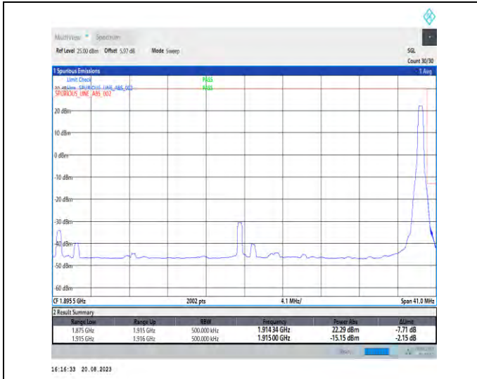
1-N25-PC3-15-40-H-2-DFT-PI2BPSK-Edge_1RB_Right-t-1@215-Ant3-1-seegraph-PASS-see graph
