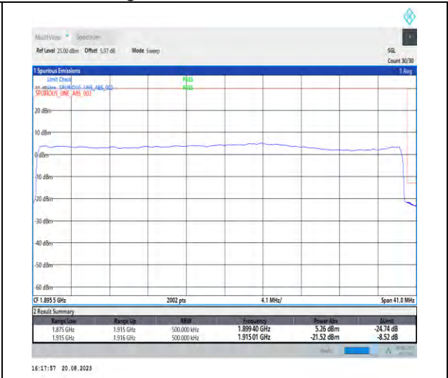
1-N25-PC3-15-40-H-3-DFT-PI2BPSK-Outer_Full-216@0-Ant3-1-seegraph-PASS-see graph
