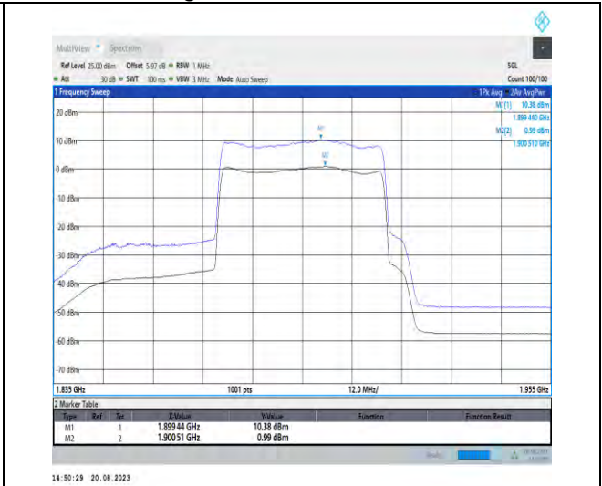
1-N25-PC3-15-40-H-2-CP-256QAM-Outer_Full-216 @0-Ant3-9.39-100%-0.00-9.39-PASS-≤13
