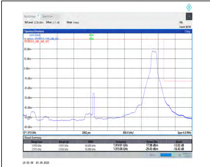
1-N25-PC3-15-5-H-2-DFT-PI2BPSK-Edge_1RB_Right-1@24-Ant3-1-seegraph-PASS-see graph
