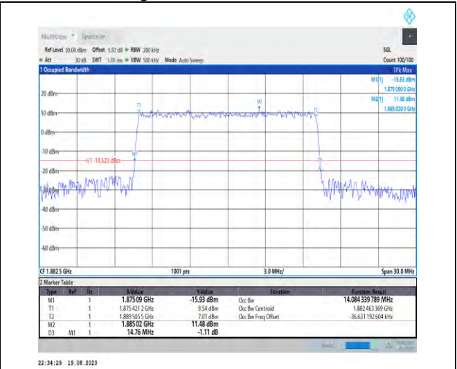
1-N25-PC3-15-15-M-8-CP-64QAM-Outer_Full-79@0 -Ant3-14.084-14.760-≤15-PASS
