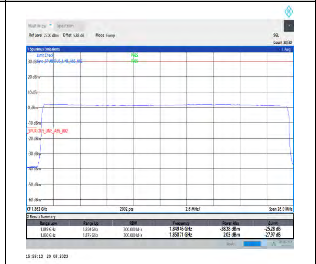
1-N25-PC3-15-25-L-6-CP-QPSK-Outer_Full-133@0-Ant3-1-seegraph-PASS-see graph
