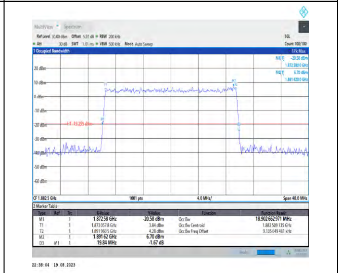
1-N25-PC3-15-20-M-9-CP-256QAM-Outer_Full-106@0 -Ant3-18.903-19.840-≤20-PASS
