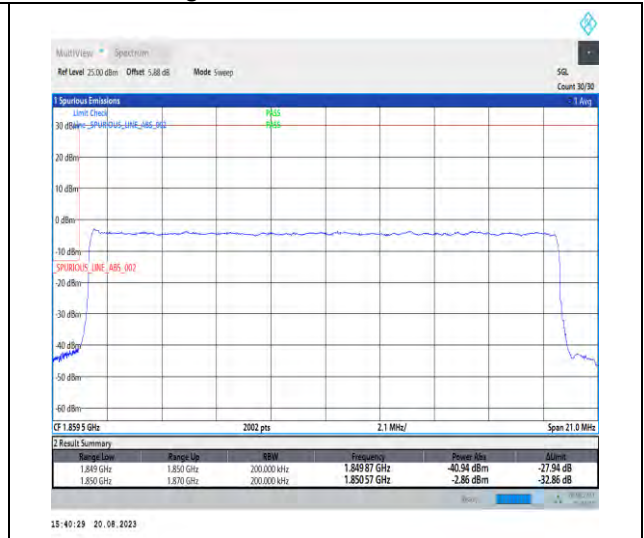
1-N25-PC3-15-20-L-3-DFT-PI2BPSK-Outer_Full-100@0-Ant3-1-seegrph-PASS-see graph
