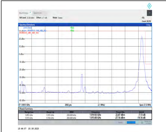
1-N25-PC3-15-20-H-2-DFT-PI2BPSK-Edge_1RB_Right-t-1@105-Ant3-1-seegraph-PASS-see graph
