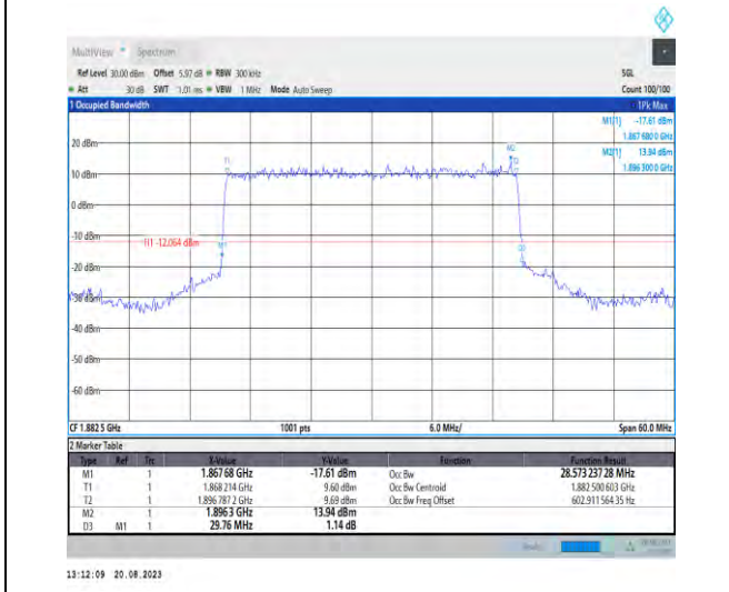
1-N25-PC3-15-30-M-2-DFT-PI2BPSK-Outer_Full-160 @0-Ant3-28.573-29.760-≤30-PASS
