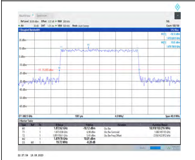
1-N25-PC3-15-20-M-8-CP-64QAM-Outer_Full-106@0 -Ant3-18.918-19.720-≤20-PASS
