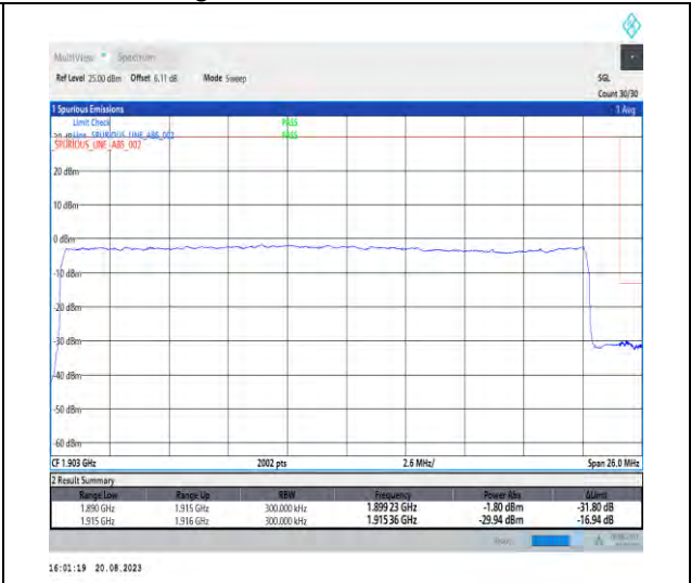
1-N25-PC3-15-25-H-3-DFT-PI2BPSK-Outer_Full-1-28@0-Ant3-1-seegraph-PASS-see graph
