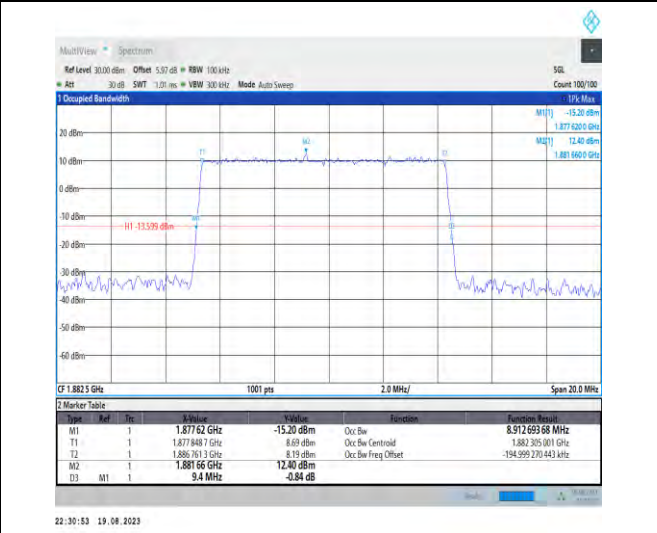
1-N25-PC3-15-10-M-3-DFT-16QAM-Outer_Full-50@0-Ant3-8.913-9.400-≤10-PASS
