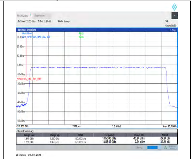
1-N25-PC3-15-15-L-3-DFT-PI2BPSK-Outer_Full-75@0-Ant3-1-seegraph-PASS-see graph
