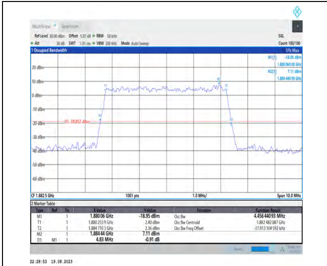
1-N25-PC3-15-5-M-9-CP-256QAM-Outer_Full-25@0 -Ant3-4.456-4.830-≤5-PASS
