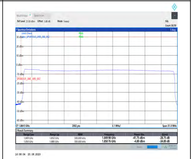
1-N25-PC3-15-30-L-6-CP-QPSK-Outer_Full-160@0-Ant3-1-seegrph-PASS-see graph
