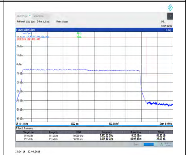
1-N25-PC3-15-5-H-6-CP-QPSK-Outer_Full-25@0-Ant3-1-seegraph-PASS-see graph
