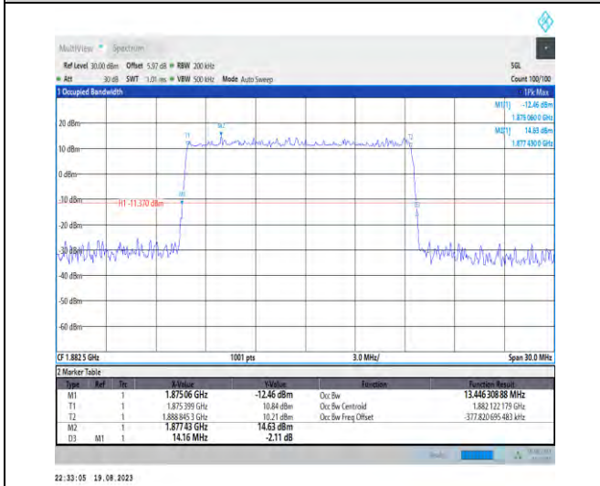
1-N25-PC3-15-15-M-1-DFT-QPSK-Outer_Full-75@0 -Ant3-13.446-14.160-≤15-PASS
