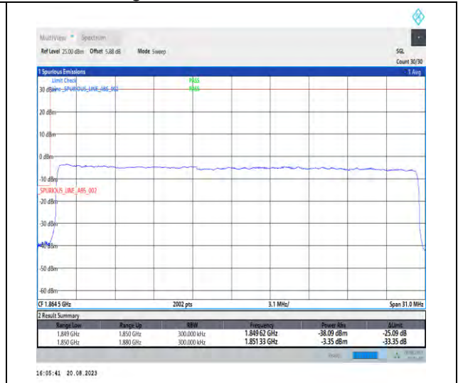
1-N25-PC3-15-30-L-3-DFT-PI2BPSK-Outer_Full-160@0-Ant3-1-seegrph-PASS-see graph
