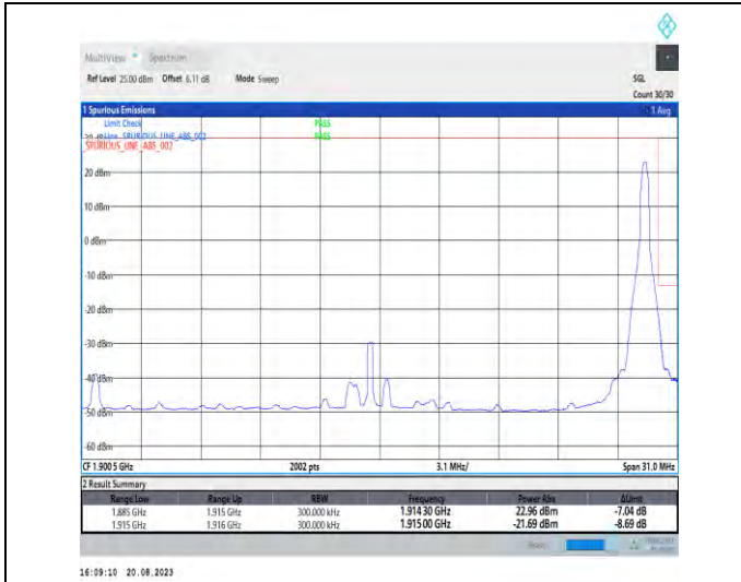
1-N25-PC3-15-30-H-2-DFT-PI2BPSK-Edge_1RB_Right-t-1@159-Ant3-1-seegraph-PASS-see graph
