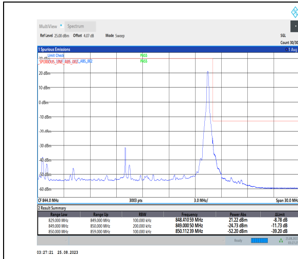
1-N5-PC3-15-20-H-2-DFT-PI2BPSK-Edge_1RB_Right-1@105-Ant1-1--PASS-see graph
