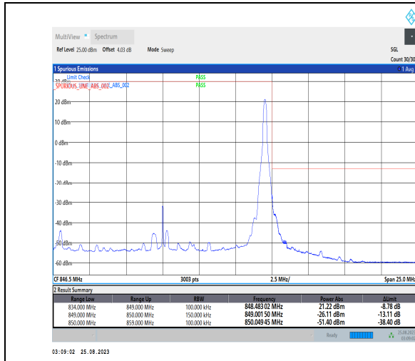
1-N5-PC3-15-15-H-2-DFT-PI2BPSK-Edge_1RB_Right-1@78-Ant1-1--PASS-see graph
