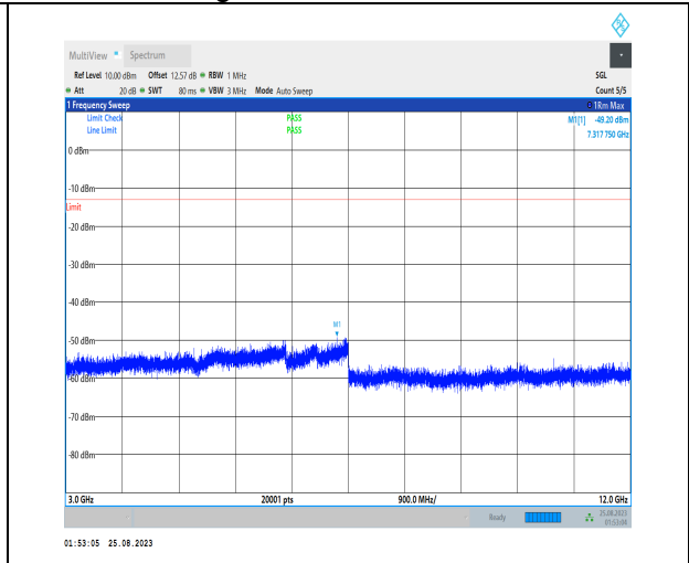
1-N5-PC3-15-20-M-1-DFT-PI2BPSK-Inner_1RB_Left -1@1-3000-12000-Ant1-7317.75--49.20--13-PASS
