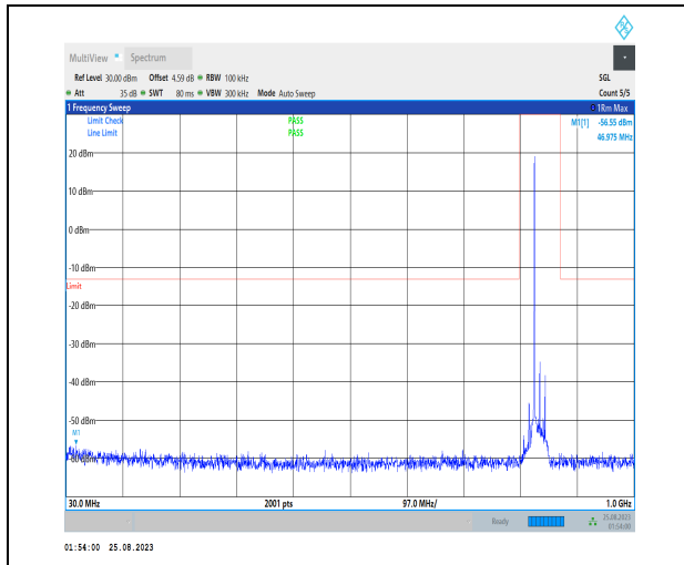
1-N5-PC3-15-20-H-1-DFT-PI2BPSK-Inner_1RB_Left -1@1-30-1000-Ant1-46.98--56.55--13-PASS
