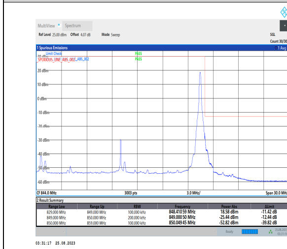
1-N5-PC3-15-20-H-5-CP-QPSK-Edge_1RB_Right-1@105-Ant1-1--PASS-see graph
