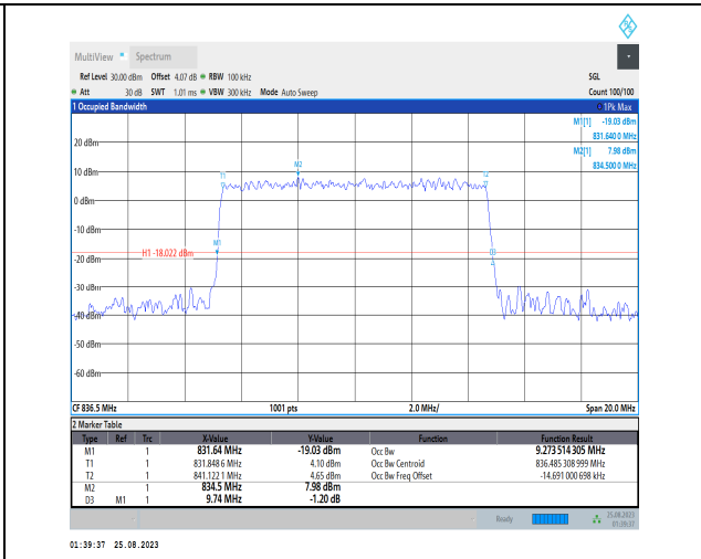
1-N5-PC3-15-10-M-9-CP-256QAM-Outer_Full-52@0- Ant1-9.274-9.740-≤10-PASS
