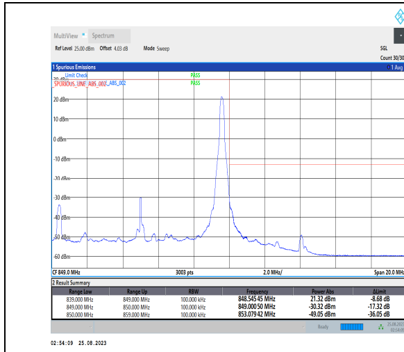
1-N5-PC3-15-10-H-2-DFT-PI2BPSK-Edge_1RB_Right-1@51-Ant1-1--PASS-see graph
