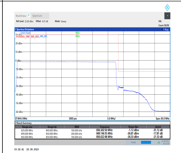
1-N5-PC3-15-20-H-6-CP-QPSK-Outer_Full-106@0-Ant1-1--PASS-see graph
