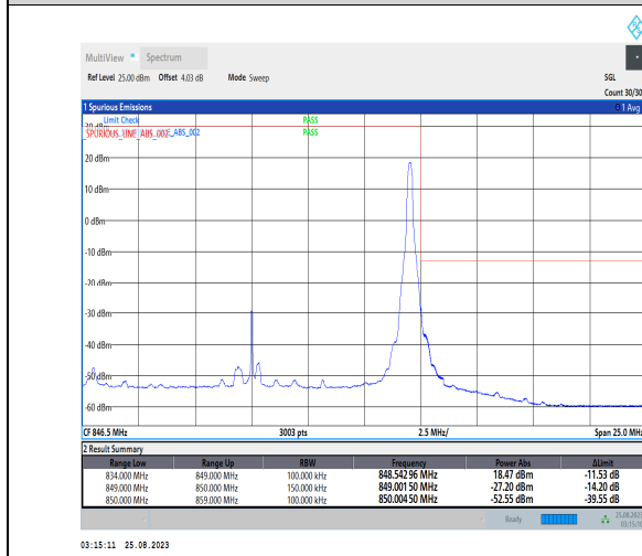
1-N5-PC3-15-15-H-5-CP-QPSK-Edge_1RB_Right-1@78-Ant1-1--PASS-see graph
