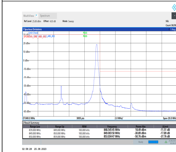
1-N5-PC3-15-10-H-5-CP-QPSK-Edge_1RB_Right-1@51-Ant1-1--PASS-see graph
