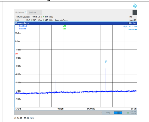
1-N5-PC3-15-20-H-1-DFT-PI2BPSK-Inner_1RB_Left -1@1-1000-3000-Ant1-2489.50--27.21--13-PASS
