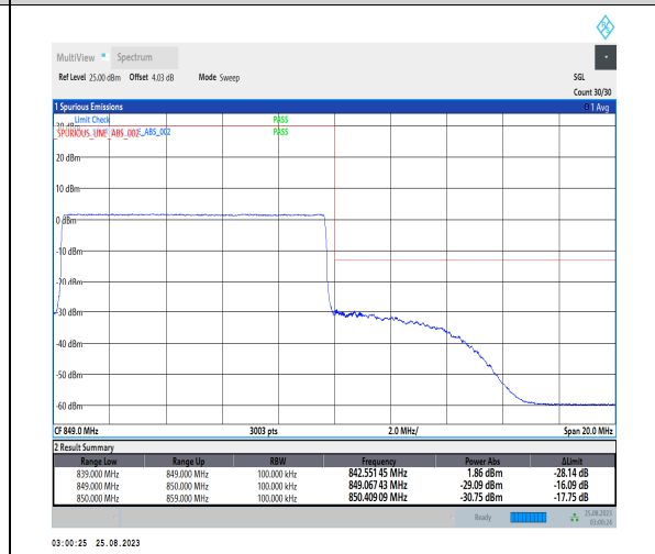
1-N5-PC3-15-10-H-6-CP-QPSK-Outer_Full-52@0-Ant1-1--PASS-see graph
