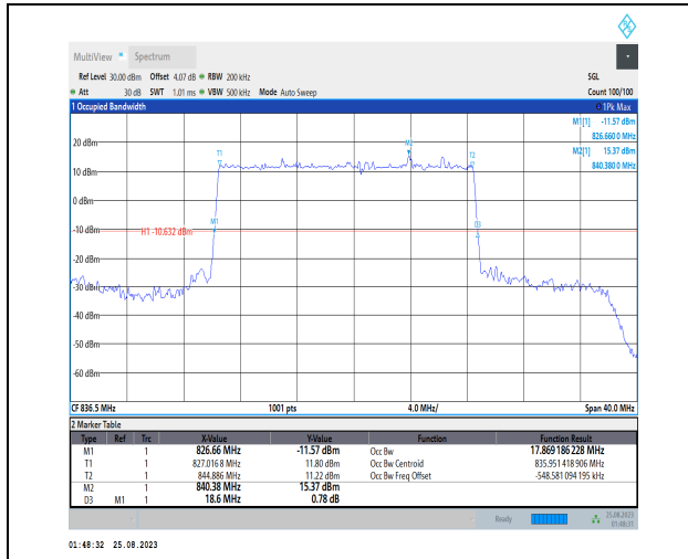
1-N5-PC3-15-20-M-2-DFT-PI2BPSK-Outer_Full-100 @0-Ant1-17.869-18.600-<20-PASS
