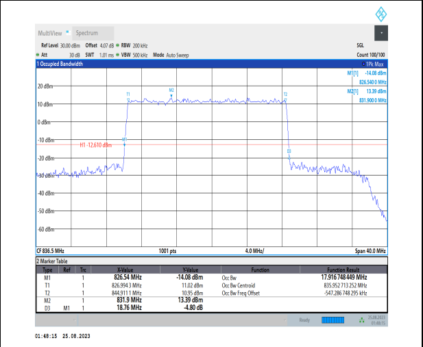
1-N5-PC3-15-20-M-1-DFT-QPSK-Outer_Full-100@0-Ant1-17.917-18.760-≤20-PASS
