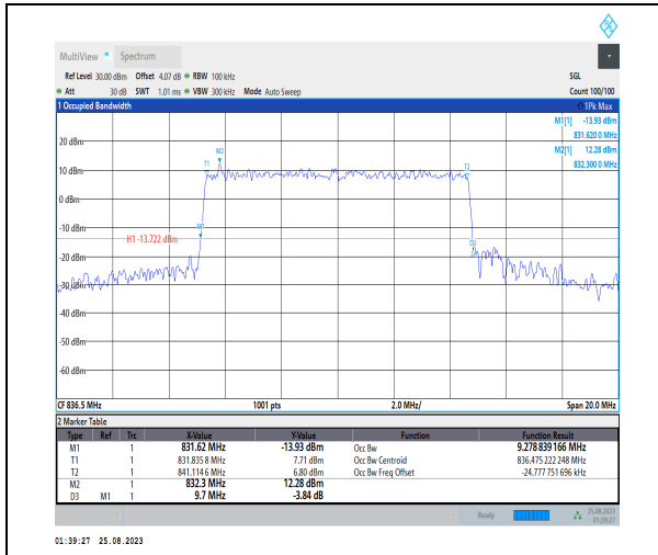
1-N5-PC3-15-10-M-8-CP-64QAM-Outer_Full-52@0 -Ant1-9.279-9.700-≤10-PASS
