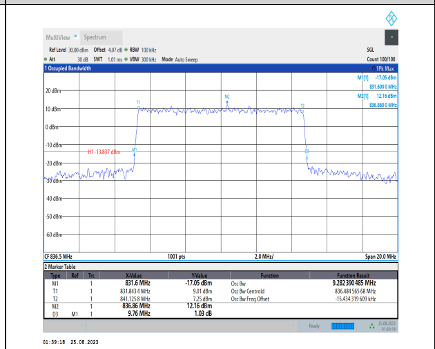
1-N5-PC3-15-10-M-7-CP-16QAM-Outer_Full-52@0-Ant1-9.282-9.760-≤10-PASS
