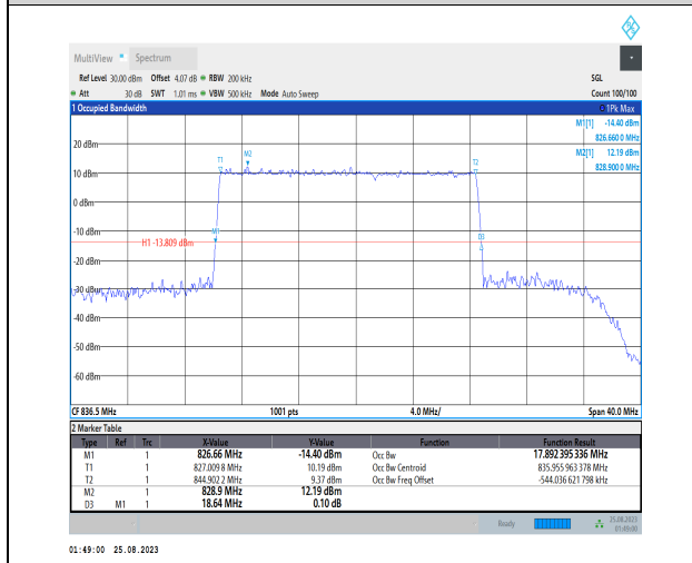
1-N5-PC3-15-20-M-4-DFT-64QAM-Outer_Full-100 @0-Ant1-17.892-18.640-<20-PASS
