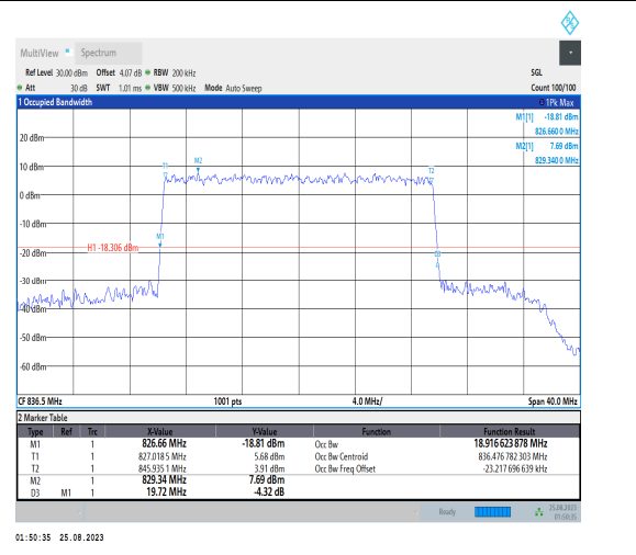
1-N5-PC3-15-20-M-9-CP-256QAM-Outer_Full-106@0-Ant1-18.917-19.720-≤20-PASS
