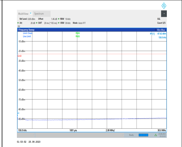
1-N5-PC3-15-20-H-1-DFT-PI2BPSK-Inner_1RB_Left -1@1-0.15-30-Ant1-0.15--87.62--23-PASS
