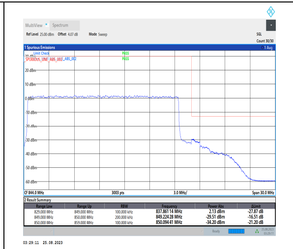
1-N5-PC3-15-20-H-3-DFT-PI2BPSK-Outer_Full-10@0-Ant1-1--PASS-see graph
