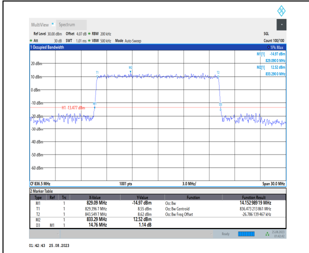
1-N5-PC3-15-15-M-7-CP-16QAM-Outer_Full-79@0-Ant1-14.153-14.760-≤15-PASS
