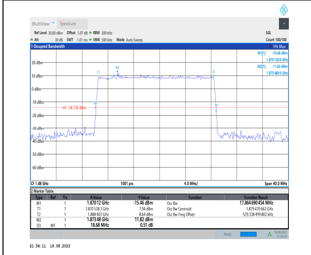
1-N2-PC3-15-20-M-4-DFT-64QAM-Outer_Full-100 @0-Ant3-17.865-18.680-≤20-PASS
