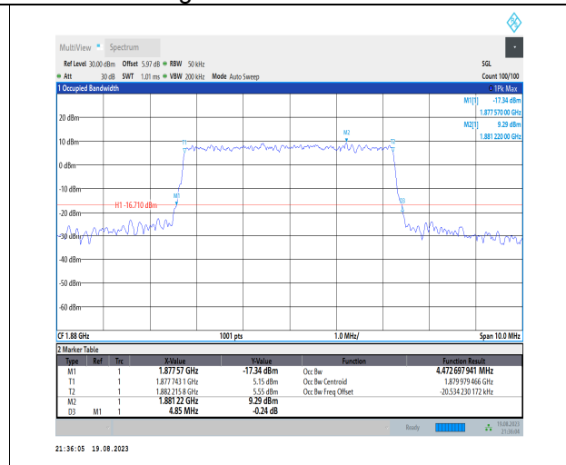
1-N2-PC3-15-5-M-6-CP-QPSK-Outer_Full-25@0-An t3-4.473-4.850-≤5-PASS
