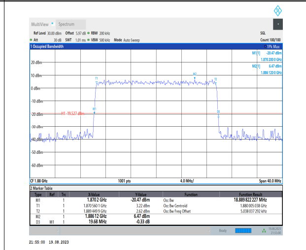
1-N2-PC3-15-20-M-9-CP-256QAM-Outer_Full-106@0-Ant3-18.89-19.680-<20-PASS
