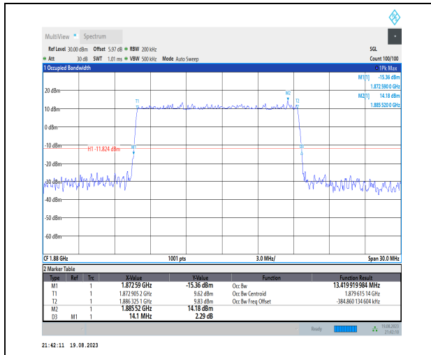
1-N2-PC3-15-15-M-3-DFT-16QAM-Outer_Full-75@0 -Ant3-13.42-14.100≤15-PASS
