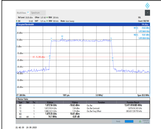
1-N2-PC3-15-15-M-5-DFT-256QAM-Outer_Full-75@0 -Ant3-13.412-14.100≤15-PASS
