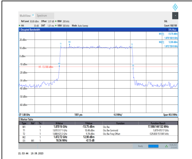
1-N2-PC3-15-20-M-2-DFT-PI2BPSK-Outer_Full-100 @0-Ant3-17.906-18.560-≤20-PASS
