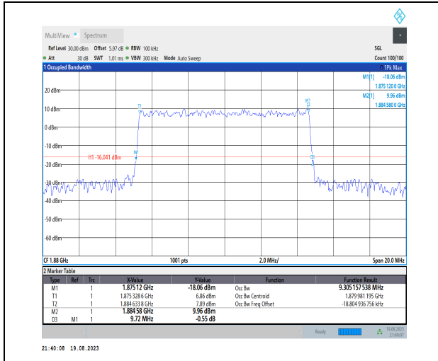
1-N2-PC3-15-10-M-8-CP-64QAM-Outer_Full-52@0-Ant3-9.305-9.720-≤10-PASS
