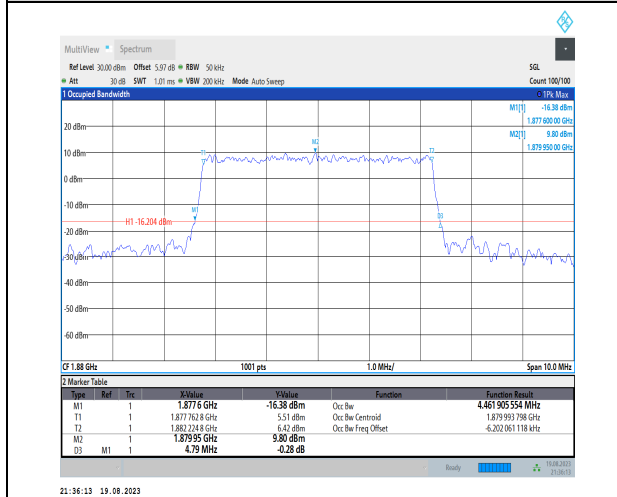
1-N2-PC3-15-5-M-7-CP-16QAM-Outer_Full-25@0-A nt3-4.462-4.790-≤5-PASS
