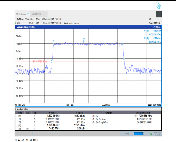
1-N2-PC3-15-15-M-6-CP-QPSK-Outer_Full-79@0-A nt3-14.117-14.850≤15-PASS
