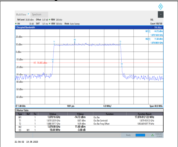
1-N2-PC3-15-20-M-3-DFT-16QAM-Outer_Full-100 @0-Ant3-17.877-18.640-≤20-PASS
