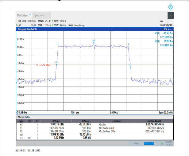
1-N2-PC3-15-10-M-1-DFT-QPSK-Outer_Full-50@0-Ant3-8.897-9.420-≤10-PASS
