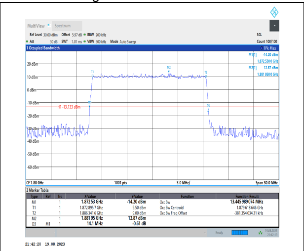
1-N2-PC3-15-15-M-4-DFT-64QAM-Outer_Full-75@0 -Ant3-13.446-14.100≤15-PASS
