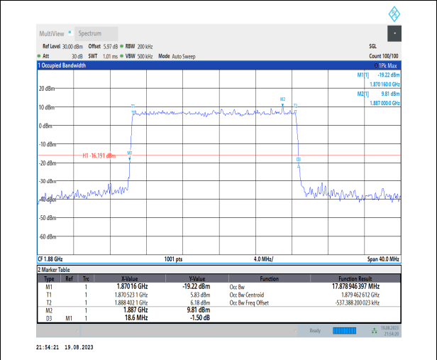
1-N2-PC3-15-20-M-5-DFT-256QAM-Outer_Full-100 @0-Ant3-17.879-18.600-≤20-PASS
