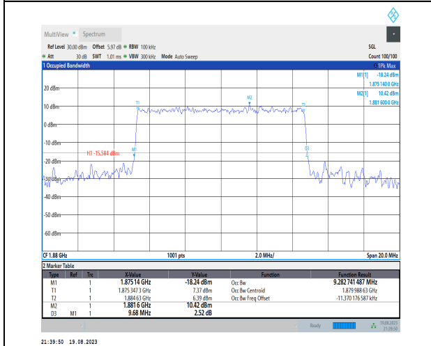
1-N2-PC3-15-10-M-6-CP-QPSK-Outer_Full-52@0-Ant3-9.283-9.680-≤10-PASS
