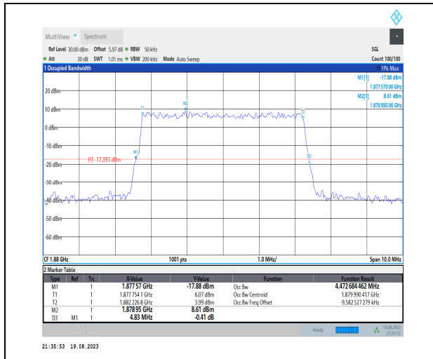
1-N2-PC3-15-5-M-5-DFT-256QAM-Outer_Full-25@0 -Ant3-4.473-4.830-≤5-PASS
