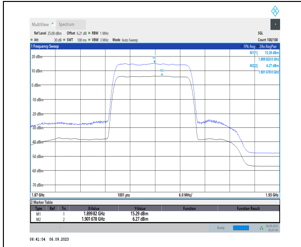
1-N2-PC3-15-20-H-1-DFT-256QAM-Outer_Full-100 @0-Ant3-9.02-100%-0.00-9.02-PASS-≤13
