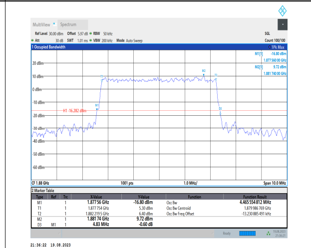
1-N2-PC3-15-5-M-8-CP-64QAM-Outer_Full-25@0-A nt3-4.466-4.830-≤5-PASS
