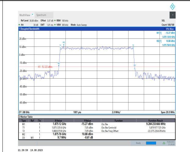
1-N2-PC3-15-10-M-7-CP-16QAM-Outer_Full-52@0-Ant3-9.284-9.700-≤10-PASS
