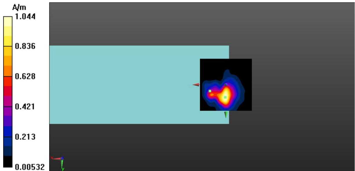
Fig A.12 T-Coil WLAN 5.2GHz-Z
