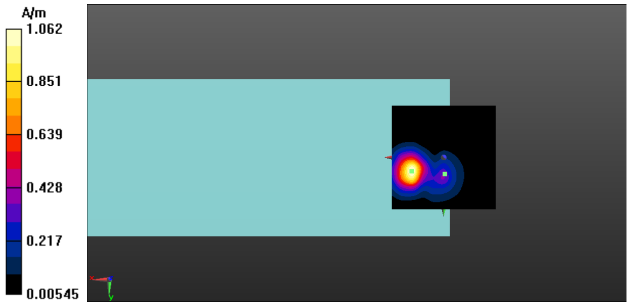
Fig A.11 T-Coil WLAN 2.4GHz-Z
