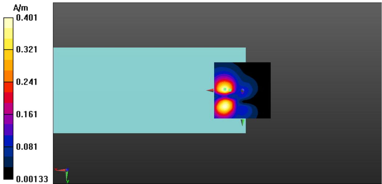
Fig A.10 T-Coil LTE-Band 66-Y
