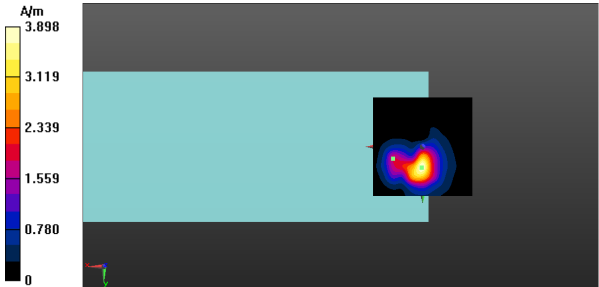
Fig A.18 T-Coil WLAN 2.4GHz-Z
