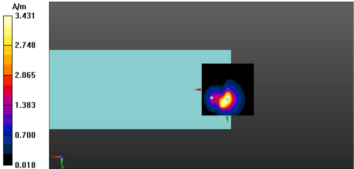
Fig A.17 T-Coil LTE-Band 4-Z
