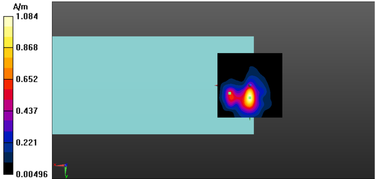
Fig A.14 T-Coil WLAN 5.5GHz-Z
