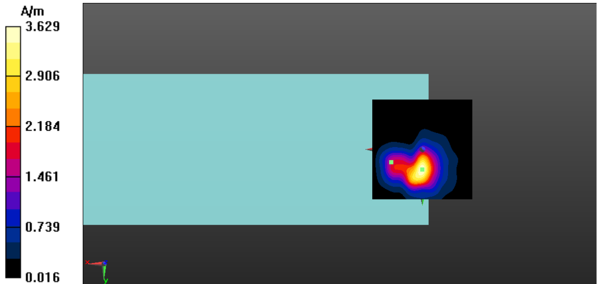
Fig A.16 T-Coil WCDMA Band 2-Z
