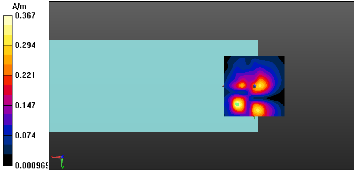
Fig A.13 T-Coil WLAN 5.3GHz-Y
