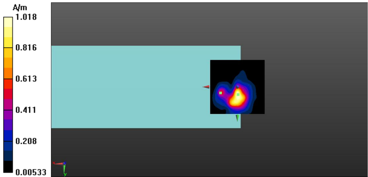
Fig A.15 T-Coil WLAN 5.8GHz-Z
