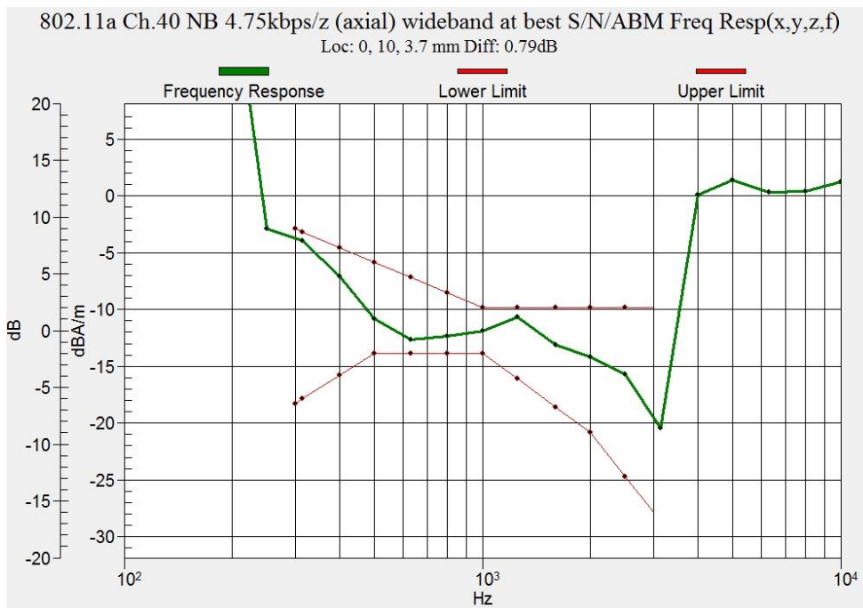
Figure B.12 Frequency Response of WLAN 5.2GHz
