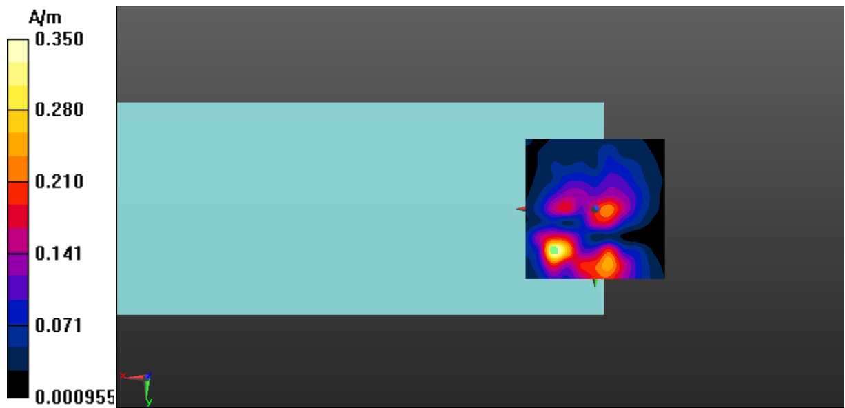
Fig A.15 T-Coil WLAN 5.8GHz-Y
