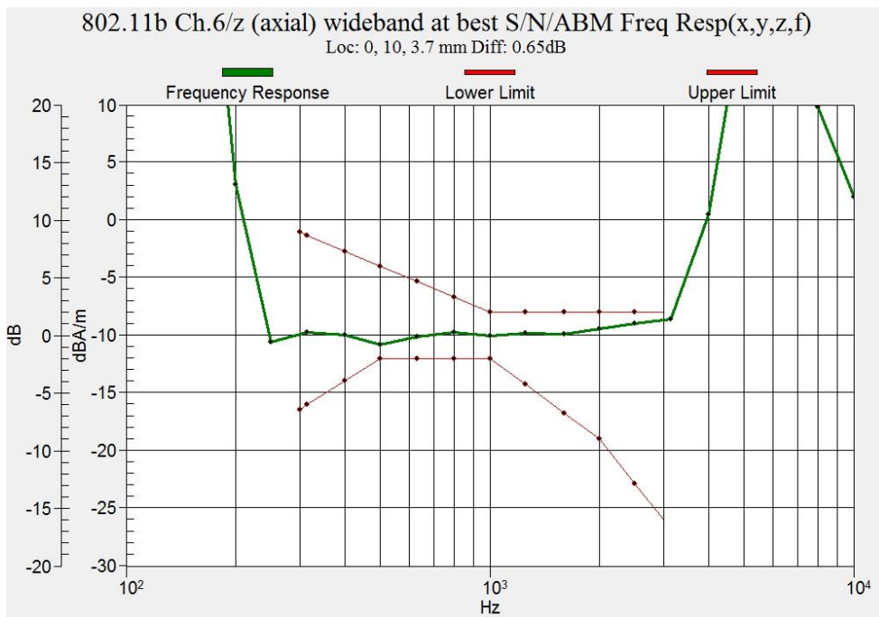
Figure B.18 Frequency Response of WLAN 2.4GHz (Google Duo)
