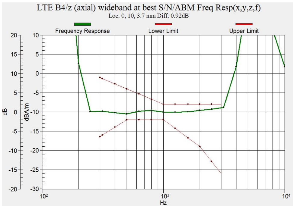
Figure B.17 Frequency Response of LTE Band 4 (Google Duo)
