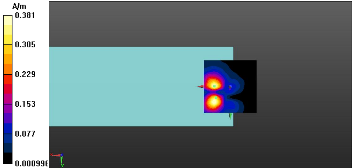
Fig A.14 T-Coil WLAN 5.5GHz-Y
