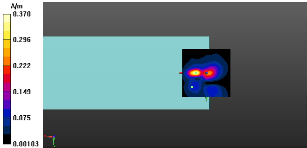
Fig A.8 T-Coil LTE-Band 14-Y
