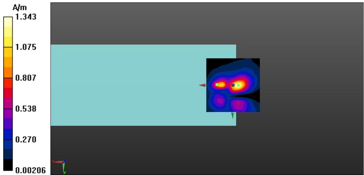
Fig A.17 T-Coil LTE-Band 4-Y
