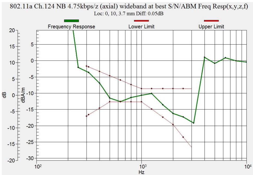
Figure B.14 Frequency Response of WLAN 5.5GHz
