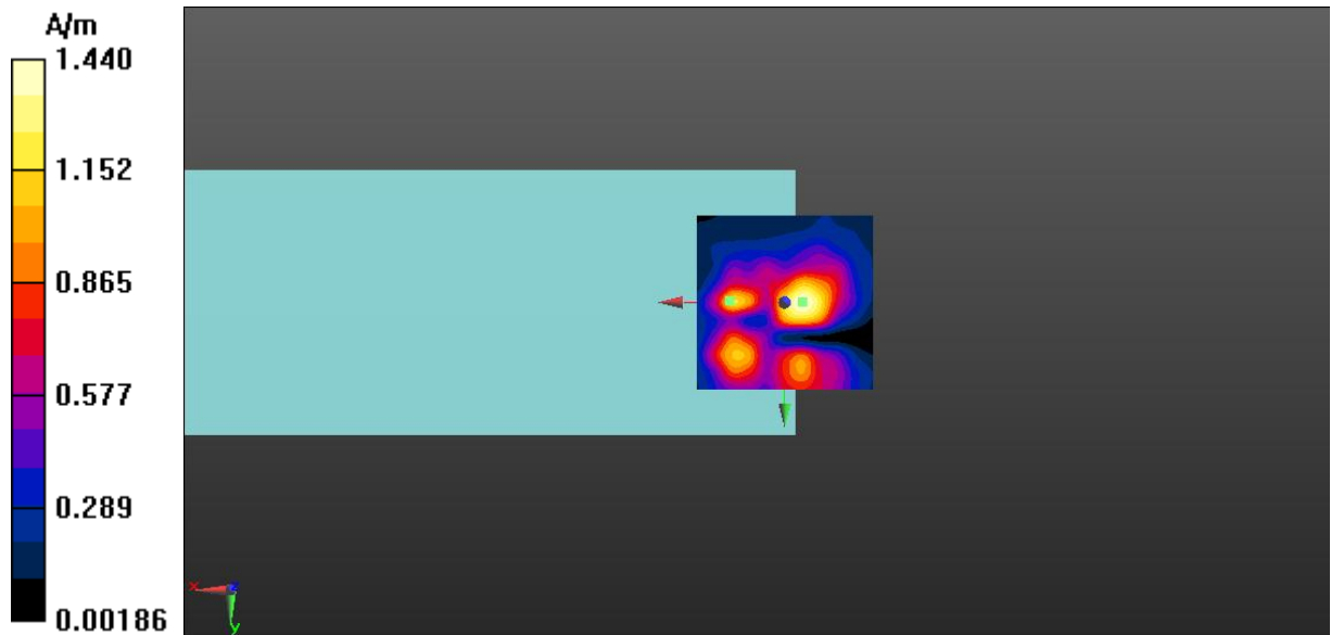
Fig A.16 T-Coil WCDMA Band 2-Y
