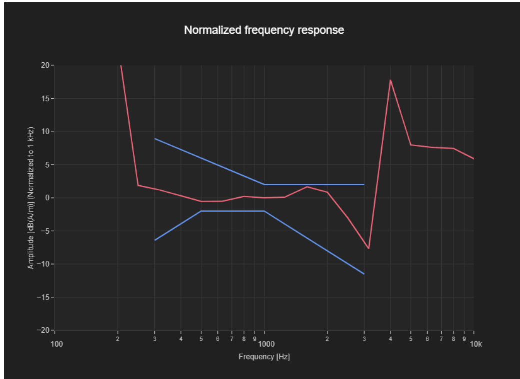
Figure C.1 Frequency Response of VoNR B2-N77
