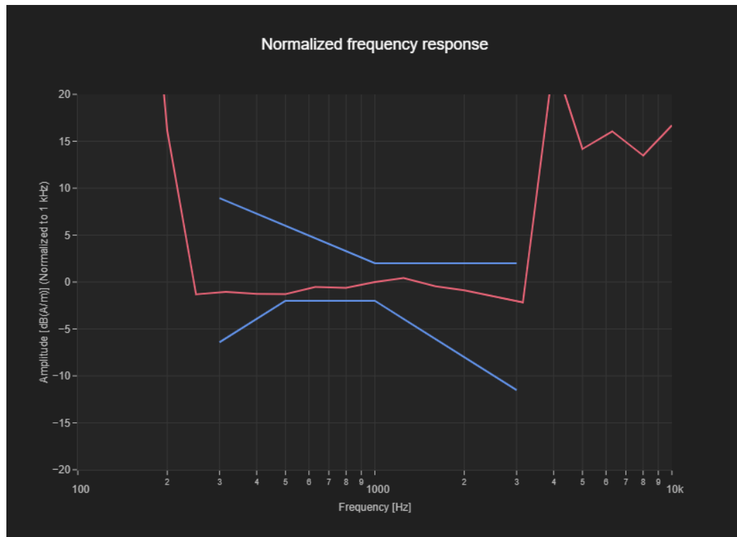
Figure C.2 Frequency Response of WiFi2.4G-OTT
