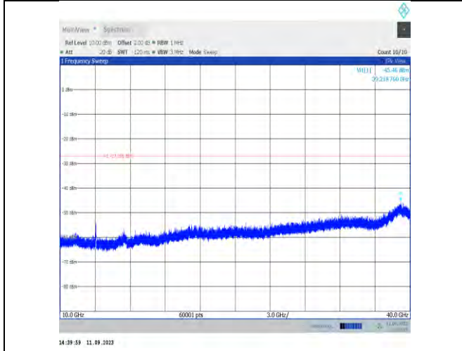
11ax40MIMO-Ant7-6525-10000~40000
