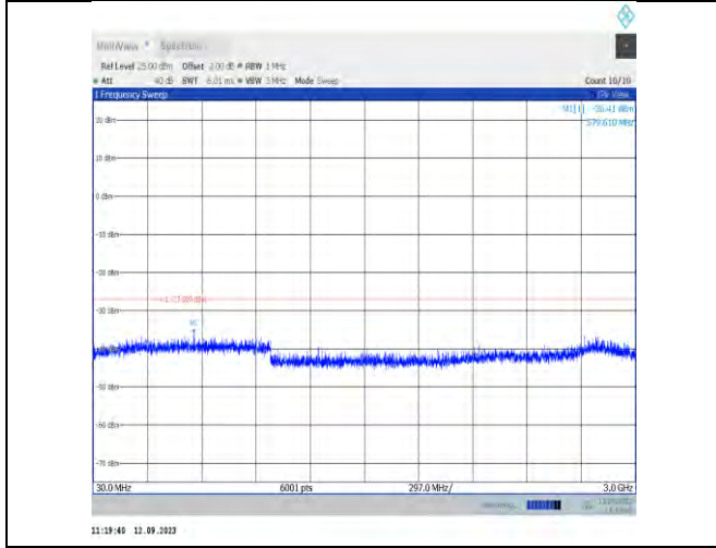
11ax80MIMO-Ant7-6625-30~3000
