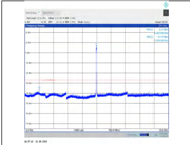
11ax40MIMO-Ant9-6485-3000~10000
