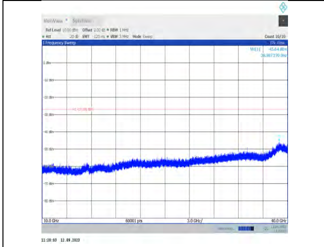
11ax80MIMO-Ant7-6625-10000~40000
