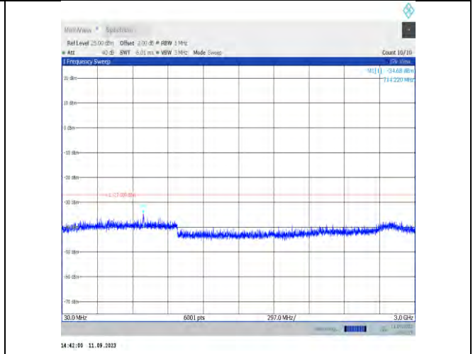
11ax40MIMO-Ant9-6525-30~3000
