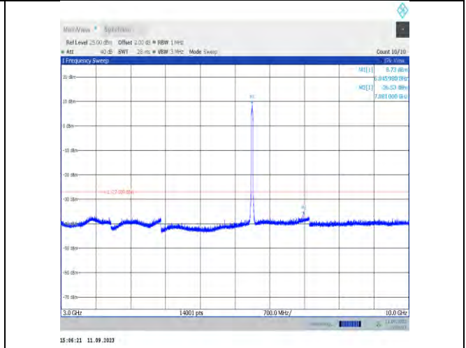
11ax40MIMO-Ant7-6845-3000~10000
