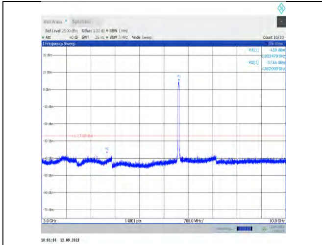
11ax40MIMO-Ant9-6925-3000~10000
