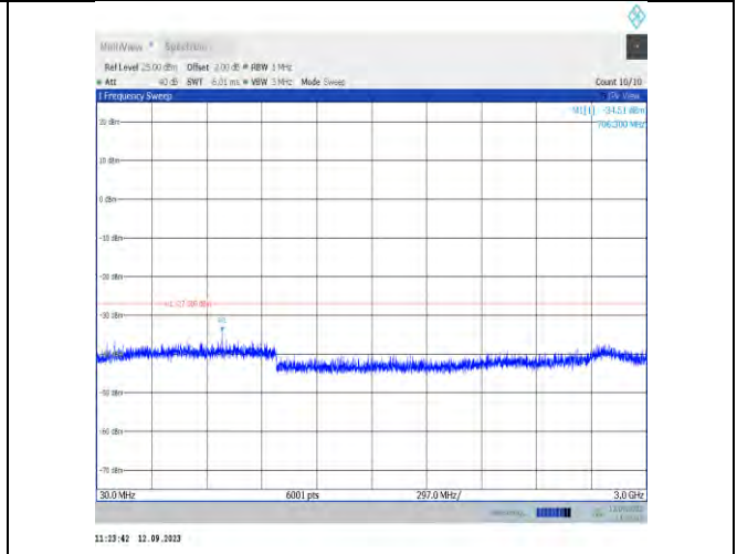
11ax80MIMO-Ant9-6625-30~3000
