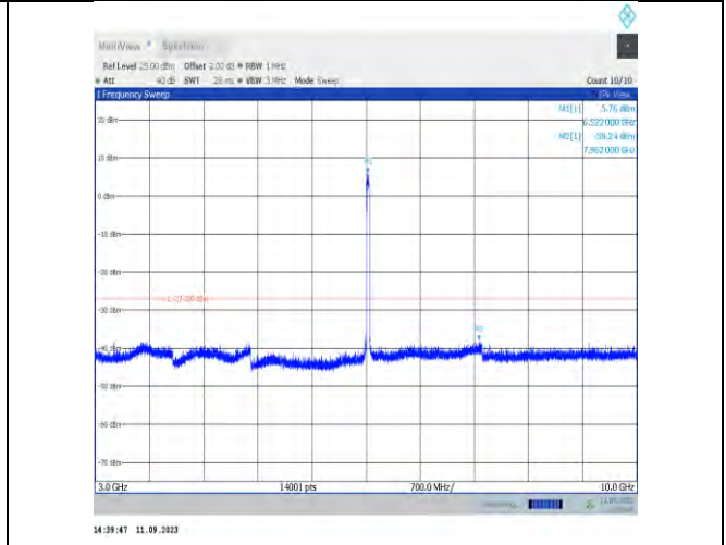
11ax40MIMO-Ant7-6525-3000~10000
