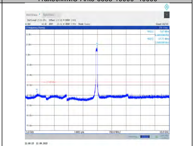
11ax80MIMO-Ant7-6465-3000~10000
