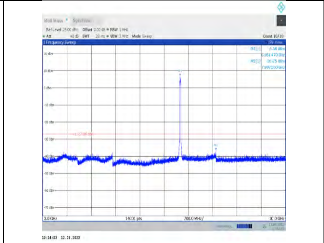
11ax40MIMO-Ant7-6965-3000~10000
