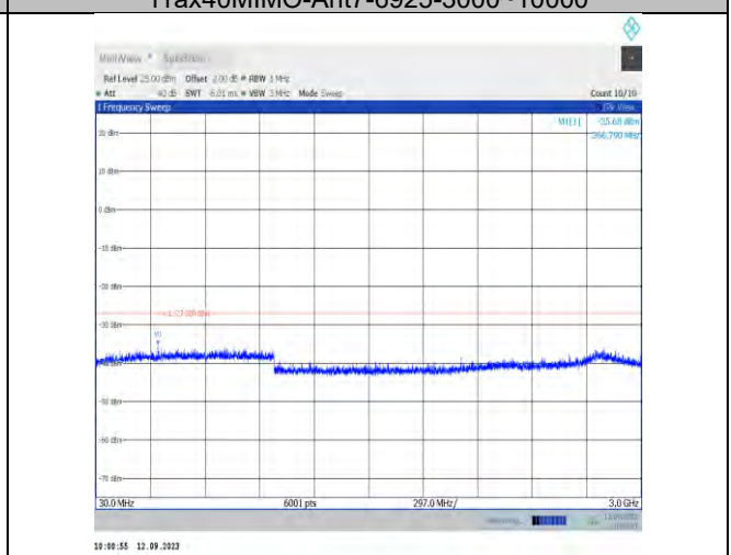
11ax40MIMO-Ant9-6925-30~3000
