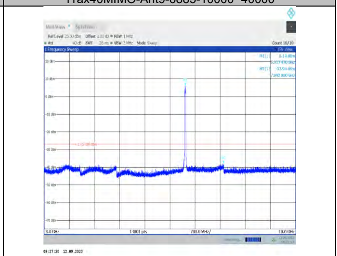
11ax40MIMO-Ant7-6925-3000~10000
