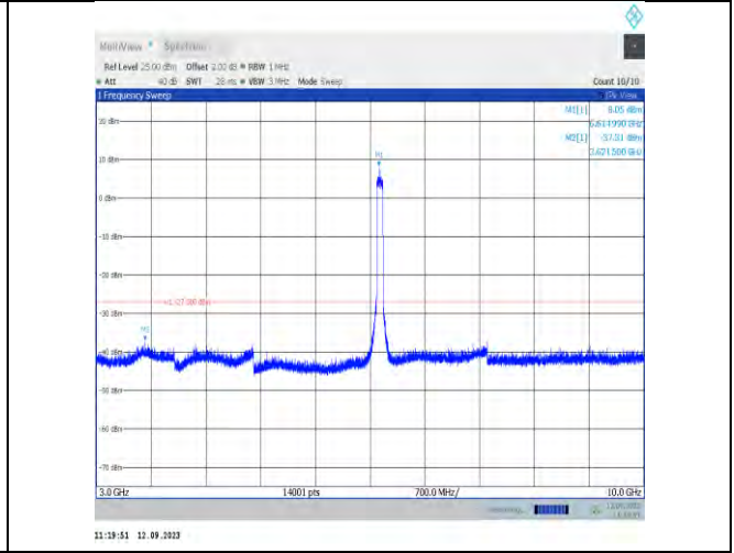
11ax80MIMO-Ant7-6625-3000~10000
