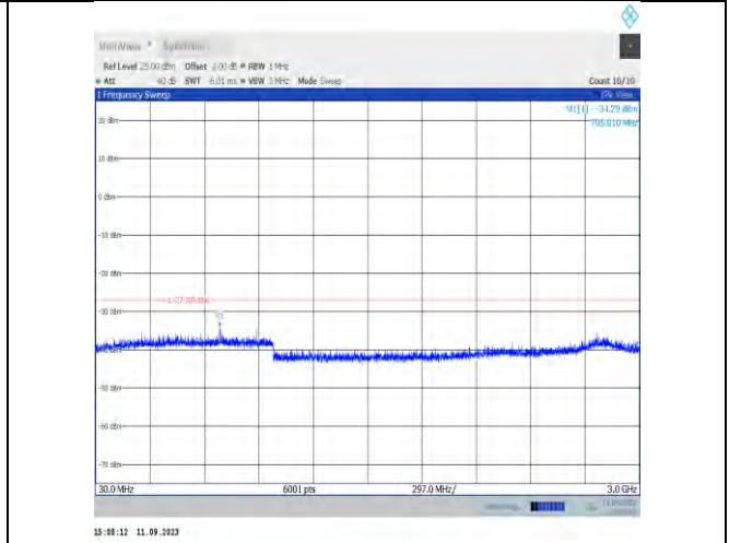
11ax40MIMO-Ant9-6845-30~3000
