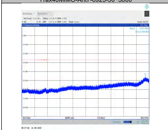
11ax40MIMO-Ant7-6925-10000~40000
