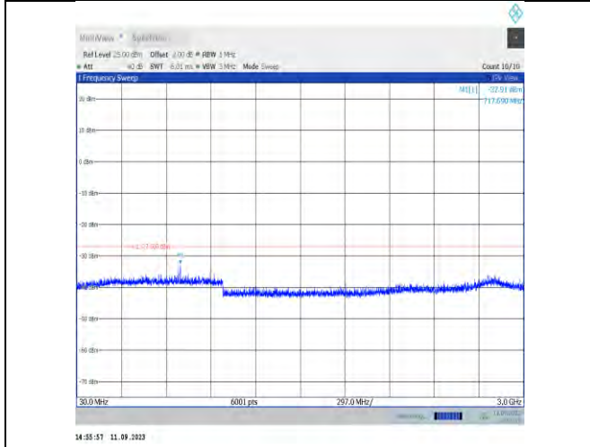
11ax40MIMO-Ant7-6845-30~3000
