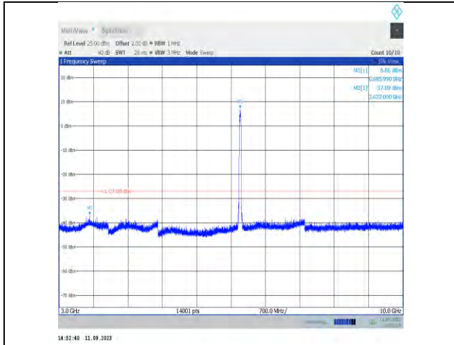
11ax40MIMO-Ant9-6685-3000~10000
