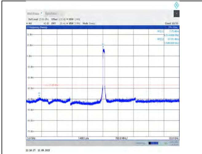
11ax80MIMO-Ant9-6545-3000~10000
