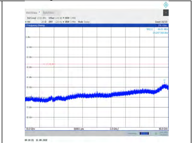
11ax40MIMO-Ant9-6885-10000~40000
