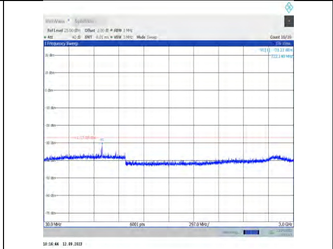
11ax40MIMO-Ant9-6965-30~3000
