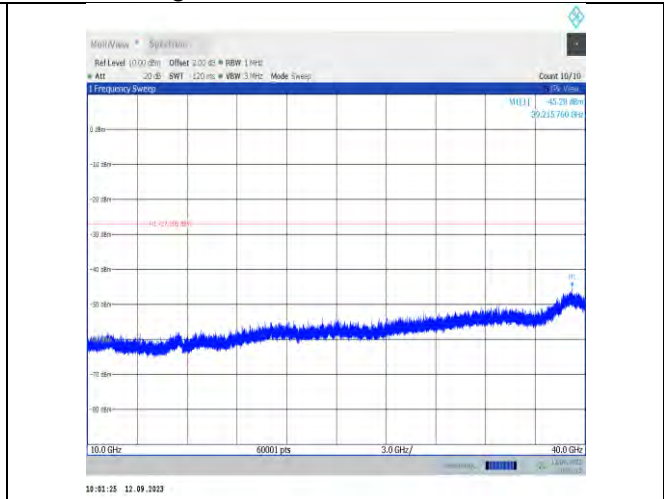
11ax40MIMO-Ant9-6925-10000~40000
