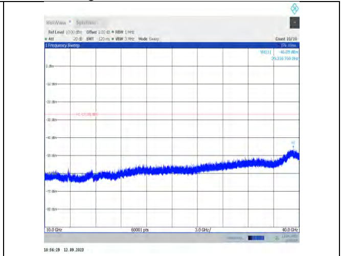
11ax80MIMO-Ant9-6385-10000~40000
