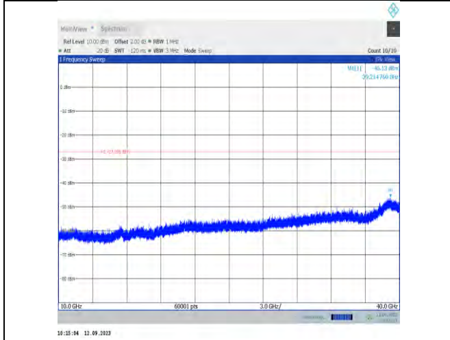
11ax40MIMO-Ant7-6965-10000~40000
