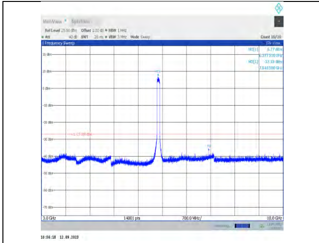
11ax80MIMO-Ant9-6385-3000~10000
