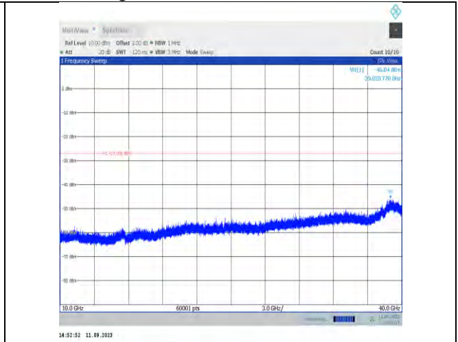
11ax40MIMO-Ant9-6685-10000~40000
