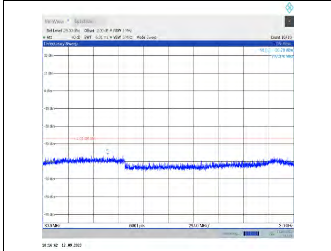
11ax40MIMO-Ant7-6965-30~3000
