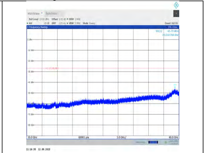
11ax80MIMO-Ant9-6545-10000~40000
