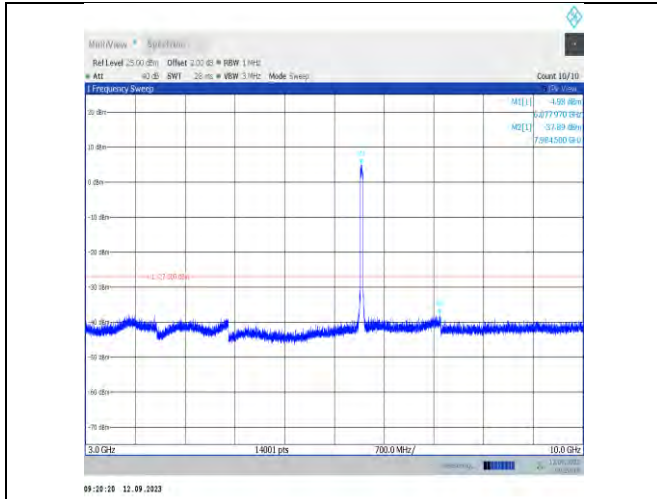
11ax40MIMO-Ant9-6885-3000~10000
