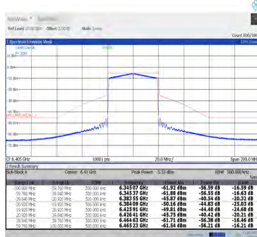
NTNV-11ax40MIMO-Ant9-6405-PASS
