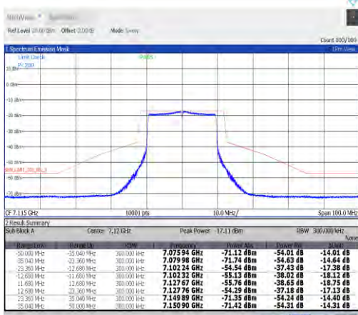
NTVN-11ax20MIMO-Ant7-7115-PASS
