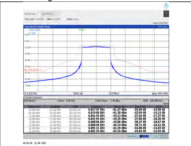
NTNV-11ax20MIMO-Ant9-6855-PASS
