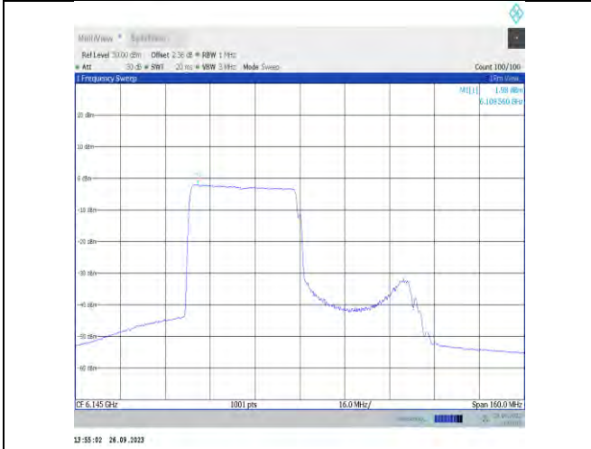
11ax80MIMO-Ant7-6145-PASS
