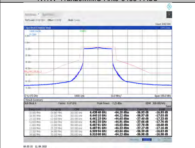
NTNV-11ax20MIMO-Ant9-6475-PASS
