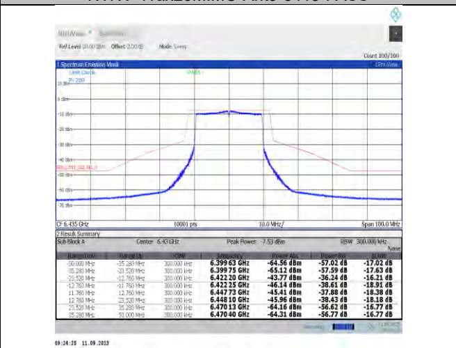
NTNV-11ax20MIMO-Ant9-6435-PASS
