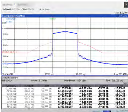
NTNV-11ax40MIMO-Ant7-6165-PASS
