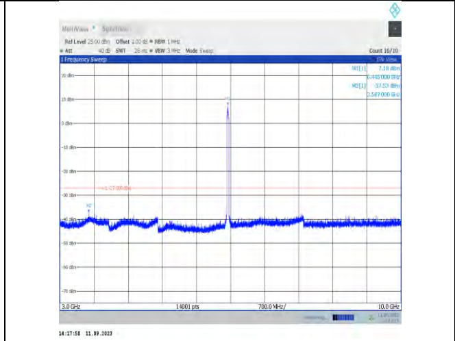
11ax40MIMO-Ant7-6445-3000~10000
