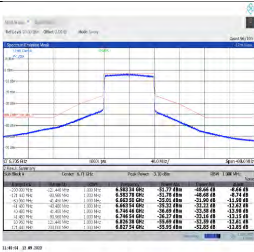
NTVN-11ax80MIMO-Ant7-6705-PASS
