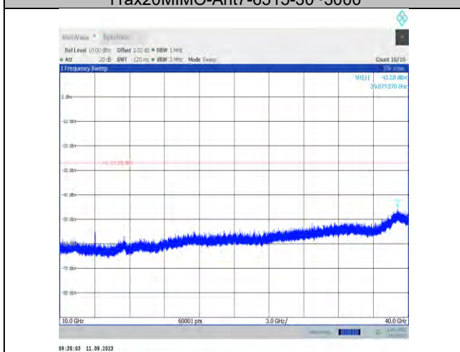
11ax20MIMO-Ant7-6515-10000~40000
