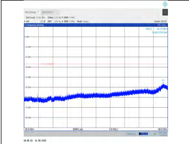
11ax40MIMO-Ant7-6405-10000~40000
