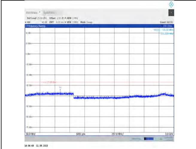
11ax40MIMO-Ant7-6405-30~3000
