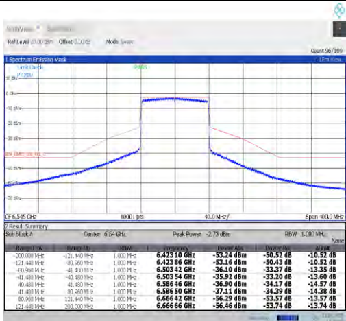
NTVN-11ax80MIMO-Ant7-6545-PASS
