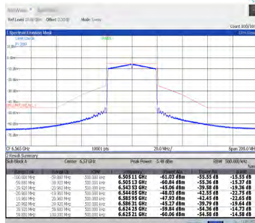
NTVN-11ax40MIMO-Ant9-6565-PASS
