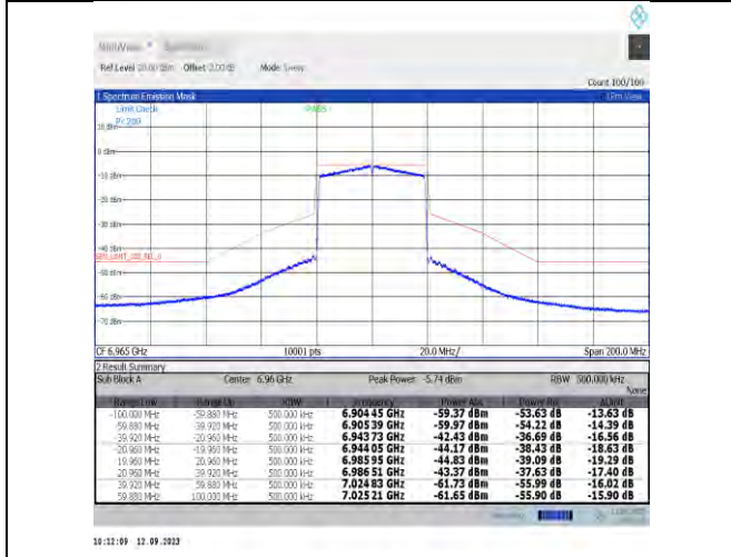
NTVN-11ax40MIMO-Ant7-6965-PASS
