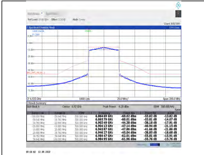
NTVN-11ax40MIMO-Ant7-6925-PASS
