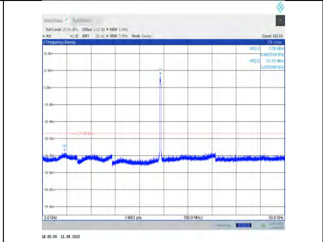
11ax40MIMO-Ant7-6405-3000~10000
