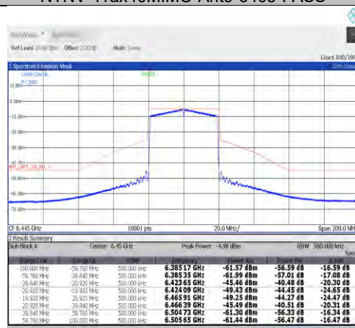
NTNV-11ax40MIMO-Ant9-6445-PASS
