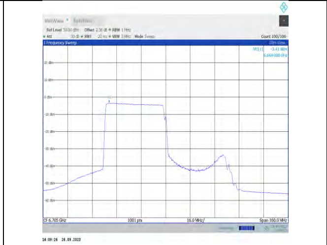
11x80MIMO-Ant9-6705-PASS
