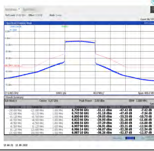
NTVN-11ax80MIMO-Ant9-6865-PASS
