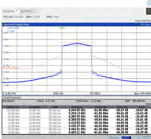
NTNV-11ax40MIMO-Ant7-6405-PASS
