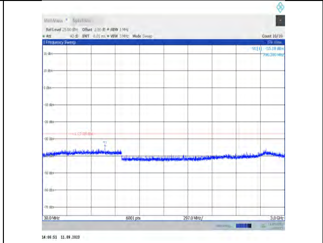
11ax40MIMO-Ant9-6405-30~3000
