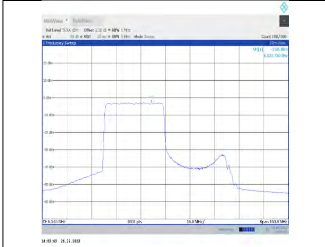
11x80MIMO-Ant7-6545-PASS
