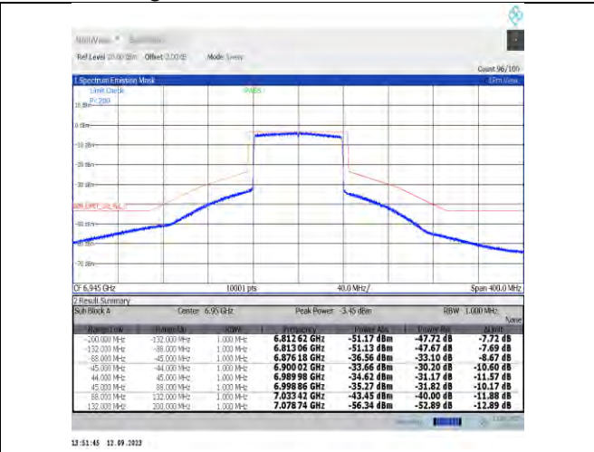
NTVN-11ax80MIMO-Ant9-6945-PASS
