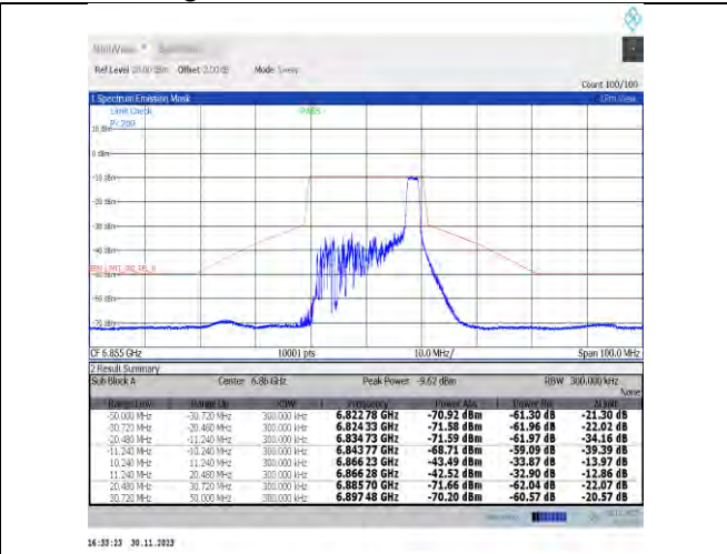
NTNV-11ax20MIMO-Ant9-6855-26Tone-RU8-PASS
