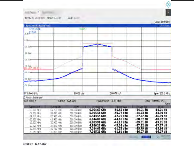
NTVN-11ax40MIMO-Ant9-6965-PASS
