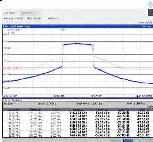
NTVN-11ax80MIMO-Ant9-6545-PASS
