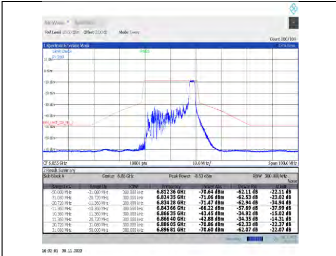
NTNV-11ax20MIMO-Ant7-6855-26Tone-RU8-PASS
