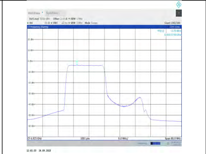
11ax40MIMO-Ant9-6925-PASS
