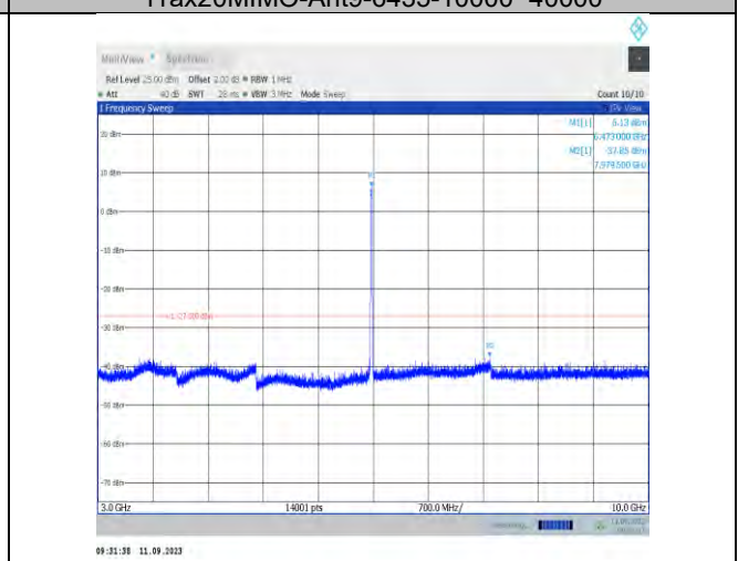
11ax20MIMO-Ant7-6475-3000~10000
