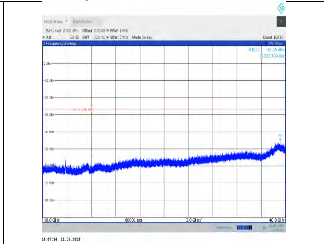
11ax40MIMO-Ant9-6405-10000~40000
