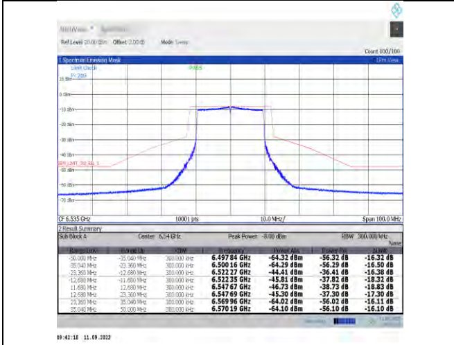
NTNV-11ax20MIMO-Ant7-6535-PASS
