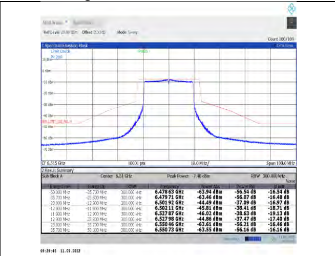
NTNV-11ax20MIMO-Ant9-6515-PASS
