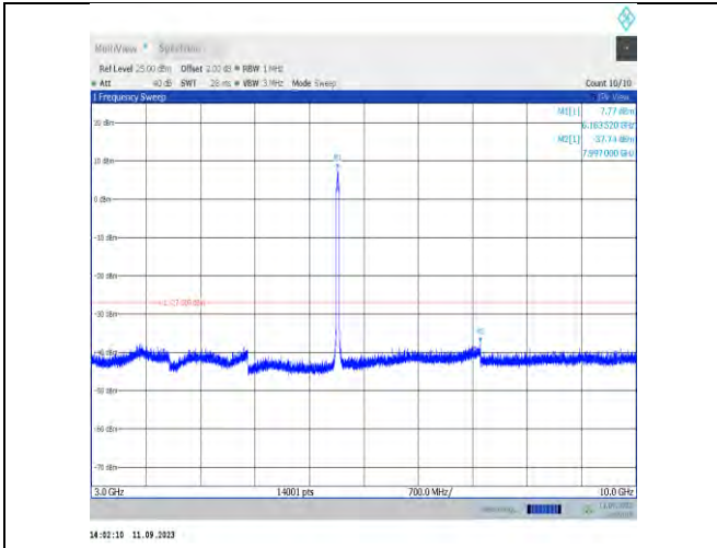
11ax40MIMO-Ant9-6165-3000~10000
