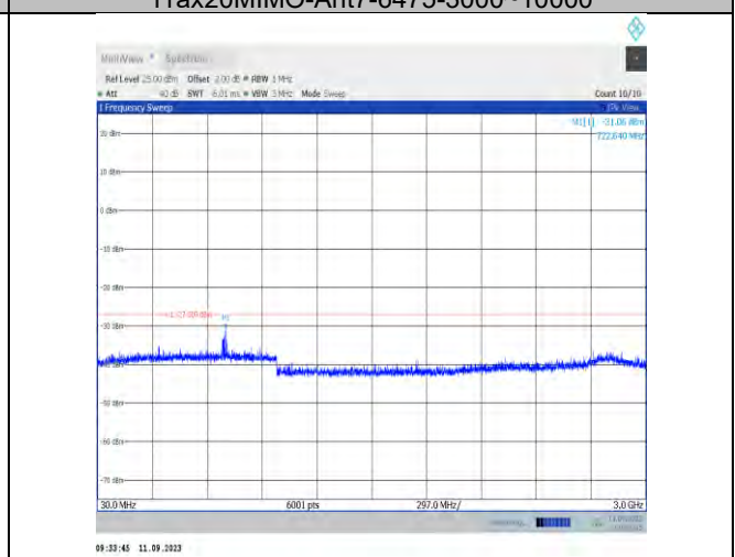
11ax20MIMO-Ant9-6475-30~3000
