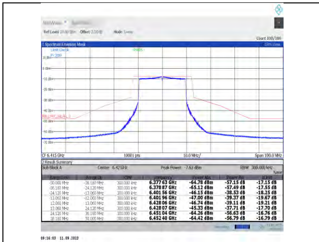
NTNV-11ax20MIMO-Ant7-6415-PASS
