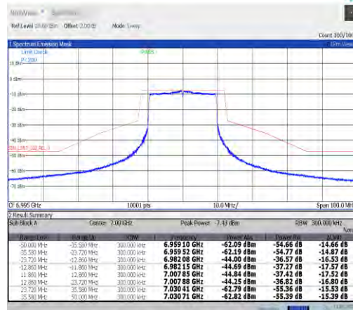
NTVN-11ax20MIMO-Ant9-6995-PASS
