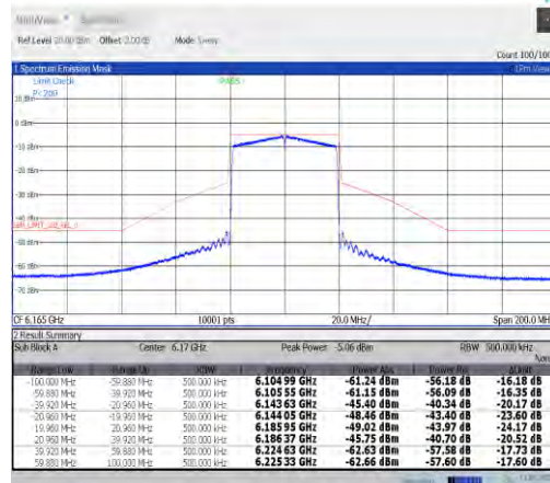
NTNV-11ax40MIMO-Ant9-6165-PASS
