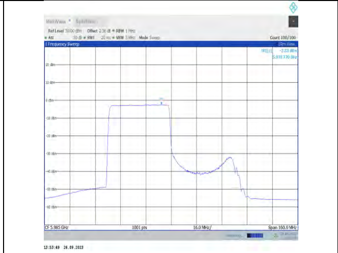
11ax80MIMO-Ant9-5985-PASS
