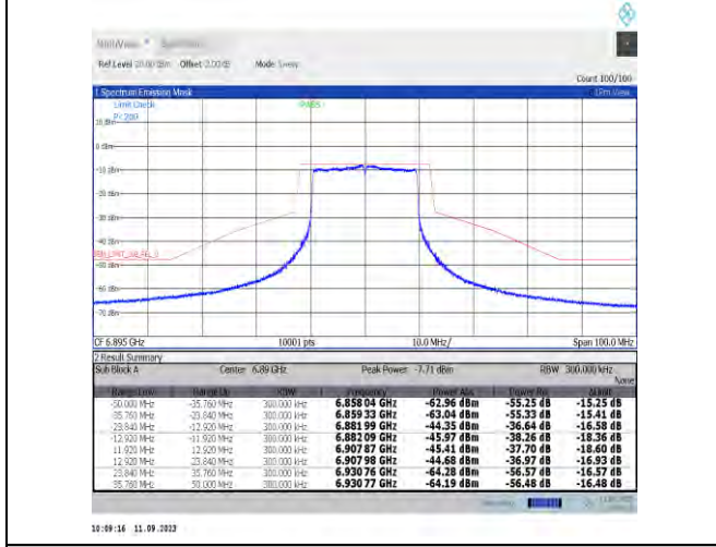
NTNV-11ax20MIMO-Ant7-6895-PASS
