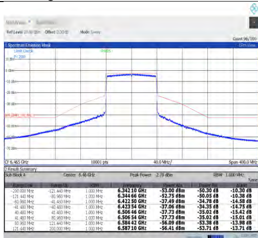
NTVN-11ax80MIMO-Ant9-6465-PASS
