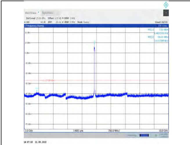
11ax40MIMO-Ant9-6405-3000~10000
