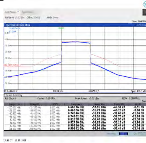
NTVN-11ax80MIMO-Ant9-6785-PASS
