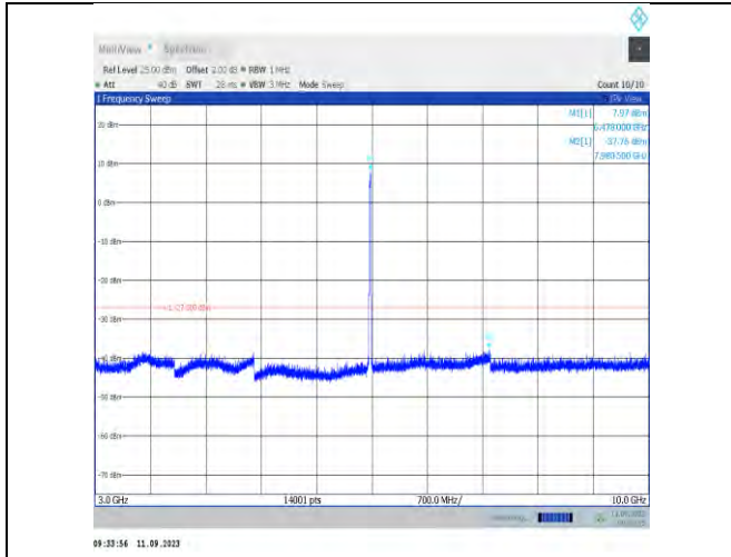
11ax20MIMO-Ant9-6475-3000~10000
