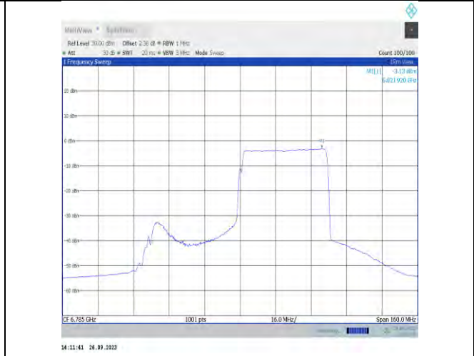
11x80MIMO-Ant9-6785-PASS
