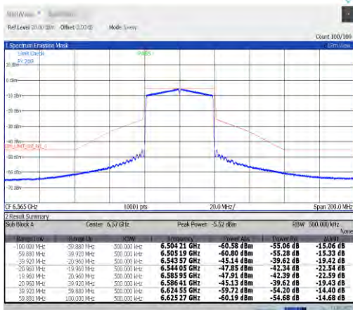
NTVN-11ax40MIMO-Ant7-6565-PASS
