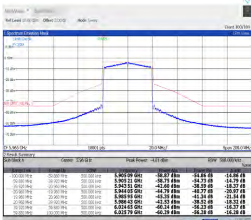
NTVN-11ax40MIMO-Ant7-5965-PASS
