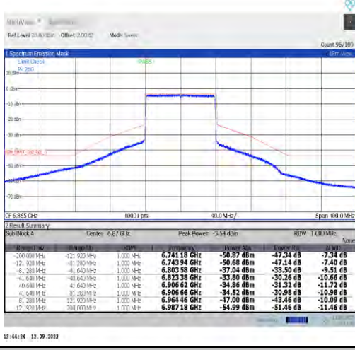
NTVN-11ax80MIMO-Ant7-6865-PASS
