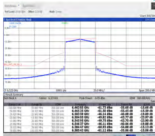
NTVN-11ax40MIMO-Ant9-6525-PASS
