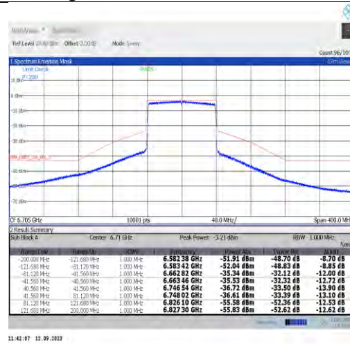
NTVN-11ax80MIMO-Ant9-6705-PASS
