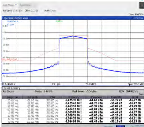
NTVN-11ax40MIMO-Ant7-6485-PASS
