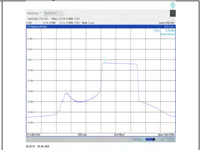
11ax80MIMO-Ant9-6865-PASS
