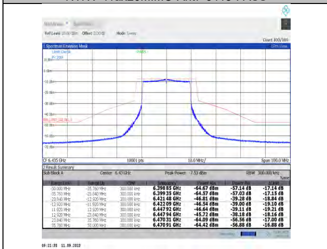
NTNV-11ax20MIMO-Ant7-6435-PASS
