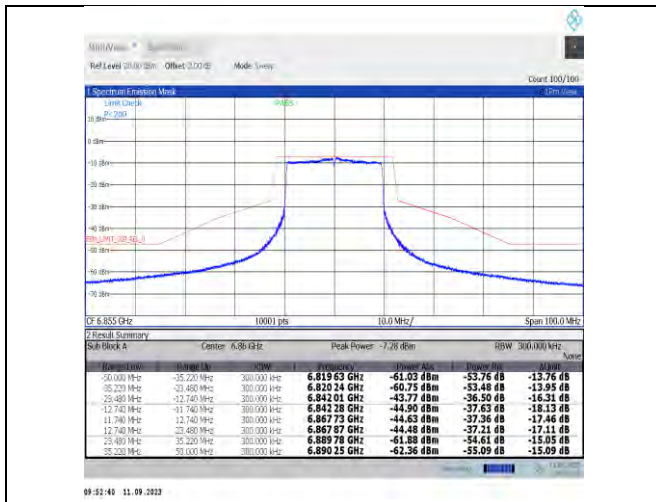
NTNV-11ax20MIMO-Ant7-6855-PASS
