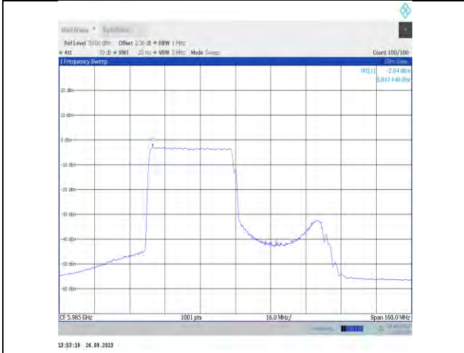
11ax80MIMO-Ant7-5985-PASS
