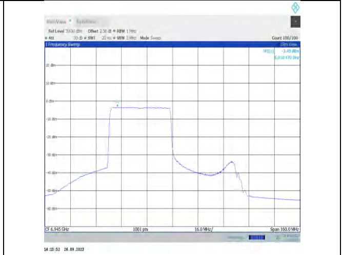
11ax80MIMO-Ant9-6945-PASS
