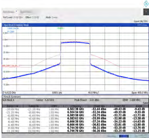
NTVN-11ax80MIMO-Ant7-6625-PASS
