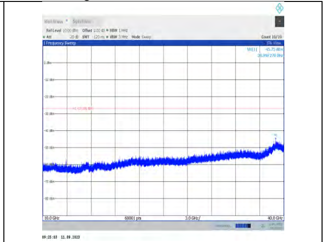
11ax20MIMO-Ant9-6435-10000~40000
