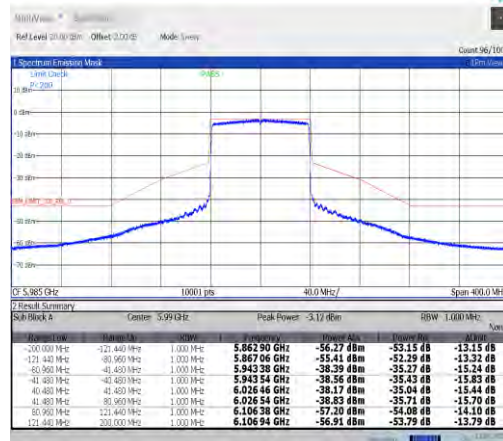
NTVN-11ax80MIMO-Ant9-5985-PASS
