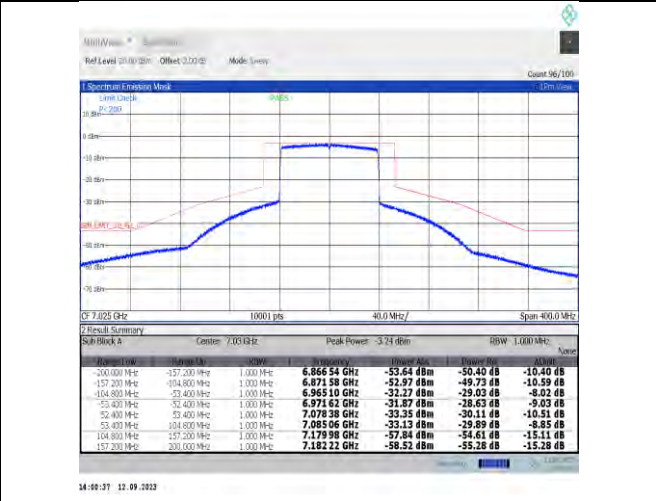
NTVN-11ax80MIMO-Ant9-7025-PASS
