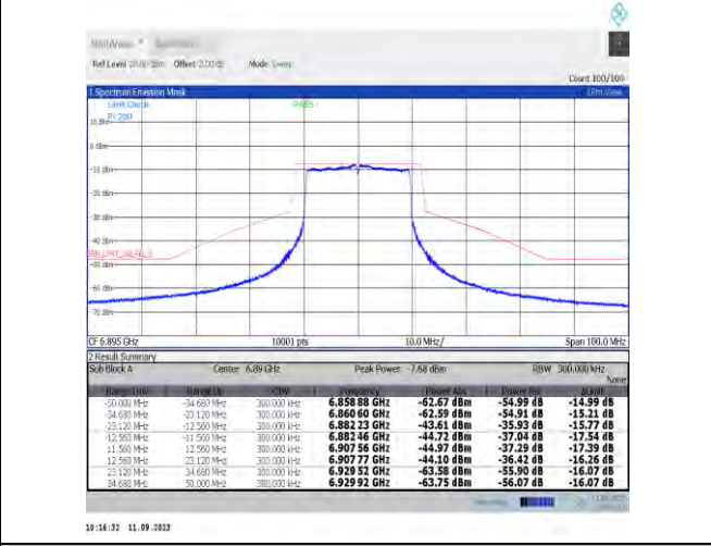
NTNV-11ax20MIMO-Ant9-6895-PASS
