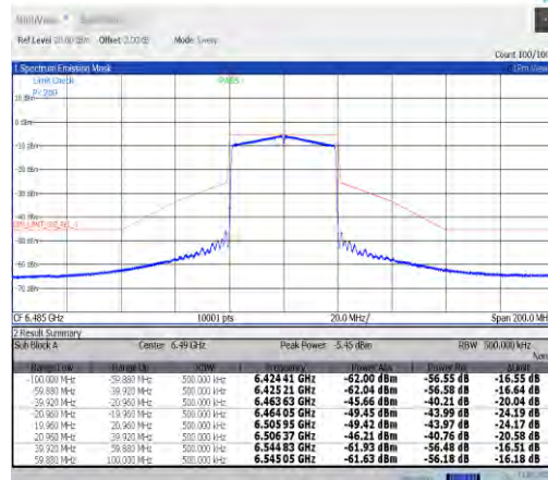
NTVN-11ax40MIMO-Ant9-6485-PASS
