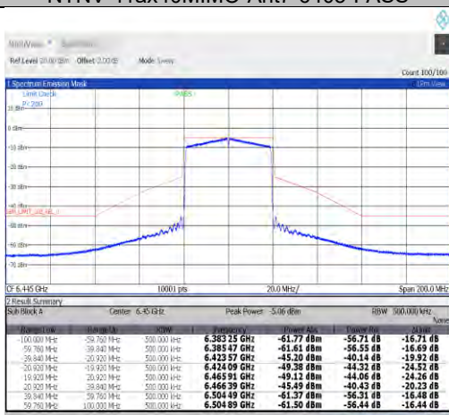
NTNV-11ax40MIMO-Ant7-6445-PASS
