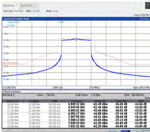
NTVN-11ax20MIMO-Ant7-6995-PASS
