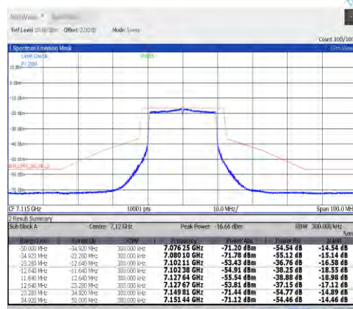
NTVN-11ax20MIMO-Ant9-7115-PASS
