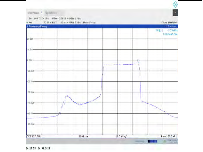
11ax80MIMO-Ant9-7025-PASS
