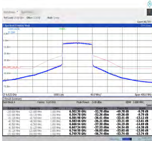
NTVN-11ax80MIMO-Ant9-6625-PASS
