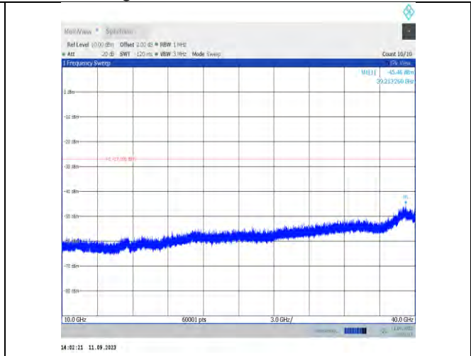
11ax40MIMO-Ant9-6165-10000~40000
