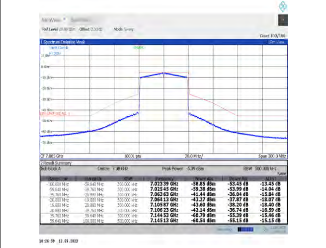
NTVN-11ax40MIMO-Ant9-7085-PASS
