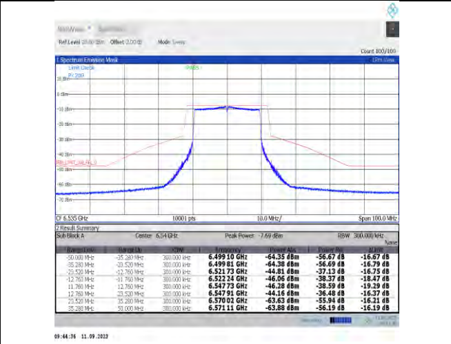
NTNV-11ax20MIMO-Ant9-6535-PASS
