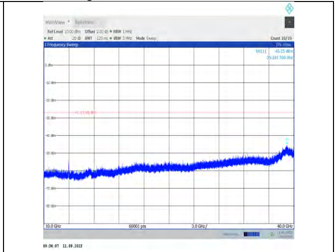
11ax20MIMO-Ant9-6475-10000~40000
