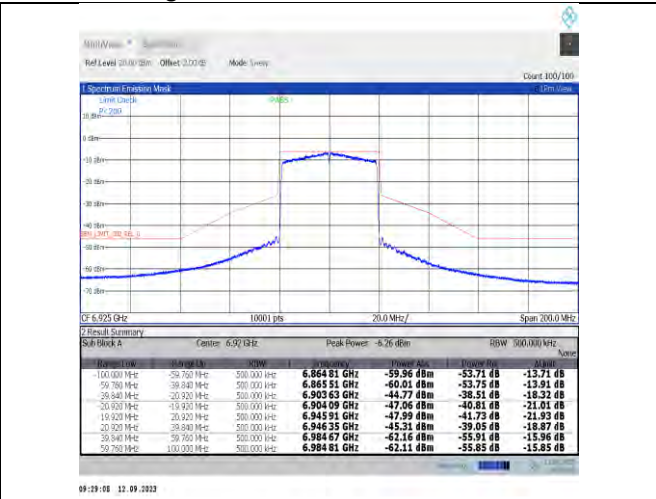
NTVN-11ax40MIMO-Ant9-6925-PASS
