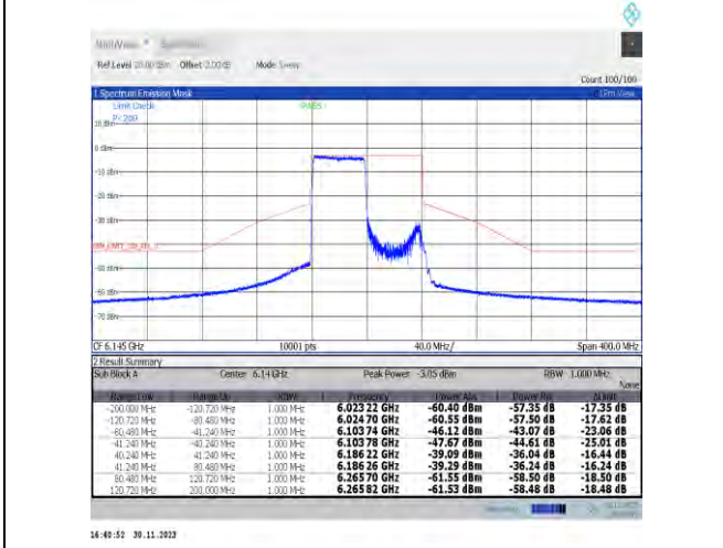
NTNV-11ax80MIMO-Ant7-6145-484Tone-RU65-PASS
