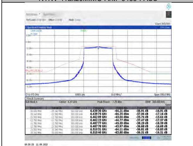
NTNV-11ax20MIMO-Ant7-6475-PASS
