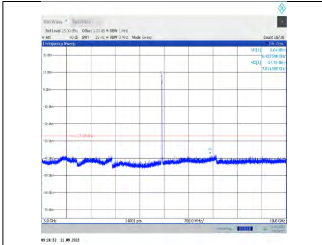
11ax20MIMO-Ant9-6435-3000~10000
