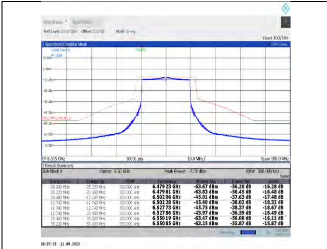
NTNV-11ax20MIMO-Ant7-6515-PASS
