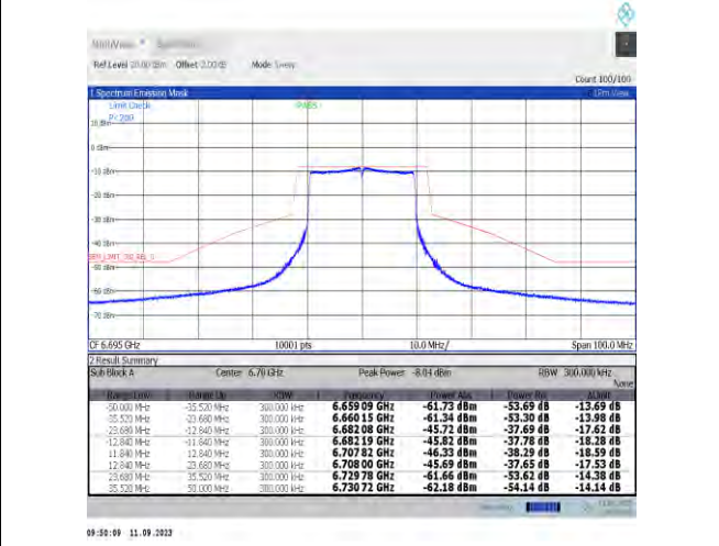
NTNV-11ax20MIMO-Ant9-6695-PASS
