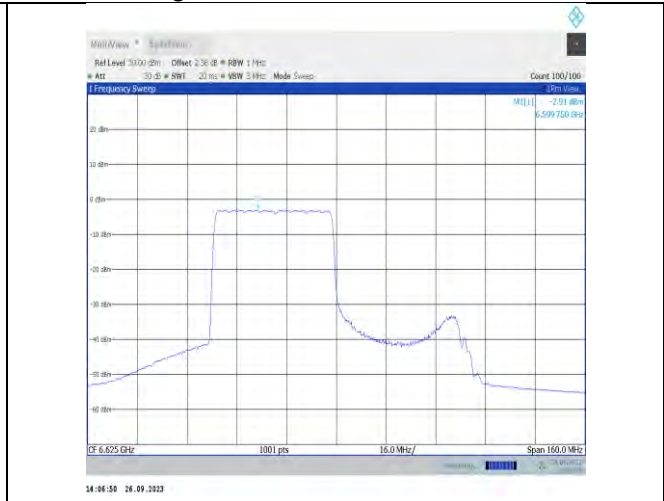
11x80MIMO-Ant9-6625-PASS
