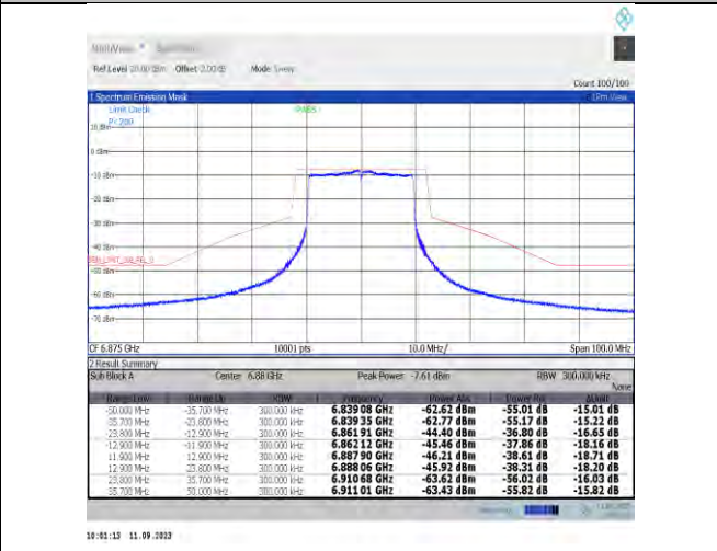
NTNV-11ax20MIMO-Ant9-6875-PASS
