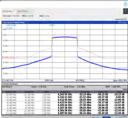
NTVN-11ax80MIMO-Ant7-6465-PASS
