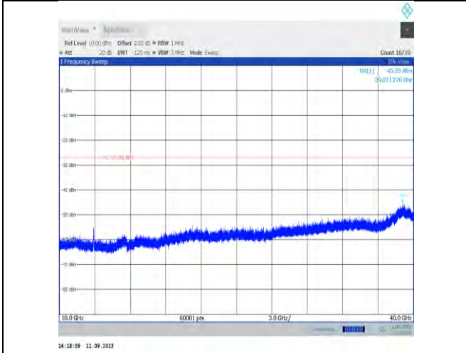
11ax40MIMO-Ant7-6445-10000~40000
