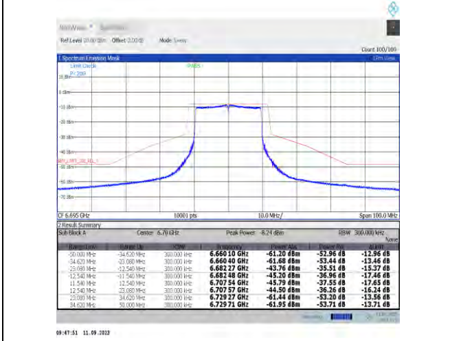
NTNV-11ax20MIMO-Ant7-6695-PASS
