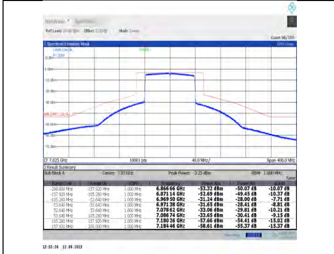
NTVN-11ax80MIMO-Ant7-7025-PASS
