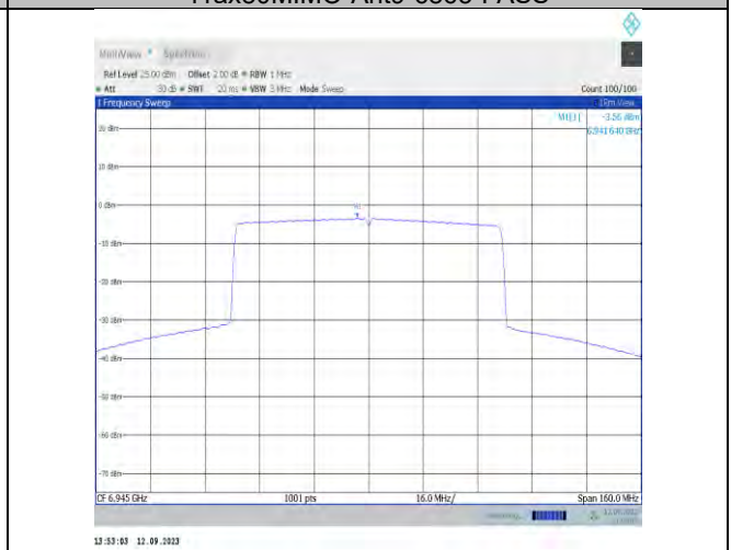
11ax80MIMO-Ant9-6945-PASS
