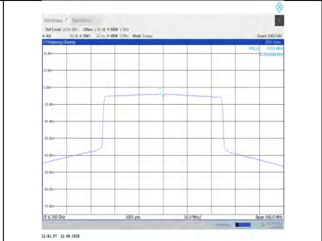
11ax80MIMO-Ant9-6705-PASS
