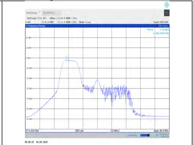
11x20MIMO-Ant7-6435-PASS
