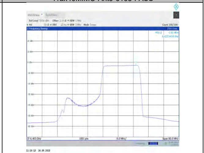
11ax40MIMO-Ant9-6405-PASS
