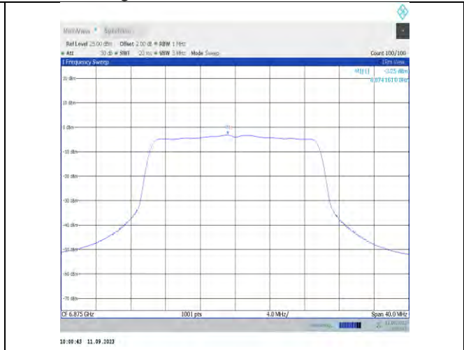
11x20MIMO-Ant9-6875-PASS
