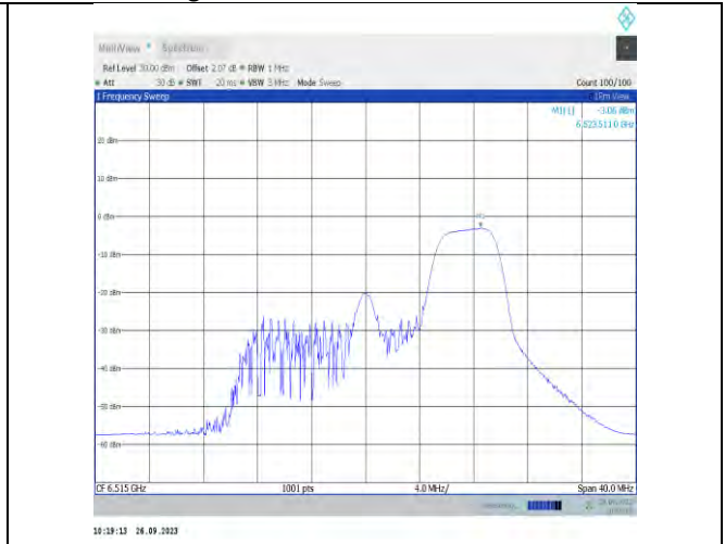
11ax20MIMO-Ant7-6515-PASS
