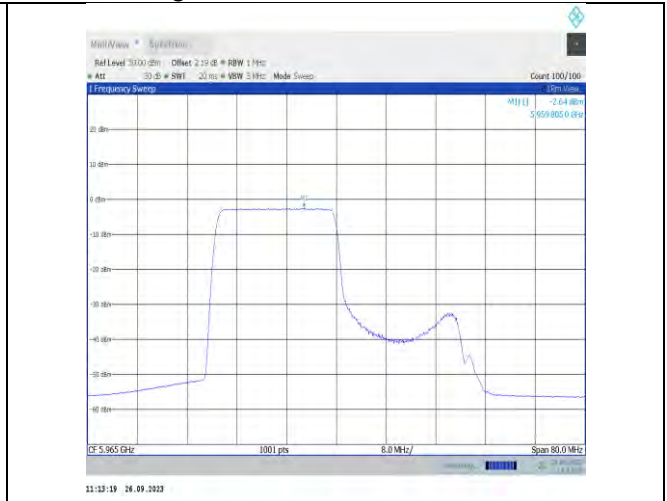
11ax40MIMO-Ant9-5965-PASS
