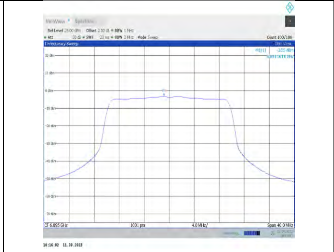
11x20MIMO-Ant9-6895-PASS
