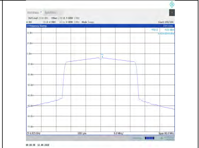
11ax40MIMO-Ant9-6925-PASS
