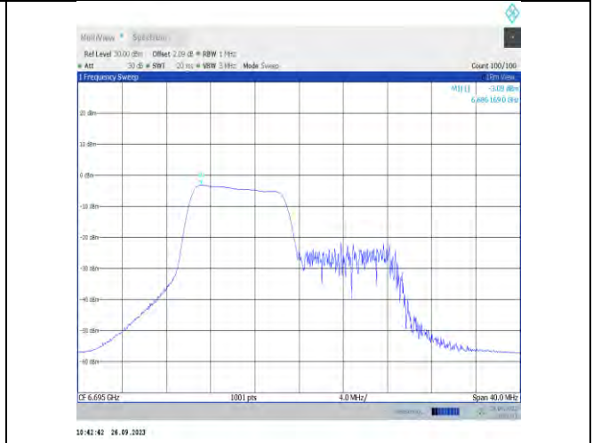
11ax20MIMO-Ant9-6695-PASS
