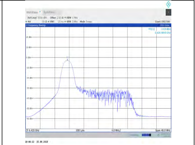
11x20MIMO-Ant9-6435-PASS
