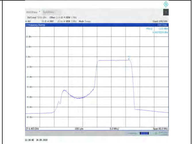
11ax40MIMO-Ant9-6485-PASS
