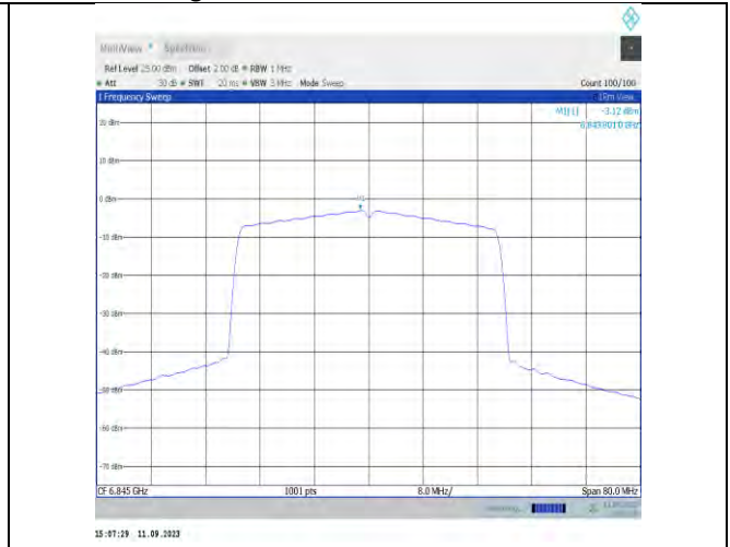
11ax40MIMO-Ant9-6845-PASS
