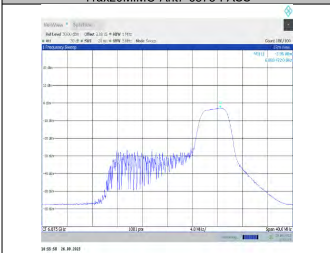
11ax20MIMO-Ant9-6875-PASS
