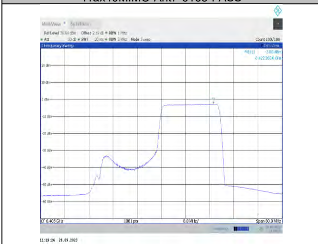
11ax40MIMO-Ant7-6405-PASS
