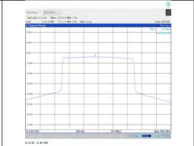
11ax80MIMO-Ant9-6625-PASS
