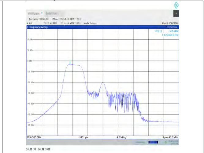
11x20MIMO-Ant7-6535-PASS
