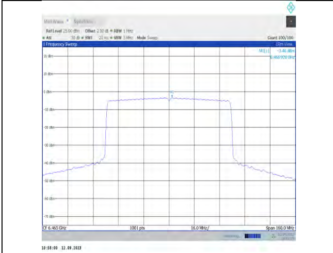
11ax80MIMO-Ant7-6465-PASS
