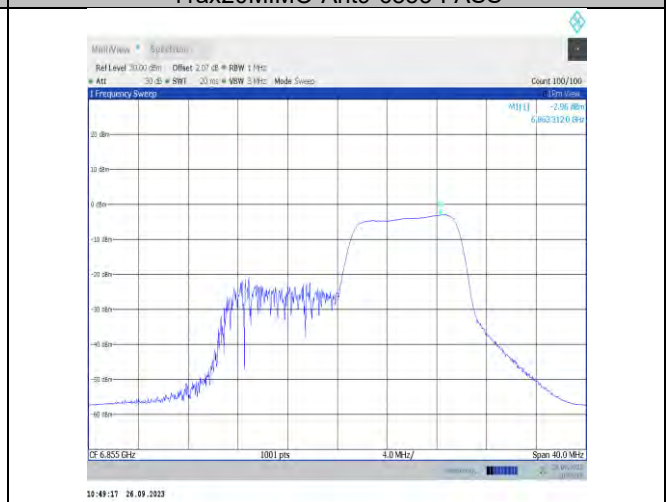
11ax20MIMO-Ant9-6855-PASS
