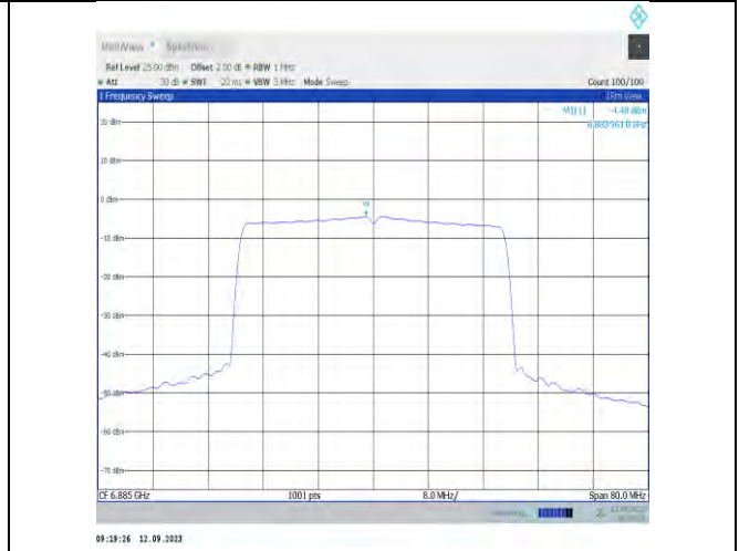
11ax40MIMO-Ant9-6885-PASS
