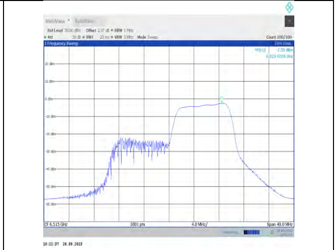
11ax20MIMO-Ant9-6515-PASS
