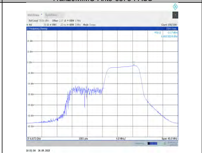
11ax20MIMO-Ant9-6875-PASS
