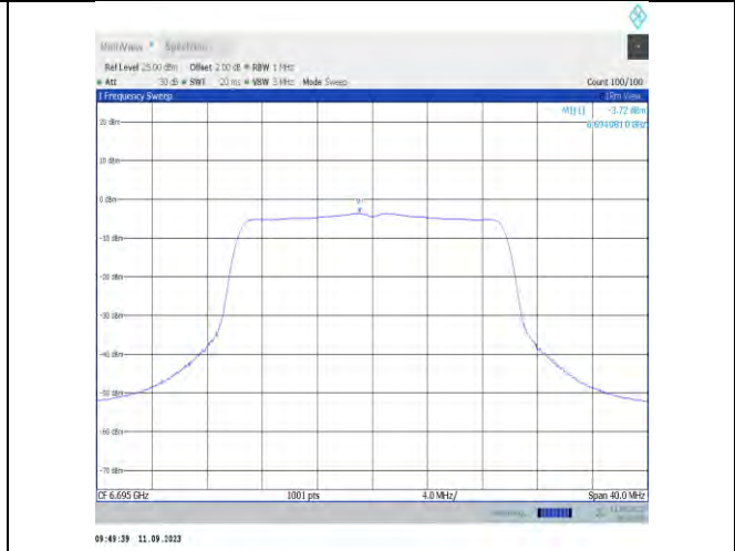
11x20MIMO-Ant9-6695-PASS
