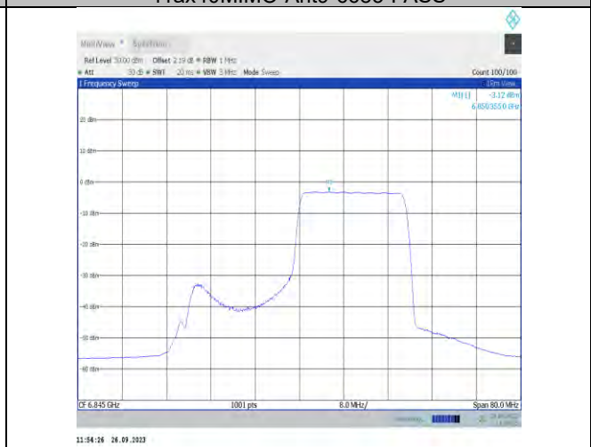
11ax40MIMO-Ant9-6845-PASS
