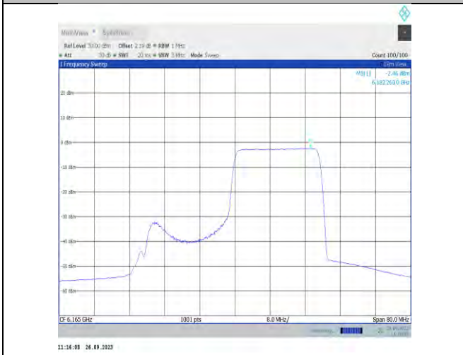
11ax40MIMO-Ant7-6165-PASS
