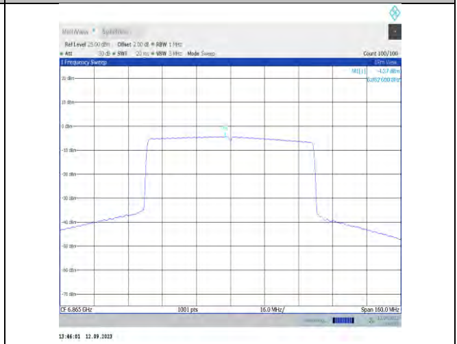
11ax80MIMO-Ant9-6865-PASS
