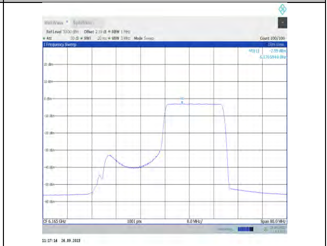
11ax40MIMO-Ant9-6165-PASS
