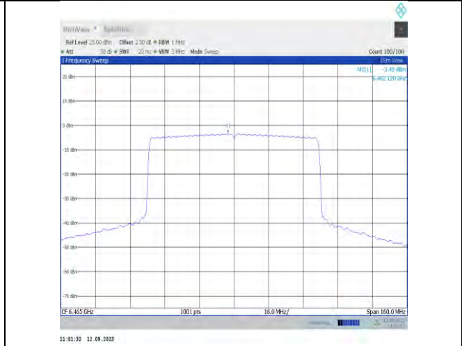
11ax80MIMO-Ant9-6465-PASS
