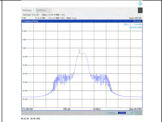
11ax20MIMO-Ant9-6995-PASS
