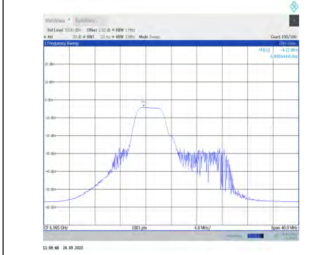
11ax20MIMO-Ant9-6995-PASS
