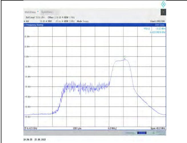
11ax20MIMO-Ant9-6415-PASS
