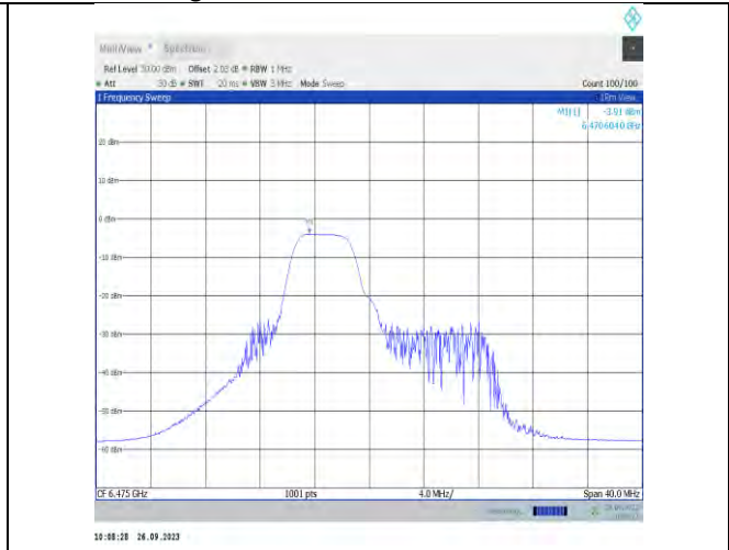
11ax20MIMO-Ant7-6475-PASS
