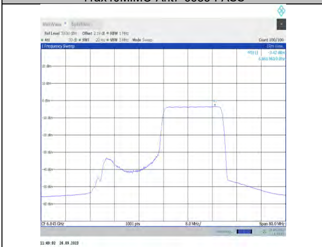
11ax40MIMO-Ant7-6845-PASS
