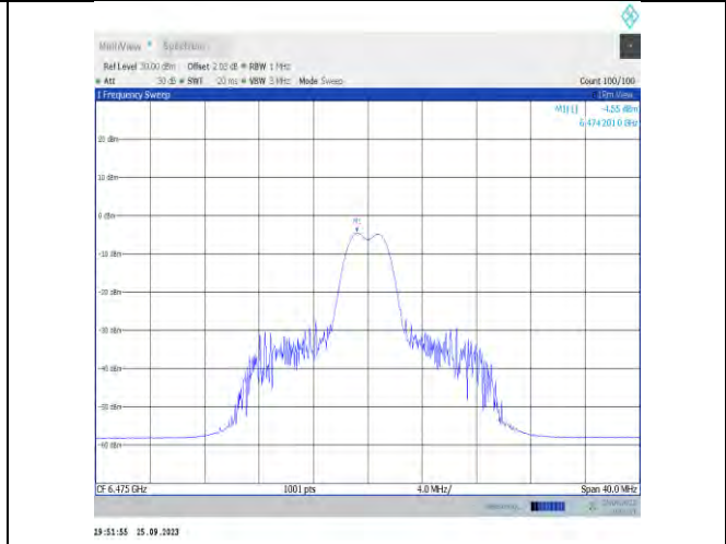
11ax20MIMO-Ant9-6475-PASS
