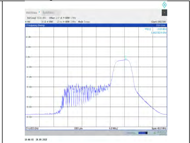
11ax20MIMO-Ant7-6855-PASS
