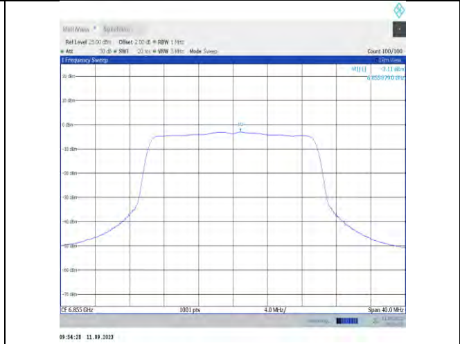
11x20MIMO-Ant9-6855-PASS
