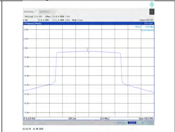
11ax80MIMO-Ant9-6545-PASS
