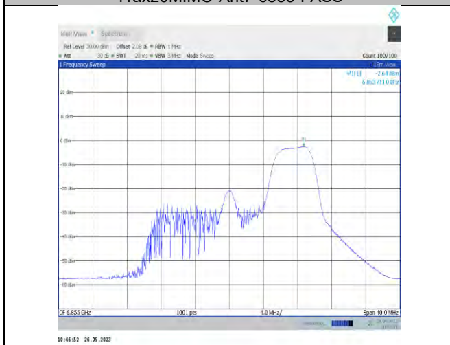
11ax20MIMO-Ant9-6855-PASS
