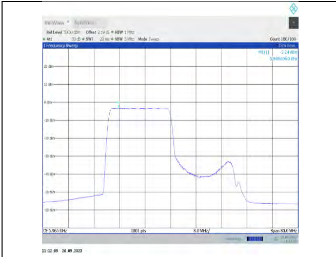
11ax40MIMO-Ant7-5965-PASS
