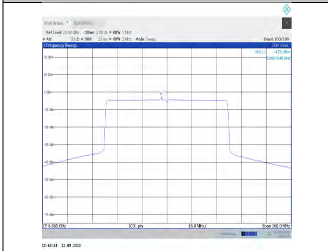
11ax80MIMO-Ant7-6865-PASS
