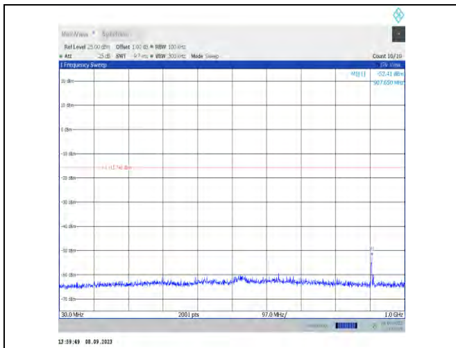
11ax20MIMO-Ant7-2437-30~1000-PASS
