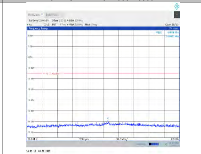
11ax20MIMO-Ant9-2437-30~1000-PASS
