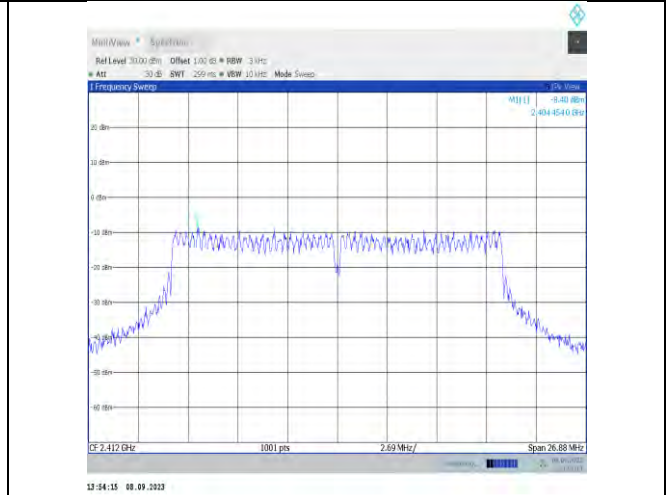
11ax20MIMO-Ant7-2412-PASS
