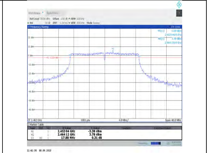
11n20MIMO-Ant9-2462-PASS
