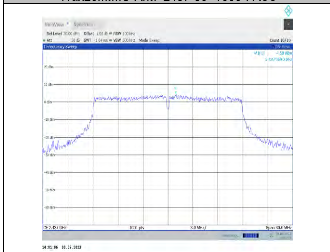
11ax20MIMO-Ant9-2437-0~Reference-PASS
