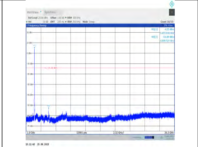
11g-Ant9-2417-1000~26500-PASS
