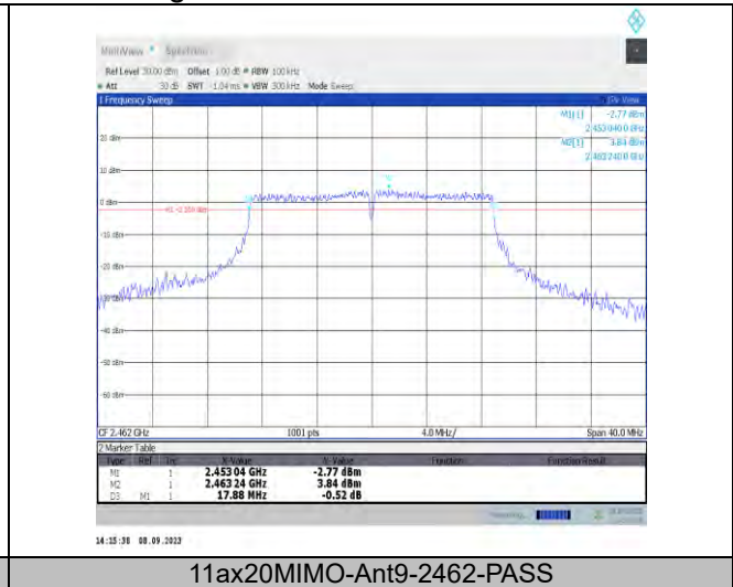
11ax20MIMO-Ant9-2462-PASS
