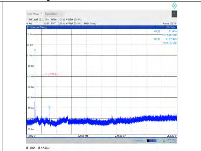
11n20MIMO-Ant7-2417-1000~26500-PASS
