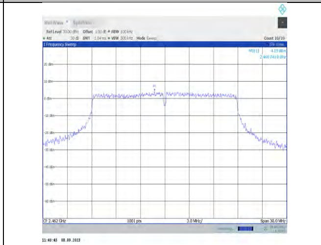
11n20MIMO-Ant7-2462-0~Reference-PASS
