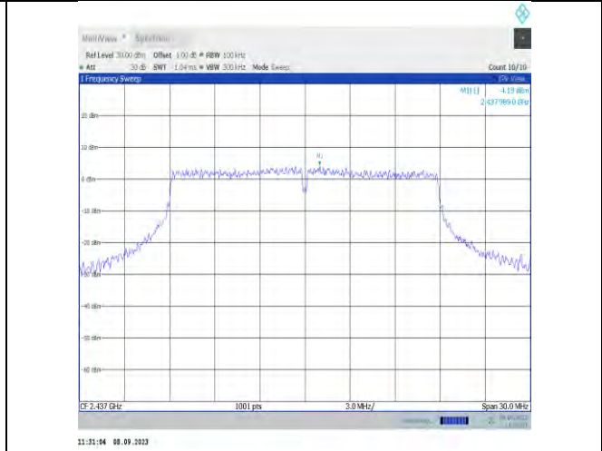
11n20MIMO-Ant7-2437-0~Reference-PASS
