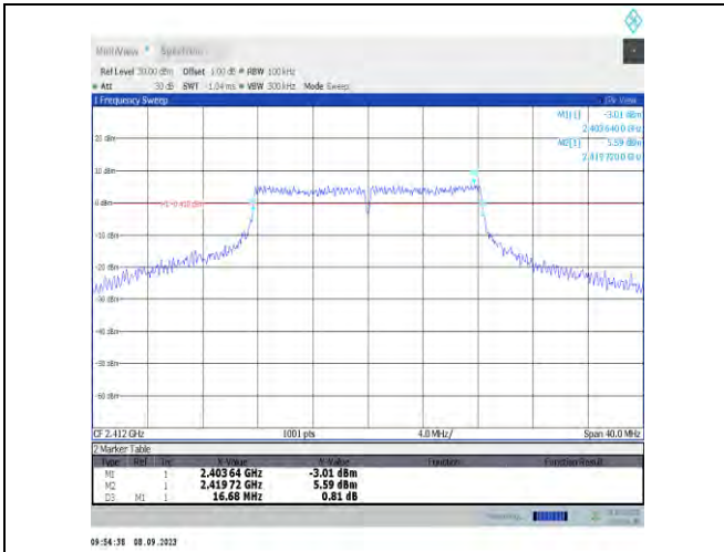
11g-Ant9-2412-PASS
