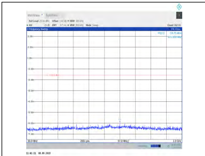
11n20MIMO-Ant7-2462-30~1000-PASS
