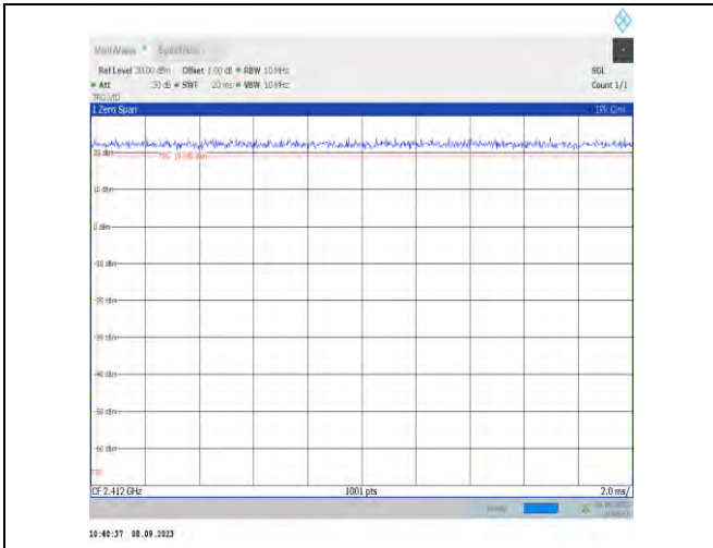
NTVN-11n20MIMO-Ant7-2412
