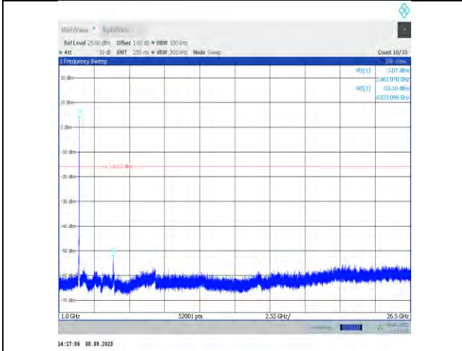
11ax20MIMO-Ant9-2462-1000~26500-PASS
