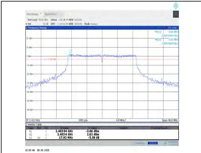
11x20MIMO-Ant7-2412-PASS
