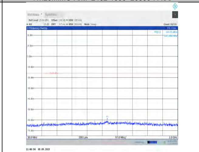
11n20MIMO-Ant9-2462-30~1000-PASS
