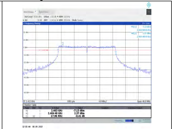
11x20MIMO-Ant9-2412-PASS
