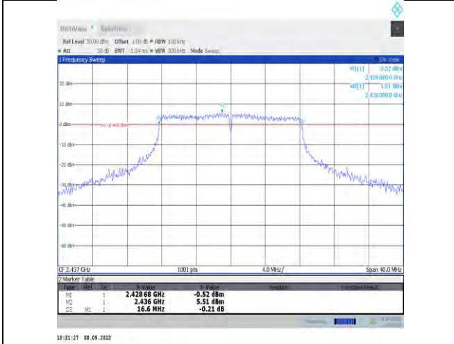
11g-Ant9-2437-PASS
