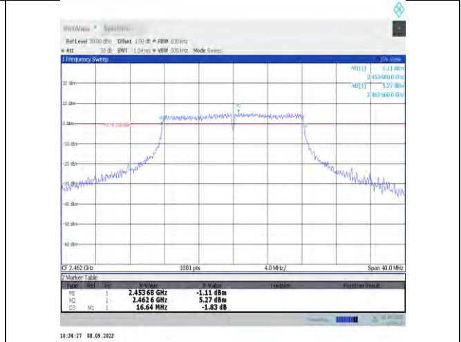
11g-Ant9-2462-PASS
