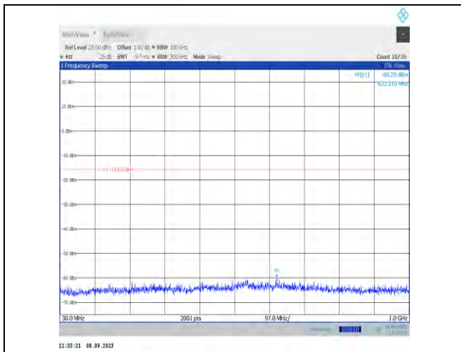
11n20MIMO-Ant7-2437-30~1000-PASS
