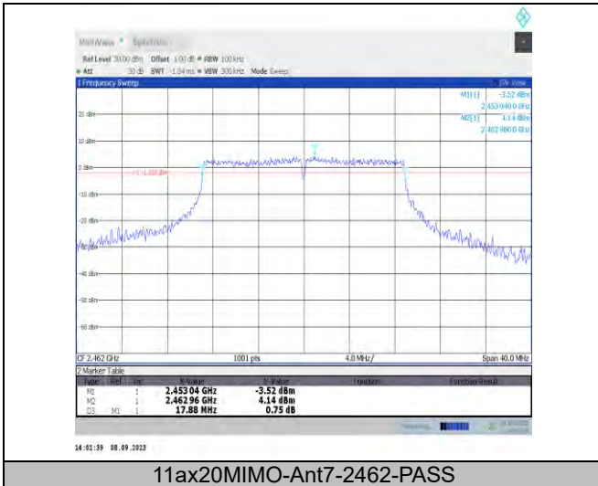
11ax20MIMO-Ant7-2462-PASS
