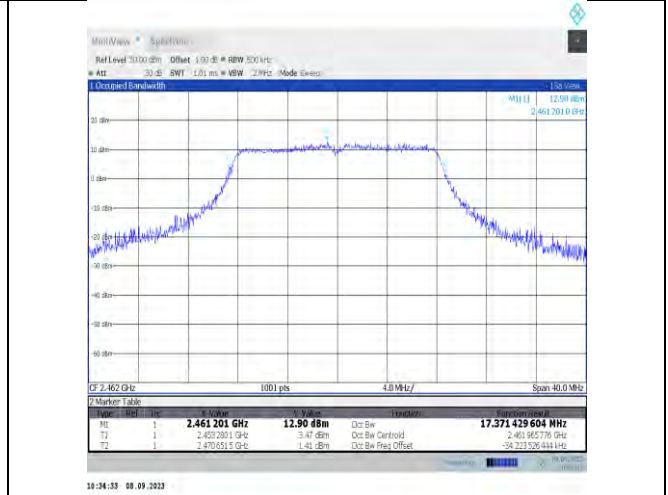
11g-Ant9-2462
