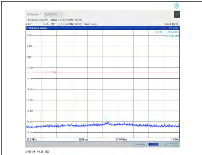
11g-Ant9-2437-30~1000-PASS
