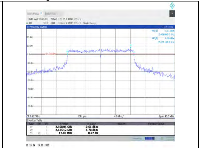
11n20MIMO-Ant9-2417-PASS
