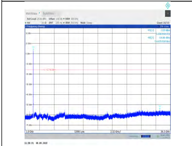
11n20MIMO-Ant9-2437-1000~26500-PASS
