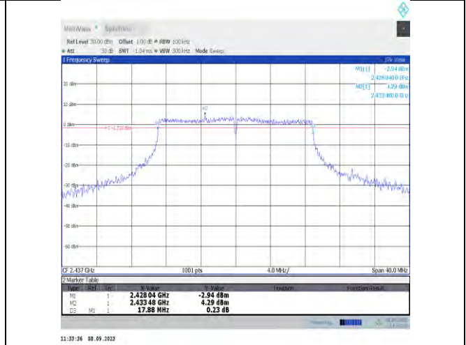
11n20MIMO-Ant9-2437-PASS
