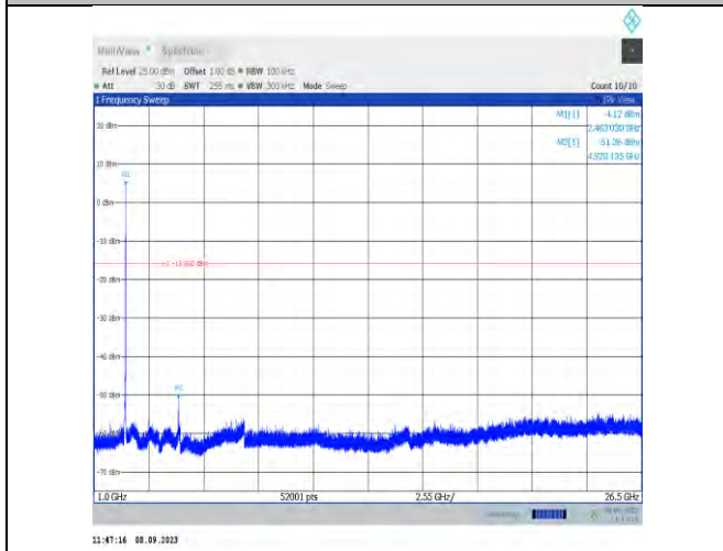
11n20MIMO-Ant9-2462-1000~26500-PASS
