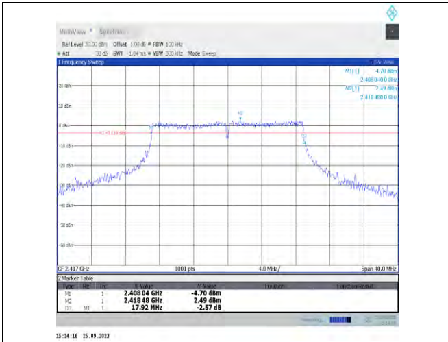
11n20MIMO-Ant7-2417-PASS
