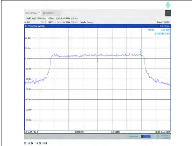
11ax20MIMO-Ant9-2457-0~Reference-PASS
