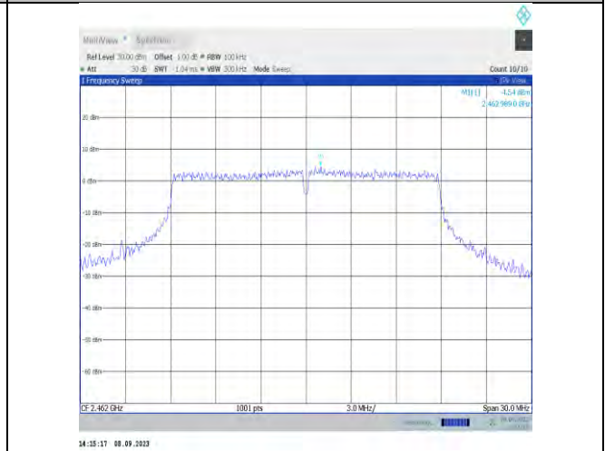
11ax20MIMO-Ant7-2462-0~Reference-PASS
