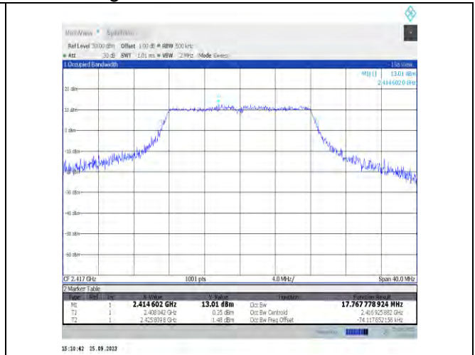
11g-Ant9-2417
