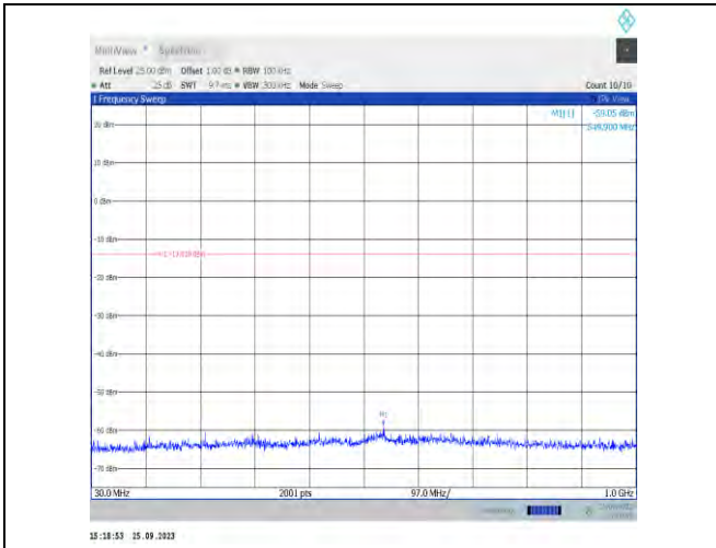
11ax20MIMO-Ant7-2457-30~1000-PASS
