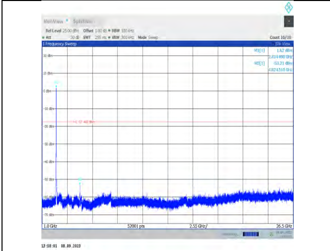
11ax20MIMO-Ant9-2412-1000~26500-PASS
