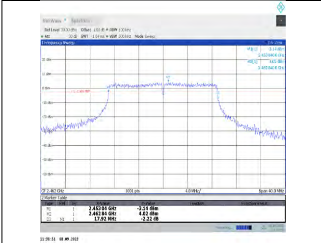
11n20MIMO-Ant7-2462-PASS
