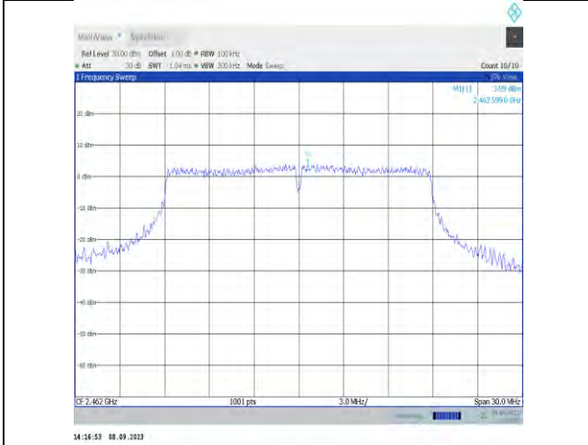
11ax20MIMO-Ant9-2462-0~Reference-PASS
