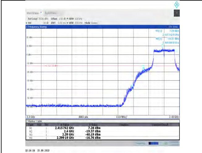
11n20MIMO-Ant9-2417-PASS
