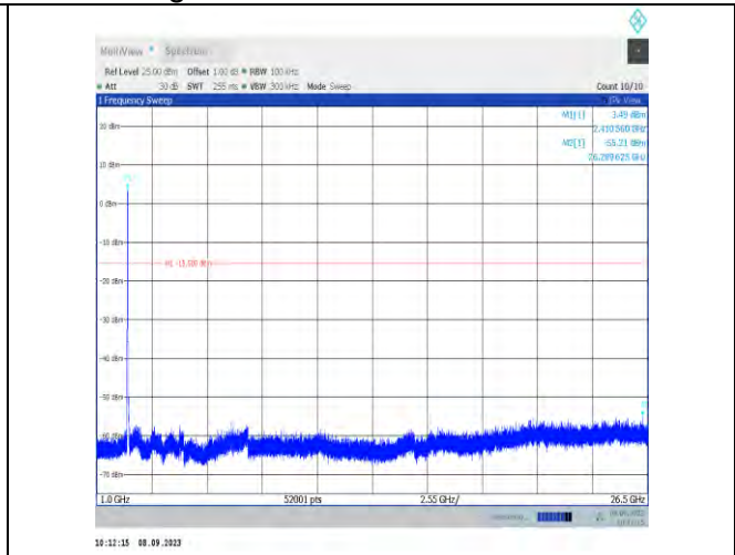
11g-Ant9-2412-1000~26500-PASS
