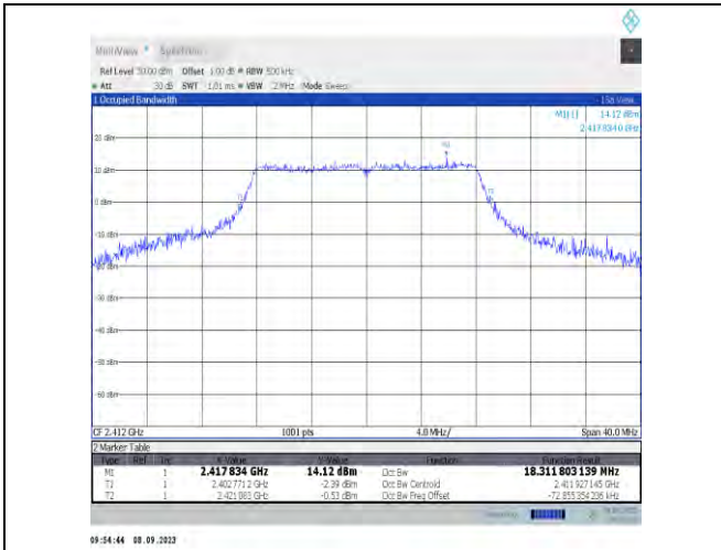
11g-Ant9-2412
