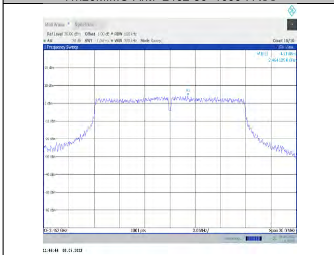
11n20MIMO-Ant9-2462-0~Reference-PASS
