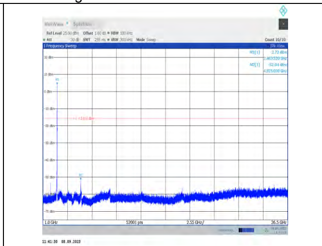
11n20MIMO-Ant7-2462-1000~26500-PASS
