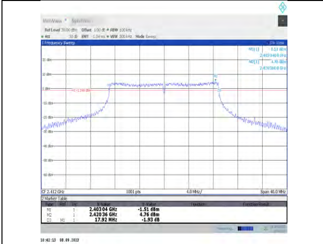
11n20MIMO-Ant7-2412-PASS
