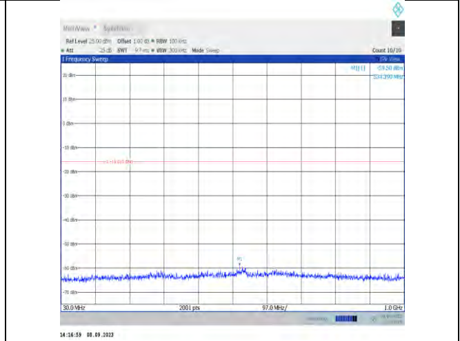
11ax20MIMO-Ant9-2462-30~1000-PASS
