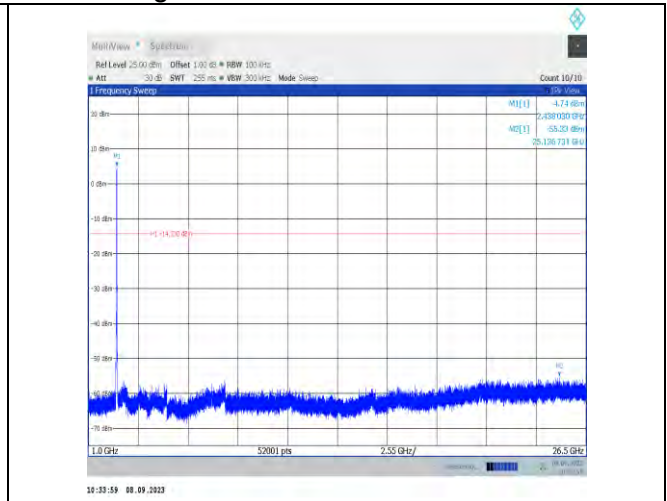
11g-Ant9-2437-1000~26500-PASS
