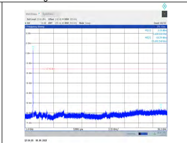
11ax20MIMO-Ant7-2437-1000~26500-PASS
