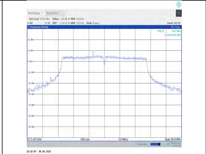
11g-Ant9-2437-0~Reference-PASS
