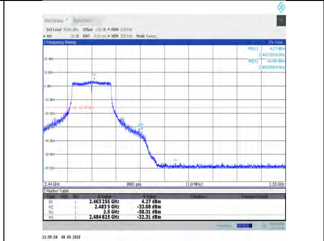
11n20MIMO-Ant7-2462-PASS
