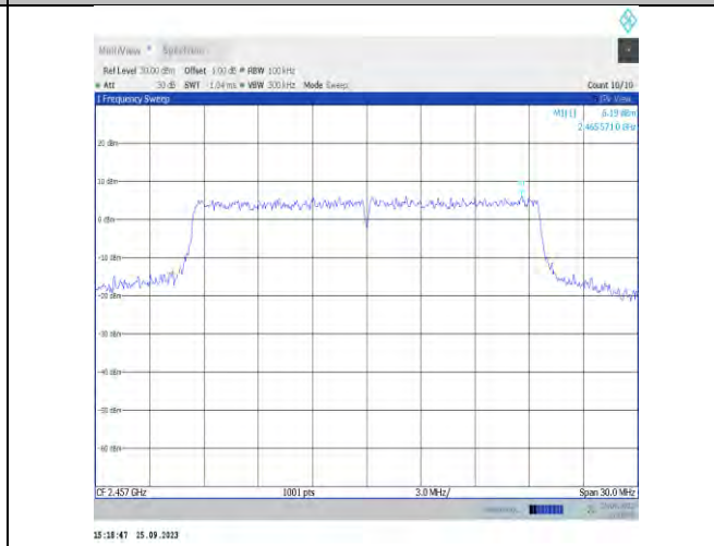
11ax20MIMO-Ant7-2457-0~Reference-PASS
