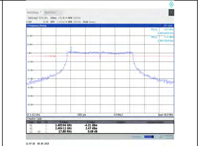
11n20MIMO-Ant9-2412-PASS
