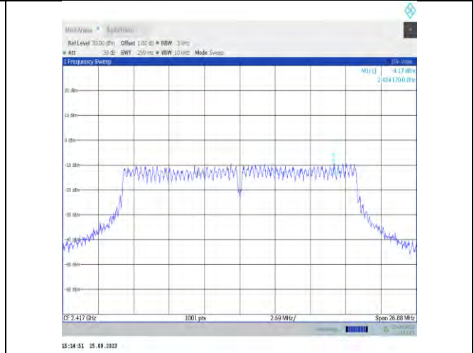
11n20MIMO-Ant7-2417-PASS
