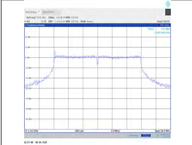
11ax20MIMO-Ant9-2412-0~Reference-PASS
