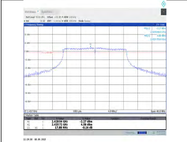
11n20MIMO-Ant7-2437-PASS
