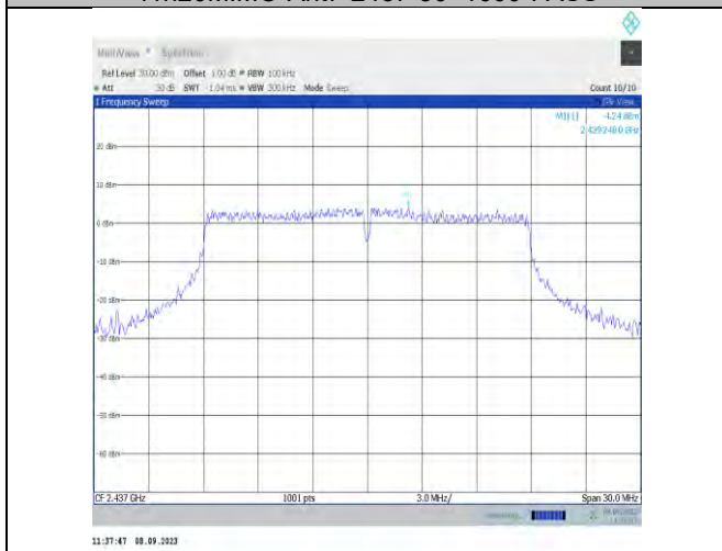
11n20MIMO-Ant9-2437-0~Reference-PASS
