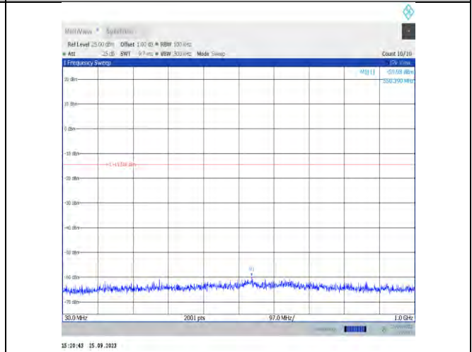
11ax20MIMO-Ant9-2457-30~1000-PASS
