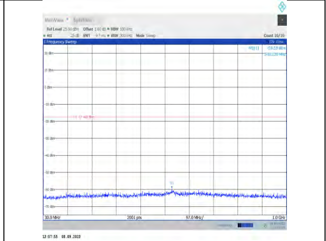
11ax20MIMO-Ant9-2412-30~1000-PASS
