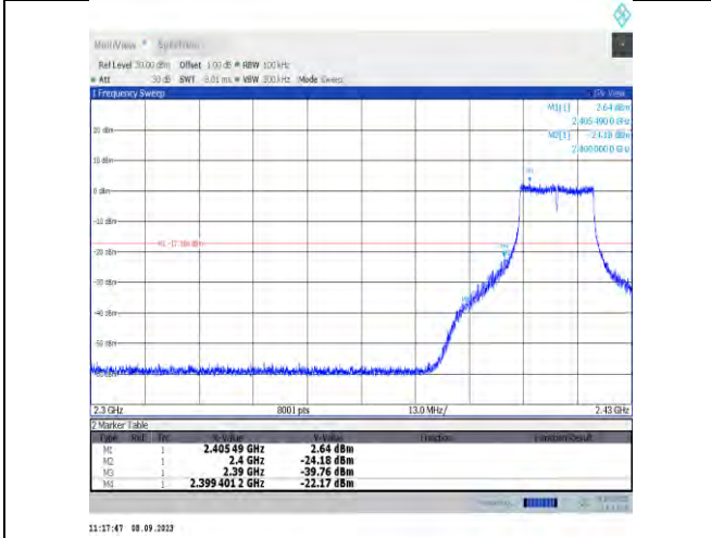
11n20MIMO-Ant9-2412-PASS
