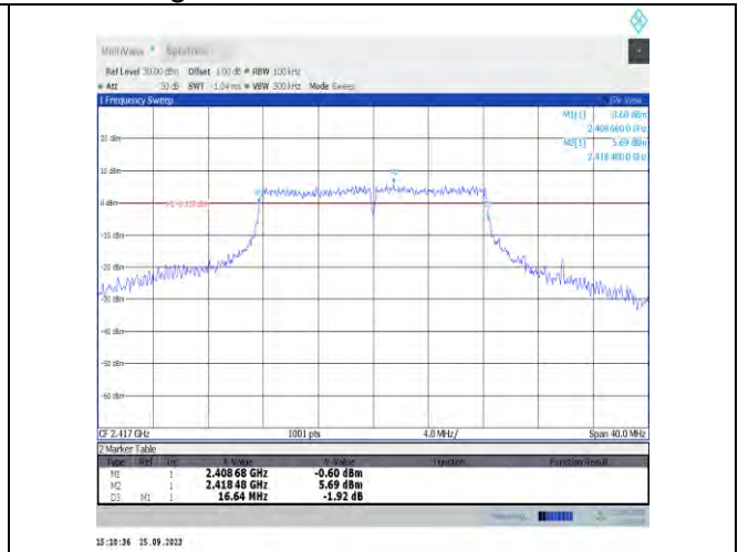
11g-Ant9-2417-PASS
