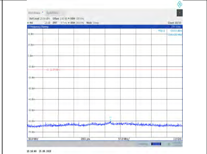
11n20MIMO-Ant9-2417-30~1000-PASS
