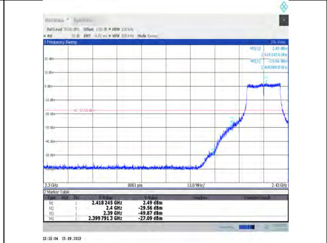
11n20MIMO-Ant7-2417-PASS
