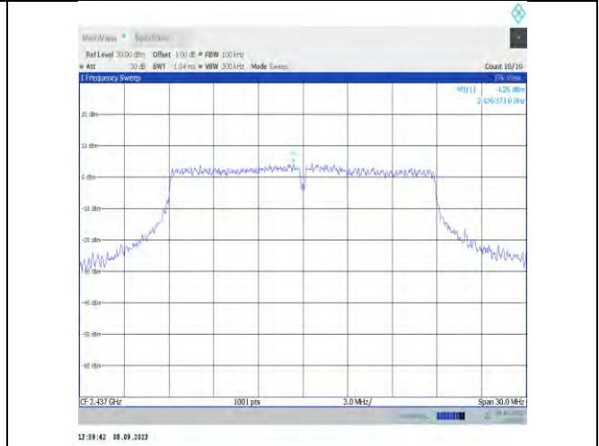
11ax20MIMO-Ant7-2437-0~Reference-PASS
