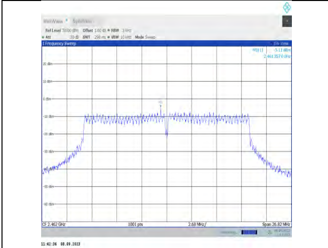
11n20MIMO-Ant9-2462-PASS
