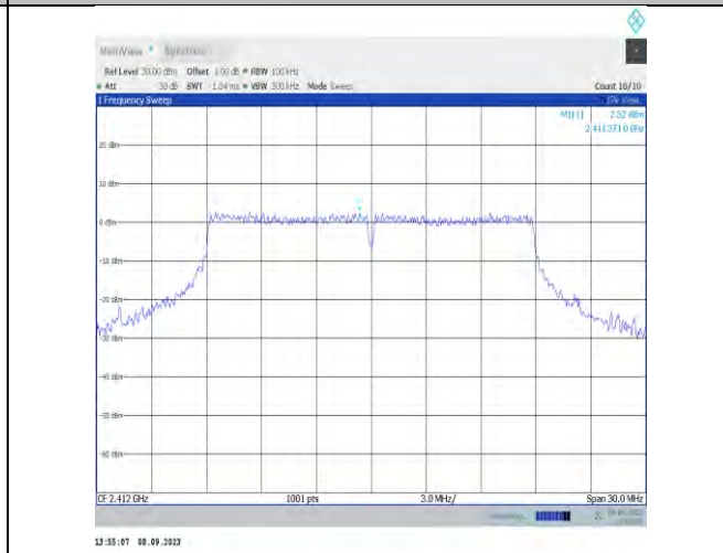
11ax20MIMO-Ant7-2412-0~Reference-PASS
