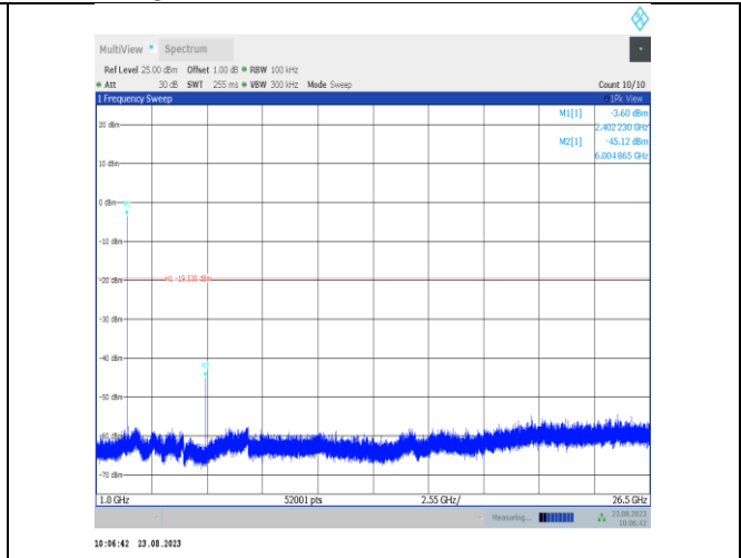
BLE_2M-Ant7-2402-1000~26500-PASS
