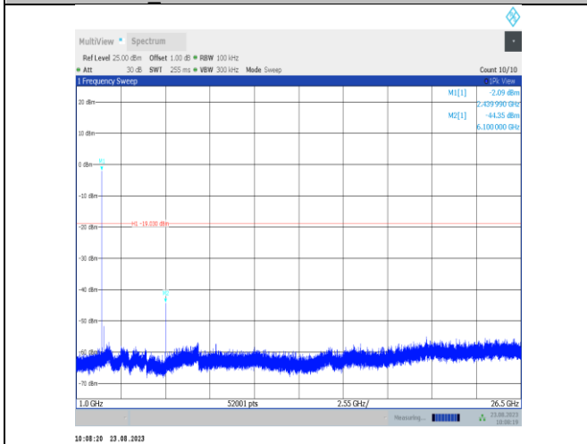
BLE_2M-Ant7-2440-1000~26500-PASS
