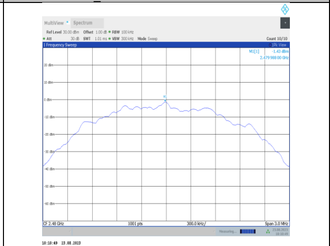
BLE_2M-Ant7-2480-0~Reference-PASS
