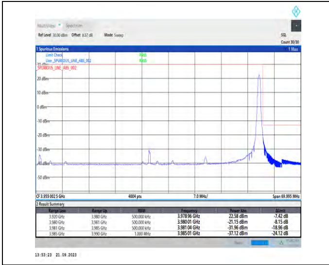
1-N77-3700-3980-PC2-30-60-H-2-DFT-PI2BPSK-Edge_1RB_Right-1@161-Ant5-1--PASS-see graph
