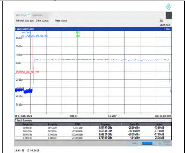
1-N77-3700-3980-PC2-30-80-L-3-DFT-PI2BPSK-Outer_Full-216@0-Ant5-1--PASS-see graph
