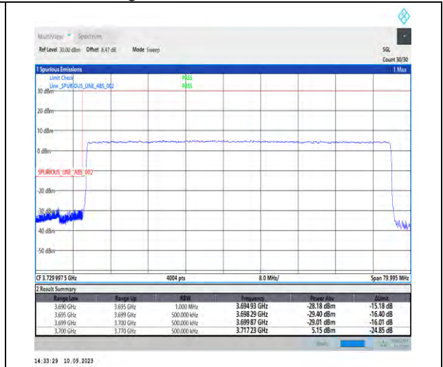
1-N77-3700-3980-PC2-30-70-L-3-DFT-PI2BPSK-Outer_Full-180@0-Ant5-1--PASS-see graph
