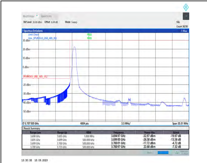
1-N77-3700-3980-PC2-30-25-L-1-DFT-PI2BPSK-Edge_1RB_Left-1@0-Ant5-1--PASS-see graph
