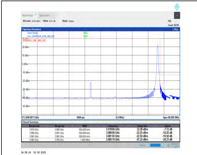
1-N77-3700-3980-PC2-30-70-H-2-DFT-PI2BPSK-Edge_1RB_Right-1@188-Ant5-1--PASS-see graph
