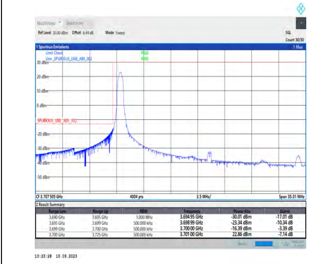
1-N77-3700-3980-PC2-30-25-L-4-CP-QPSK-Edge_1RB_Left-1@0-Ant5-1--PASS-see graph
