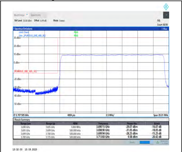
1-N77-3700-3980-PC2-30-25-L-3-DFT-PI2BPSK-Outer_Full-64@0-Ant5-1--PASS-see graph
