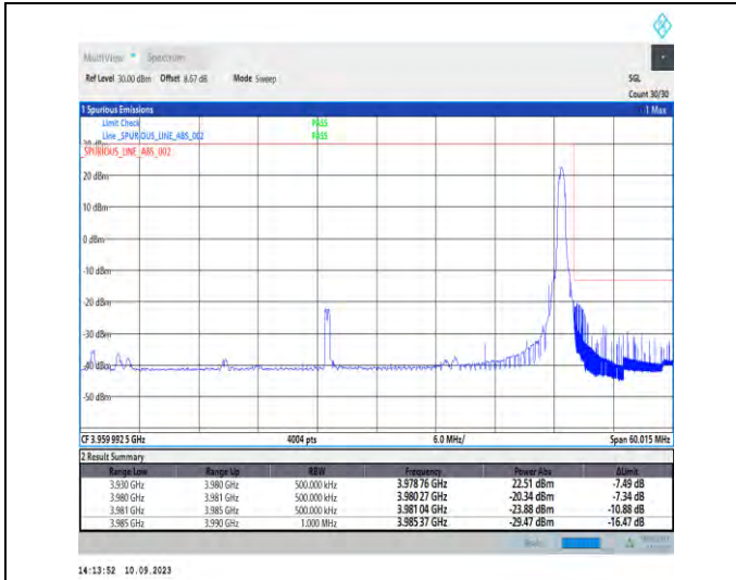
1-N77-3700-3980-PC2-30-50-H-2-DFT-PI2BPSK-Edge_1RB_Right-1@132-Ant5-1--PASS-see graph
