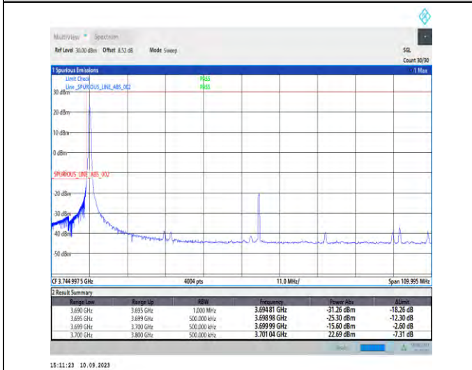
1-N77-3700-3980-PC2-30-100-L-4-CP-QPSK-Edge_1RB_Left-1@0-Ant5-1--PASS-see graph
