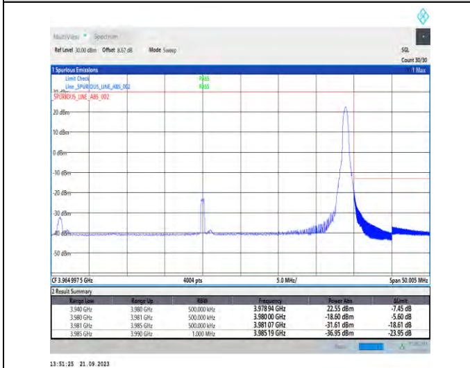
1-N77-3700-3980-PC2-30-40-H-5-CP-QPSK-Edge_1RB_Right-1@105-Ant5-1--PASS-see graph
