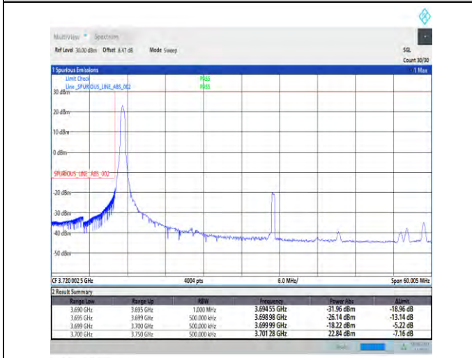
1-N77-3700-3980-PC2-30-50-L-1-DFT-PI2BPSK-Edge_1RB_Left-1@0-Ant5-1--PASS-see graph
