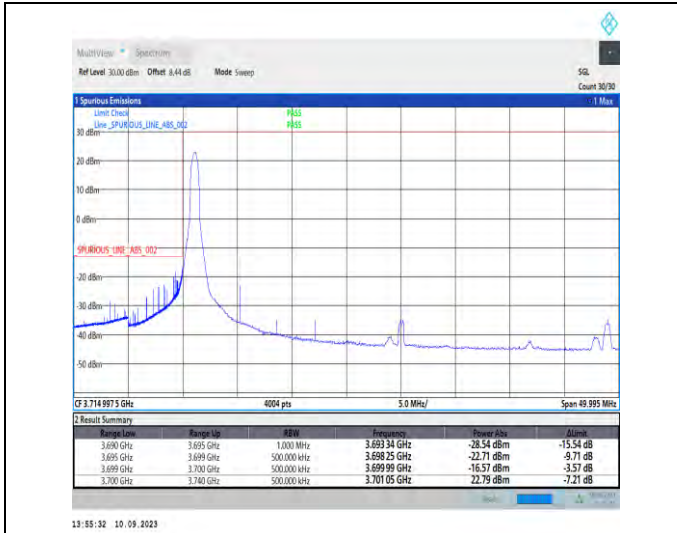
1-N77-3700-3980-PC2-30-40-L-1-DFT-PI2BPSK-Edge_1RB_Left-1@0-Ant5-1--PASS-see graph
