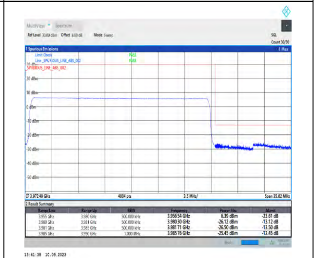
1-N77-3700-3980-PC2-30-25-H-6-CP-QPSK-Outer_Full-65@0-Ant5-1--PASS-see graph
