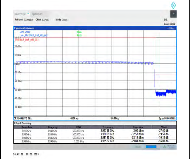
1-N77-3700-3980-PC2-30-70-H-6-CP-QPSK-Outer_Full-189@0-Ant5-1--PASS-see graph
