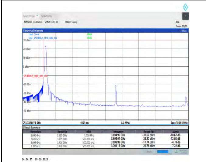
1-N77-3700-3980-PC2-30-70-L-4-CP-QPSK-Edge_1RB_Left-1@0-Ant5-1--PASS-see graph
