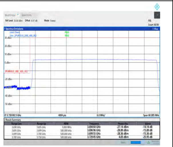
1-N77-3700-3980-PC2-30-50-L-3-DFT-PI2BPSK-Outer_Full-128@0-Ant5-1--PASS-see graph
