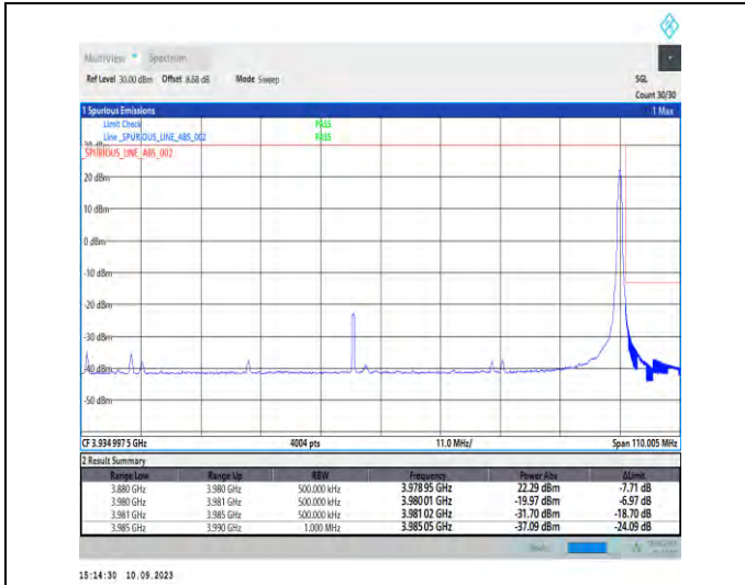
1-N77-3700-3980-PC2-30-100-H-2-DFT-PI2BPSK-Edge_1_RB_Right-1@272-Ant5-1--PASS-see graph
