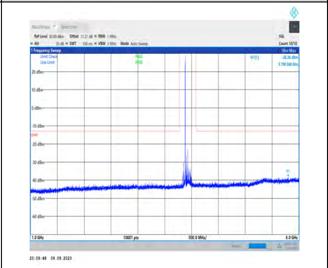
1-N77-3700-3980-PC2-30-100-H-1-DFT-PI2BPSK-In ner_1RB_Left-1@1-1000-6000-Ant5-5798.50--38.36- -13-PASS
