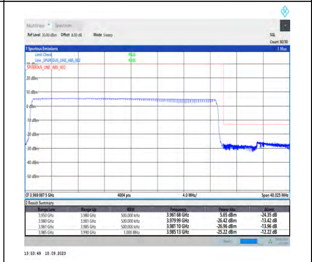
1-N77-3700-3980-PC2-30-30-H-6-CP-QPSK-Outer_Full-78@0-Ant5-1--PASS-see graph
