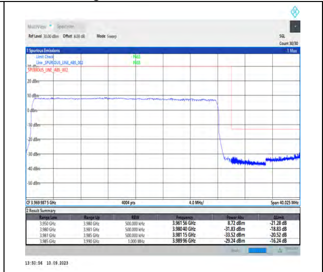
1-N77-3700-3980-PC2-30-30-H-3-DFT-PI2BPSK-Outer_Full-75@0-Ant5-1--PASS-see graph
