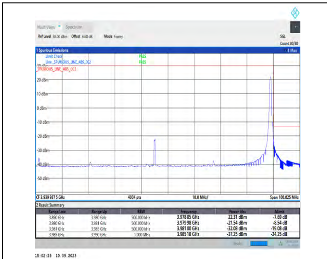
1-N77-3700-3980-PC2-30-90-H-2-DFT-PI2BPSK-Edge_1RB_Right-1@244-Ant5-1--PASS-see graph
