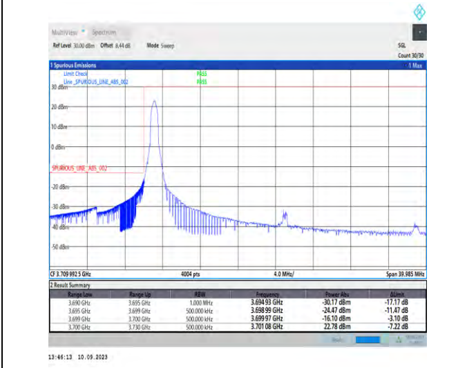
1-N77-3700-3980-PC2-30-30-L-4-CP-QPSK-Edge_1RB_Left-1@0-Ant5-1--PASS-see graph
