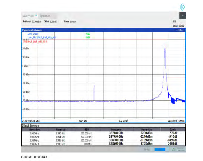
1-N77-3700-3980-PC2-30-80-H-2-DFT-PI2BPSK-Edge_1RB_Right-1@216-Ant5-1--PASS-see graph
