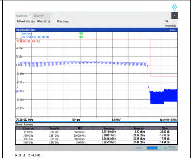
1-N77-3700-3980-PC2-30-50-H-6-CP-QPSK-Outer_Full-133@0-Ant5-1--PASS-see graph
