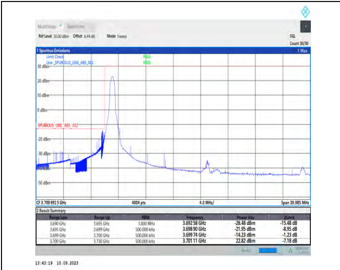
1-N77-3700-3980-PC2-30-30-L-1-DFT-PI2BPSK-Edge_1RB_Left-1@0-Ant5-1--PASS-see graph
