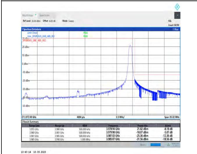
1-N77-3700-3980-PC2-30-25-H-5-CP-QPSK-Edge_1RB_Right-1@64-Ant5-1--PASS-see graph
