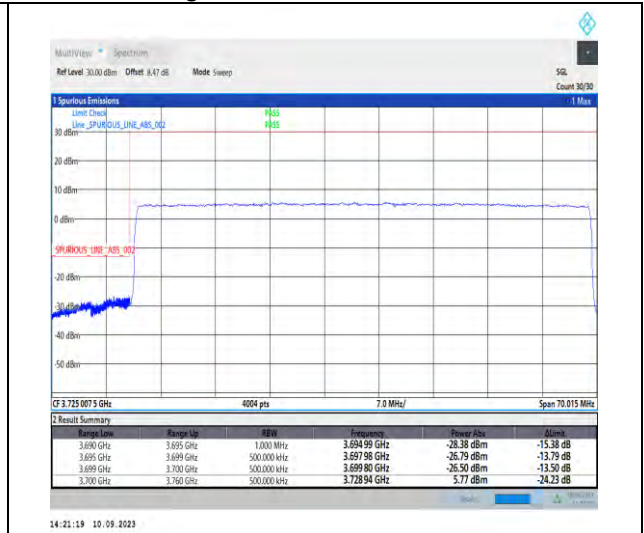
1-N77-3700-3980-PC2-30-60-L-3-DFT-PI2BPSK-Outer_Full-162@0-Ant5-1--PASS-see graph
