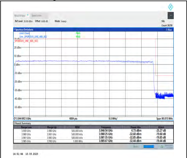
1-N77-3700-3980-PC2-30-80-H-3-DFT-PI2BPSK-Outer_Full-216@0-Ant5-1--PASS-see graph
