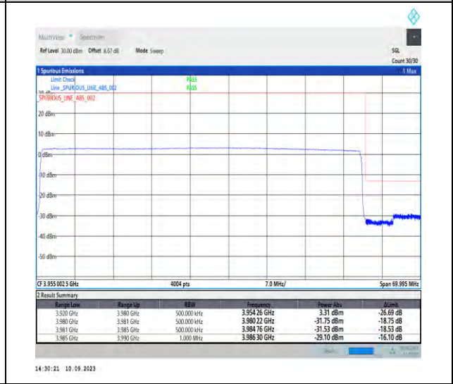
1-N77-3700-3980-PC2-30-60-H-6-CP-QPSK-Outer_Full-162@0-Ant5-1--PASS-see graph
