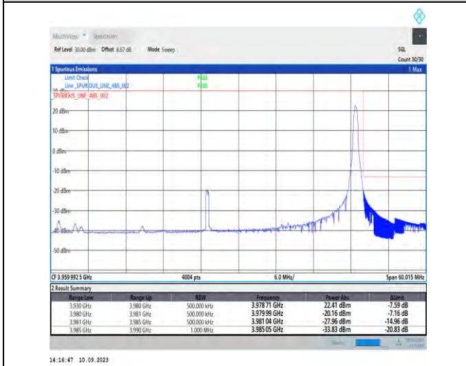
1-N77-3700-3980-PC2-30-50-H-5-CP-QPSK-Edge_1RB_Right-1@132-Ant5-1--PASS-see graph
