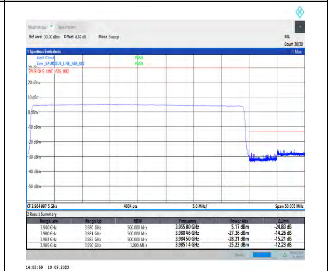
1-N77-3700-3980-PC2-30-40-H-6-CP-QPSK-Outer_Full-106@0-Ant5-1--PASS-see graph
