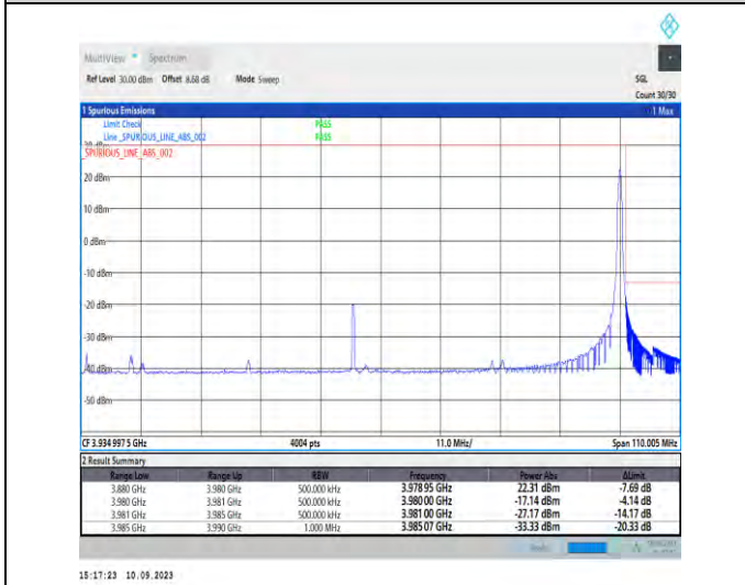
1-N77-3700-3980-PC2-30-100-H-5-CP-QPSK-Edge_1_RB_Right-1@272-Ant5-1--PASS-see graph
