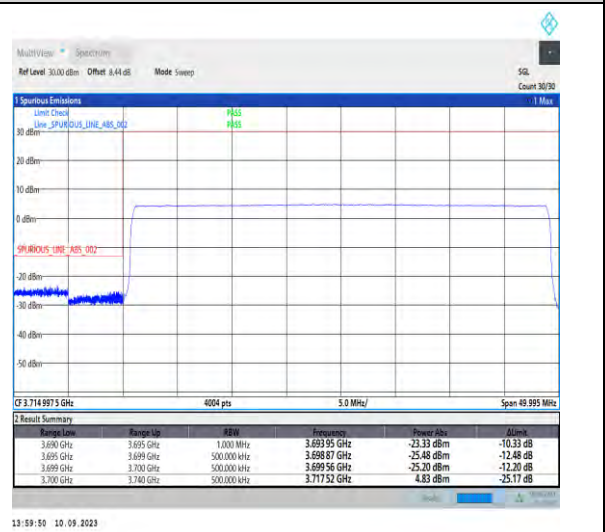
1-N77-3700-3980-PC2-30-40-L-6-CP-QPSK-Outer_Full-106@0-Ant5-1--PASS-see graph
