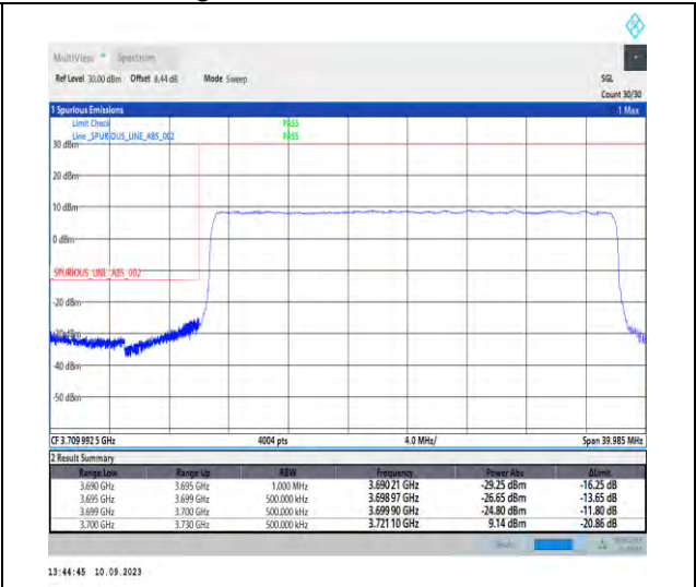
1-N77-3700-3980-PC2-30-30-L-3-DFT-PI2BPSK-Outer_Full-75@0-Ant5-1--PASS-see graph
