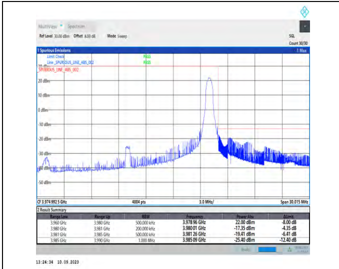
1-N77-3700-3980-PC2-30-20-H-2-DFT-PI2BPSK-Edge_1RB_Right-1@50-Ant5-1--PASS-see graph
