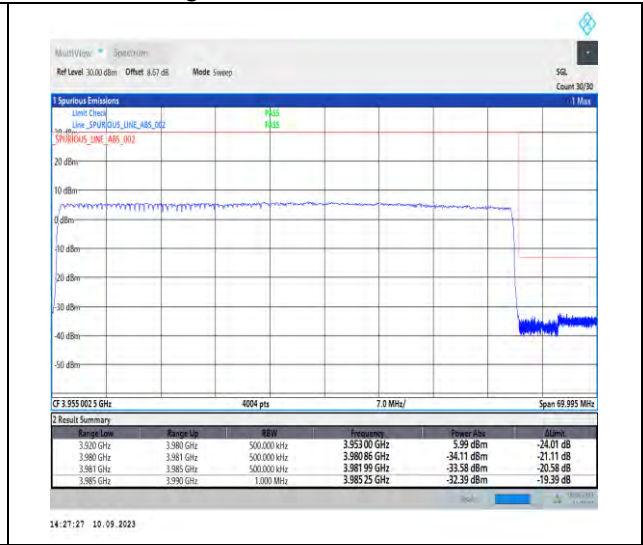
1-N77-3700-3980-PC2-30-60-H-3-DFT-PI2BPSK-Outer_Full-162@0-Ant5-1--PASS-see graph
