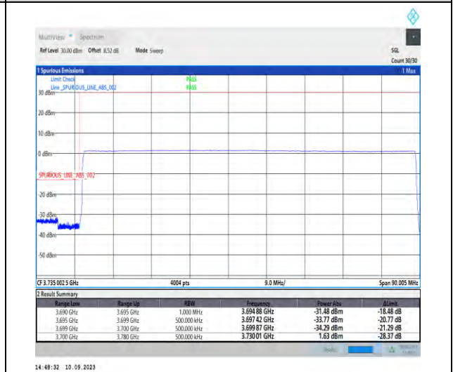
1-N77-3700-3980-PC2-30-80-L-6-CP-QPSK-Outer_Full-217@0-Ant5-1--PASS-see graph
