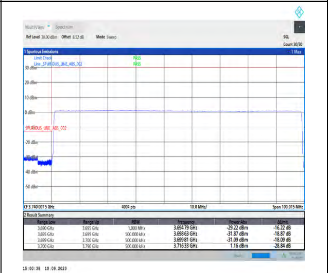
1-N77-3700-3980-PC2-30-90-L-6-CP-QPSK-Outer_Full-245@0-Ant5-1--PASS-see graph
