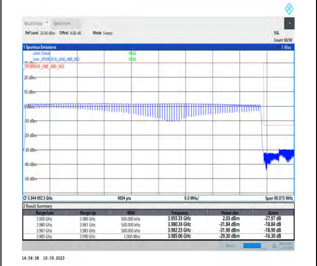
1-N77-3700-3980-PC2-30-80-H-6-CP-QPSK-Outer_Full-217@0-Ant5-1--PASS-see graph
