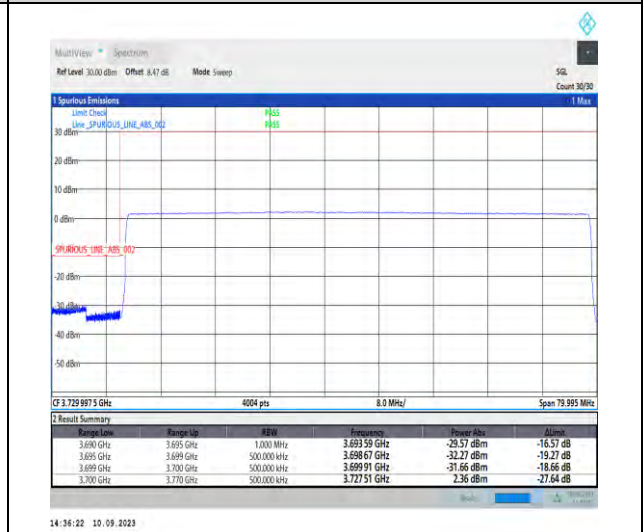
1-N77-3700-3980-PC2-30-70-L-6-CP-QPSK-Outer_Full-189@0-Ant5-1--PASS-see graph
