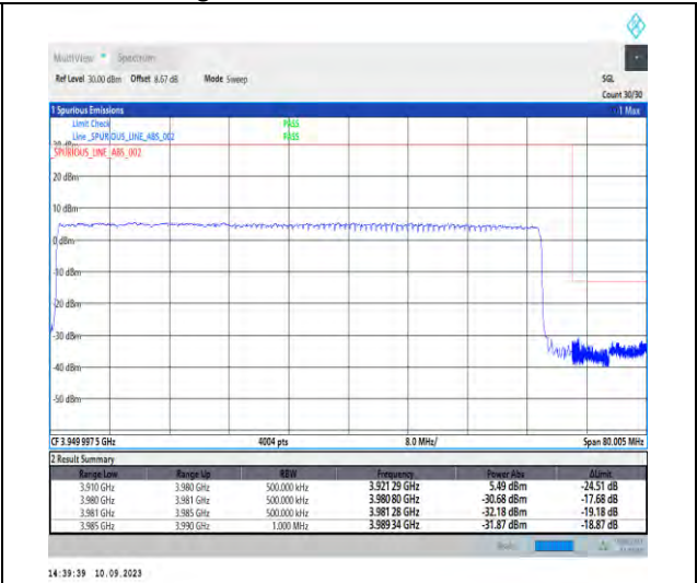
1-N77-3700-3980-PC2-30-70-H-3-DFT-PI2BPSK-Outer_Full-180@0-Ant5-1--PASS-see graph
