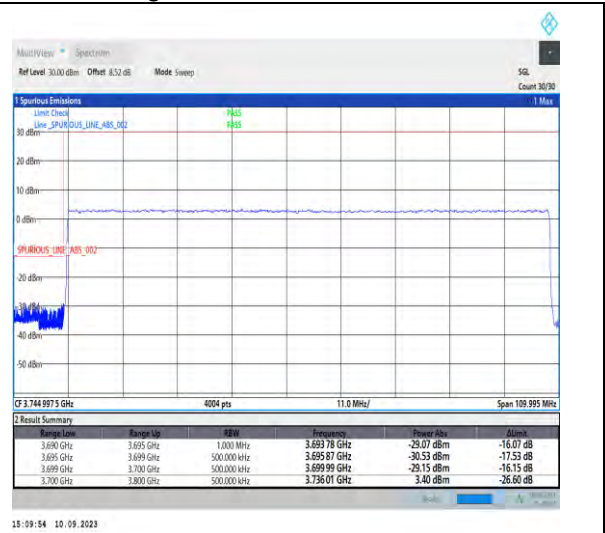
1-N77-3700-3980-PC2-30-100-L-3-DFT-PI2BPSK-Outer_Full-270@0-Ant5-1--PASS-see graph
