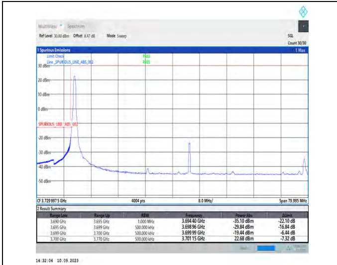
1-N77-3700-3980-PC2-30-70-L-1-DFT-PI2BPSK-Edge_1RB_Left-1@0-Ant5-1--PASS-see graph
