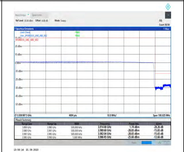
1-N77-3700-3980-PC2-30-90-H-6-CP-QPSK-Outer_Full-245@0-Ant5-1--PASS-see graph
