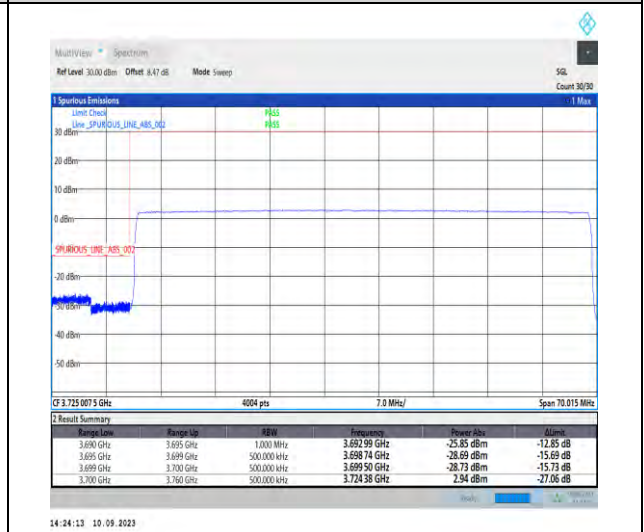
1-N77-3700-3980-PC2-30-60-L-6-CP-QPSK-Outer_Full-162@0-Ant5-1--PASS-see graph
