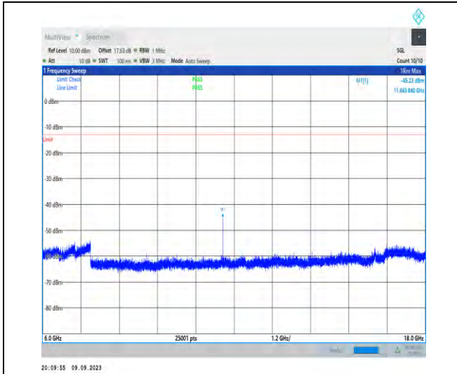
1-N77-3700-3980-PC2-30-100-H-1-DFT-PI2BPSK-In ner_1RB_Left-1@1-6000-18000-Ant5-11643.84--45. 23--13-PASS
