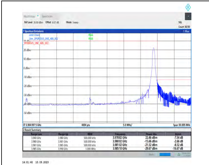
1-N77-3700-3980-PC2-30-40-H-2-DFT-PI2BPSK-Edge_1RB_Right-1@105-Ant5-1--PASS-see graph
