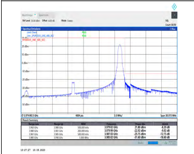
1-N77-3700-3980-PC2-30-20-H-5-CP-QPSK-Edge_1RB_Right-1@50-Ant5-1--PASS-see graph
