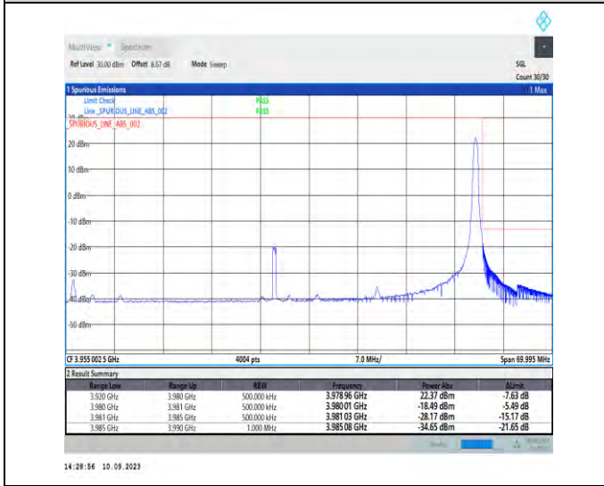
1-N77-3700-3980-PC2-30-60-H-5-CP-QPSK-Edge_1RB_Right-1@161-Ant5-1--PASS-see graph
