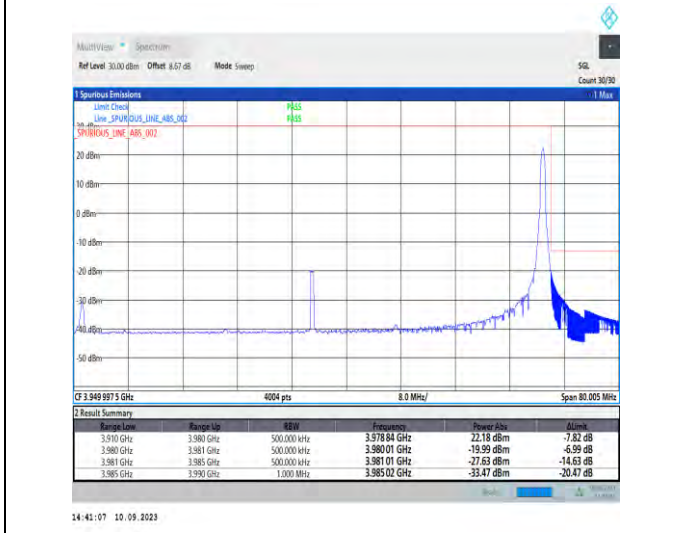
1-N77-3700-3980-PC2-30-70-H-5-CP-QPSK-Edge_1RB_Right-1@188-Ant5-1--PASS-see graph
