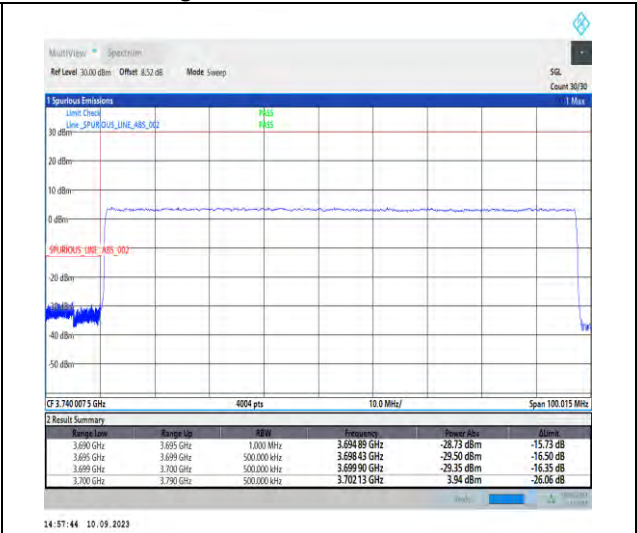
1-N77-3700-3980-PC2-30-90-L-3-DFT-PI2BPSK-Outer_Full-240@0-Ant5-1--PASS-see graph
