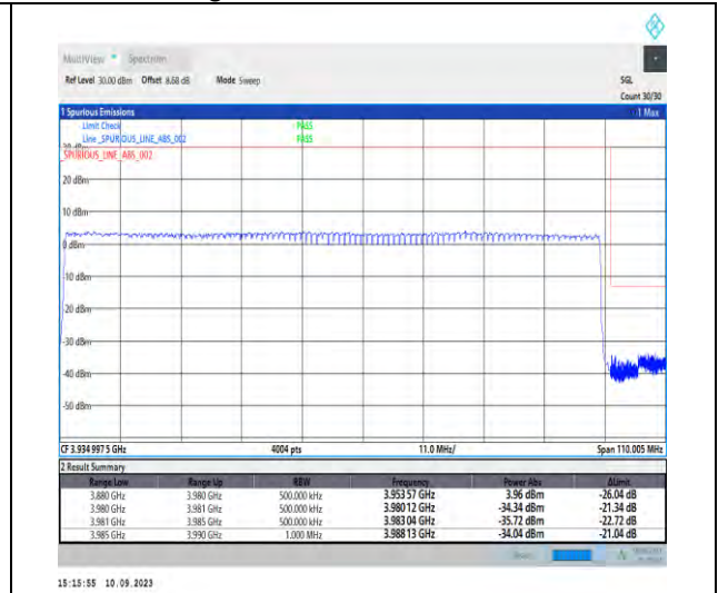
1-N77-3700-3980-PC2-30-100-H-3-DFT-PI2BPSK-Outer_Full-270@0-Ant5-1--PASS-see graph
