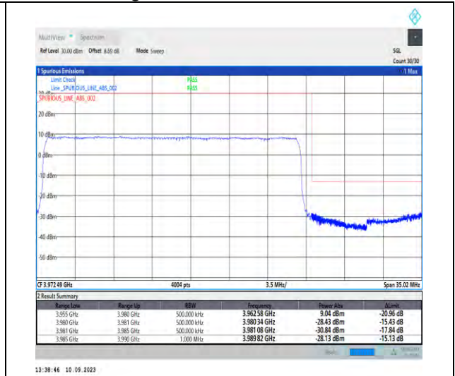
1-N77-3700-3980-PC2-30-25-H-3-DFT-PI2BPSK-Outer_Full-64@0-Ant5-1--PASS-see graph
