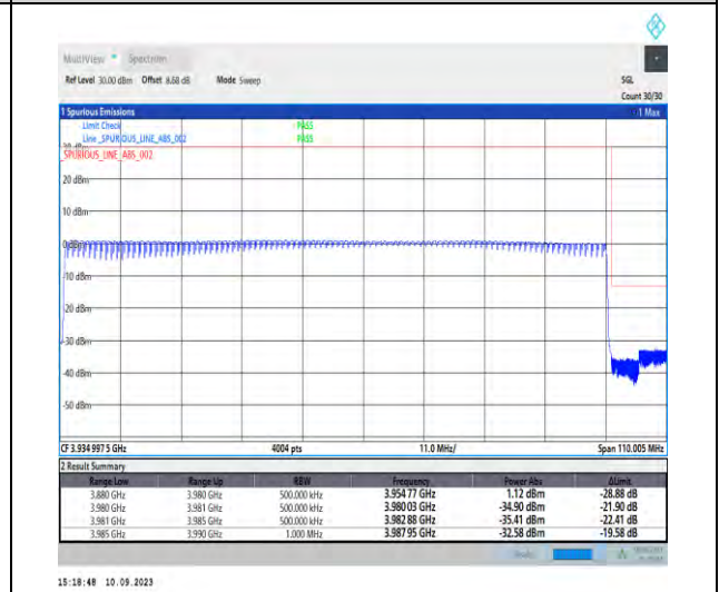
1-N77-3700-3980-PC2-30-100-H-6-CP-QPSK-Outer_Full-273@0-Ant5-1--PASS-see graph
