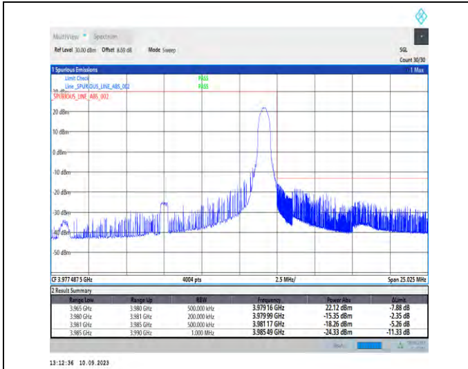
1-N77-3700-3980-PC2-30-15-H-2-DFT-PI2BPSK-Edge_1RB_Right-1@37-Ant5-1--PASS-see graph
