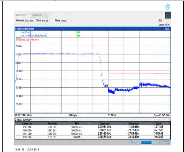
1-N77-3700-3980-PC2-30-15-H-3-DFT-PI2BPSK-Outer_Full-36@0-Ant5-1--PASS-see graph
