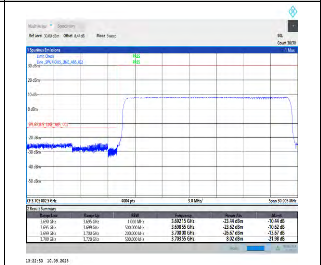
1-N77-3700-3980-PC2-30-20-L-6-CP-QPSK-Outer_Full-51@0-Ant5-1--PASS-see graph
