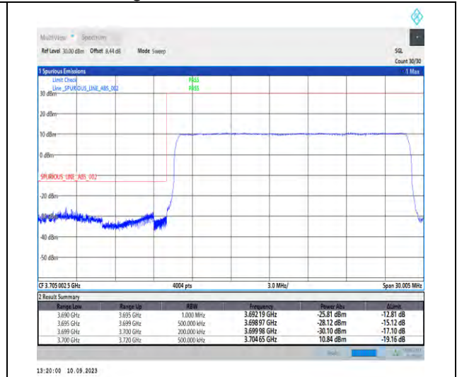
1-N77-3700-3980-PC2-30-20-L-3-DFT-PI2BPSK-Outer_Full-50@0-Ant5-1--PASS-see graph
