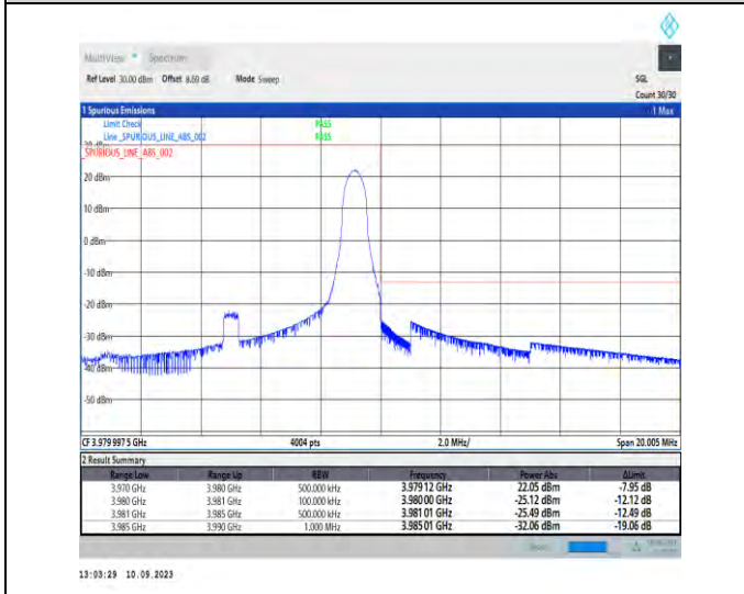
1-N77-3700-3980-PC2-30-10-H-5-CP-QPSK-Edge_1RB_Right-1@23-Ant5-1--PASS-see graph
