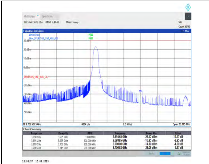
1-N77-3700-3980-PC2-30-15-L-1-DFT-PI2BPSK-Edge_1RB_Left-1@0-Ant5-1--PASS-see graph
