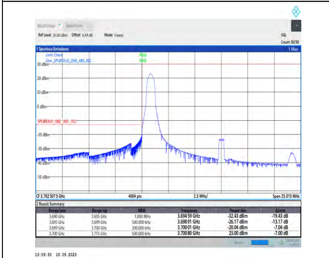
1-N77-3700-3980-PC2-30-15-L-4-CP-QPSK-Edge_1RB_Left-1@0-Ant5-1--PASS-see graph
