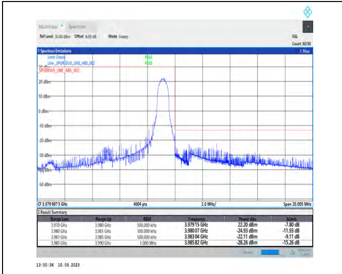
1-N77-3700-3980-PC2-30-10-H-2-DFT-PI2BPSK-Edge_1RB_Right-1@23-Ant5-1--PASS-see graph
