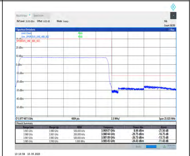
1-N77-3700-3980-PC2-30-15-H-6-CP-QPSK-Outer_Full-38@0-Ant5-1--PASS-see graph
