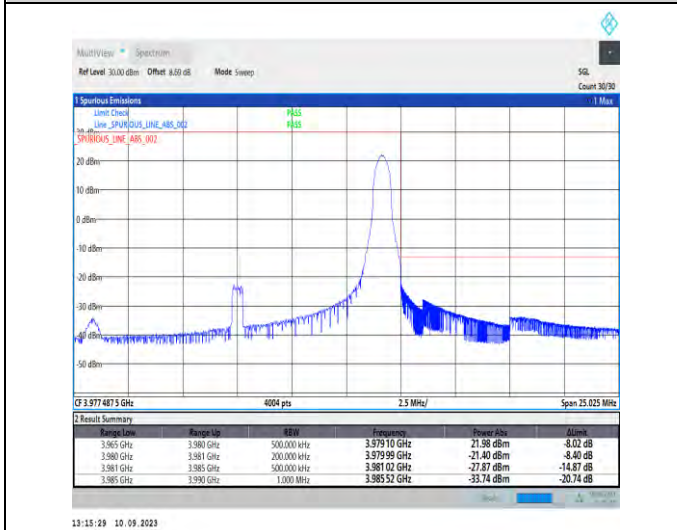
1-N77-3700-3980-PC2-30-15-H-5-CP-QPSK-Edge_1RB_Right-1@37-Ant5-1--PASS-see graph
