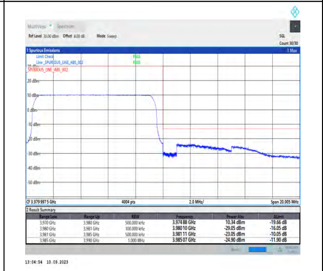
1-N77-3700-3980-PC2-30-10-H-6-CP-QPSK-Outer_Full-24@0-Ant5-1--PASS-see graph
