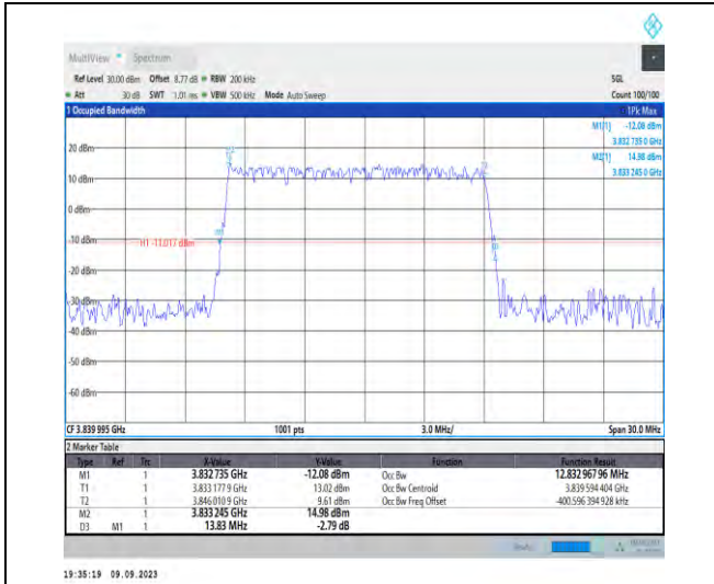
1-N77-3700-3980-PC2-30-15-M-4-DFT-64QAM-Out_er_Full-36@0-Ant5-12.833-13.830-≤15-PASS
