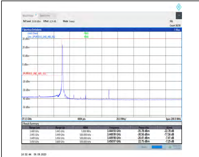
1-N77-3450-3550-PC2-30-60-L-1-DFT-PI2BPSK-Edge_1RB_Left-1@0-Ant5-1--PASS-see graph
