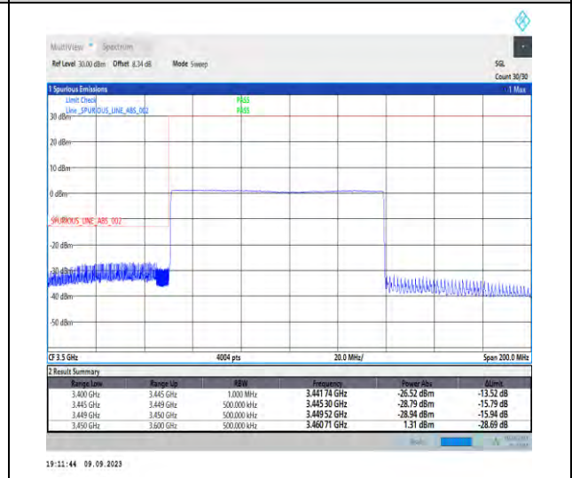
1-N77-3450-3550-PC2-30-90-L-6-CP-QPSK-Outer_Full-245@0-Ant5-1--PASS-see graph
