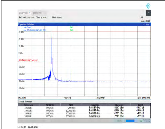
1-N77-3450-3550-PC2-30-60-L-4-CP-QPSK-Edge_1RB_Left-1@0-Ant5-1--PASS-see graph
