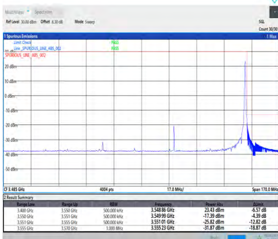
1-N77-3450-3550-PC2-30-90-H-5-CP-QPSK-Edge_1RB_Right-1@244-Ant5-1--PASS-see graph
