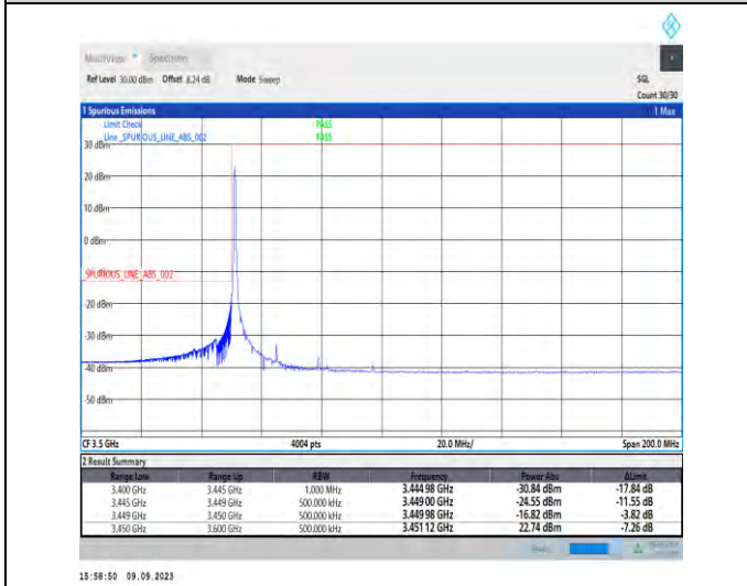
1-N77-3450-3550-PC2-30-30-L-4-CP-QPSK-Edge_1RB_Left-1@0-Ant5-1--PASS-see graph
