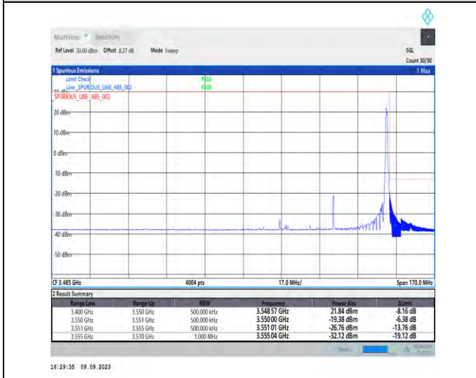
1-N77-3450-3550-PC2-30-50-H-5-CP-QPSK-Edge_1RB_Right-1@132-Ant5-1--PASS-see graph
