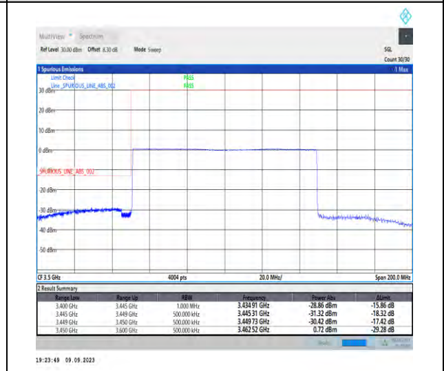
1-N77-3450-3550-PC2-30-100-L-6-CP-QPSK-Outer_Full-273@0-Ant5-1--PASS-see graph
