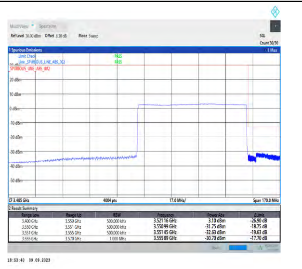
1-N77-3450-3550-PC2-30-70-H-6-CP-QPSK-Outer_Full-189@0-Ant5-1--PASS-see graph
