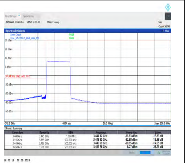
1-N77-3450-3550-PC2-30-30-L-6-CP-QPSK-Outer_Full-78@0-Ant5-1--PASS-see graph
