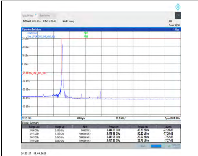
1-N77-3450-3550-PC2-30-50-L-1-DFT-PI2BPSK-Edge_1RB_Left-1@0-Ant5-1--PASS-see graph
