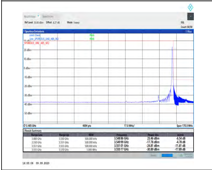
1-N77-3450-3550-PC2-30-30-H-5-CP-QPSK-Edge_1RB_Right-1@77-Ant5-1--PASS-see graph
