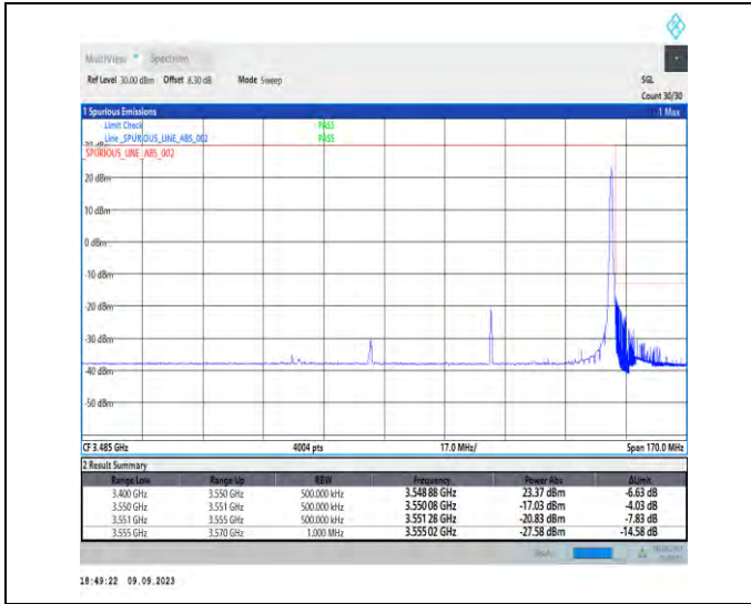
1-N77-3450-3550-PC2-30-70-H-2-DFT-PI2BPSK-Edge_1RB_Right-1@188-Ant5-1--PASS-see graph
