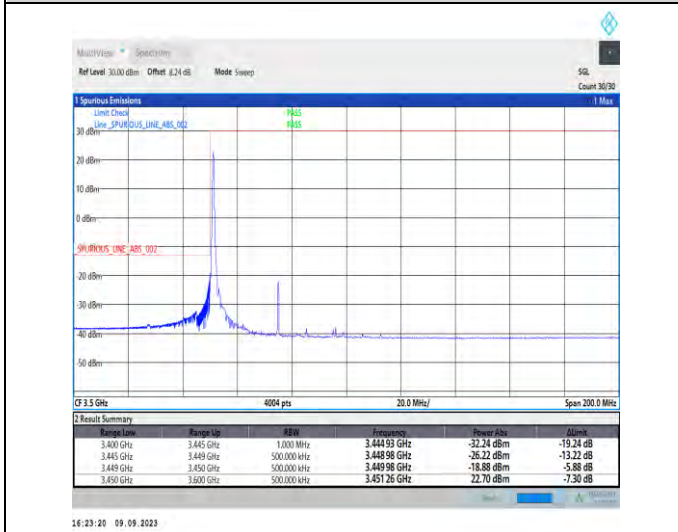
1-N77-3450-3550-PC2-30-50-L-4-CP-QPSK-Edge_1RB_Left-1@0-Ant5-1--PASS-see graph
