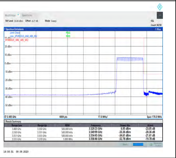
1-N77-3450-3550-PC2-30-30-H-6-CP-QPSK-Outer_Full-78@0-Ant5-1--PASS-see graph
