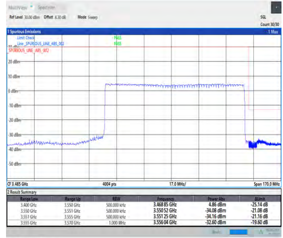
1-N77-3450-3550-PC2-30-90-H-3-DFT-PI2BPSK-Outer_Full-240@0-Ant5-1--PASS-see graph
