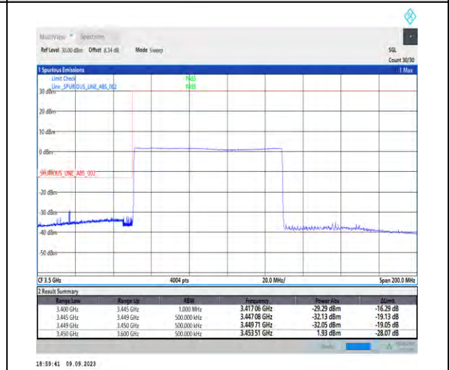
1-N77-3450-3550-PC2-30-80-L-6-CP-QPSK-Outer_Full-217@0-Ant5-1--PASS-see graph
