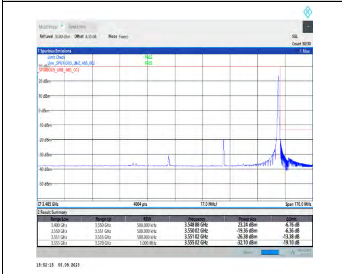
1-N77-3450-3550-PC2-30-70-H-5-CP-QPSK-Edge_1RB_Right-1@188-Ant5-1--PASS-see graph
