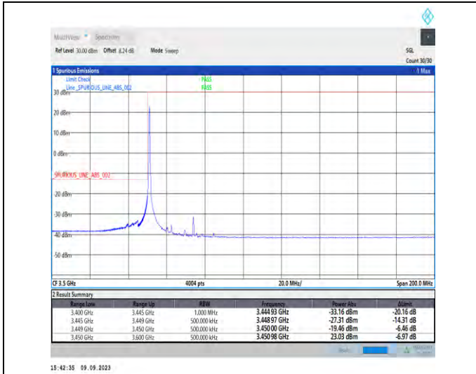
1-N77-3450-3550-PC2-30-25-L-1-DFT-PI2BPSK-Edge_1RB_Left-1@0-Ant5-1--PASS-see graph
