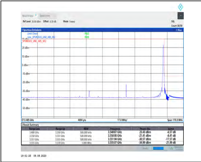
1-N77-3450-3550-PC2-30-80-H-2-DFT-PI2BPSK-Edge_1RB_Right-1@216-Ant5-1--PASS-see graph
