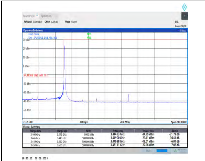
1-N77-3450-3550-PC2-30-80-L-1-DFT-PI2BPSK-Edge_1RB_Left-1@0-Ant5-1--PASS-see graph
