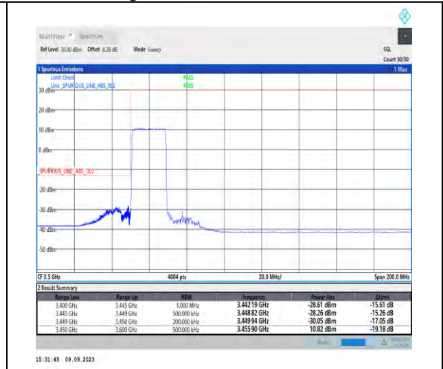
1-N77-3450-3550-PC2-30-20-L-3-DFT-PI2BPSK-Outer_Full-50@0-Ant5-1--PASS-see graph
