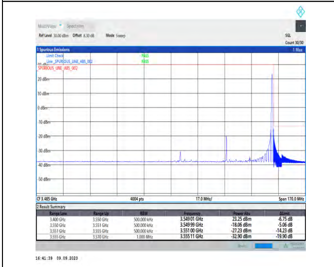
1-N77-3450-3550-PC2-30-60-H-5-CP-QPSK-Edge_1RB_Right-1@161-Ant5-1--PASS-see graph
