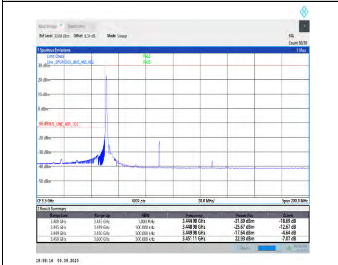
1-N77-3450-3550-PC2-30-80-L-4-CP-QPSK-Edge_1RB_Left-1@0-Ant5-1--PASS-see graph
