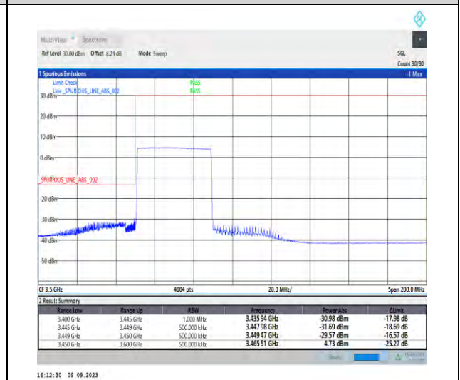
1-N77-3450-3550-PC2-30-40-L-6-CP-QPSK-Outer_Full-106@0-Ant5-1--PASS-see graph
