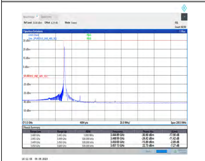
1-N77-3450-3550-PC2-30-40-L-4-CP-QPSK-Edge_1RB_Left-1@0-Ant5-1--PASS-see graph
