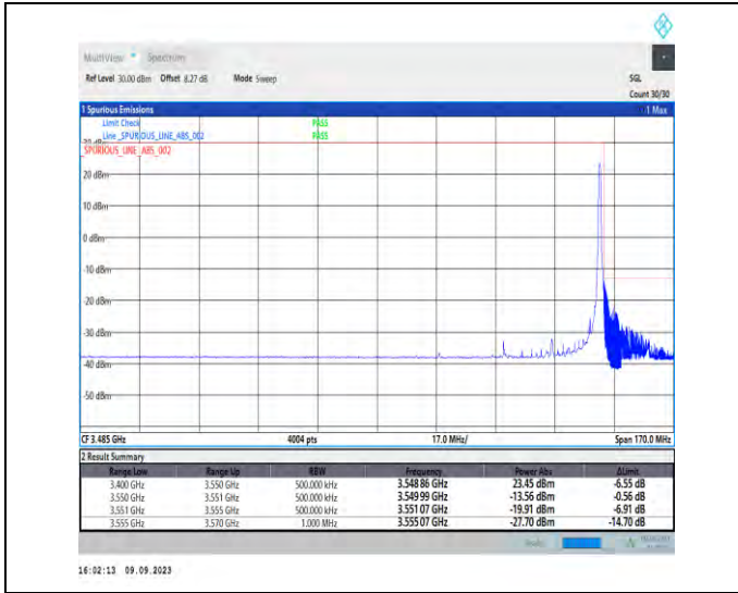
1-N77-3450-3550-PC2-30-30-H-2-DFT-PI2BPSK-Edge_1RB_Right-1@77-Ant5-1--PASS-see graph
