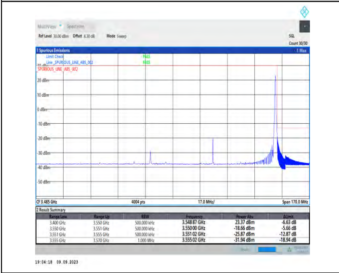
1-N77-3450-3550-PC2-30-80-H-5-CP-QPSK-Edge_1RB_Right-1@216-Ant5-1--PASS-see graph
