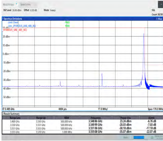
1-N77-3450-3550-PC2-30-90-H-2-DFT-PI2BPSK-Edge_1RB_Right-1@244-Ant5-1--PASS-see graph
