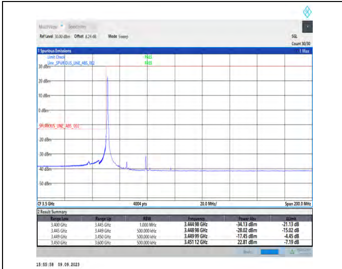
1-N77-3450-3550-PC2-30-30-L-1-DFT-PI2BPSK-Edge_1RB_Left-1@0-Ant5-1--PASS-see graph
