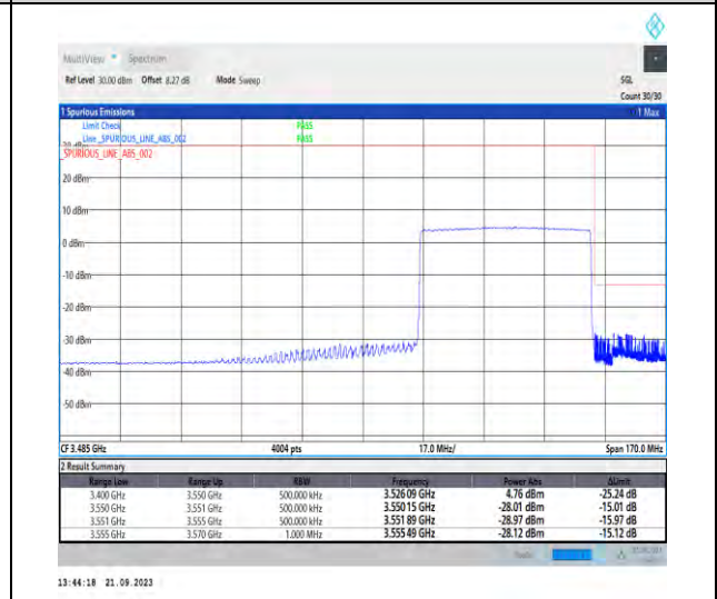
1-N77-3450-3550-PC2-30-50-H-6-CP-QPSK-Outer_Full-133@0-Ant5-1--PASS-see graph
