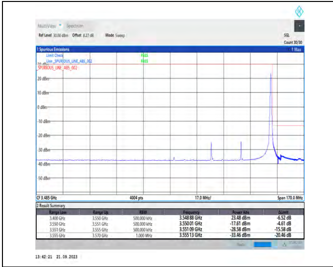
1-N77-3450-3550-PC2-30-40-H-2-DFT-PI2BPSK-Edge_1RB_Right-1@105-Ant5-1--FAIL-see graph
