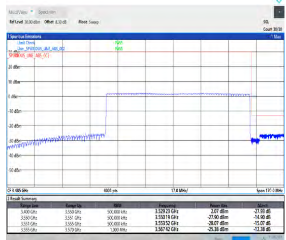
1-N77-3450-3550-PC2-30-90-H-6-CP-QPSK-Outer_Full-245@0-Ant5-1--PASS-see graph
