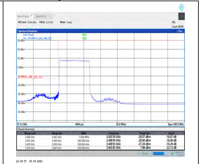
1-N77-3450-3550-PC2-30-40-L-3-DFT-PI2BPSK-Outer_Full-100@0-Ant5-1--PASS-see graph
