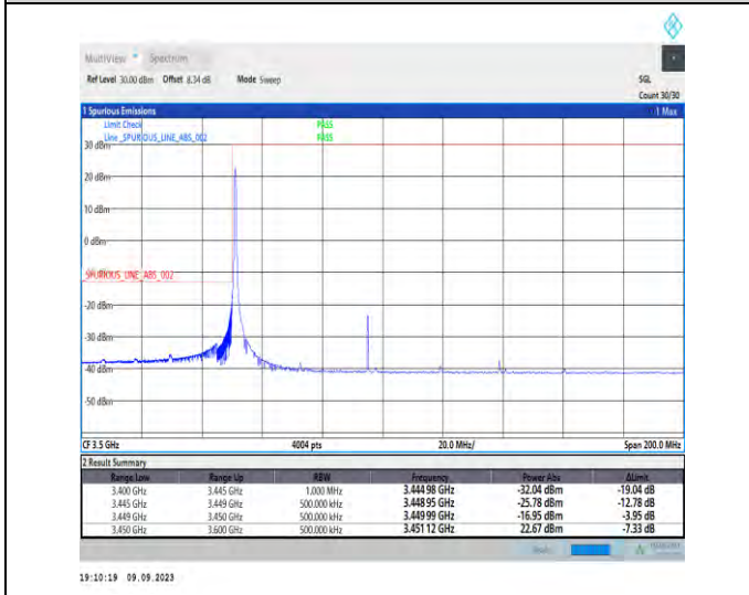
1-N77-3450-3550-PC2-30-90-L-4-CP-QPSK-Edge_1RB_Left-1@0-Ant5-1--PASS-see graph
