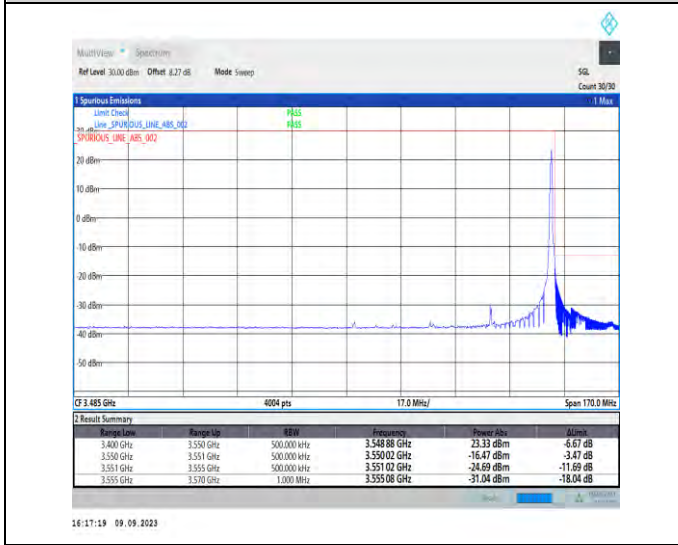
1-N77-3450-3550-PC2-30-40-H-5-CP-QPSK-Edge_1RB_Right-1@105-Ant5-1--PASS-see graph
