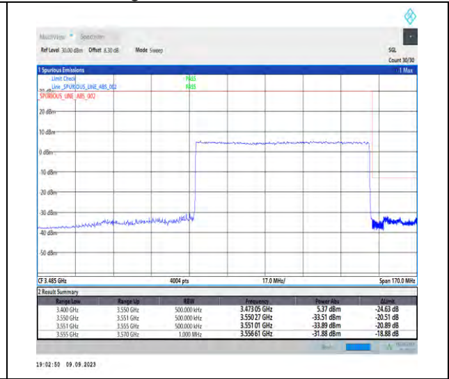
1-N77-3450-3550-PC2-30-80-H-3-DFT-PI2BPSK-Outer_Full-216@0-Ant5-1--PASS-see graph
