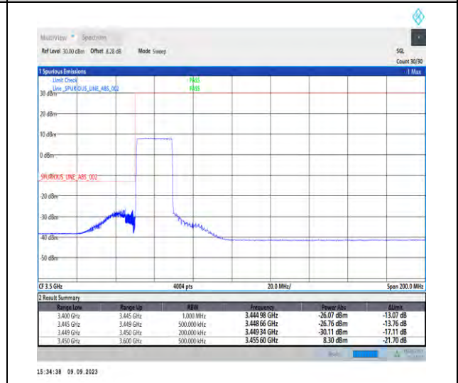
1-N77-3450-3550-PC2-30-20-L-6-CP-QPSK-Outer_Full-51@0-Ant5-1--PASS-see graph
