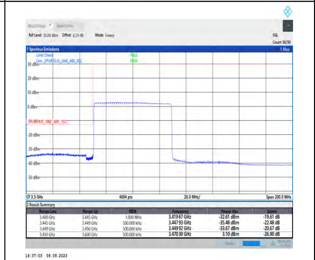
1-N77-3450-3550-PC2-30-60-L-6-CP-QPSK-Outer_Full-162@0-Ant5-1--PASS-see graph
