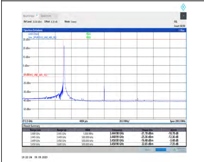
1-N77-3450-3550-PC2-30-100-L-4-CP-QPSK-Edge_1_RB_Left-1@0-Ant5-1--PASS-see graph
