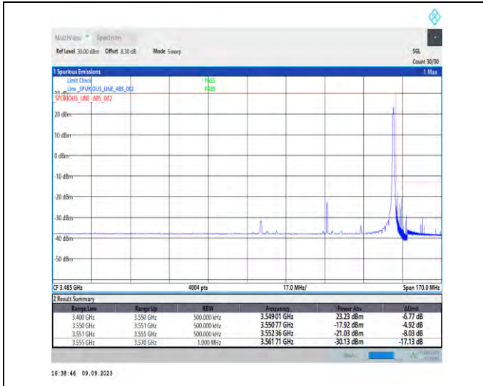
1-N77-3450-3550-PC2-30-60-H-2-DFT-PI2BPSK-Edge_1RB_Right-1@161-Ant5-1--PASS-see graph
