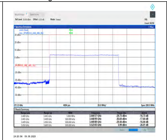
1-N77-3450-3550-PC2-30-100-L-3-DFT-PI2BPSK-Outer_Full-270@0-Ant5-1--PASS-see graph
