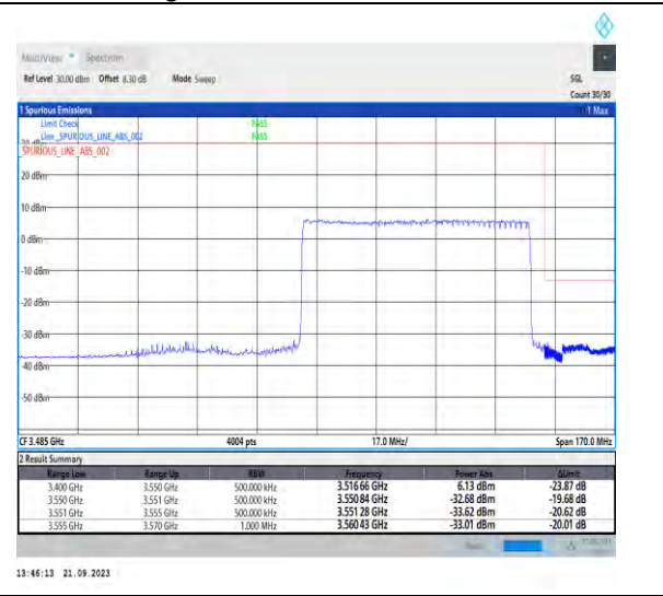
1-N77-3450-3550-PC2-30-70-H-3-DFT-PI2BPSK-Outer_Full-180@0-Ant5-1--PASS-see graph
