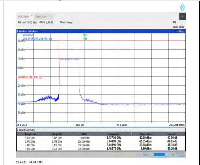
1-N77-3450-3550-PC2-30-25-L-3-DFT-PI2BPSK-Outer_Full-64@0-Ant5-1--PASS-see graph
