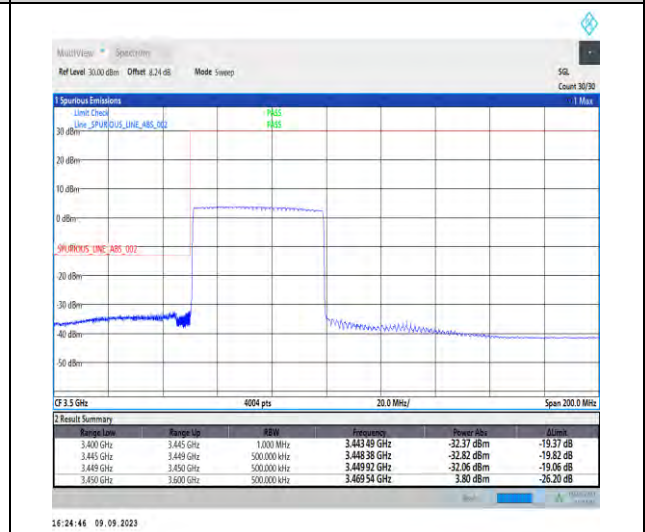
1-N77-3450-3550-PC2-30-50-L-6-CP-QPSK-Outer_Full-133@0-Ant5-1--PASS-see graph
