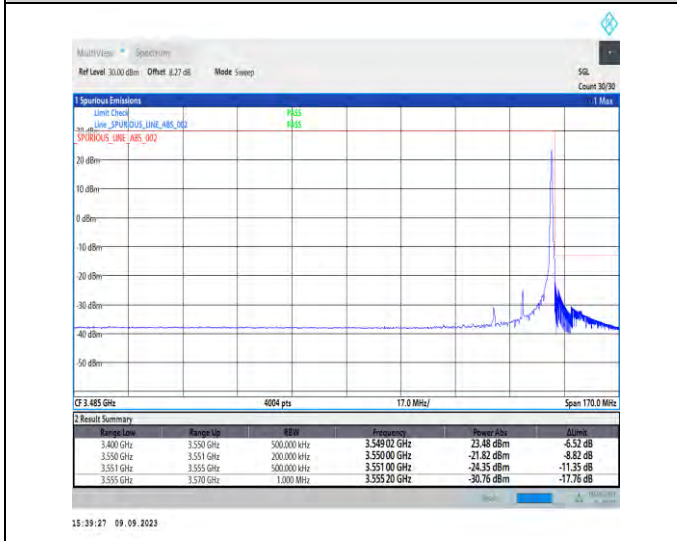
1-N77-3450-3550-PC2-30-20-H-5-CP-QPSK-Edge_1RB_Right-1@50-Ant5-1--PASS-see graph
