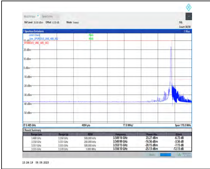
1-N77-3450-3550-PC2-30-15-H-2-DFT-PI2BPSK-Edge_1RB_Right-1@37-Ant5-1--PASS-see graph
