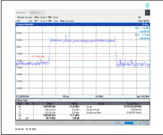
1-N77-3450-3550-PC2-30-70-M-7-CP-16QAM-Outer _Full-189@0-Ant5-67.516-69.720-≤70-PASS
