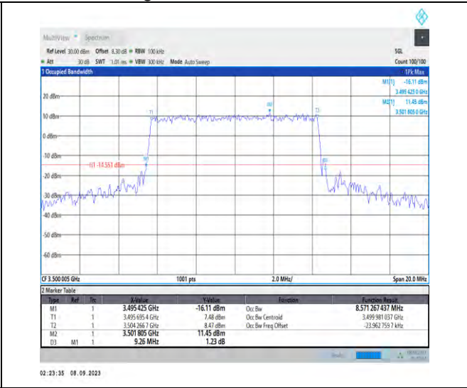
1-N77-3450-3550-PC2-30-10-M-6-CP-QPSK-Outer _Full-24@0-Ant5-8.571-9.260-≤10-PASS
