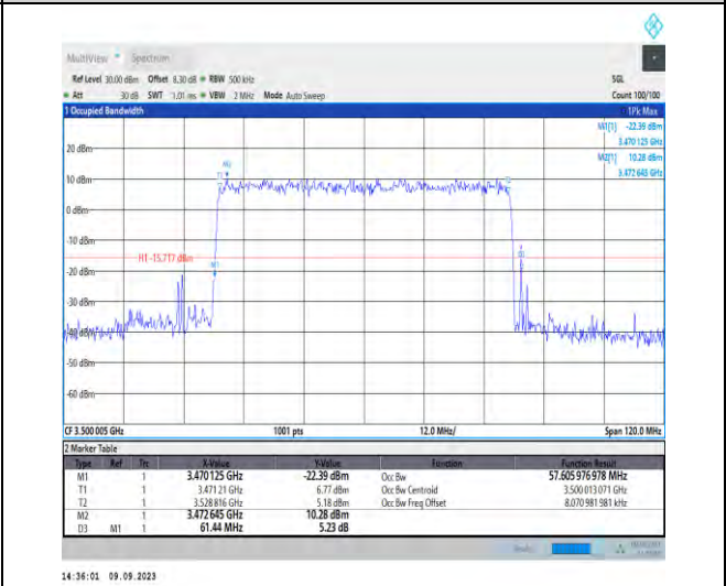
1-N77-3450-3550-PC2-30-60-M-5-DFT-256QAM-Outer_Full-162@0-Ant5-57.606-61.440-≤60-PASS
