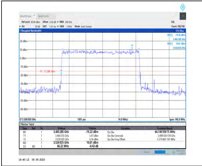
1-N77-3450-3550-PC2-30-70-M-5-DFT-256QAM-Out _Full-180@0-Ant5-64.15-66.220-≤70-PASS
