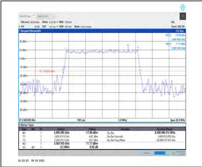
1-N77-3450-3550-PC2-30-10-M-5-DFT-256QAM-Out _Full-24@0-Ant5-8.59-9.200-≤10-PASS
