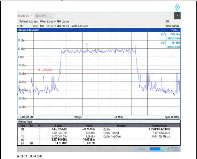
1-N77-3450-3550-PC2-30-15-M-9-CP-256QAM-Outer_Full-38@0-Ant5-13.585-14.250-≤15-PASS
