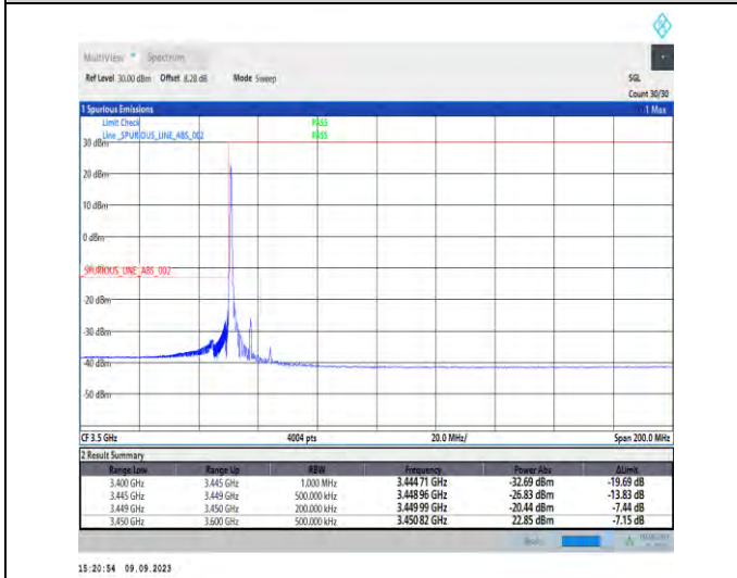
1-N77-3450-3550-PC2-30-15-L-4-CP-QPSK-Edge_1RB_Left-1@0-Ant5-1--PASS-see graph
