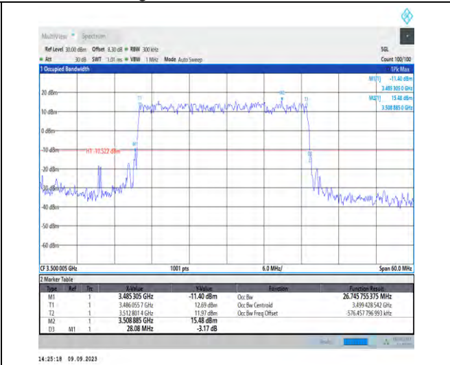
1-N77-3450-3550-PC2-30-30-M-2-DFT-PI2BPSK-Outer_Full-75@0-Ant5-26.746-28.080-≤30-PASS
