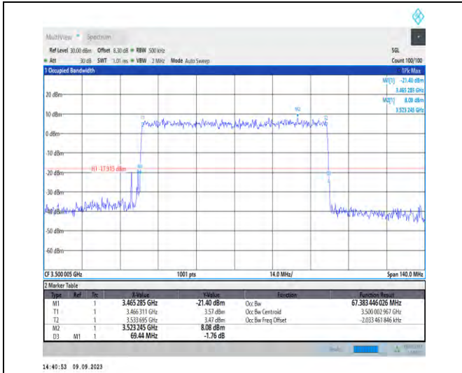
1-N77-3450-3550-PC2-30-70-M-9-CP-256QAM-Outer_Full-189@0-Ant5-67.383-69.440-≤70-PASS
