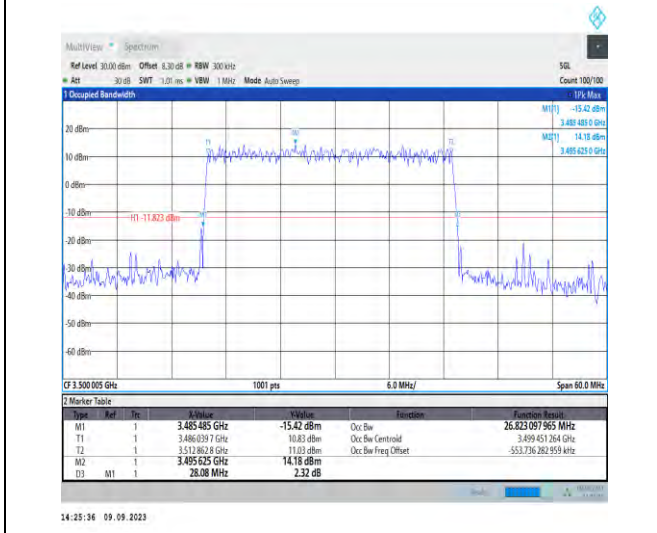
1-N77-3450-3550-PC2-30-30-M-3-DFT-16QAM-Outer_Full-75@0-Ant5-26.823-28.080-≤30-PASS
