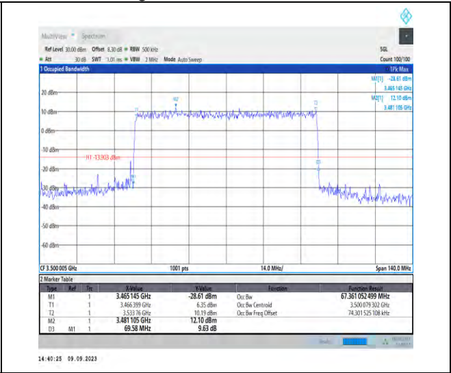
1-N77-3450-3550-PC2-30-70-M-6-CP-QPSK-Outer _Full-189@0-Ant5-67.361-69.580-≤70-PASS
