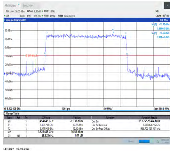
1-N77-3450-3550-PC2-30-90-M-2-DFT-PI2BPSK-Outer_Full-240@0-Ant5-85.676-88.920-≤90-PASS
