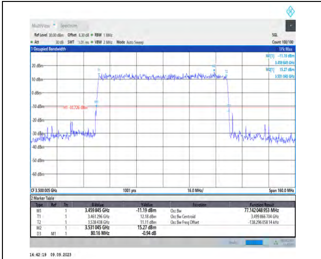
1-N77-3450-3550-PC2-30-80-M-4-DFT-64QAM-Outer_Full-216@0-Ant5-77.142-80.160-≤80-PASS
