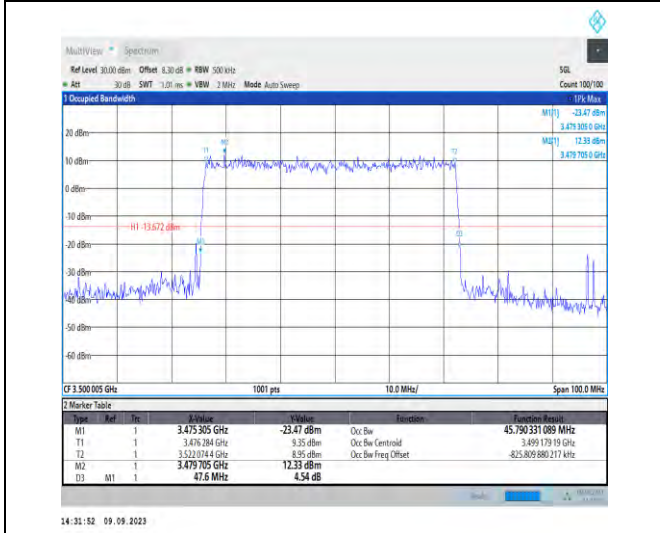
1-N77-3450-3550-PC2-30-50-M-5-DFT-256QAM-Outer_Full-128@0-Ant5-45.79-47.600-≤50-PASS
