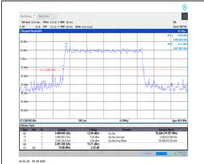
1-N77-3450-3550-PC2-30-20-M-7-CP-16QAM-Outer_Full-51@0-Ant5-18.206-19.080-≤20-PASS
