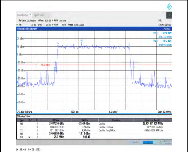
1-N77-3450-3550-PC2-30-25-M-5-DFT-256QAM-Outer_Full-64@0-Ant5-22.904-25.300-≤25-PASS
