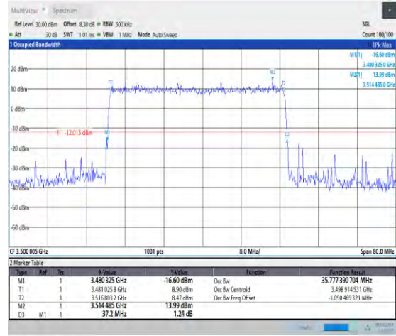
1-N77-3450-3550-PC2-30-40-M-5-DFT-256QAM-Outer_Full-100@0-Ant5-35.777-37.200-≤40-PASS
