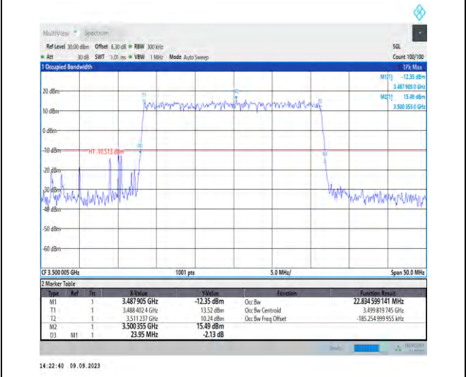
1-N77-3450-3550-PC2-30-25-M-1-DFT-QPSK-Outer_Full-64@0-Ant5-22.835-23.950-≤25-PASS
