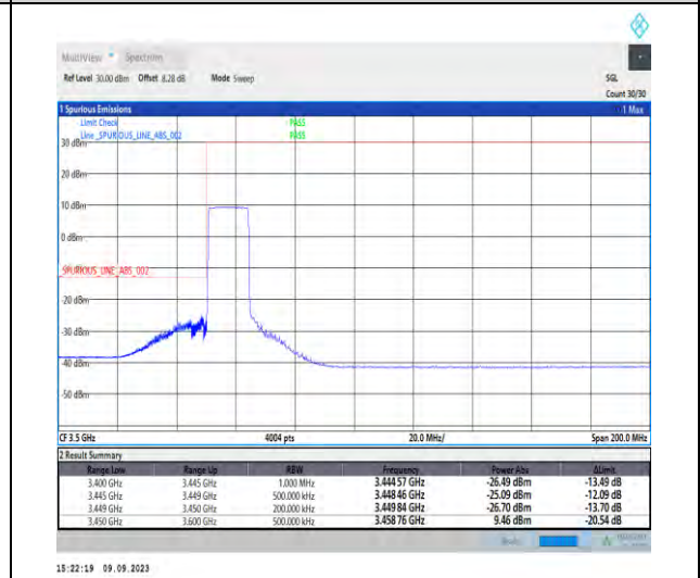
1-N77-3450-3550-PC2-30-15-L-6-CP-QPSK-Outer_Full-38@0-Ant5-1--PASS-see graph
