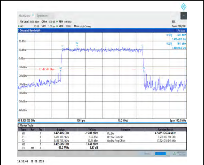
1-N77-3450-3550-PC2-30-50-M-6-CP-QPSK-Outer_Full-133@0-Ant5-47.425-49.200-≤50-PASS
