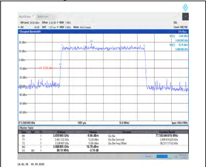
1-N77-3450-3550-PC2-30-80-M-1-DFT-QPSK-Outer_Full-216@0-Ant5-77.166-80.160-≤80-PASS
