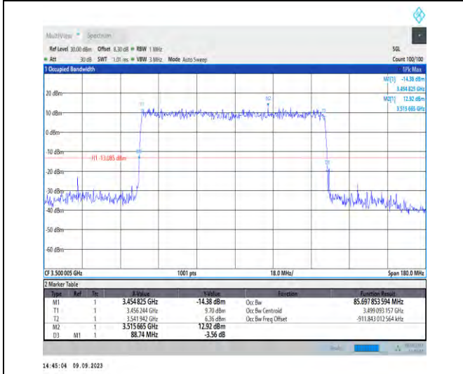
1-N77-3450-3550-PC2-30-90-M-5-DFT-256QAM-Outer_Full-240@0-Ant5-85.698-88.740-≤90-PASS
