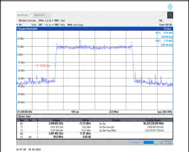
1-N77-3450-3550-PC2-30-100-M-5-DFT-256QAM-Outer_Full-270@0-Ant5-96.229-99.800-≤100-PASS
