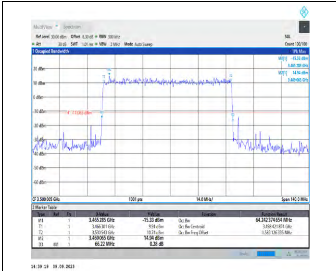
1-N77-3450-3550-PC2-30-70-M-1-DFT-QPSK-Outer_Full-180@0-Ant5-64.242-66.220-≤70-PASS
