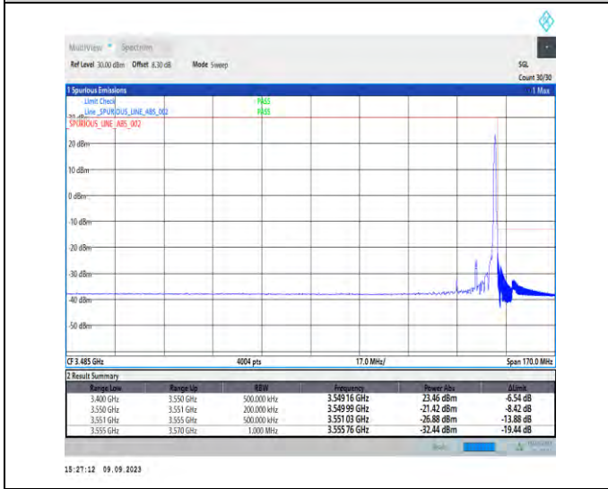
1-N77-3450-3550-PC2-30-15-H-5-CP-QPSK-Edge_1RB_Right-1@37-Ant5-1--PASS-see graph
