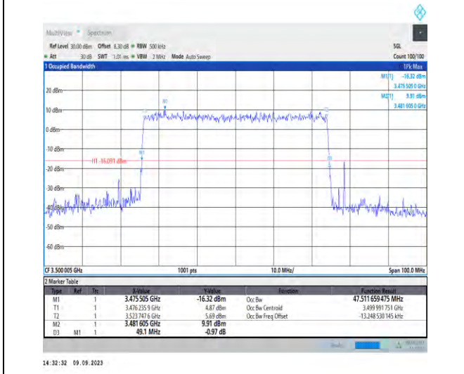
1-N77-3450-3550-PC2-30-50-M-9-CP-256QAM-Outer _Full-133@0-Ant5-47.512-49.100-≤50-PASS
