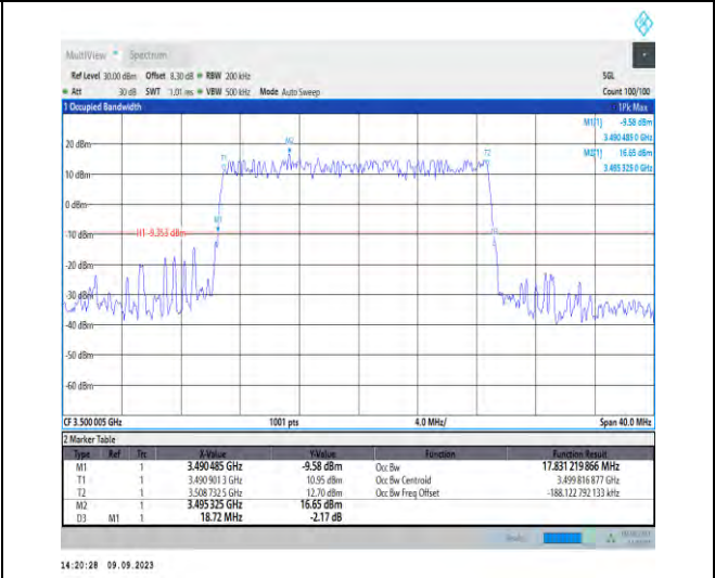
1-N77-3450-3550-PC2-30-20-M-2-DFT-PI2BPSK-Outer_Full-50@0-Ant5-17.831-18.720-≤20-PASS
