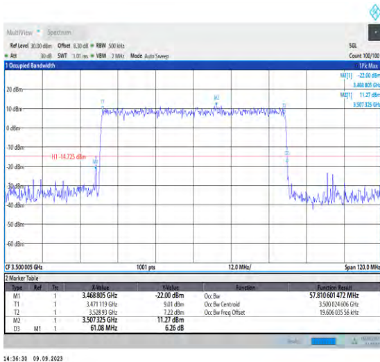
1-N77-3450-3550-PC2-30-60-M-8-CP-64QAM-Outer_Full-162@0-Ant5-57.811-61.080-≤60-PASS
