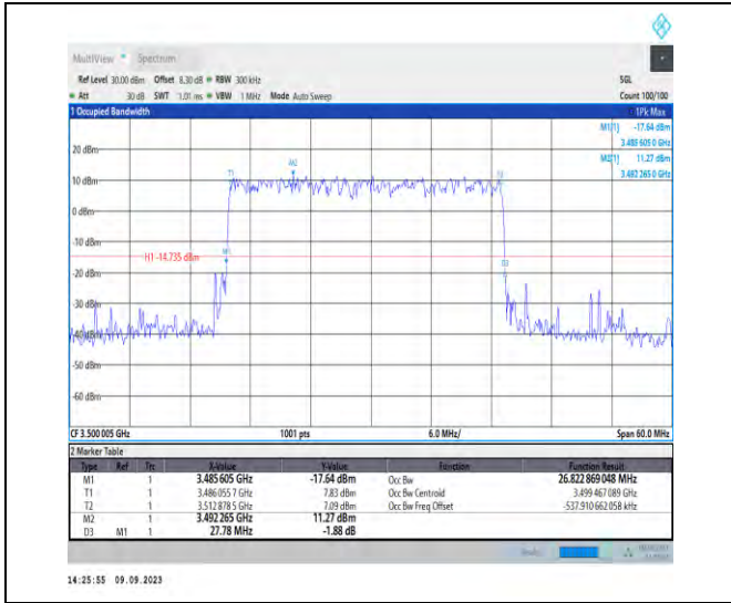
1-N77-3450-3550-PC2-30-30-M-5-DFT-256QAM-Out _Full-75@0-Ant5-26.823-27.780-≤30-PASS
