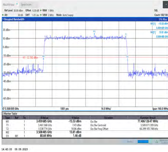
1-N77-3450-3550-PC2-30-80-M-8-CP-64QAM-Outer_Full-217@0-Ant5-77.406-80.640-≤80-PASS
