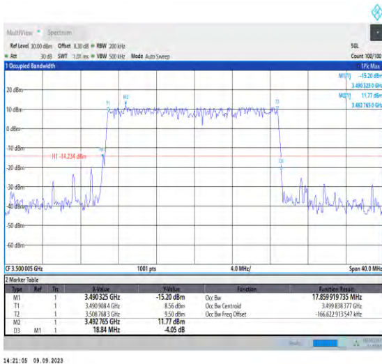
1-N77-3450-3550-PC2-30-20-M-5-DFT-256QAM-Outer_Full-50@0-Ant5-17.86-18.840-≤20-PASS
