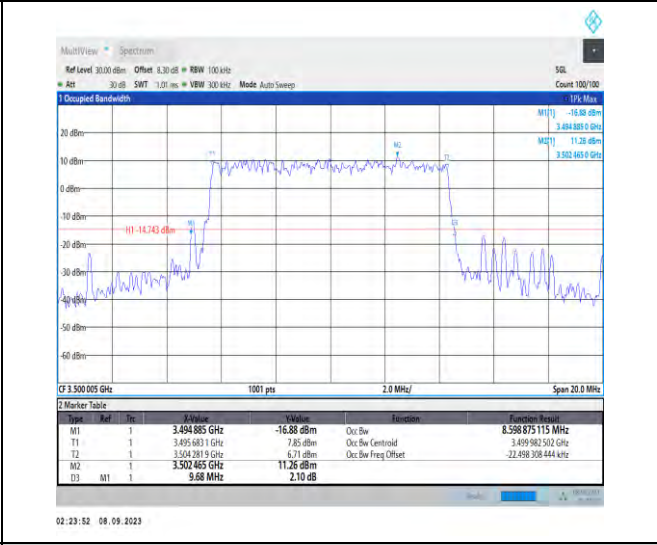
1-N77-3450-3550-PC2-30-10-M-8-CP-64QAM-Outer _Full-24@0-Ant5-8.599-9.680-≤10-PASS
