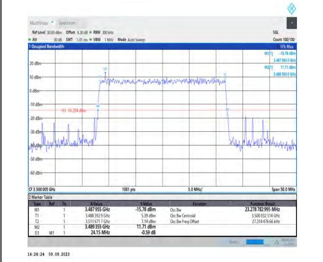
1-N77-3450-3550-PC2-30-25-M-9-CP-256QAM-Outer_Full-65@0-Ant5-23.279-24.150-≤25-PASS
