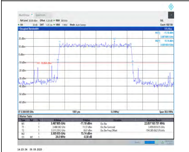
1-N77-3450-3550-PC2-30-25-M-4-DFT-64QAM-Outer_Full-64@0-Ant5-22.857-24.000-≤25-PASS
