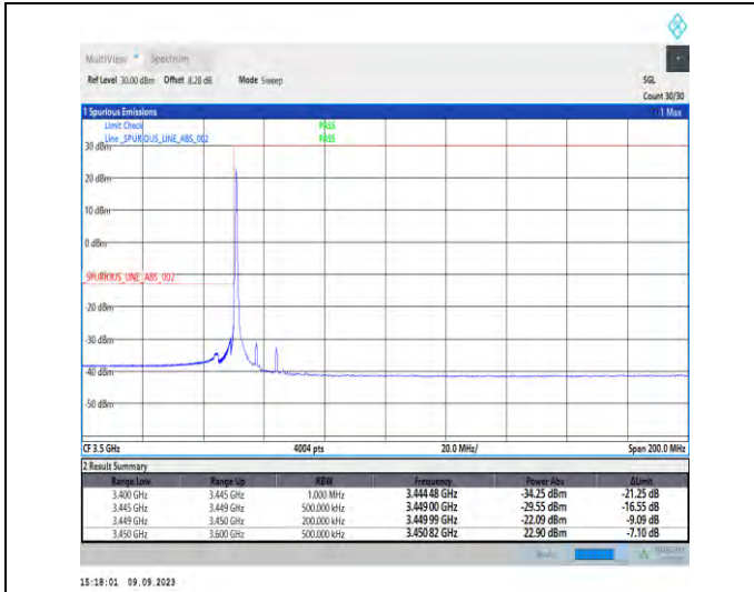
1-N77-3450-3550-PC2-30-15-L-1-DFT-PI2BPSK-Edge_1RB_Left-1@0-Ant5-1--PASS-see graph
