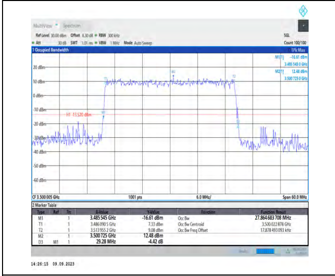
1-N77-3450-3550-PC2-30-30-M-7-CP-16QAM-Outer _Full-78@0-Ant5-27.865-29.280-≤30-PASS
