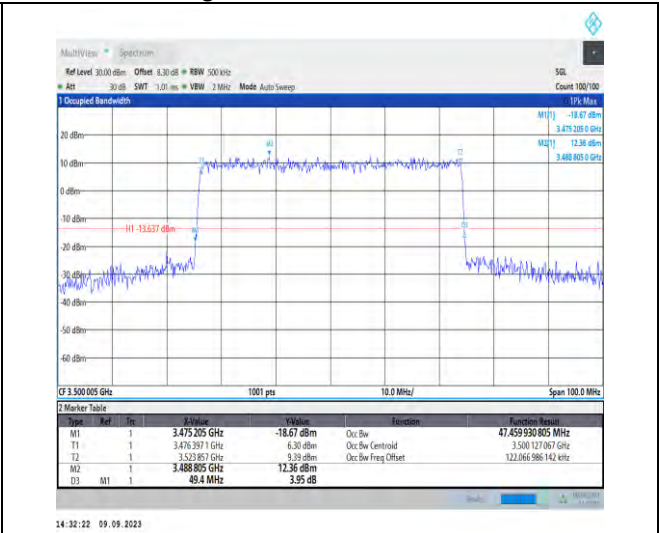
1-N77-3450-3550-PC2-30-50-M-8-CP-64QAM-Outer _Full-133@0-Ant5-47.46-49.400-≤50-PASS
