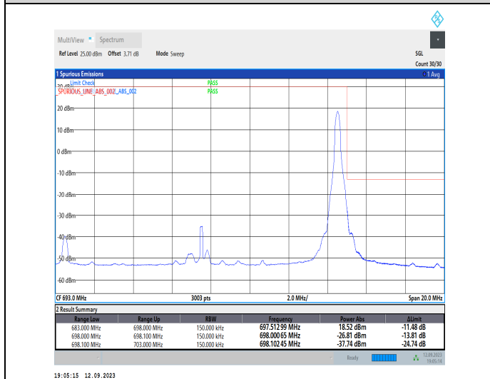
1-N71-PC3-15-15-H-5-CP-QPSK-Edge_1RB_Right-1 @78-Ant1-1--PASS-see graph
