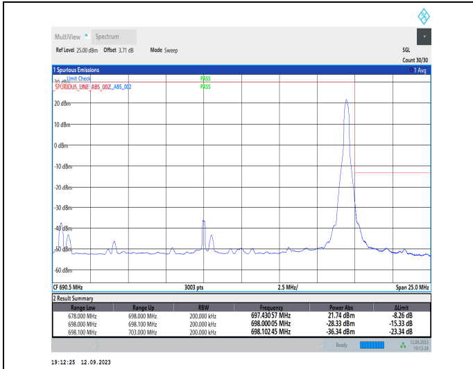
1-N71-PC3-15-20-H-2-DFT-PI2BPSK-Edge_1RB_Righ t-1@105-Ant1-1--PASS-see graph
