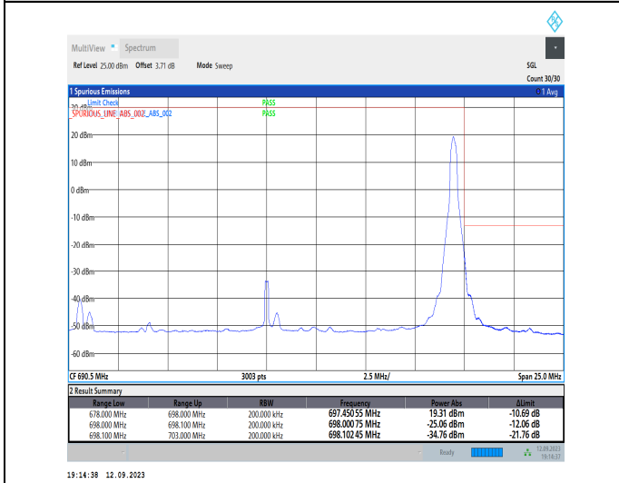
1-N71-PC3-15-20-H-5-CP-QPSK-Edge_1RB_Right-1 @105-Ant1-1--PASS-see graph
