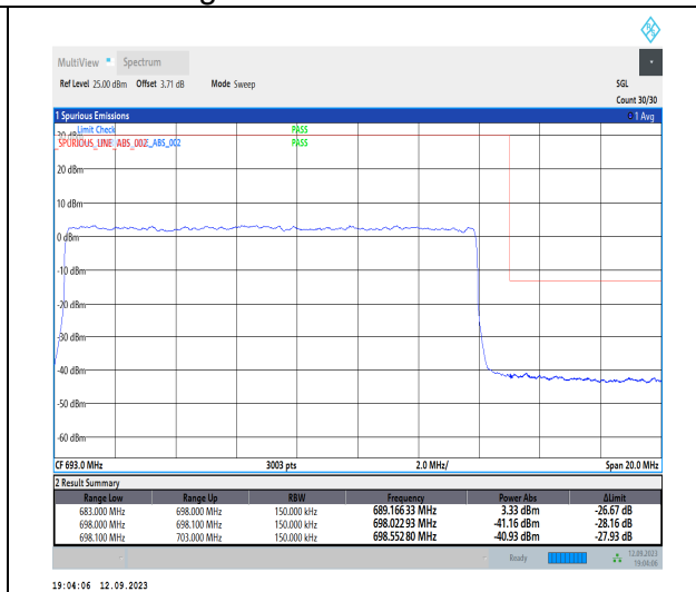
1-N71-PC3-15-15-H-3-DFT-PI2BPSK-Outer_Full-7 5@0-Ant1-1--PASS-see graph
