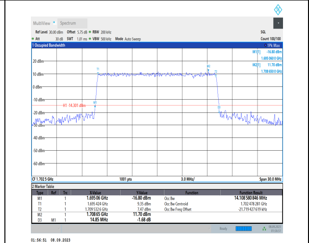
1-N70-PC3-15-15-M-6-CP-QPSK-Outer_Full-79@0- Ant2-14.109-14.850≤15-PASS
