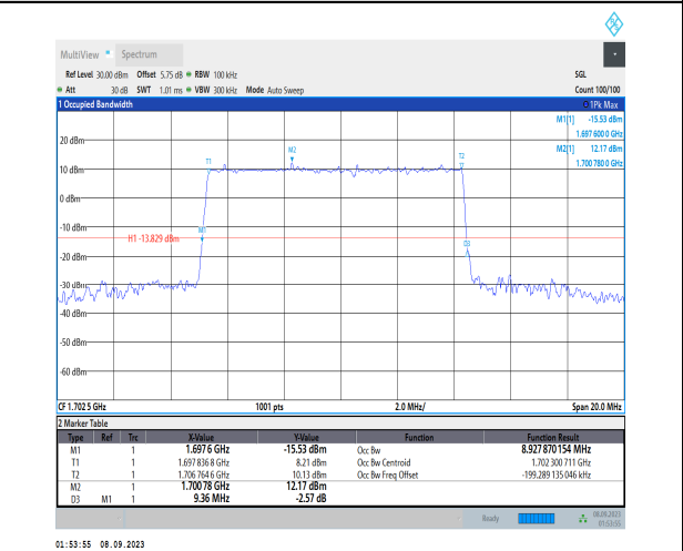
1-N70-PC3-15-10-M-3-DFT-16QAM-Outer_Full-50@0 -Ant2-8.928-9.360-≤10-PASS
