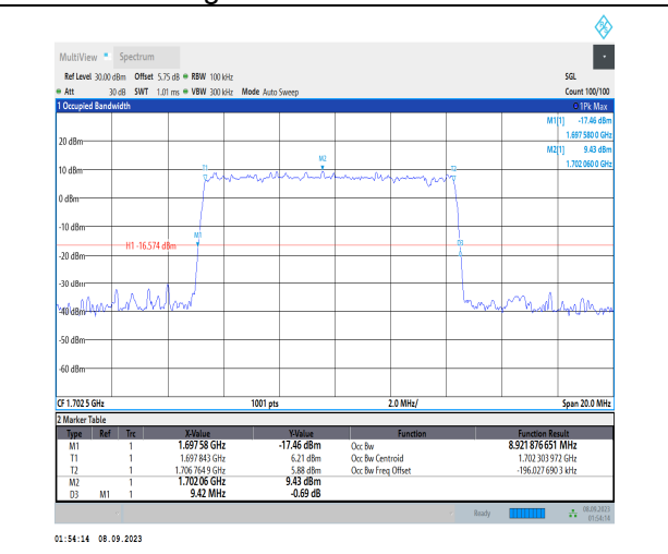
1-N70-PC3-15-10-M-5-DFT-256QAM-Outer_Full-50 @0-Ant2-8.922-9.420-≤10-PASS
