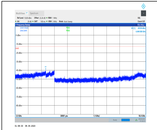
1-N70-PC3-15-15-L-1-DFT-PI2BPSK-Inner_1RB_Le ft-1@1-3000-18000-Ant2-6494.50--39.58--13-PASS
