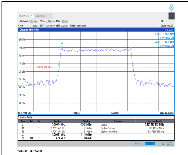
1-N70-PC3-15-5-M-5-DFT-256QAM-Outer_Full-25@ 0-Ant2-4.467-4.740-≤5-PASS
