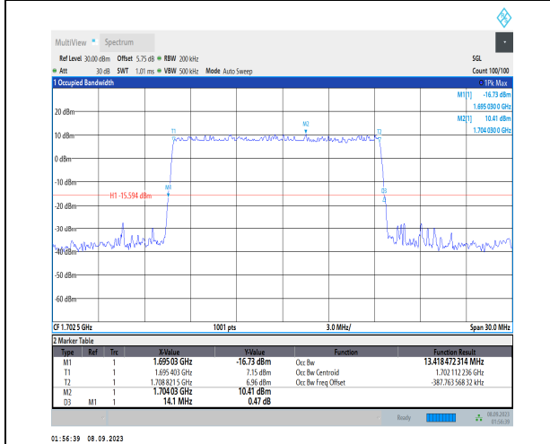
1-N70-PC3-15-15-M-5-DFT-256QAM-Outer_Full-75 @0-Ant2-13.418-14.100≤15-PASS
