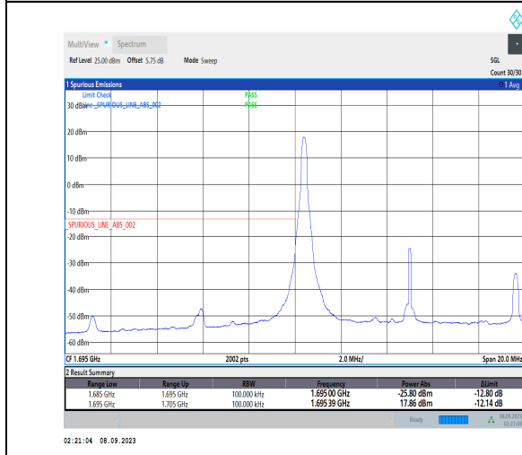
1-N70-PC3-15-10-L-4-CP-QPSK-Edge_1RB_Left-1@0-Ant2-1-seegraph-PASS-see graph
