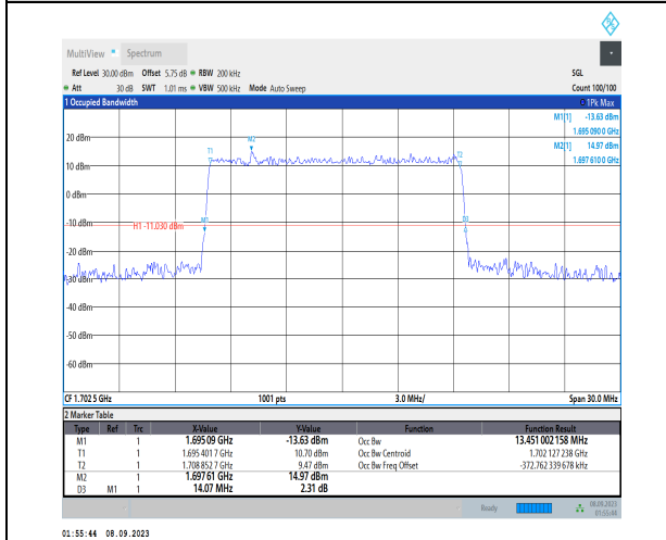
1-N70-PC3-15-15-M-1-DFT-QPSK-Outer_Full-75@0 -Ant2-13.451-14.070-≤15-PASS
