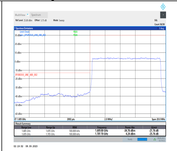
1-N70-PC3-15-10-L-3-DFT-PI2BPSK-Outer_Full-50@0-Ant2-1-seegraph-PASS-see graph
