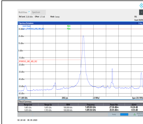
1-N70-PC3-15-10-L-1-DFT-PI2BPSK-Edge_1RB_Left-1@0-Ant2-1-seegraph-PASS-see graph
