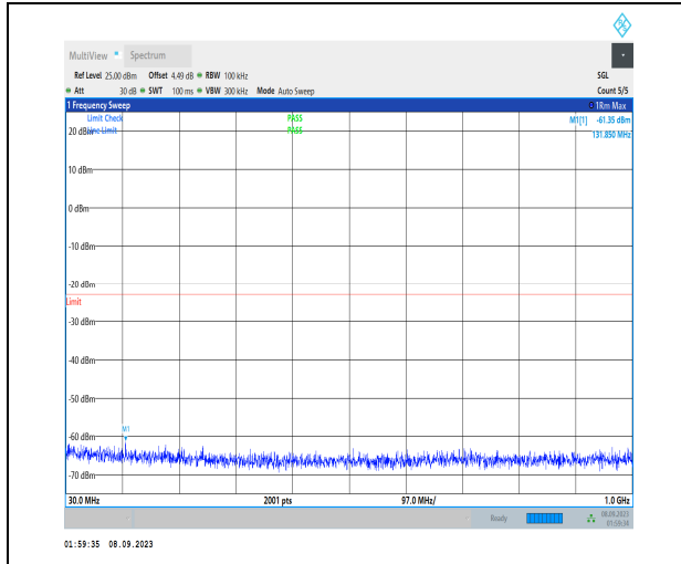
1-N70-PC3-15-15-H-1-DFT-PI2BPSK-Inner_1RB_Le ft-1@1-30-1000-Ant2-131.85--61.35--23-PASS
