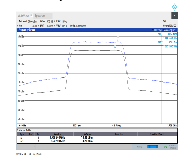
1-N70-PC3-15-15-H-2-CP-256QAM-Outer_Full-79@ 0-Ant2-9.64-100%-0.00-9.64-PASS-≤13
