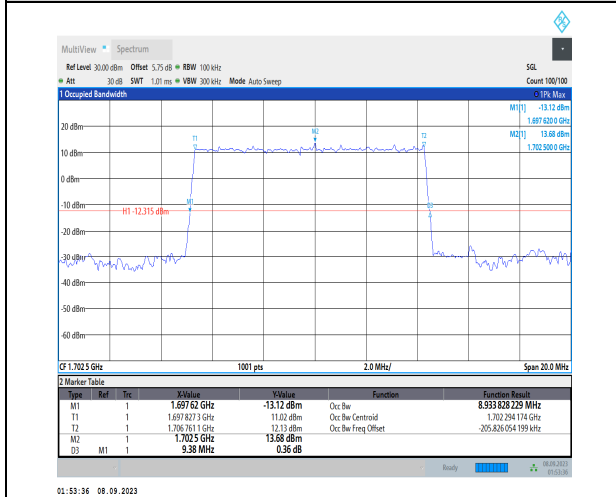
1-N70-PC3-15-10-M-2-DFT-PI2BPSK-Outer_Full-50@0 -Ant2-8.934-9.380-≤10-PASS
