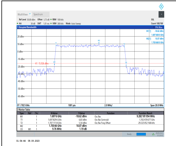
1-N70-PC3-15-10-M-8-CP-64QAM-Outer_Full-52@0 -Ant2-9.282-9.760-≤10-PASS
