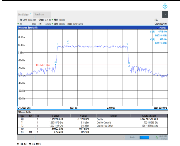
1-N70-PC3-15-10-M-6-CP-QPSK-Outer_Full-52@0- Ant2-9.272-9.760-≤10-PASS
