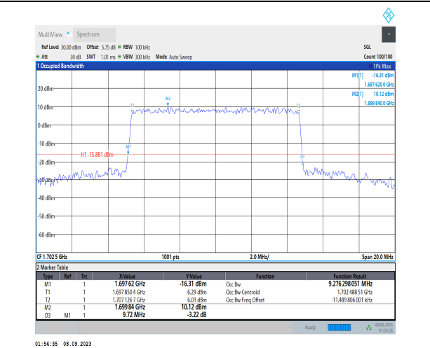
1-N70-PC3-15-10-M-7-CP-16QAM-Outer_Full-52@0 -Ant2-9.276-9.720-≤10-PASS
