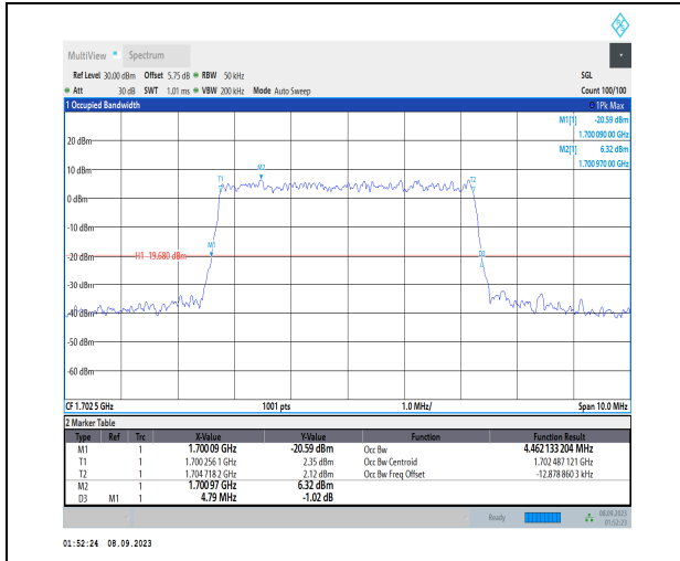
1-N70-PC3-15-5-M-9-CP-256QAM-Outer_Full-25@0 -Ant2-4.462-4.790-≤5-PASS
