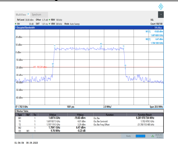
1-N70-PC3-15-10-M-9-CP-256QAM-Outer_Full-52@0 -Ant2-9.282-9.760-≤10-PASS
