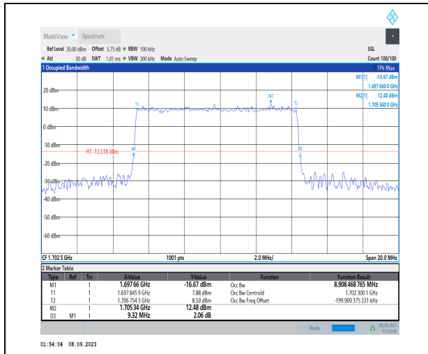
1-N70-PC3-15-10-M-4-DFT-64QAM-Outer_Full-50@ 0-Ant2-8.908-9.320-≤10-PASS
