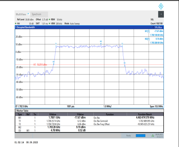
1-N70-PC3-15-5-M-8-CP-64QAM-Outer_Full-25@0- Ant2-4.463-4.780-≤5-PASS
