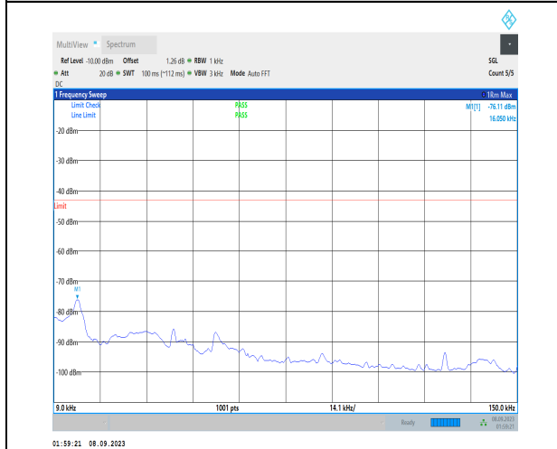
1-N70-PC3-15-15-H-1-DFT-PI2BPSK-Inner_1RB_Le ft-1@1-0.009-0.15-Ant2-0.02--76.11--43-PASS
