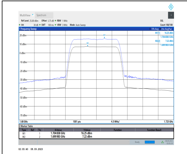
1-N70-PC3-15-15-H-1-DFT-256QAM-Outer_Full-75 @0-Ant2-9.03-100%-0.00-9.03-PASS-≤13
