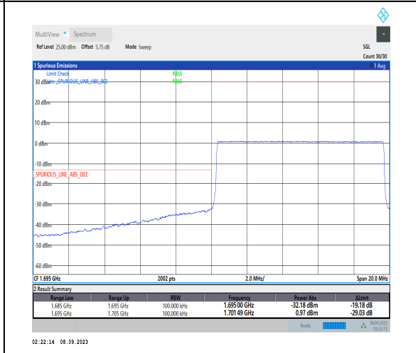
1-N70-PC3-15-10-L-6-CP-QPSK-Outer_Full-52@0-Ant2-1-seegraph-PASS-see graph
