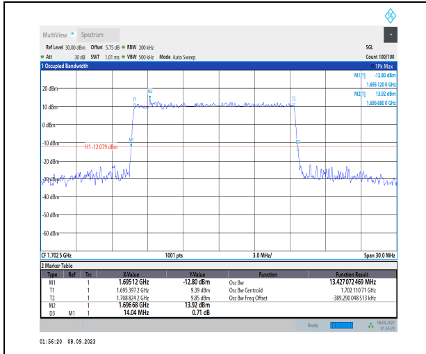
1-N70-PC3-15-15-M-3-DFT-16QAM-Outer_Full-75@ 0-Ant2-13.427-14.040≤15-PASS
