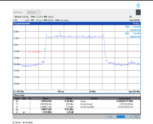
1-N70-PC3-15-15-M-2-DFT-PI2BPSK-Outer_Full-75@0 -Ant2-13.444-14.160-≤15-PASS
