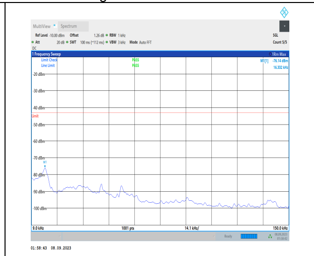
1-N70-PC3-15-15-M-1-DFT-PI2BPSK-Inner_1RB_Le ft-1@1-0.009-0.15-Ant2-0.02--76.14--43-PASS
