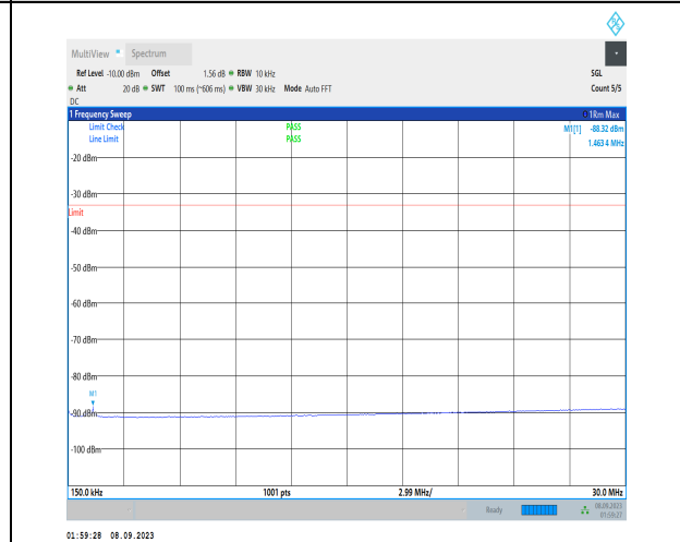
1-N70-PC3-15-15-H-1-DFT-PI2BPSK-Inner_1RB_Le ft-1@1-0.15-30-Ant2-1.46--88.32--33-PASS
