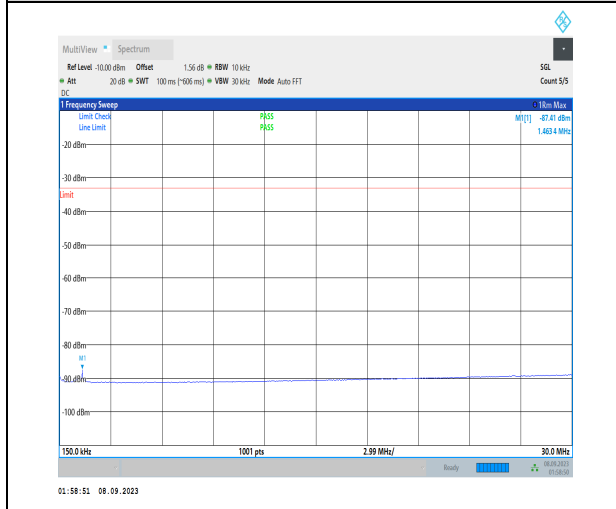
1-N70-PC3-15-15-M-1-DFT-PI2BPSK-Inner_1RB_Le ft-1@1-0.15-30-Ant2-1.46--87.41--33-PASS
