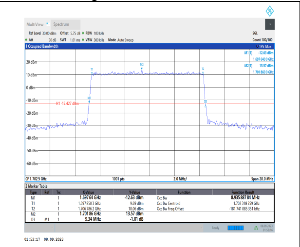
1-N70-PC3-15-10-M-1-DFT-QPSK-Outer_Full-50@0 -Ant2-8.936-9.340-≤10-PASS
