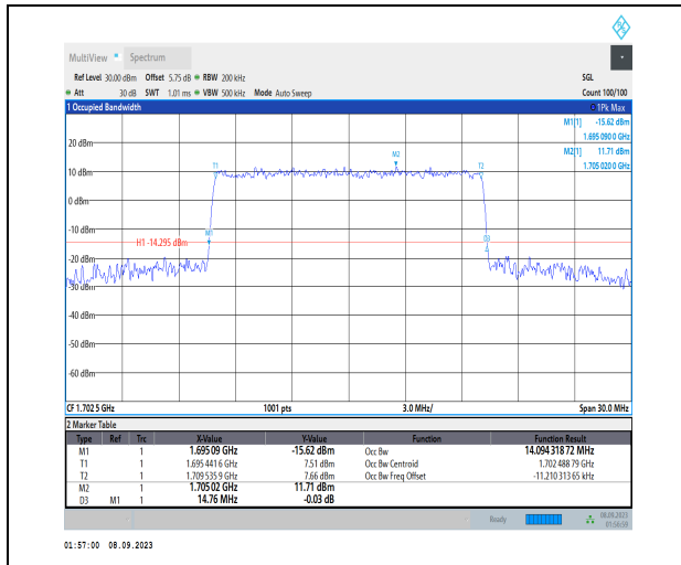
1-N70-PC3-15-15-M-7-CP-16QAM-Outer_Full-79@0 -Ant2-14.094-14.760-≤15-PASS
