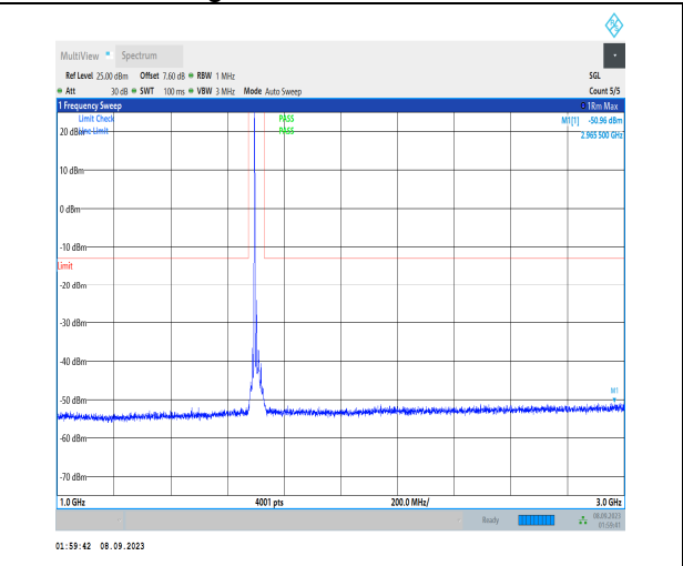
1-N70-PC3-15-15-H-1-DFT-PI2BPSK-Inner_1RB_Le ft-1@1-1000-3000-Ant2-2965.50--50.96--13-PASS
