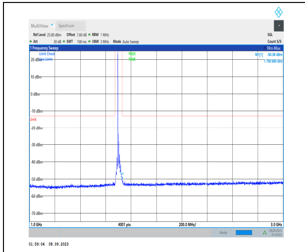
1-N70-PC3-15-15-M-1-DFT-PI2BPSK-Inner_1RB_Le ft-1@1-1000-3000-Ant2-1730.50--50.38--13-PASS
