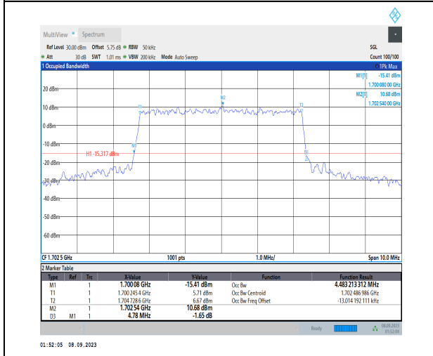
1-N70-PC3-15-5-M-7-CP-16QAM-Outer_Full-25@0- Ant2-4.483-4.780-≤5-PASS
