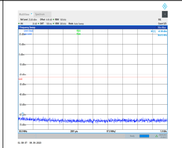
1-N70-PC3-15-15-M-1-DFT-PI2BPSK-Inner_1RB_Le ft-1@1-30-1000-Ant2-58.62--61.98--23-PASS
