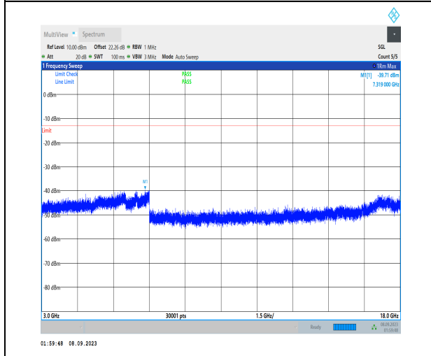
1-N70-PC3-15-15-H-1-DFT-PI2BPSK-Inner_1RB_Le ft-1@1-3000-18000-Ant2-7319.00--39.71--13-PASS
