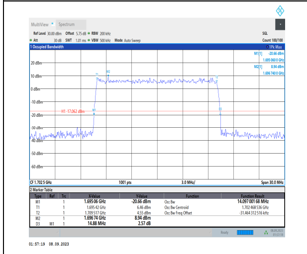
1-N70-PC3-15-15-M-9-CP-256QAM-Outer_Full-79@0 -Ant2-14.097-14.880-≤15-PASS
