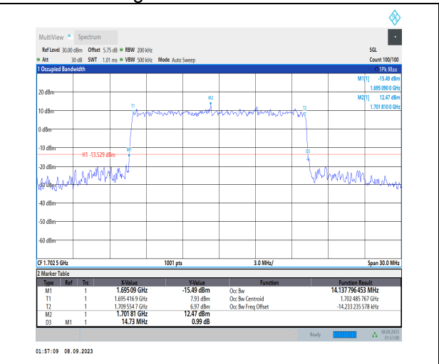
1-N70-PC3-15-15-M-8-CP-64QAM-Outer_Full-79@0 -Ant2-14.138-14.730-≤15-PASS
