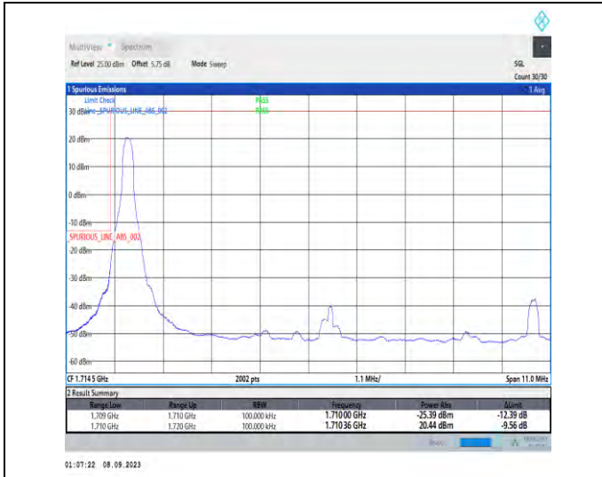
1-N66-PC3-15-10-L-1-DFT-PI2BPSK-Edge_1RB_Left-1@0-Ant2-1-seegraph-PASS-see graph
