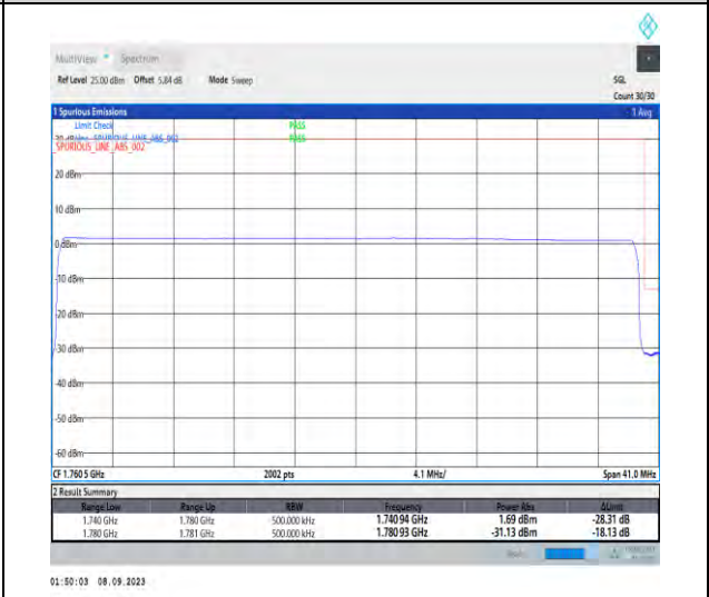
1-N66-PC3-15-40-H-6-CP-QPSK-Outer_Full-216@0-Ant2-1-seegraph-PASS-see graph
