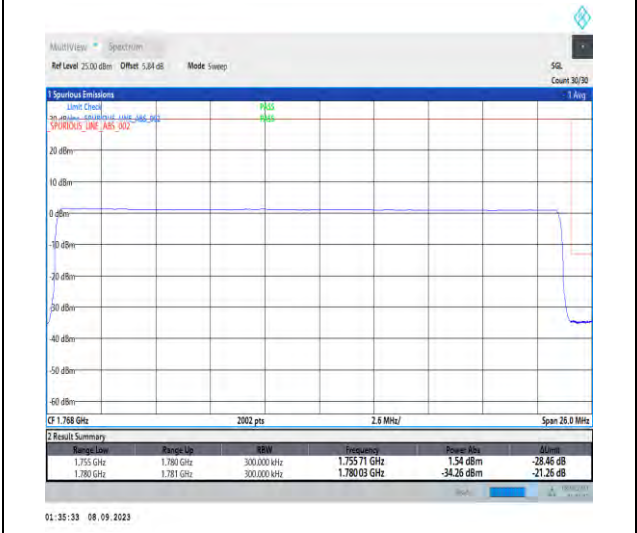
1-N66-PC3-15-25-H-6-CP-QPSK-Outer_Full-133@0-Ant2-1-seegraph-PASS-see graph
