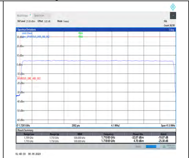
1-N66-PC3-15-40-L-3-DFT-PI2BPSK-Outer_Full-216@0-Ant2-1-seegraph-PASS-see graph
