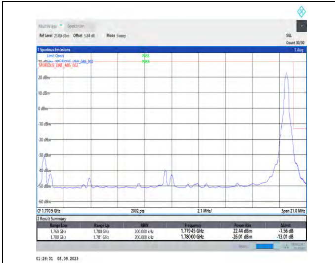
1-N66-PC3-15-20-H-2-DFT-PI2BPSK-Edge_1RB_Right-t-1@105-Ant2-1-seegraph-PASS-see graph
