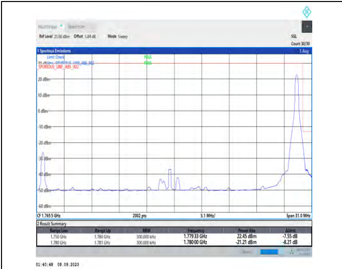
1-N66-PC3-15-30-H-2-DFT-PI2BPSK-Edge_1RB_Right-t-1@159-Ant2-1-seegraph-PASS-see graph
