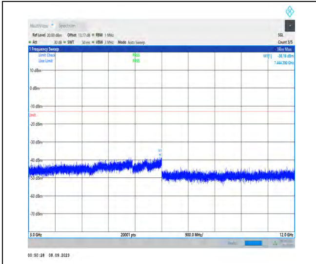
1-N66-PC3-15-40-H-1-DFT-PI2BPSK-Inner_1RB_L eft-1@1-3000-12000-Ant2-7444.20--38.18--13-PAS S
