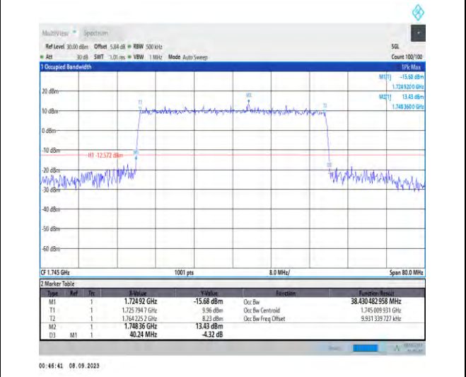
1-N66-PC3-15-40-M-6-CP-QPSK-Outer_Full-216 @0-Ant2-38.43-40.240-≤40-PASS
