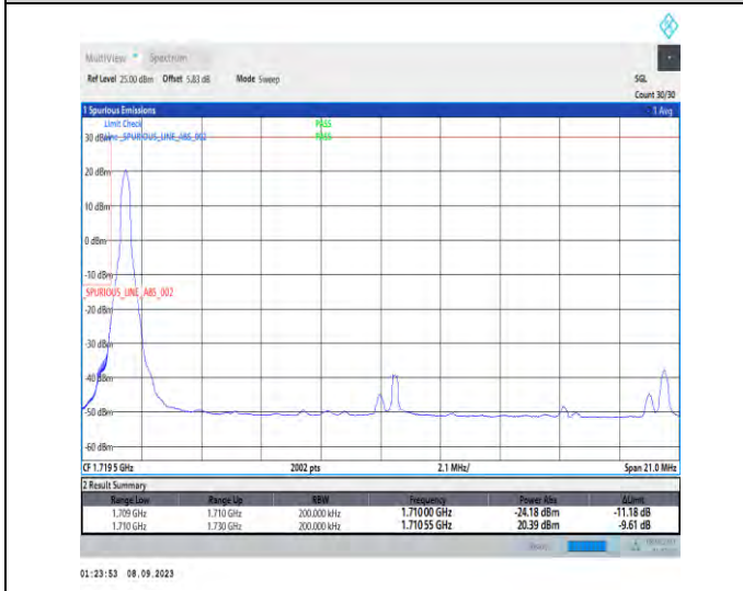
1-N66-PC3-15-20-L-4-CP-QPSK-Edge_1RB_Left-1@0-Ant2-1-seegraph-PASS-see graph
