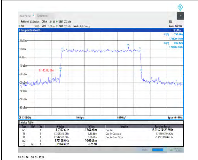
1-N66-PC3-15-20-M-8-CP-64QAM-Outer_Full-106@0 0-Ant2-18.915-19.640-≤20-PASS
