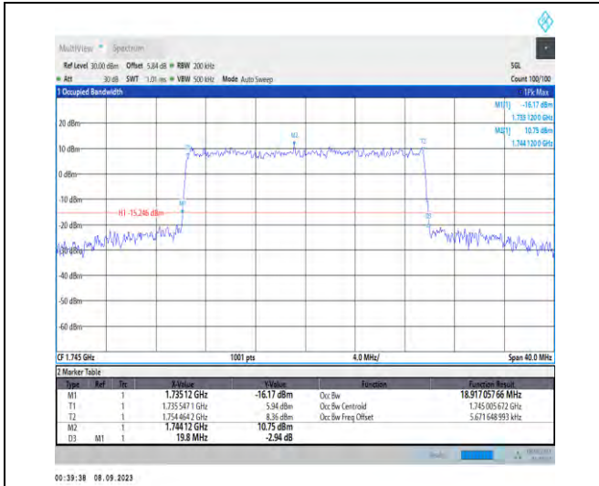
1-N66-PC3-15-20-M-6-CP-QPSK-Outer_Full-106@0 -Ant2-18.917-19.800-≤20-PASS
