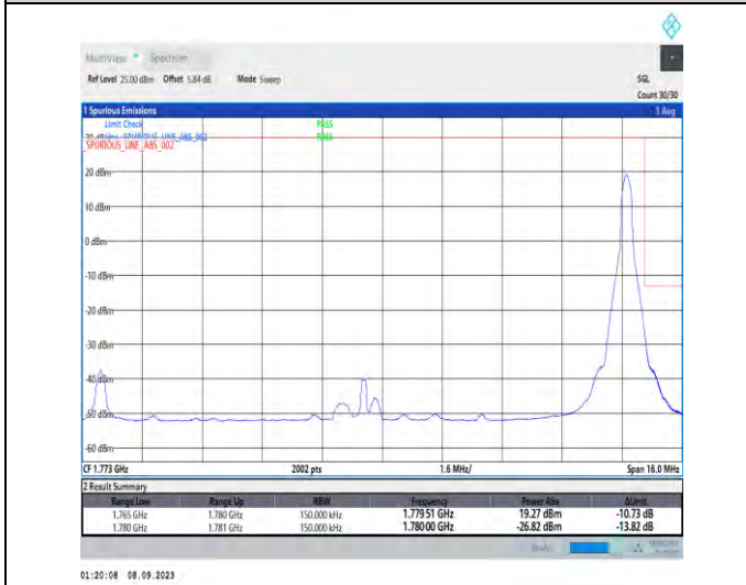
1-N66-PC3-15-15-H-5-CP-QPSK-Edge_1RB_Right-1 @78-Ant2-1-seegraph-PASS-see graph
