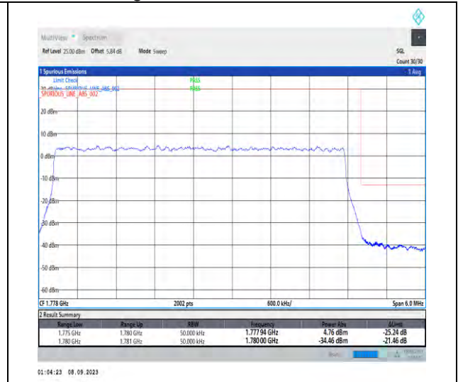
1-N66-PC3-15-5-H-3-DFT-PI2BPSK-Outer_Full-25@0-Ant2-1-seegraph-PASS-see graph
