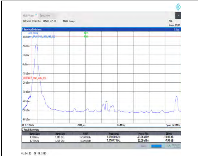
1-N66-PC3-15-15-L-1-DFT-PI2BPSK-Edge_1RB_Left-1@0-Ant2-1-seegraph-PASS-see graph
