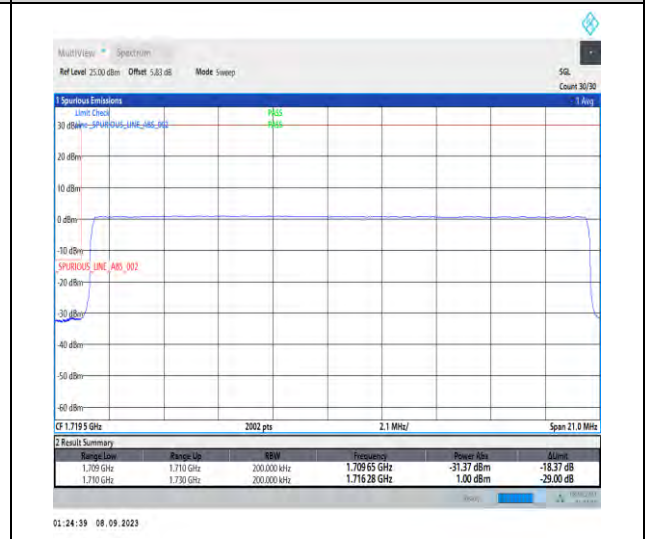
1-N66-PC3-15-20-L-6-CP-QPSK-Outer_Full-106@0-Ant2-1-seegraph-PASS-see graph
