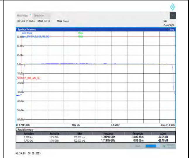
1-N66-PC3-15-30-L-6-CP-QPSK-Outer_Full-160@0-Ant2-1-seegrph-PASS-see graph
