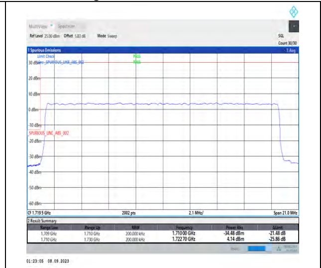
1-N66-PC3-15-20-L-3-DFT-PI2BPSK-Outer_Full-100@0-Ant2-1-seegraph-PASS-see graph
