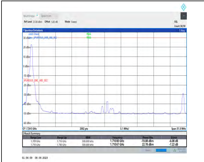
1-N66-PC3-15-30-L-1-DFT-PI2BPSK-Edge_1RB_Left-1@0-Ant2-1-seegrph-PASS-see graph
