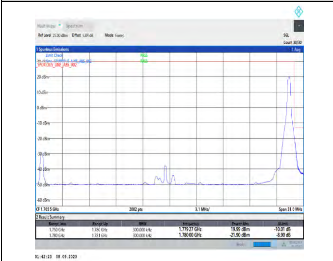
1-N66-PC3-15-30-H-5-CP-QPSK-Edge_1RB_Right-1@159-Ant2-1-seegraph-PASS-see graph
