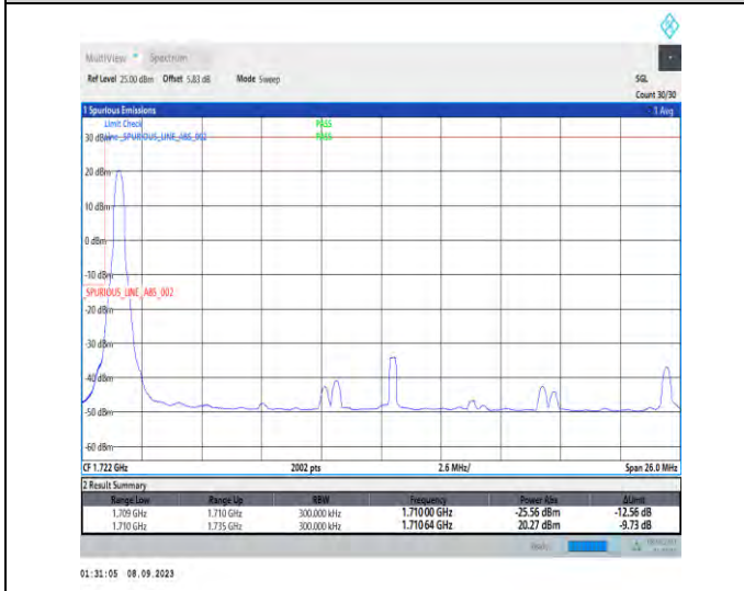
1-N66-PC3-15-25-L-4-CP-QPSK-Edge_1RB_Left-1@0-Ant2-1-seegraph-PASS-see graph
