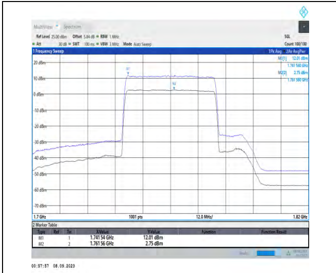
1-N66-PC3-15-40-H-1-DFT-256QAM-Outer_Full-216 @0-Ant2-9.26-100%-0.00-9.26-PASS-≤13
