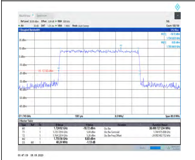
1-N66-PC3-15-40-M-9-CP-256QAM-Outer_Full-216 @0-Ant2-38.491-40.240-≤40-PASS
