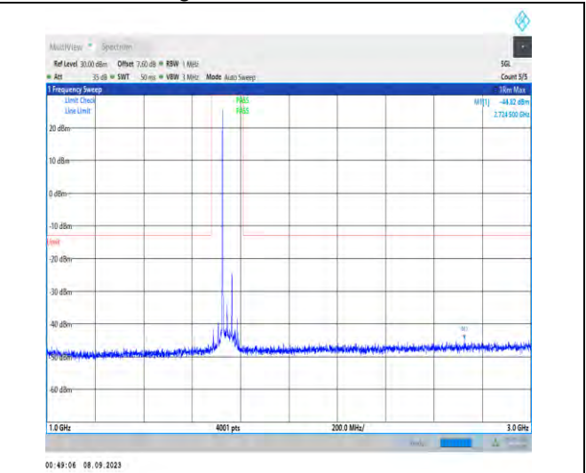
1-N66-PC3-15-40-M-1-DFT-PI2BPSK-Inner_1RB_L ef t-1@1-1000-3000-Ant2-2724.50--44.82--13-PASS
