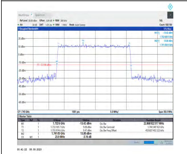
1-N66-PC3-15-25-M-3-DFT-16QAM-Outer_Full-128 @0-Ant2-22.869-23.900-≤25-PASS
