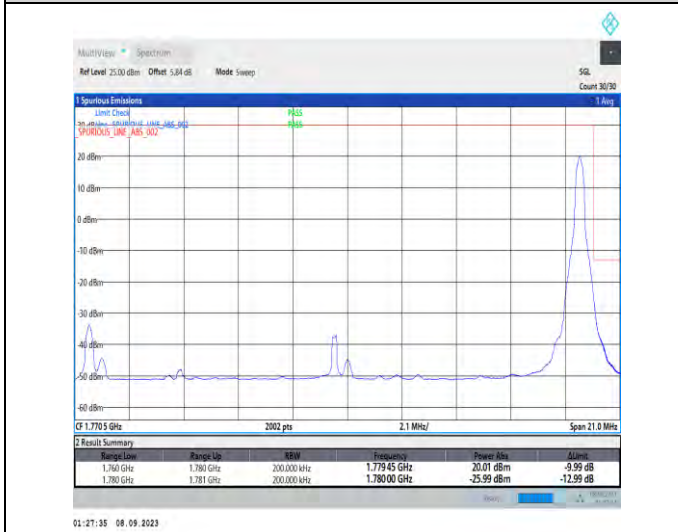
1-N66-PC3-15-20-H-5-CP-QPSK-Edge_1RB_Right-1@105-Ant2-1-seegraph-PASS-see graph
