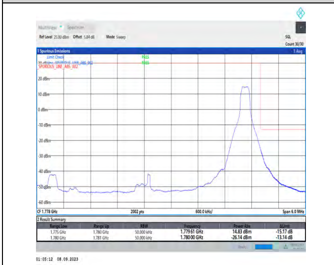
1-N66-PC3-15-5-H-5-CP-QPSK-Edge_1RB_Right-1@24-Ant2-1-seegraph-PASS-see graph
