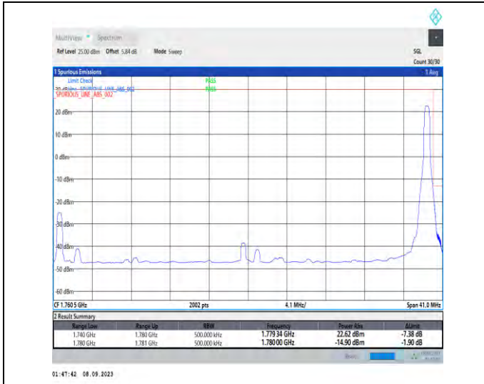
1-N66-PC3-15-40-H-2-DFT-PI2BPSK-Edge_1RB_Right-t-1@215-Ant2-1-seegraph-PASS-see graph
