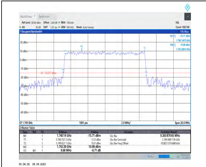
1-N66-PC3-15-10-M-8-CP-64QAM-Outer_Full-52@0 -Ant2-9.264-9.680-≤10-PASS
