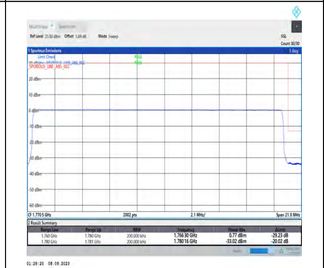
1-N66-PC3-15-20-H-6-CP-QPSK-Outer_Full-106@0-Ant2-1-seegraph-PASS-see graph
