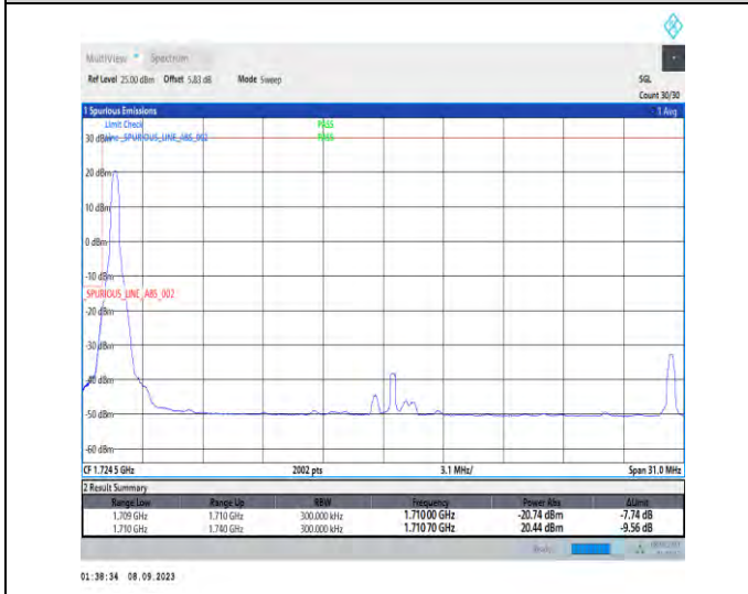
1-N66-PC3-15-30-L-4-CP-QPSK-Edge_1RB_Left-1@0-Ant2-1-seegrph-PASS-see graph
