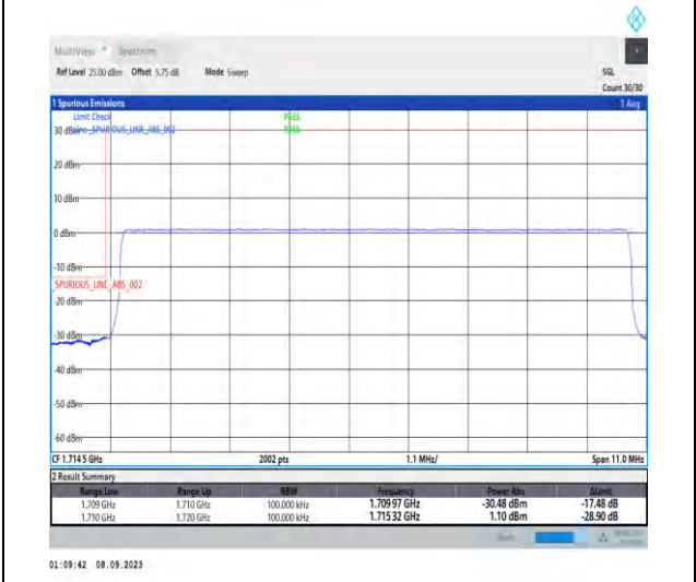
1-N66-PC3-15-10-L-6-CP-QPSK-Outer_Full-52@0-Ant2-1-seegraph-PASS-see graph
