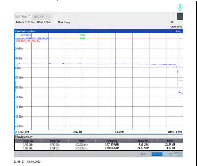
1-N66-PC3-15-40-H-3-DFT-PI2BPSK-Outer_Full-216@0-Ant2-1-seegraph-PASS-see graph
