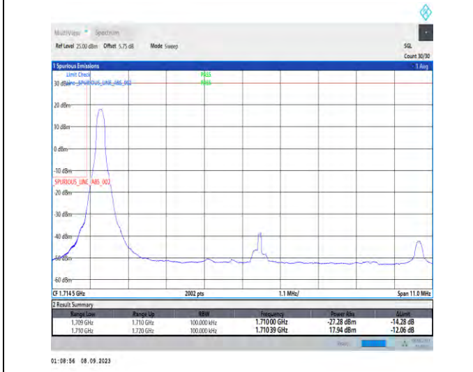
1-N66-PC3-15-10-L-4-CP-QPSK-Edge_1RB_Left-1@0-Ant2-1-seegraph-PASS-see graph
