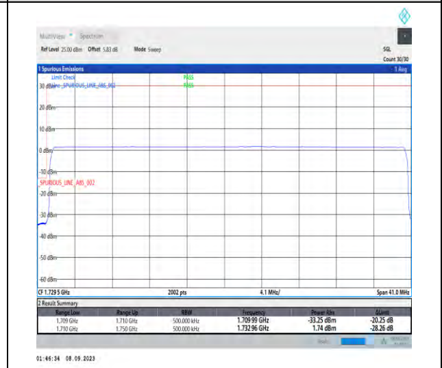
1-N66-PC3-15-40-L-6-CP-QPSK-Outer_Full-216@0-Ant2-1-seegraph-PASS-see graph
