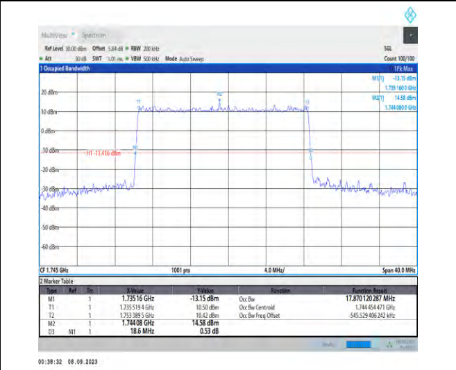
1-N66-PC3-15-20-M-1-DFT-QPSK-Outer_Full-100@0 -Ant2-17.87-18.600-≤20-PASS
