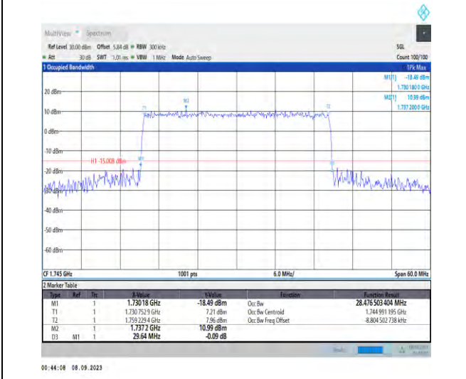
1-N66-PC3-15-30-M-6-CP-QPSK-Outer_Full-160@0 -Ant2-28.477-29.640-≤30-PASS
