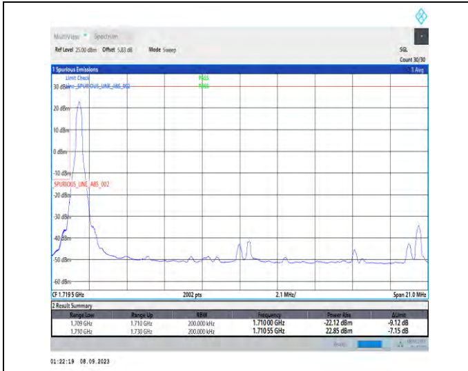
1-N66-PC3-15-20-L-1-DFT-PI2BPSK-Edge_1RB_Left-1@0-Ant2-1-seegraph-PASS-see graph
