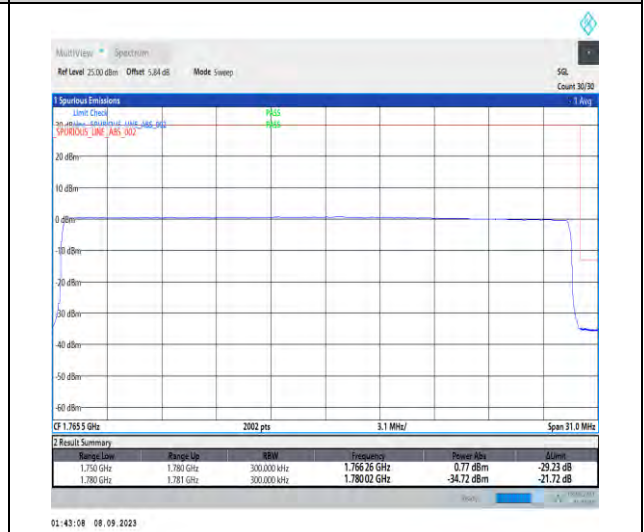
1-N66-PC3-15-30-H-6-CP-QPSK-Outer_Full-160@0-Ant2-1-seegraph-PASS-see graph
