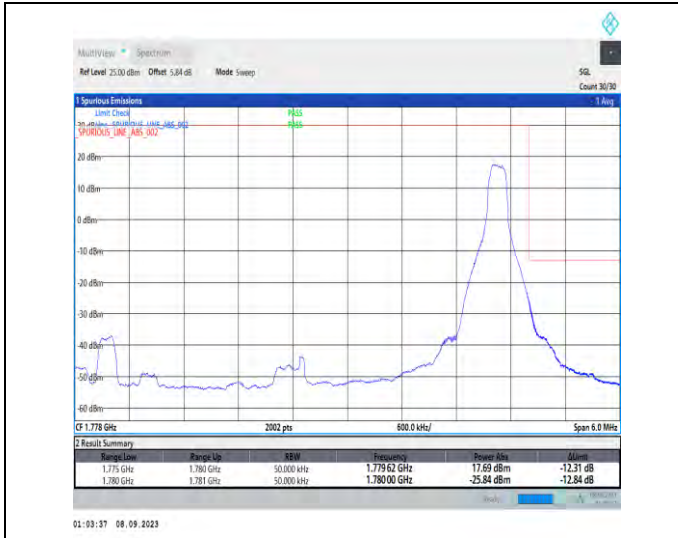
1-N66-PC3-15-5-H-2-DFT-PI2BPSK-Edge_1RB_Right-1@24-Ant2-1-seegraph-PASS-see graph
