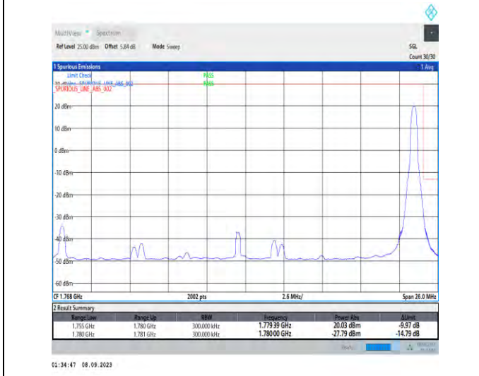
1-N66-PC3-15-25-H-5-CP-QPSK-Edge_1RB_Right-1@132-Ant2-1-seegraph-PASS-see graph
