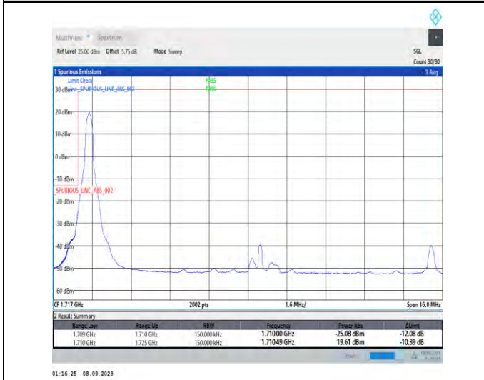
1-N66-PC3-15-15-L-4-CP-QPSK-Edge_1RB_Left-1@0-Ant2-1-seegraph-PASS-see graph
