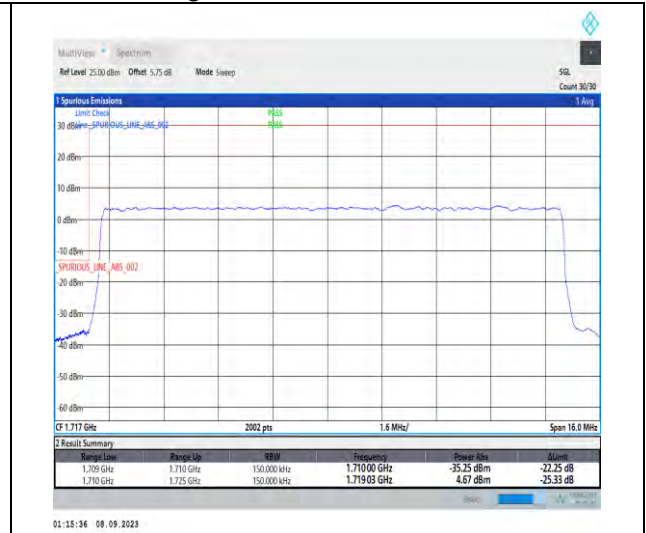
1-N66-PC3-15-15-L-3-DFT-PI2BPSK-Outer_Full-75@0-Ant2-1-seegraph-PASS-see graph
