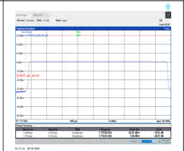
1-N66-PC3-15-15-L-6-CP-QPSK-Outer_Full-79@0-Ant2-1-seegraph-PASS-see graph
