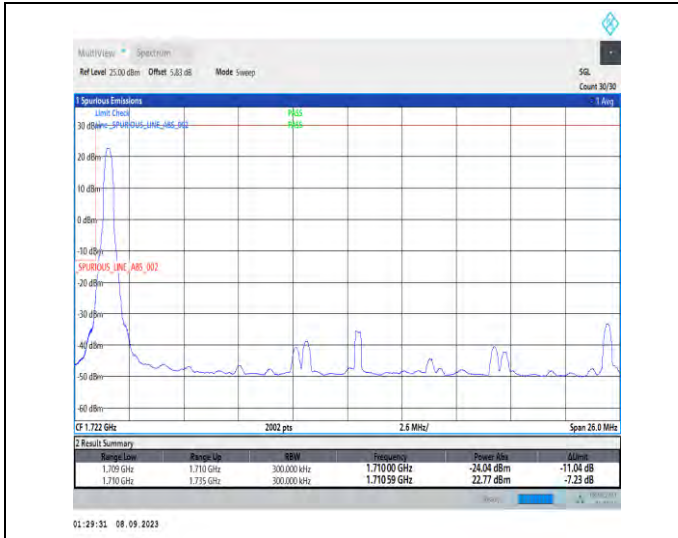
1-N66-PC3-15-25-L-1-DFT-PI2BPSK-Edge_1RB_Left-1@0-Ant2-1-seegraph-PASS-see graph
