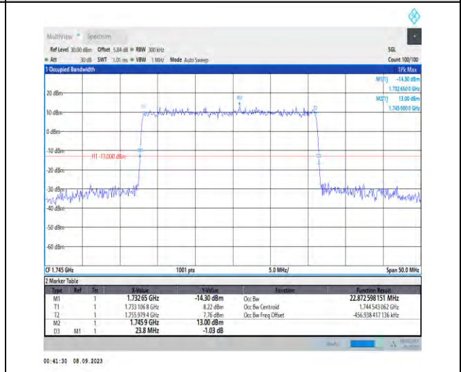
1-N66-PC3-15-25-M-4-DFT-64QAM-Outer_Full-128 @0-Ant2-22.873-23.800-≤25-PASS
