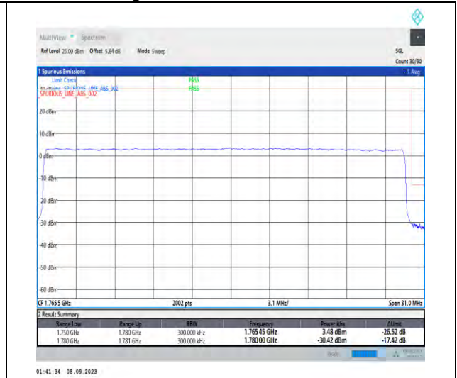
1-N66-PC3-15-30-H-3-DFT-PI2BPSK-Outer_Full-160@0-Ant2-1-seegraph-PASS-see graph
