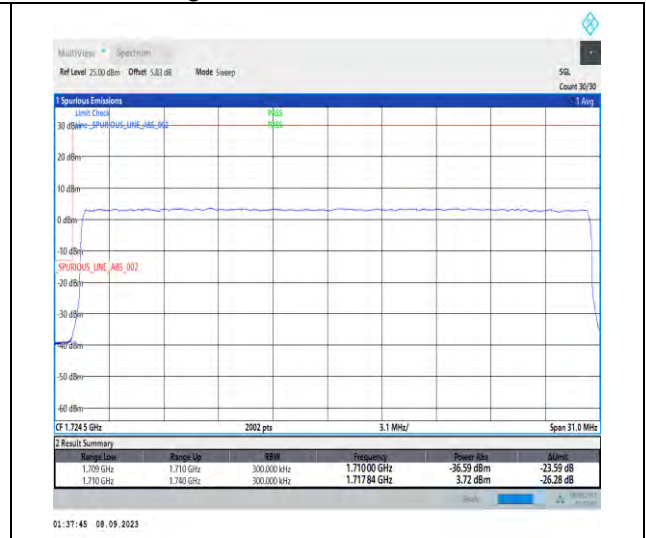
1-N66-PC3-15-30-L-3-DFT-PI2BPSK-Outer_Full-160@0-Ant2-1-seegrph-PASS-see graph
