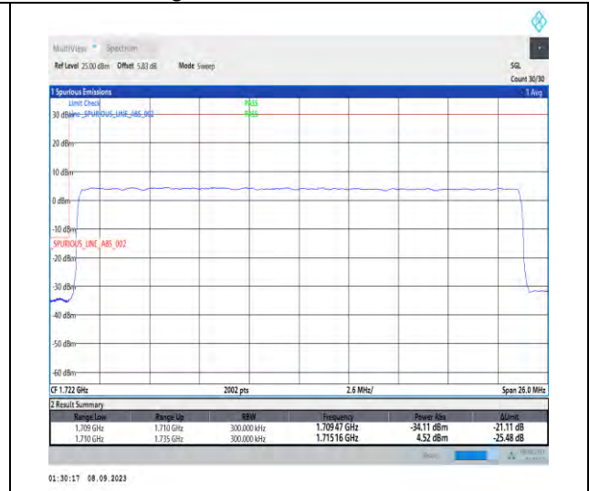
1-N66-PC3-15-25-L-3-DFT-PI2BPSK-Outer_Full-1 28@0-Ant2-1-seegraph-PASS-see graph
