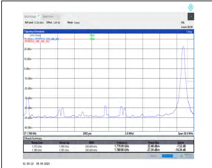
1-N66-PC3-15-25-H-2-DFT-PI2BPSK-Edge_1RB_Right-t-1@132-Ant2-1-seegraph-PASS-see graph
