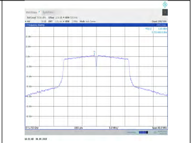
11n40MIMO-Ant9-5755-PASS
