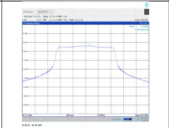
11n20MIMO-Ant9-5700-PASS
