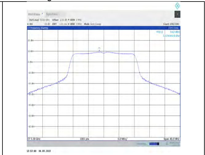
11a-Ant7-5580-PASS
