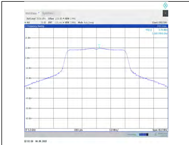
11a-Ant7-5500-PASS
