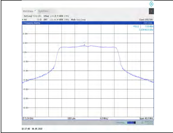
11n20MIMO-Ant7-5240-PASS
