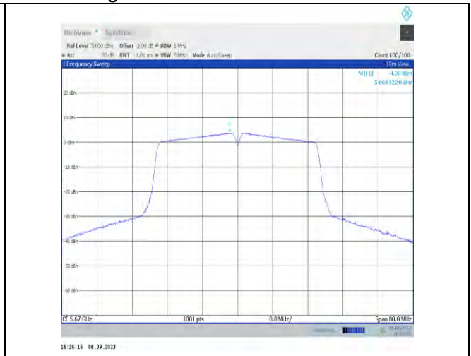
11n40MIMO-Ant9-5670-PASS
