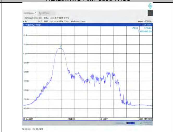
11ax20MIMO-Ant9-5500-PASS
