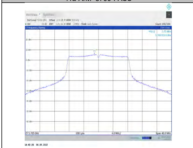
11a-Ant7-5785-PASS
