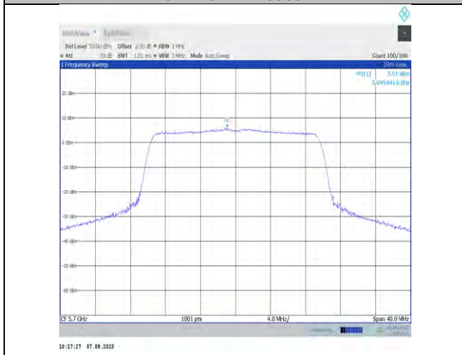
11x20MIMO-Ant7-5700-PASS
