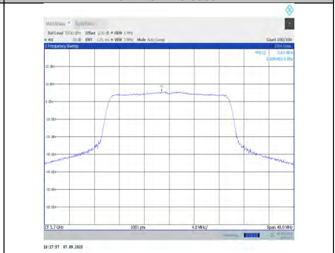
11x20MIMO-Ant9-5700-PASS
