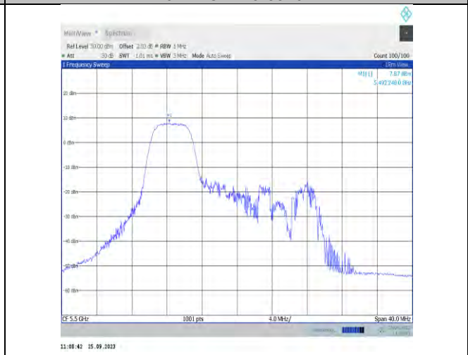
11ax20MIMO-Ant7-5500-PASS
