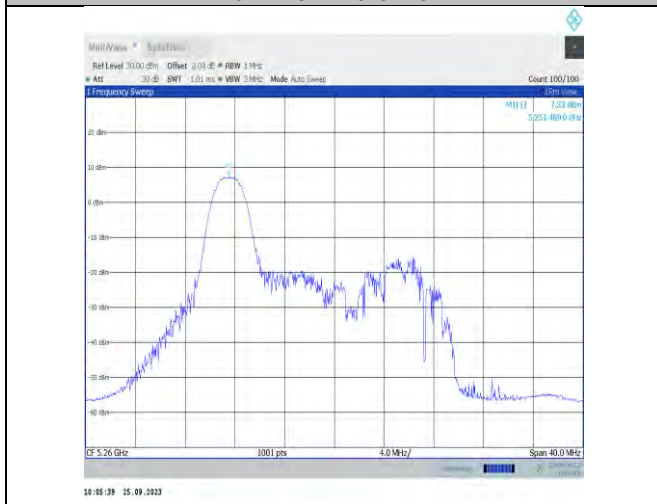
11ax20MIMO-Ant7-5260-PASS
