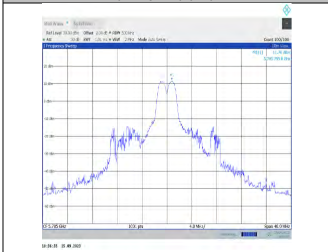
11x20MIMO-Ant7-5785-PASS
