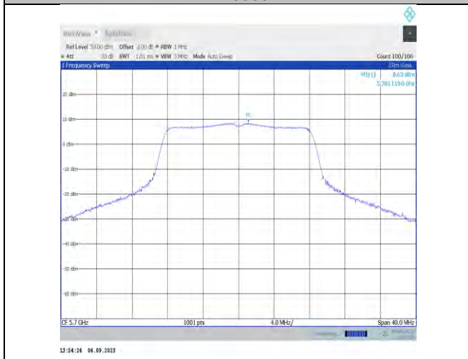
11a-Ant7-5700-PASS
