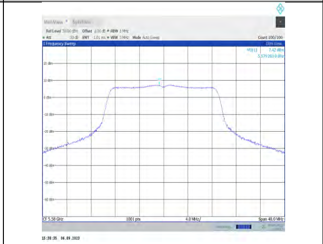
11n20MIMO-Ant9-5580-PASS
