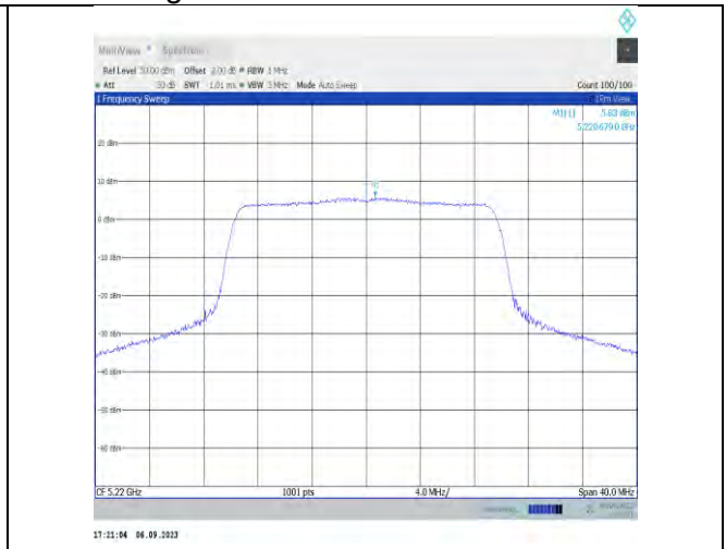
11ax20MIMO-Ant9-5220-PASS
