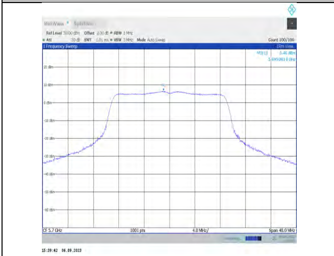
11n20MIMO-Ant7-5700-PASS
