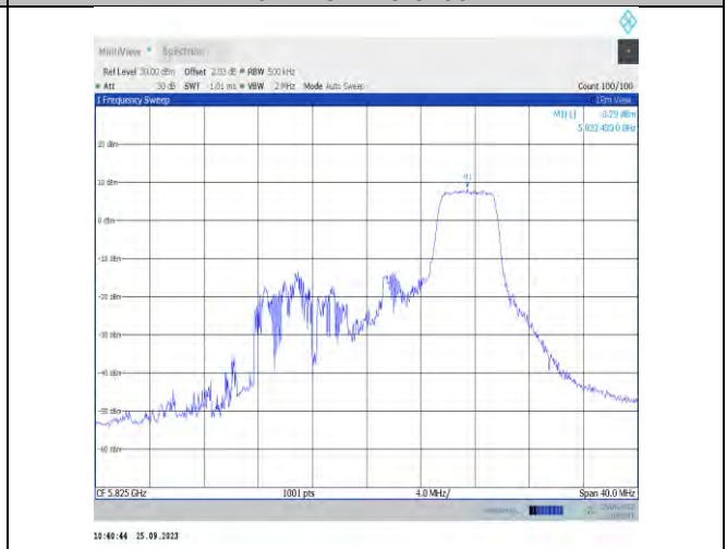
11x20MIMO-Ant7-5825-PASS
