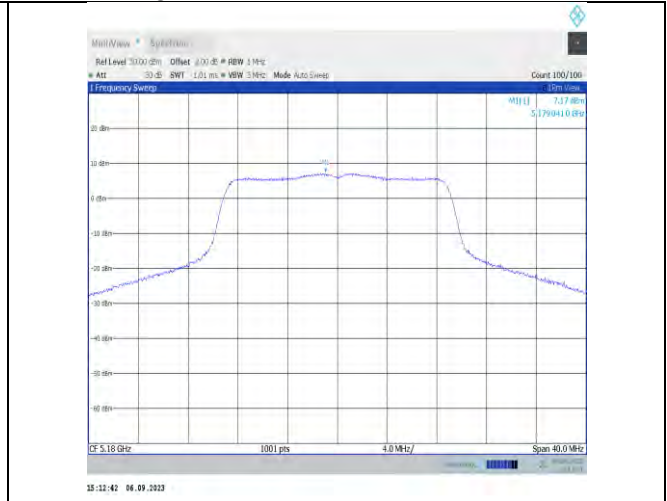
11n20MIMO-Ant9-5180-PASS
