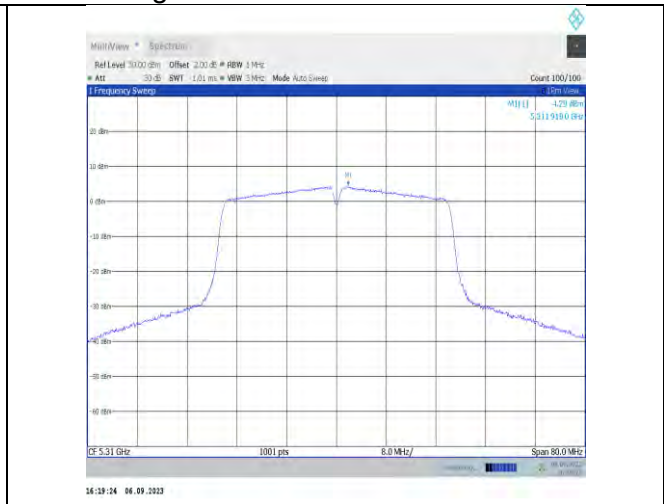
11n40MIMO-Ant9-5310-PASS
