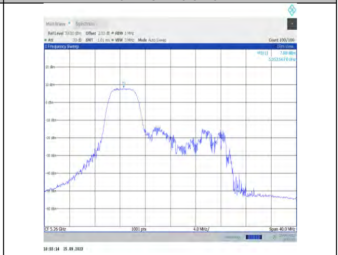
11ax20MIMO-Ant7-5260-PASS
