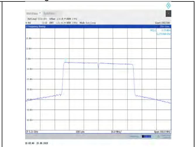
11ac80MIMO-Ant9-5210-PASS
