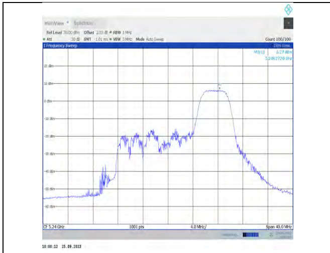
11ax20MIMO-Ant9-5240-PASS
