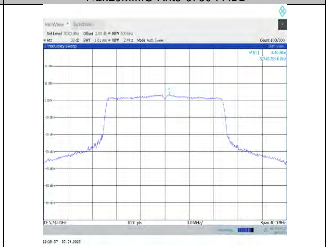
11x20MIMO-Ant9-5745-PASS
