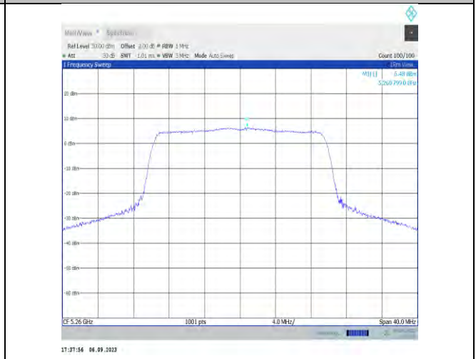
11ax20MIMO-Ant9-5260-PASS
