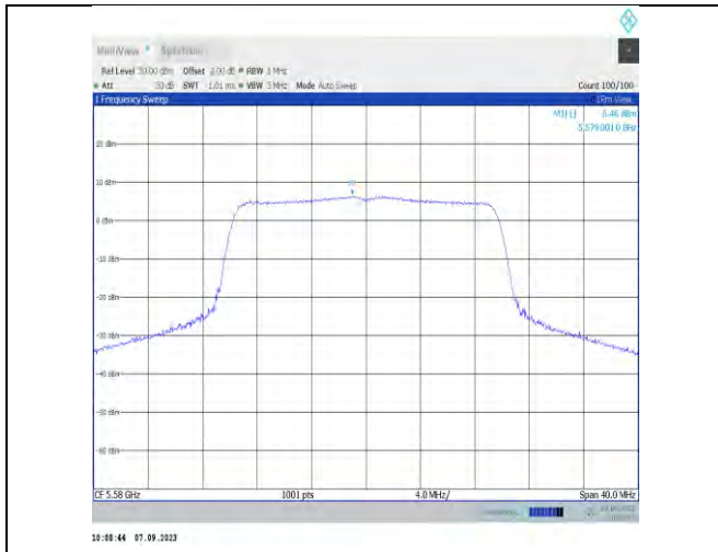
11x20MIMO-Ant7-5580-PASS
