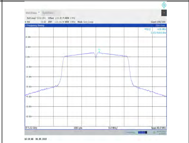
11n40MIMO-Ant9-5510-PASS
