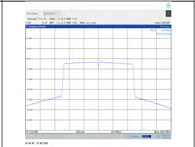
11ac80MIMO-Ant9-5530-PASS
