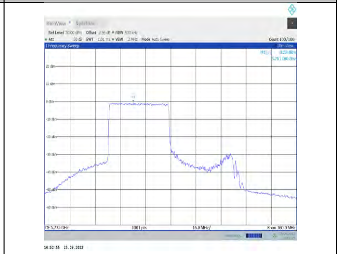
11ax80MIMO-Ant9-5775-PASS
