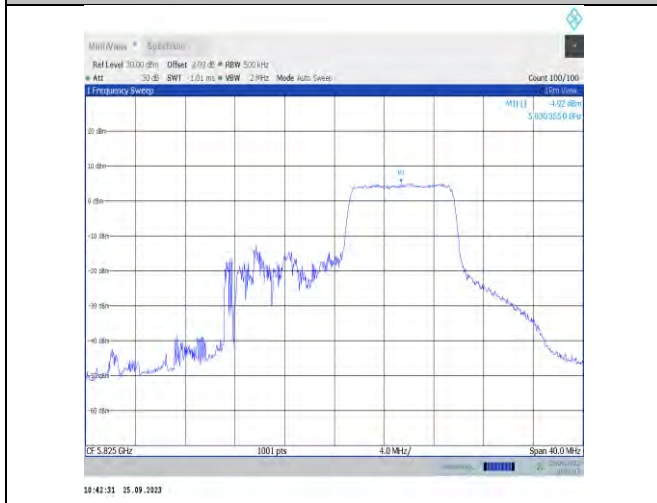
11x20MIMO-Ant7-5825-PASS
