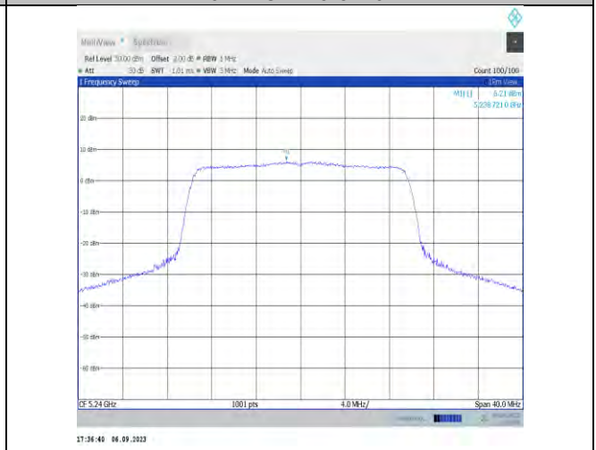
11ax20MIMO-Ant9-5240-PASS
