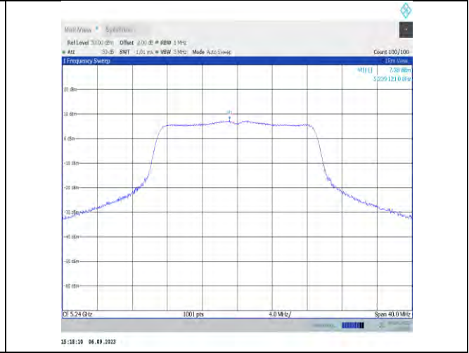
11n20MIMO-Ant9-5240-PASS
