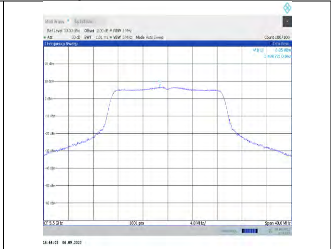
11n20MIMO-Ant9-5500-PASS
