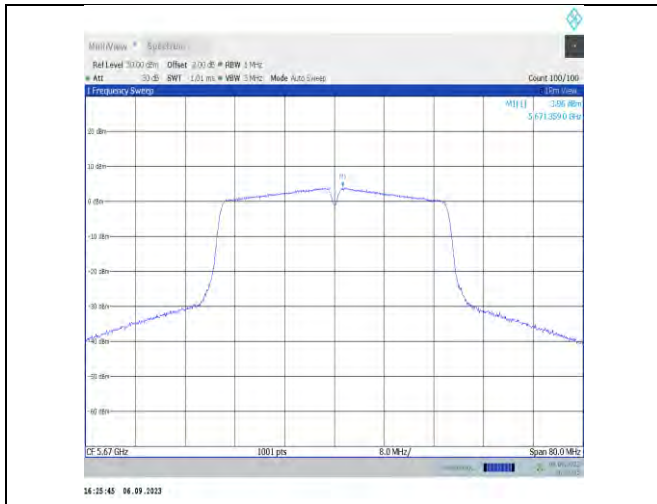
11n40MIMO-Ant7-5670-PASS
