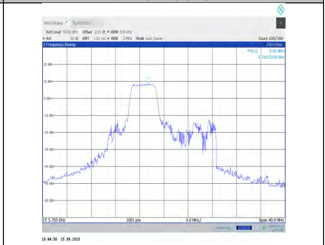
11x20MIMO-Ant7-5785-PASS
