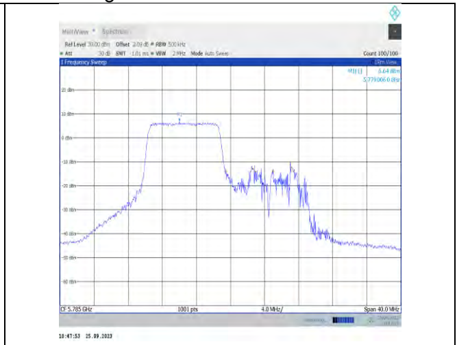
11x20MIMO-Ant9-5785-PASS
