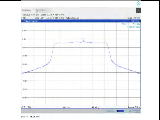
11n20MIMO-Ant9-5220-PASS
