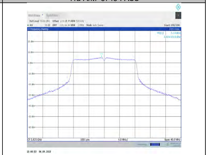
11a-Ant7-5825-PASS
