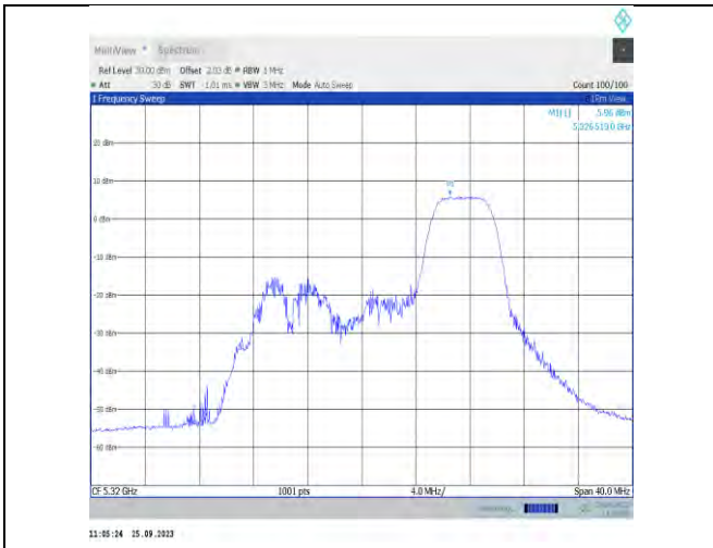
11ax20MIMO-Ant9-5320-PASS
