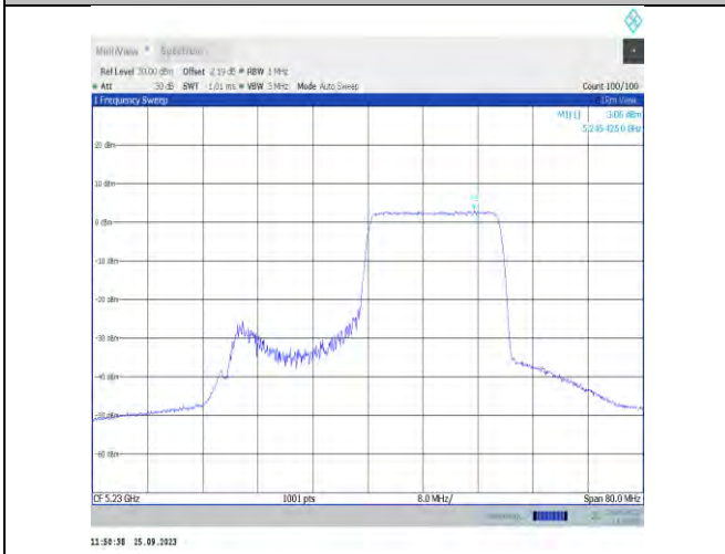
11ax40MIMO-Ant7-5230-PASS
