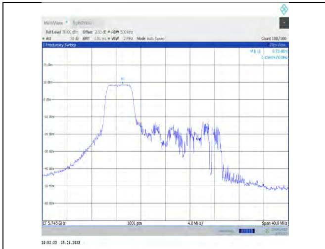
11x20MIMO-Ant9-5745-PASS
