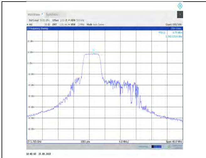
11x20MIMO-Ant9-5785-PASS
