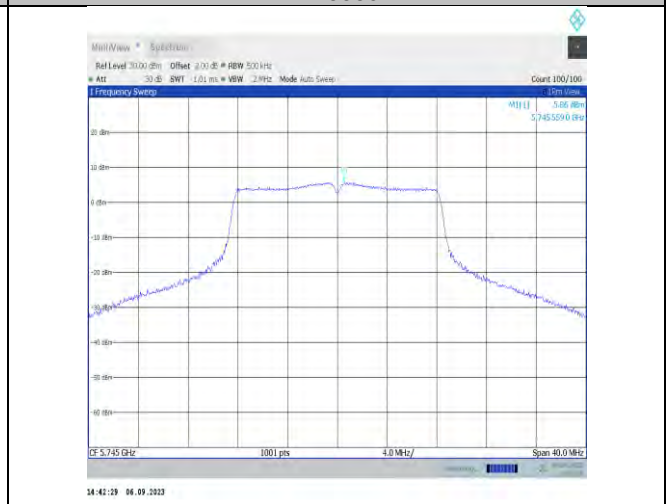
11a-Ant7-5745-PASS
