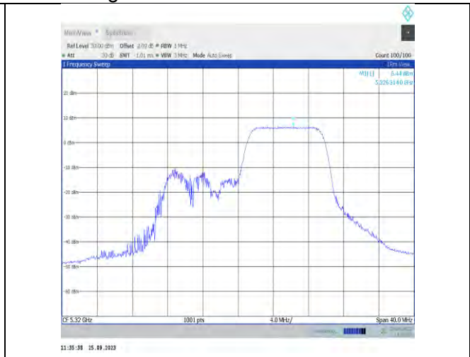
11ax20MIMO-Ant9-5320-PASS
