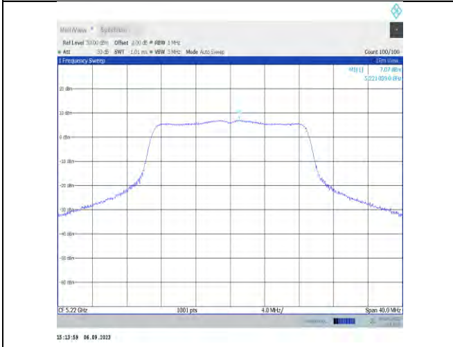
11n20MIMO-Ant7-5220-PASS
