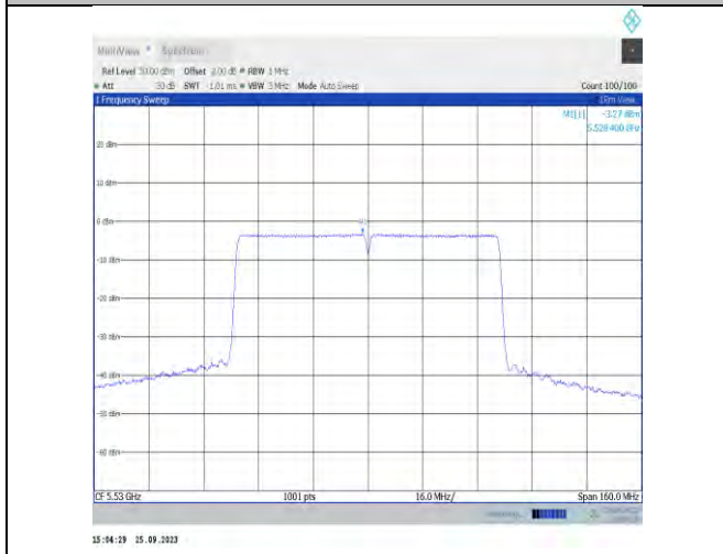
11ac80MIMO-Ant7-5530-PASS
