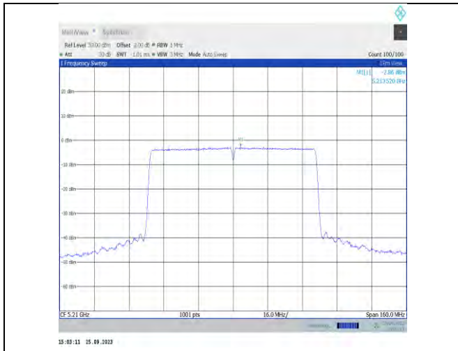
11ac80MIMO-Ant7-5210-PASS
