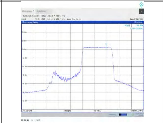
11ax40MIMO-Ant9-5230-PASS
