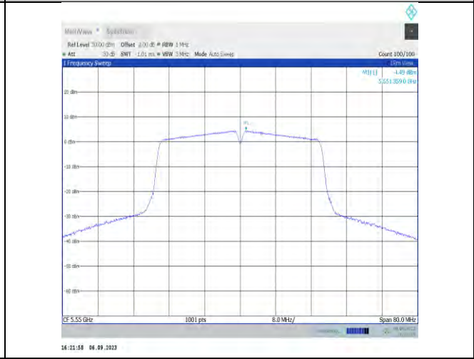
11n40MIMO-Ant9-5550-PASS
