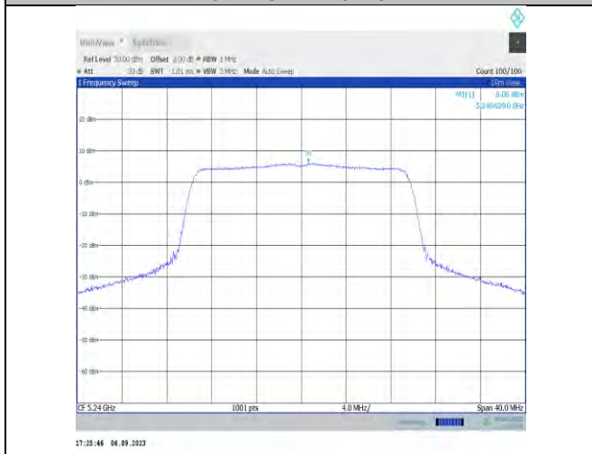
11ax20MIMO-Ant7-5240-PASS
