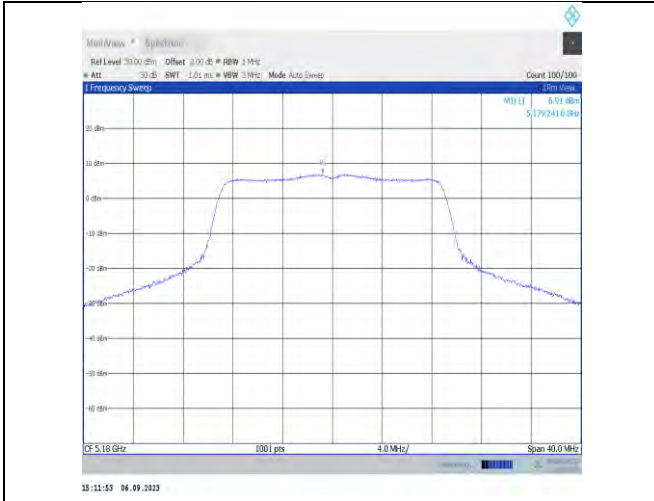
11n20MIMO-Ant7-5180-PASS
