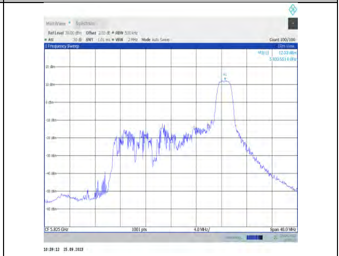
11x20MIMO-Ant9-5825-PASS
