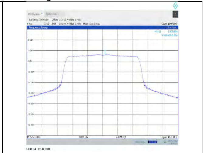
11x20MIMO-Ant9-5580-PASS
