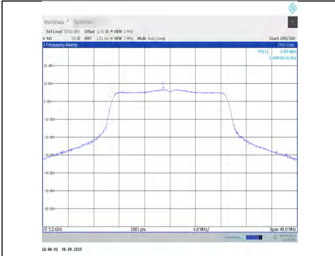
11n20MIMO-Ant7-5500-PASS
