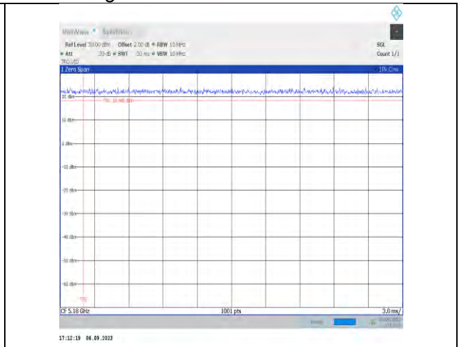
NTNV-11ax20MIMO-Ant9-5180
