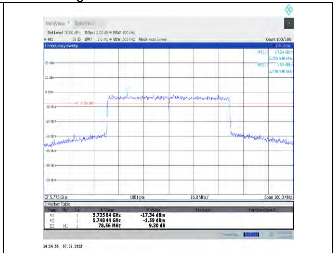
11x80MIMO-Ant7-5775-PASS
