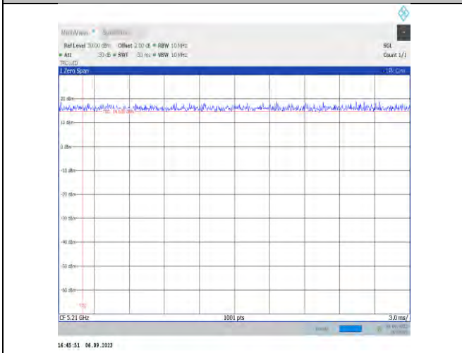
NTNV-11ac80MIMO-Ant7-5210
