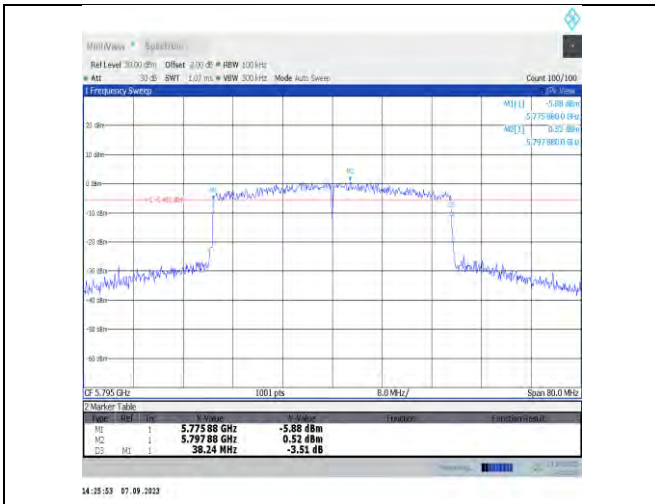
11x40MIMO-Ant9-5795-PASS
