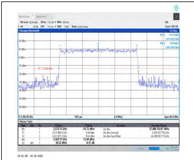
1-N41-PC2-30-40-M-9-CP-256QAM-Outer_Full-106 @0-Ant3-37.887-39.520-≤40-PASS
