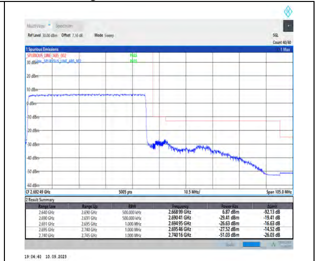
1-N41-PC2-30-50-H-3-DFT-PI2BPSK-Outer_Full-1 28@0-Ant3-1--PASS-see graph
