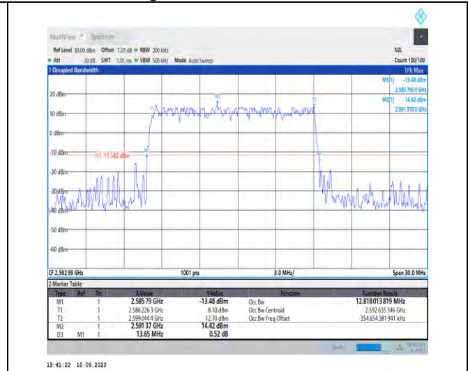
1-N41-PC2-30-15-M-5-DFT-256QAM-Outer_Full-36@ 0-Ant3-12.818-13.650-≤15-PASS
