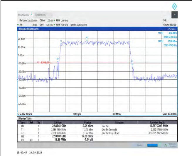
1-N41-PC2-30-15-M-2-DFT-PI2BPSK-Outer_Full-36@ 0-Ant3-12.787-13.890-≤15-PASS
