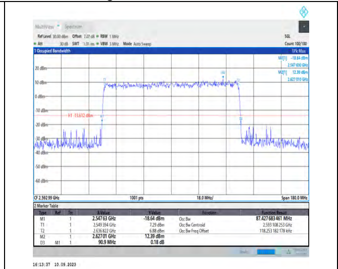
1-N41-PC2-30-90-M-9-CP-256QAM-Outer_Full-245 @0-Ant3-87.428-90.900-≤90-PASS
