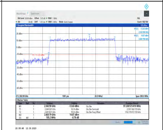
1-N41-PC2-30-100-M-6-CP-QPSK-Outer_Full-273 @0-Ant3-97.331-105.200-≤100-PASS
