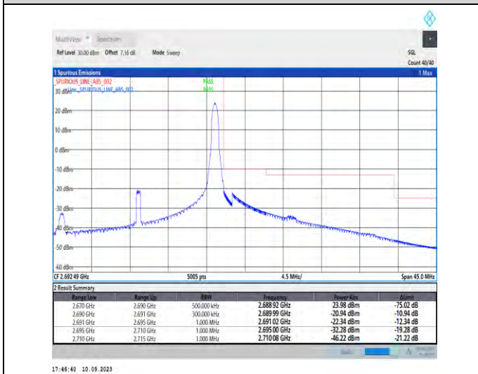
1-N41-PC2-30-20-H-5-CP-QPSK-Edge_1RB_Right-1 @50-Ant3-1--PASS-see graph
