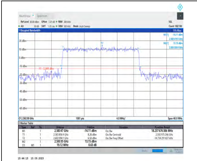
1-N41-PC2-30-20-M-7-CP-16QAM-Outer_Full-51@0 -Ant3-18.238-19.120-≤20-PASS
