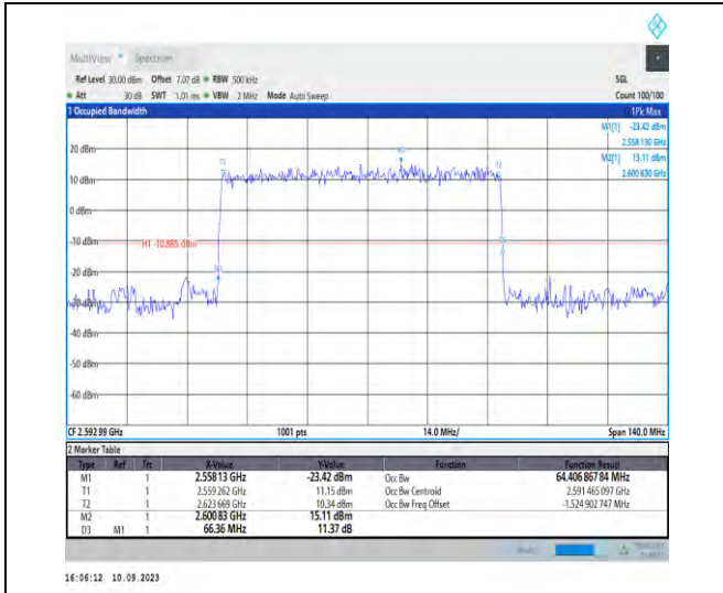
1-N41-PC2-30-70-M-2-DFT-PI2BPSK-Outer_Full-180 @0-Ant3-64.407-66.360-≤70-PASS
