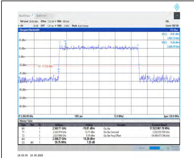
1-N41-PC2-30-60-M-3-DFT-16QAM-Outer_Full-162 @0-Ant3-57.924-59.760-≤60-PASS
