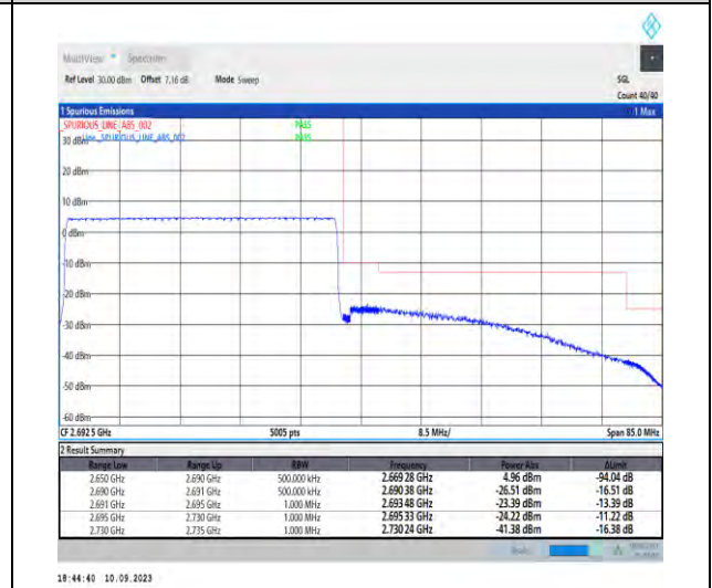
1-N41-PC2-30-40-H-6-CP-QPSK-Outer_Full-106 @0-Ant3-1--PASS-see graph
