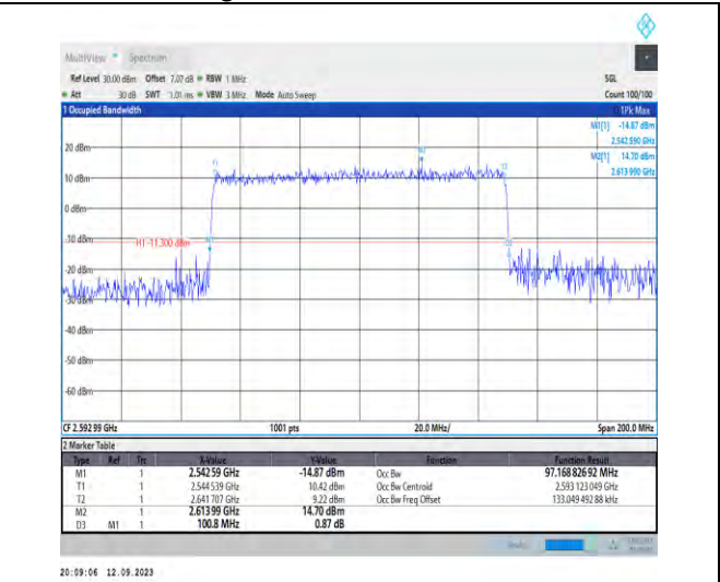
1-N41-PC2-30-100-M-8-CP-64QAM-Outer_Full-273 @0-Ant3-97.169-100.800-≤100-PASS
