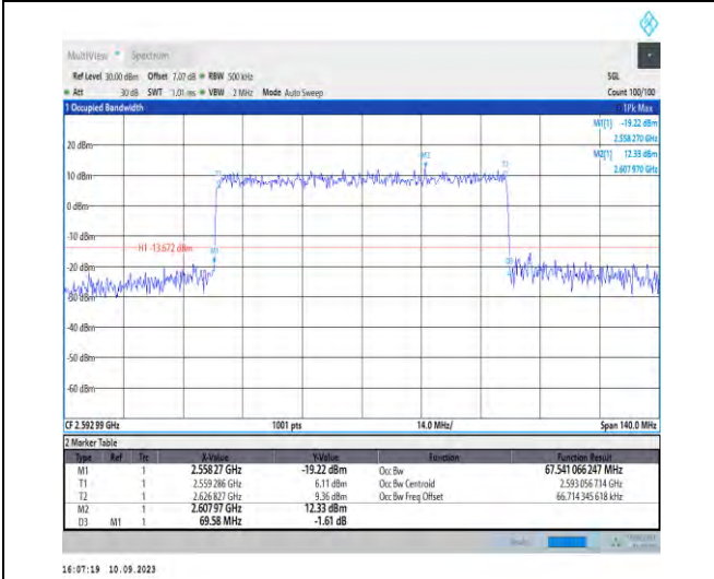
1-N41-PC2-30-70-M-8-CP-64QAM-Outer_Full-189@0 -Ant3-67.541-69.580-≤70-PASS
