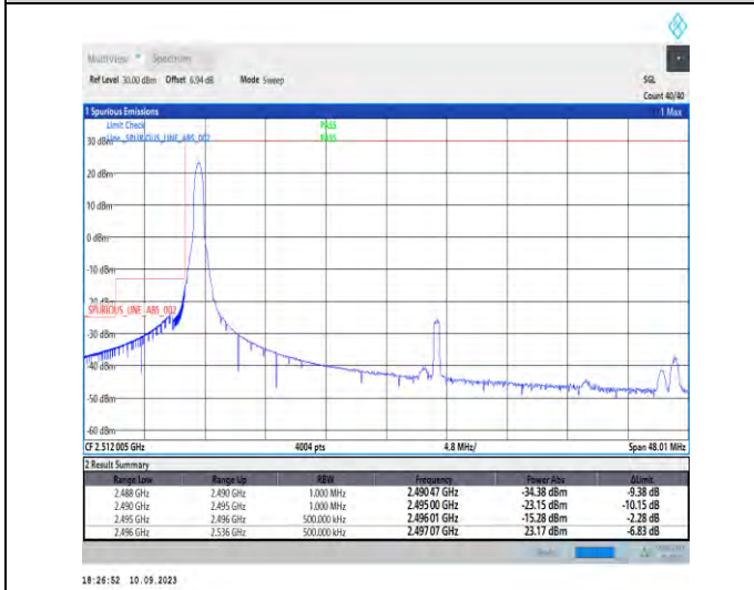
1-N41-PC2-30-40-L-4-CP-QPSK-Edge_1RB_Left-1@0-Ant3-1--PASS-see graph
