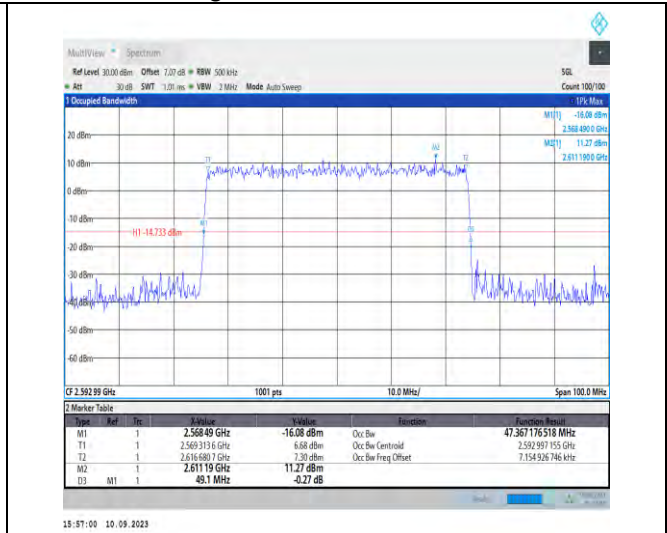
1-N41-PC2-30-50-M-9-CP-256QAM-Outer_Full-133 @0-Ant3-47.367-49.100-≤50-PASS
