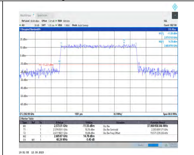
1-N41-PC2-30-40-M-6-CP-QPSK-Outer_Full-106@0 -Ant3-37.901-40.240-≤40-PASS
