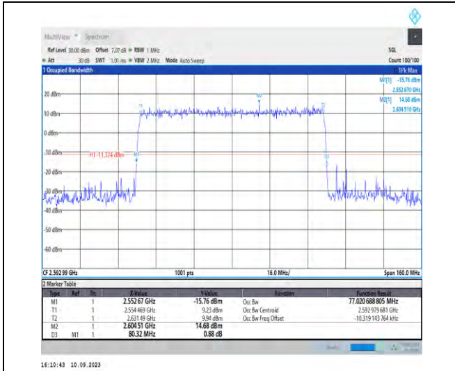
1-N41-PC2-30-80-M-5-DFT-256QAM-Outer_Full-216 @0-Ant3-77.021-80.320-≤80-PASS
