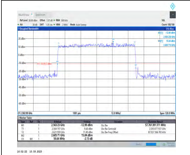
1-N41-PC2-30-60-M-1-DFT-QPSK-Outer_Full-162@ 0-Ant3-57.761-59.640-≤60-PASS
