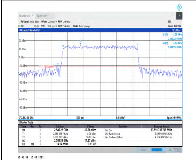
1-N41-PC2-30-15-M-6-CP-QPSK-Outer_Full-38@0- Ant3-13.592-14.940-≤15-PASS
