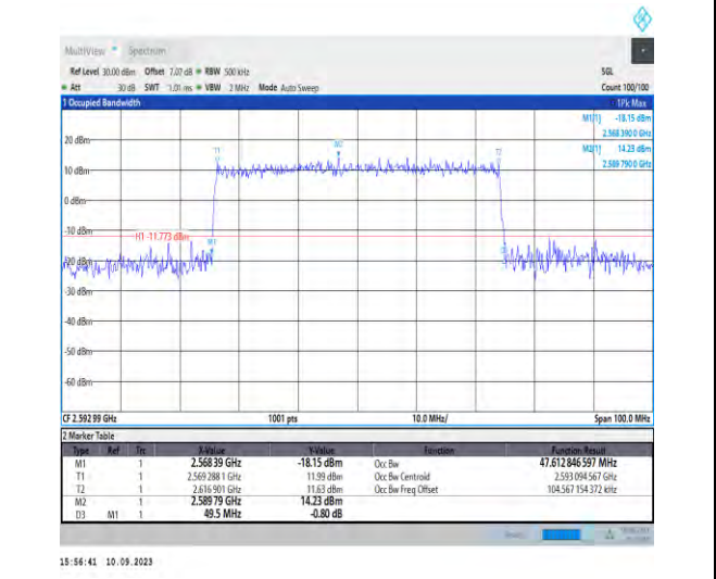
1-N41-PC2-30-50-M-7-CP-16QAM-Outer_Full-133@0-Ant3-47.613-49.500-≤50-PASS
