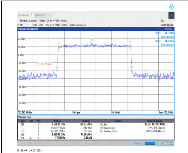
1-N41-PC2-30-50-M-4-DFT-64QAM-Outer_Full-128 @0-Ant3-45.677-47.600-≤50-PASS
