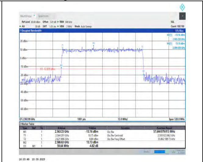
1-N41-PC2-30-60-M-8-CP-64QAM-Outer_Full-162@ 0-Ant3-57.645-59.640-≤60-PASS
