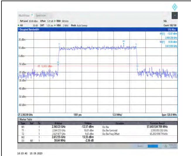
1-N41-PC2-30-60-M-7-CP-16QAM-Outer_Full-162@ 0-Ant3-57.644-59.640-≤60-PASS
