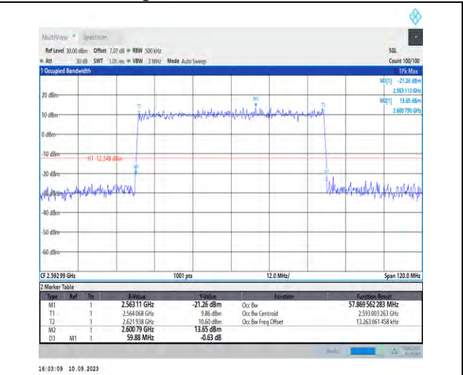
1-N41-PC2-30-60-M-4-DFT-64QAM-Outer_Full-162 @0-Ant3-57.87-59.880-≤60-PASS
