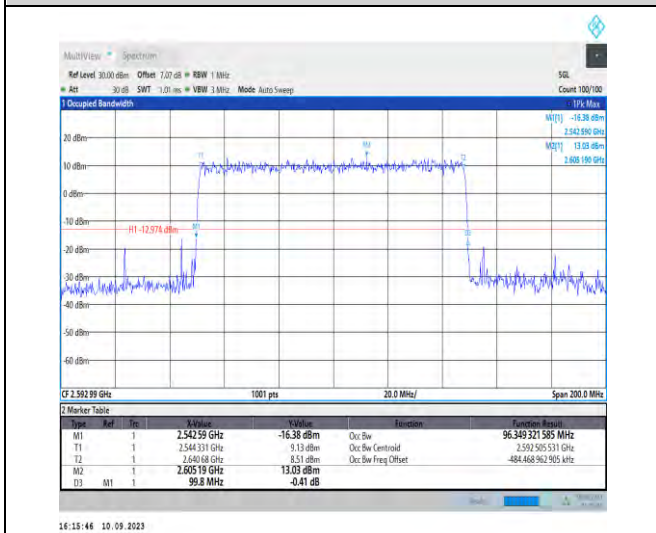
1-N41-PC2-30-100-M-5-DFT-256QAM-Outer_Full-270 @0-Ant3-96.349-99.800-≤100-PASS
