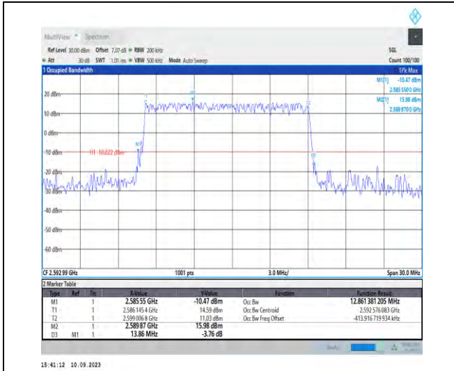
1-N41-PC2-30-15-M-4-DFT-64QAM-Outer_Full-36@ 0-Ant3-12.861-13.860-≤15-PASS
