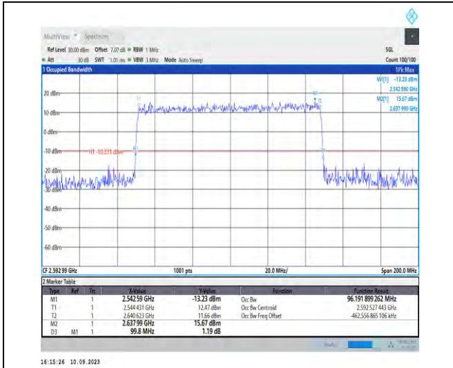
1-N41-PC2-30-100-M-3-DFT-16QAM-Outer_Full-270 @0-Ant3-96.192-99.800-≤100-PASS
