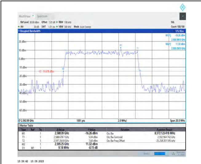
1-N41-PC2-30-10-M-9-CP-256QAM-Outer_Full-24@ 0-Ant3-8.572-9.180-≤10-PASS
