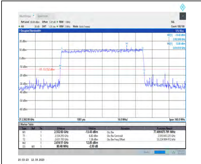
1-N41-PC2-30-80-M-9-CP-256QAM-Outer_Full-217 @0-Ant3-77.5-80.480-≤80-PASS
