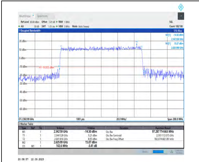
1-N41-PC2-30-100-M-7-CP-16QAM-Outer_Full-273 @0-Ant3-97.288-102.600-≤100-PASS
