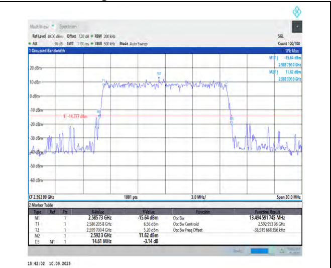
1-N41-PC2-30-15-M-9-CP-256QAM-Outer_Full-38@0 -Ant3-13.495-14.610-≤15-PASS
