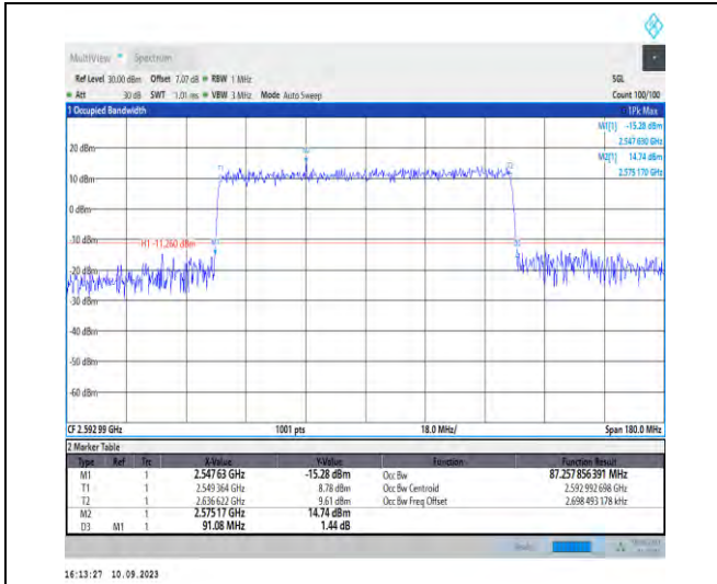
1-N41-PC2-30-90-M-8-CP-64QAM-Outer_Full-245@ 0-Ant3-87.258-91.080-≤90-PASS
