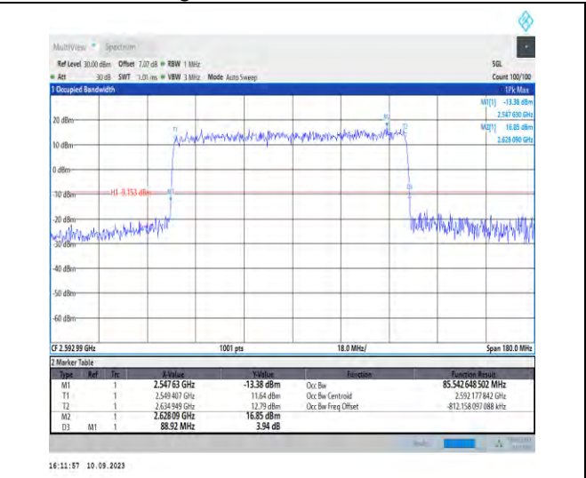
1-N41-PC2-30-90-M-1-DFT-QPSK-Outer_Full-240 @0-Ant3-85.543-88.920-≤90-PASS
