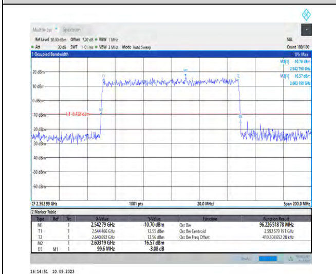
1-N41-PC2-30-100-M-1-DFT-QPSK-Outer_Full-270 @0-Ant3-96.227-99.600-≤100-PASS
