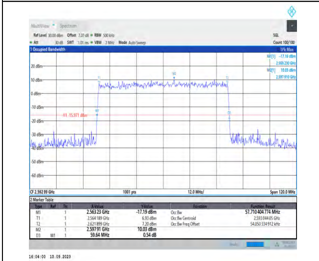
1-N41-PC2-30-60-M-9-CP-256QAM-Outer_Full-162 @0-Ant3-57.71-59.640-≤60-PASS
