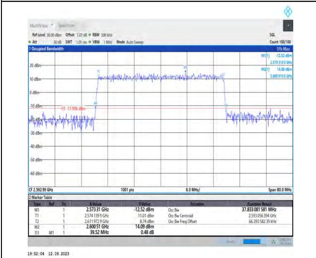
1-N41-PC2-30-40-M-7-CP-16QAM-Outer_Full-106@ 0-Ant3-37.833-39.520-≤40-PASS
