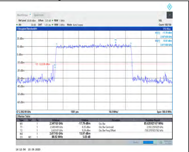
1-N41-PC2-30-90-M-5-DFT-256QAM-Outer_Full-240 @0-Ant3-85.621-88.920-≤90-PASS
