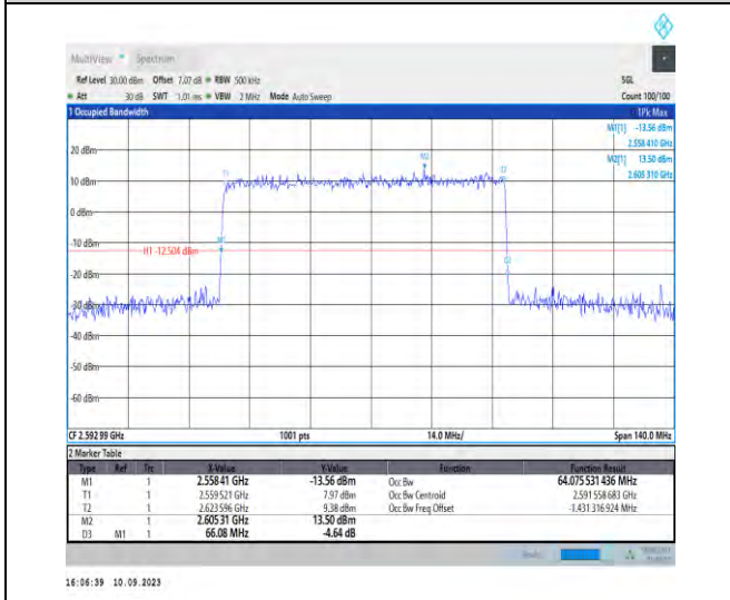
1-N41-PC2-30-70-M-4-DFT-64QAM-Outer_Full-180 @0-Ant3-64.076-66.080-≤70-PASS
