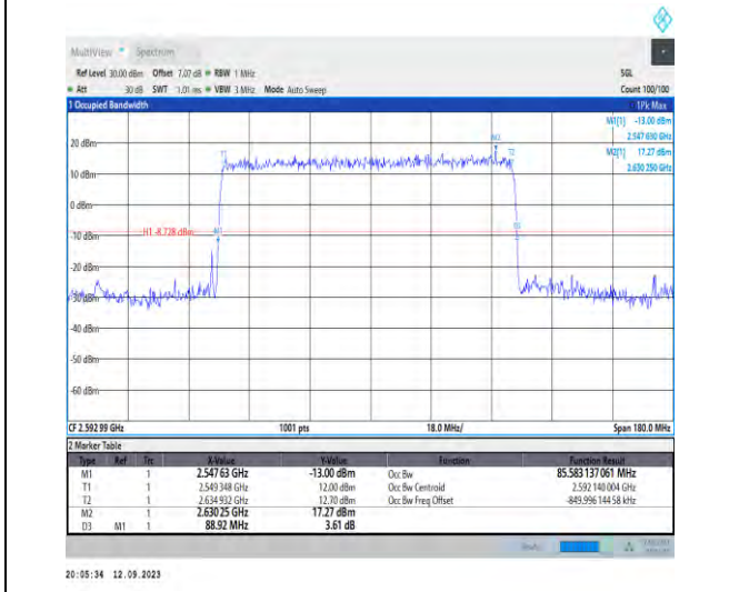
1-N41-PC2-30-90-M-2-DFT-PI2BPSK-Outer_Full-240 @0-Ant3-85.583-88.920-≤90-PASS
