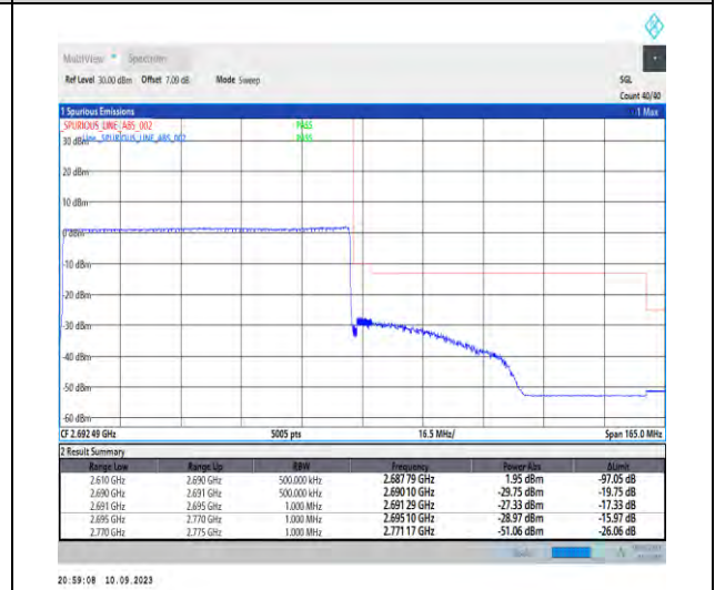
1-N41-PC2-30-80-H-6-CP-QPSK-Outer_Full-217 @0-Ant3-1--PASS-see graph
