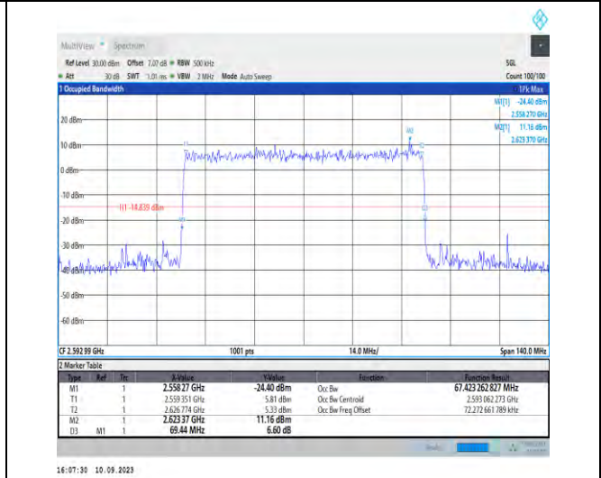
1-N41-PC2-30-70-M-9-CP-256QAM-Outer_Full-189@0 -Ant3-67.423-69.440-≤70-PASS
