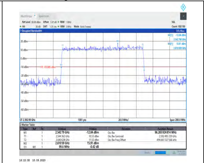
1-N41-PC2-30-100-M-4-DFT-64QAM-Outer_Full-270 @0-Ant3-96.266-99.600-≤100-PASS
