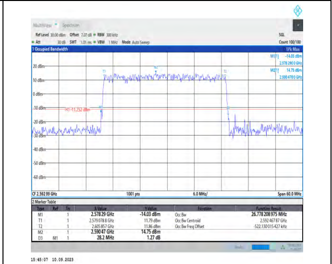
1-N41-PC2-30-30-M-1-DFT-QPSK-Outer_Full-75@0 -Ant3-26.778-28.200-≤30-PASS
