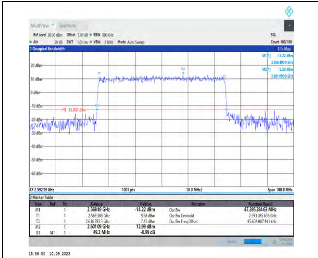
1-N41-PC2-30-50-M-8-CP-64QAM-Outer_Full-133@ 0-Ant3-47.395-49.200-≤50-PASS
