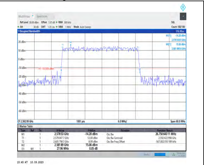
1-N41-PC2-30-30-M-3-DFT-16QAM-Outer_Full-75 @0-Ant3-26.751-27.960-≤30-PASS
