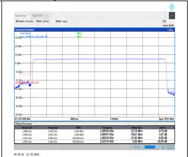
1-N41-PC2-30-70-L-3-DFT-PI2BPSK-Outer_Full-180@0-Ant3-1--PASS-see graph
