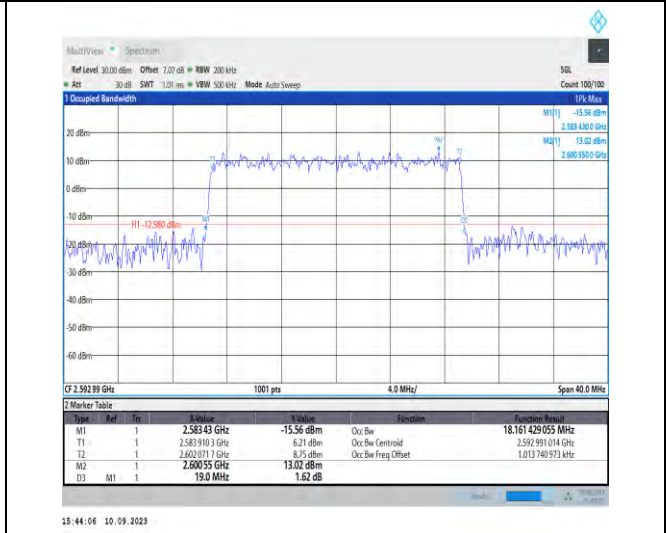
1-N41-PC2-30-20-M-6-CP-QPSK-Outer_Full-51@0- Ant3-18.161-19.000-≤20-PASS
