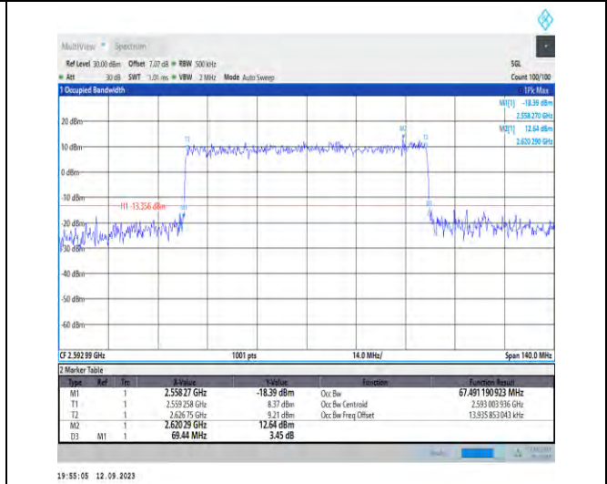
1-N41-PC2-30-70-M-7-CP-16QAM-Outer_Full-189@0 -Ant3-67.491-69.440-≤70-PASS
