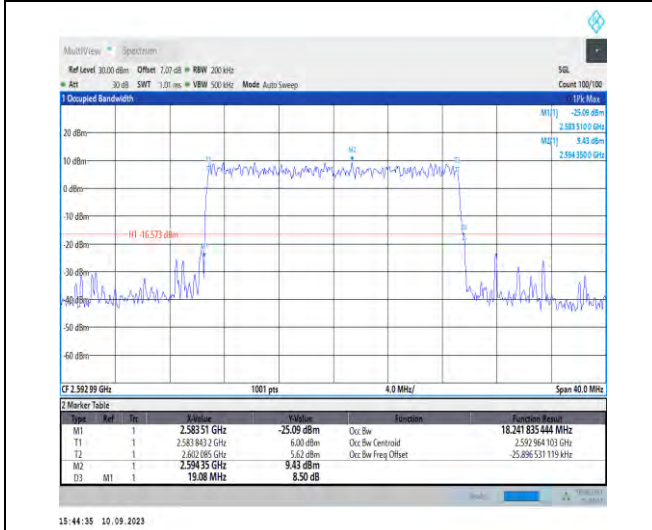
1-N41-PC2-30-20-M-9-CP-256QAM-Outer_Full-51@0 0-Ant3-18.242-19.080-≤20-PASS
