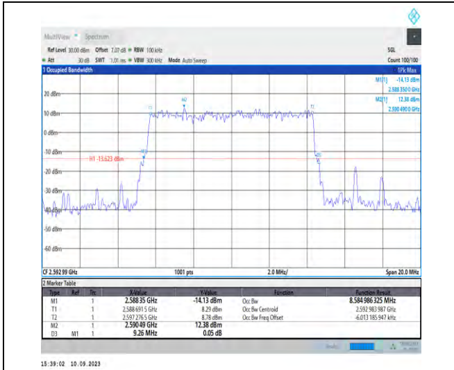
1-N41-PC2-30-10-M-5-DFT-256QAM-Outer_Full-24@0-Ant3-8.585-9.260-≤10-PASS
