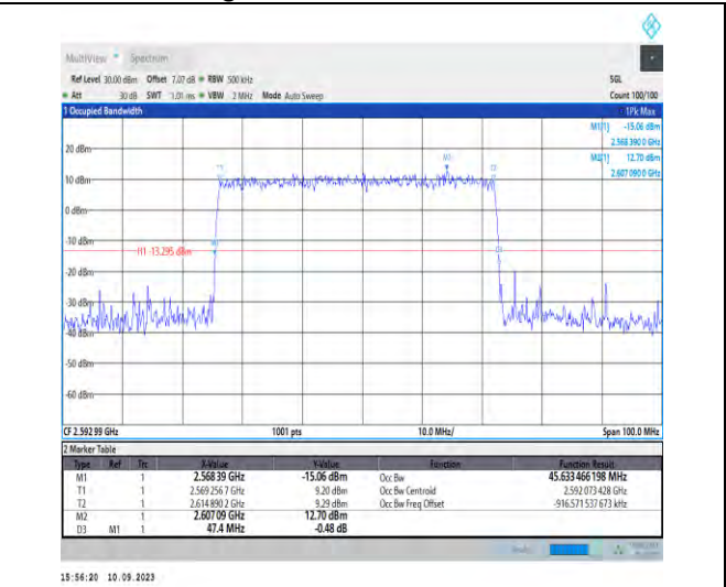
1-N41-PC2-30-50-M-5-DFT-256QAM-Outer_Full-128 @0-Ant3-45.633-47.400-≤50-PASS
