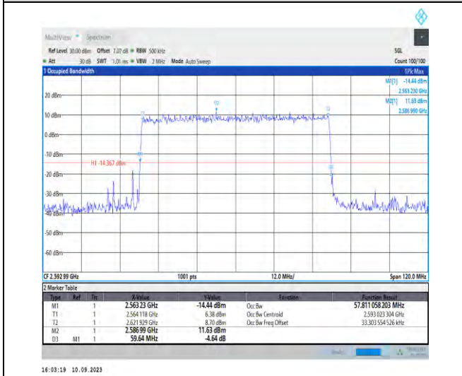
1-N41-PC2-30-60-M-5-DFT-256QAM-Outer_Full-162 @0-Ant3-57.811-59.640-≤60-PASS
