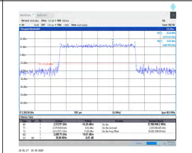
1-N41-PC2-30-40-M-8-CP-64QAM-Outer_Full-106@ 0-Ant3-37.982-39.840-≤40-PASS
