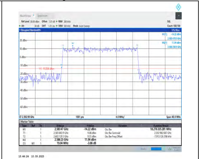
1-N41-PC2-30-20-M-8-CP-64QAM-Outer_Full-51@0 -Ant3-18.276-19.040-≤20-PASS
