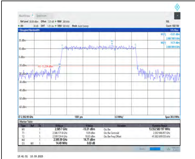
1-N41-PC2-30-15-M-8-CP-64QAM-Outer_Full-38@0 -Ant3-13.553-14.490-≤15-PASS
