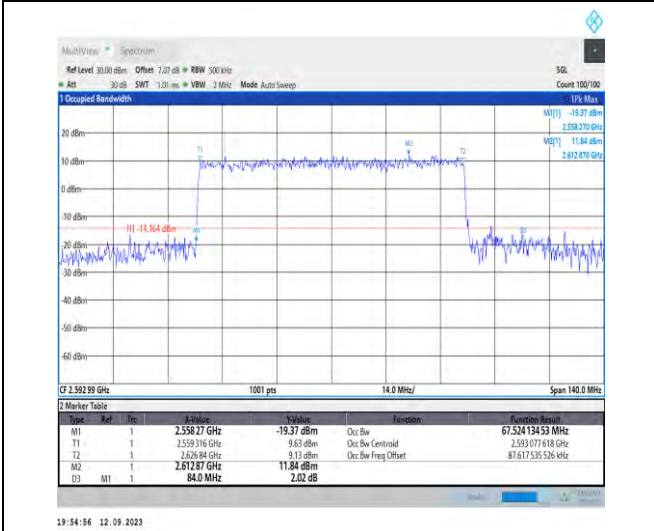
1-N41-PC2-30-70-M-6-CP-QPSK-Outer_Full-189@0 -Ant3-67.524-84.000-≤70-PASS
