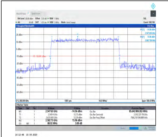
1-N41-PC2-30-90-M-4-DFT-64QAM-Outer_Full-240 @0-Ant3-85.643-88.920-≤90-PASS
