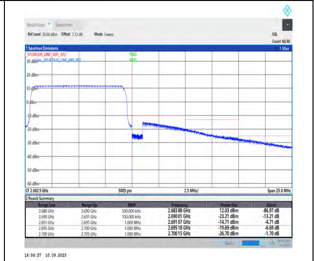
1-N41-PC2-30-10-H-6-CP-QPSK-Outer_Full-24 @0-Ant3-1--PASS-see graph
