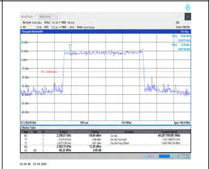
1-N41-PC2-30-70-M-5-DFT-256QAM-Outer_Full-180 @0-Ant3-64.297-66.220-≤70-PASS
