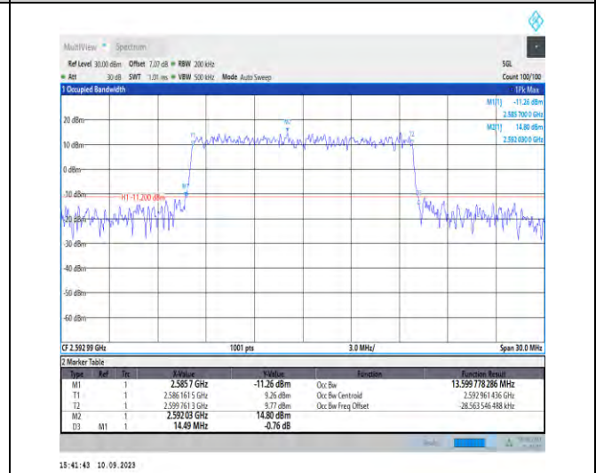
1-N41-PC2-30-15-M-7-CP-16QAM-Outer_Full-38@0- -Ant3-13.6-14.490-≤15-PASS
