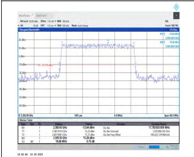
1-N41-PC2-30-20-M-1-DFT-QPSK-Outer_Full-50@0 -Ant3-17.784-18.680-≤20-PASS
