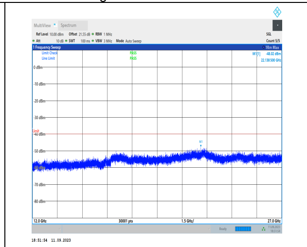
1-N30-PC3-15-10-H-1-DFT-PI2BPSK-Inner_1RB_Lef t-1@1-12000-27000-Ant3-22138.50--48.02--40-PASS
