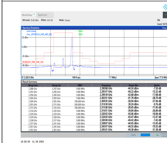
1-N30-PC3-15-10-H-5-CP-QPSK-Edge_1RB_Right-1@51-Ant3-1--PASS-see graph
