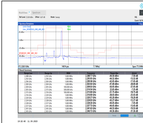
1-N30-PC3-15-10-H-2-DFT-PI2BPSK-Edge_1RB_Right-t1@51-Ant3-1--PASS-see graph
