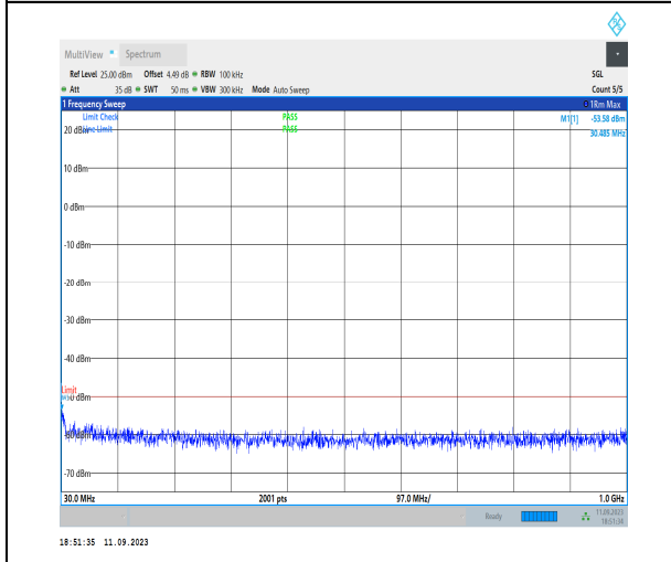
1-N30-PC3-15-10-H-1-DFT-PI2BPSK-Inner_1RB_L eft-1@1-30-1000-Ant3-30.49--53.58--50-PASS
