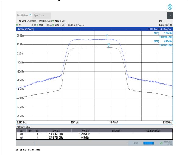
1-N30-PC3-15-10-H-2-CP-256QAM-Outer_Full-52@ 0-Ant3-9.48-100%-0.00-9.48-PASS-≤13
