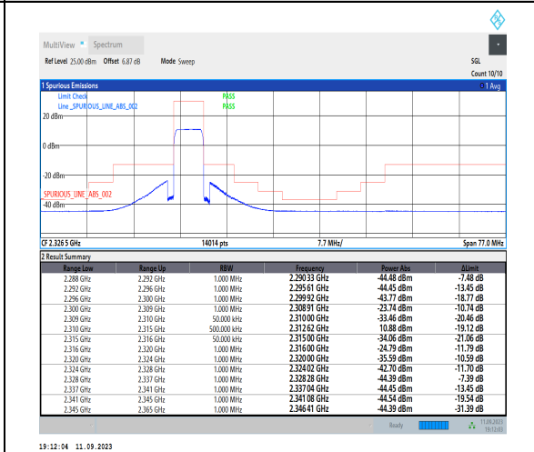
1-N30-PC3-15-5-H-6-CP-QPSK-Outer_Full-25@0-Ant3-1--PASS-see graph
