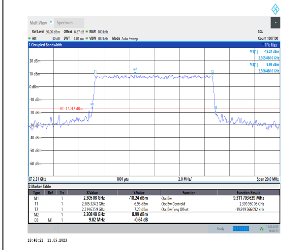
1-N30-PC3-15-10-M-6-CP-QPSK-Outer_Full-52@0- Ant3-9.312-9.820-≤10-PASS
