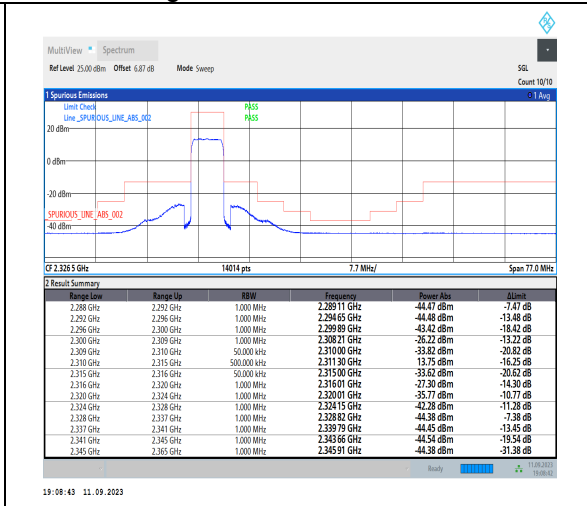
1-N30-PC3-15-5-H-3-DFT-PI2BPSK-Outer_Full-25@0-Ant3-1--PASS-see graph
