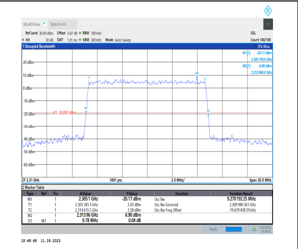
1-N30-PC3-15-10-M-9-CP-256QAM-Outer_Full-52@0 0-Ant3-9.27-9.780-≤10-PASS
