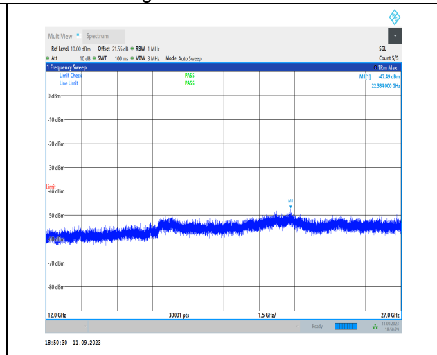
1-N30-PC3-15-10-L-1-DFT-PI2BPSK-Inner_1RB_Left -1@1-12000-27000-Ant3-22334.00--47.49--40-PASS
