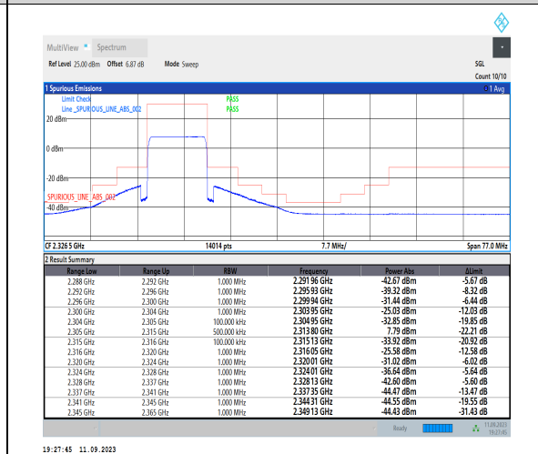
1-N30-PC3-15-10-H-6-CP-QPSK-Outer_Full-52@0-Ant3-1--PASS-see graph
