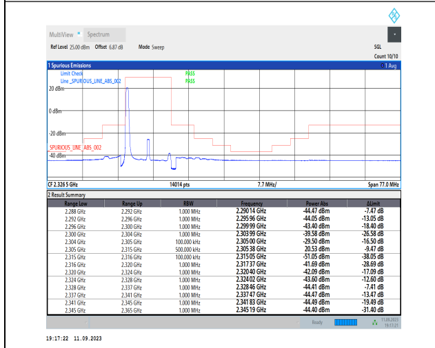
1-N30-PC3-15-10-L-4-CP-QPSK-Edge_1RB_Left-1@0-Ant3-1--PASS-see graph
