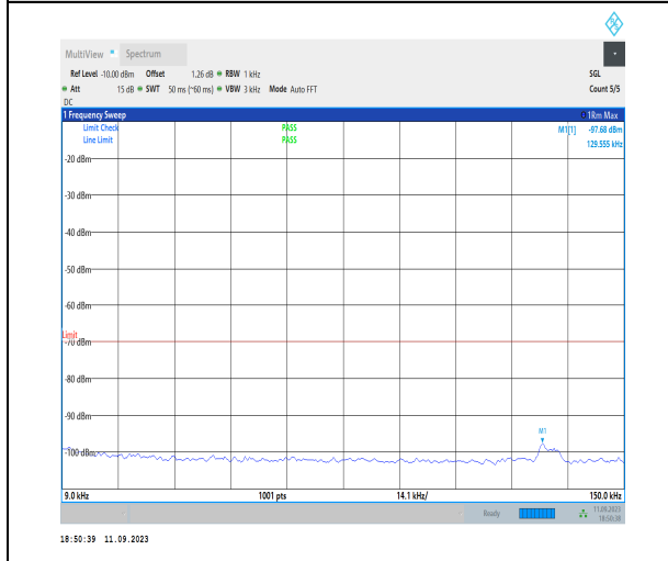
1-N30-PC3-15-10-M-1-DFT-PI2BPSK-Inner_1RB_L eft-1@1-0.009-0.15-Ant3-0.13--97.68--70-PASS
