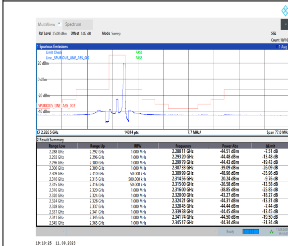
1-N30-PC3-15-5-H-5-CP-QPSK-Edge_1RB_Right-1@24-Ant3-1--PASS-see graph
