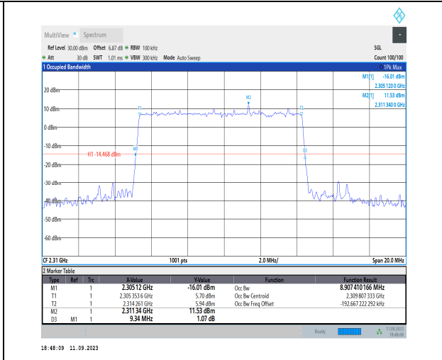
1-N30-PC3-15-10-M-5-DFT-256QAM-Outer_Full-50 @0-Ant3-8.907-9.340-≤10-PASS
