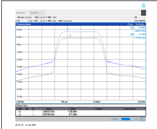
1-N30-PC3-15-10-H-1-DFT-256QAM-Outer_Full-50 @0-Ant3-8.75-100%-0.00-8.75-PASS-≤13
