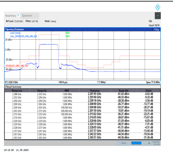
1-N30-PC3-15-10-L-3-DFT-PI2BPSK-Outer_Full-50@0-Ant3-1--PASS-see graph
