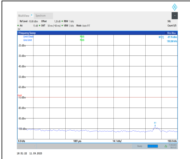
1-N30-PC3-15-10-H-1-DFT-PI2BPSK-Inner_1RB_L eft-1@1-0.009-0.15-Ant3-0.13--97.76--70-PASS
