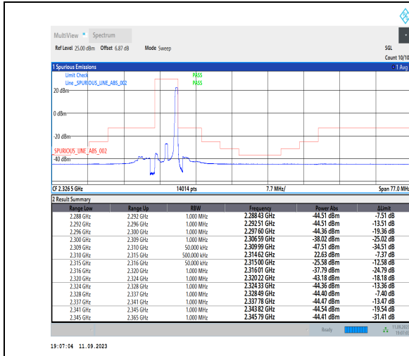
1-N30-PC3-15-5-H-2-DFT-PI2BPSK-Edge_1RB_Right-1@24-Ant3-1--PASS-see graph
