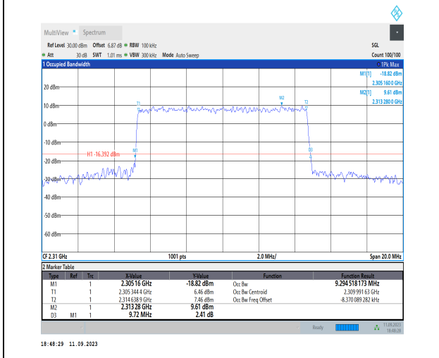
1-N30-PC3-15-10-M-7-CP-16QAM-Outer_Full-52@0 -Ant3-9.295-9.720-≤10-PASS
