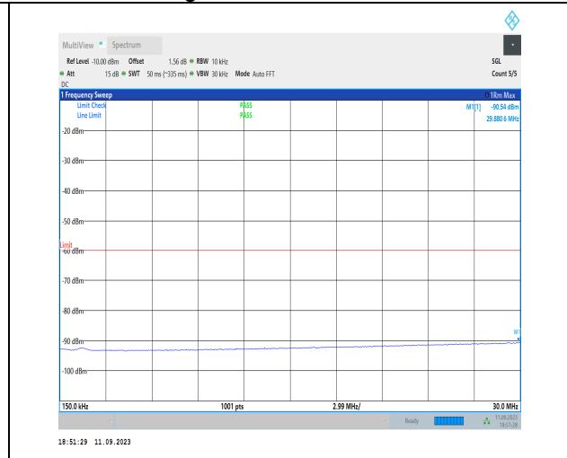
1-N30-PC3-15-10-H-1-DFT-PI2BPSK-Inner_1RB_Lef t-1@1-0.15-30-Ant3-29.88--90.54--60-PASS
