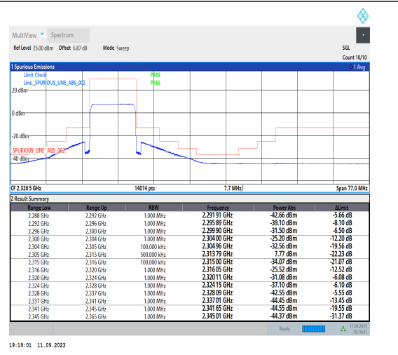
1-N30-PC3-15-10-L-6-CP-QPSK-Outer_Full-52@0-Ant3-1--PASS-see graph
