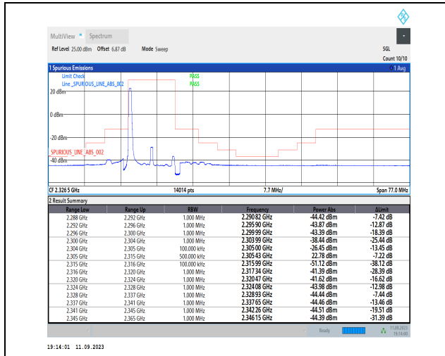
1-N30-PC3-15-10-L-1-DFT-PI2BPSK-Edge_1RB_Left-1@0-Ant3-1--PASS-see graph
