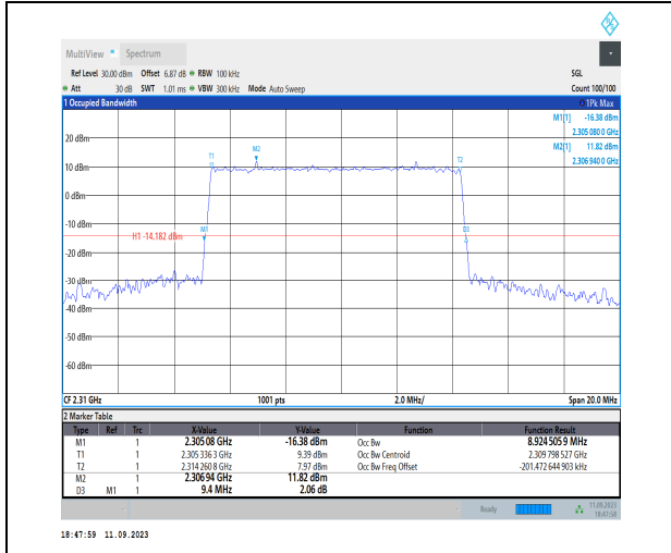
1-N30-PC3-15-10-M-4-DFT-64QAM-Outer_Full-50@ 0-Ant3-8.925-9.400-≤10-PASS
