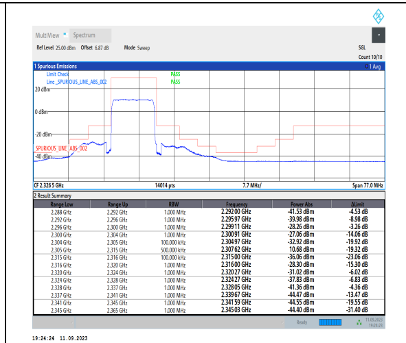
1-N30-PC3-15-10-H-3-DFT-PI2BPSK-Outer_Full-50@0-Ant3-1--PASS-see graph
