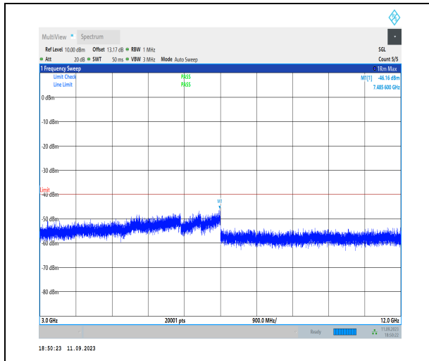
1-N30-PC3-15-10-L-1-DFT-PI2BPSK-Inner_1RB_Lef ft-1@1-3000-12000-Ant3-7485.60--46.16--40-PASS
