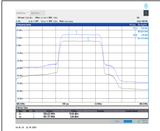
1-N26-824-849-PC3-15-20-H-1-DFT-256QAM-Outer_Full-100@0-Ant1-9.00-100%-0.00-9.00-PASS-<=13
