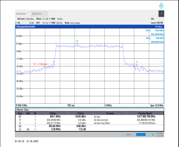
1-N26-824-849-PC3-15-5-M-8-CP-64QAM-Outer_Fu ll-25@0-Ant1-4.478-5.580-≤5-PASS
