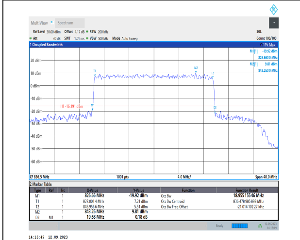
1-N26-824-849-PC3-15-20-M-8-CP-64QAM-Outer_Full-106@0-Ant1-18.955-19.680-≤20-PASS
