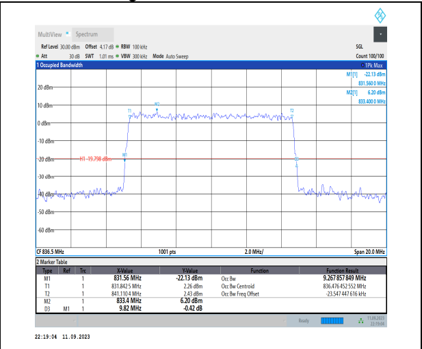
1-N26-824-849-PC3-15-10-M-9-CP-256QAM-Outer_Full-52@0-Ant1-9.268-9.820-≤10-PASS
