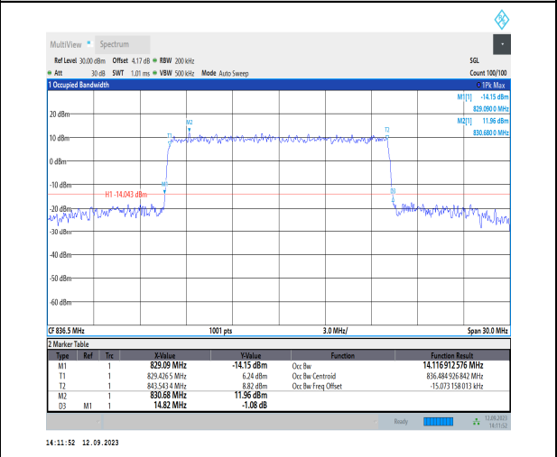
1-N26-824-849-PC3-15-15-M-6-CP-QPSK-Outer_Fu II-79@0-Ant1-14.117-14.820-≤15-PASS
