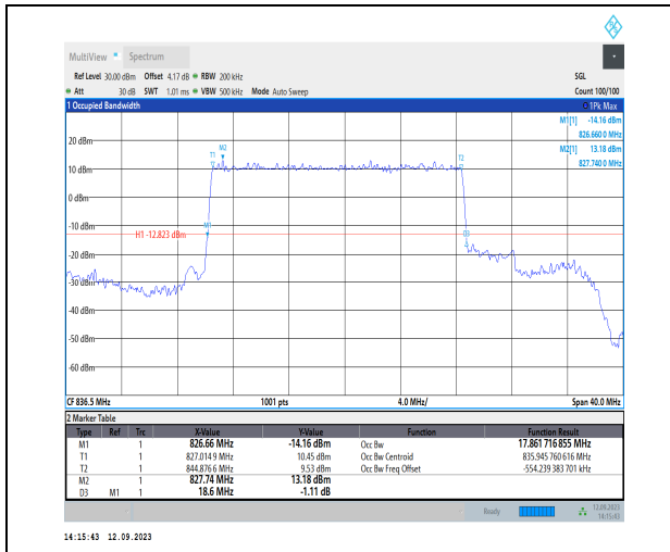
1-N26-824-849-PC3-15-20-M-2-DFT-PI2BPSK-Outer_Full-100@0-Ant1-17.862-18.600-≤20-PASS
