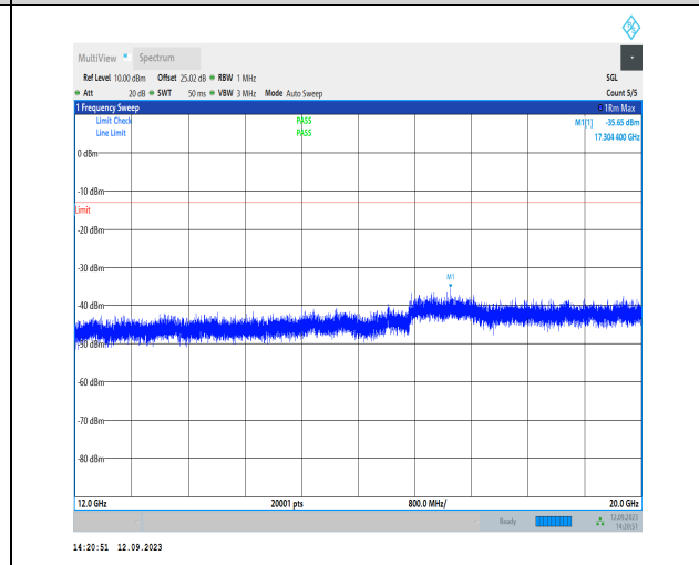
1-N26-824-849-PC3-15-20-M-1-DFT-PI2BPSK-Inner_1RB_Left-1@1-12000-20000-Ant1-17304.40--35.65- 13-PASS
