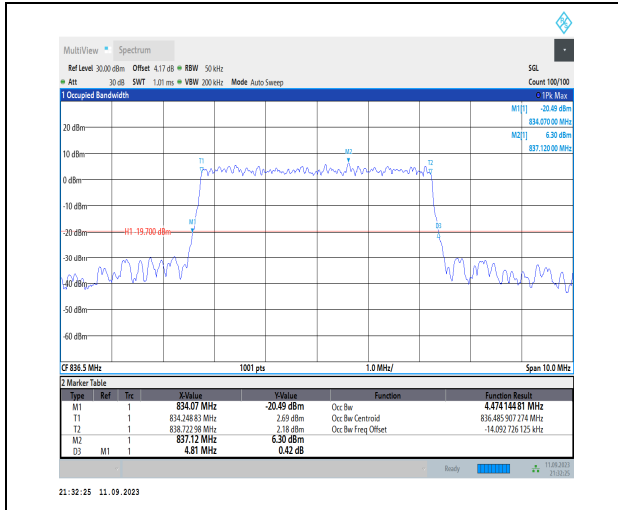
1-N26-824-849-PC3-15-5-M-9-CP-256QAM-Outer_F ull-25@0-Ant1-4.474-4.810- \leq 5-PASS
