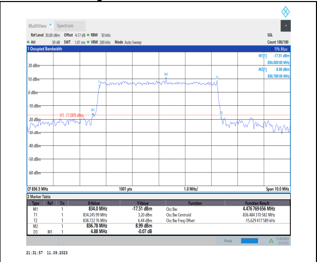
1-N26-824-849-PC3-15-5-M-6-CP-QPSK-Outer_Full-25@0-Ant1-4.477-4.880-≤5-PASS
