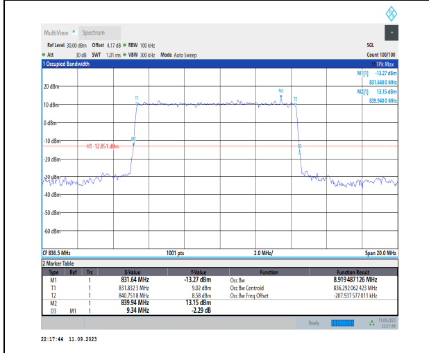
1-N26-824-849-PC3-15-10-M-2-DFT-PI2BPSK-Outer_F ull-50@0-Ant1-8.919-9.340- \leq 10-PASS
