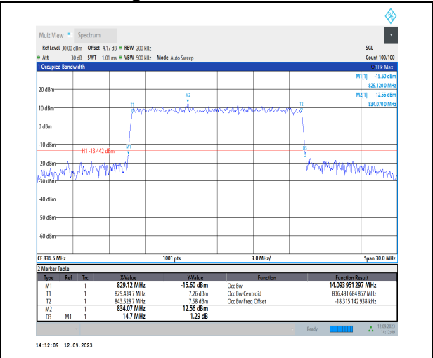
1-N26-824-849-PC3-15-15-M-8-CP-64QAM-Outer_Full-79@0-Ant1-14.094-14.700-≤15-PASS
