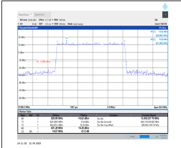
1-N26-824-849-PC3-15-15-M-3-DFT-16QAM-Outer_Full-75@0-Ant1-13.45-14.070-≤15-PASS
