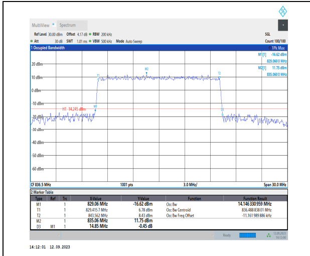
1-N26-824-849-PC3-15-15-M-7-CP-16QAM-Outer_Full-79@0-Ant1-14.146-14.850-≤15-PASS
