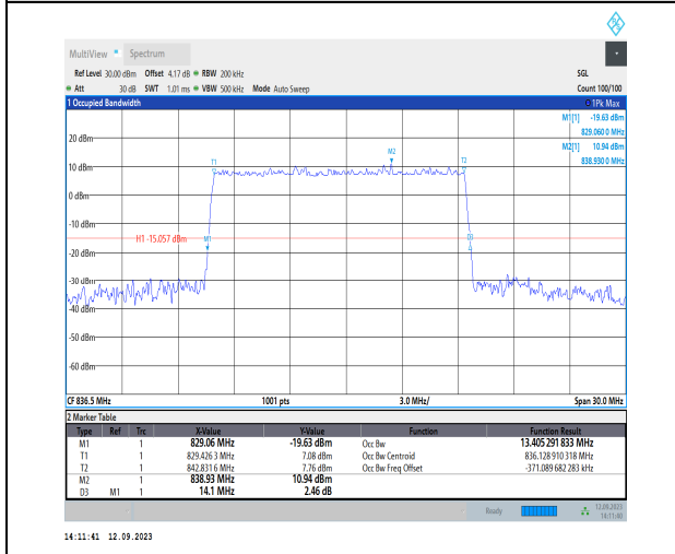
1-N26-824-849-PC3-15-15-M-5-DFT-256QAM-Outer_Full-75@0-Ant1-13.405-14.100-≤15-PASS
