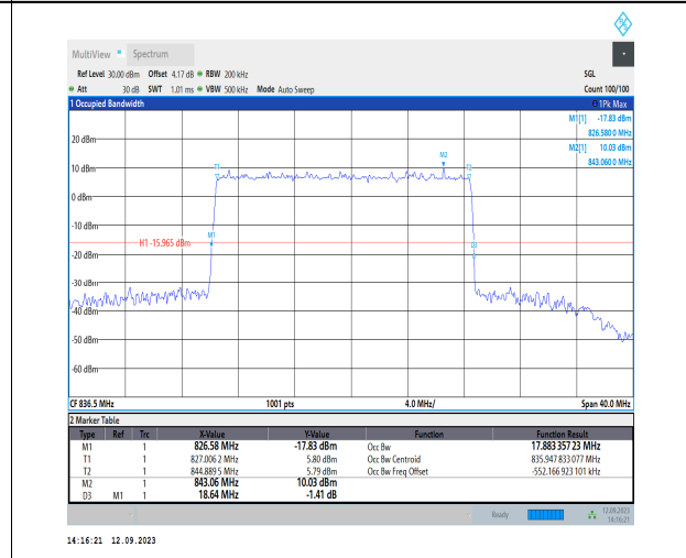
1-N26-824-849-PC3-15-20-M-5-DFT-256QAM-Outer_Full-100@0-Ant1-17.883-18.640-≤20-PASS
