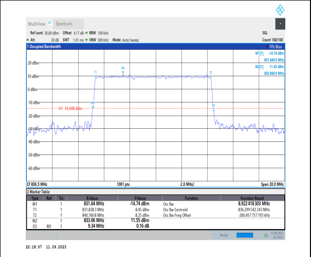
1-N26-824-849-PC3-15-10-M-3-DFT-16QAM-Outer_F ull-50@0-Ant1-8.922-9.340- \leq 10-PASS
