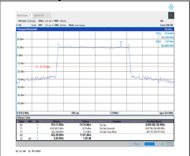
1-N26-814-824-PC3-15-10-M-1-DFT-QPSK-Outer_F ull-50@0-Ant1-8.903-9.360-<math>\leq</math>10-PASS
