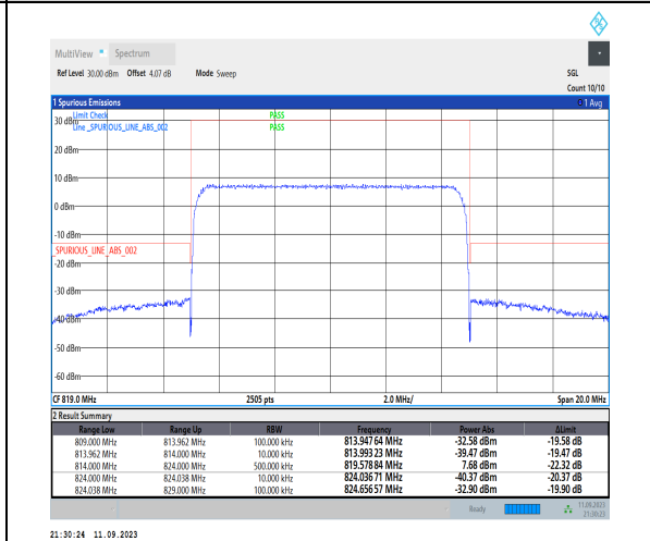
1-N26-814-824-PC3-15-10-H-6-CP-QPSK-Outer Full-52@0-Ant1-1--PASS-see graph
