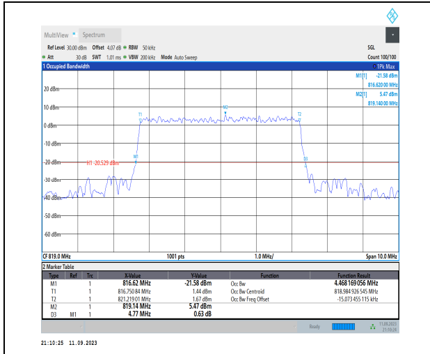
1-N26-814-824-PC3-15-5-M-9-CP-256QAM-Outer_F ull-25@0-Ant1-4.468-4.770-<math>\leq</math>5-PASS
