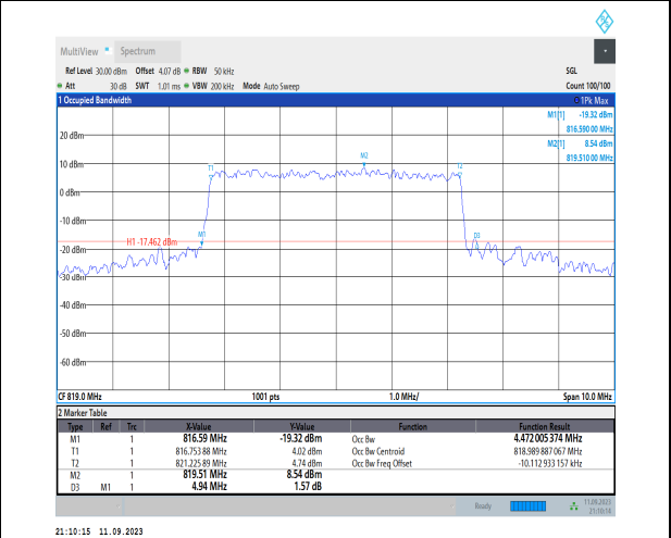
1-N26-814-824-PC3-15-5-M-8-CP-64QAM-Outer_Fu ll-25@0-Ant1-4.472-4.940-<math>\leq</math>5-PASS
