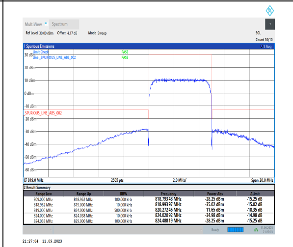
1-N26-814-824-PC3-15-5-H-6-CP-QPSK-Outer_Full-25@0-Ant1-1--PASS-see graph
