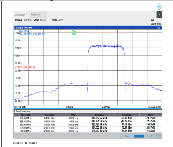
1-N26-814-824-PC3-15-5-H-3-DFT-PI2BPSK-Outer_Full-25@0-Ant1-1--PASS-see graph
