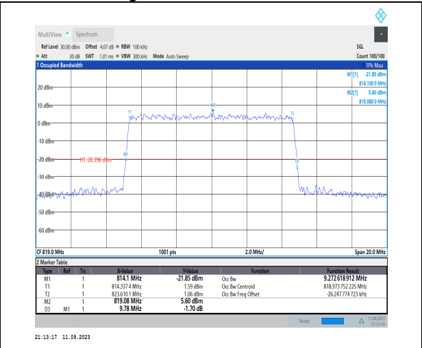
1-N26-814-824-PC3-15-10-M-9-CP-256QAM-Outer_Full-52@0-Ant1-9.273-9.780-≤10-PASS
