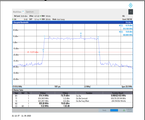
1-N26-814-824-PC3-15-10-M-5-DFT-256QAM-Outer_Full-50@0-Ant1-8.909-9.320-≤10-PASS
