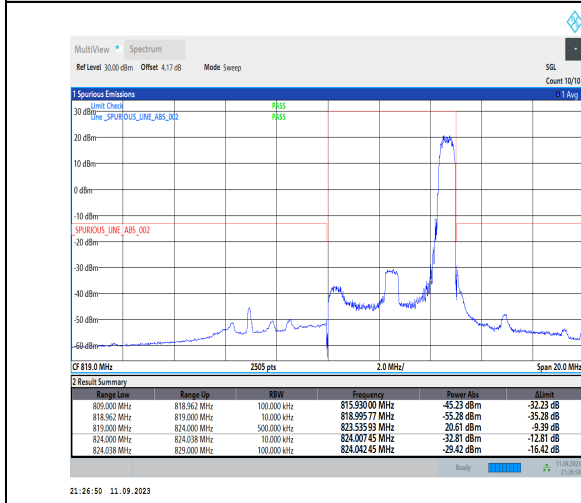
1-N26-814-824-PC3-15-5-H-5-CP-QPSK-Edge_1RB_Right-1@24-Ant1-1--PASS-see graph
