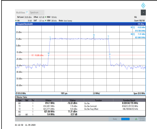
1-N26-814-824-PC3-15-10-M-2-DFT-PI2BPSK-Outer_F ull-50@0-Ant1-8.928-9.400-<math>\leq</math>10-PASS
