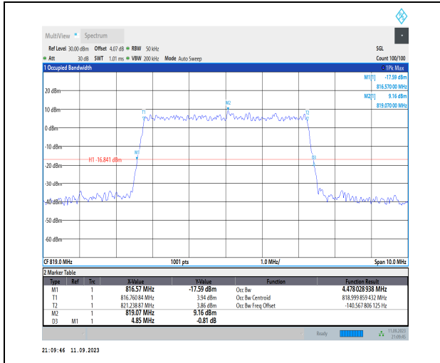
1-N26-814-824-PC3-15-5-M-5-DFT-25QAM-Outer_Full-25@0-Ant1-4.478-4.850-<math>\leq</math>5-PASS
