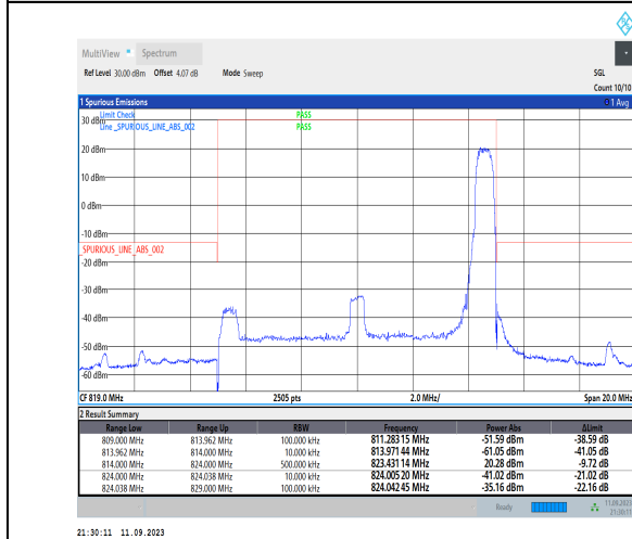
1-N26-814-824-PC3-15-10-H-5-CP-QPSK-Edge_1RB_Right-1@51-Ant1-1--PASS-see graph
