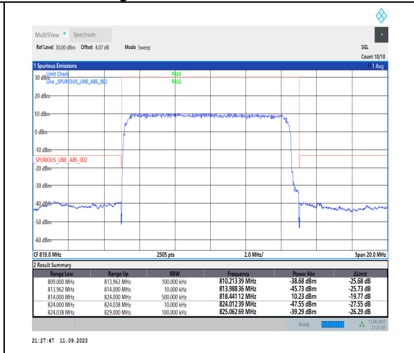
1-N26-814-824-PC3-15-10-L-3-DFT-PI2BPSK-Out_er_Full-50@0-Ant1-1--PASS-see graph
