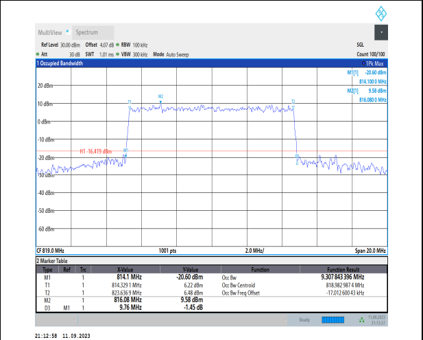
1-N26-814-824-PC3-15-10-M-7-CP-16QAM-Outer_Full-52@0-Ant1-9.308-9.760-≤10-PASS
