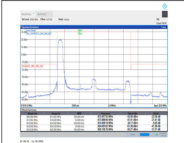
1-N26-814-824-PC3-15-10-L-4-CP-QPSK-Edge_1RB_Left-1@0-Ant1-1--PASS-see graph
