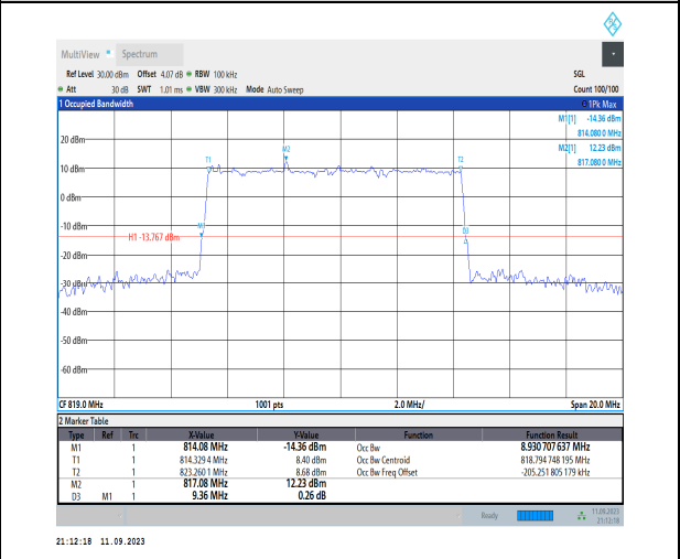
1-N26-814-824-PC3-15-10-M-3-DFT-16QAM-Outer_F ull-50@0-Ant1-8.931-9.360-<math>\leq</math>10-PASS
