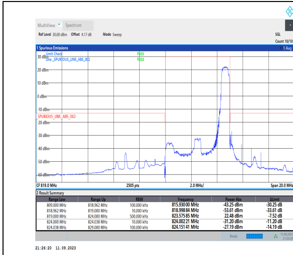
1-N26-814-824-PC3-15-5-H-2-DFT-PI2BPSK-Edge_1 RB_Right-1@24-Ant1-1--PASS-see graph
