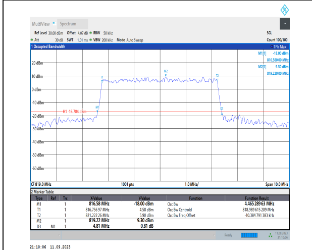
1-N26-814-824-PC3-15-5-M-7-CP-16QAM-Outer_Fu ll-25@0-Ant1-4.465-4.810-<math>\leq</math>5-PASS
