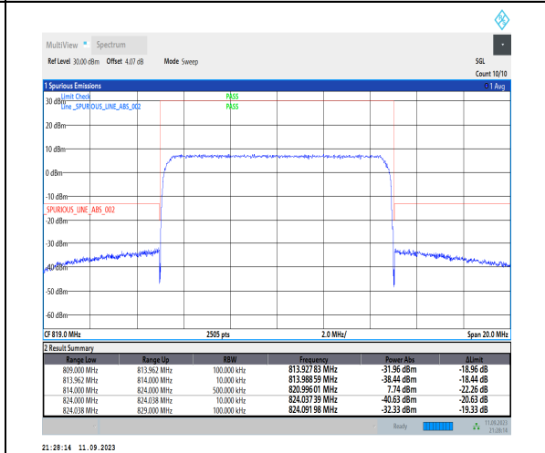
1-N26-814-824-PC3-15-10-L-6-CP-QPSK-Outer_Full-52@0-Ant1-1--PASS-see graph
