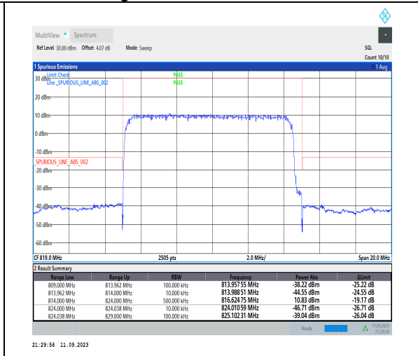
1-N26-814-824-PC3-15-10-H-3-DFT-PI2BPSK-Out er_Full-50@0-Ant1-1--PASS-see graph
